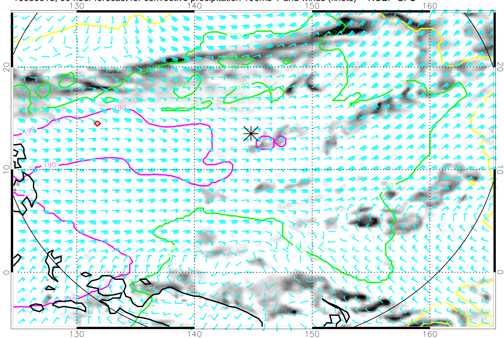
16083018, 90 hour forecast for convective precipitation 100mb T and winds (knots) -- NCEP GFS
