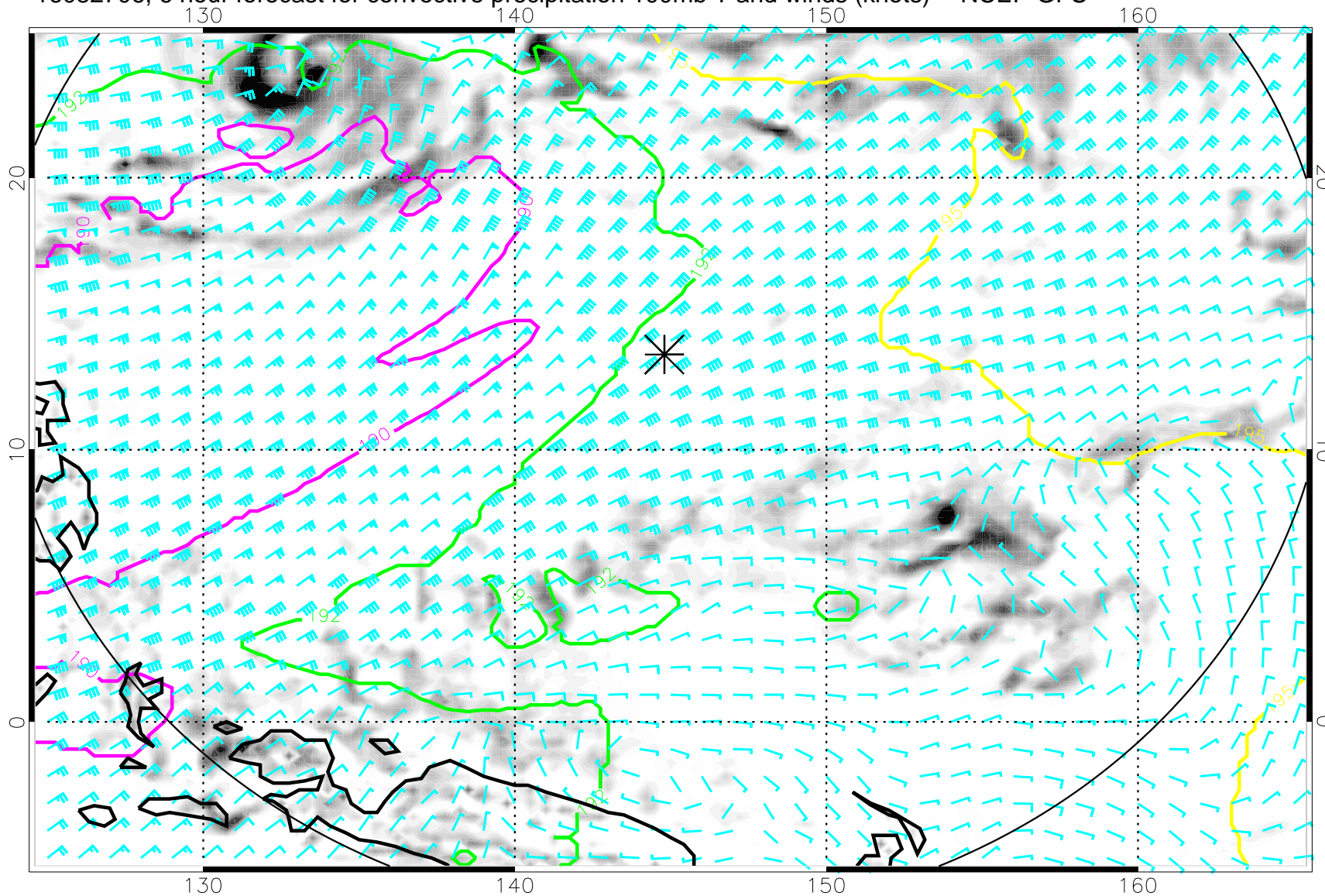
16082706, 6 hour forecast for convective precipitation 100mb T and winds (knots) -- NCEP GFS
