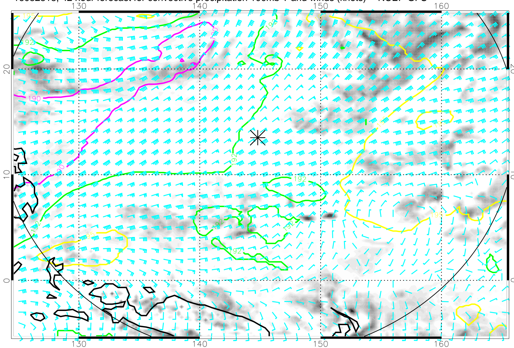
16082818, 42 hour forecast for convective precipitation 100mb T and winds (knots) -- NCEP GFS
