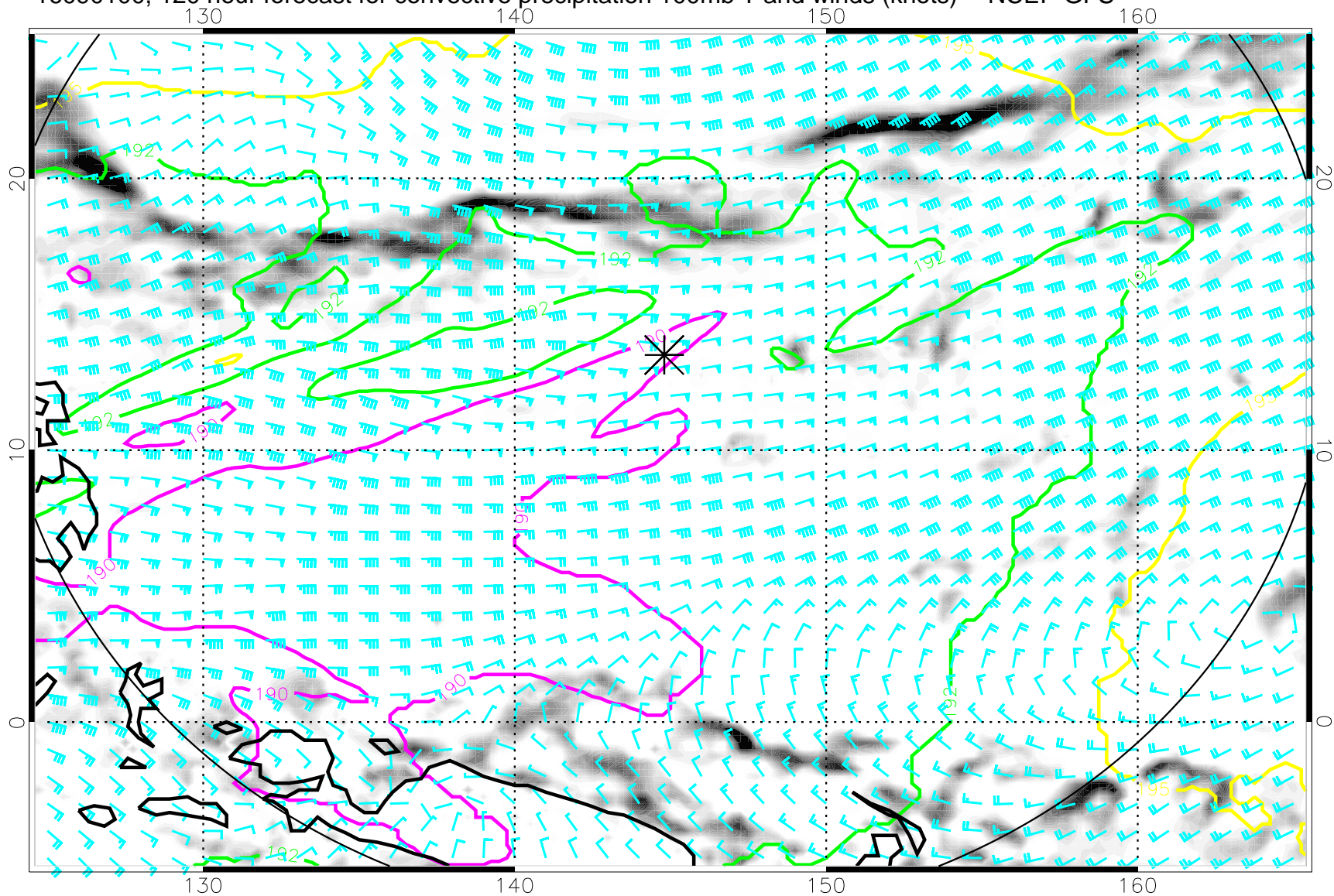
16090100, 120 hour forecast for convective precipitation 100mb T and winds (knots) -- NCEP GFS
