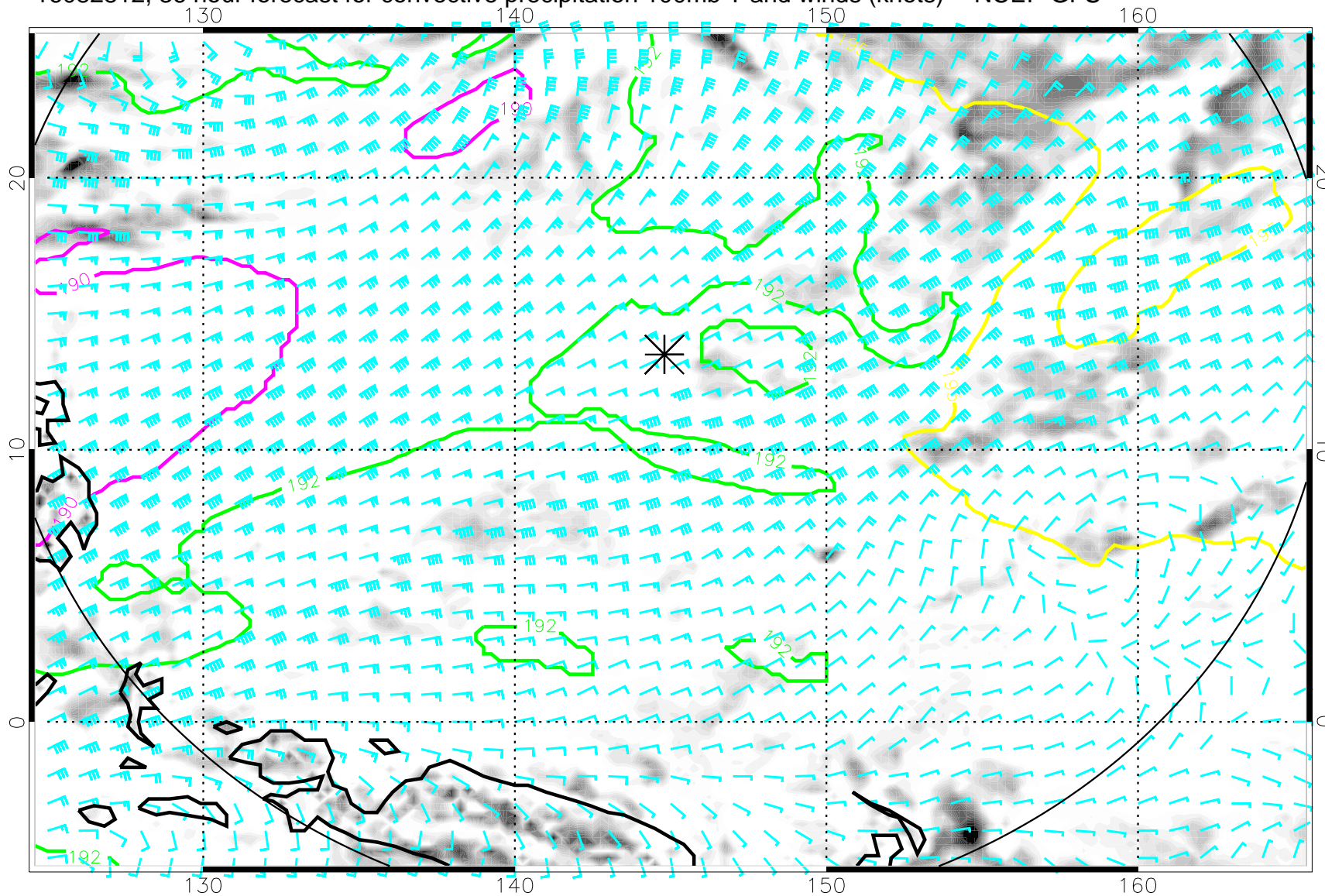
16082812, 36 hour forecast for convective precipitation 100mb T and winds (knots) -- NCEP GFS
