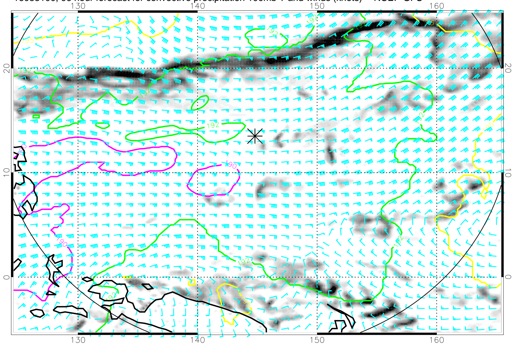
16083100, 96 hour forecast for convective precipitation 100mb T and winds (knots) -- NCEP GFS
