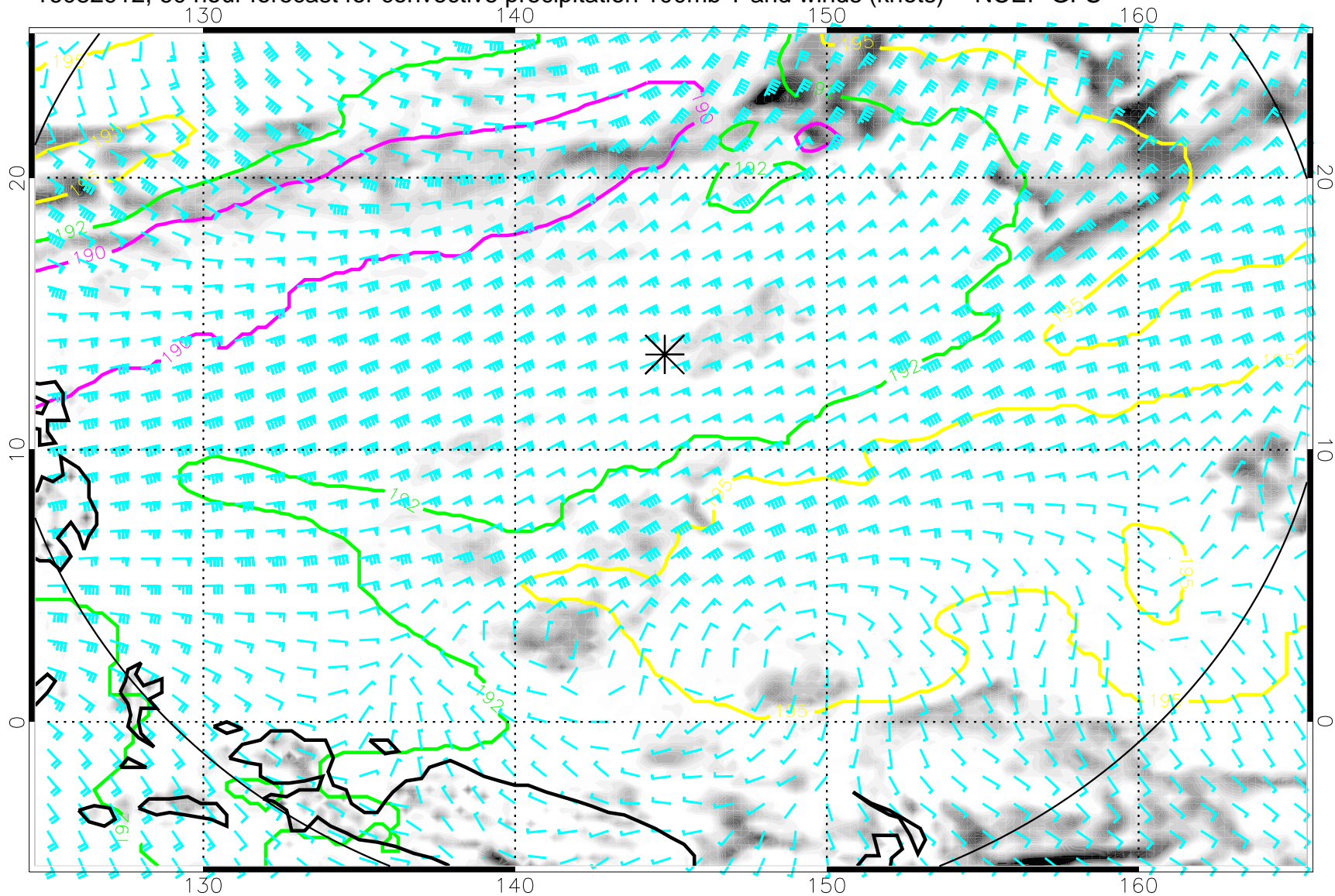
16082912, 60 hour forecast for convective precipitation 100mb T and winds (knots) -- NCEP GFS
