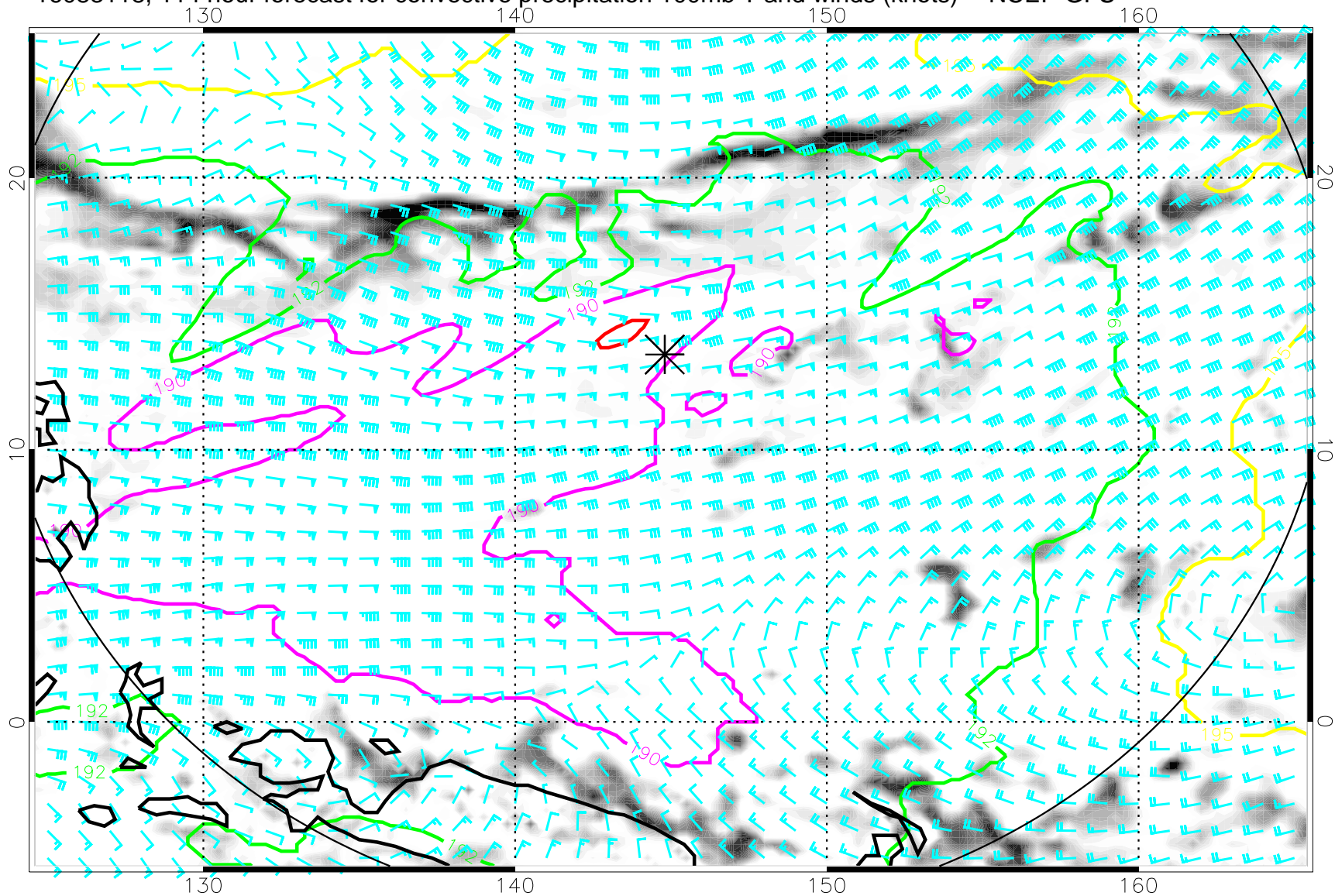
16083118, 114 hour forecast for convective precipitation 100mb T and winds (knots) -- NCEP GFS
