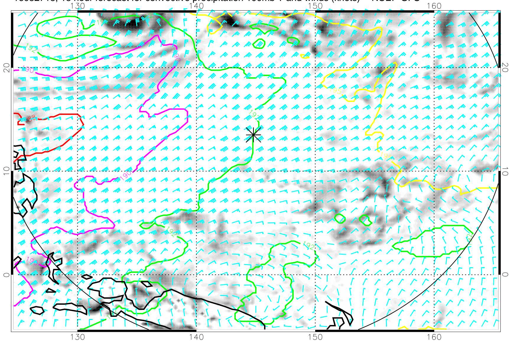
16082718, 18 hour forecast for convective precipitation 100mb T and winds (knots) -- NCEP GFS
