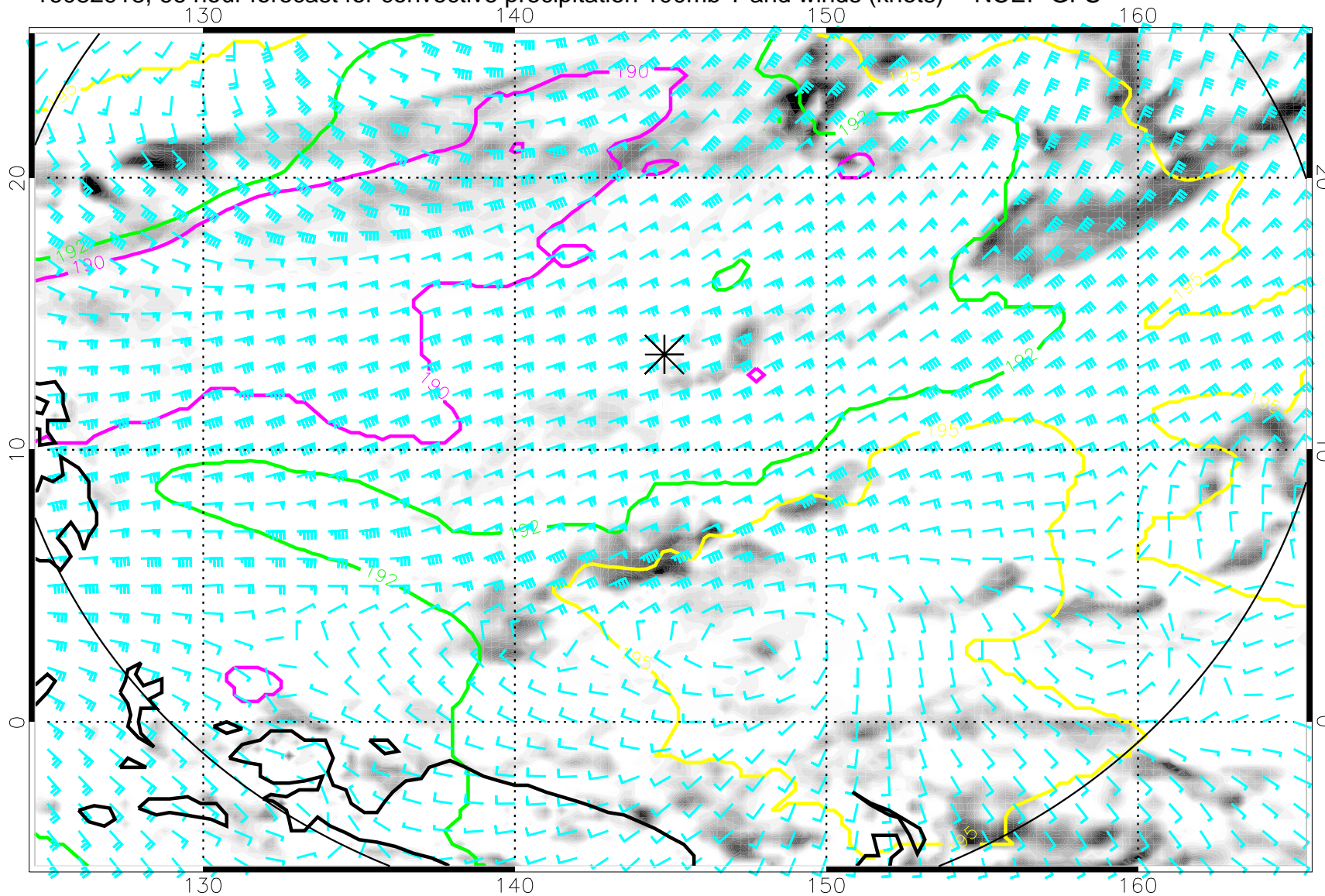
16082918, 66 hour forecast for convective precipitation 100mb T and winds (knots) -- NCEP GFS
