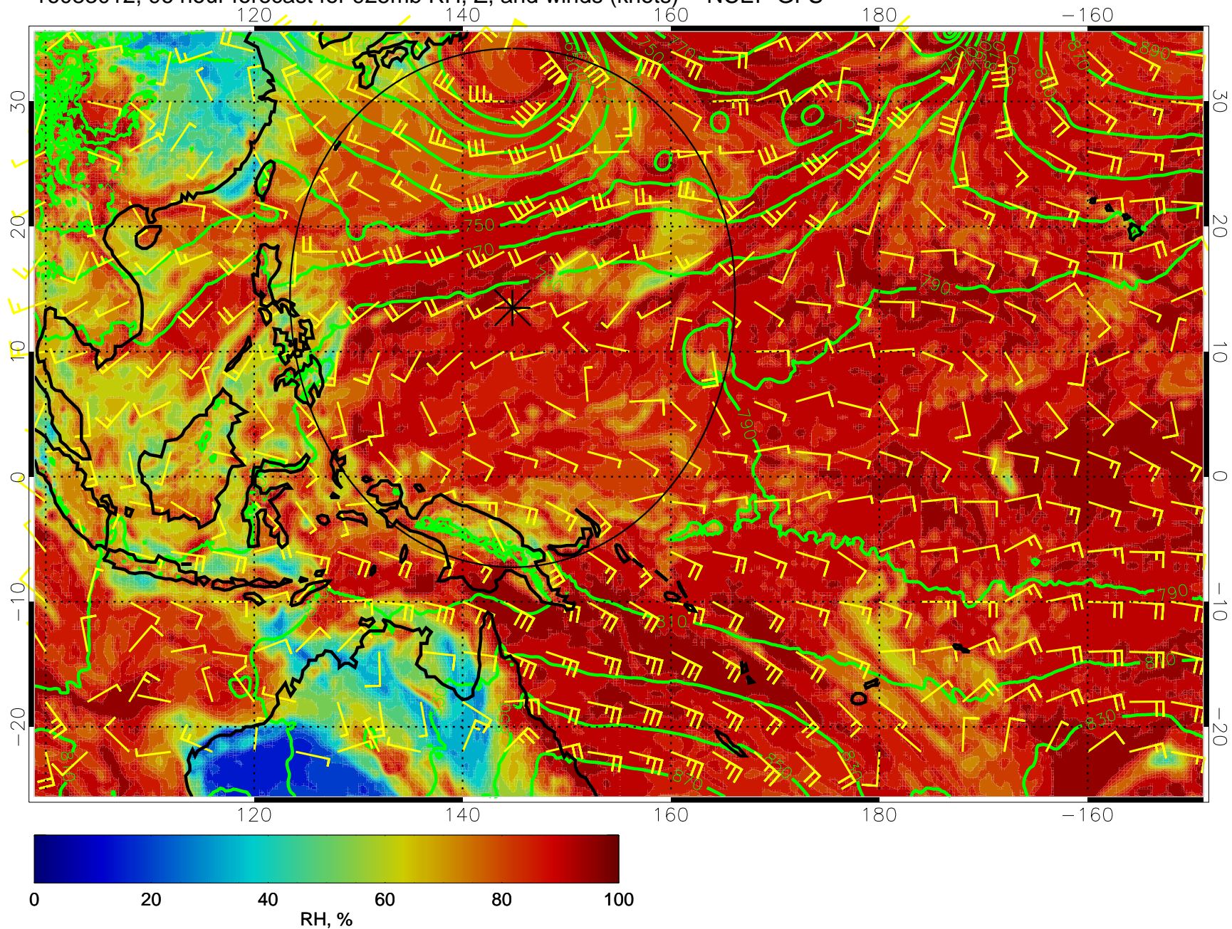
16083012, 96 hour forecast for 925mb RH, Z, and winds (knots) -- NCEP GFS
