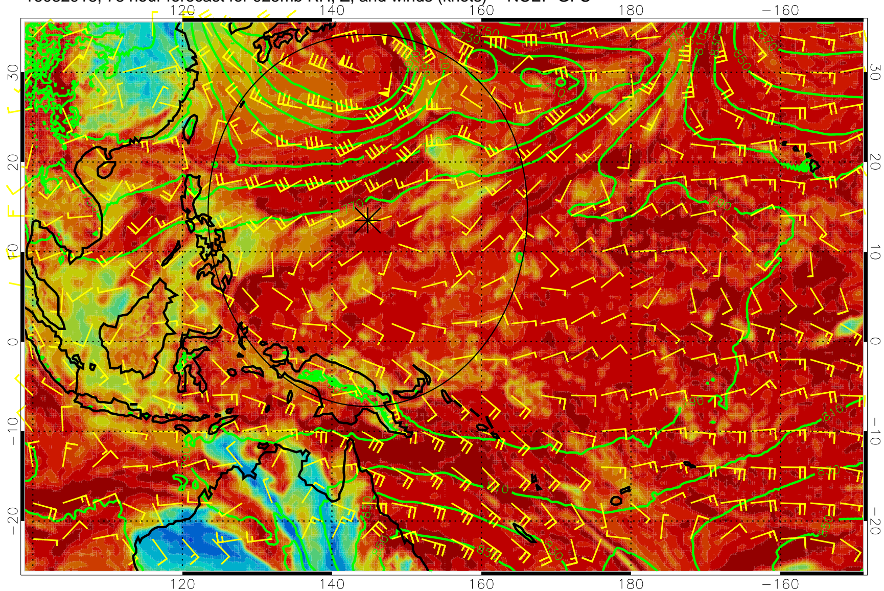
16082918, 78 hour forecast for 925mb RH, Z, and winds (knots) -- NCEP GFS
