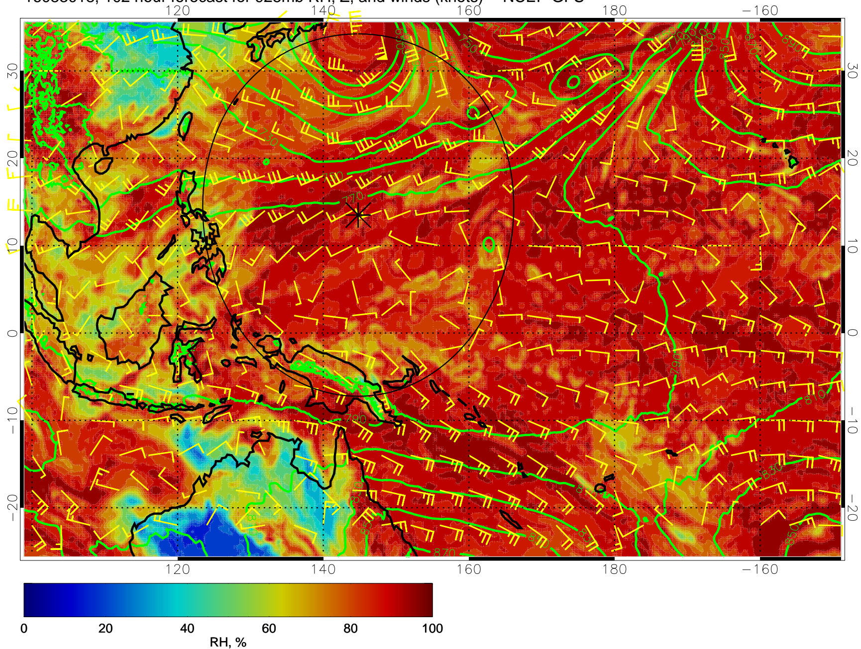
16083018, 102 hour forecast for 925mb RH, Z, and winds (knots) -- NCEP GFS
