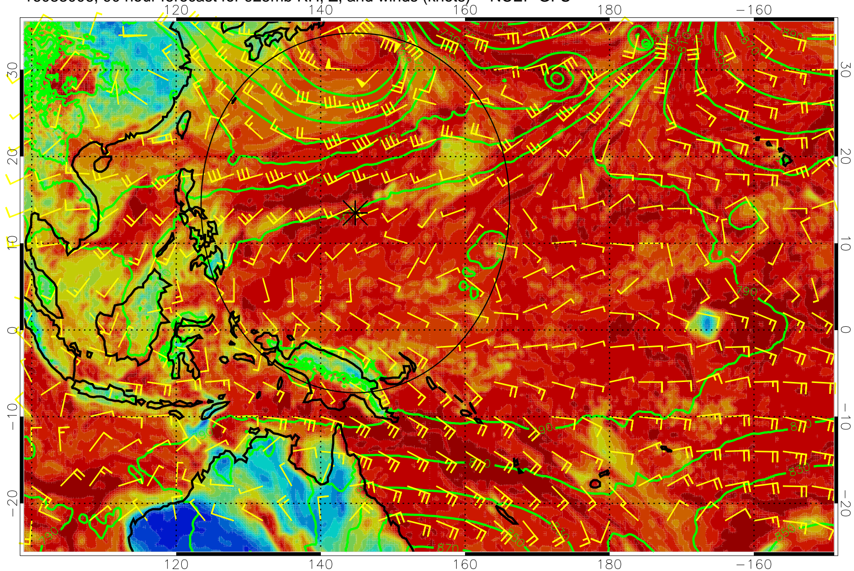
16083006, 90 hour forecast for 925mb RH, Z, and winds (knots) -- NCEP GFS
