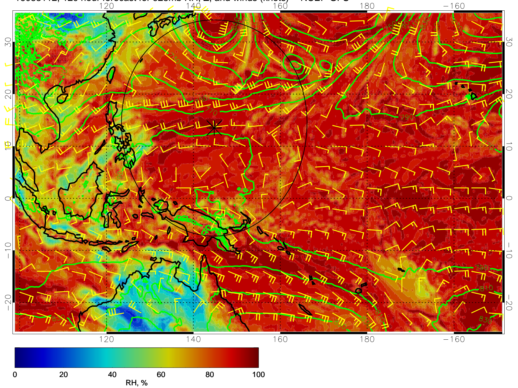
16083112, 120 hour forecast for 925mb RH, Z, and winds (knots) -- NCEP GFS
