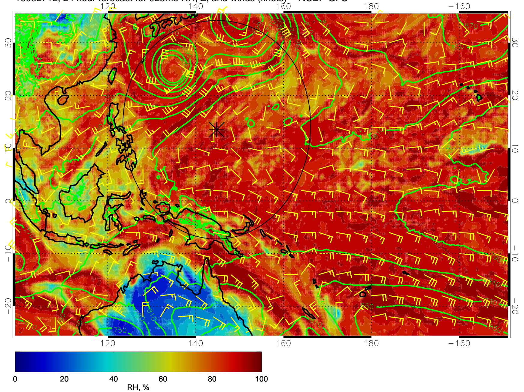
16082712, 24 hour forecast for 925mb RH, Z, and winds (knots) -- NCEP GFS
