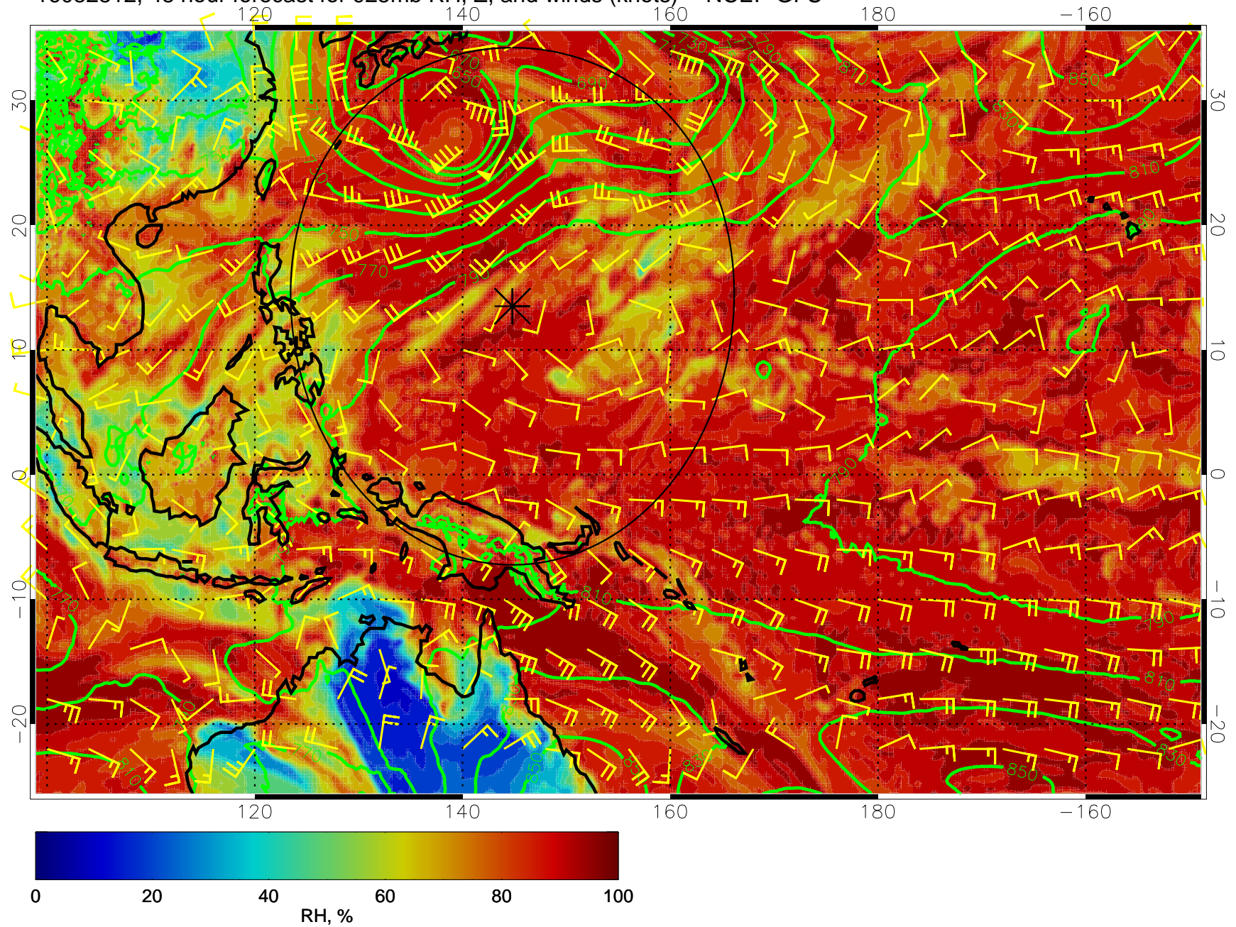
16082812, 48 hour forecast for 925mb RH, Z, and winds (knots) -- NCEP GFS
