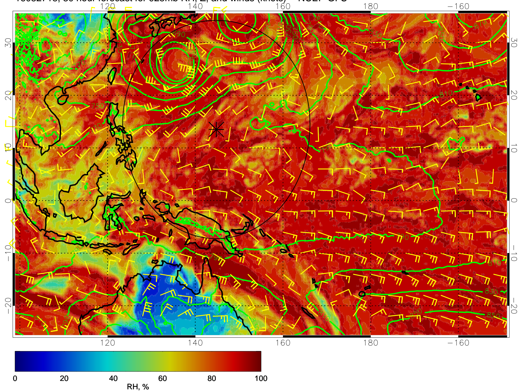
16082718, 30 hour forecast for 925mb RH, Z, and winds (knots) -- NCEP GFS
