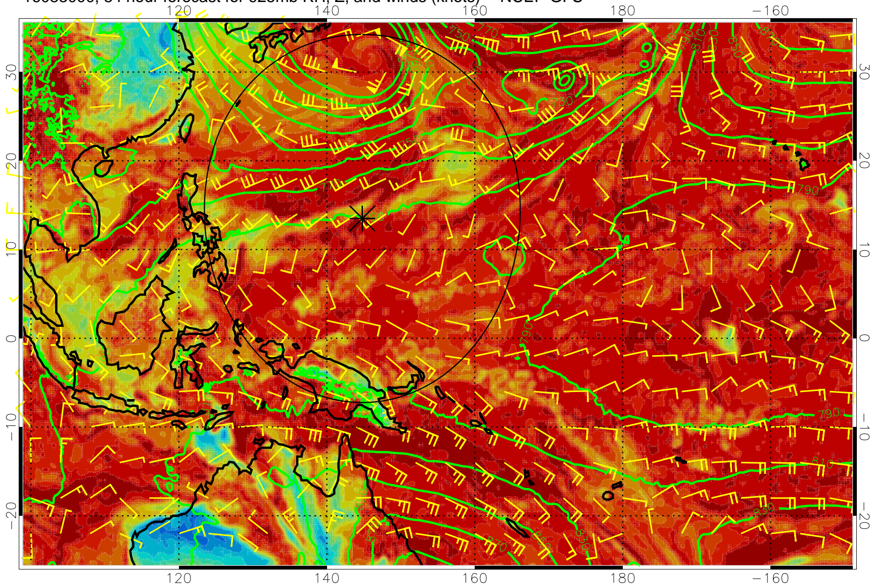
16083000, 84 hour forecast for 925mb RH, Z, and winds (knots) -- NCEP GFS
