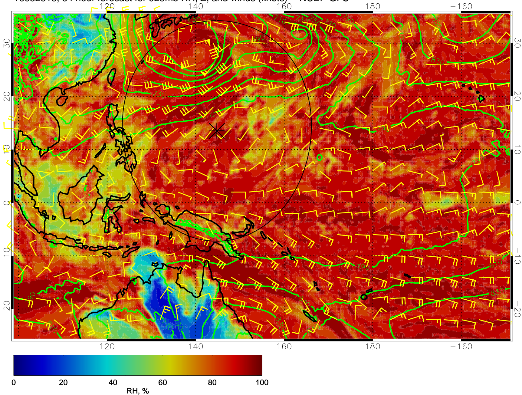
16082818, 54 hour forecast for 925mb RH, Z, and winds (knots) -- NCEP GFS
