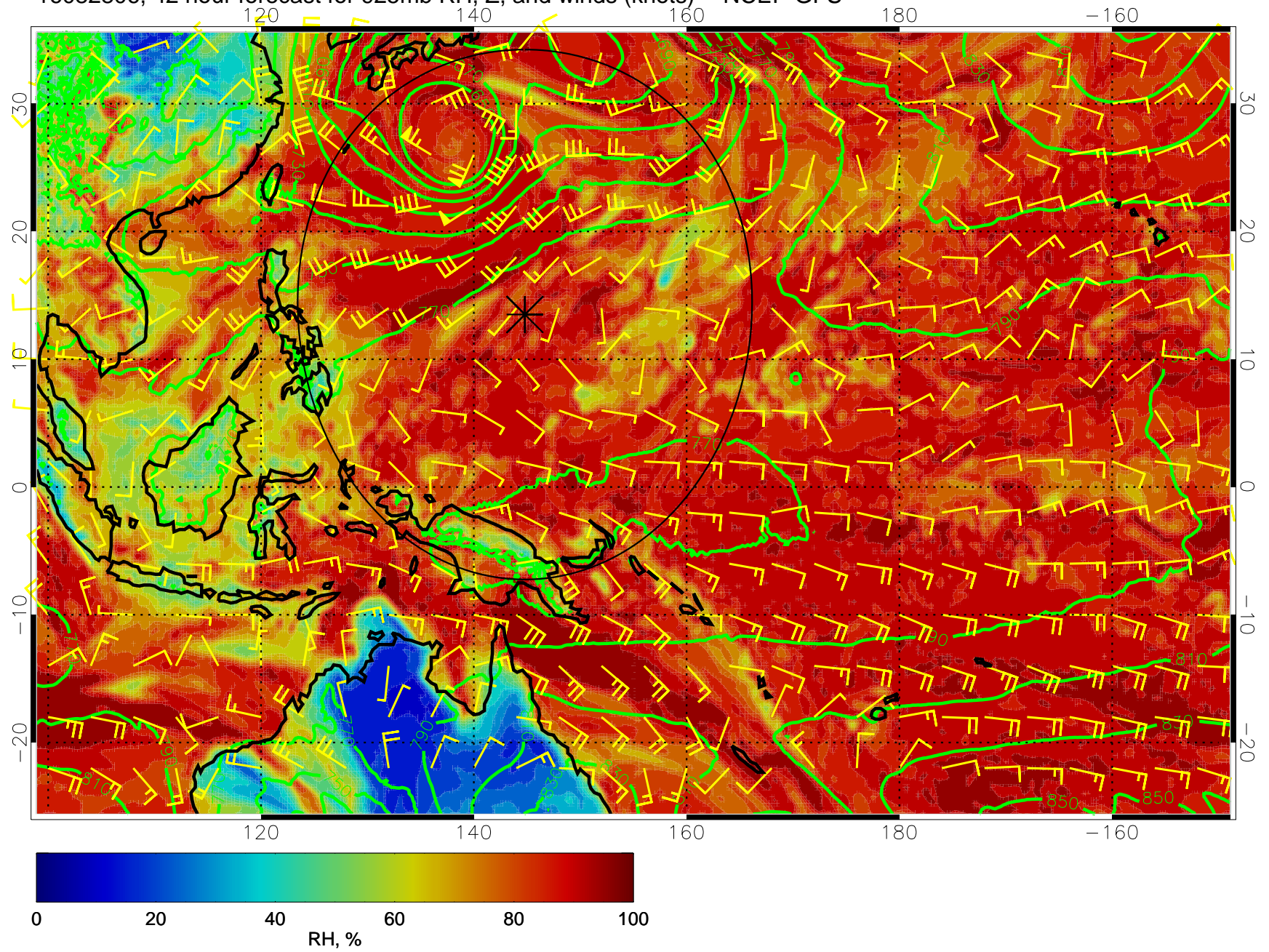
16082806, 42 hour forecast for 925mb RH, Z, and winds (knots) -- NCEP GFS
