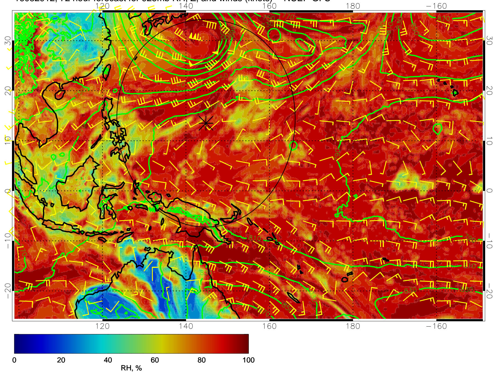
16082912, 72 hour forecast for 925mb RH, Z, and winds (knots) -- NCEP GFS
