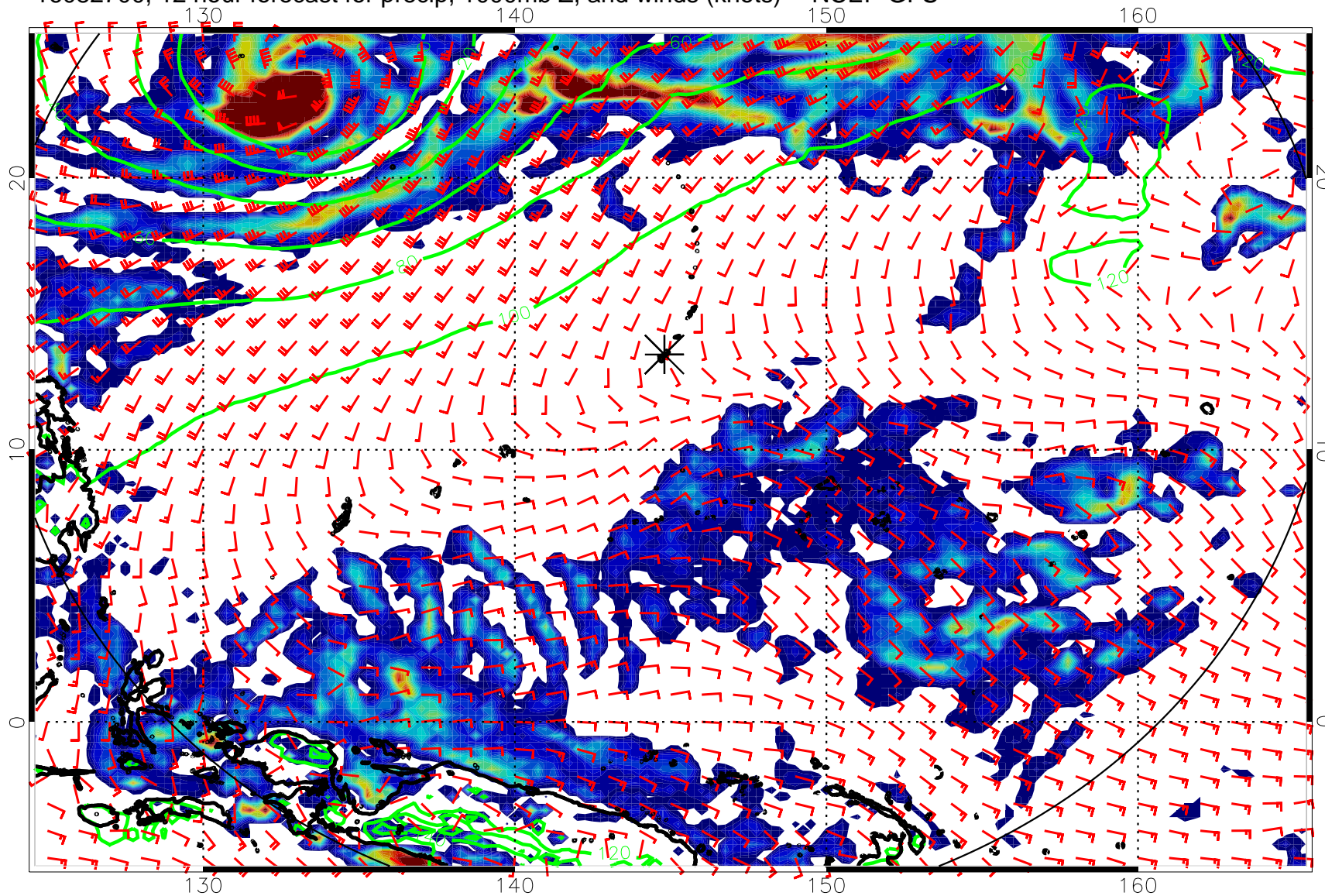
16082700, 12 hour forecast for precip, 1000mb Z, and winds (knots) -- NCEP GFS
