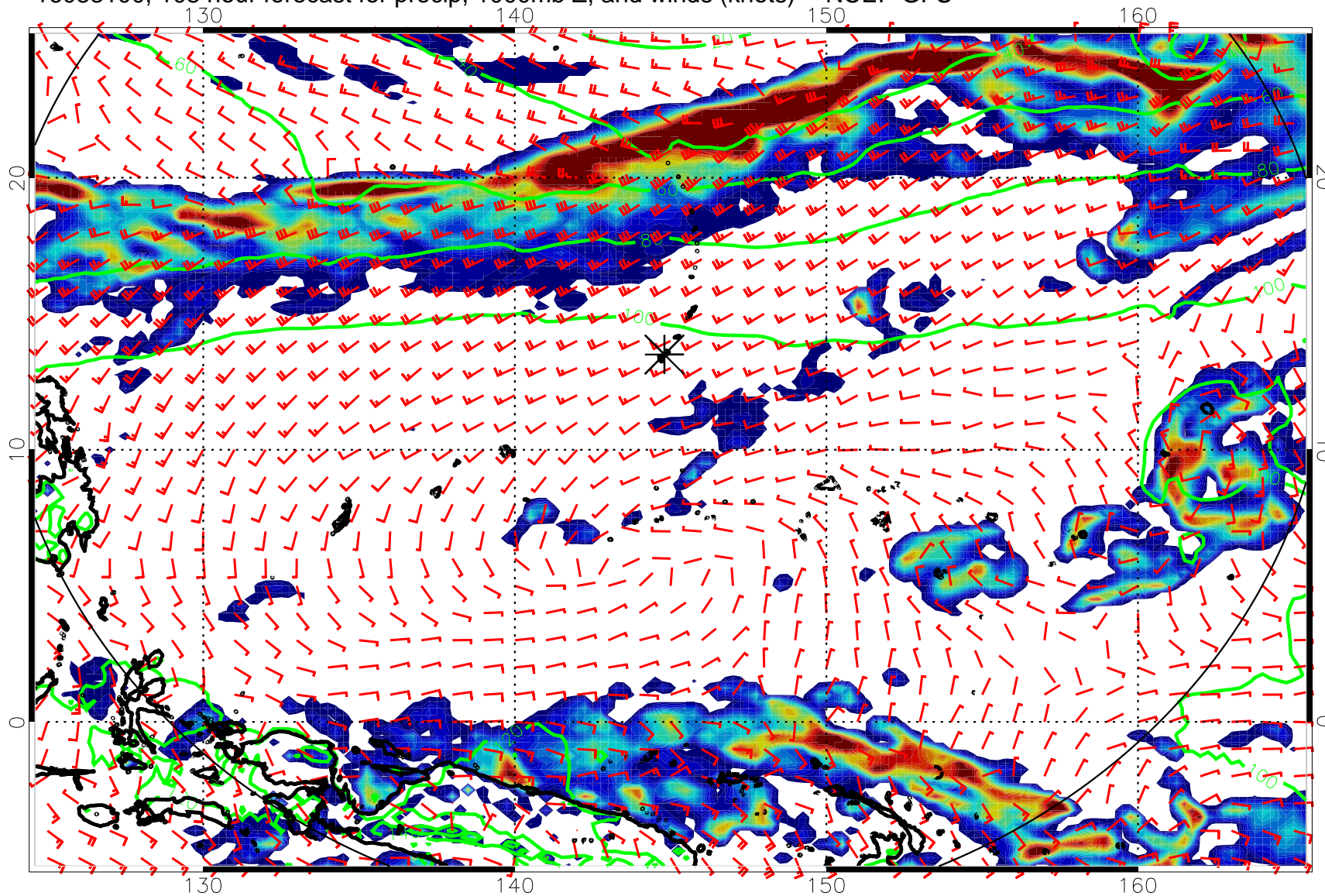
16083100, 108 hour forecast for precip, 1000mb Z, and winds (knots) -- NCEP GFS
