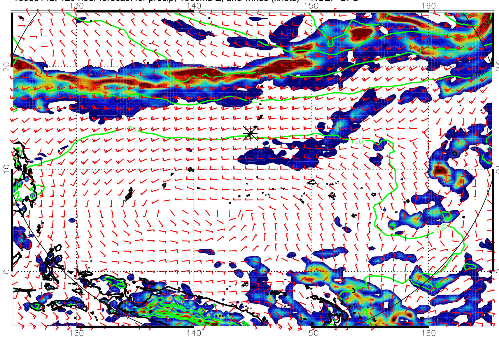
16083112, 120 hour forecast for precip, 1000mb Z, and winds (knots) -- NCEP GFS
