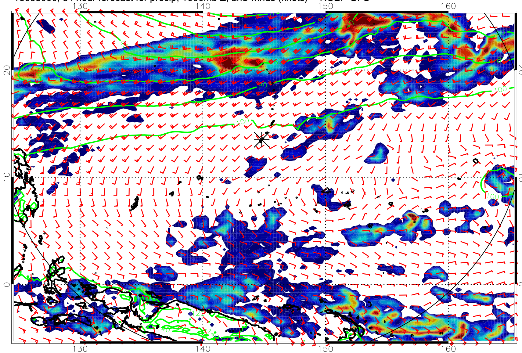
16083000, 84 hour forecast for precip, 1000mb Z, and winds (knots) -- NCEP GFS
