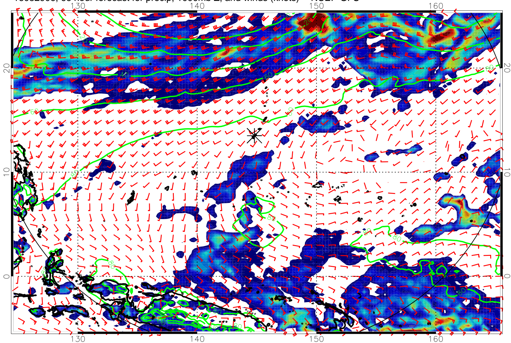
16082906, 66 hour forecast for precip, 1000mb Z, and winds (knots) -- NCEP GFS
