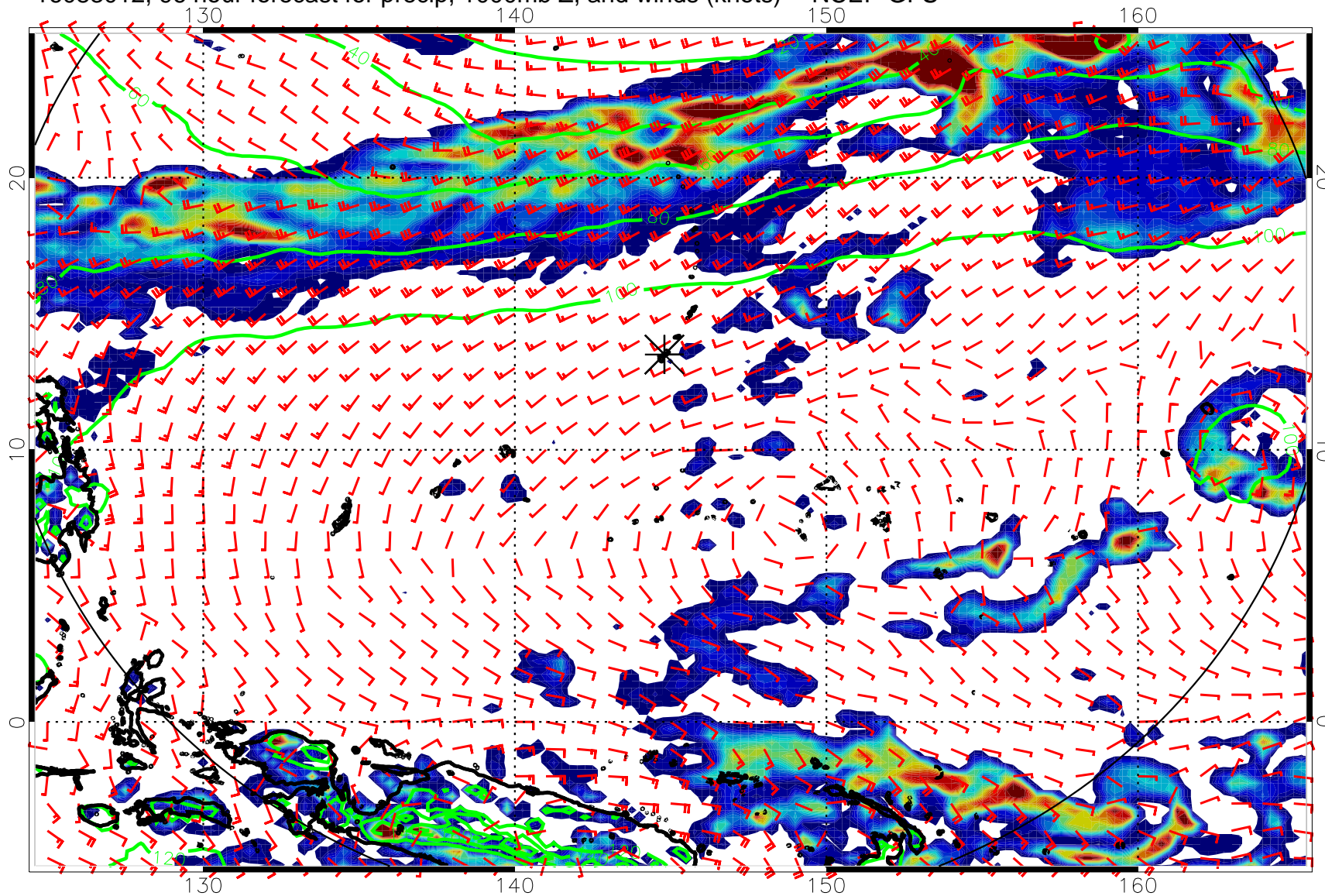
16083012, 96 hour forecast for precip, 1000mb Z, and winds (knots) -- NCEP GFS
