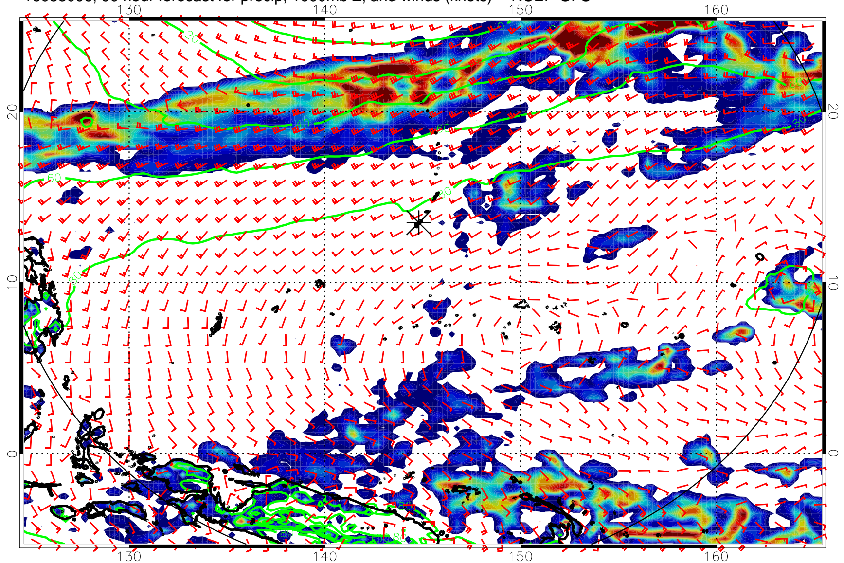
16083006, 90 hour forecast for precip, 1000mb Z, and winds (knots) -- NCEP GFS
