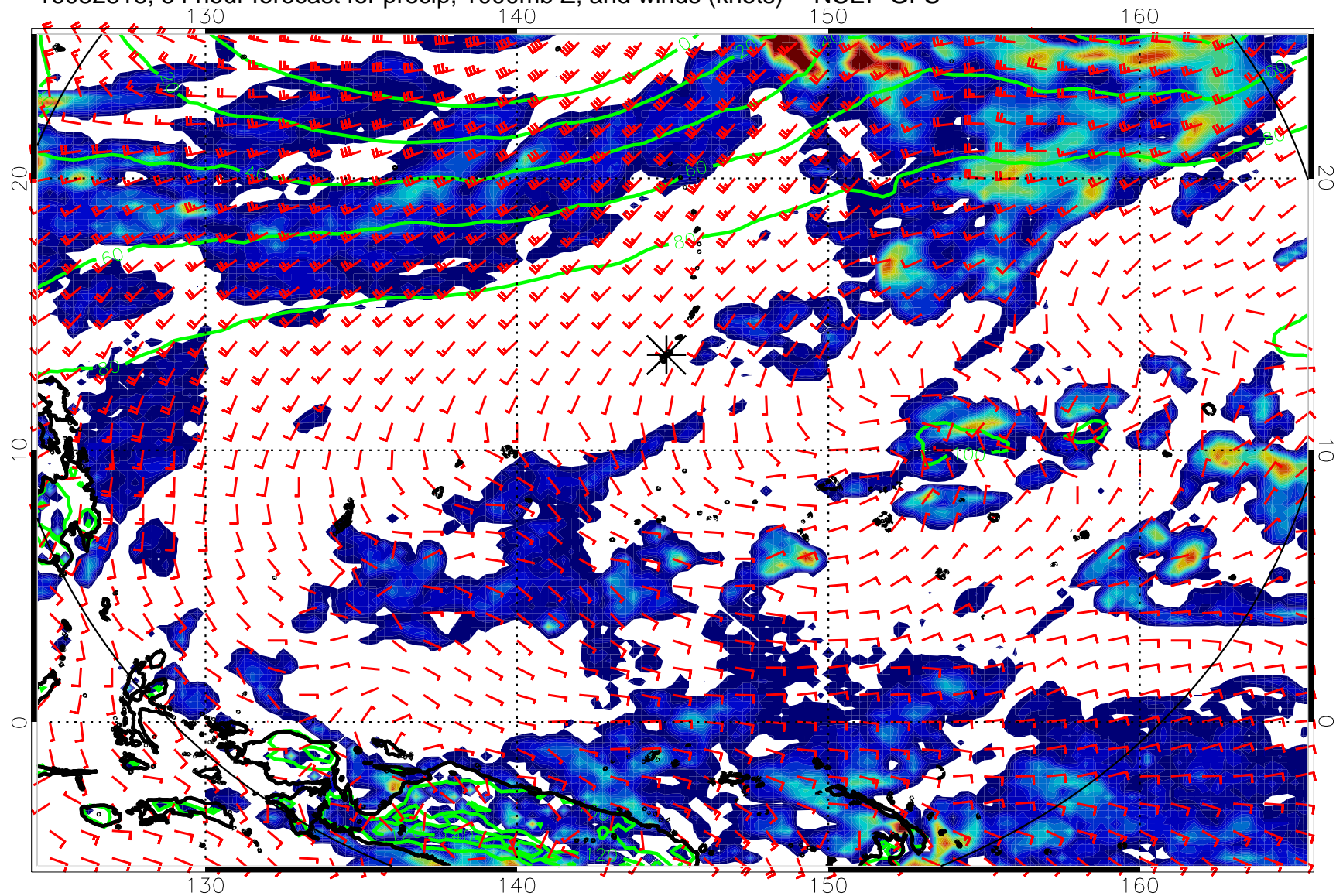
16082818, 54 hour forecast for precip, 1000mb Z, and winds (knots) -- NCEP GFS
