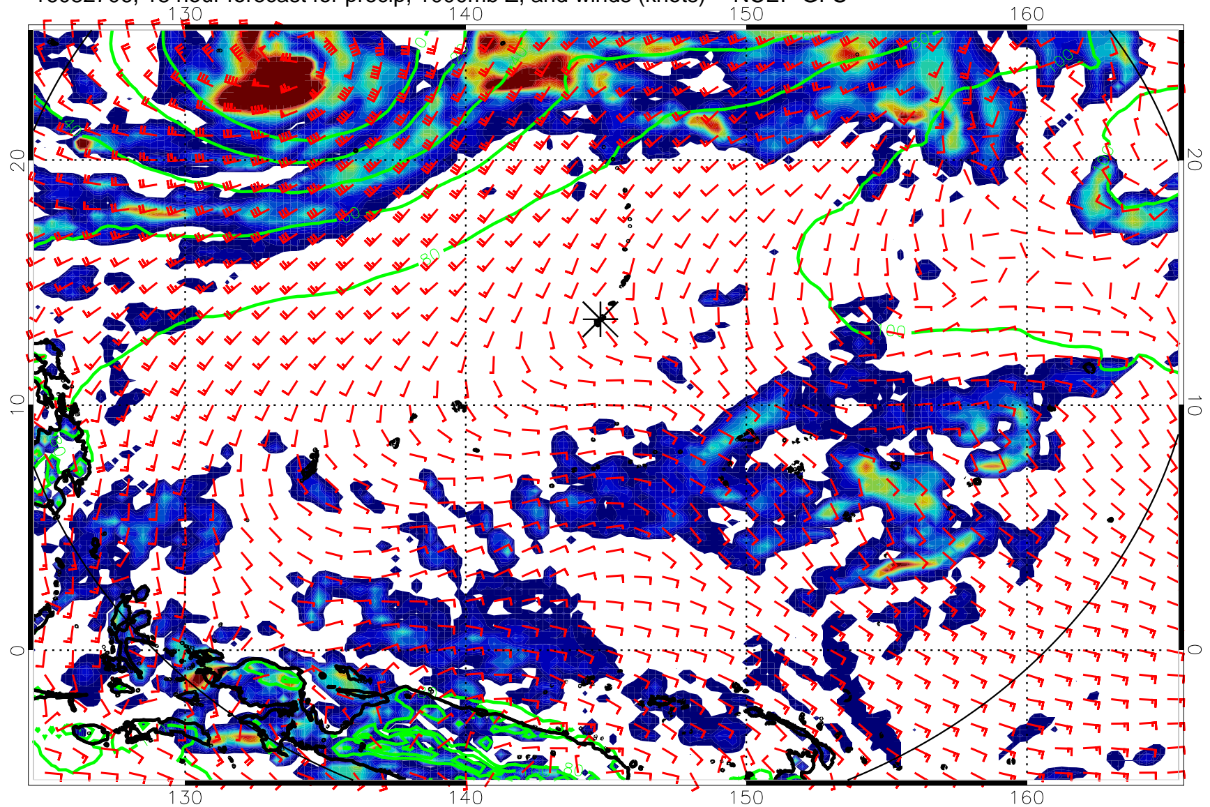
16082706, 18 hour forecast for precip, 1000mb Z, and winds (knots) -- NCEP GFS
