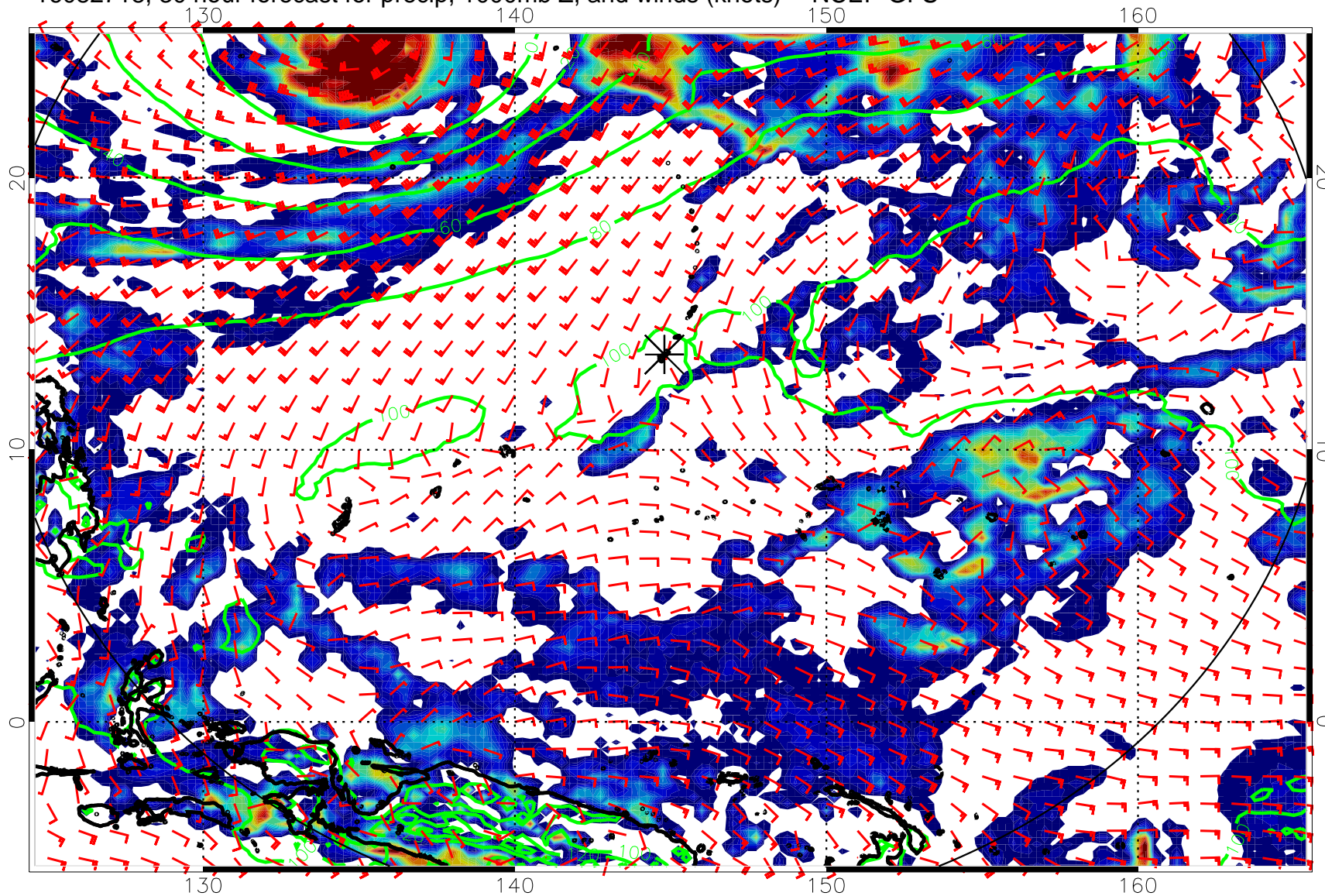
16082718, 30 hour forecast for precip, 1000mb Z, and winds (knots) -- NCEP GFS
