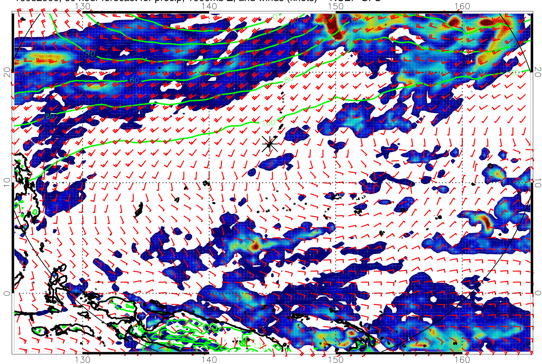
16082900, 60 hour forecast for precip, 1000mb Z, and winds (knots) -- NCEP GFS
