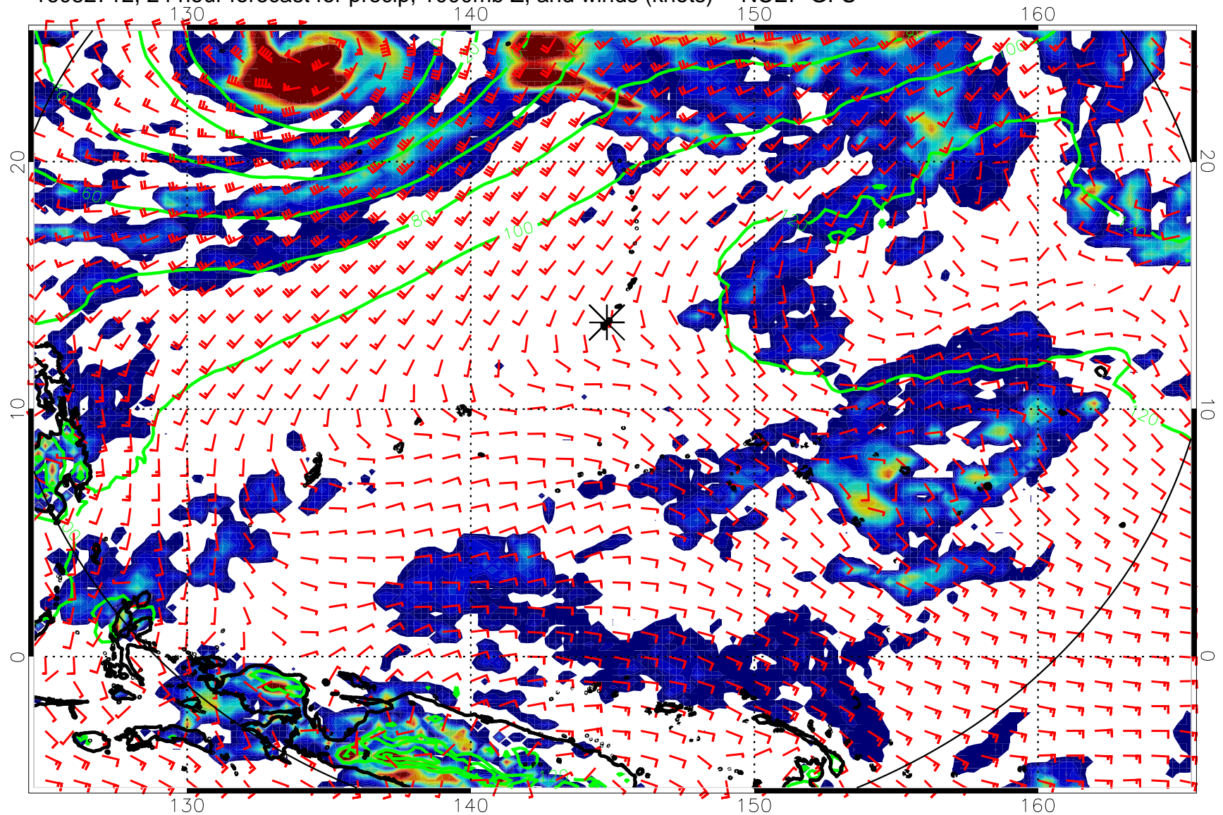
16082712, 24 hour forecast for precip, 1000mb Z, and winds (knots) -- NCEP GFS
