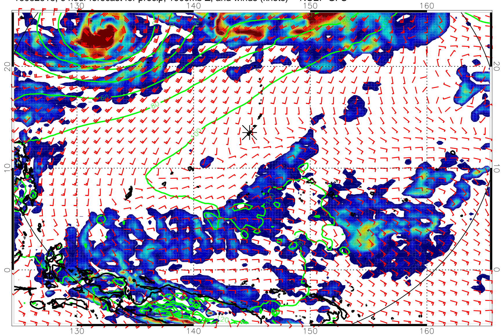
16082618, 6 hour forecast for precip, 1000mb Z, and winds (knots) -- NCEP GFS
