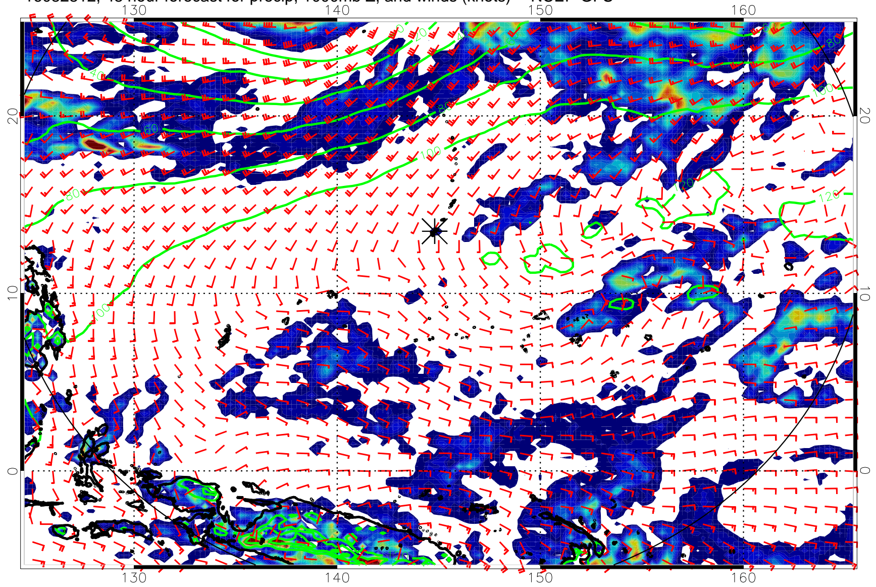
16082812, 48 hour forecast for precip, 1000mb Z, and winds (knots) -- NCEP GFS
