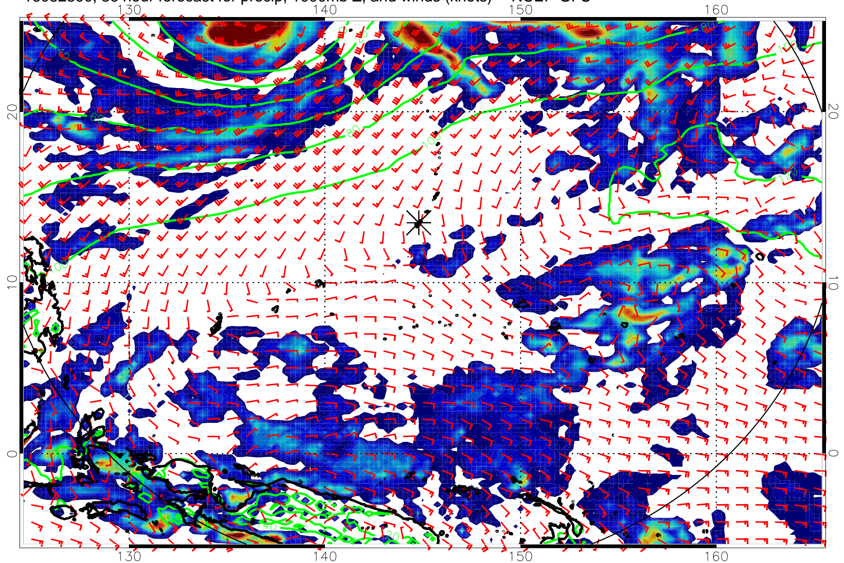
16082800, 36 hour forecast for precip, 1000mb Z, and winds (knots) -- NCEP GFS
