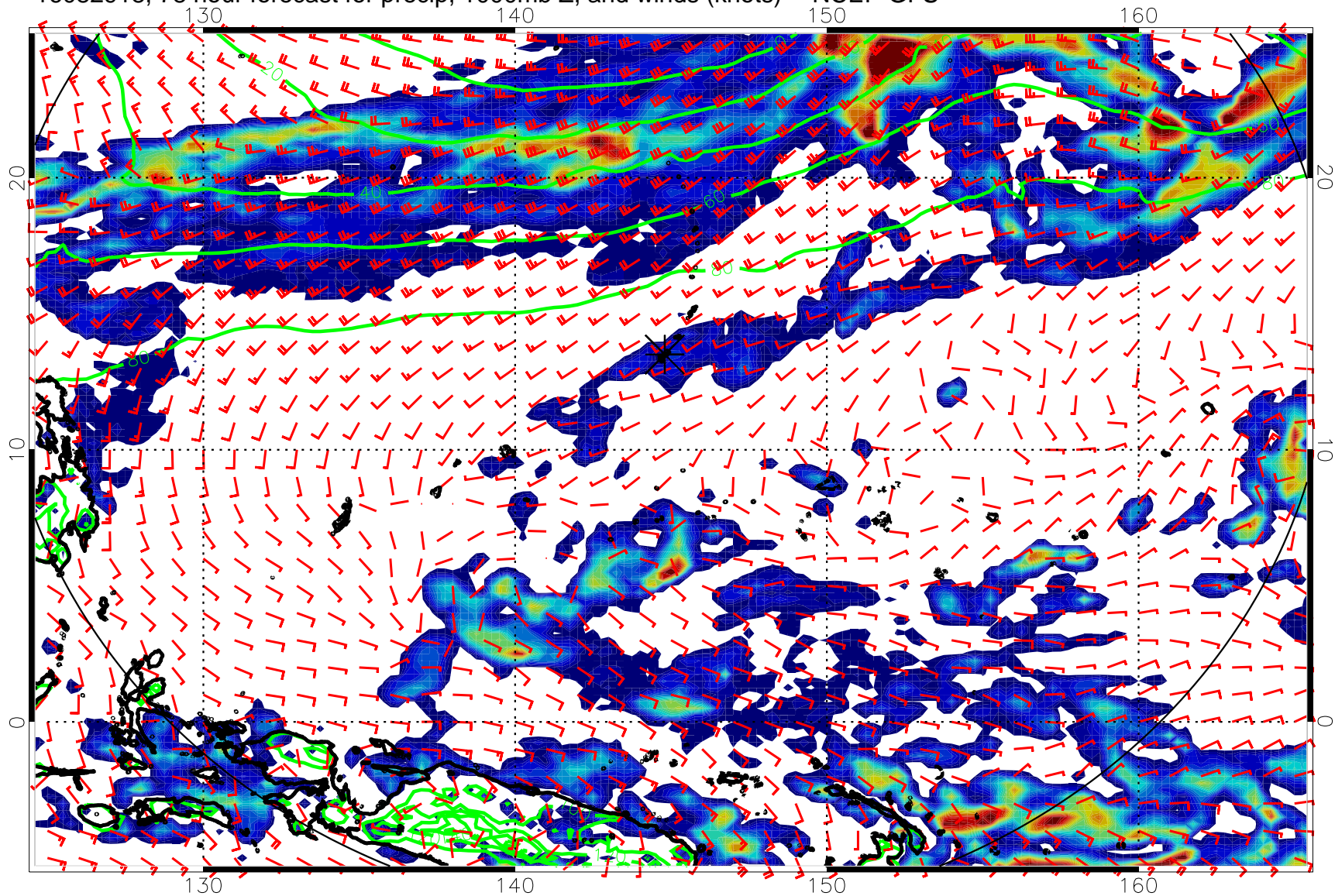
16082918, 78 hour forecast for precip, 1000mb Z, and winds (knots) -- NCEP GFS
