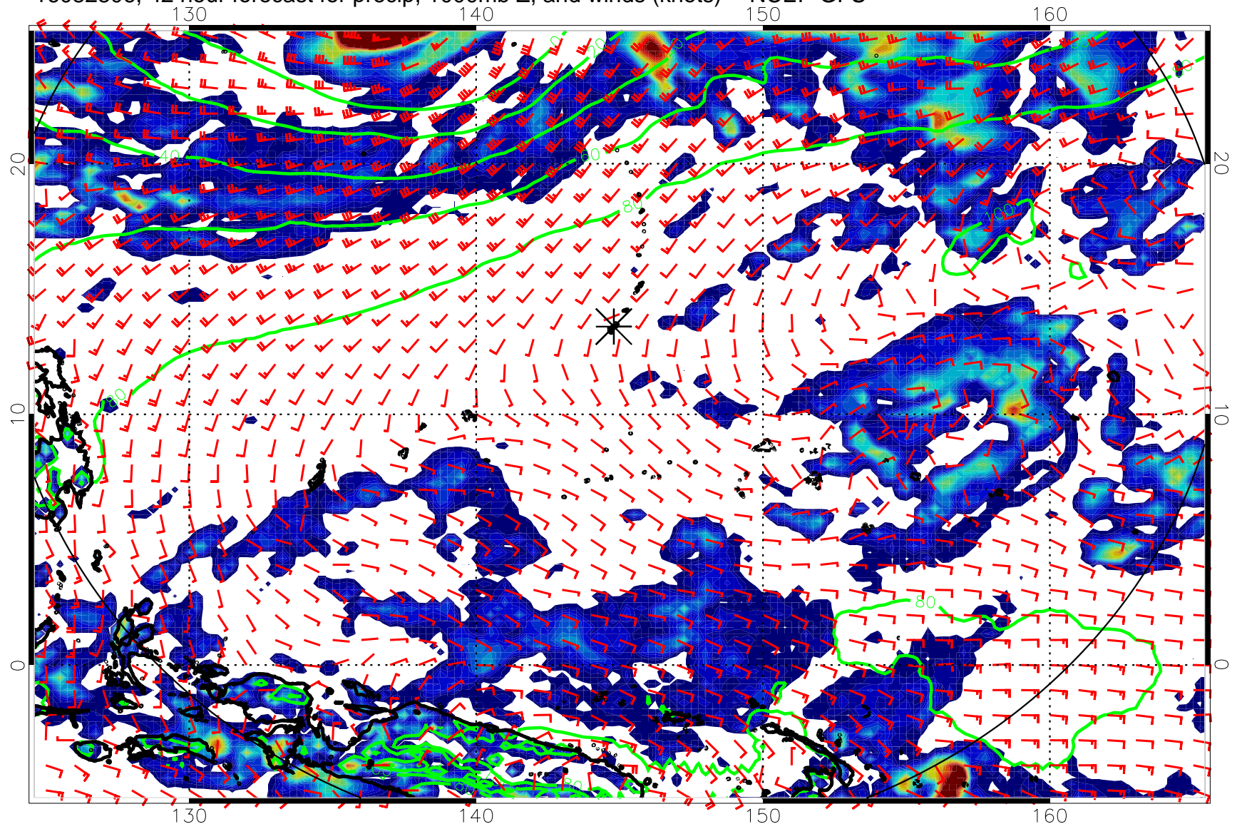
16082806, 42 hour forecast for precip, 1000mb Z, and winds (knots) -- NCEP GFS
