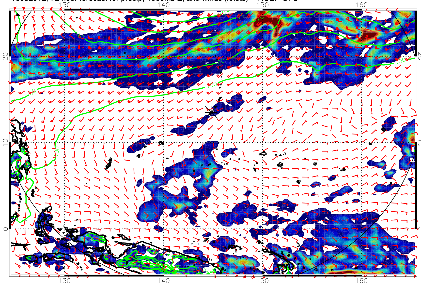
16082912, 72 hour forecast for precip, 1000mb Z, and winds (knots) -- NCEP GFS
