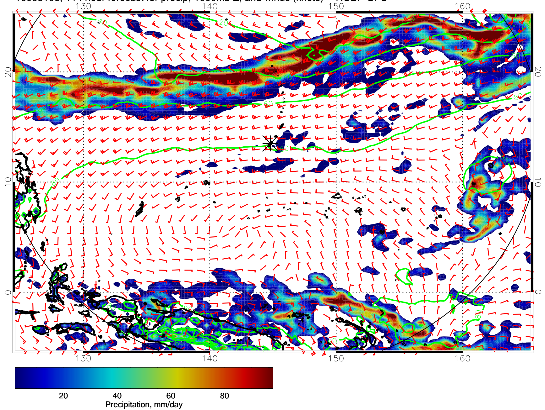
16083106, 114 hour forecast for precip, 1000mb Z, and winds (knots) -- NCEP GFS
