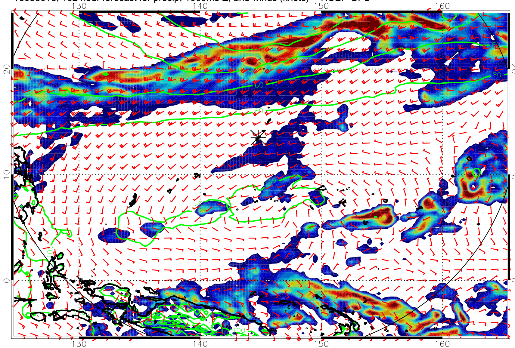
16083018, 102 hour forecast for precip, 1000mb Z, and winds (knots) -- NCEP GFS
