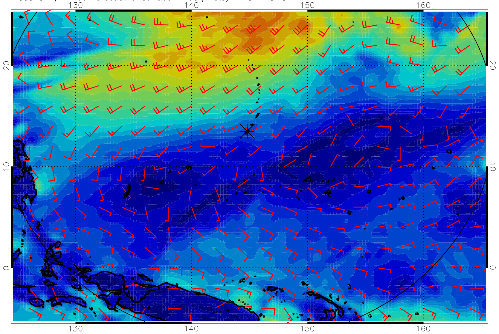
16082912, 72 hour forecast for surface winds (knots) -- NCEP GFS
