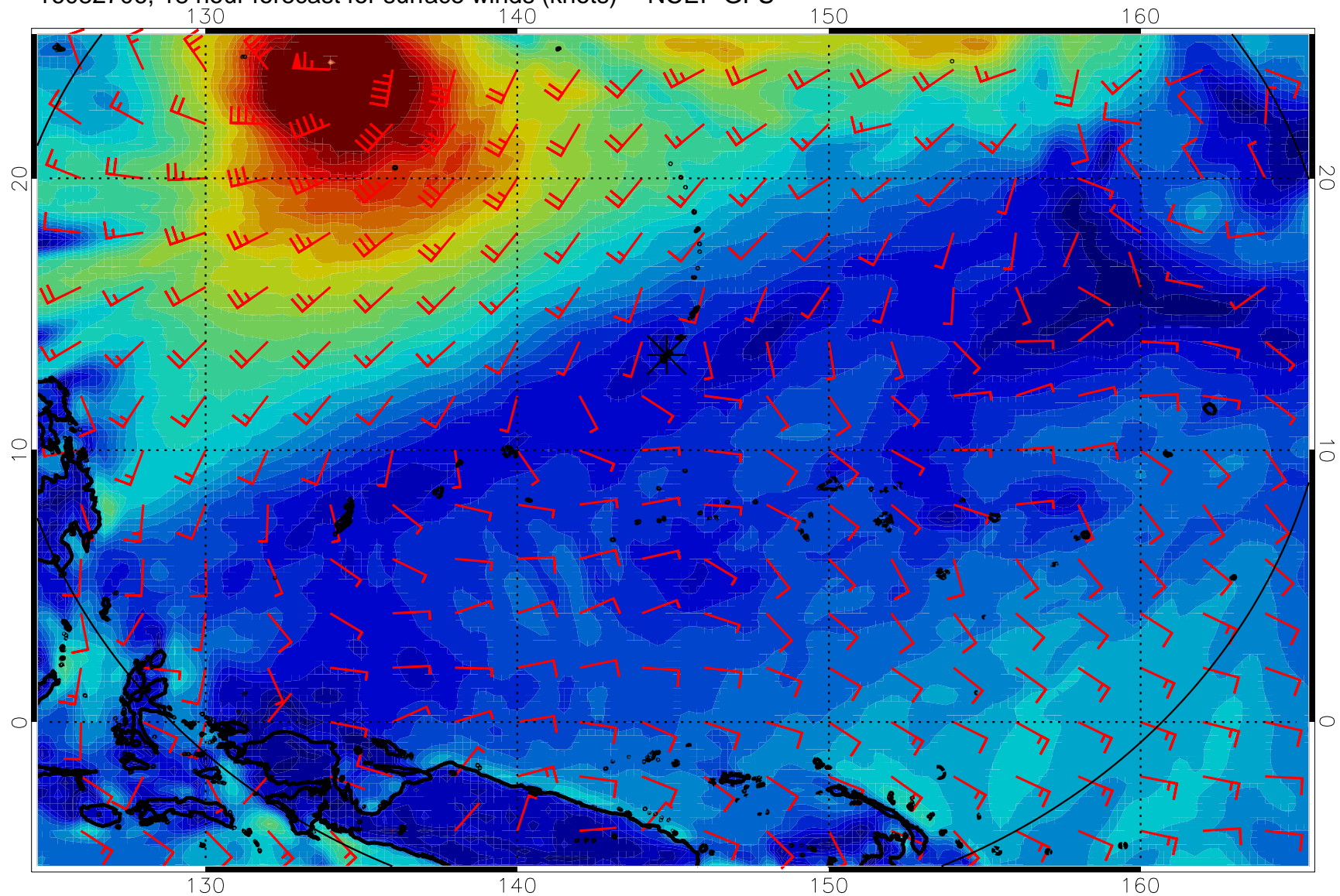
16082706, 18 hour forecast for surface winds (knots) -- NCEP GFS
