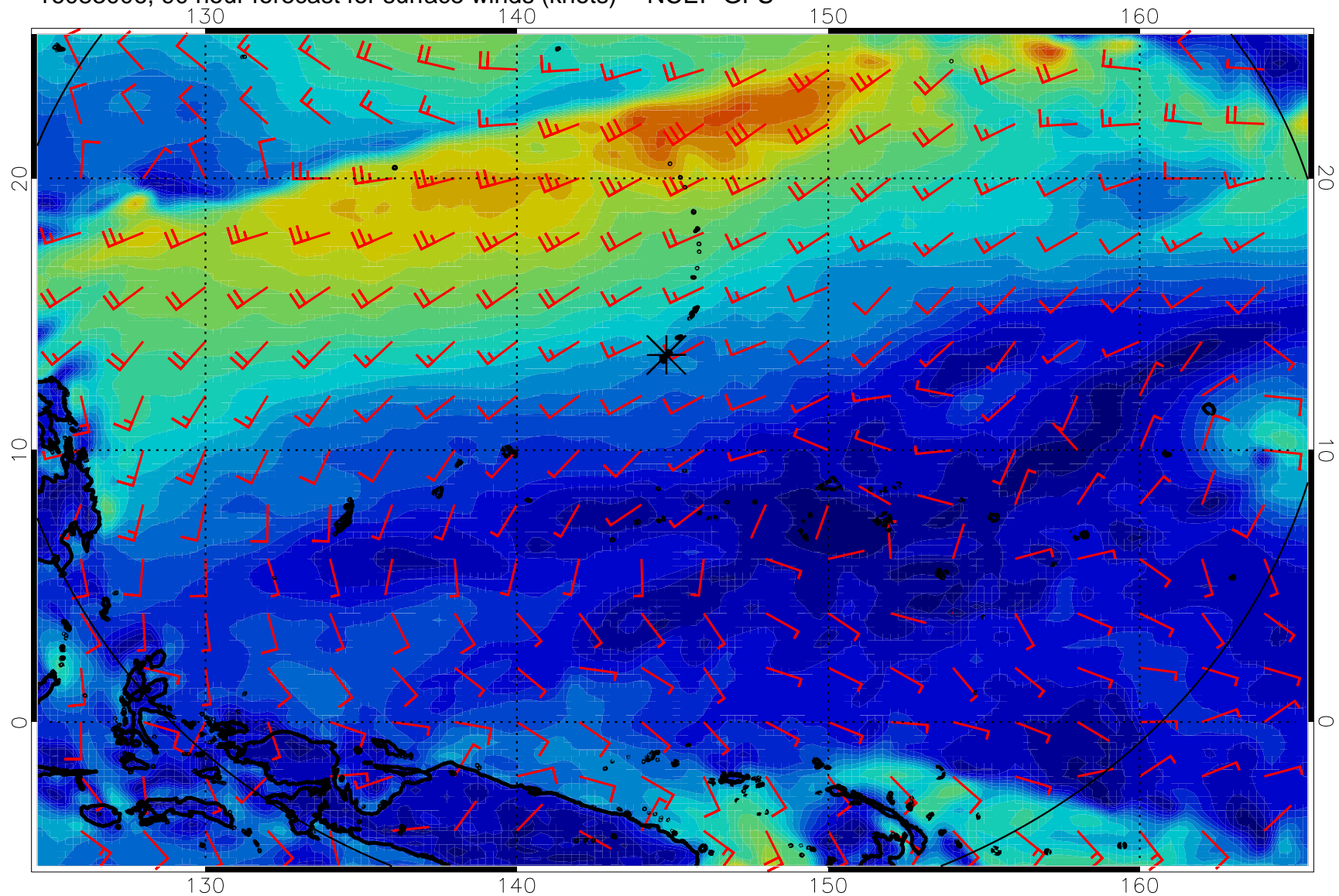
16083006, 90 hour forecast for surface winds (knots) -- NCEP GFS
