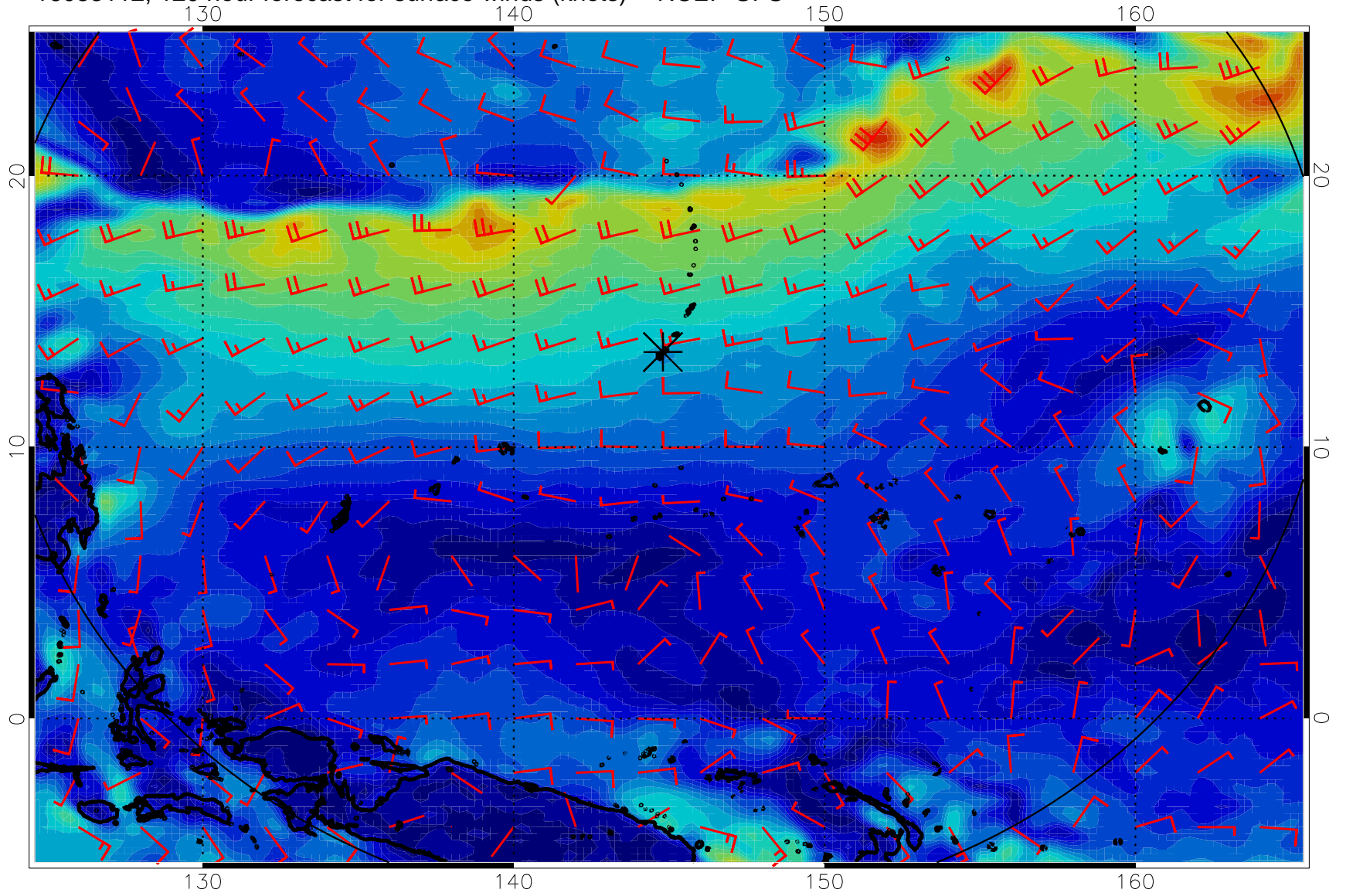
16083112, 120 hour forecast for surface winds (knots) -- NCEP GFS
