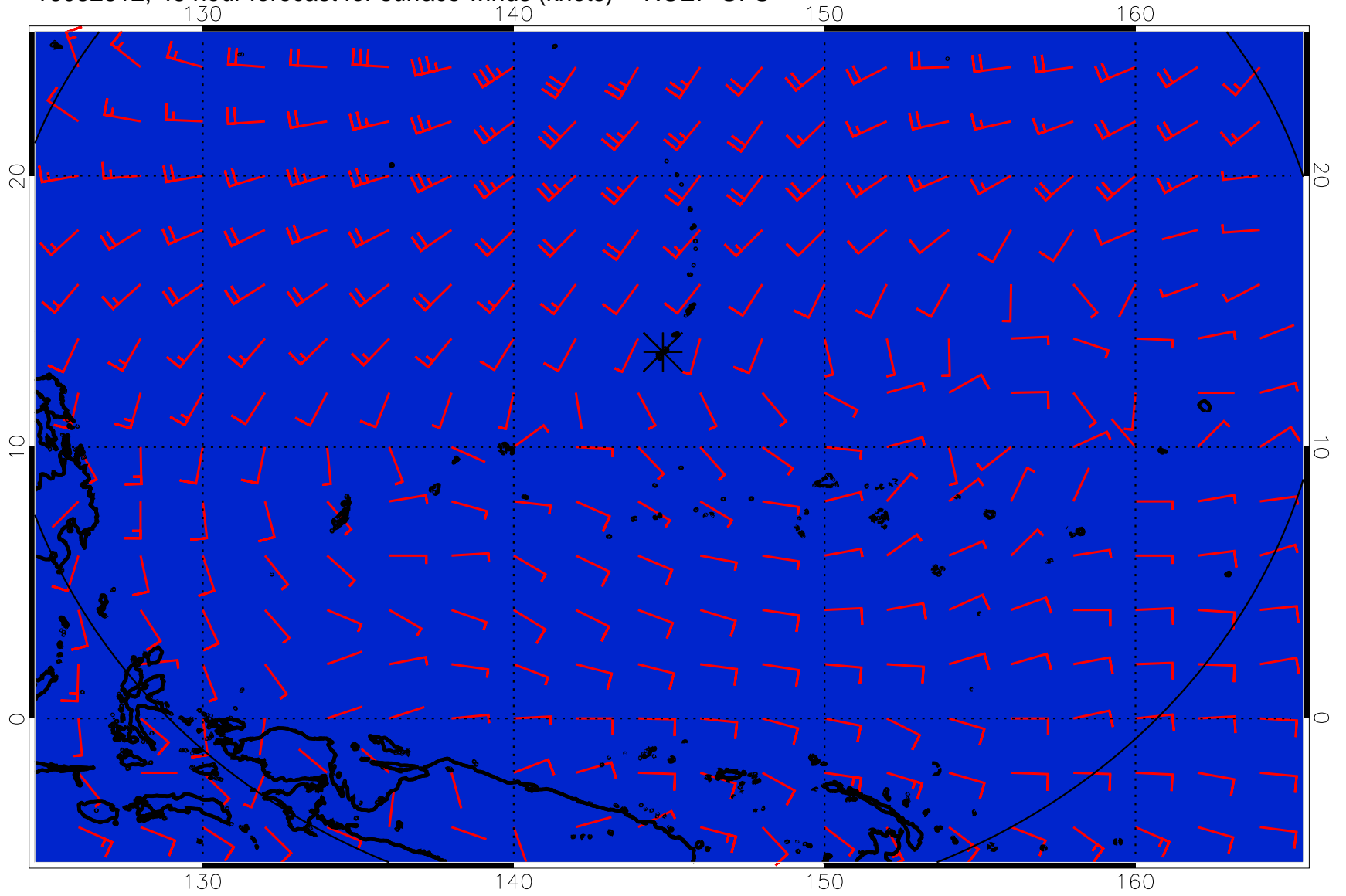
16082812, 48 hour forecast for surface winds (knots) -- NCEP GFS
