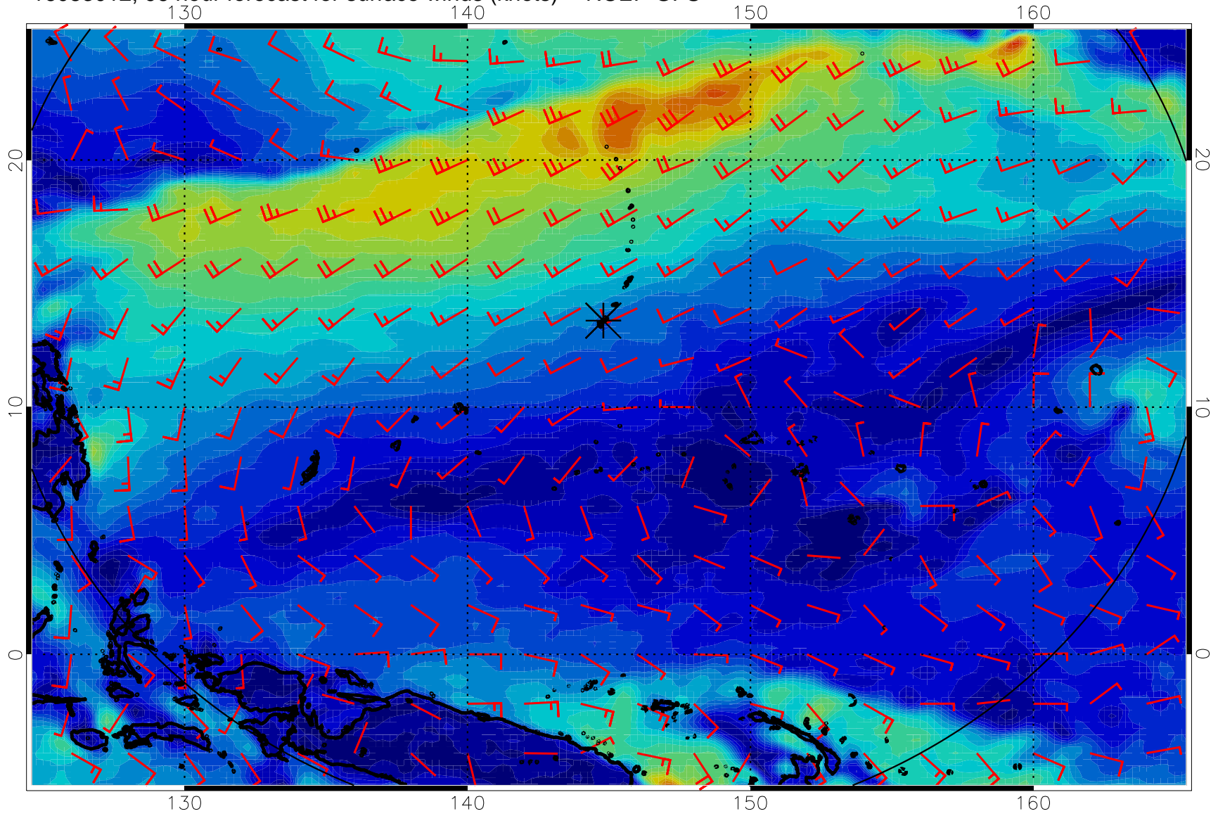
16083012, 96 hour forecast for surface winds (knots) -- NCEP GFS
