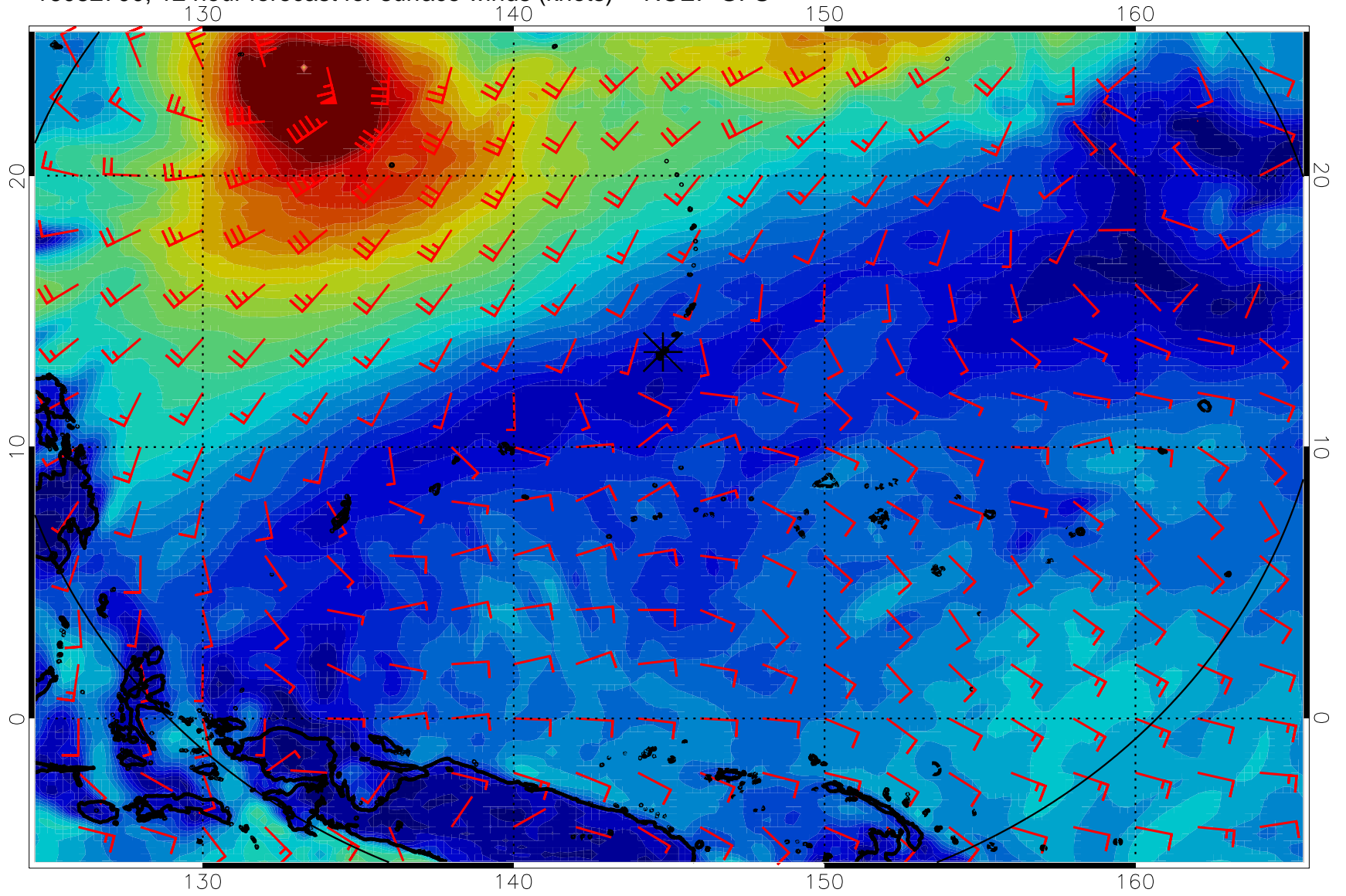
16082700, 12 hour forecast for surface winds (knots) -- NCEP GFS
