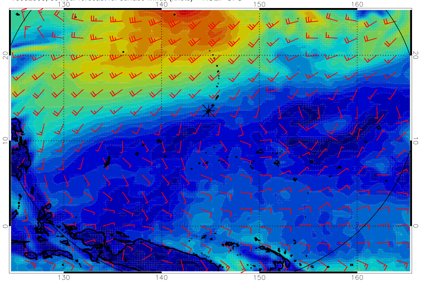
16082900, 60 hour forecast for surface winds (knots) -- NCEP GFS
