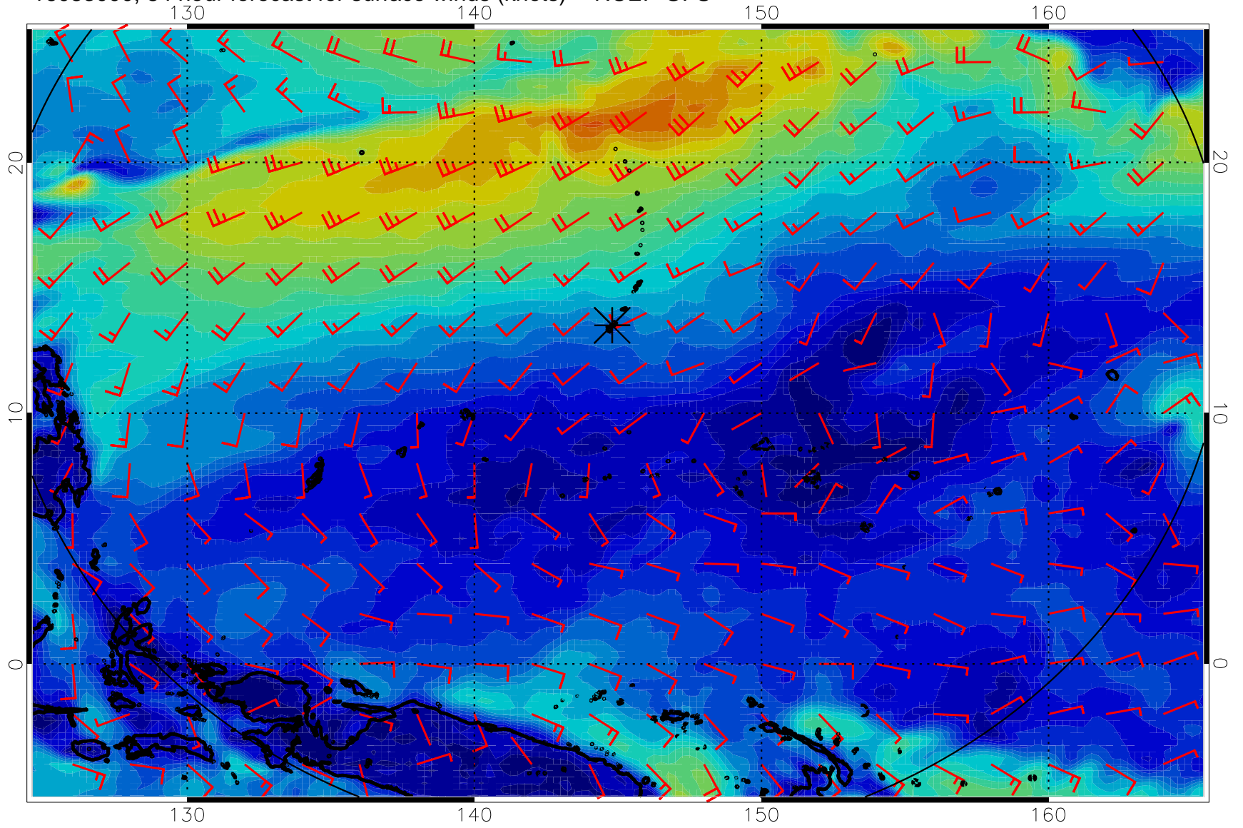
16083000, 84 hour forecast for surface winds (knots) -- NCEP GFS
