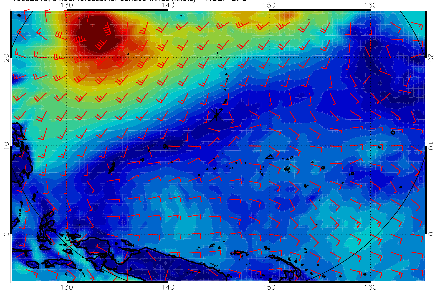
16082618, 6 hour forecast for surface winds (knots) -- NCEP GFS
