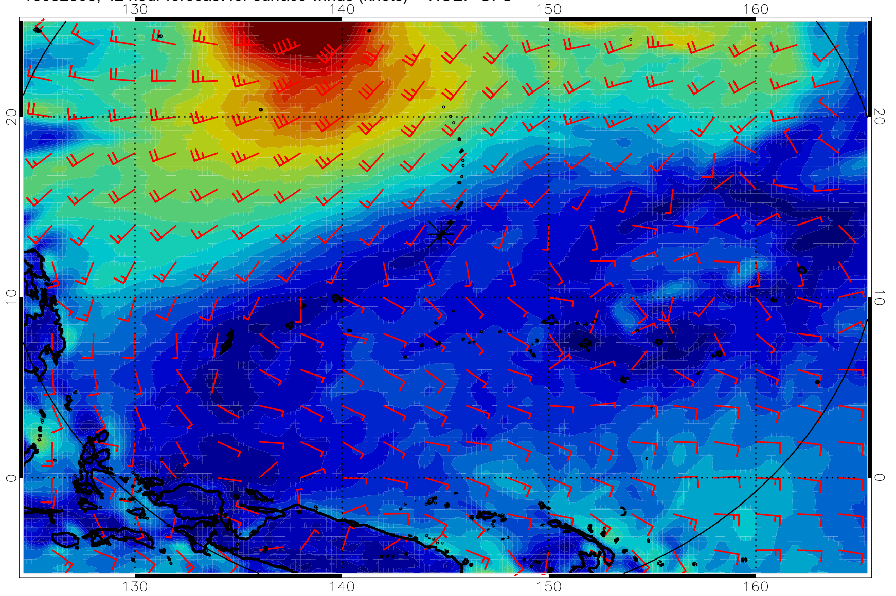
16082806, 42 hour forecast for surface winds (knots) -- NCEP GFS
