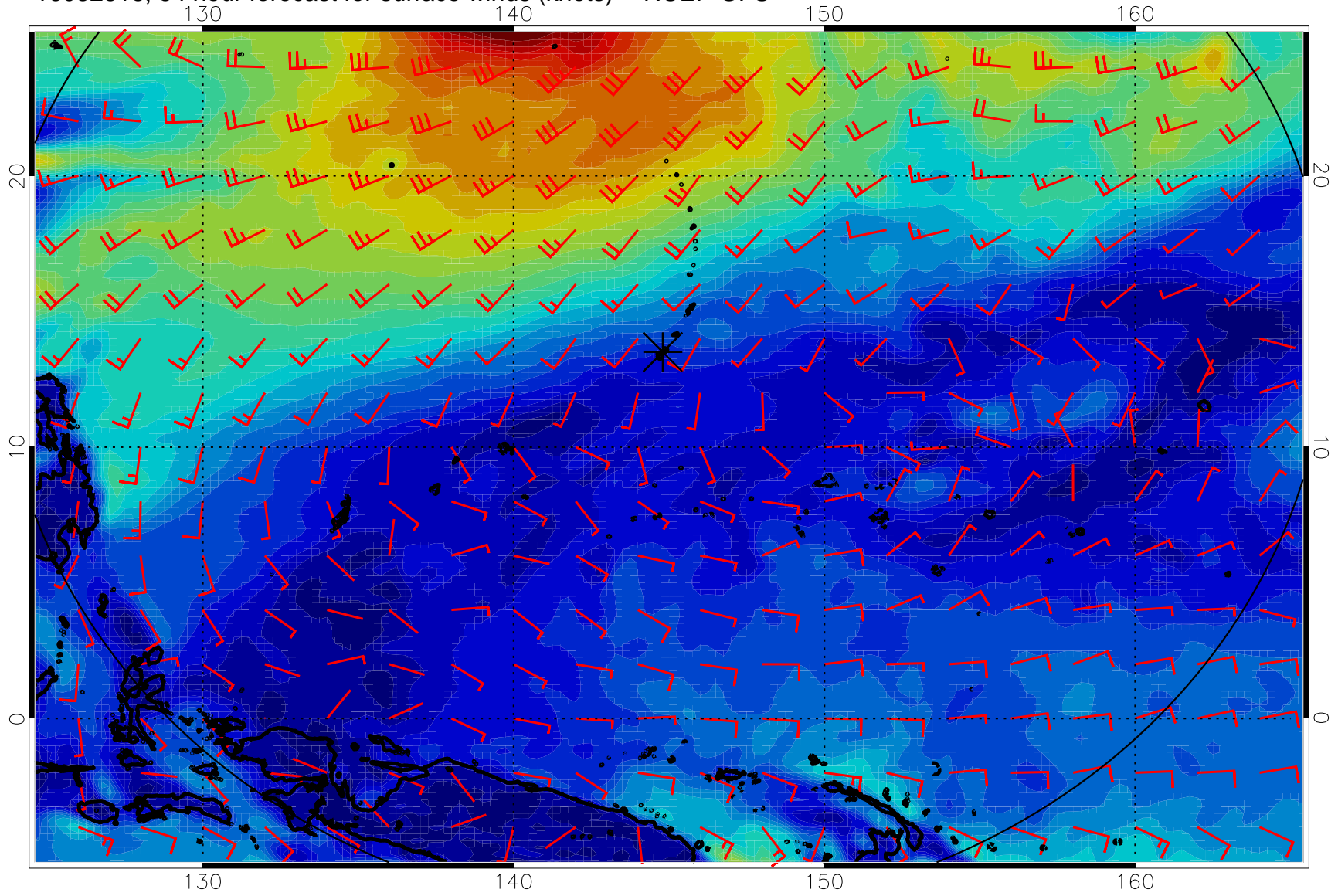
16082818, 54 hour forecast for surface winds (knots) -- NCEP GFS
