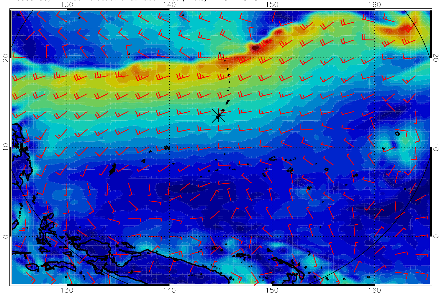
16083106, 114 hour forecast for surface winds (knots) -- NCEP GFS
