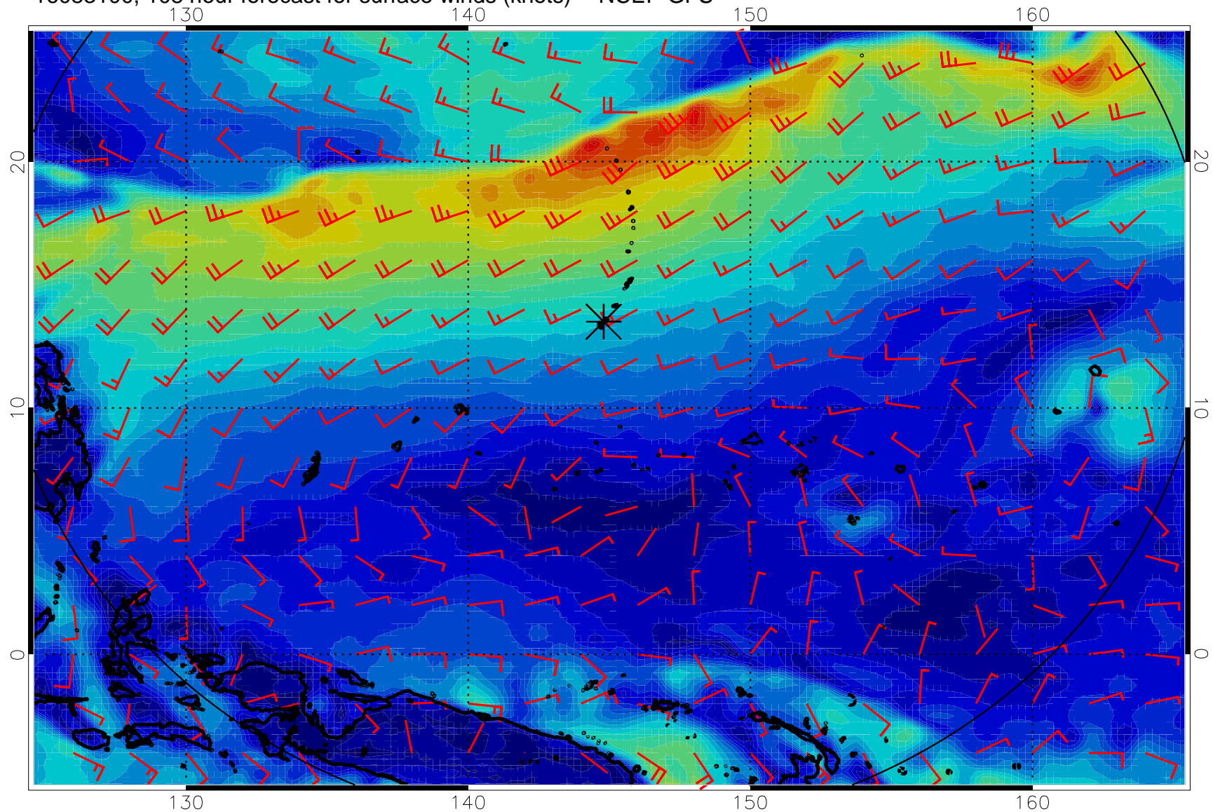
16083100, 108 hour forecast for surface winds (knots) -- NCEP GFS
