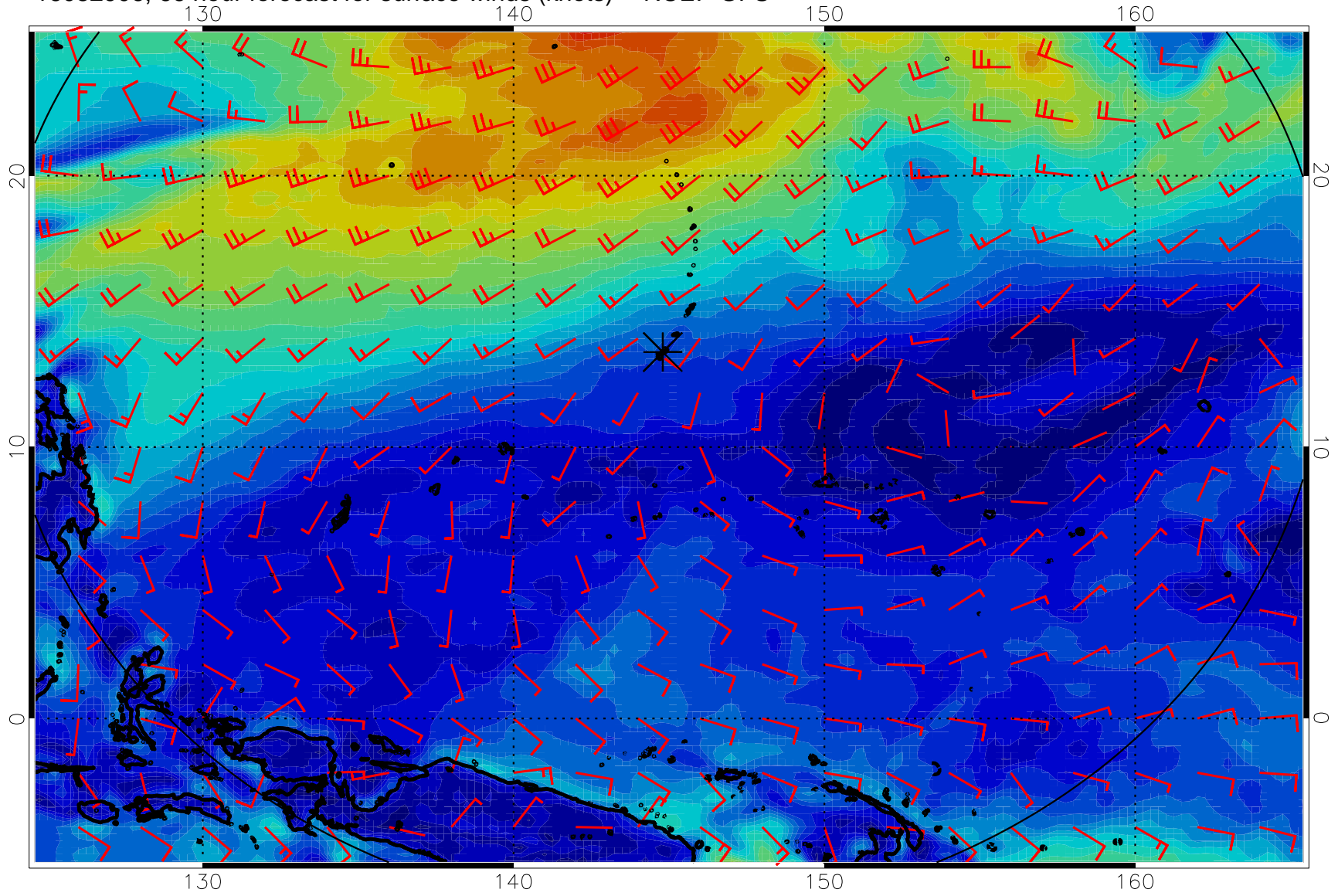
16082906, 66 hour forecast for surface winds (knots) -- NCEP GFS
