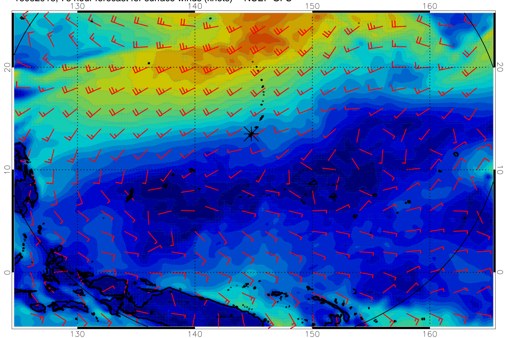
16082918, 78 hour forecast for surface winds (knots) -- NCEP GFS
