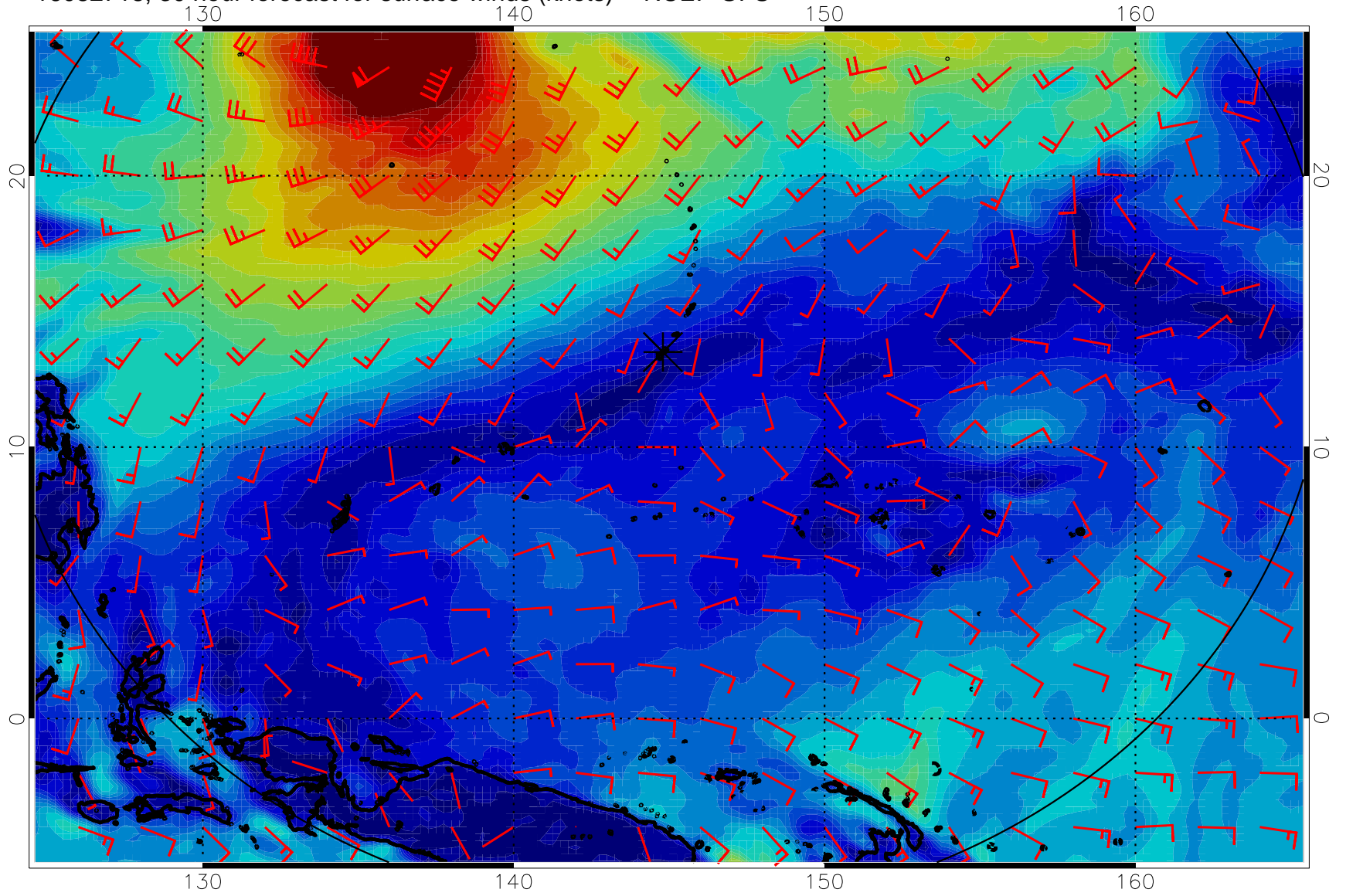
16082718, 30 hour forecast for surface winds (knots) -- NCEP GFS
