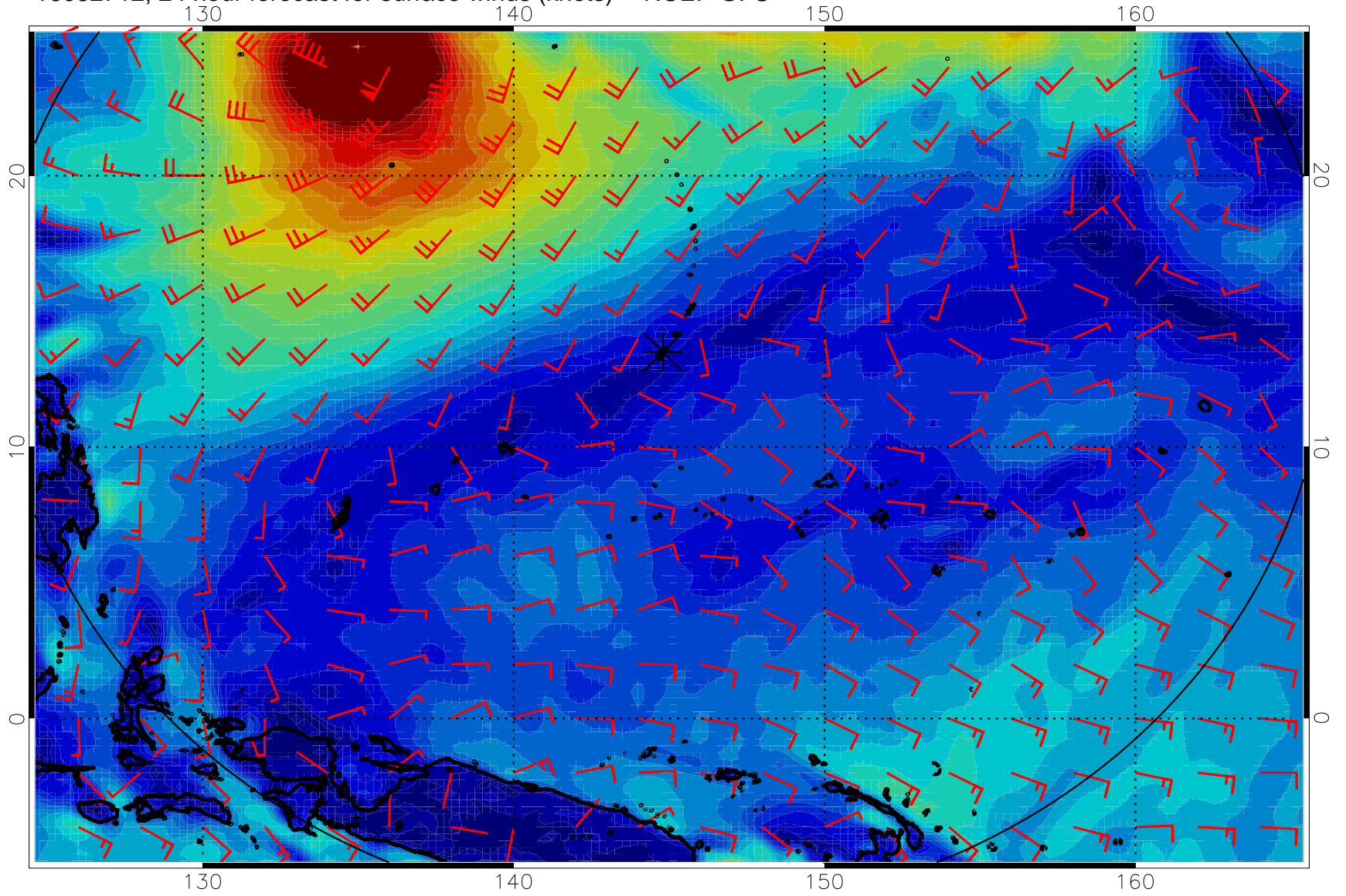
16082712, 24 hour forecast for surface winds (knots) -- NCEP GFS
