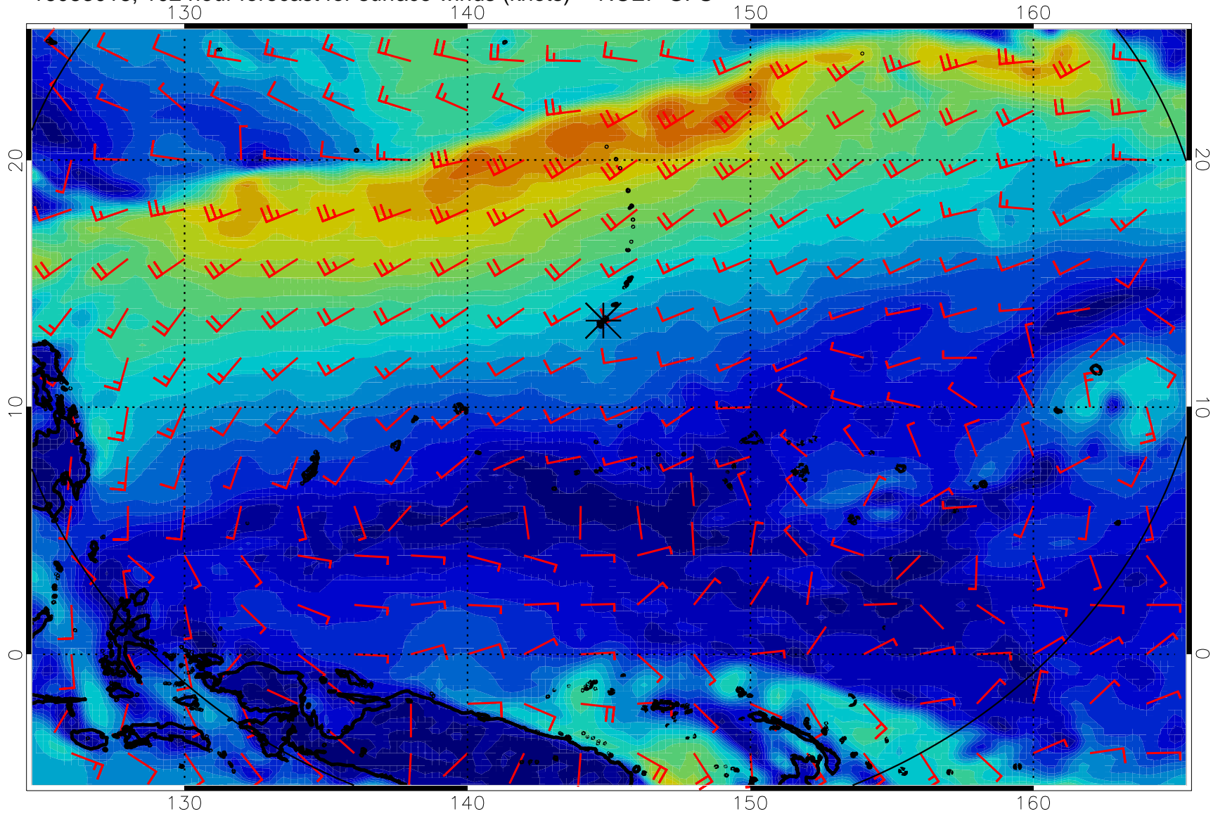
16083018, 102 hour forecast for surface winds (knots) -- NCEP GFS
