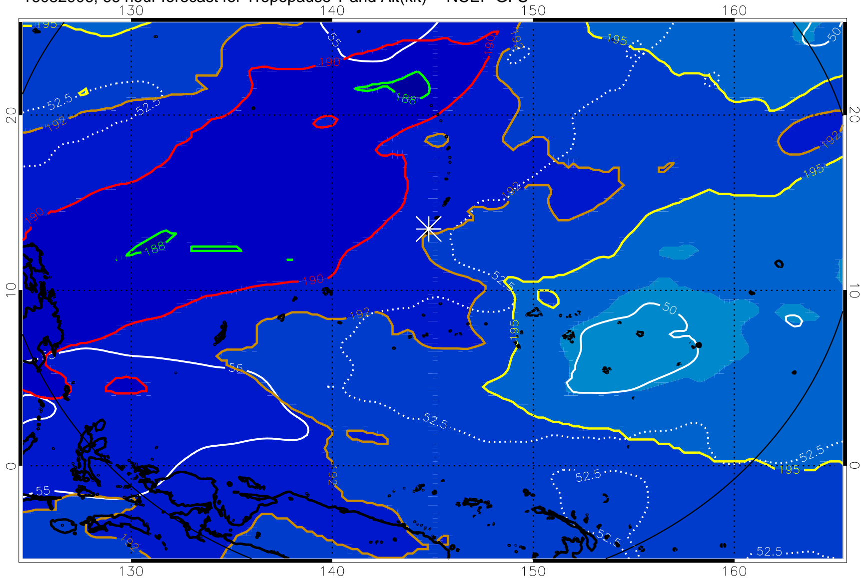
16082906, 66 hour forecast for Tropopause T and Alt(kft) -- NCEP GFS
