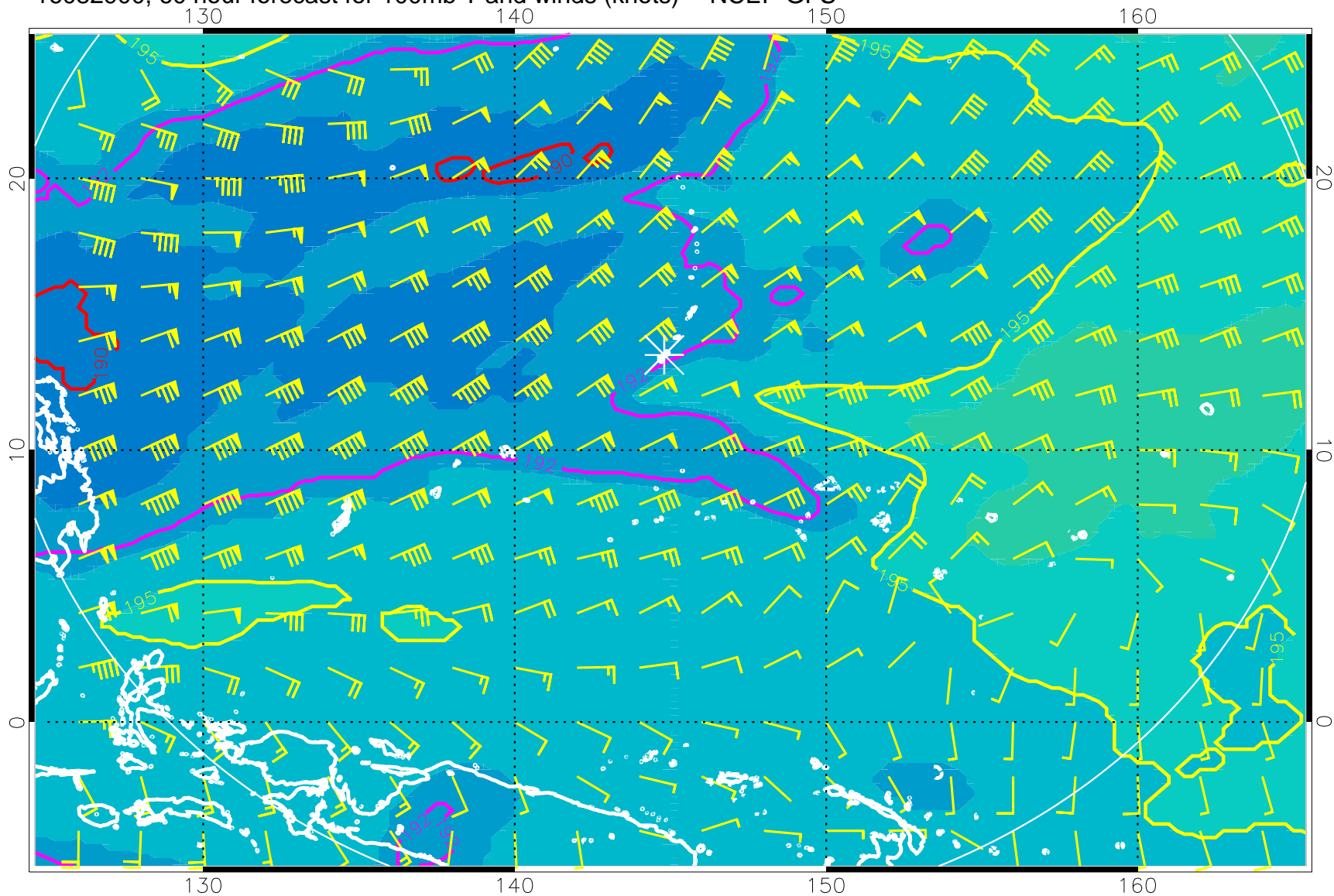
16082900, 60 hour forecast for 100mb T and winds (knots) -- NCEP GFS
