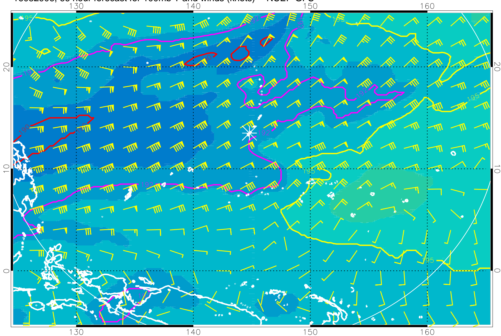
16082906, 66 hour forecast for 100mb T and winds (knots) -- NCEP GFS
