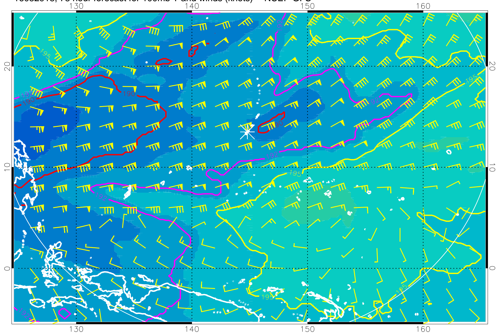
16082918, 78 hour forecast for 100mb T and winds (knots) -- NCEP GFS
