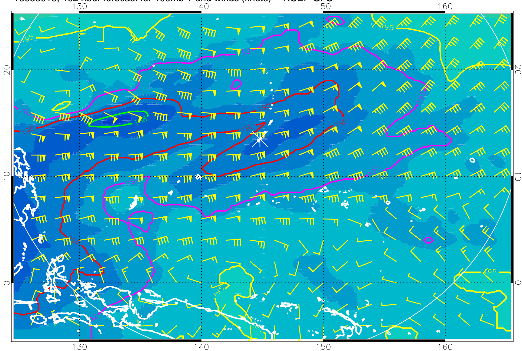
16083018, 102 hour forecast for 100mb T and winds (knots) -- NCEP GFS
