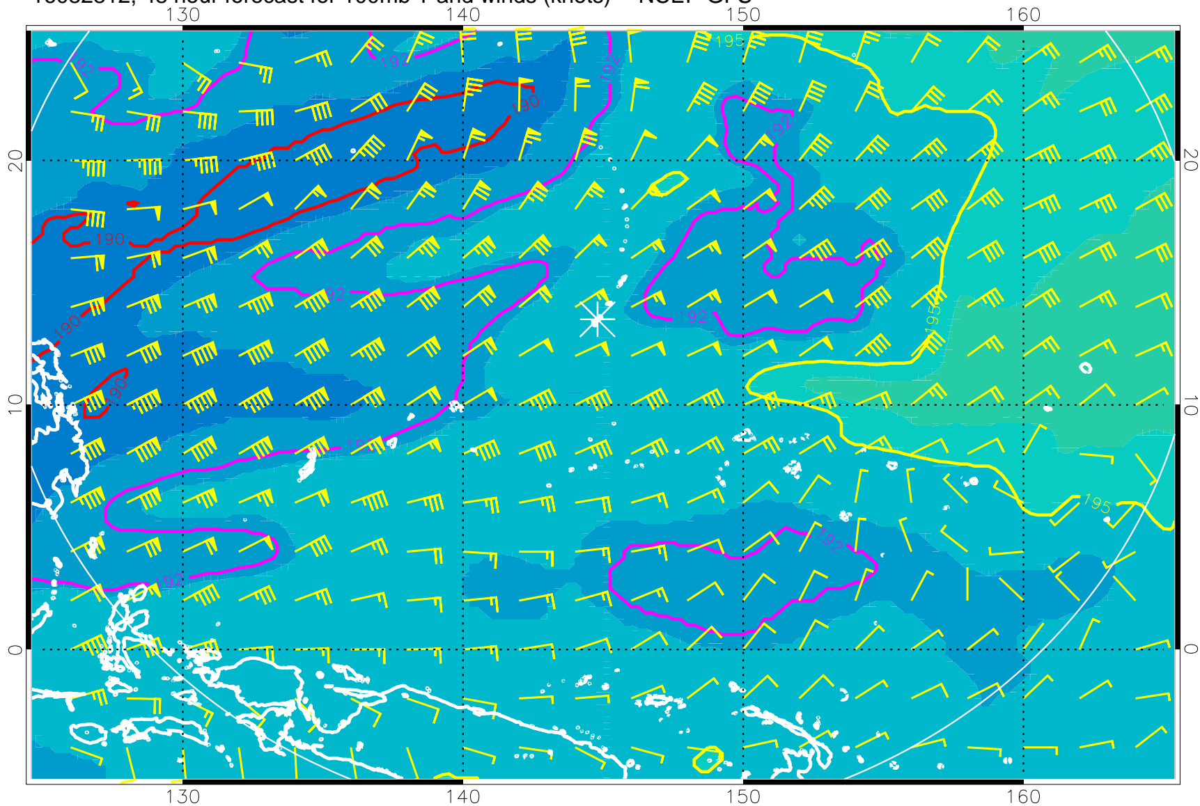
16082812, 48 hour forecast for 100mb T and winds (knots) -- NCEP GFS
