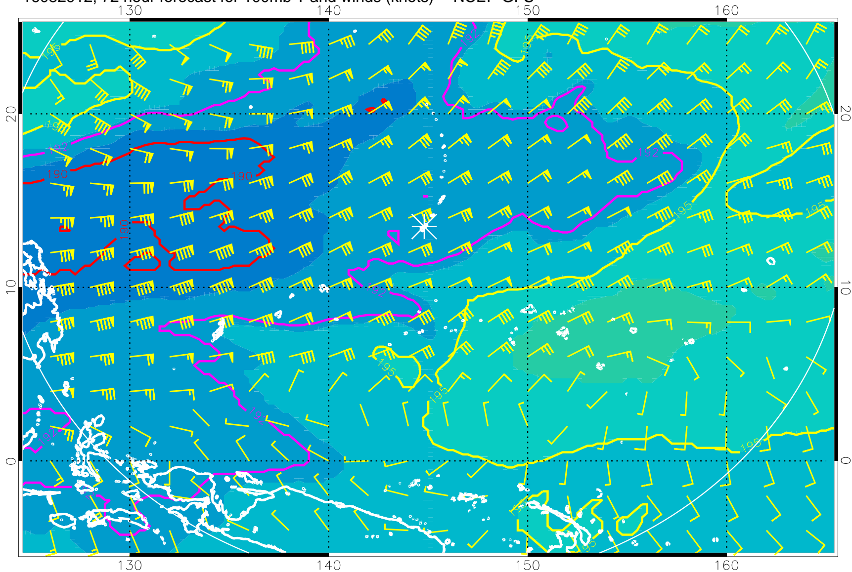
16082912, 72 hour forecast for 100mb T and winds (knots) -- NCEP GFS
