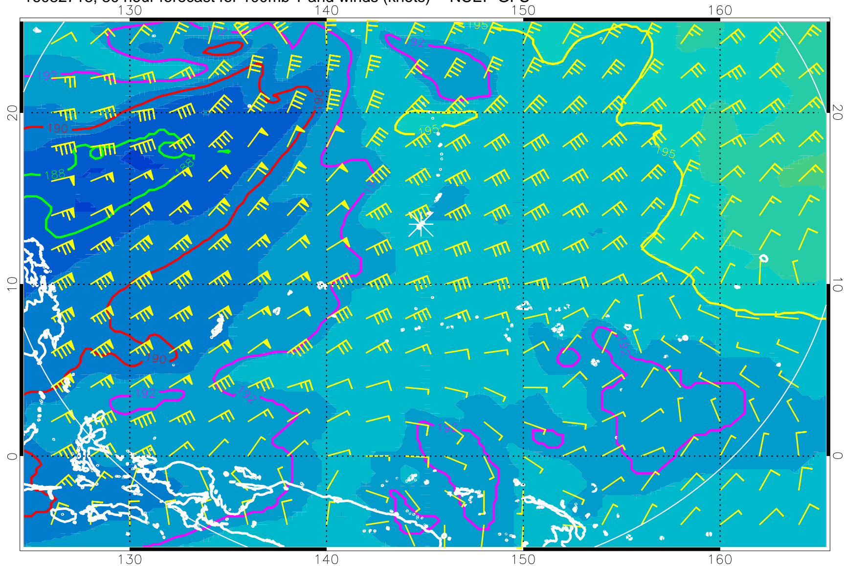
16082718, 30 hour forecast for 100mb T and winds (knots) -- NCEP GFS
