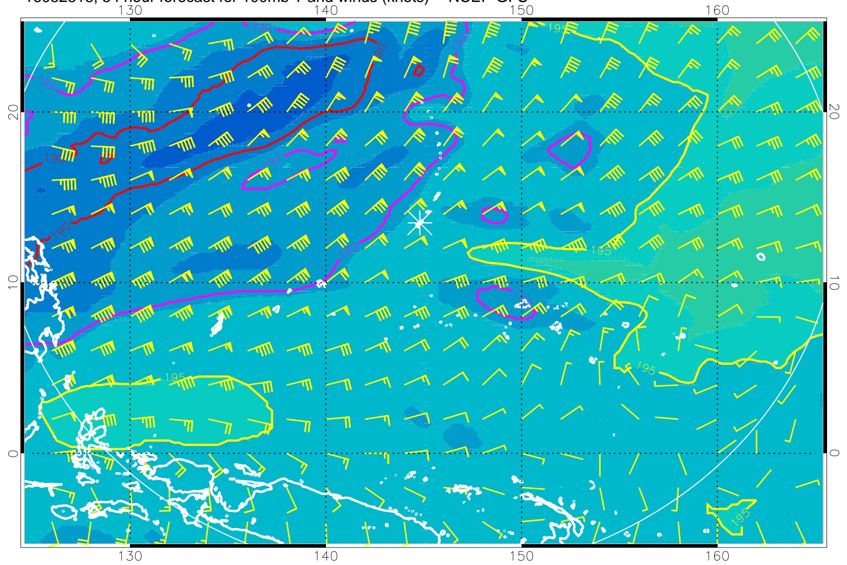
16082818, 54 hour forecast for 100mb T and winds (knots) -- NCEP GFS
