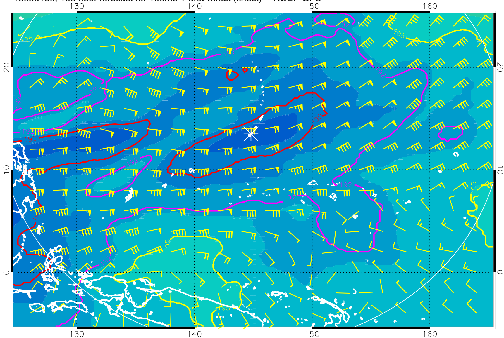
16083100, 108 hour forecast for 100mb T and winds (knots) -- NCEP GFS
