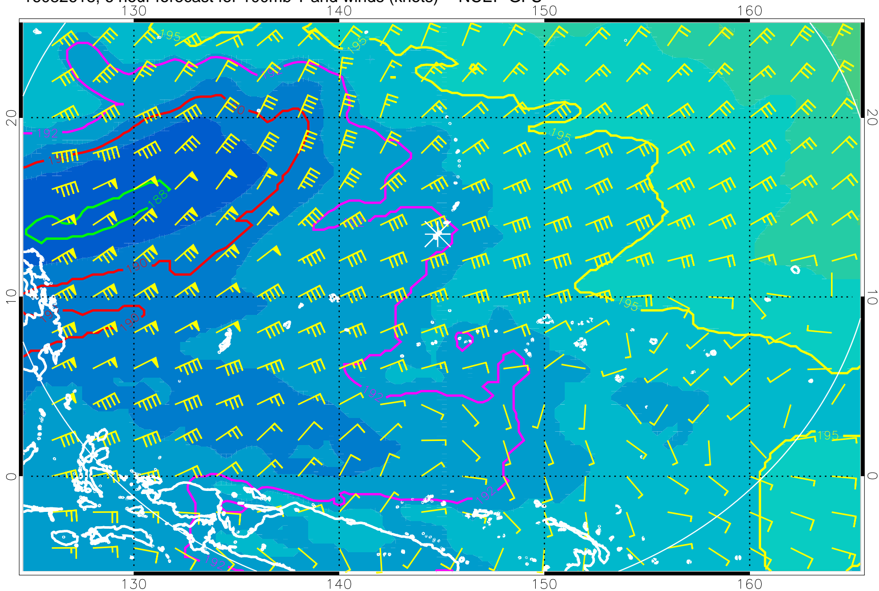
16082618, 6 hour forecast for 100mb T and winds (knots) -- NCEP GFS
