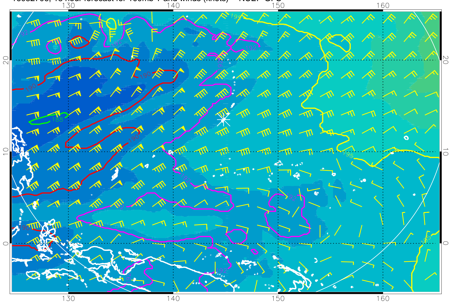
16082706, 18 hour forecast for 100mb T and winds (knots) -- NCEP GFS
