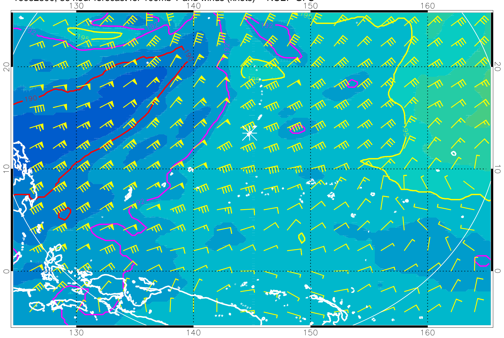
16082800, 36 hour forecast for 100mb T and winds (knots) -- NCEP GFS
