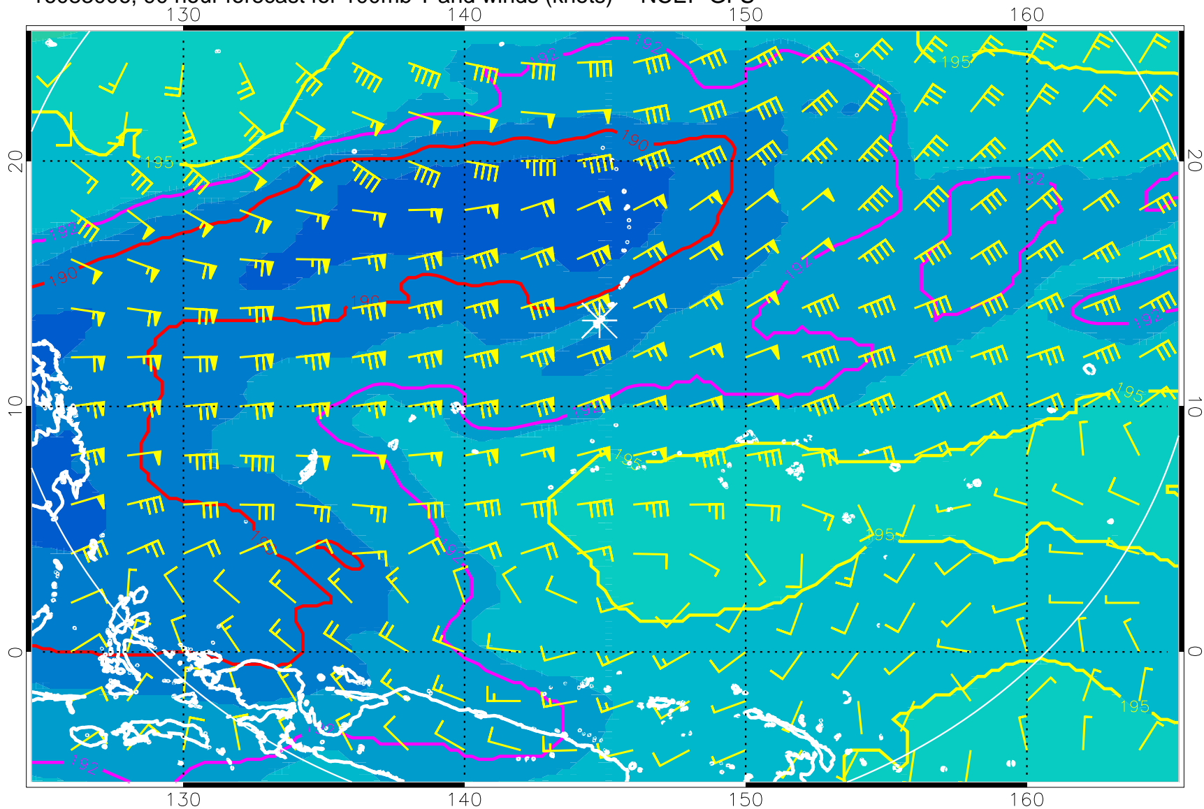
16083006, 90 hour forecast for 100mb T and winds (knots) -- NCEP GFS
