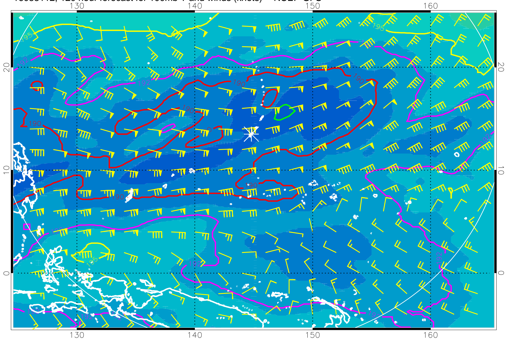
16083112, 120 hour forecast for 100mb T and winds (knots) -- NCEP GFS
