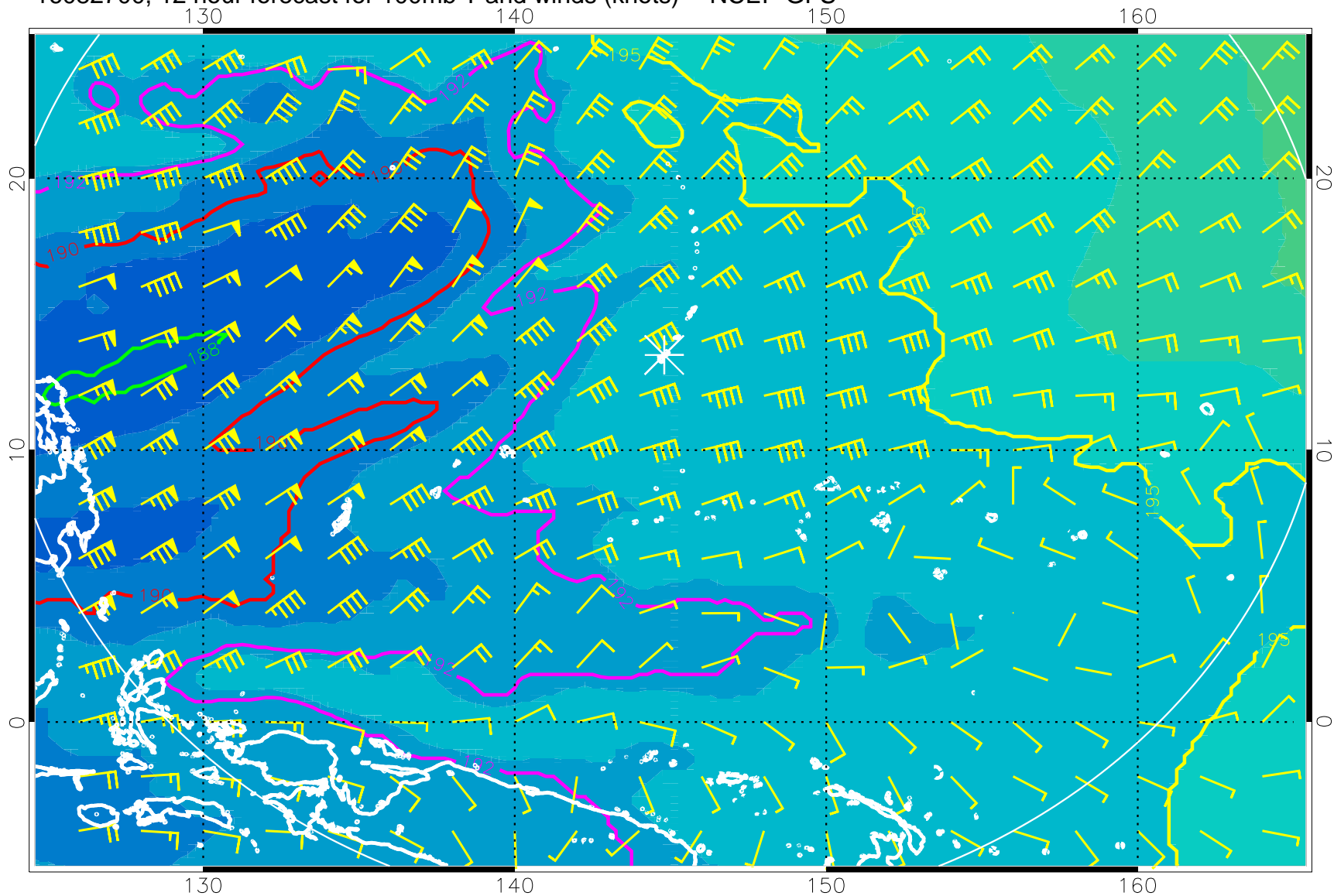
16082700, 12 hour forecast for 100mb T and winds (knots) -- NCEP GFS
