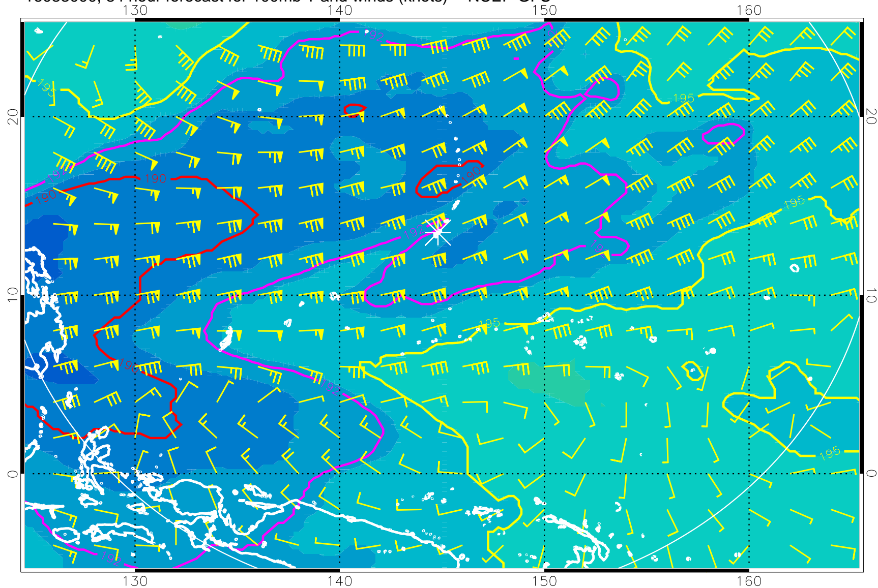
16083000, 84 hour forecast for 100mb T and winds (knots) -- NCEP GFS
