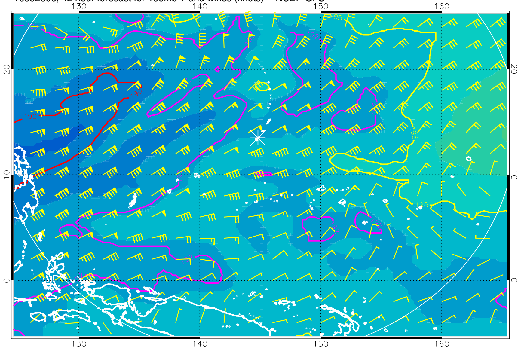
16082806, 42 hour forecast for 100mb T and winds (knots) -- NCEP GFS
