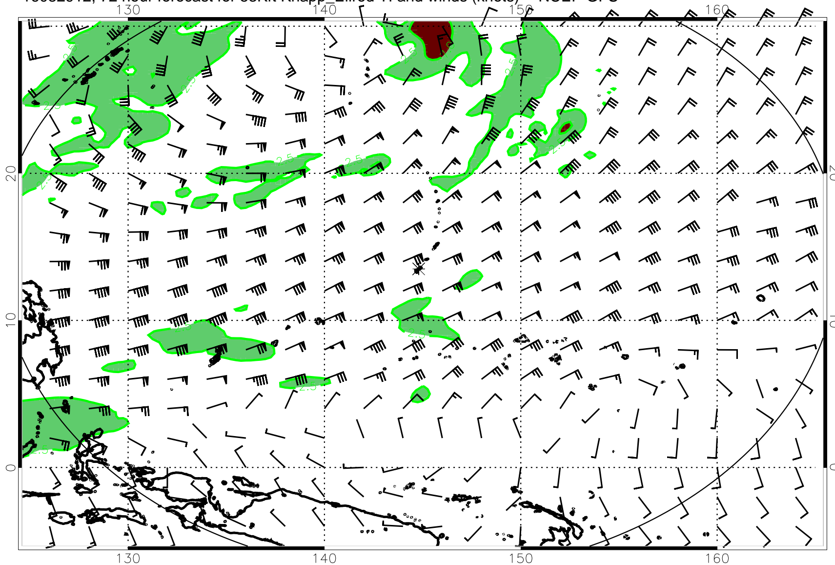
16082912, 72 hour forecast for 53Kft Knapp_Ellrod TI and winds (knots) -- NCEP GFS
