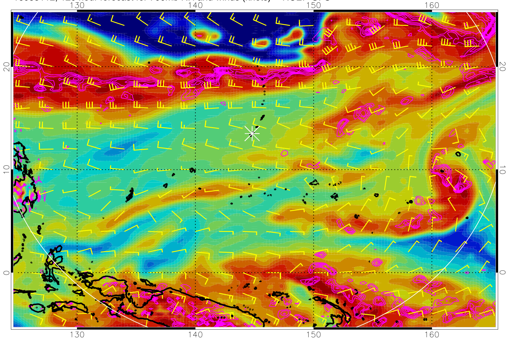
16083112, 120 hour forecast for 700mb RH and winds (knots) -- NCEP GFS
