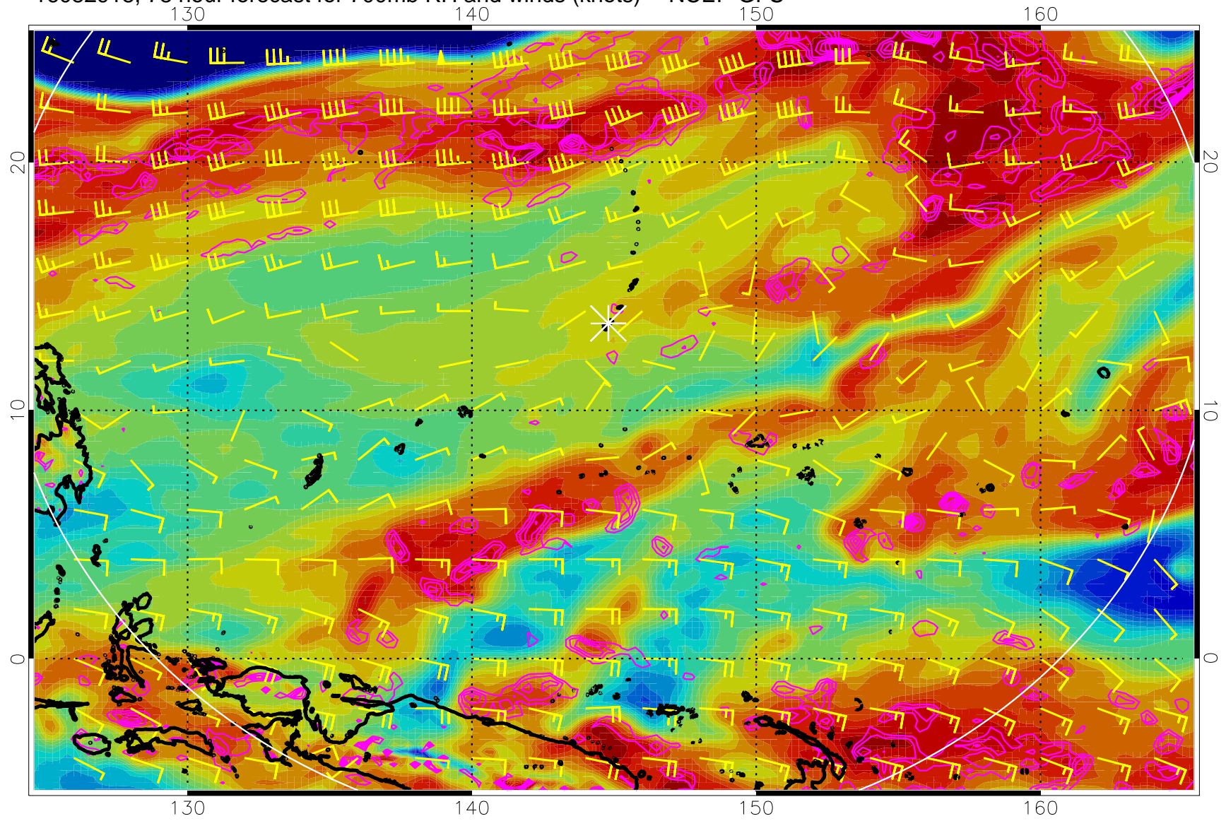
16082918, 78 hour forecast for 700mb RH and winds (knots) -- NCEP GFS
