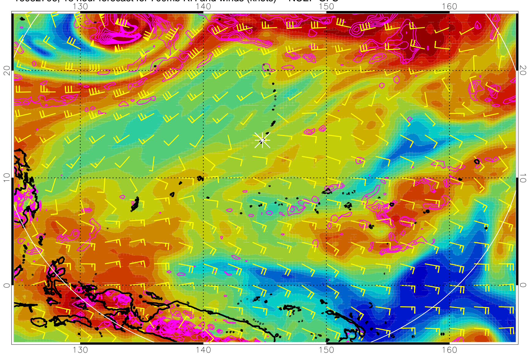
16082706, 18 hour forecast for 700mb RH and winds (knots) -- NCEP GFS
