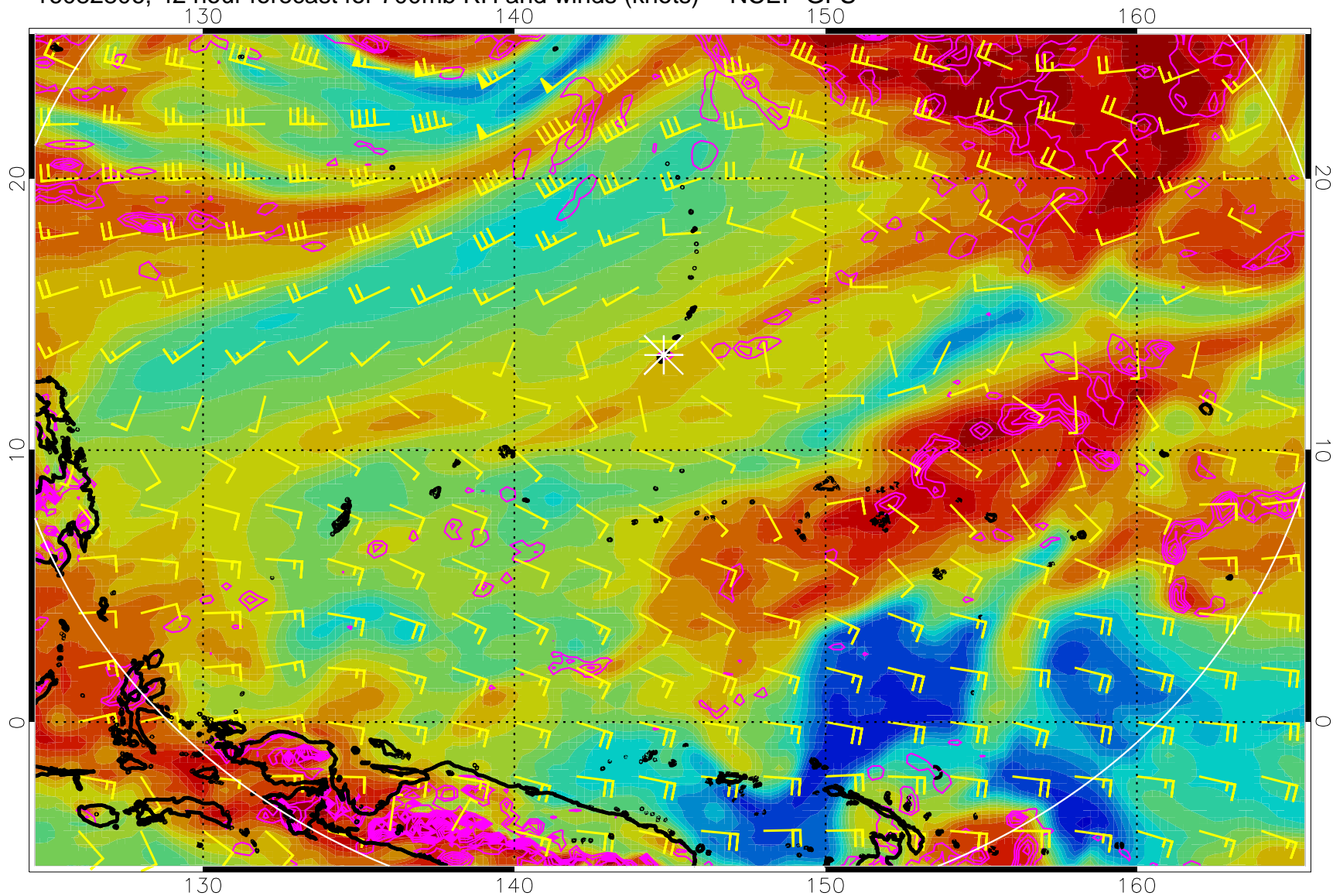
16082806, 42 hour forecast for 700mb RH and winds (knots) -- NCEP GFS
