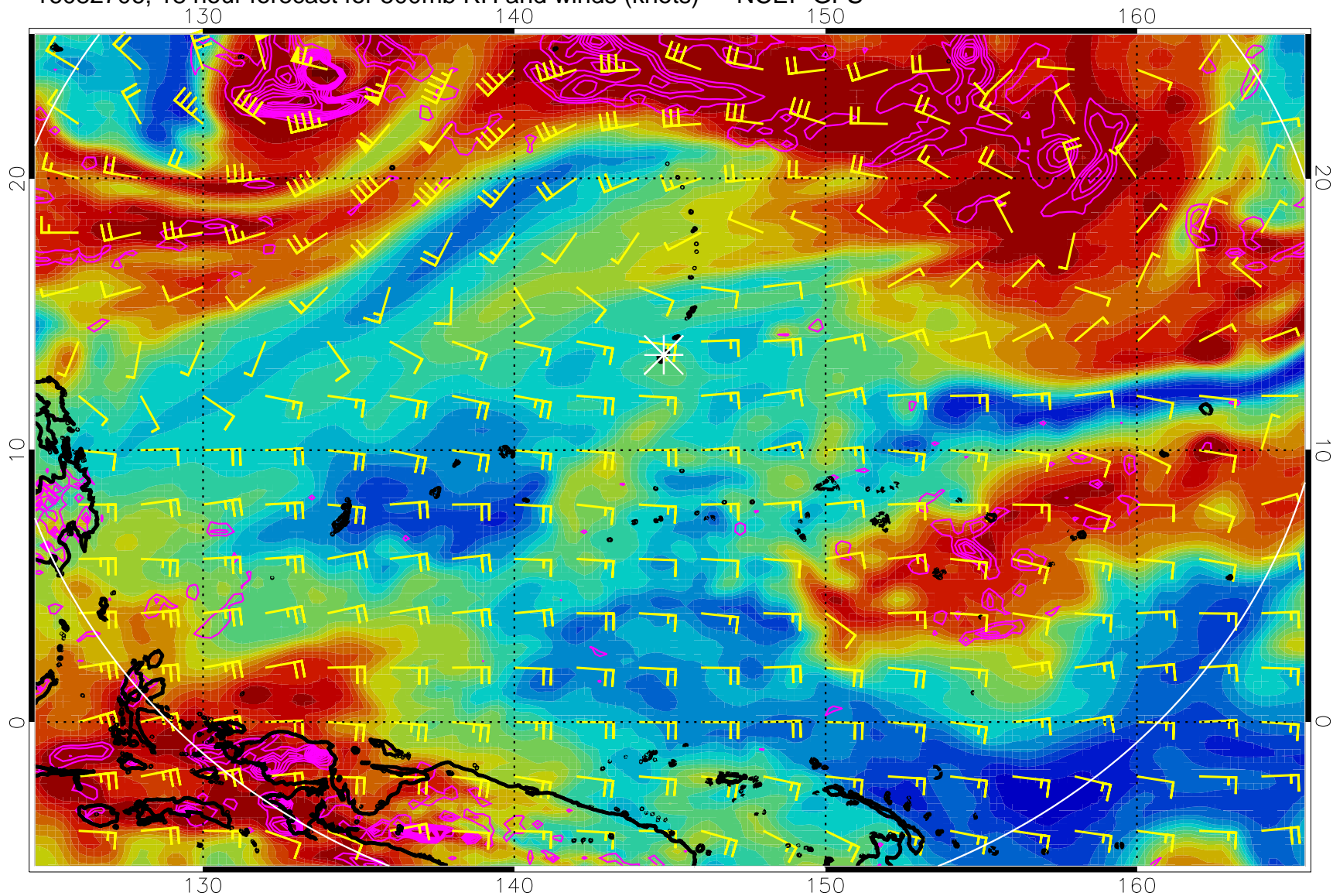
16082706, 18 hour forecast for 500mb RH and winds (knots) -- NCEP GFS
