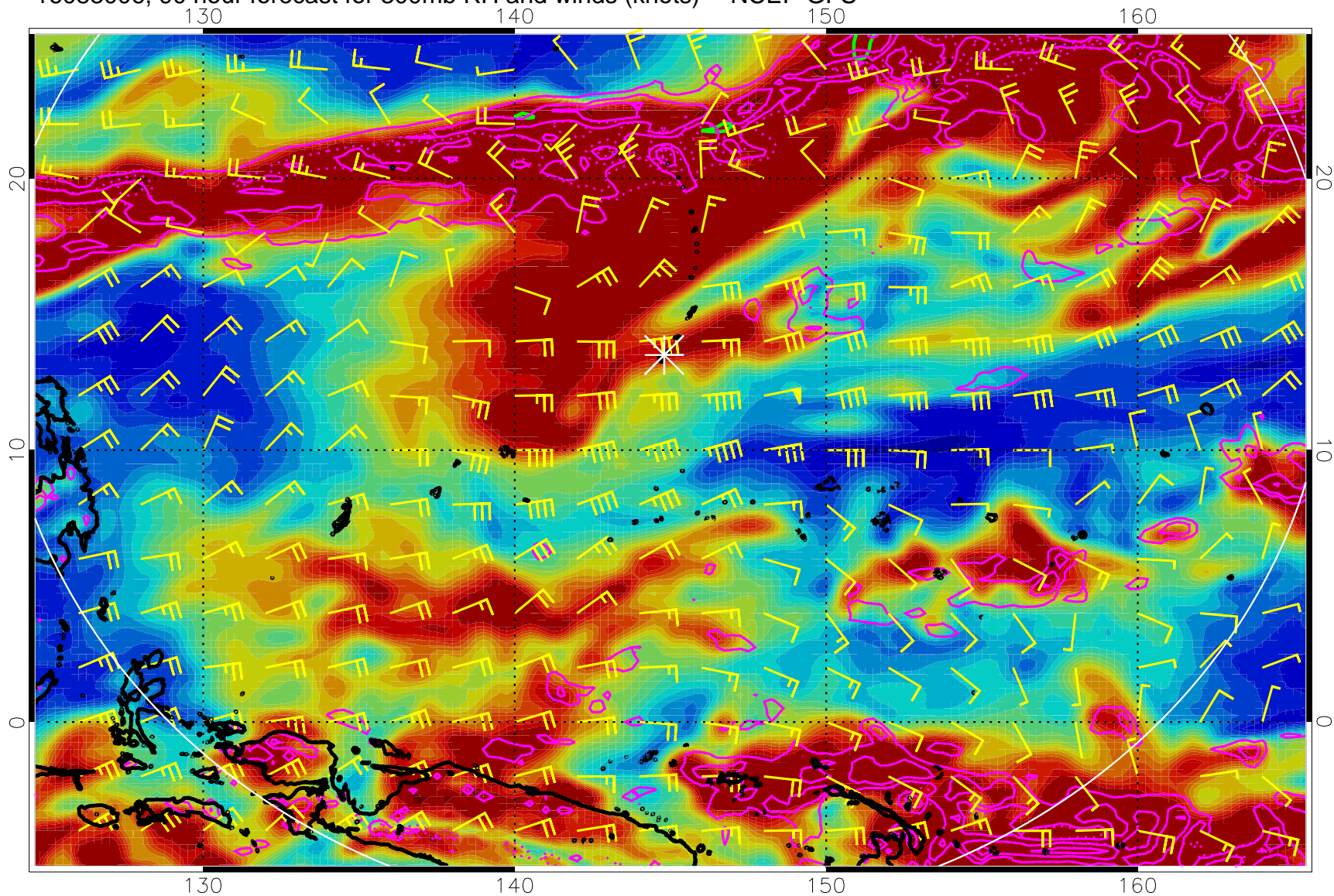
16083006, 90 hour forecast for 300mb RH and winds (knots) -- NCEP GFS
