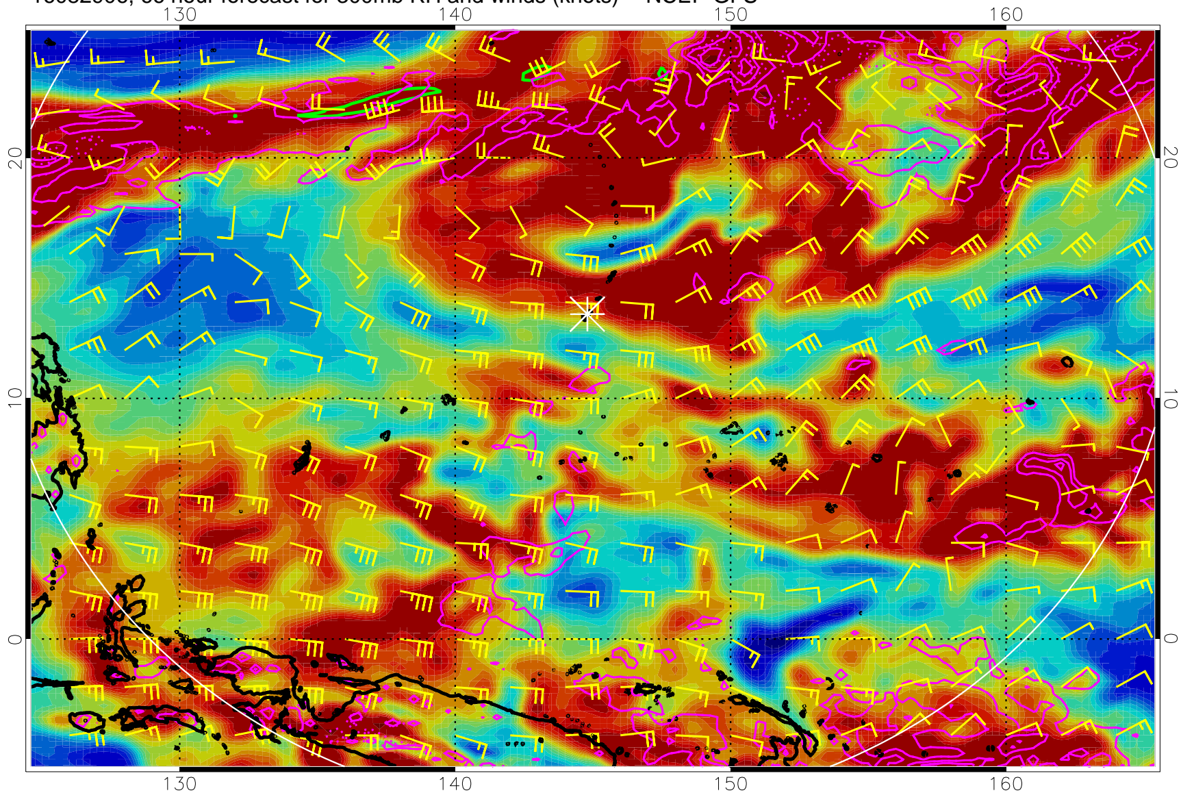
16082906, 66 hour forecast for 300mb RH and winds (knots) -- NCEP GFS
