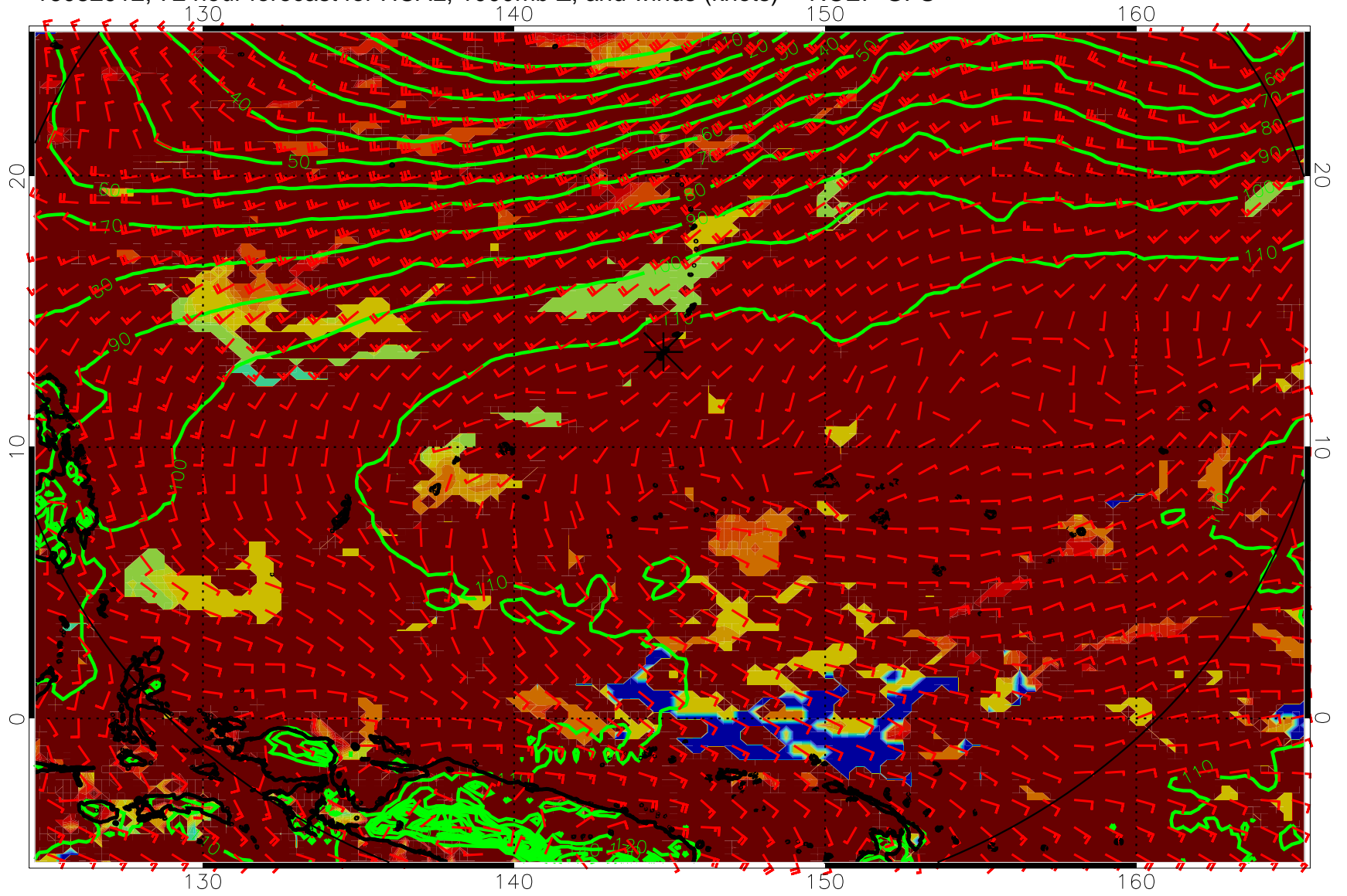
16082912, 72 hour forecast for HCAL, 1000mb Z, and winds (knots) -- NCEP GFS
