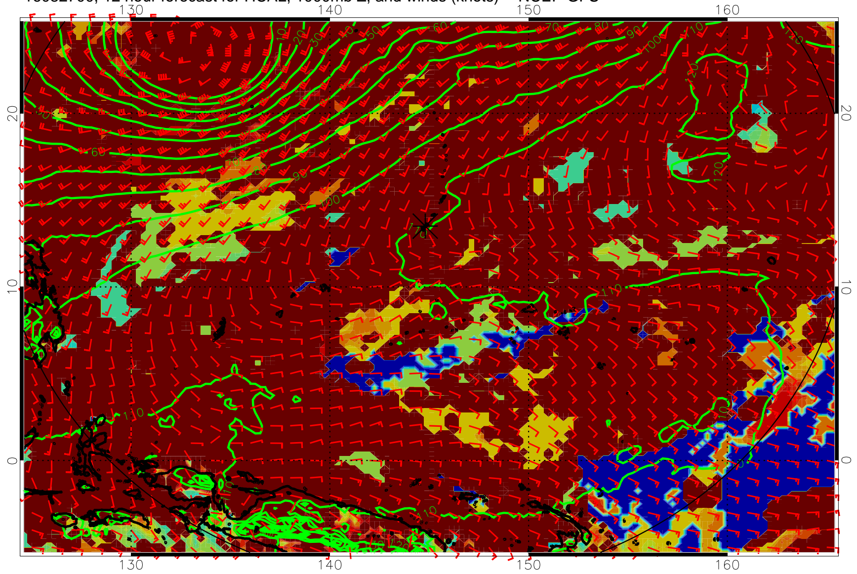
16082700, 12 hour forecast for HCAL, 1000mb Z, and winds (knots) -- NCEP GFS
