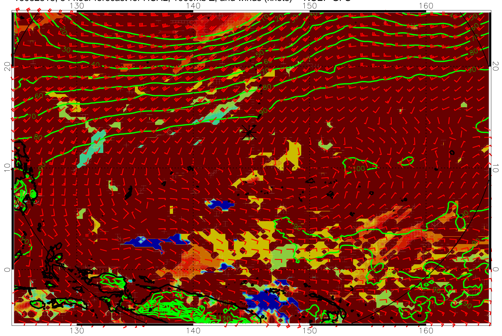
16082818, 54 hour forecast for HCAL, 1000mb Z, and winds (knots) -- NCEP GFS
