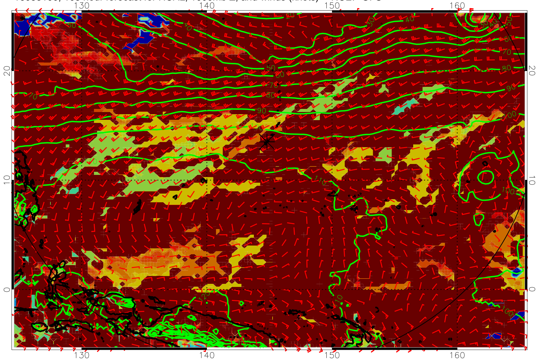
16083100, 108 hour forecast for HCAL, 1000mb Z, and winds (knots) -- NCEP GFS
