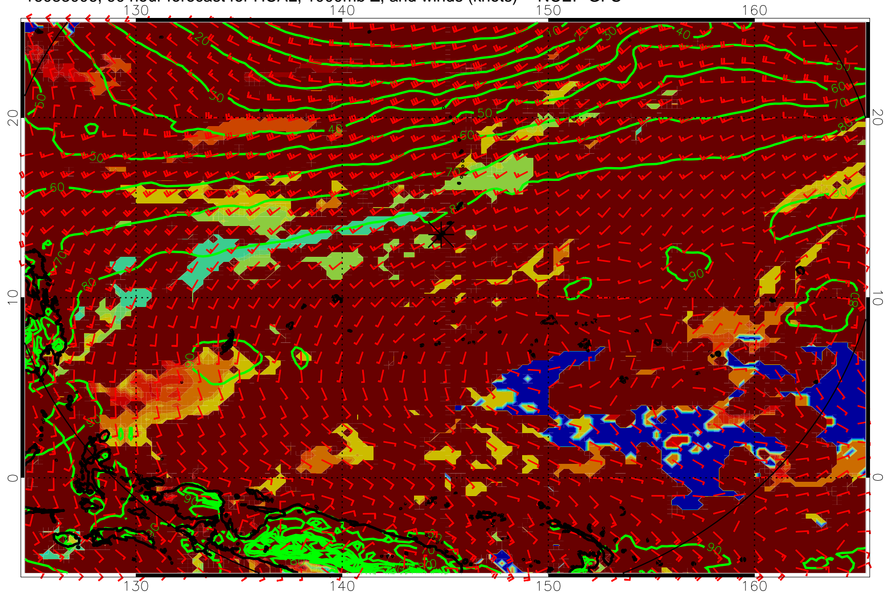
16083006, 90 hour forecast for HCAL, 1000mb Z, and winds (knots) -- NCEP GFS
