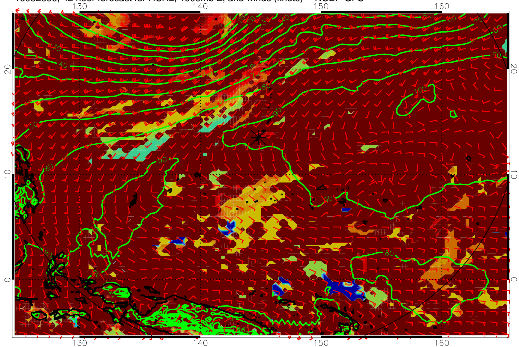
16082806, 42 hour forecast for HCAL, 1000mb Z, and winds (knots) -- NCEP GFS
