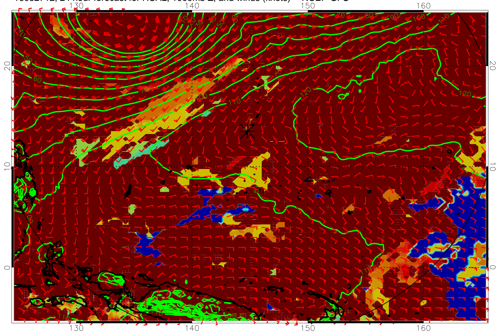
16082712, 24 hour forecast for HCAL, 1000mb Z, and winds (knots) -- NCEP GFS
