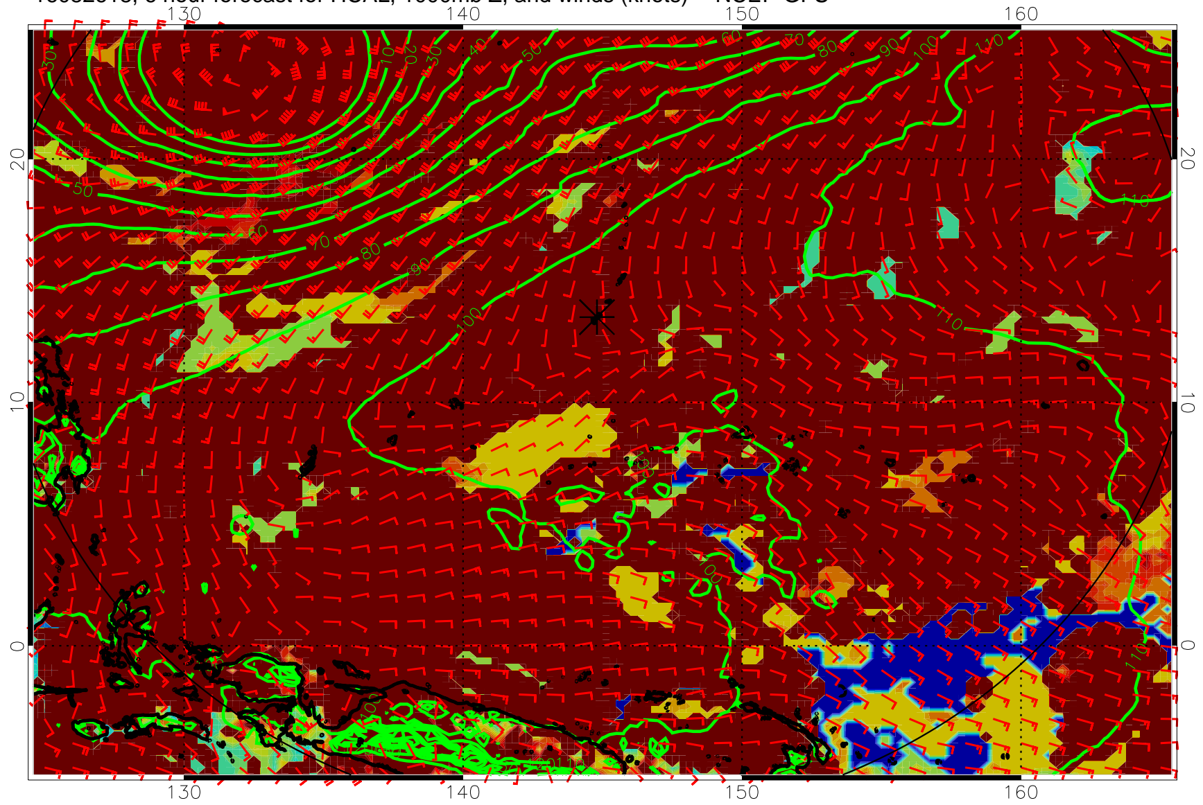
16082618, 6 hour forecast for HCAL, 1000mb Z, and winds (knots) -- NCEP GFS
