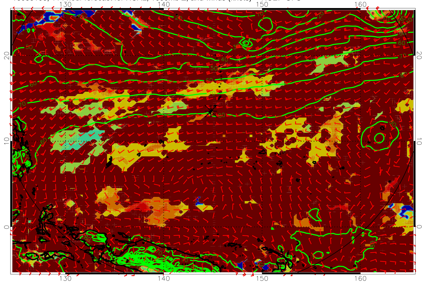
16083106, 114 hour forecast for HCAL, 1000mb Z, and winds (knots) -- NCEP GFS
