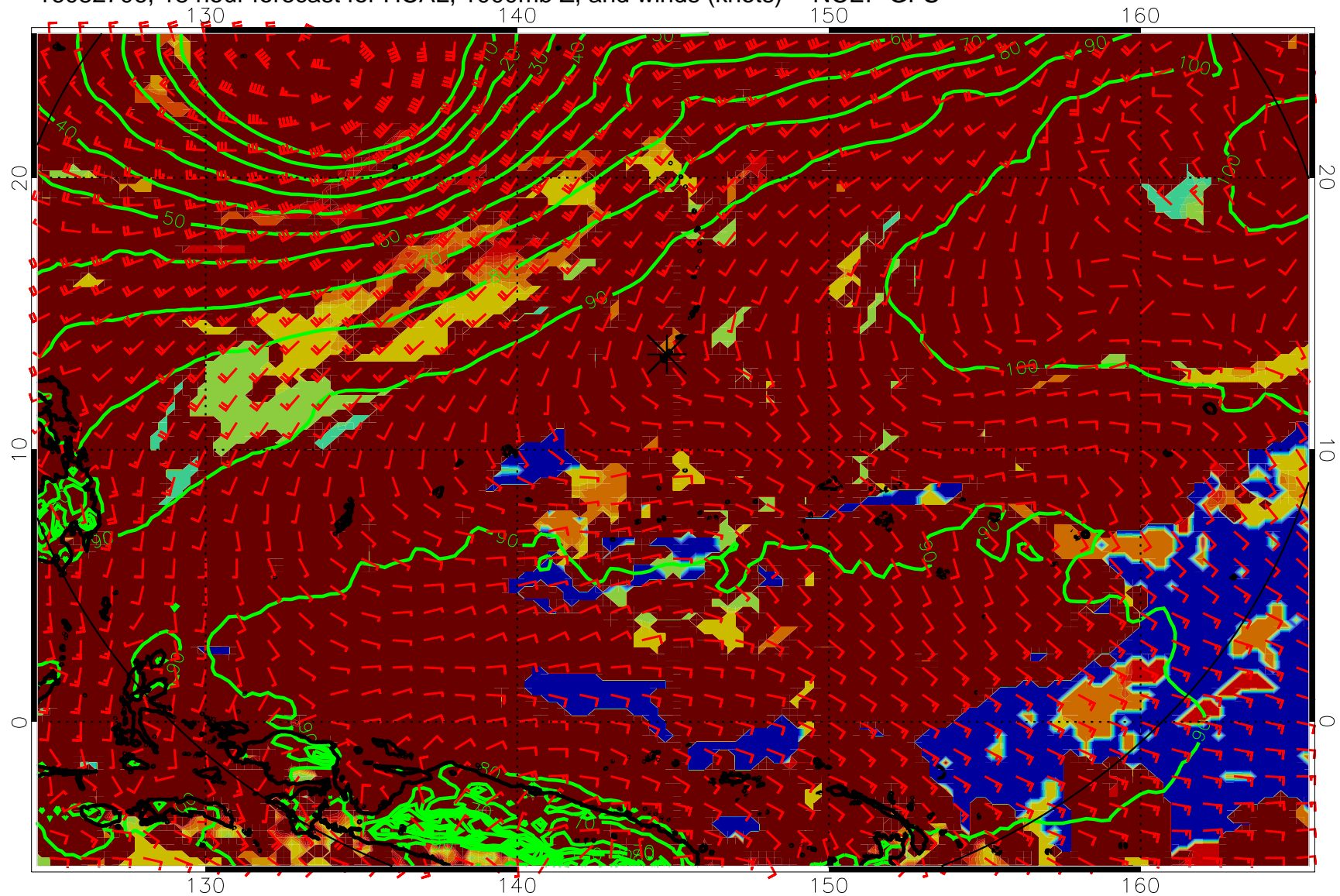
16082706, 18 hour forecast for HCAL, 1000mb Z, and winds (knots) -- NCEP GFS
