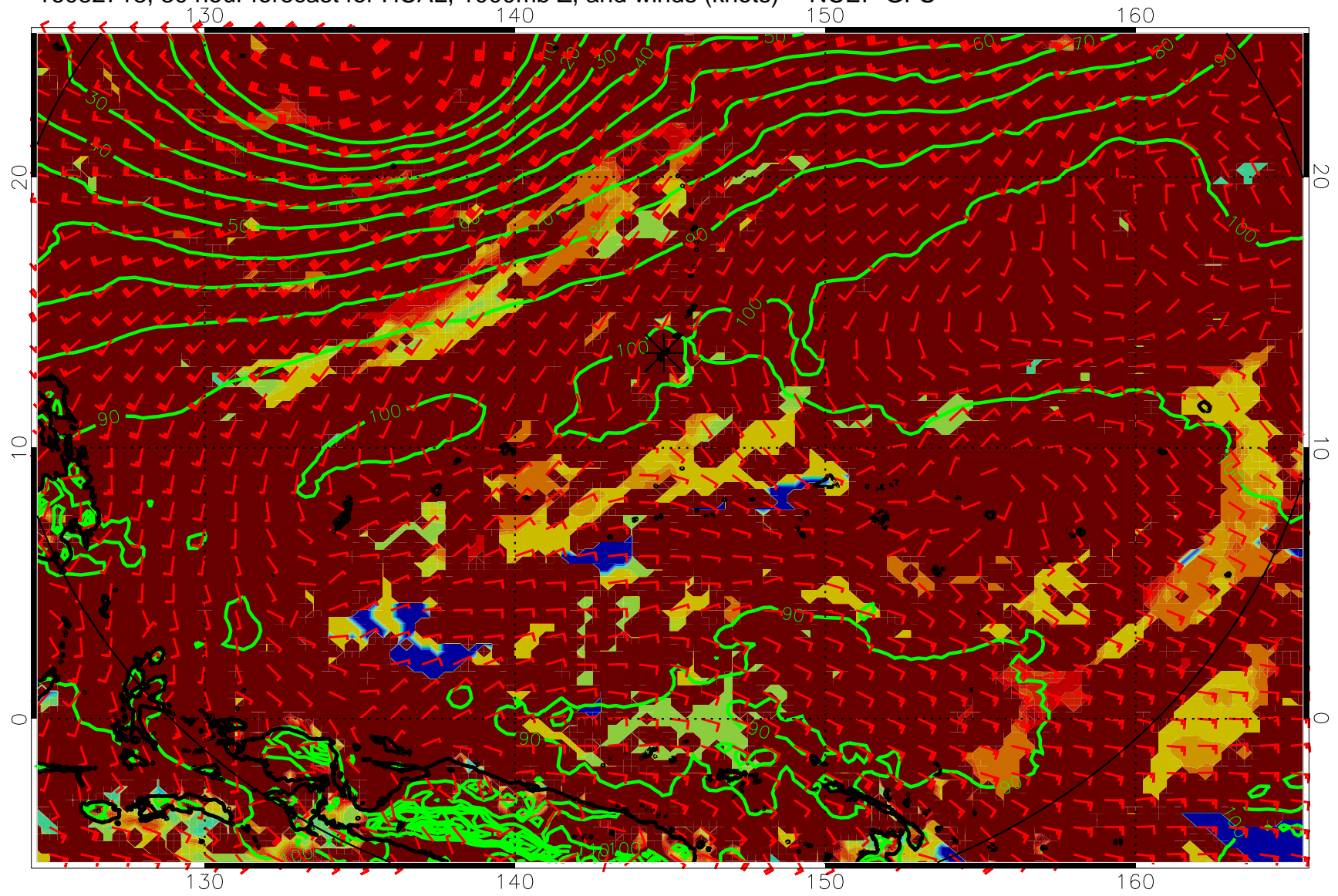
16082718, 30 hour forecast for HCAL, 1000mb Z, and winds (knots) -- NCEP GFS
