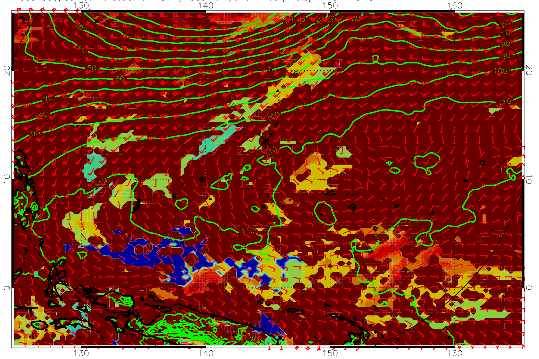
16082900, 60 hour forecast for HCAL, 1000mb Z, and winds (knots) -- NCEP GFS
