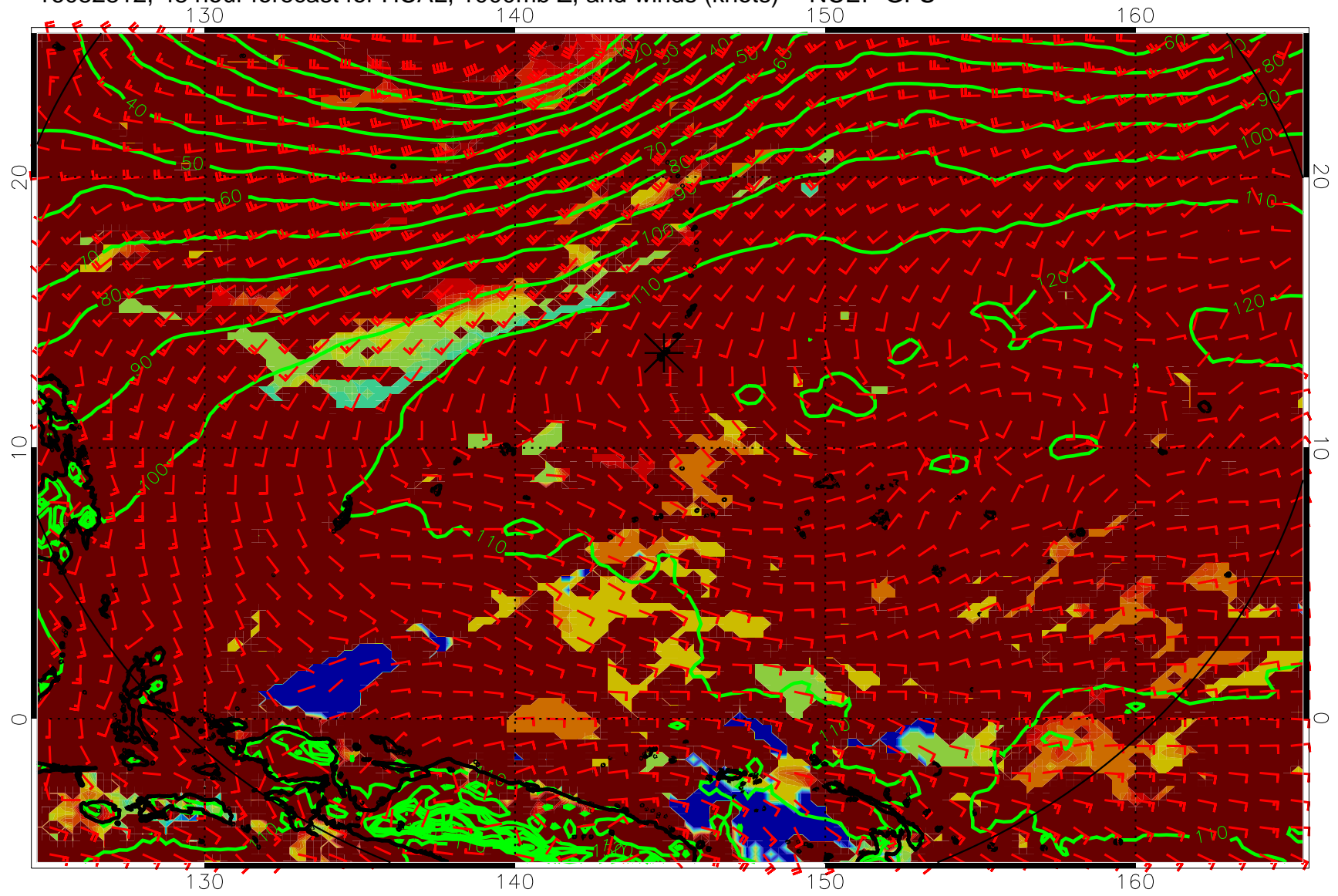
16082812, 48 hour forecast for HCAL, 1000mb Z, and winds (knots) -- NCEP GFS
