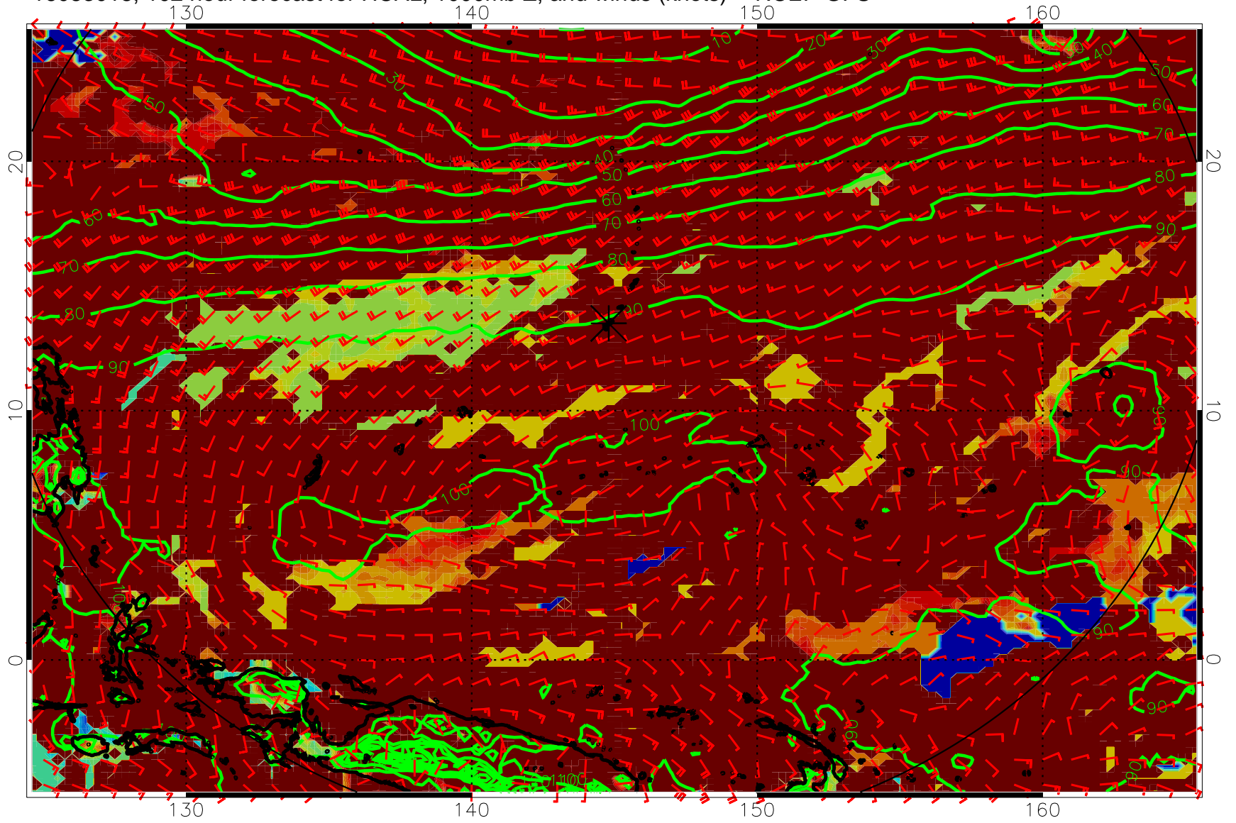
16083018, 102 hour forecast for HCAL, 1000mb Z, and winds (knots) -- NCEP GFS
