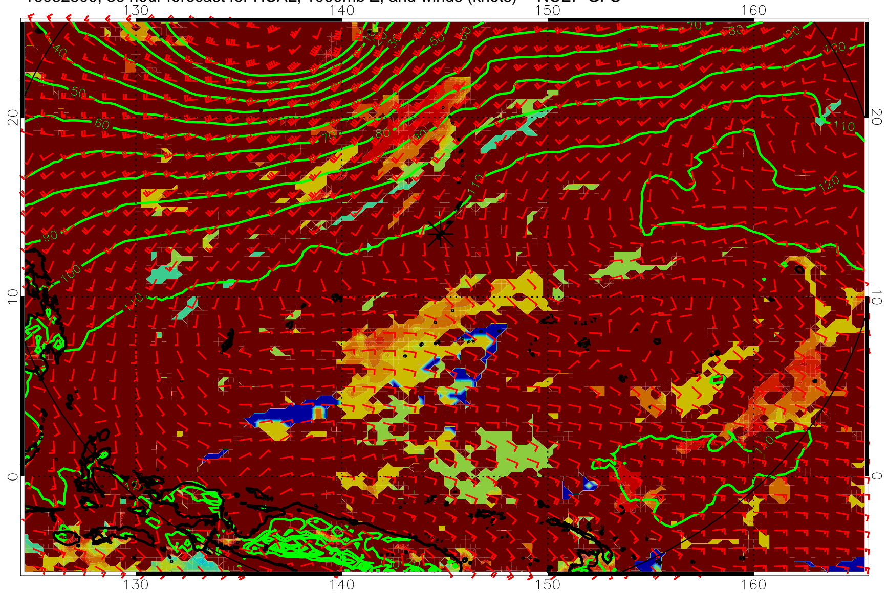
16082800, 36 hour forecast for HCAL, 1000mb Z, and winds (knots) -- NCEP GFS
