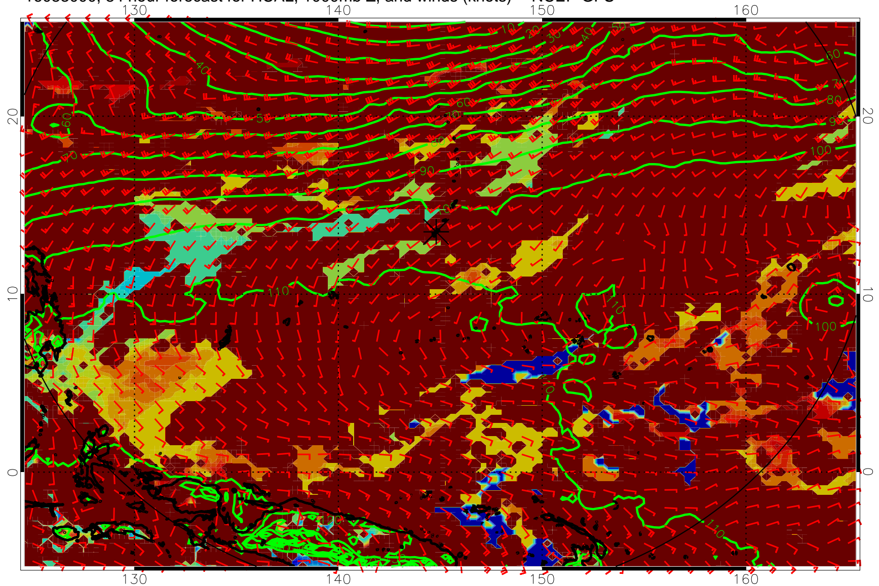
16083000, 84 hour forecast for HCAL, 1000mb Z, and winds (knots) -- NCEP GFS
