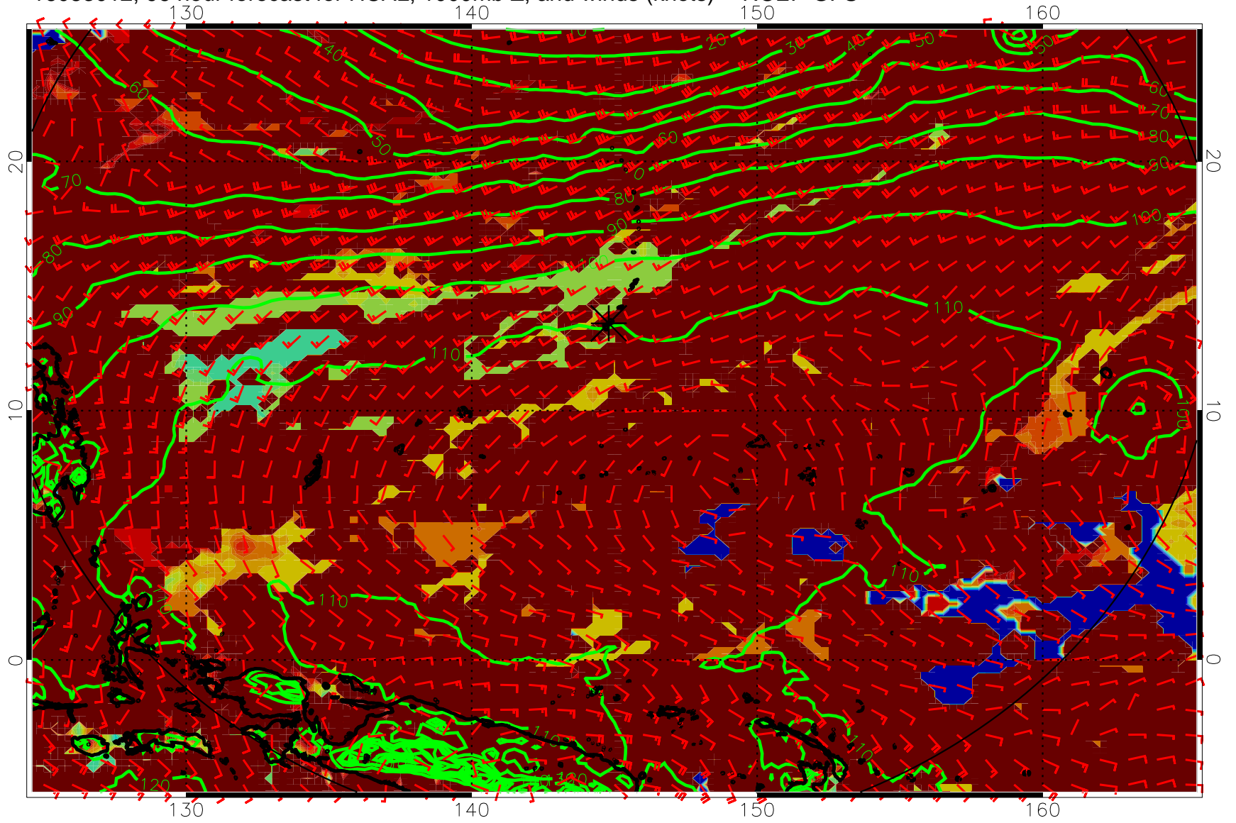
16083012, 96 hour forecast for HCAL, 1000mb Z, and winds (knots) -- NCEP GFS
