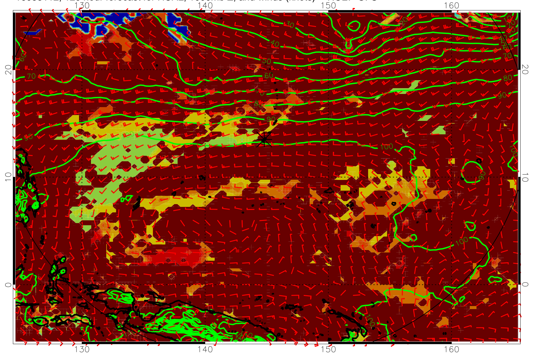
16083112, 120 hour forecast for HCAL, 1000mb Z, and winds (knots) -- NCEP GFS
