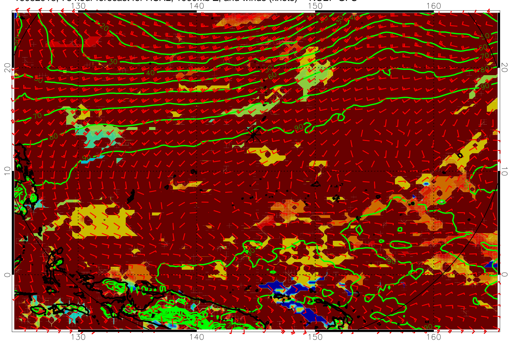
16082918, 78 hour forecast for HCAL, 1000mb Z, and winds (knots) -- NCEP GFS
