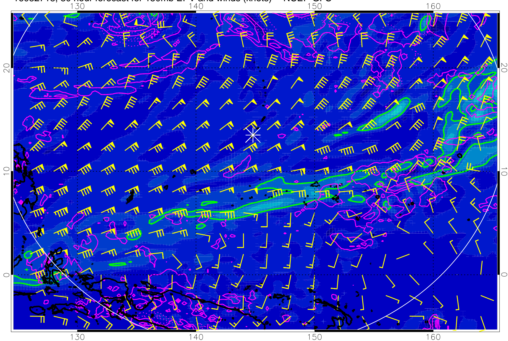
16082718, 30 hour forecast for 150mb EPV and winds (knots) -- NCEP GFS
