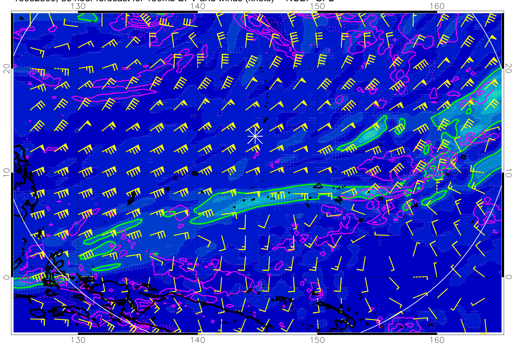
16082800, 36 hour forecast for 150mb EPV and winds (knots) -- NCEP GFS
