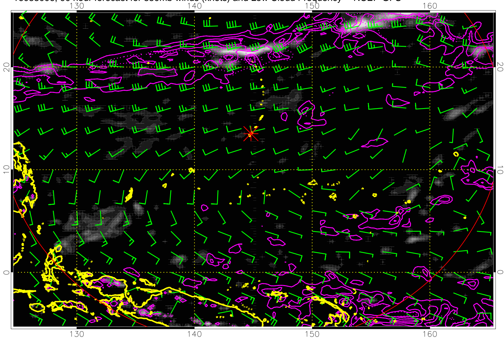
16083006, 90 hour forecast for 850mb winds (knots) and Low Cloud Frequency -- NCEP GFS
