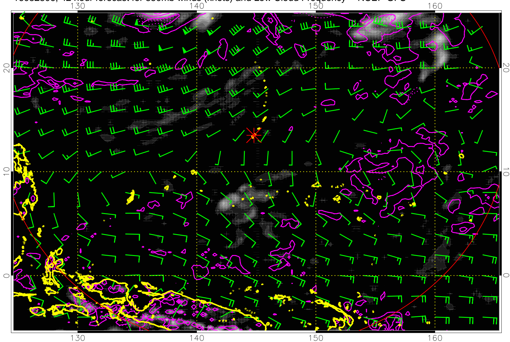
16082806, 42 hour forecast for 850mb winds (knots) and Low Cloud Frequency -- NCEP GFS
