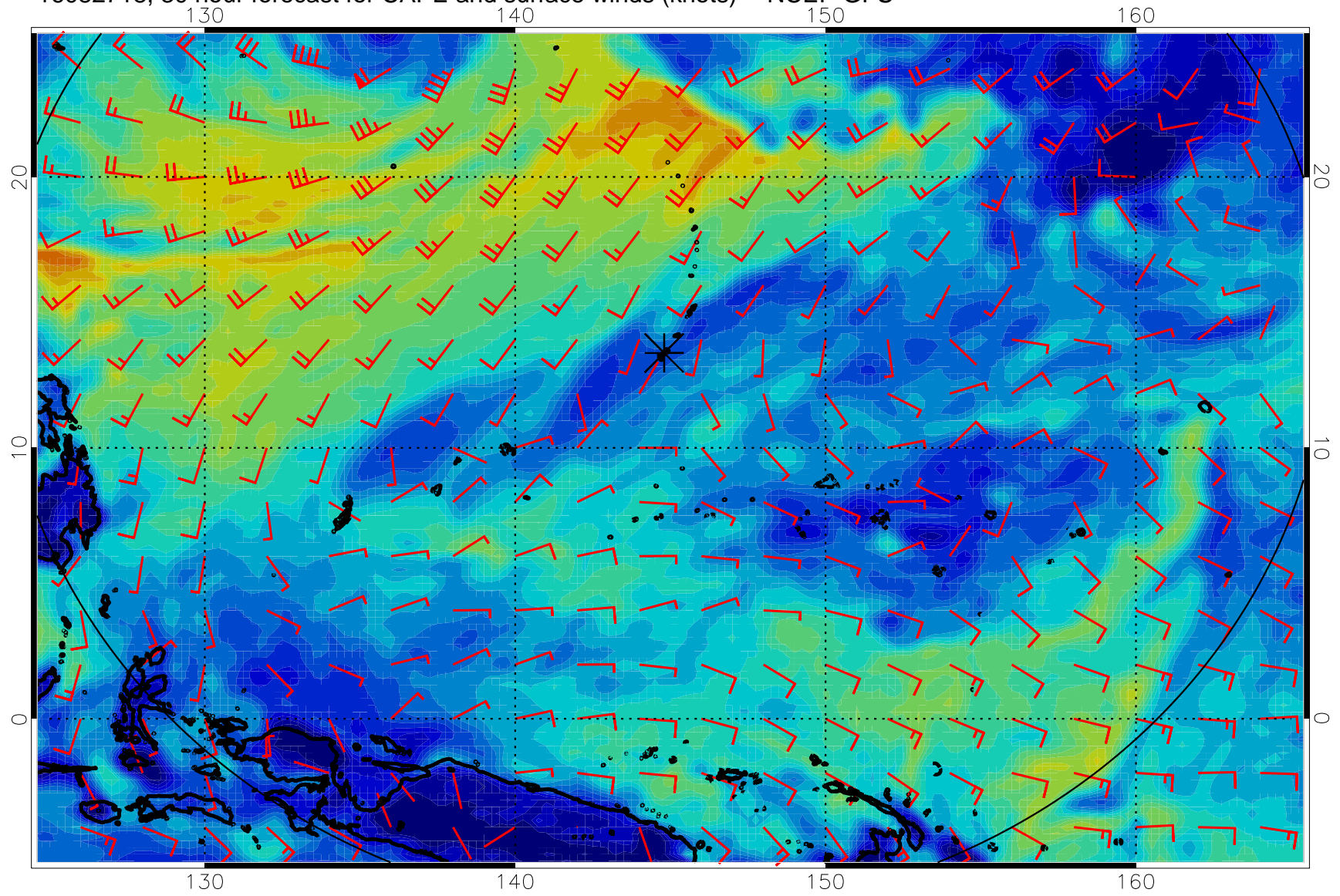
16082718, 30 hour forecast for CAPE and surface winds (knots) -- NCEP GFS
