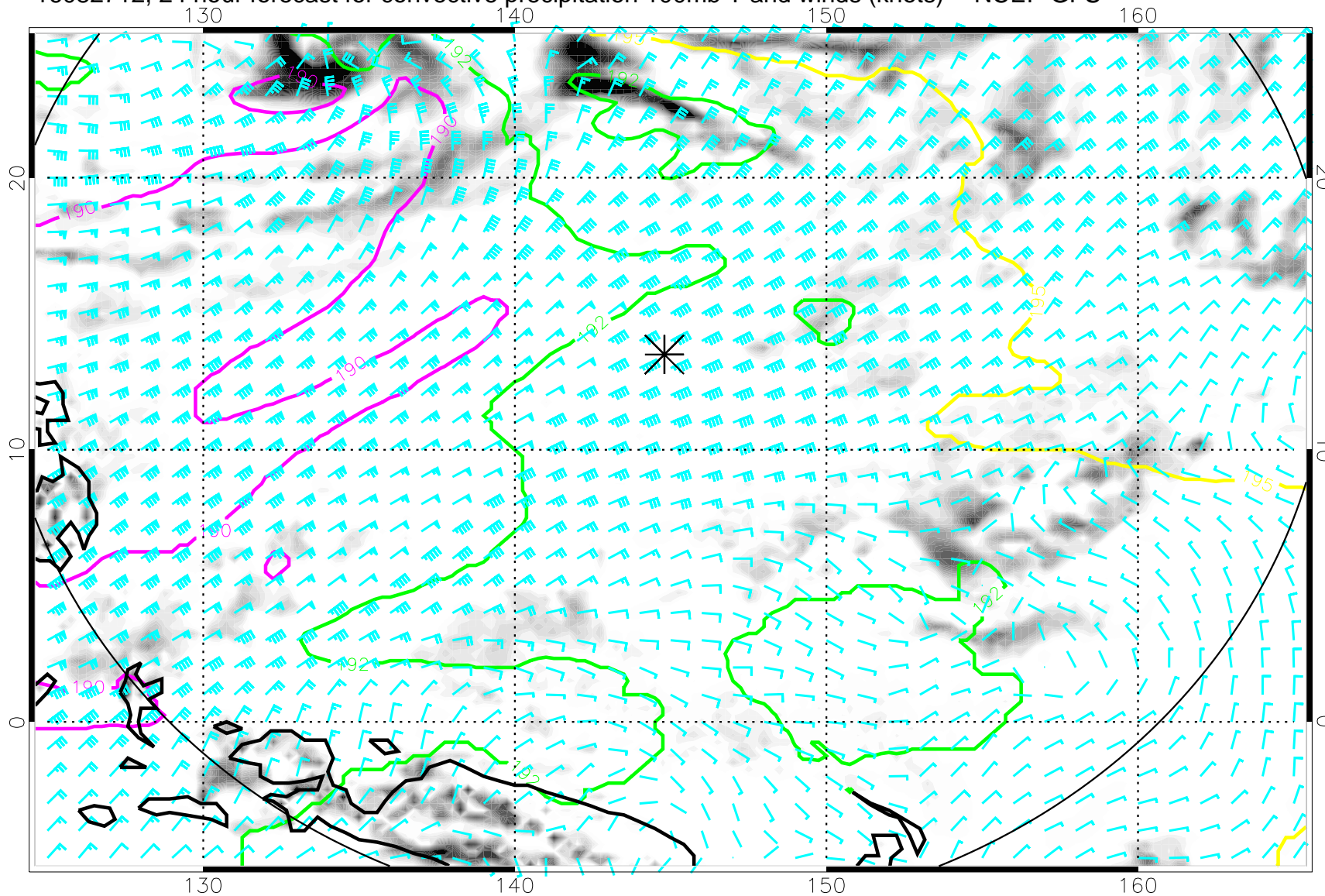
16082712, 24 hour forecast for convective precipitation 100mb T and winds (knots) -- NCEP GFS
