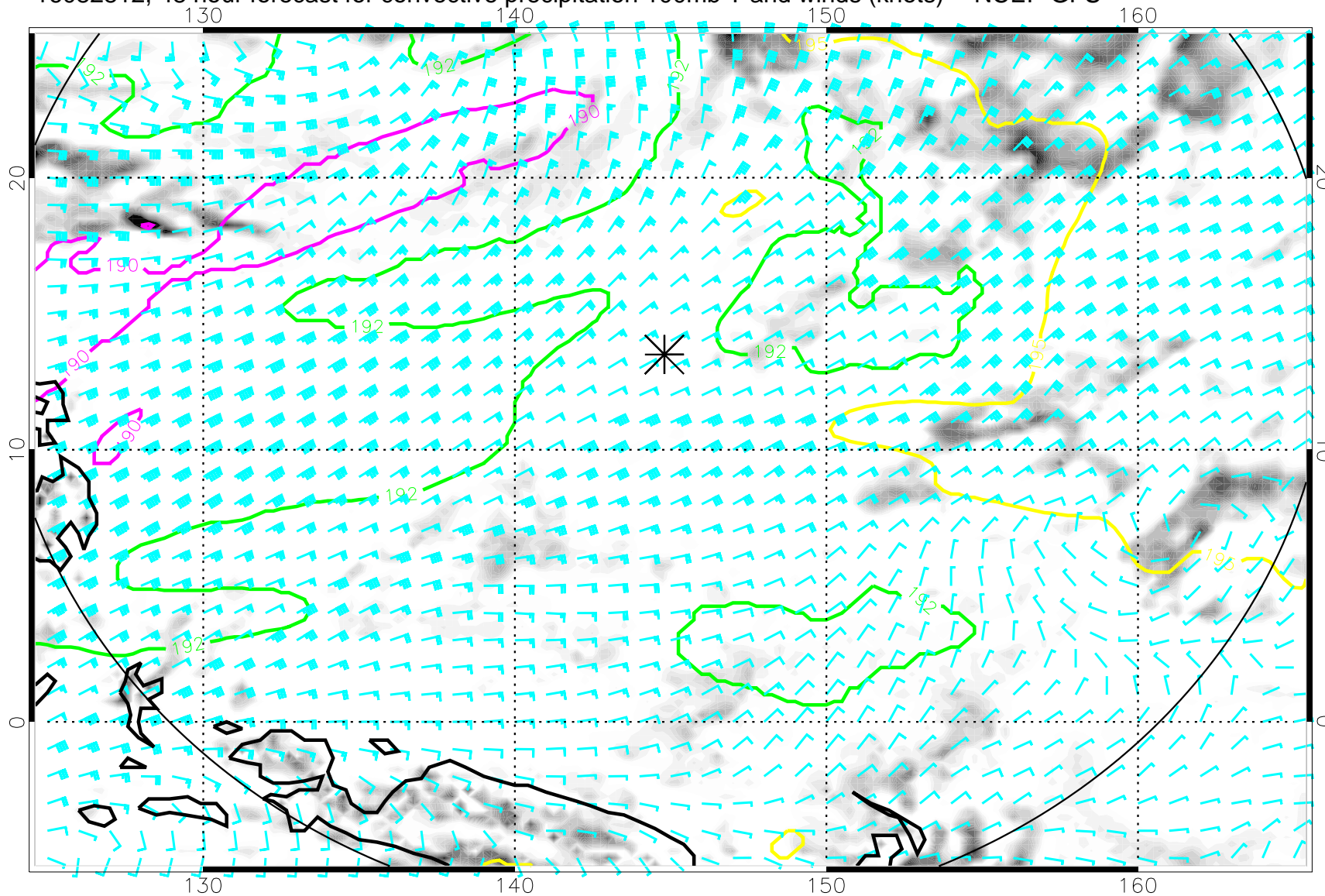
16082812, 48 hour forecast for convective precipitation 100mb T and winds (knots) -- NCEP GFS
