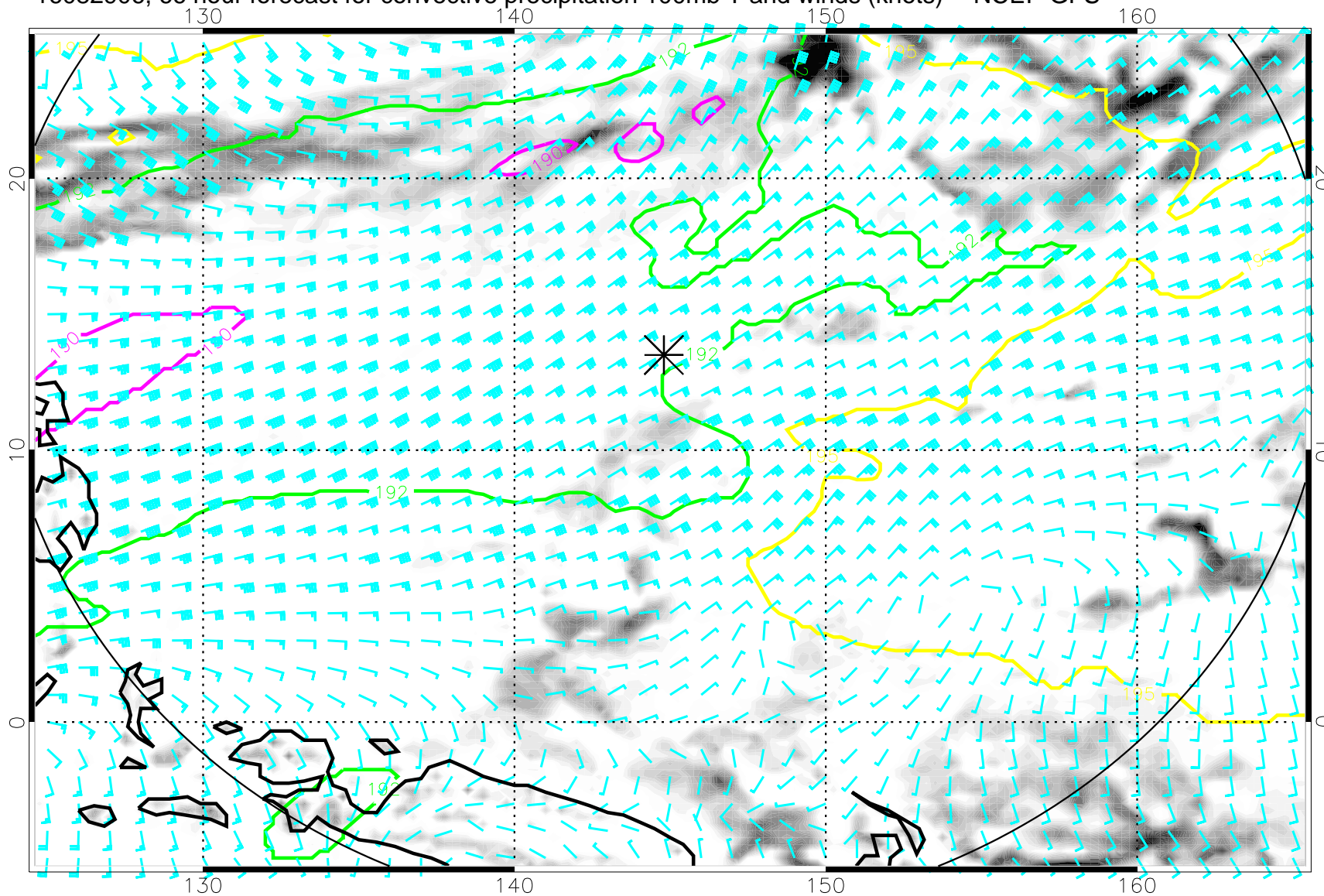
16082906, 66 hour forecast for convective precipitation 100mb T and winds (knots) -- NCEP GFS
