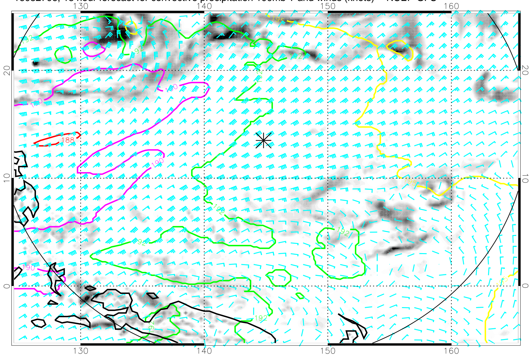
16082706, 18 hour forecast for convective precipitation 100mb T and winds (knots) -- NCEP GFS
