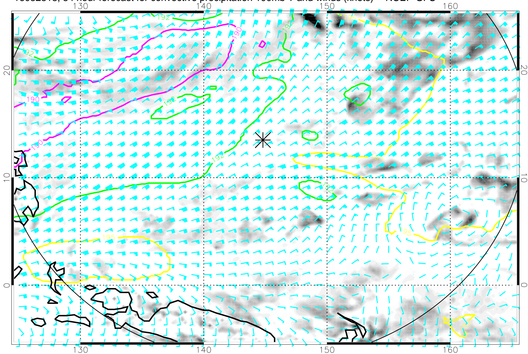
16082818, 54 hour forecast for convective precipitation 100mb T and winds (knots) -- NCEP GFS
