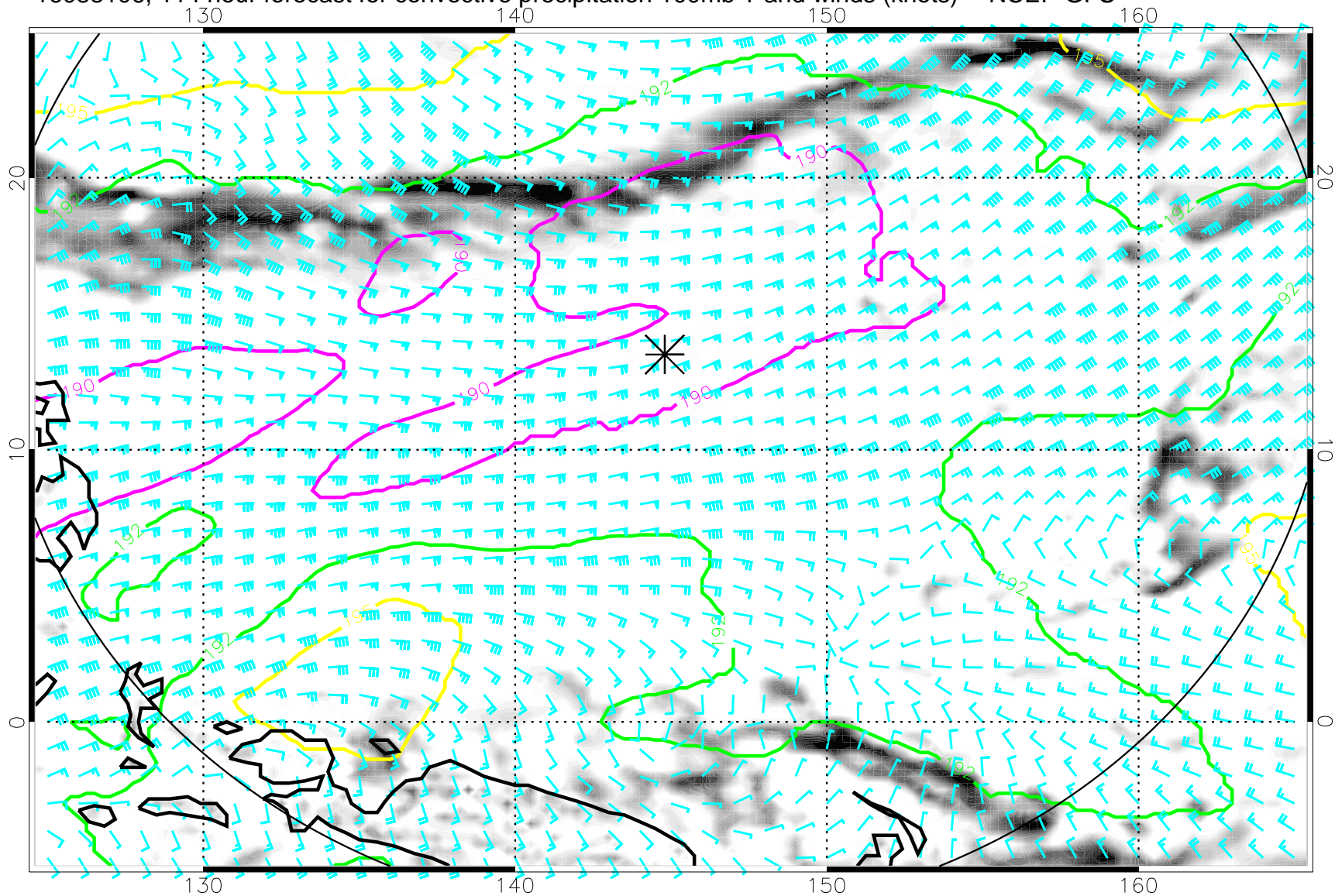
16083106, 114 hour forecast for convective precipitation 100mb T and winds (knots) -- NCEP GFS
