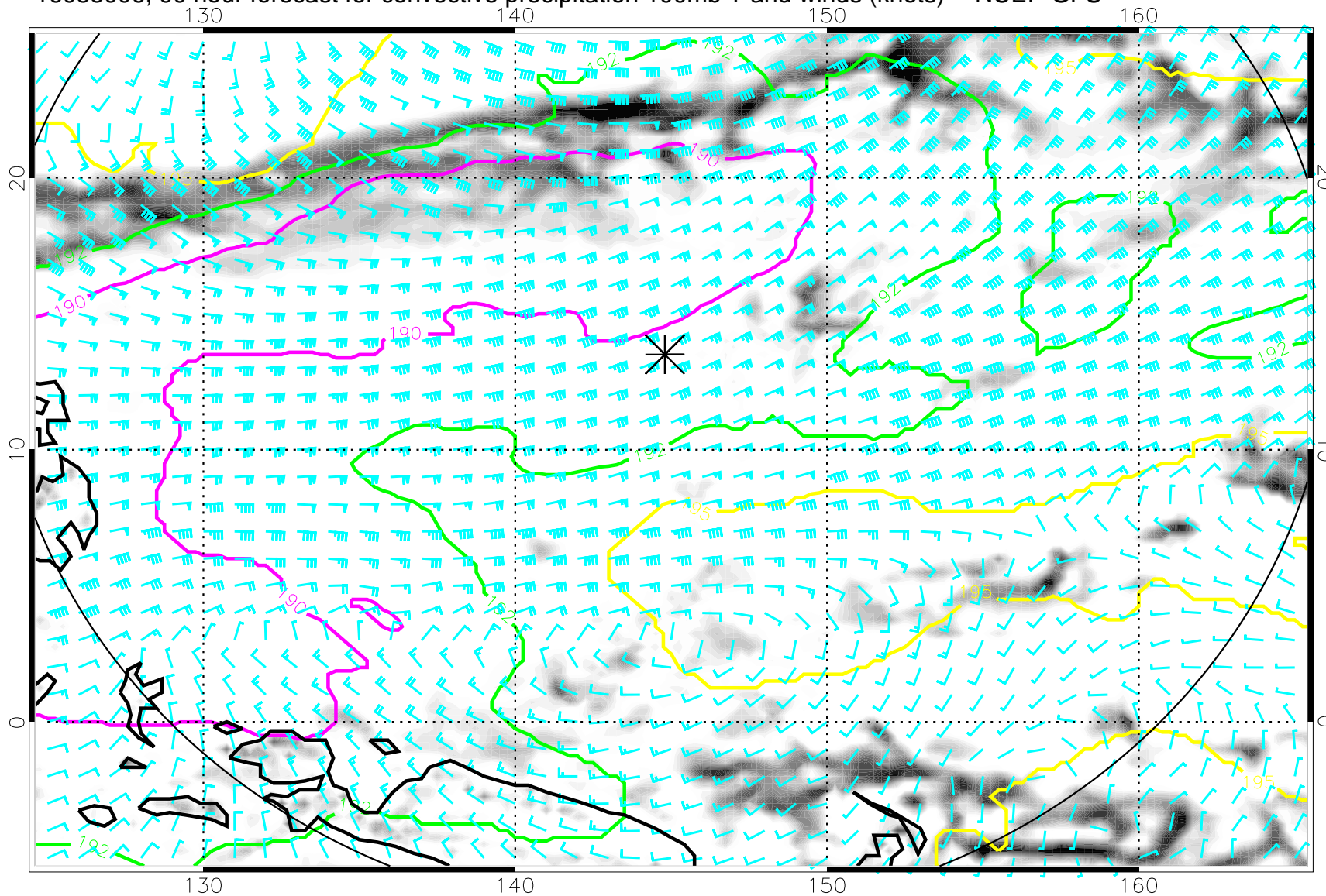
16083006, 90 hour forecast for convective precipitation 100mb T and winds (knots) -- NCEP GFS
