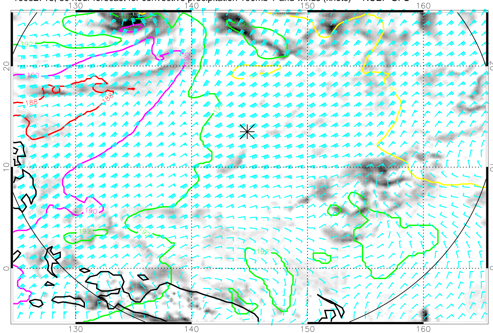
16082718, 30 hour forecast for convective precipitation 100mb T and winds (knots) -- NCEP GFS
