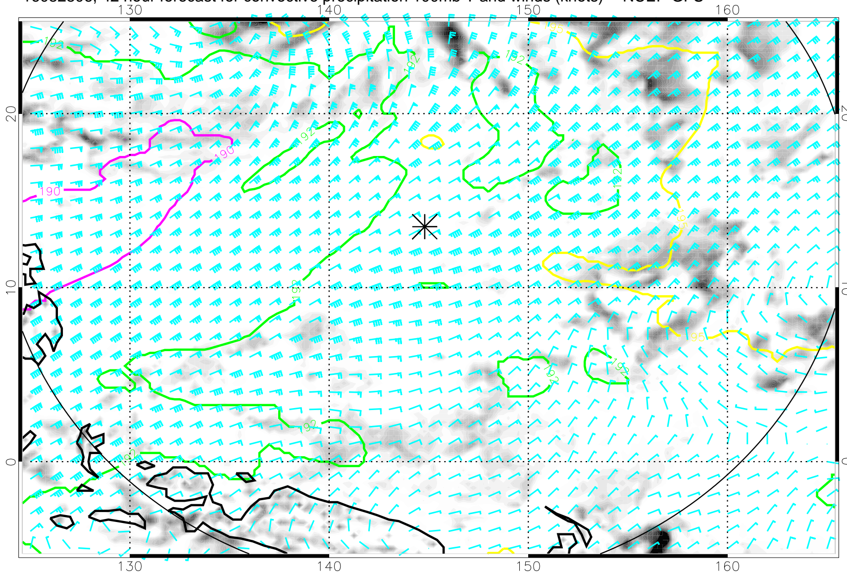
16082806, 42 hour forecast for convective precipitation 100mb T and winds (knots) -- NCEP GFS
