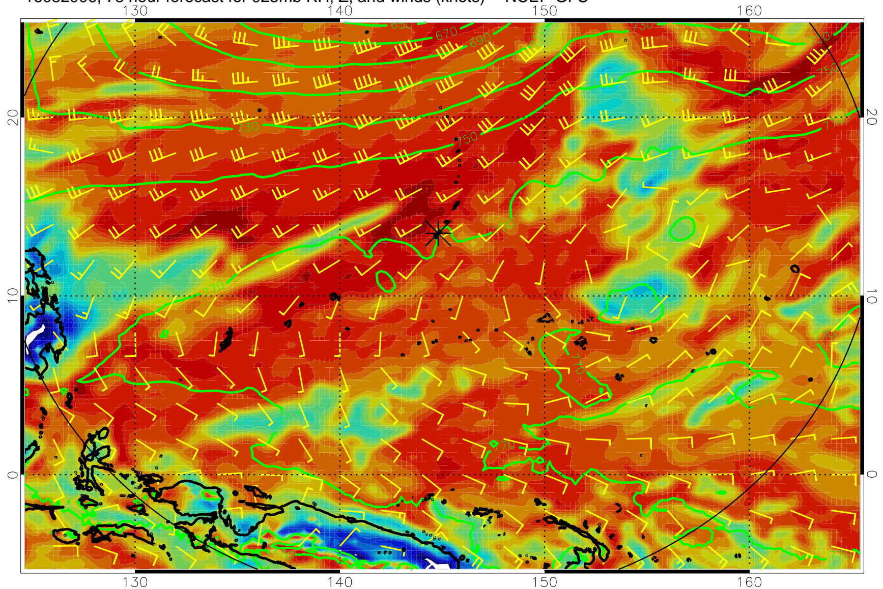
16082906, 78 hour forecast for 925mb RH, Z, and winds (knots) -- NCEP GFS
