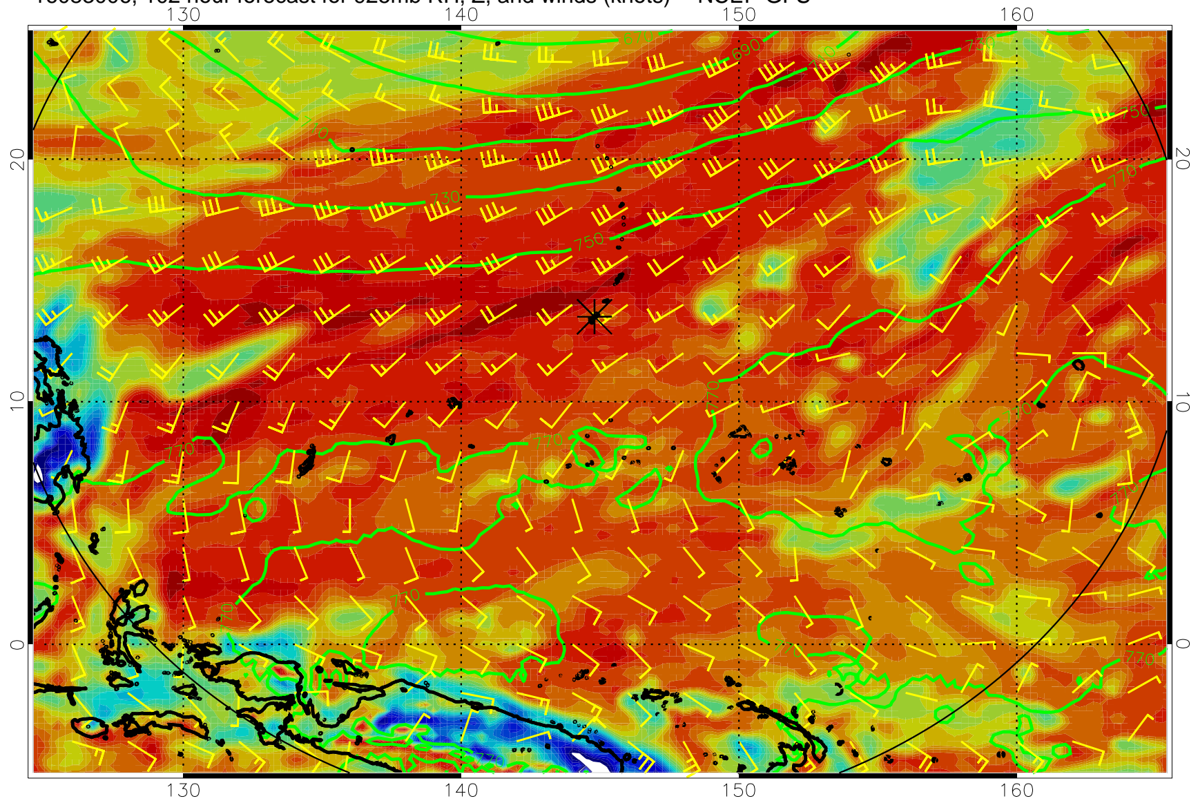
16083006, 102 hour forecast for 925mb RH, Z, and winds (knots) -- NCEP GFS
