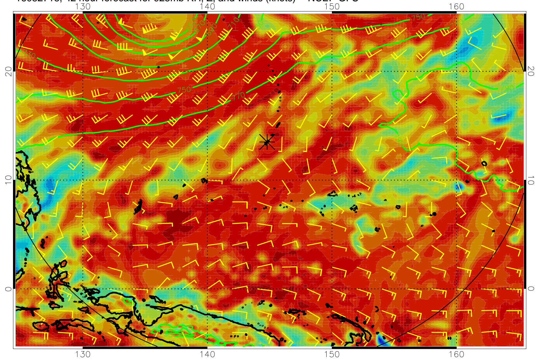
16082718, 42 hour forecast for 925mb RH, Z, and winds (knots) -- NCEP GFS
