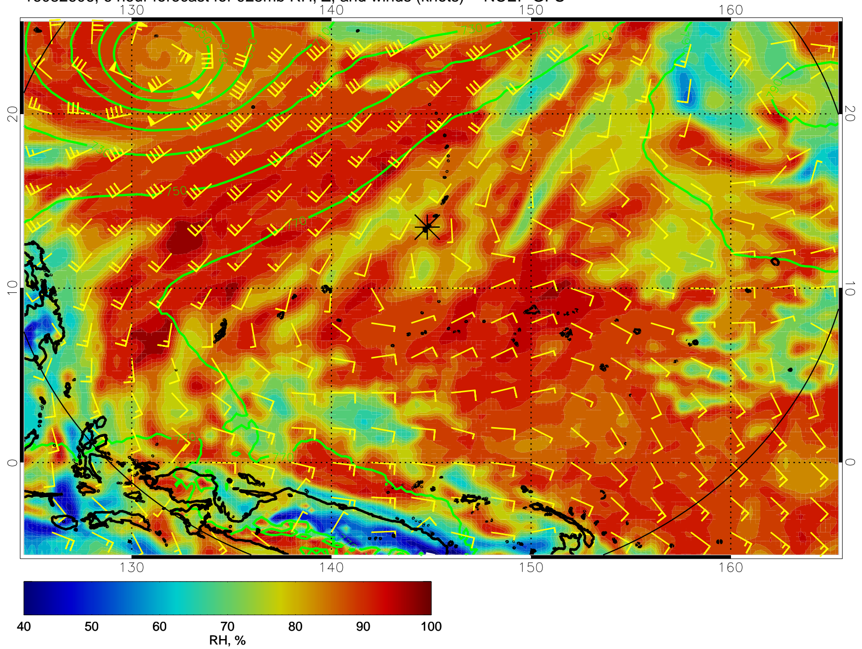
16082606, 6 hour forecast for 925mb RH, Z, and winds (knots) -- NCEP GFS
