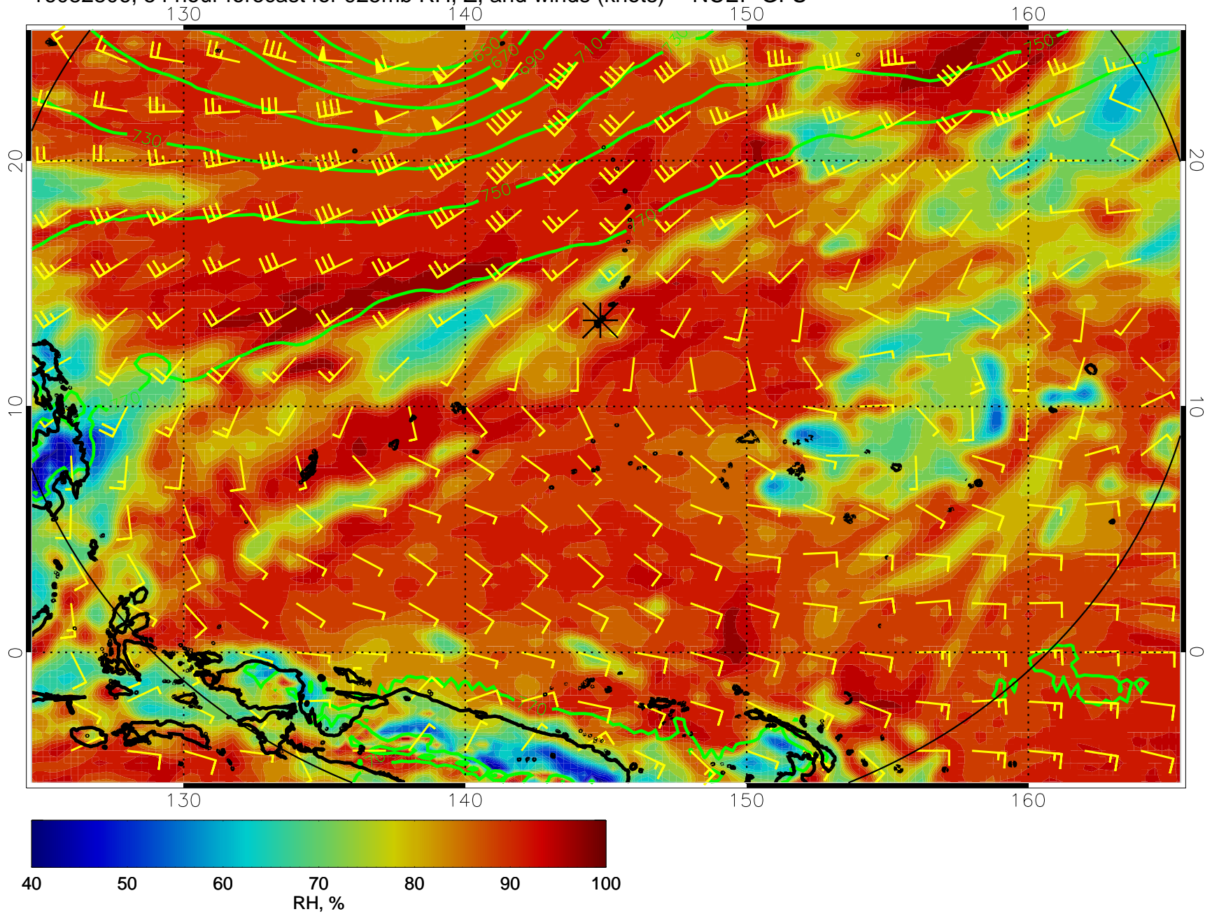
16082806, 54 hour forecast for 925mb RH, Z, and winds (knots) -- NCEP GFS
