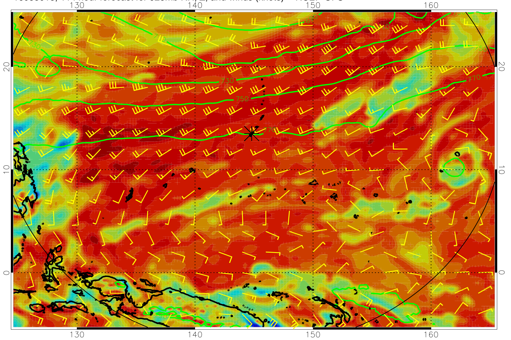
16083018, 114 hour forecast for 925mb RH, Z, and winds (knots) -- NCEP GFS
