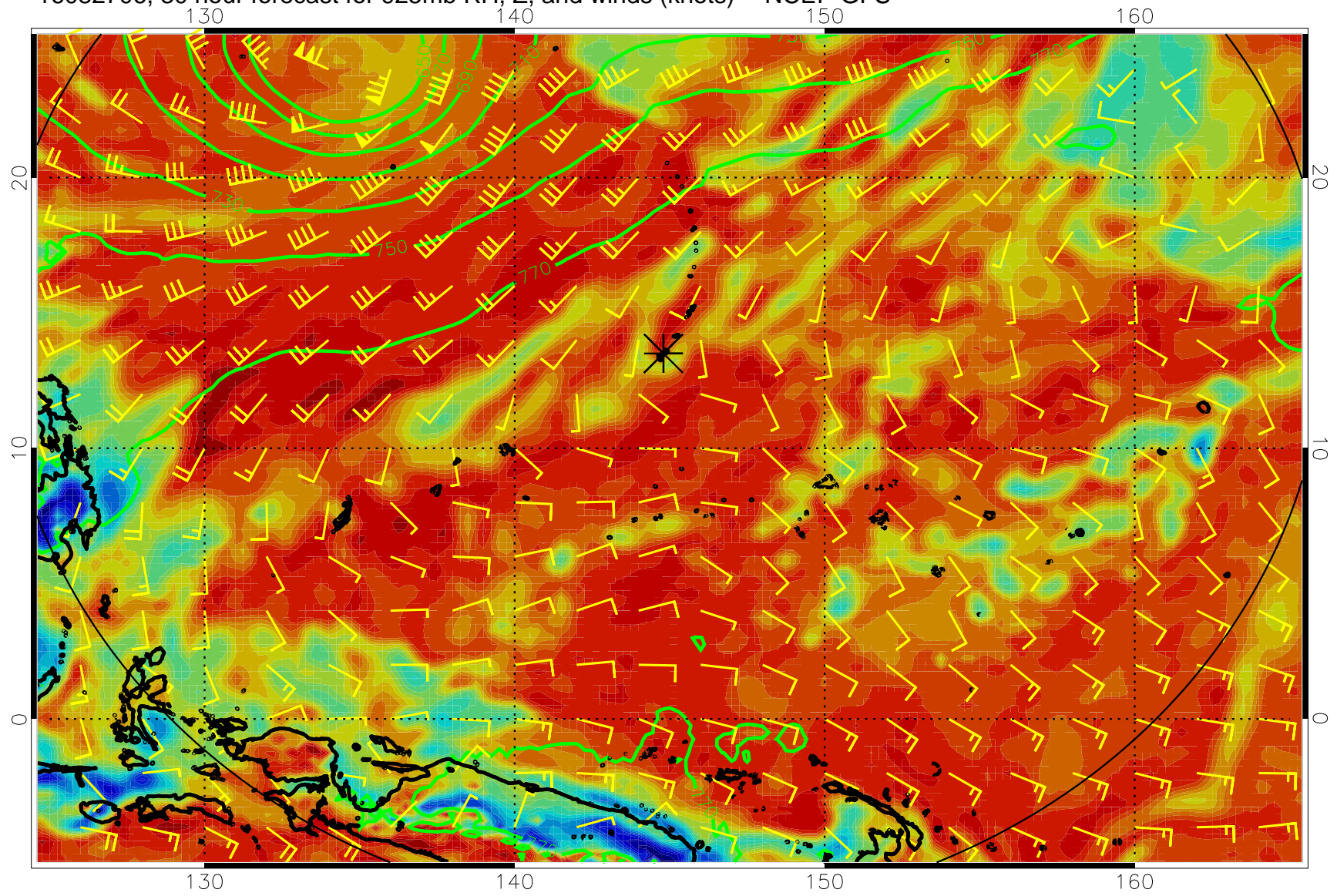
16082706, 30 hour forecast for 925mb RH, Z, and winds (knots) -- NCEP GFS
