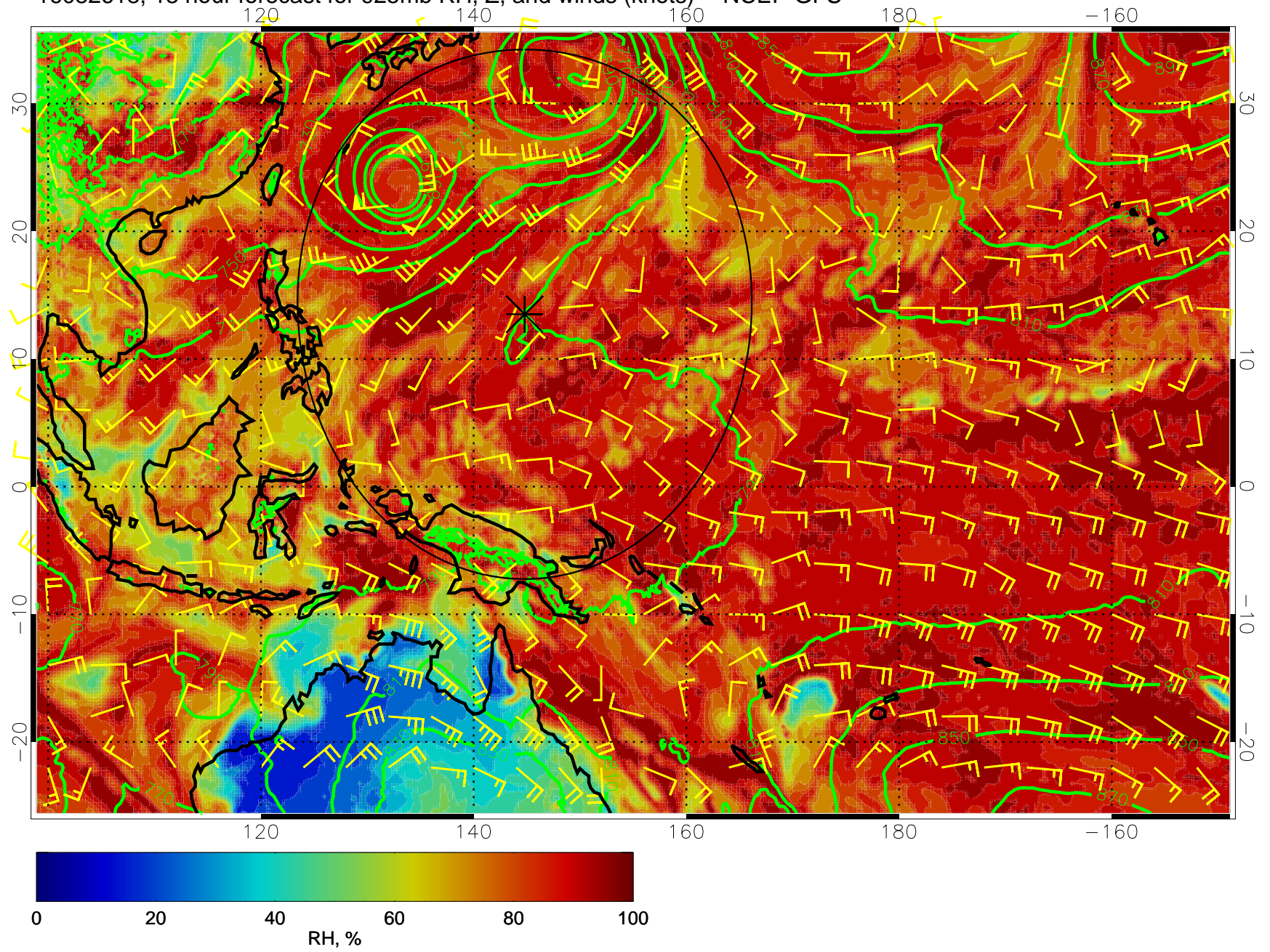
16082618, 18 hour forecast for 925mb RH, Z, and winds (knots) -- NCEP GFS
