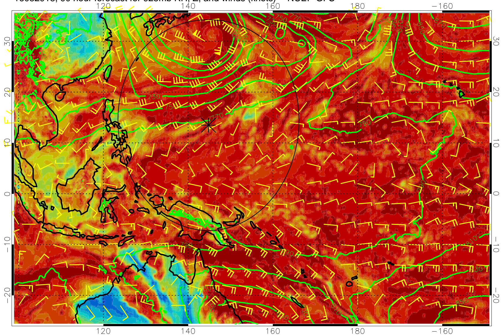
16082918, 90 hour forecast for 925mb RH, Z, and winds (knots) -- NCEP GFS
