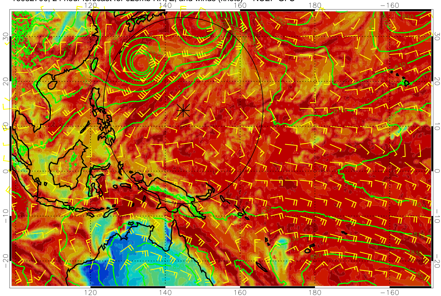
16082700, 24 hour forecast for 925mb RH, Z, and winds (knots) -- NCEP GFS
