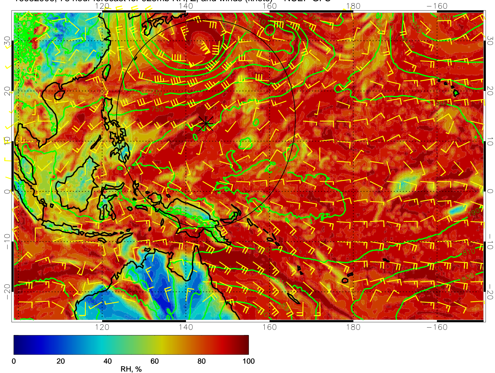
16082906, 78 hour forecast for 925mb RH, Z, and winds (knots) -- NCEP GFS
