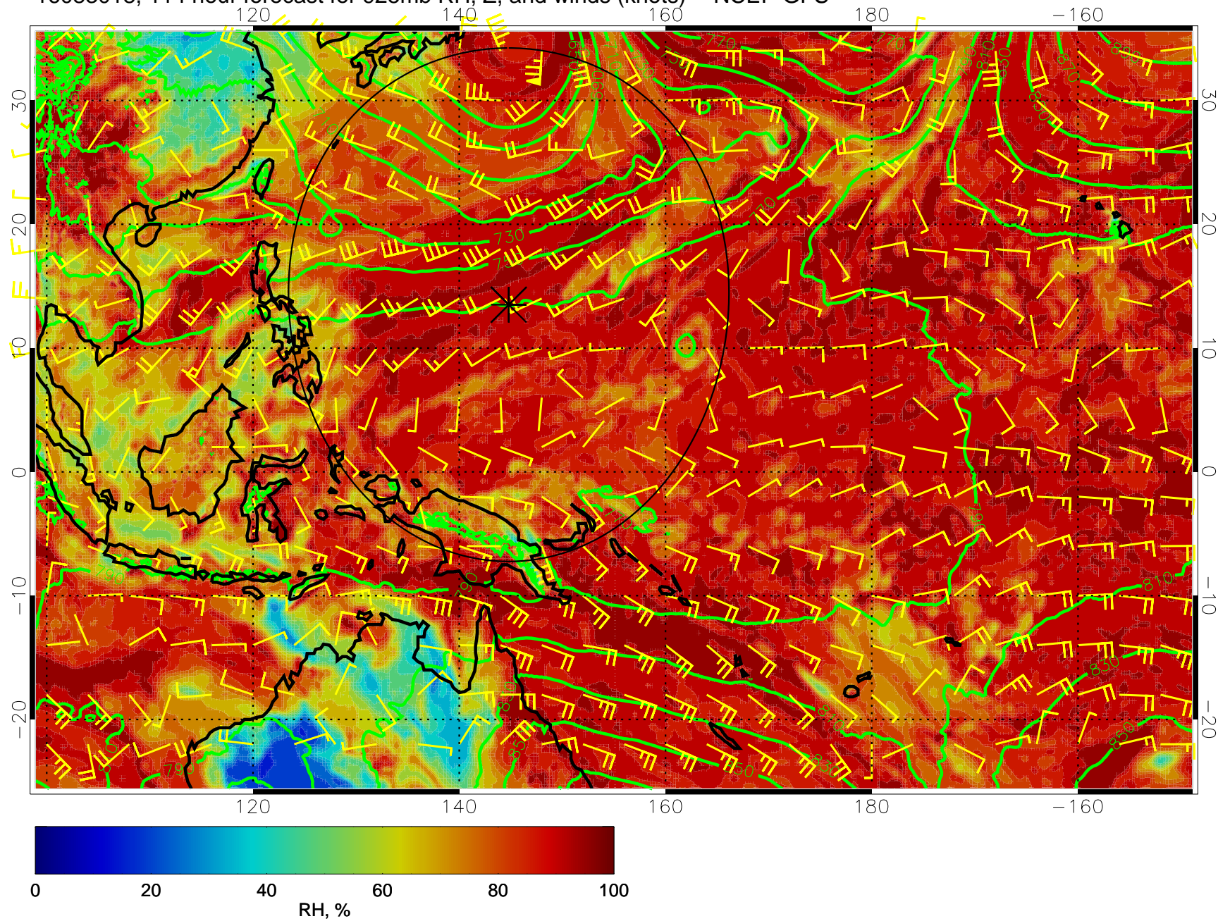
16083018, 114 hour forecast for 925mb RH, Z, and winds (knots) -- NCEP GFS
