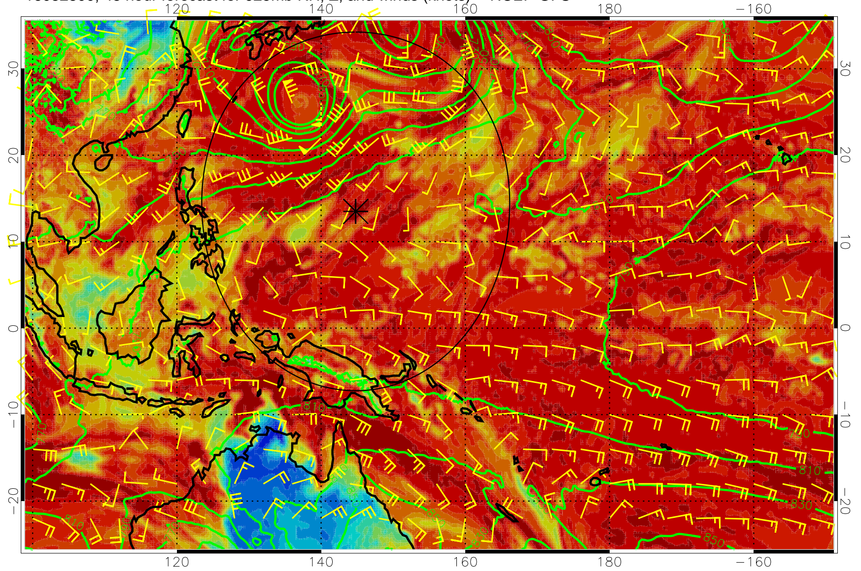
16082800, 48 hour forecast for 925mb RH, Z, and winds (knots) -- NCEP GFS
