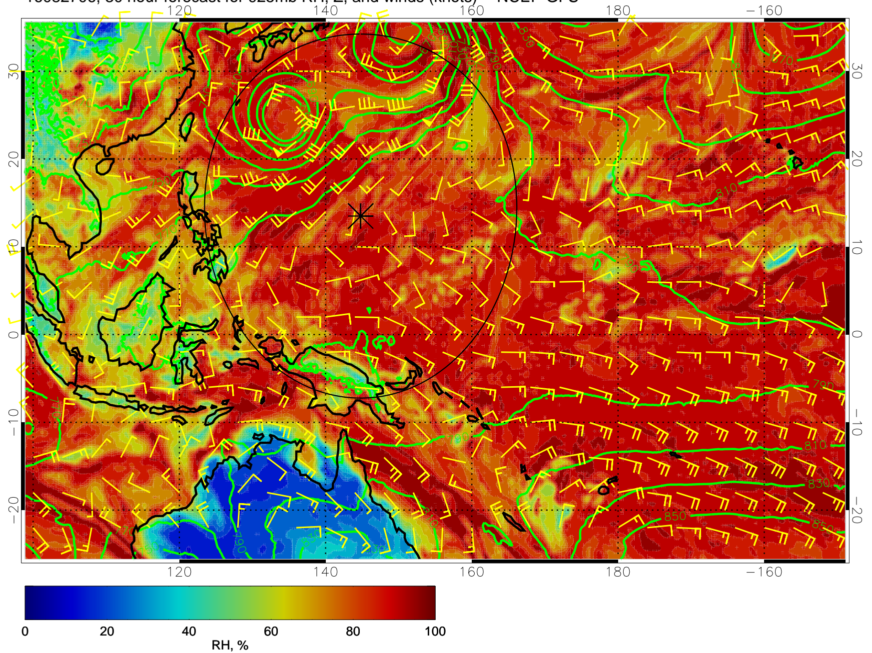
16082706, 30 hour forecast for 925mb RH, Z, and winds (knots) -- NCEP GFS
