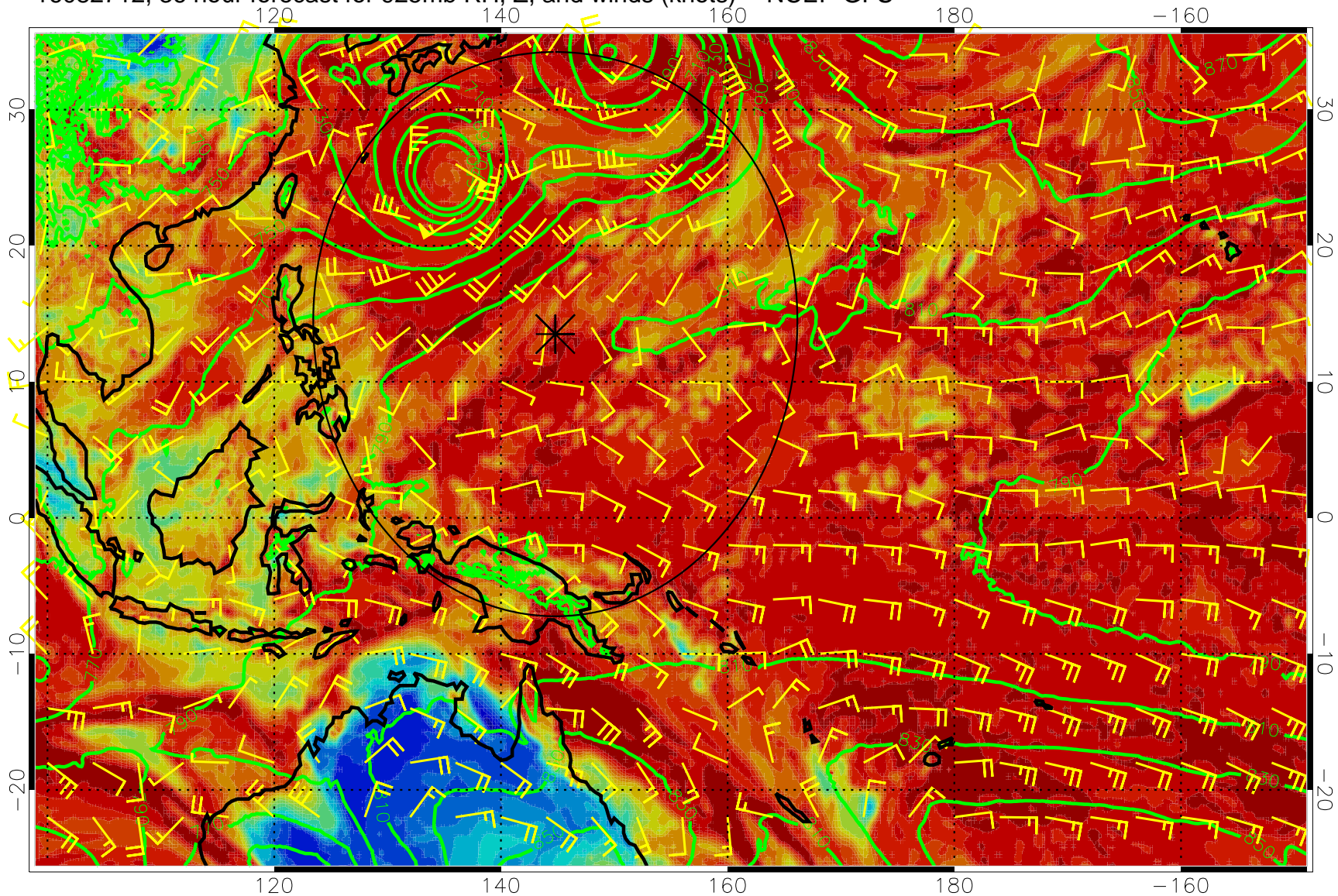
16082712, 36 hour forecast for 925mb RH, Z, and winds (knots) -- NCEP GFS
