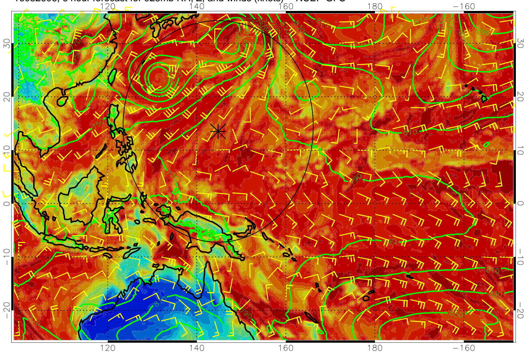
16082606, 6 hour forecast for 925mb RH, Z, and winds (knots) -- NCEP GFS
