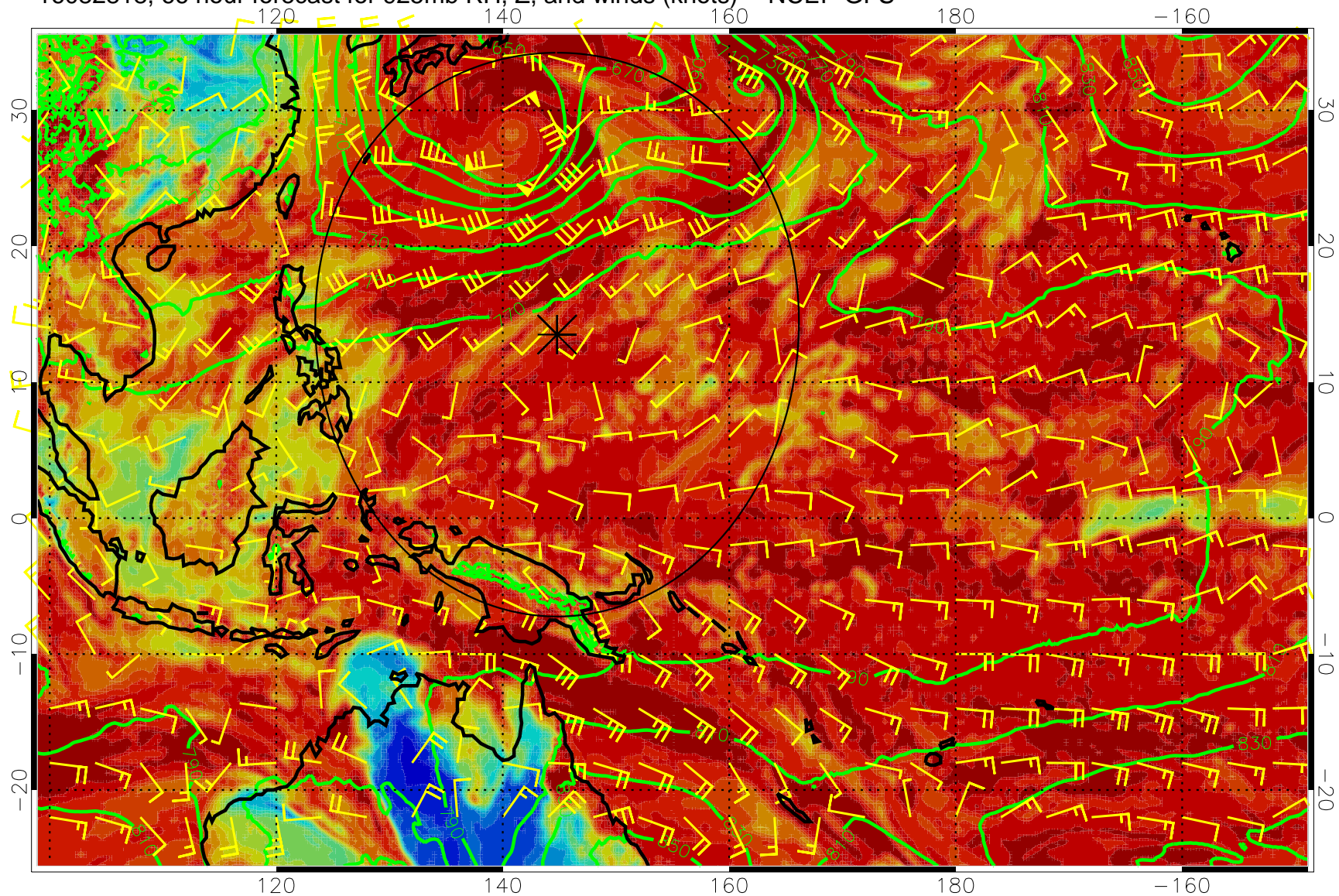
16082818, 66 hour forecast for 925mb RH, Z, and winds (knots) -- NCEP GFS
