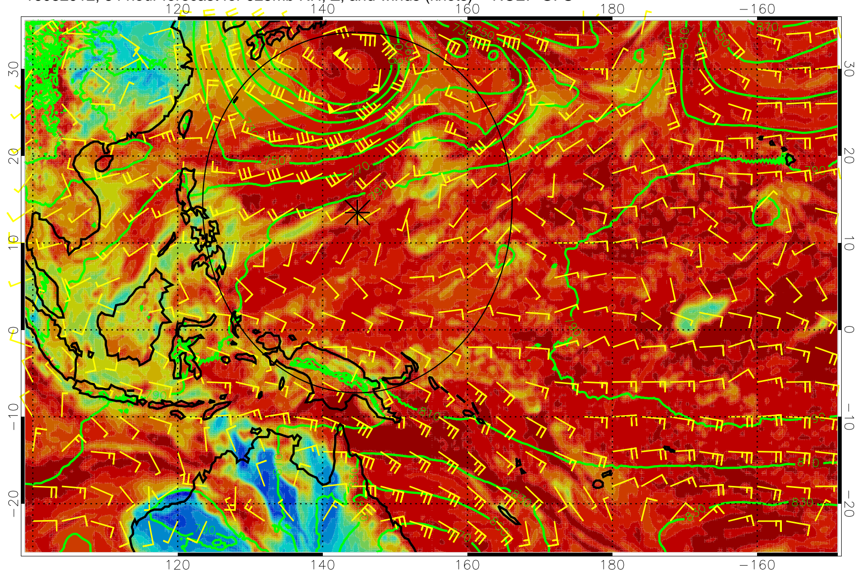
16082912, 84 hour forecast for 925mb RH, Z, and winds (knots) -- NCEP GFS
