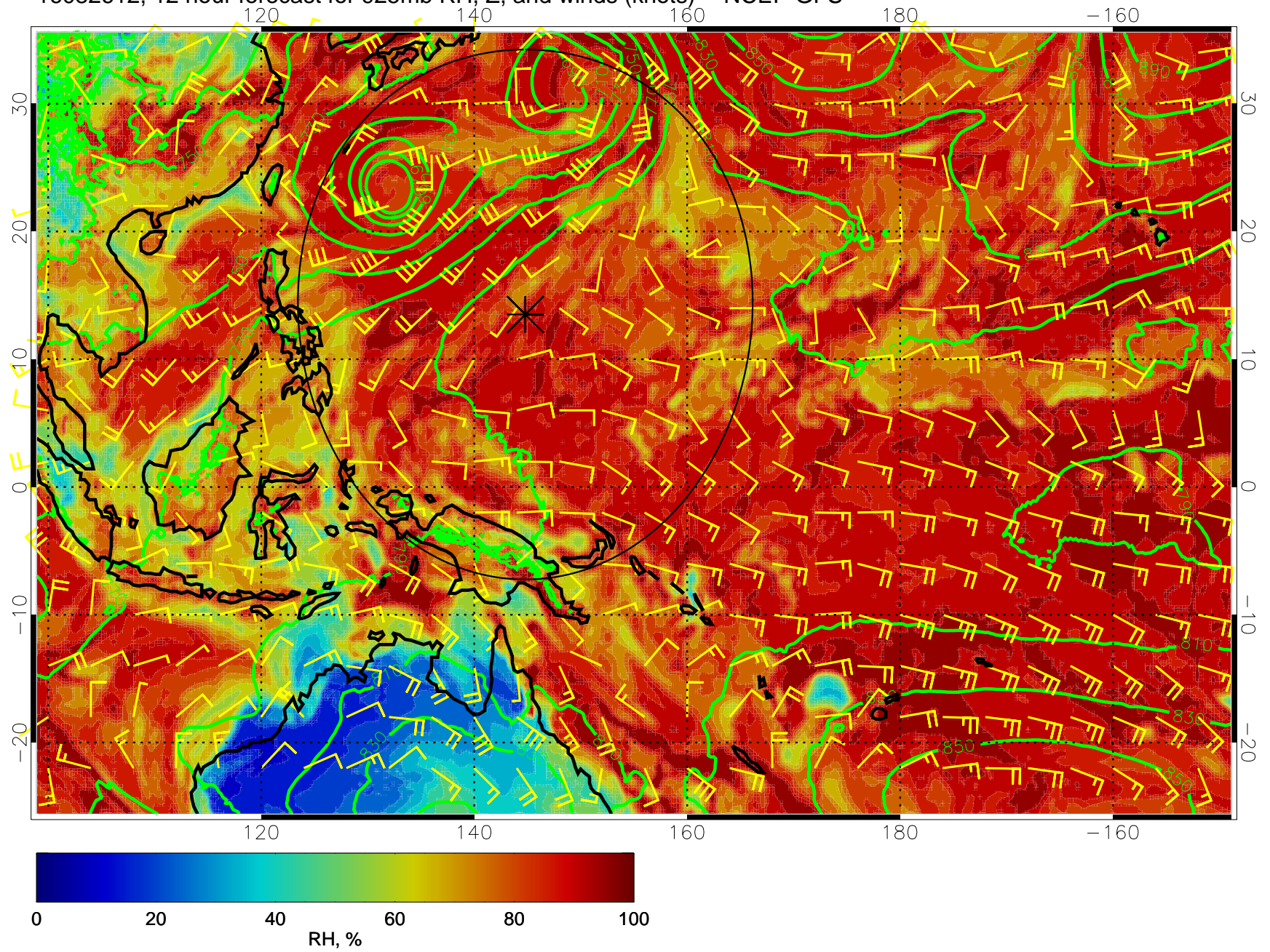
16082612, 12 hour forecast for 925mb RH, Z, and winds (knots) -- NCEP GFS
