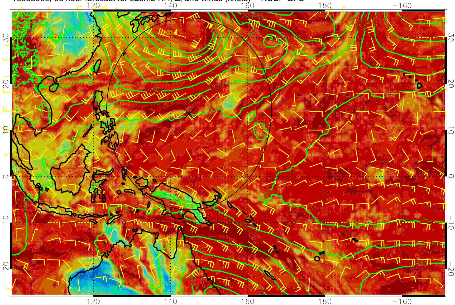
16083000, 96 hour forecast for 925mb RH, Z, and winds (knots) -- NCEP GFS
