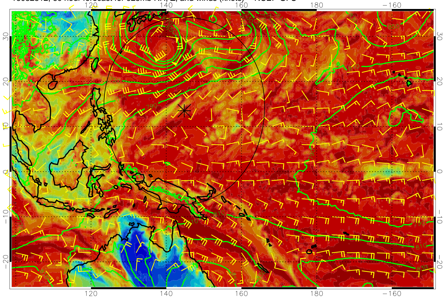
16082812, 60 hour forecast for 925mb RH, Z, and winds (knots) -- NCEP GFS
