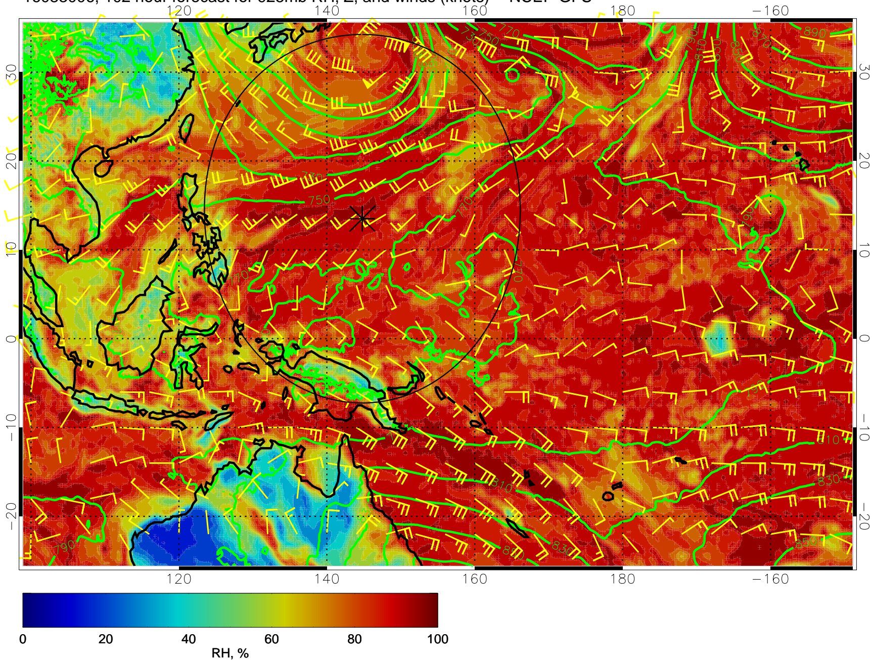
16083006, 102 hour forecast for 925mb RH, Z, and winds (knots) -- NCEP GFS
