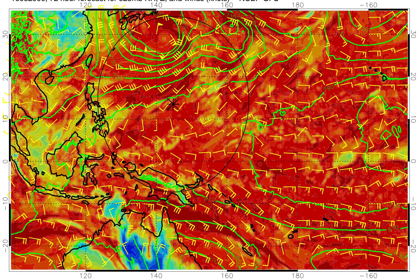
16082900, 72 hour forecast for 925mb RH, Z, and winds (knots) -- NCEP GFS
