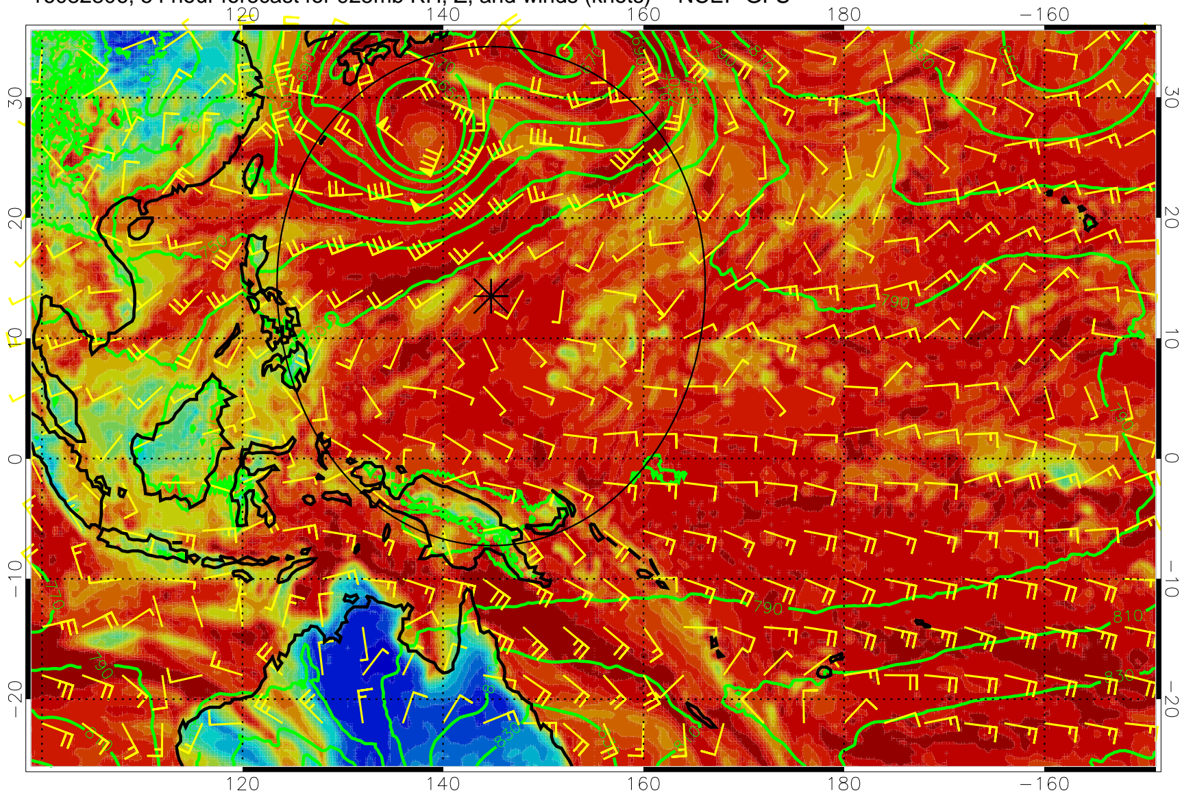
16082806, 54 hour forecast for 925mb RH, Z, and winds (knots) -- NCEP GFS
