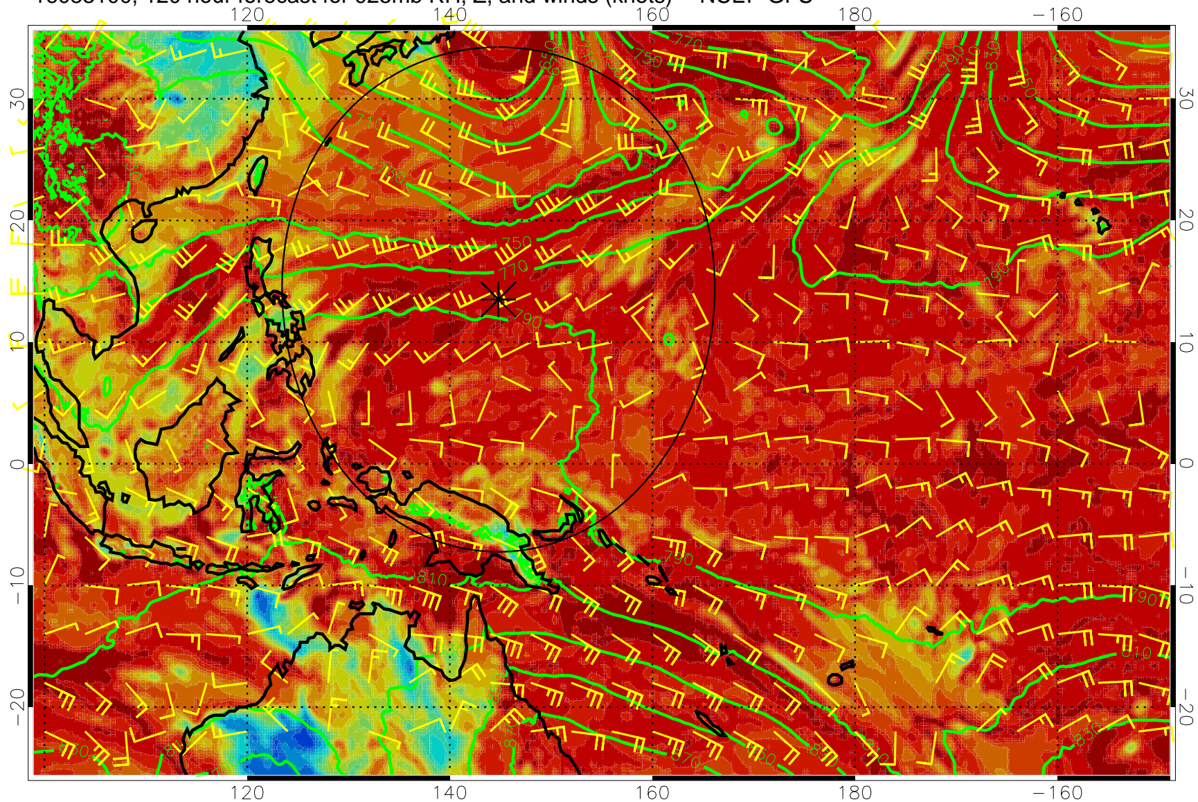
16083100, 120 hour forecast for 925mb RH, Z, and winds (knots) -- NCEP GFS
