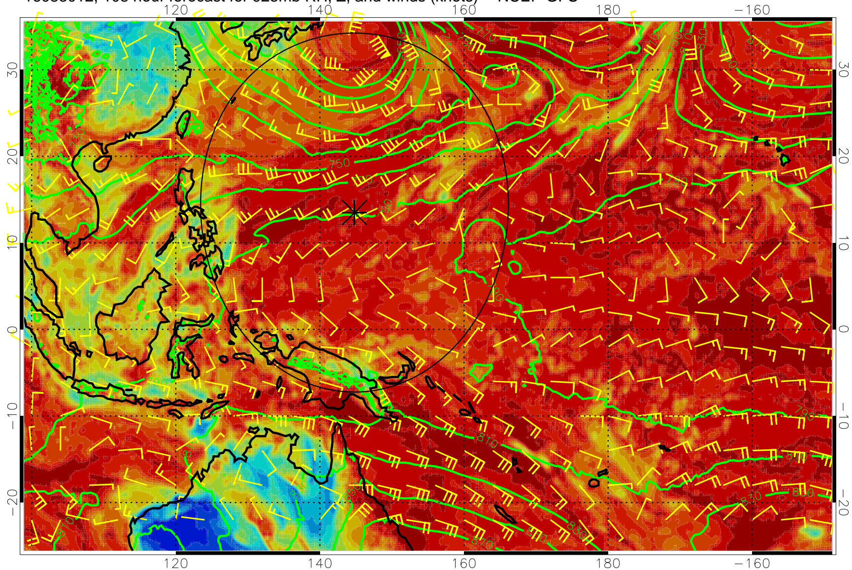
16083012, 108 hour forecast for 925mb RH, Z, and winds (knots) -- NCEP GFS
