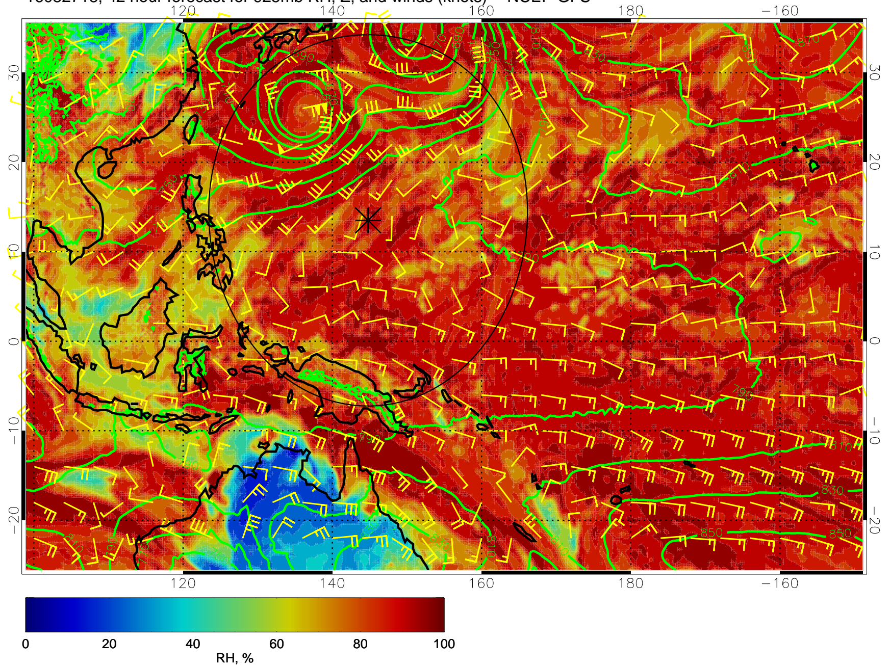
16082718, 42 hour forecast for 925mb RH, Z, and winds (knots) -- NCEP GFS
