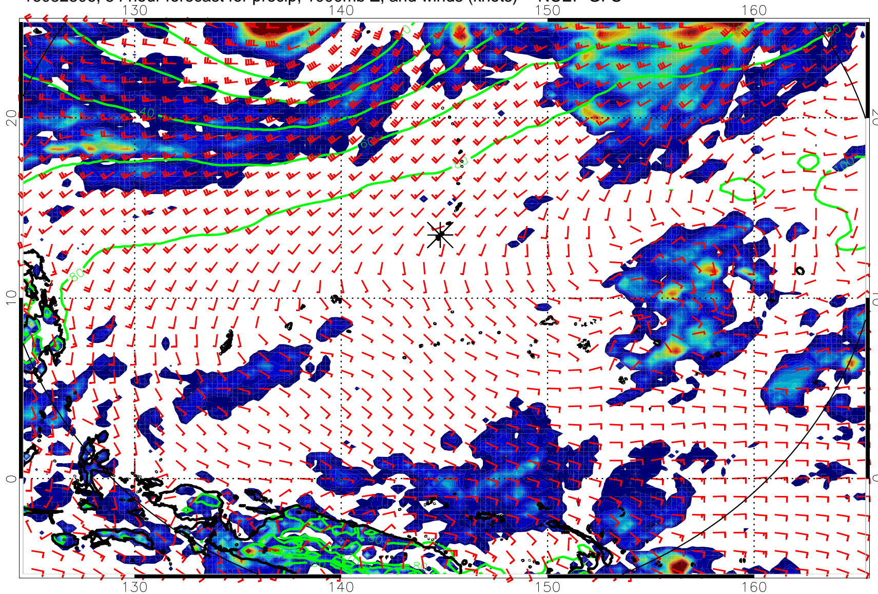
16082806, 54 hour forecast for precip, 1000mb Z, and winds (knots) -- NCEP GFS
