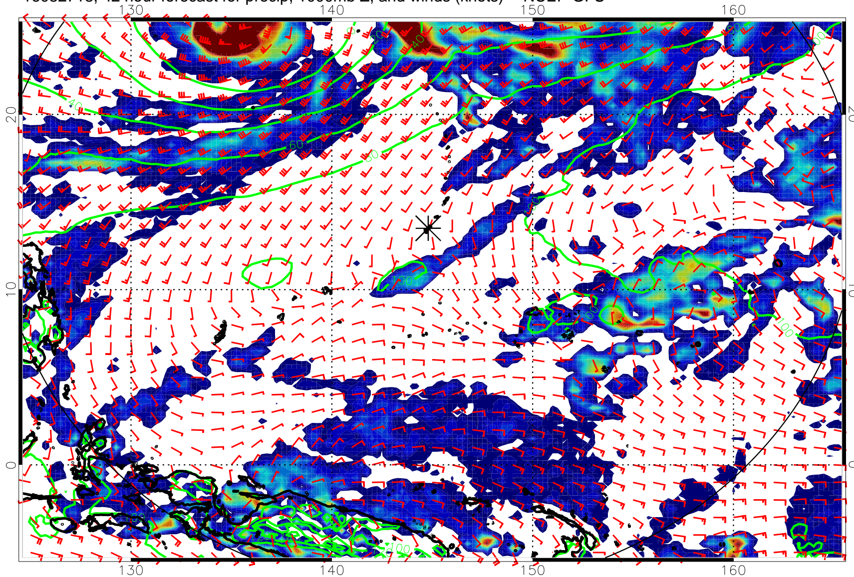
16082718, 42 hour forecast for precip, 1000mb Z, and winds (knots) -- NCEP GFS
