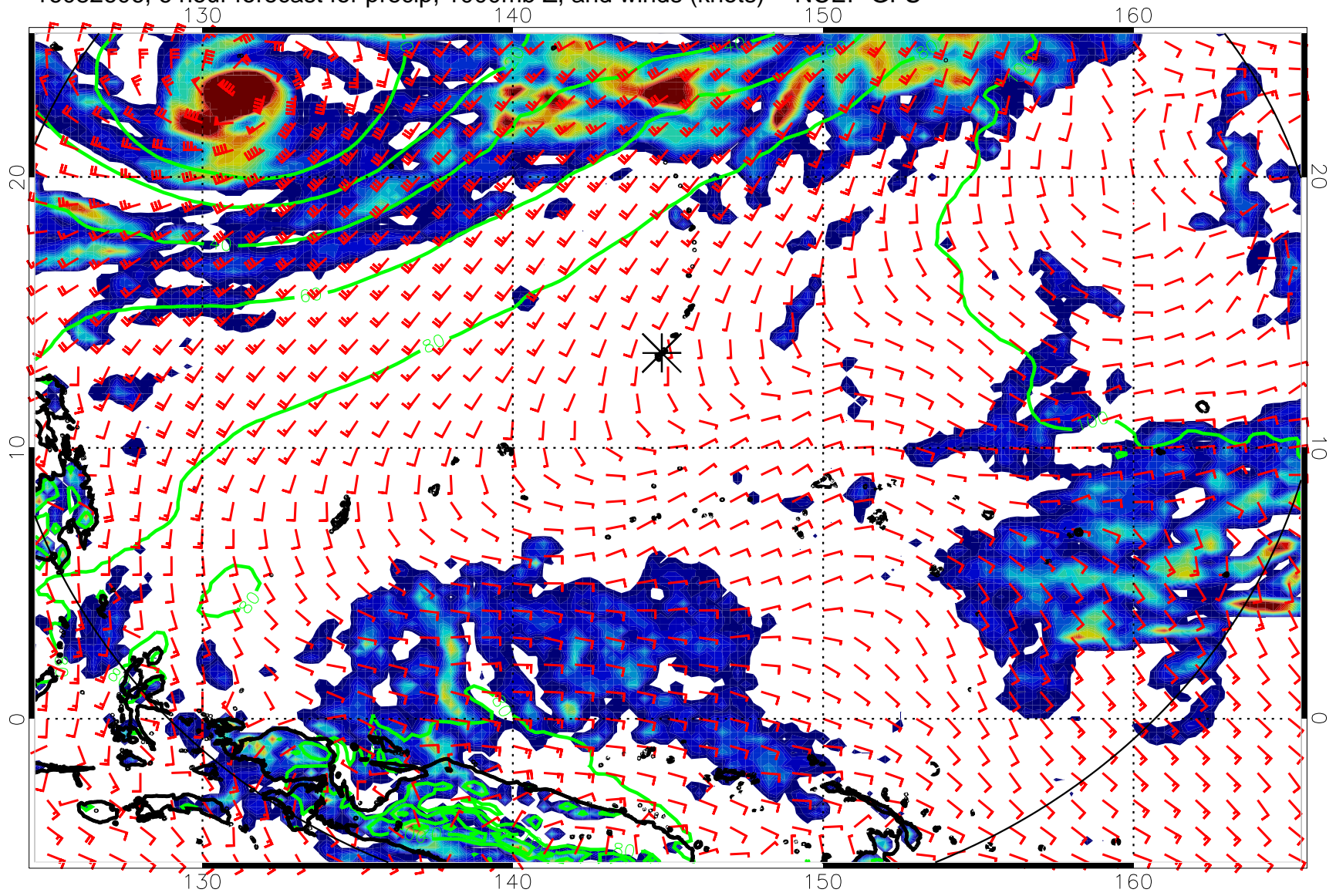
16082606, 6 hour forecast for precip, 1000mb Z, and winds (knots) -- NCEP GFS
