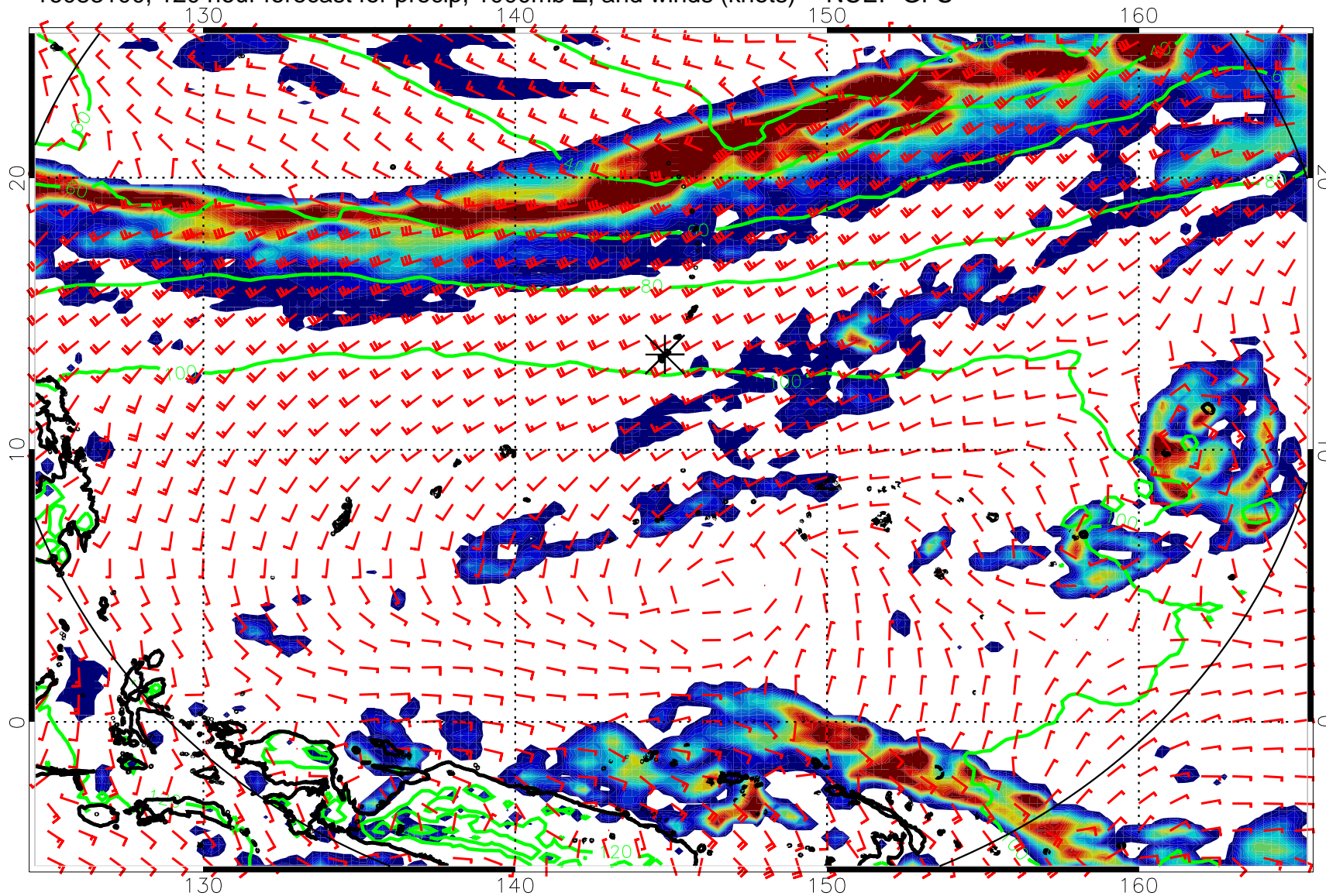
16083100, 120 hour forecast for precip, 1000mb Z, and winds (knots) -- NCEP GFS
