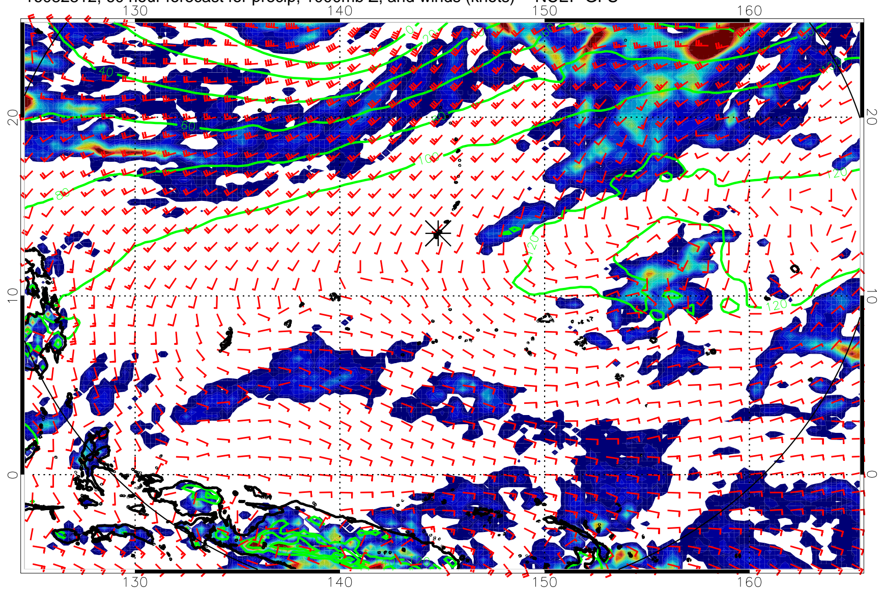
16082812, 60 hour forecast for precip, 1000mb Z, and winds (knots) -- NCEP GFS
