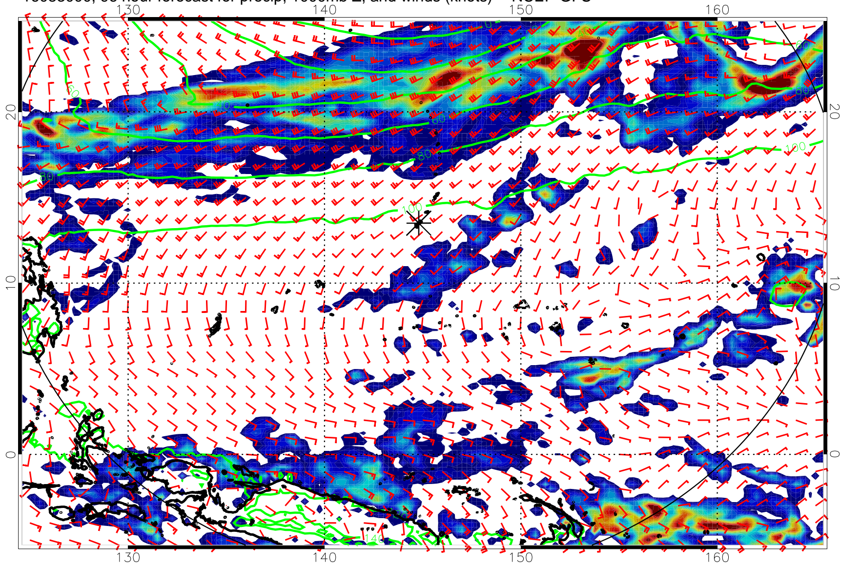
16083000, 96 hour forecast for precip, 1000mb Z, and winds (knots) -- NCEP GFS
