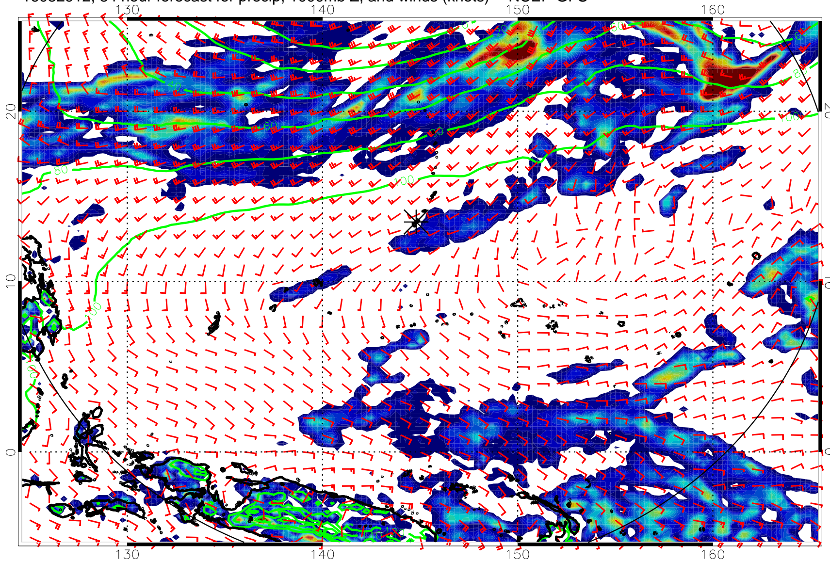
16082912, 84 hour forecast for precip, 1000mb Z, and winds (knots) -- NCEP GFS
