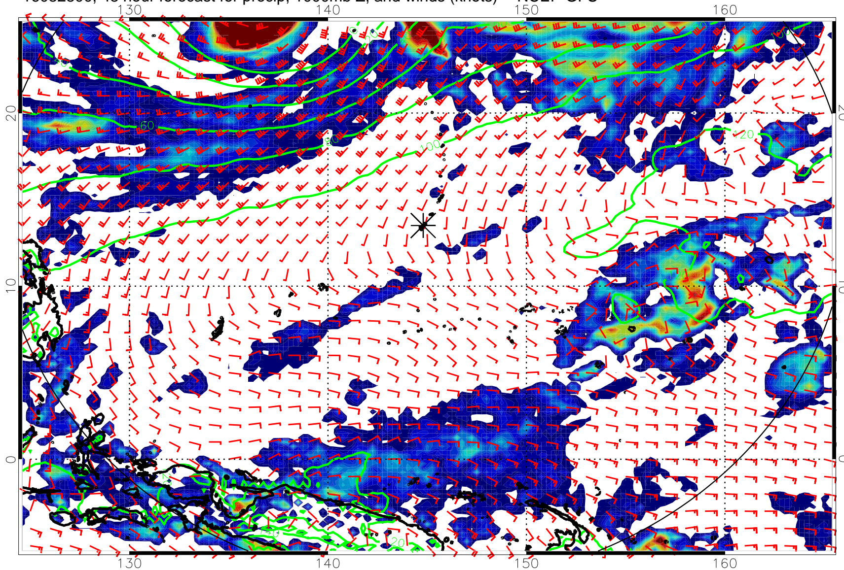
16082800, 48 hour forecast for precip, 1000mb Z, and winds (knots) -- NCEP GFS
