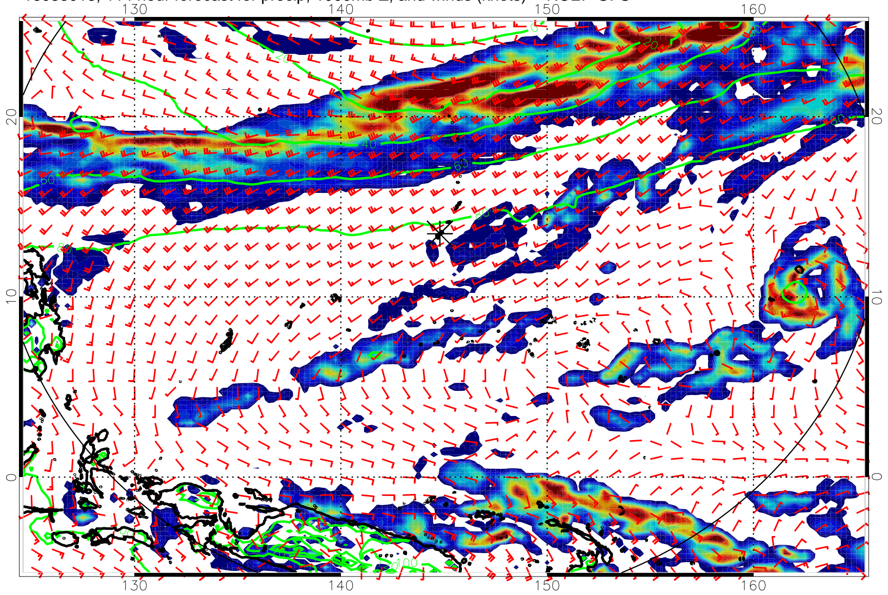
16083018, 114 hour forecast for precip, 1000mb Z, and winds (knots) -- NCEP GFS
