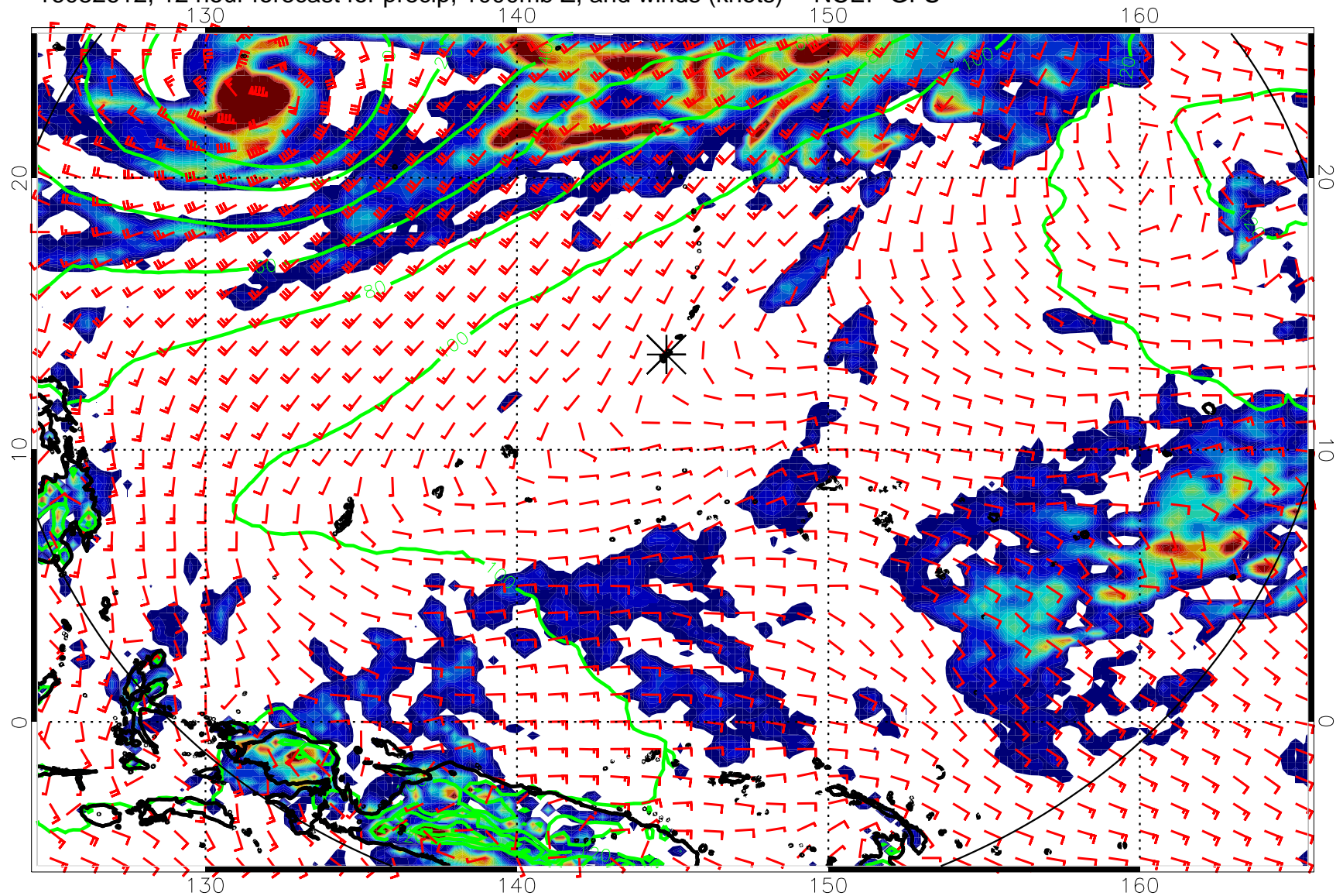
16082612, 12 hour forecast for precip, 1000mb Z, and winds (knots) -- NCEP GFS
