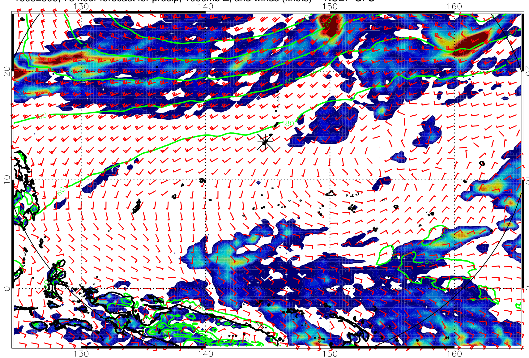
16082906, 78 hour forecast for precip, 1000mb Z, and winds (knots) -- NCEP GFS
