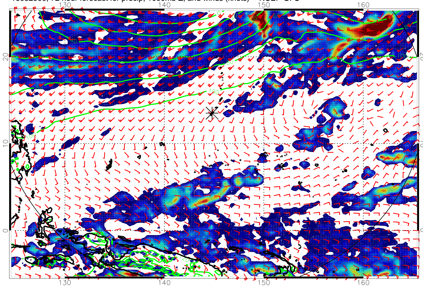
16082900, 72 hour forecast for precip, 1000mb Z, and winds (knots) -- NCEP GFS
