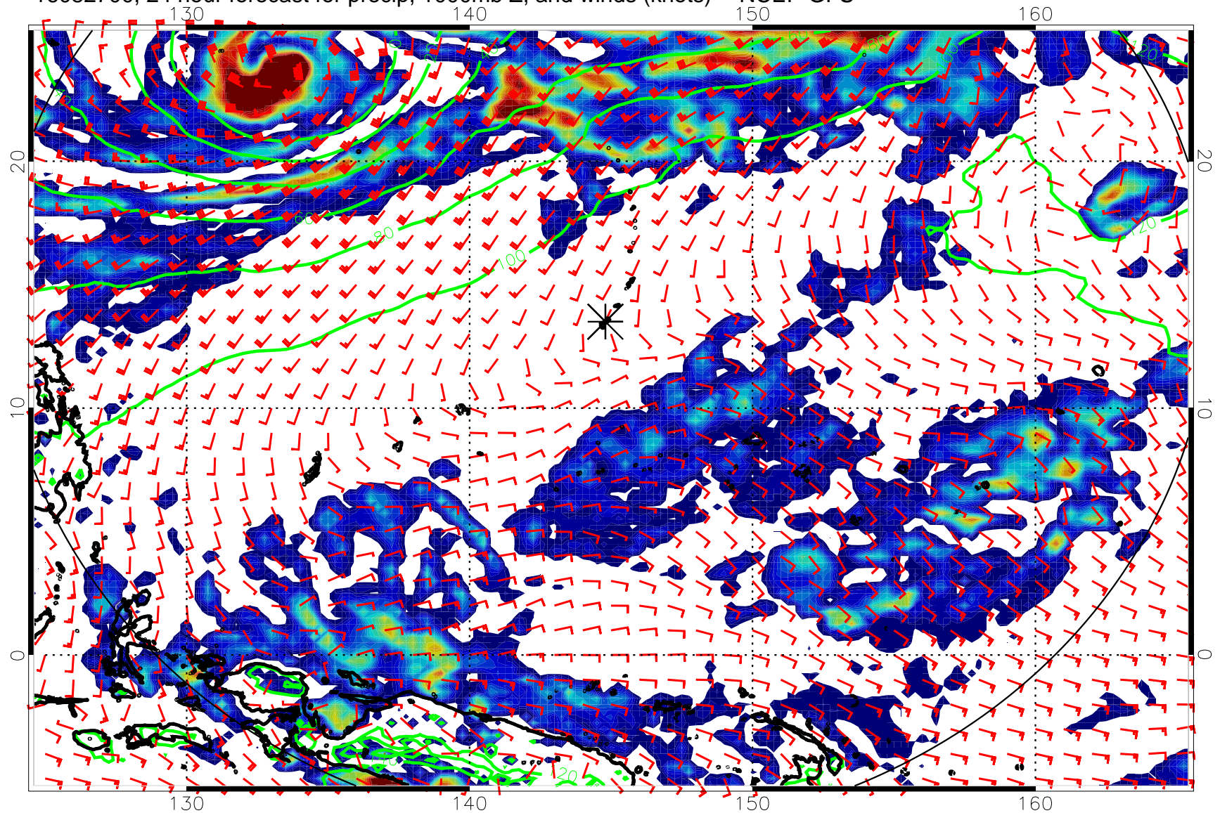
16082700, 24 hour forecast for precip, 1000mb Z, and winds (knots) -- NCEP GFS
