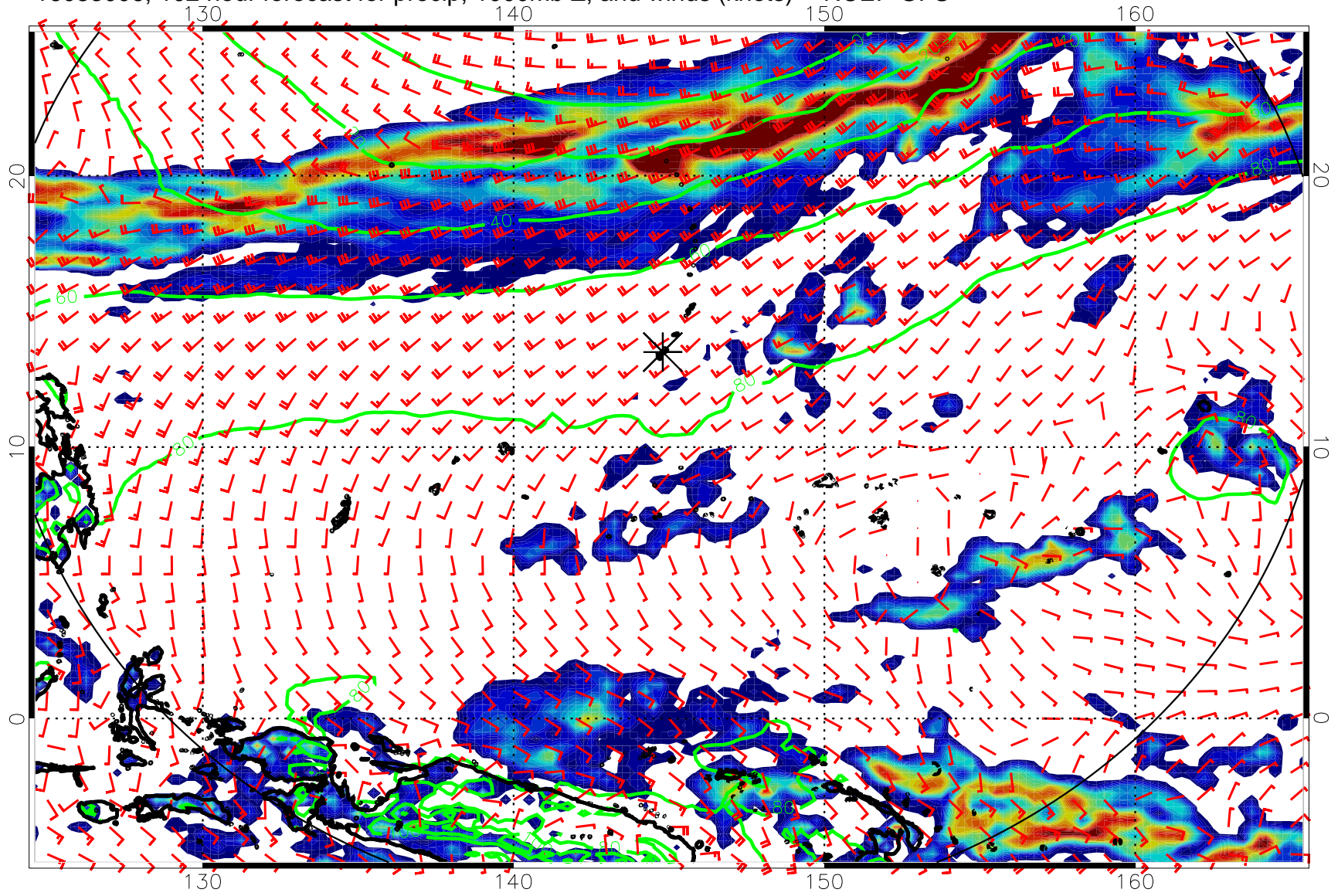
16083006, 102 hour forecast for precip, 1000mb Z, and winds (knots) -- NCEP GFS
