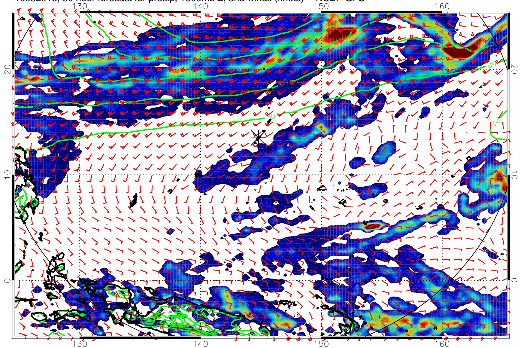
16082918, 90 hour forecast for precip, 1000mb Z, and winds (knots) -- NCEP GFS
