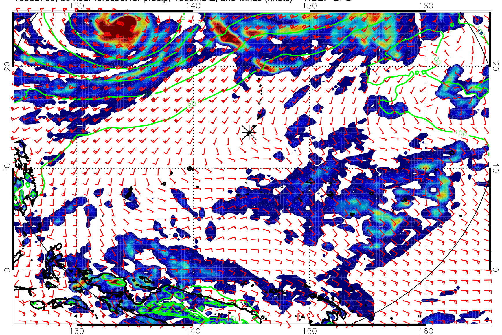
16082706, 30 hour forecast for precip, 1000mb Z, and winds (knots) -- NCEP GFS
