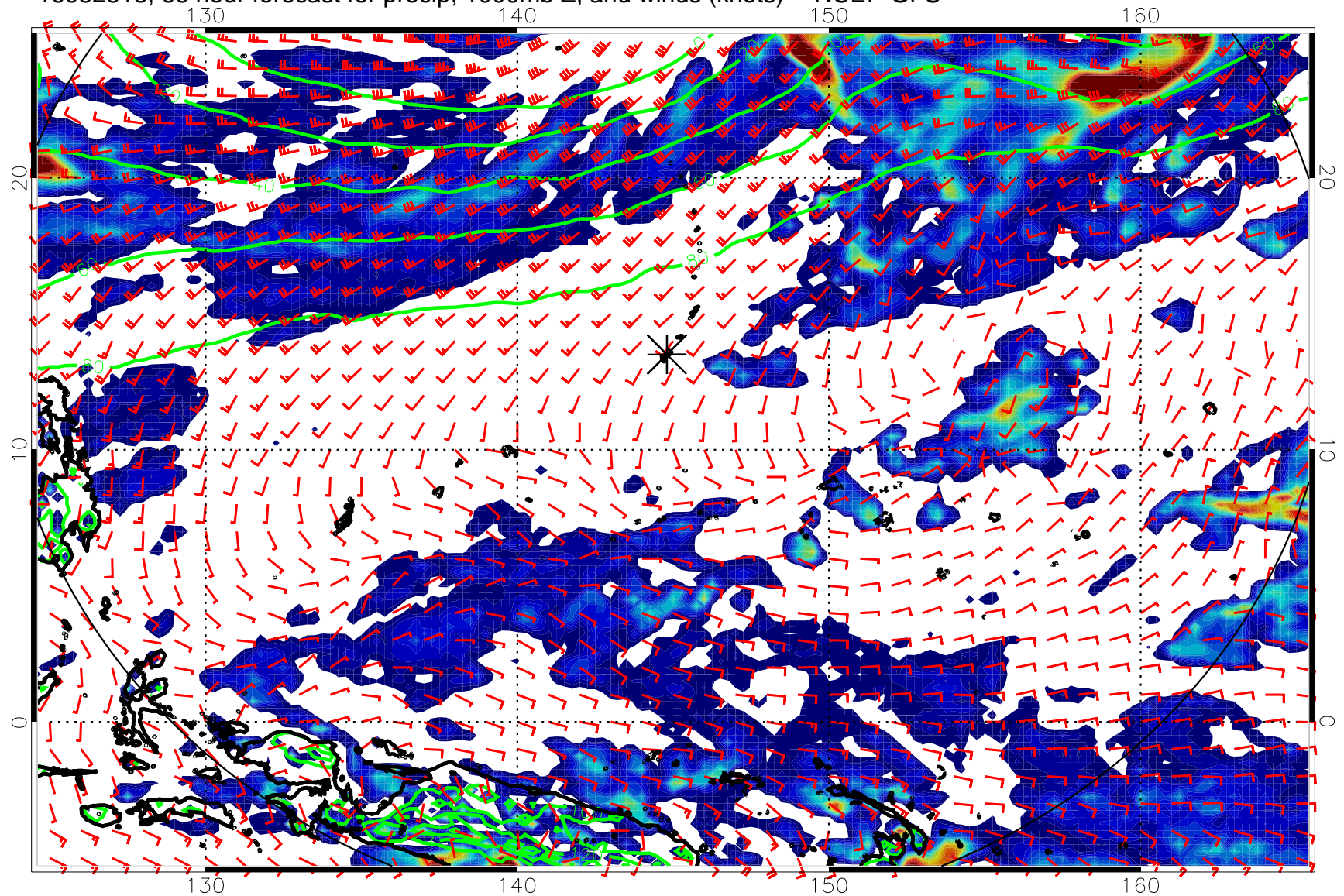
16082818, 66 hour forecast for precip, 1000mb Z, and winds (knots) -- NCEP GFS
