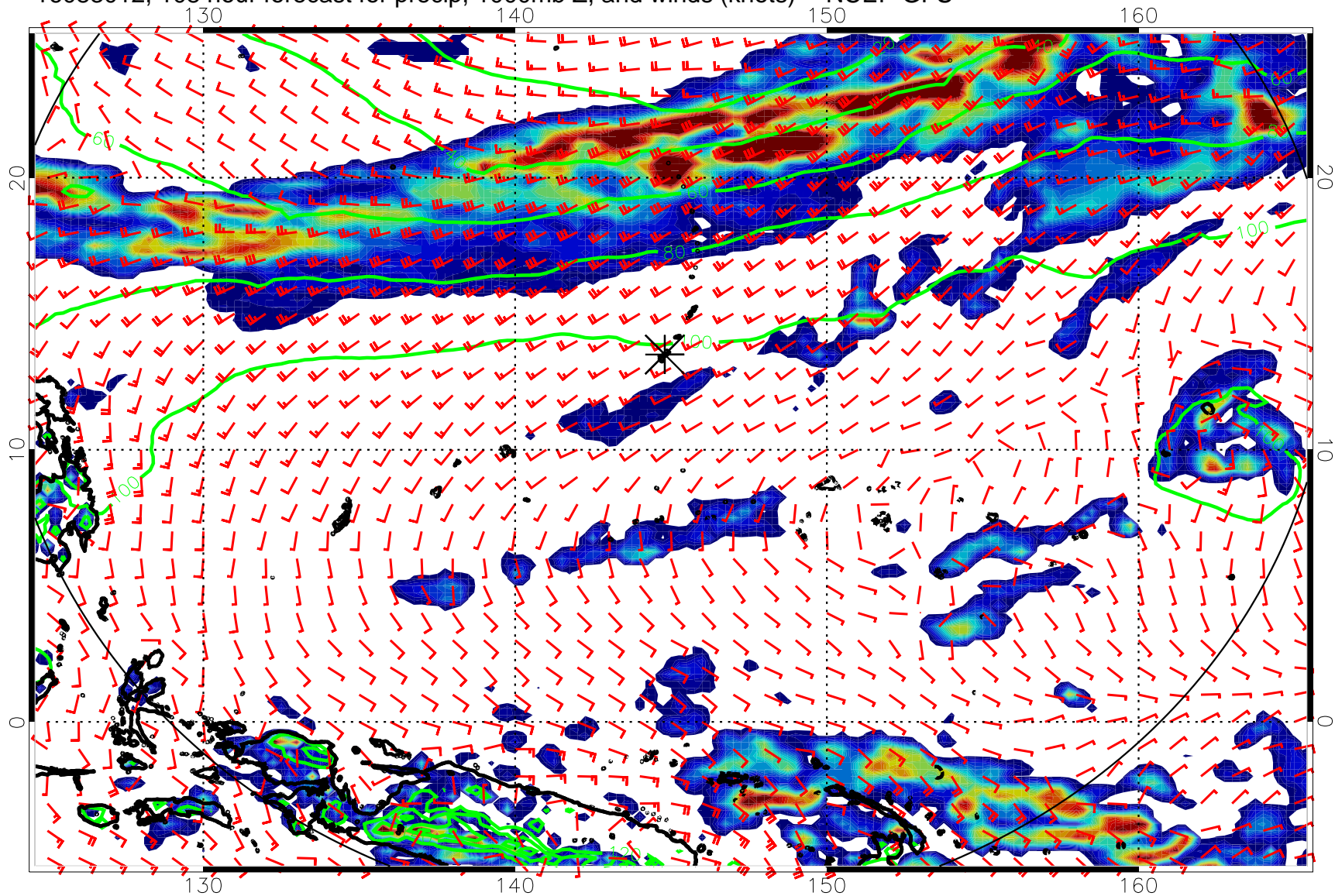
16083012, 108 hour forecast for precip, 1000mb Z, and winds (knots) -- NCEP GFS
