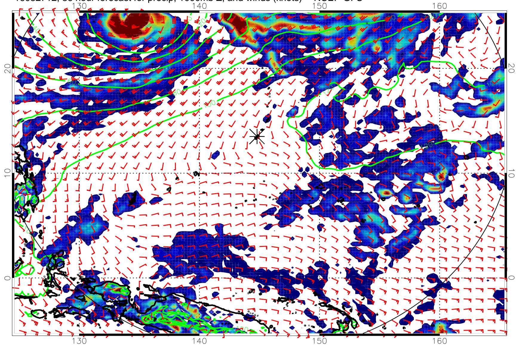
16082712, 36 hour forecast for precip, 1000mb Z, and winds (knots) -- NCEP GFS
