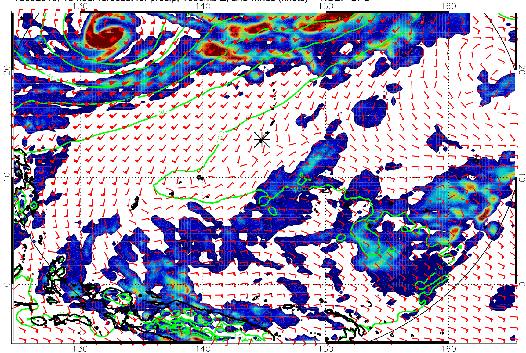
16082618, 18 hour forecast for precip, 1000mb Z, and winds (knots) -- NCEP GFS
