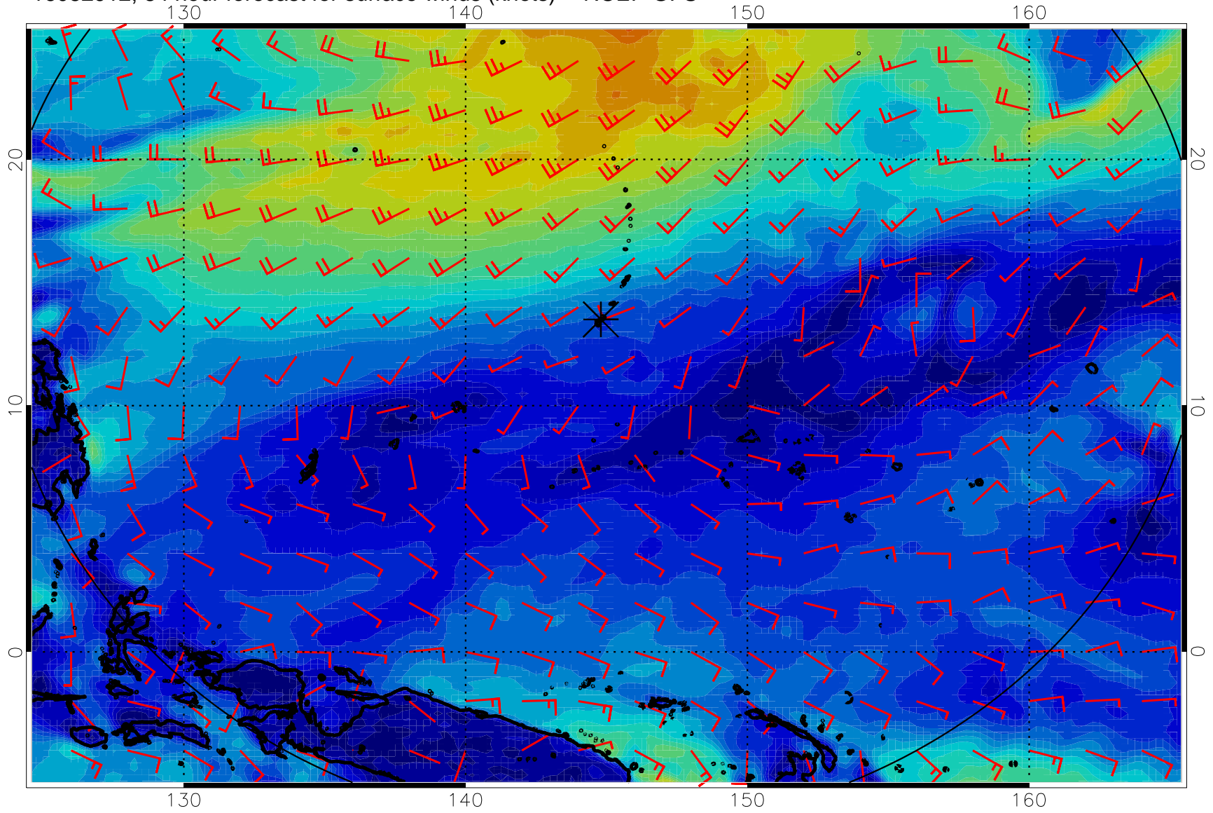
16082912, 84 hour forecast for surface winds (knots) -- NCEP GFS
