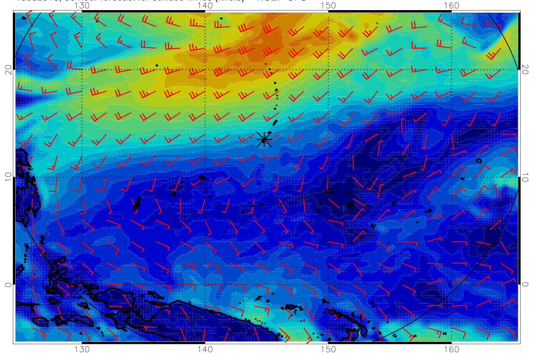
16082918, 90 hour forecast for surface winds (knots) -- NCEP GFS
