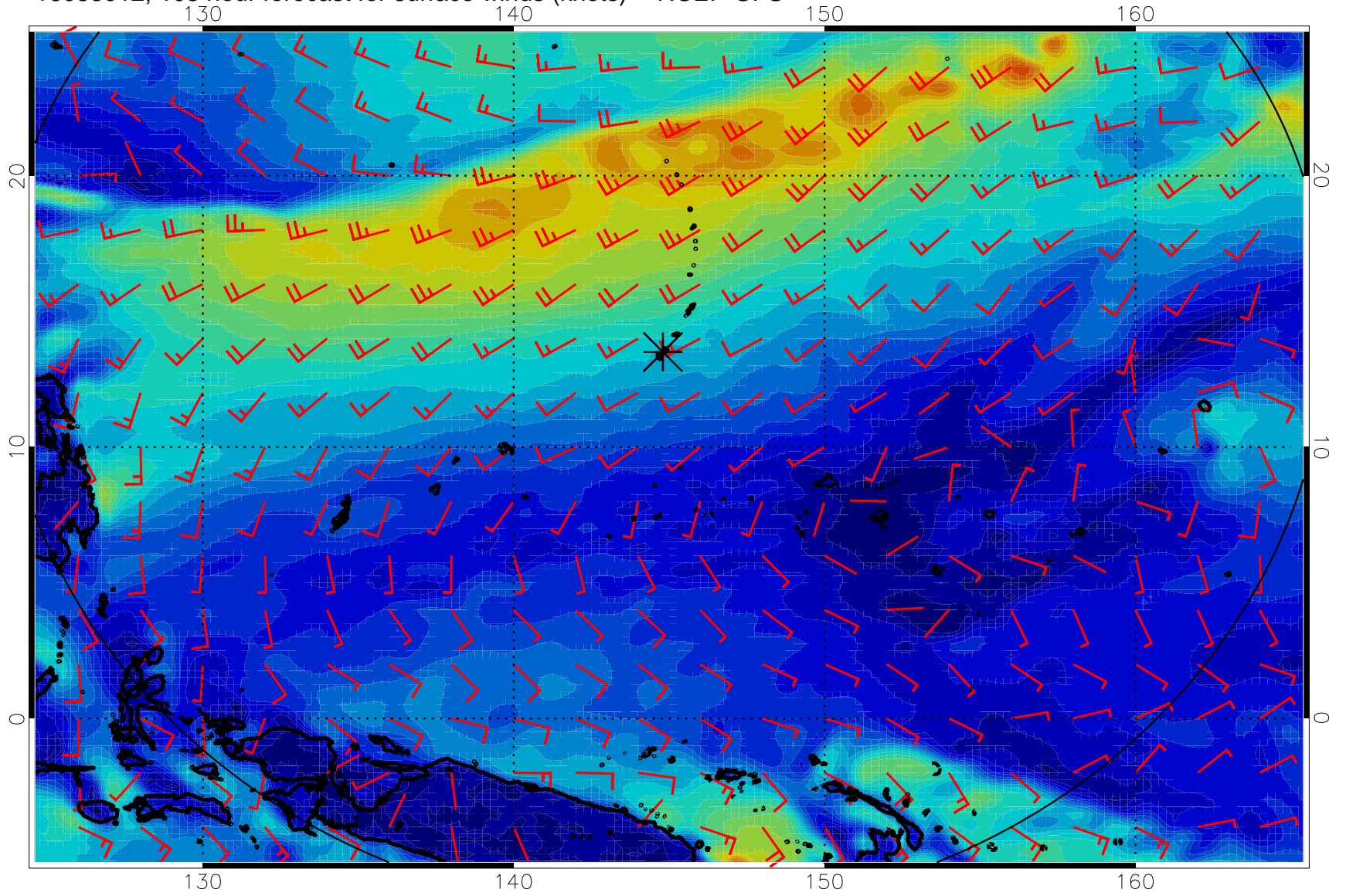
16083012, 108 hour forecast for surface winds (knots) -- NCEP GFS
