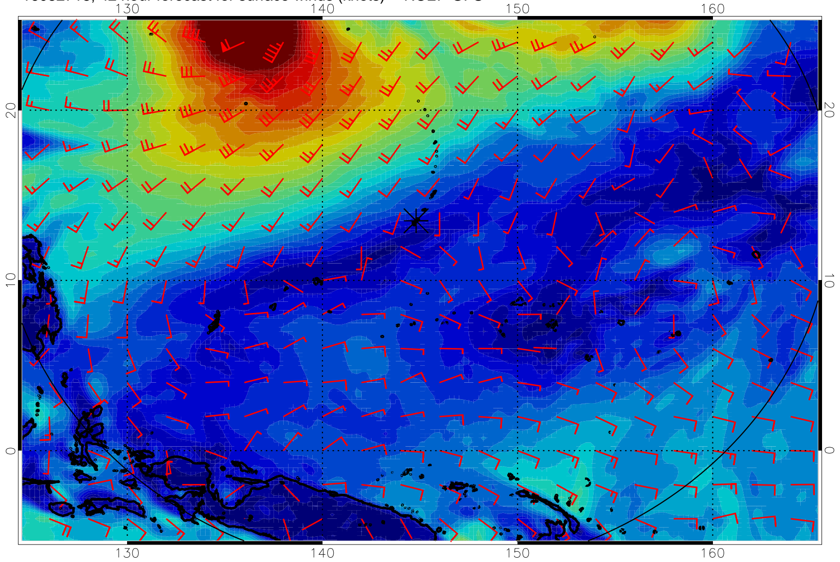
16082718, 42 hour forecast for surface winds (knots) -- NCEP GFS
