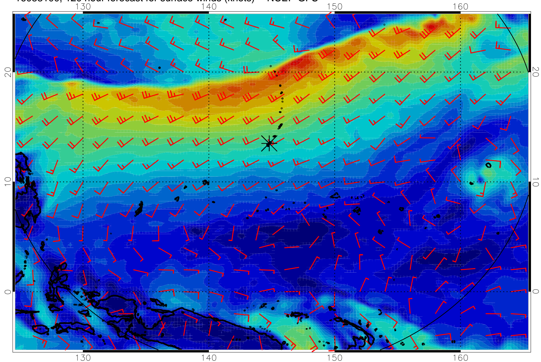
16083100, 120 hour forecast for surface winds (knots) -- NCEP GFS
