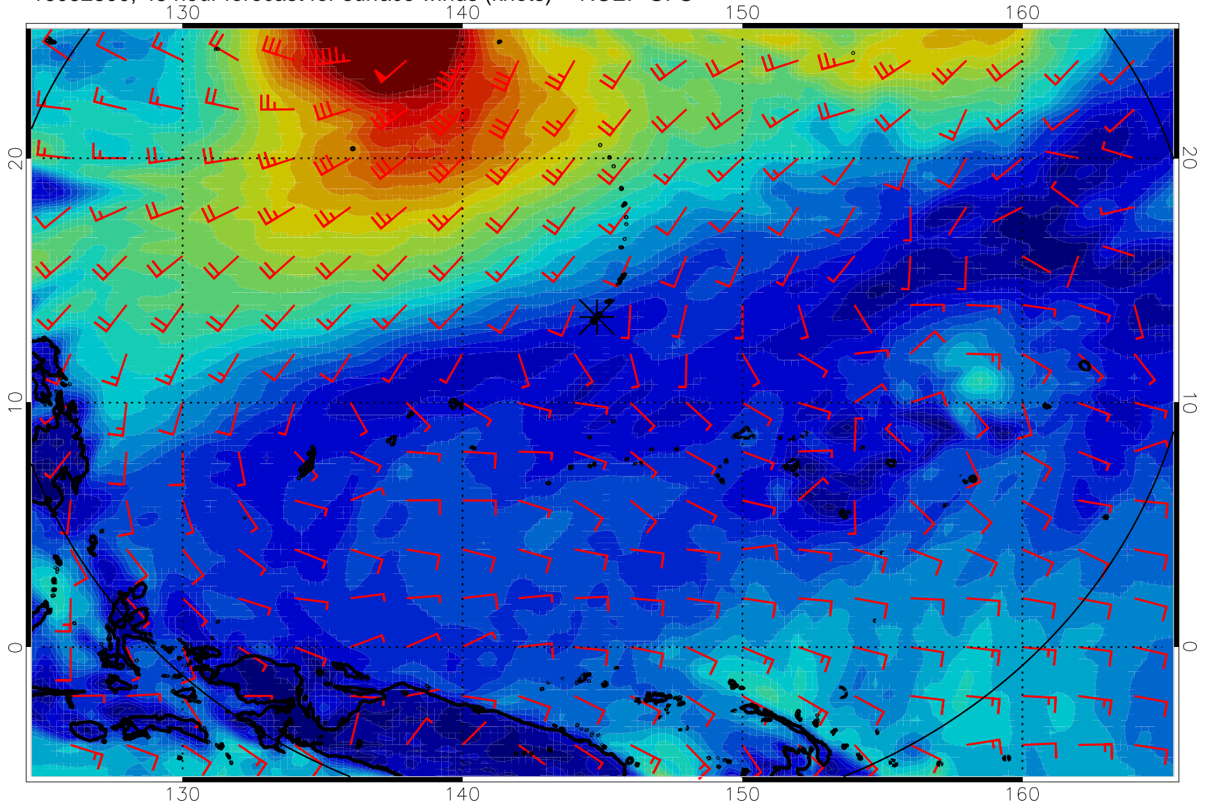
16082800, 48 hour forecast for surface winds (knots) -- NCEP GFS
