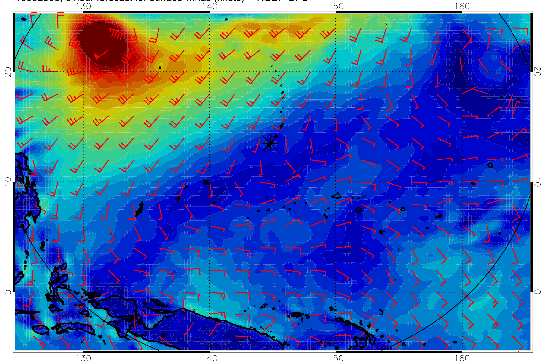
16082606, 6 hour forecast for surface winds (knots) -- NCEP GFS
