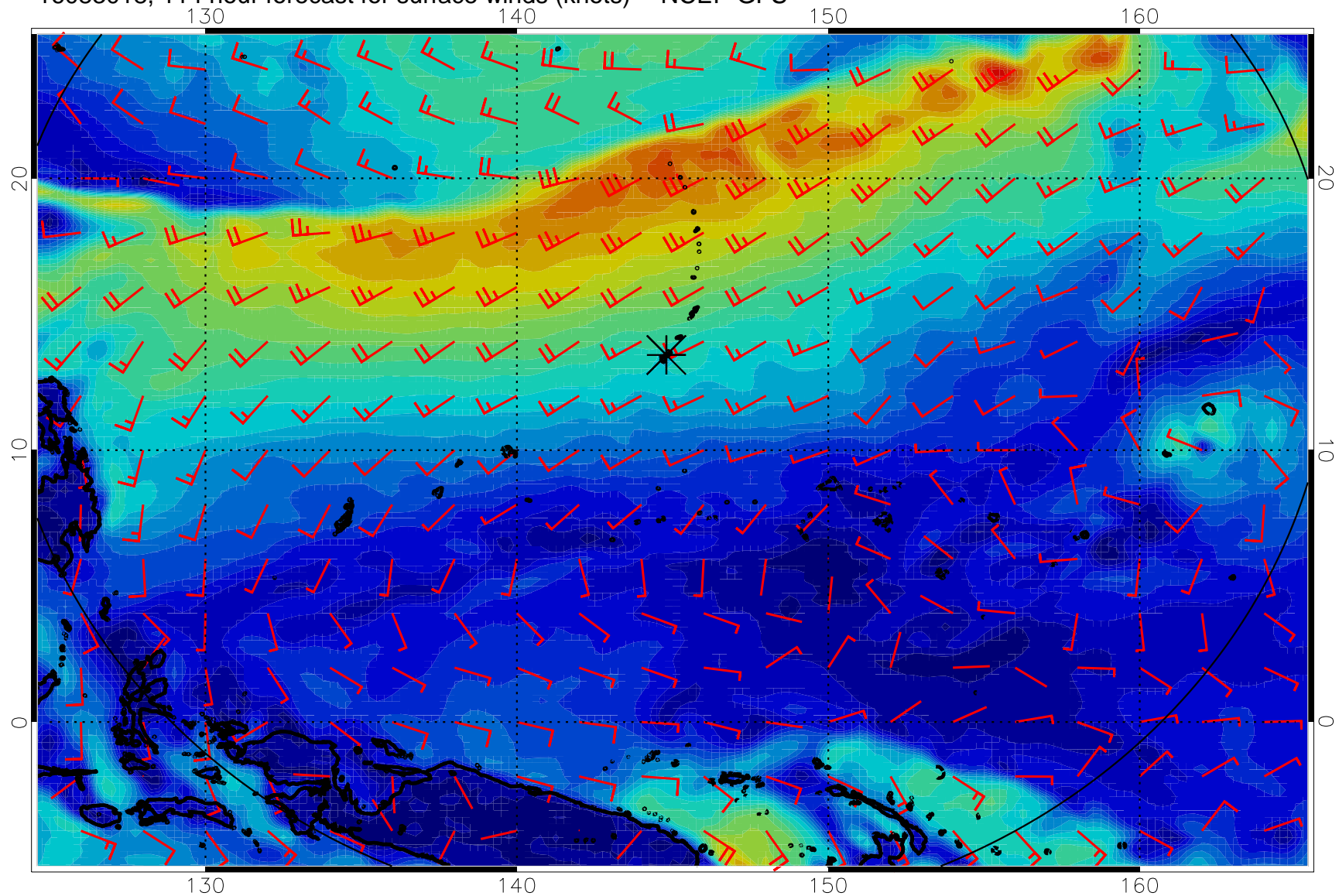
16083018, 114 hour forecast for surface winds (knots) -- NCEP GFS
