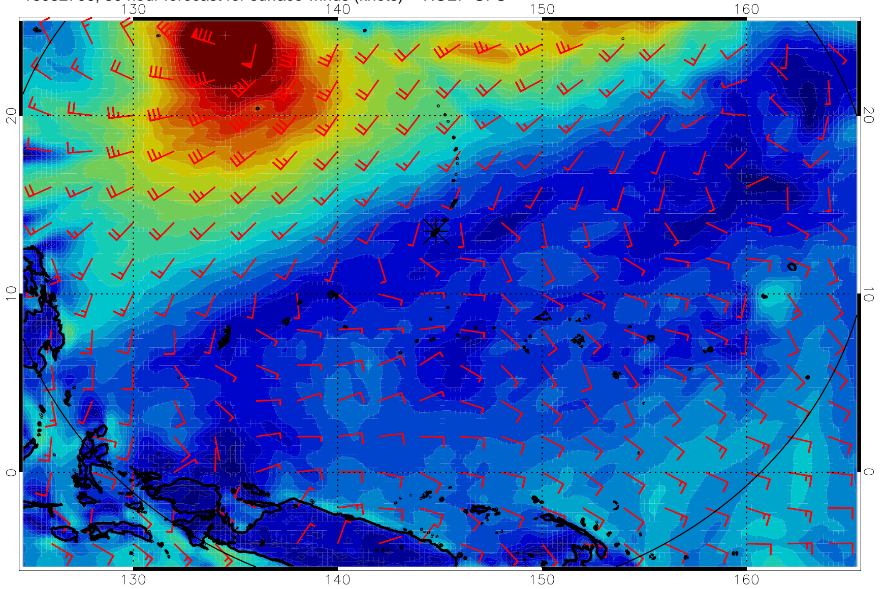
16082706, 30 hour forecast for surface winds (knots) -- NCEP GFS
