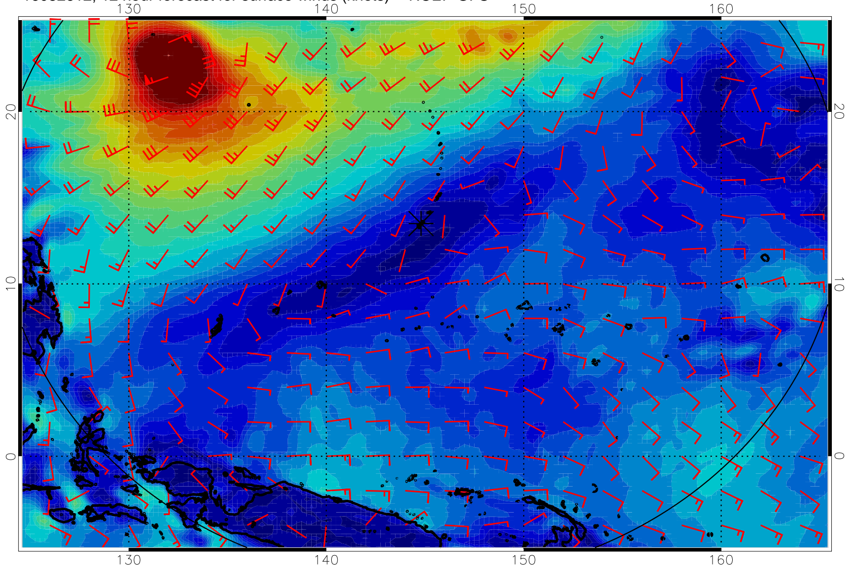
16082612, 12 hour forecast for surface winds (knots) -- NCEP GFS
