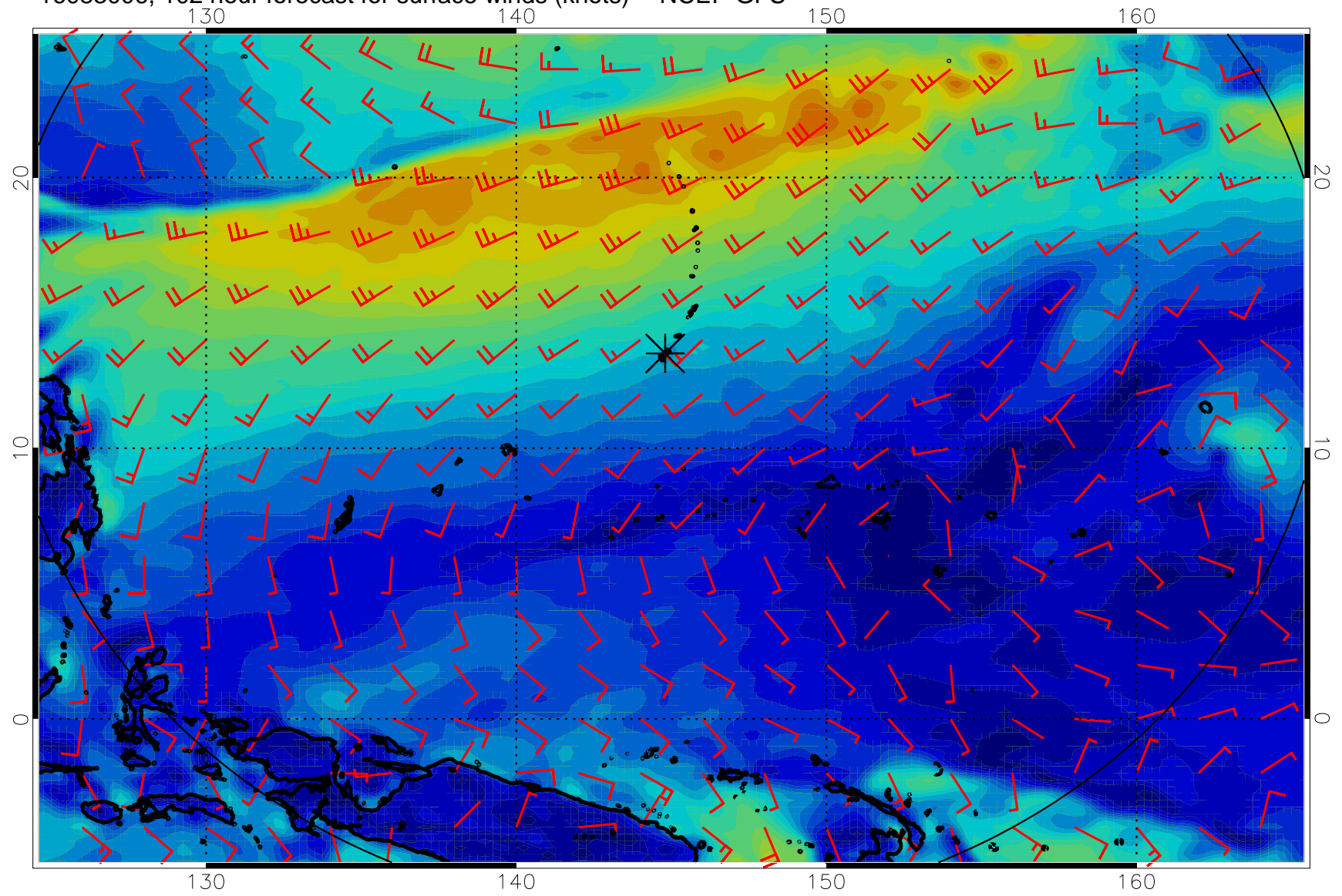
16083006, 102 hour forecast for surface winds (knots) -- NCEP GFS
