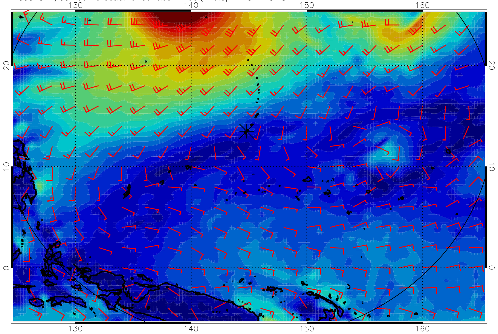
16082812, 60 hour forecast for surface winds (knots) -- NCEP GFS
