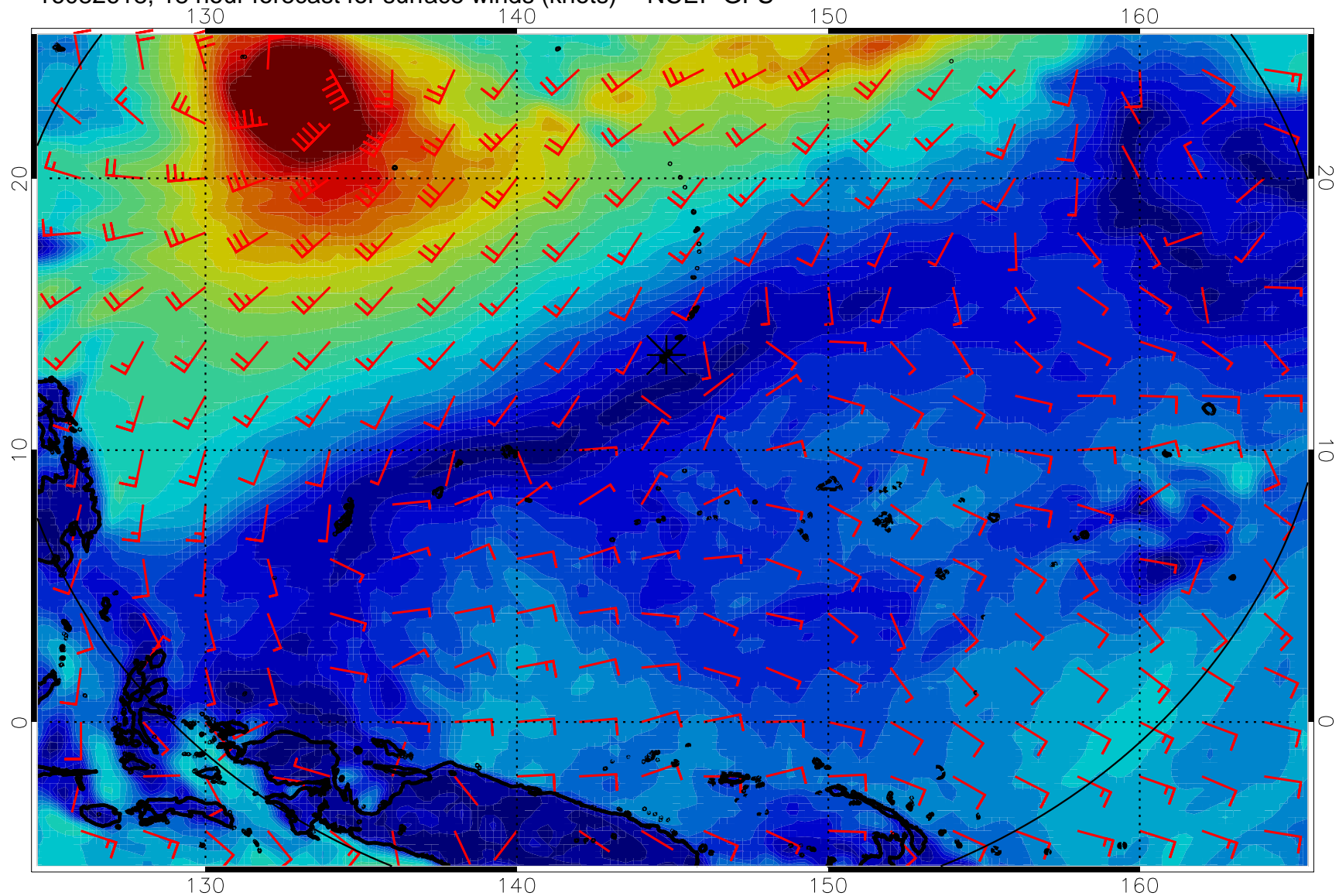
16082618, 18 hour forecast for surface winds (knots) -- NCEP GFS
