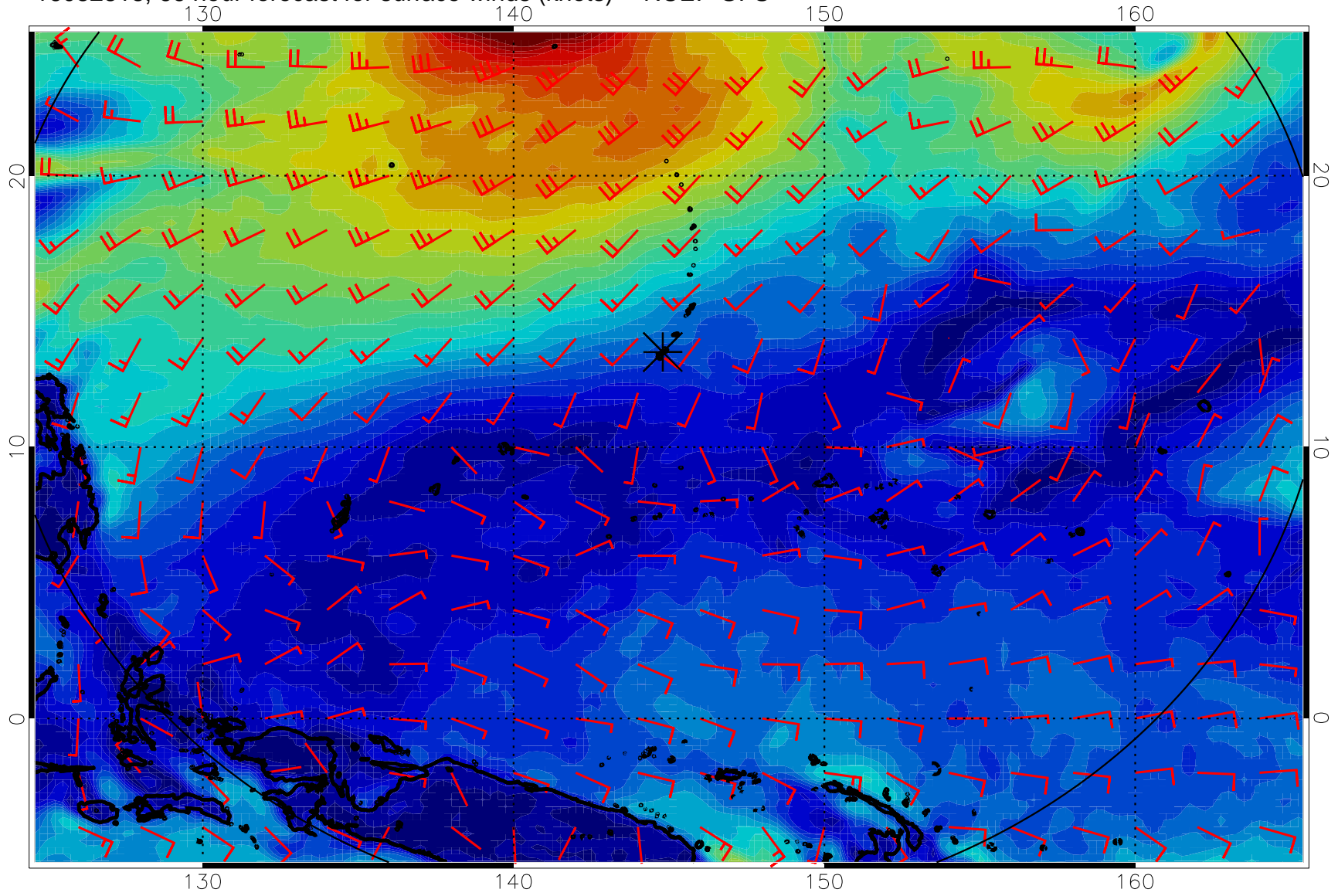
16082818, 66 hour forecast for surface winds (knots) -- NCEP GFS
