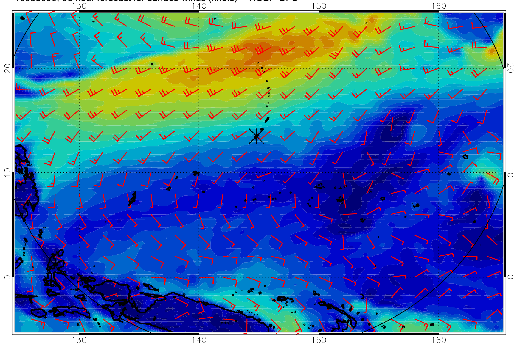
16083000, 96 hour forecast for surface winds (knots) -- NCEP GFS
