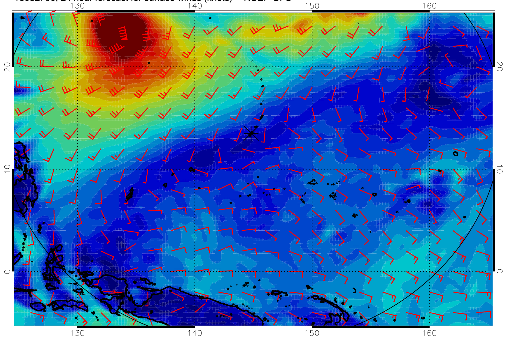
16082700, 24 hour forecast for surface winds (knots) -- NCEP GFS
