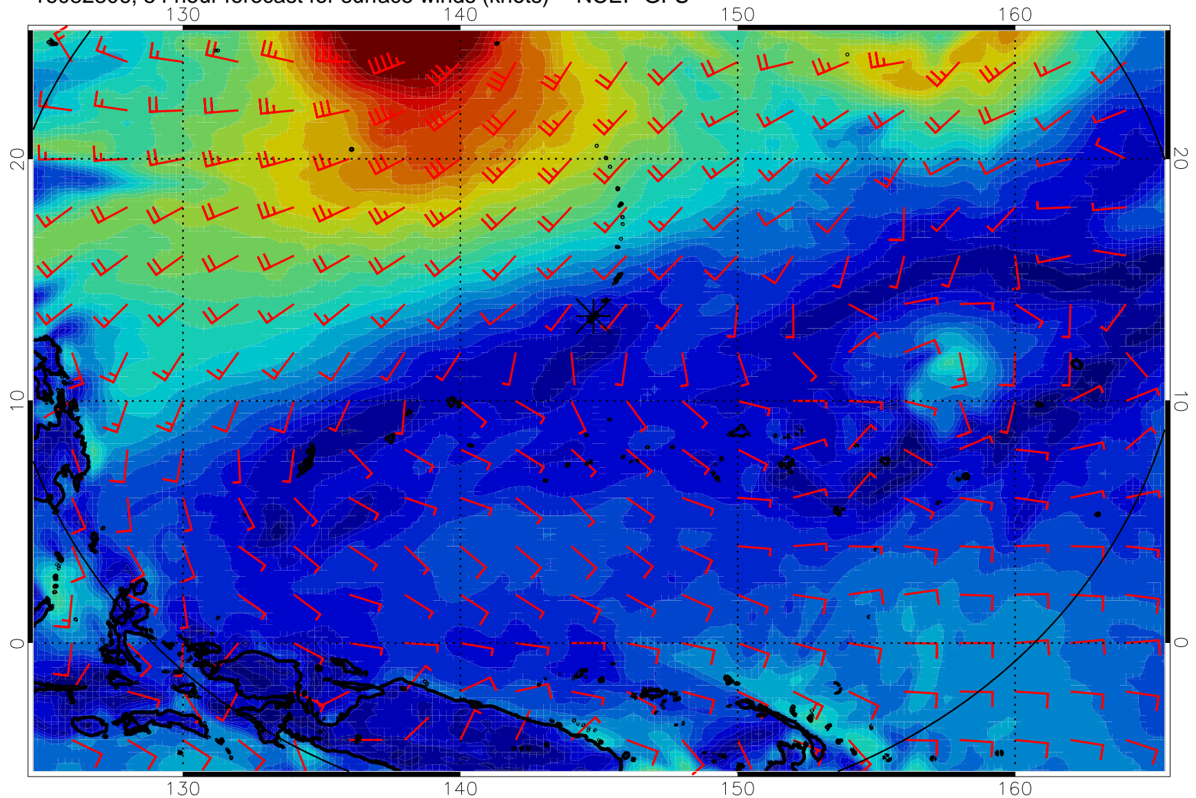
16082806, 54 hour forecast for surface winds (knots) -- NCEP GFS
