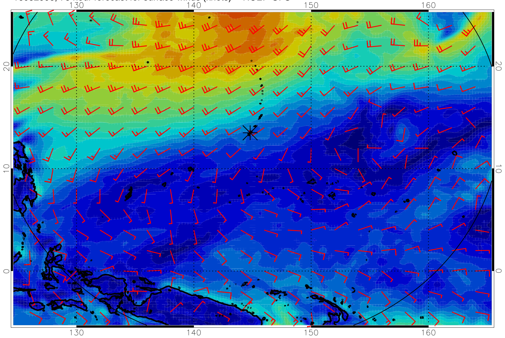
16082906, 78 hour forecast for surface winds (knots) -- NCEP GFS
