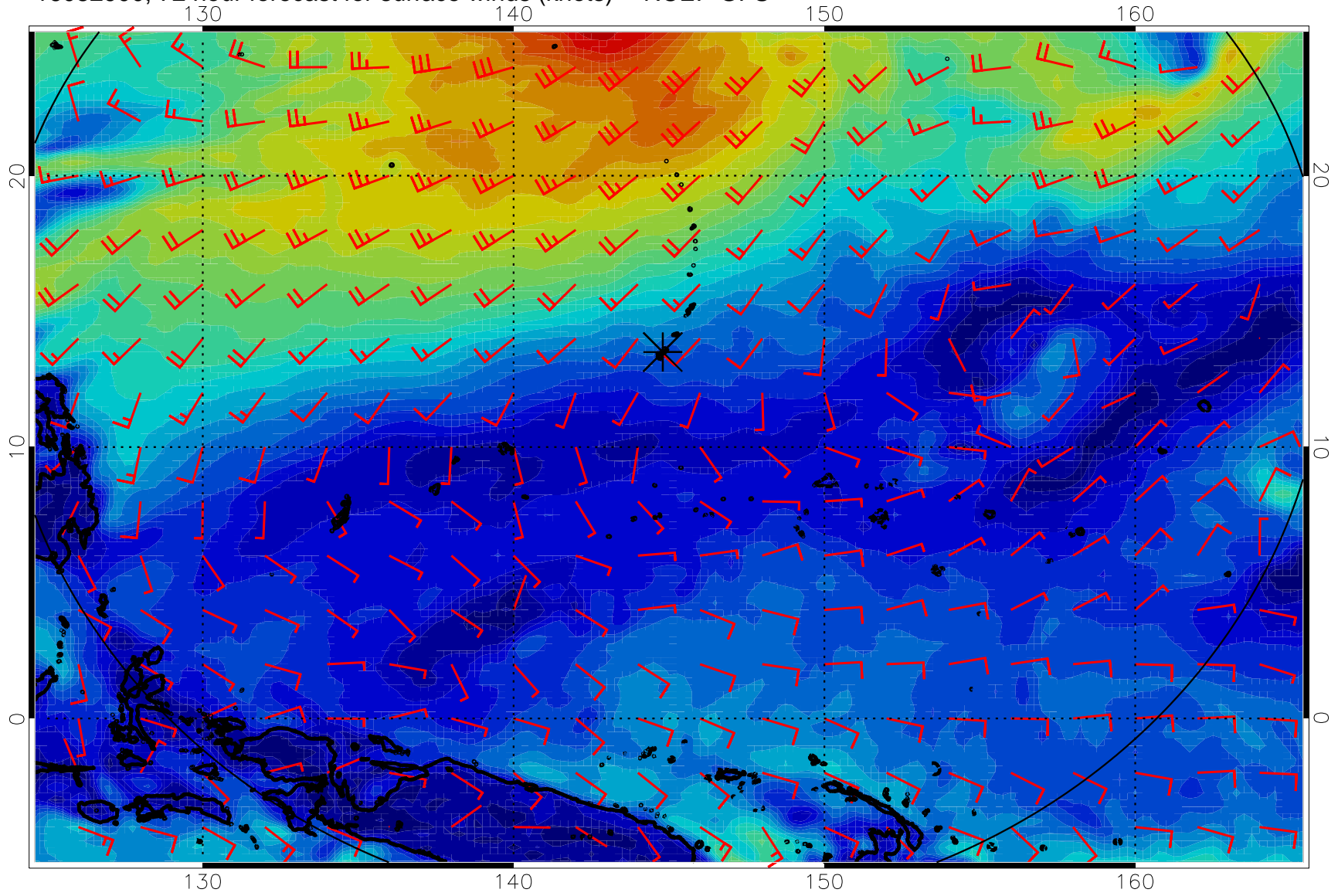
16082900, 72 hour forecast for surface winds (knots) -- NCEP GFS
