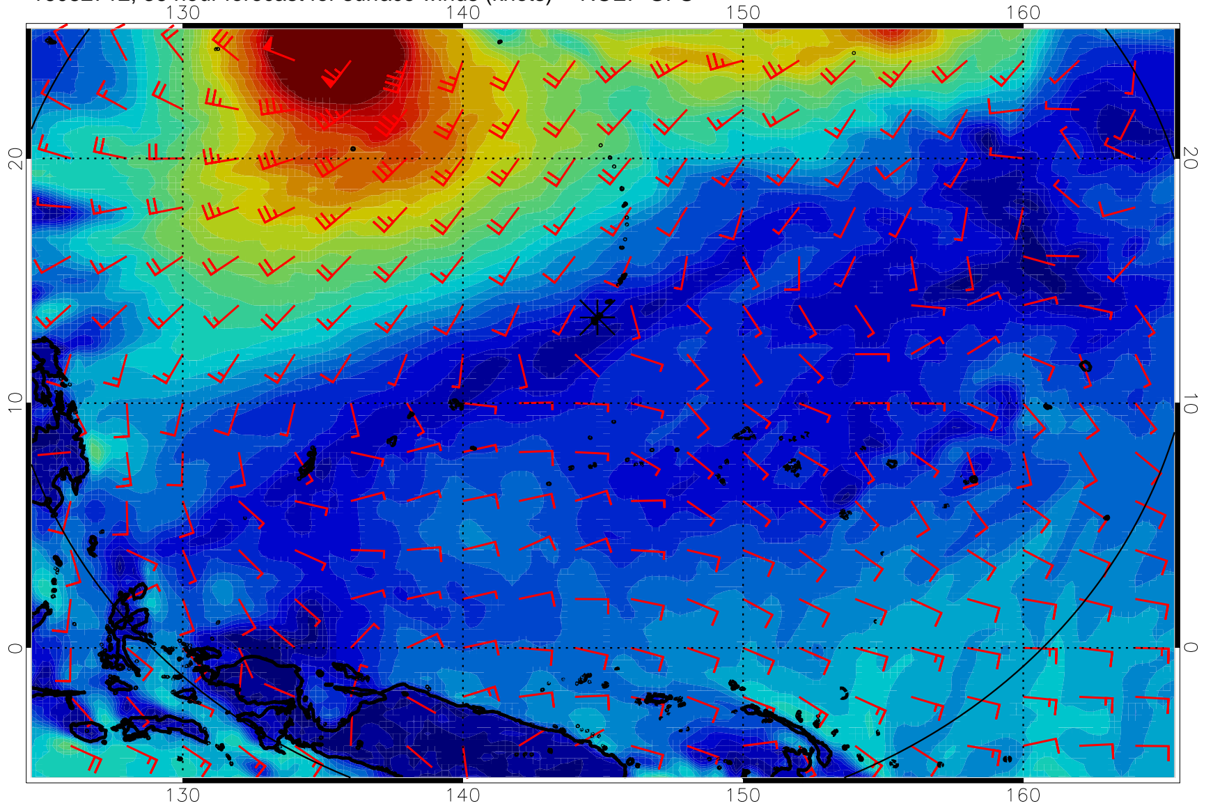
16082712, 36 hour forecast for surface winds (knots) -- NCEP GFS
