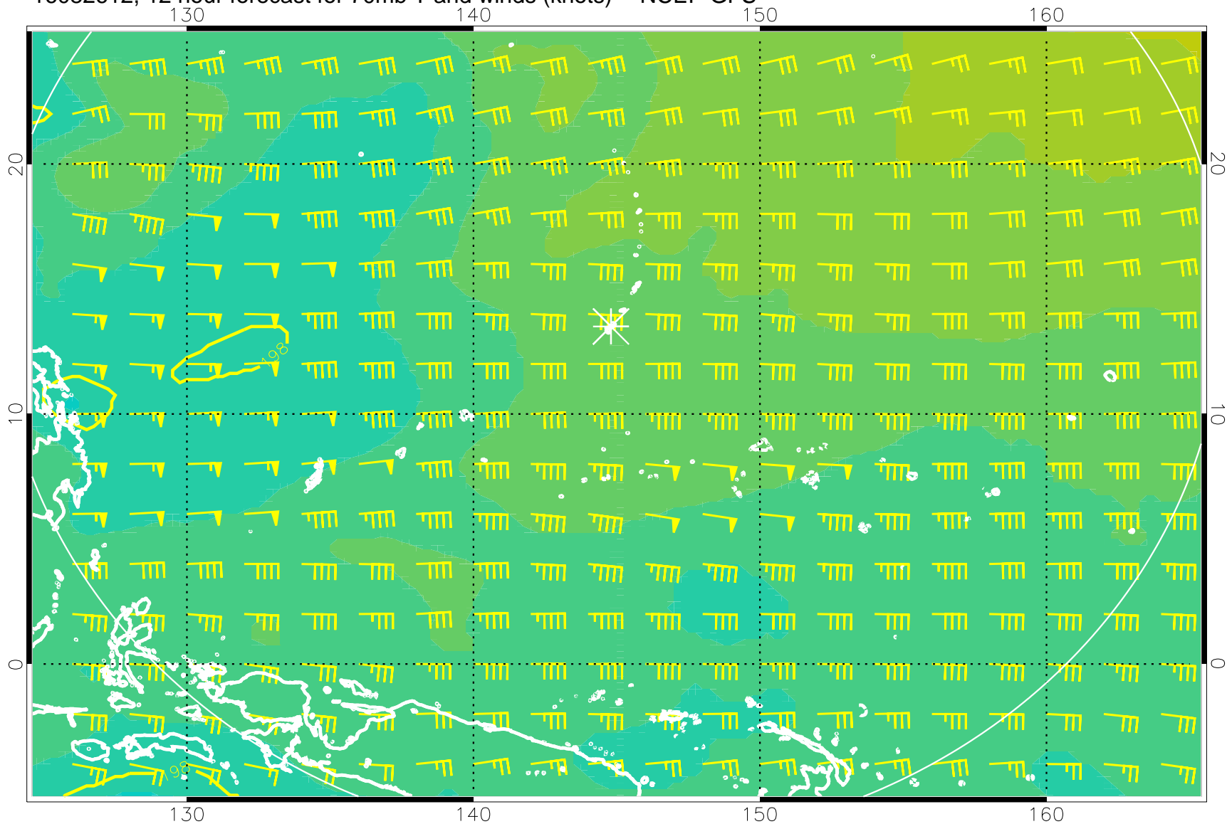
16082612, 12 hour forecast for 70mb T and winds (knots) -- NCEP GFS
