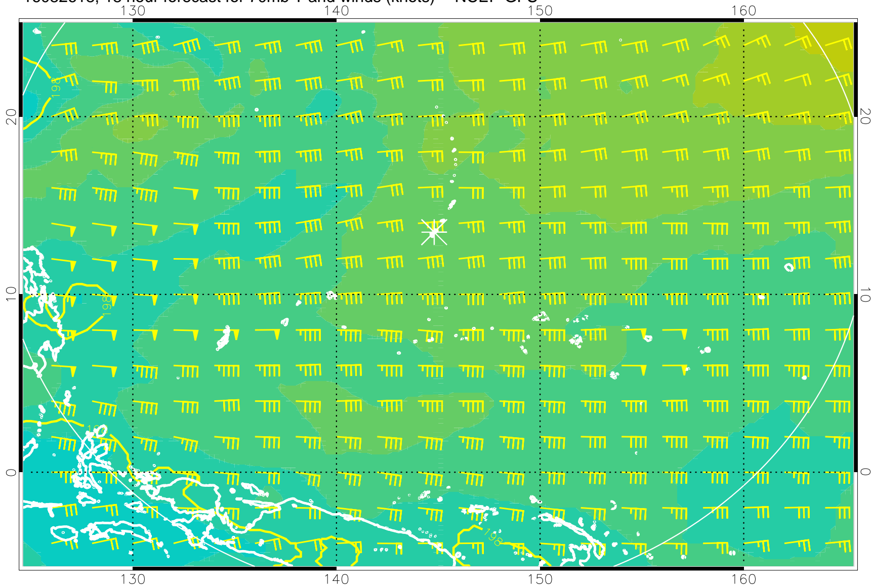
16082618, 18 hour forecast for 70mb T and winds (knots) -- NCEP GFS
