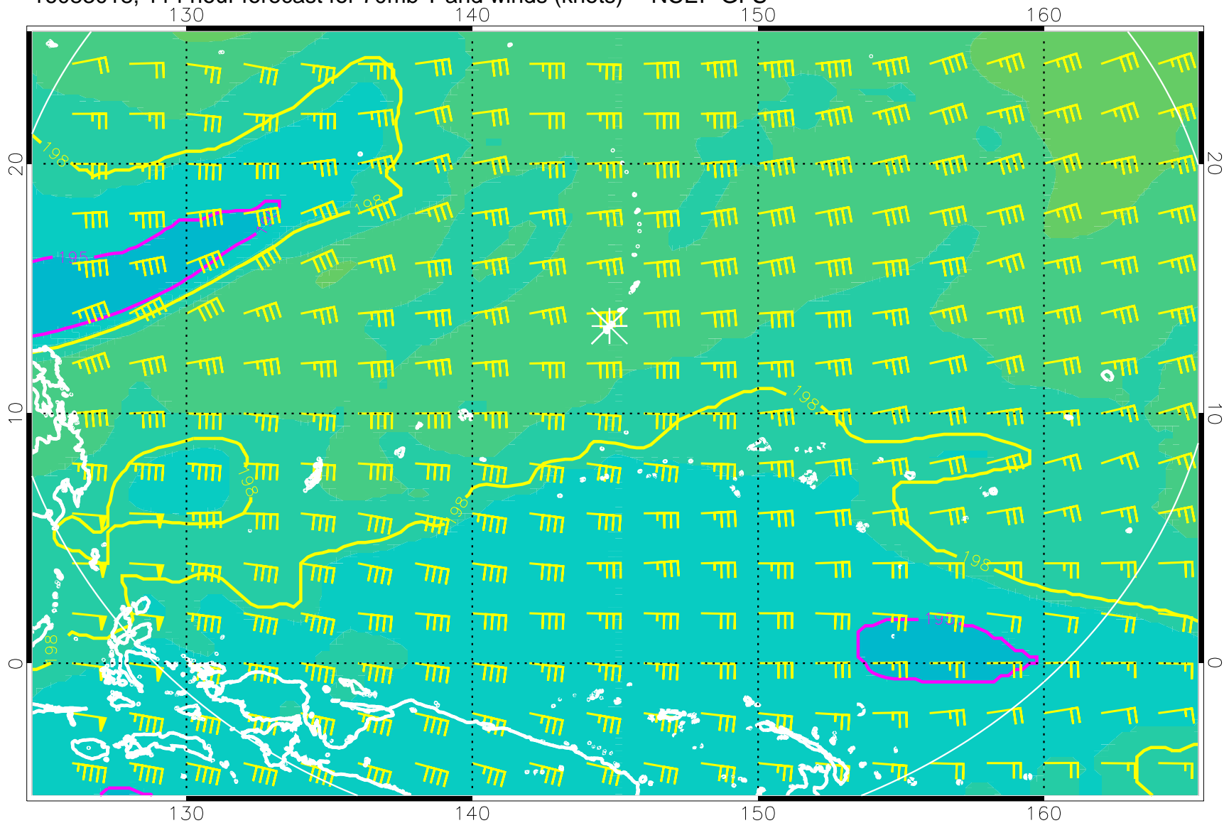
16083018, 114 hour forecast for 70mb T and winds (knots) -- NCEP GFS
