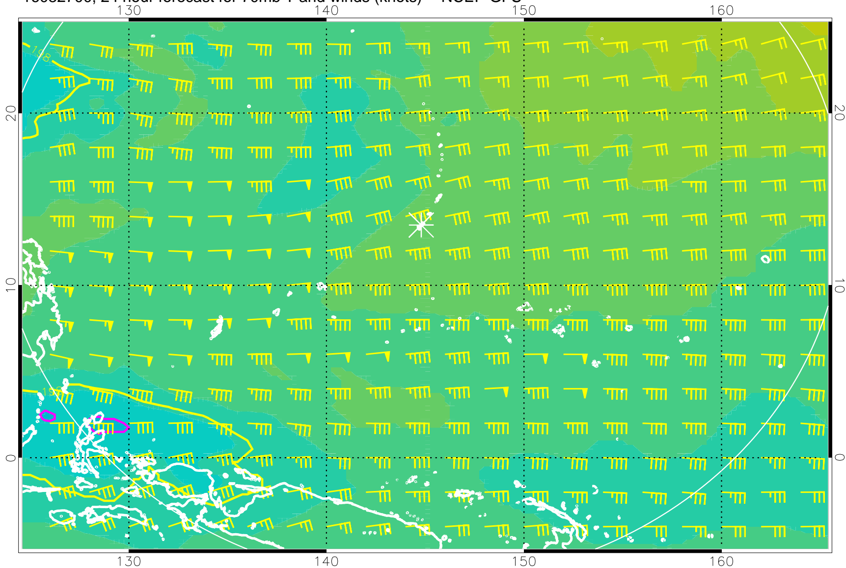
16082700, 24 hour forecast for 70mb T and winds (knots) -- NCEP GFS
