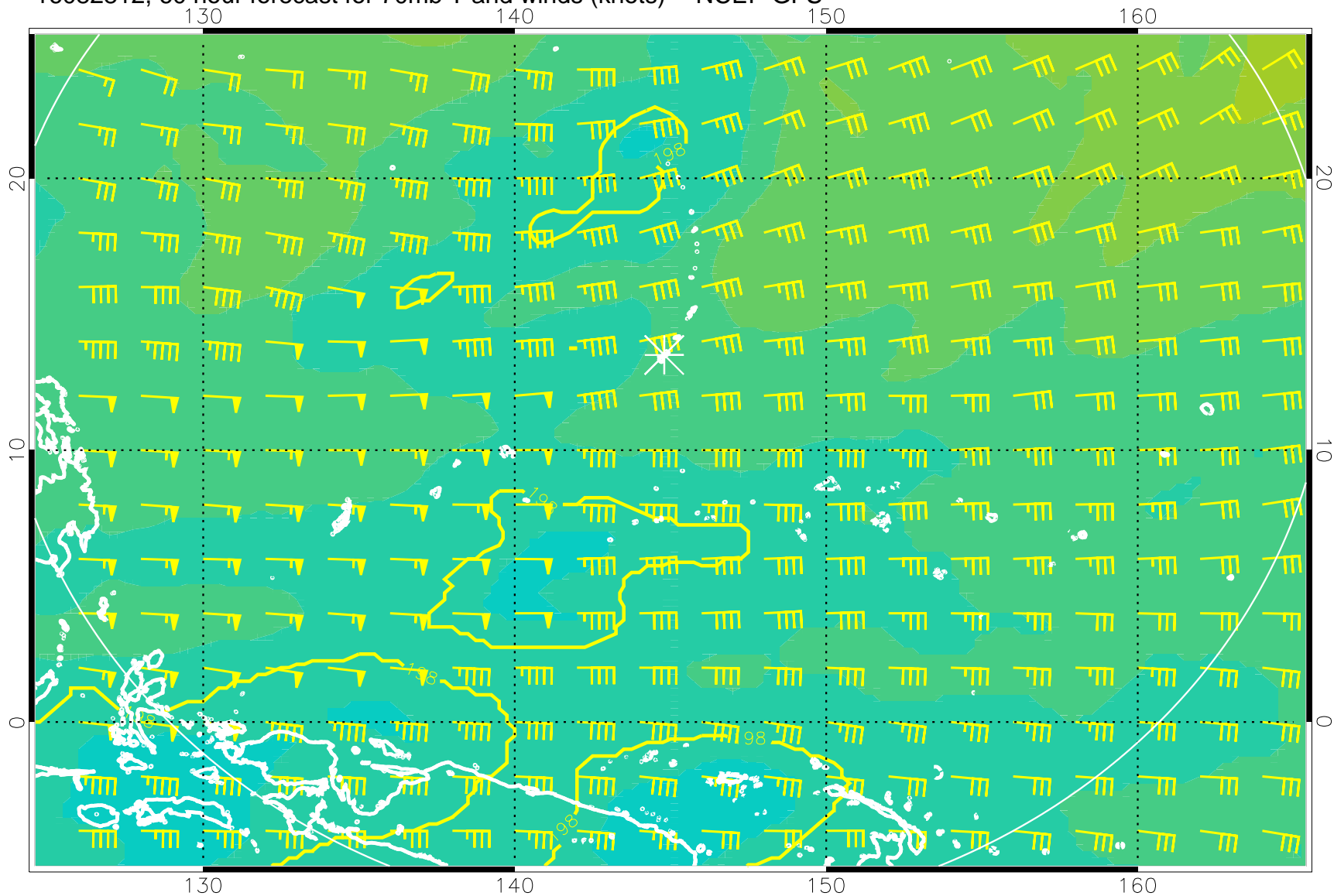
16082812, 60 hour forecast for 70mb T and winds (knots) -- NCEP GFS
