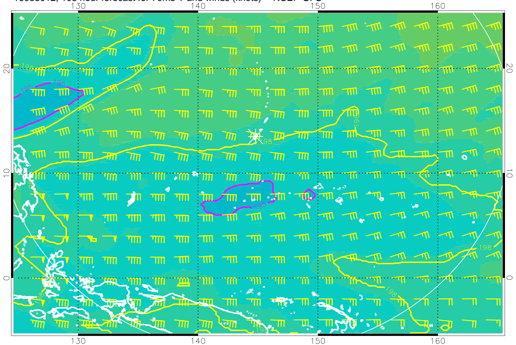
16083012, 108 hour forecast for 70mb T and winds (knots) -- NCEP GFS
