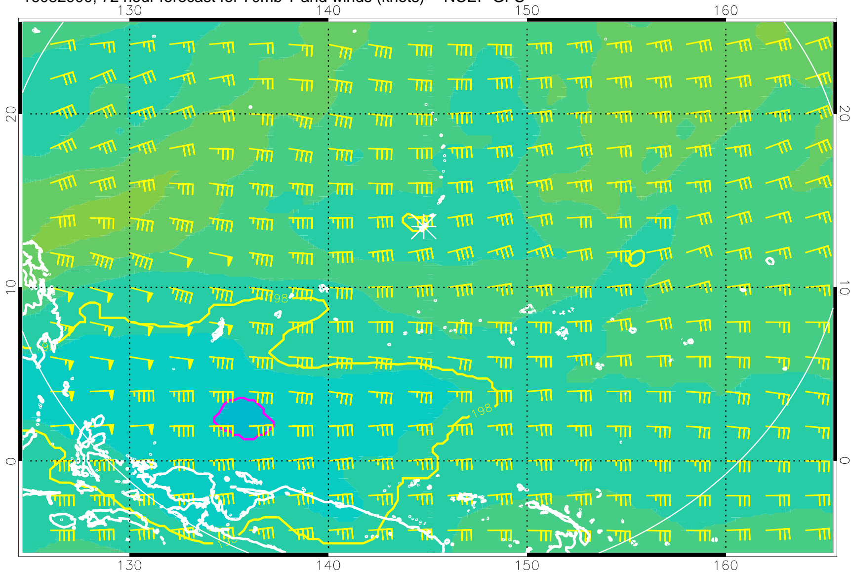
16082900, 72 hour forecast for 70mb T and winds (knots) -- NCEP GFS
