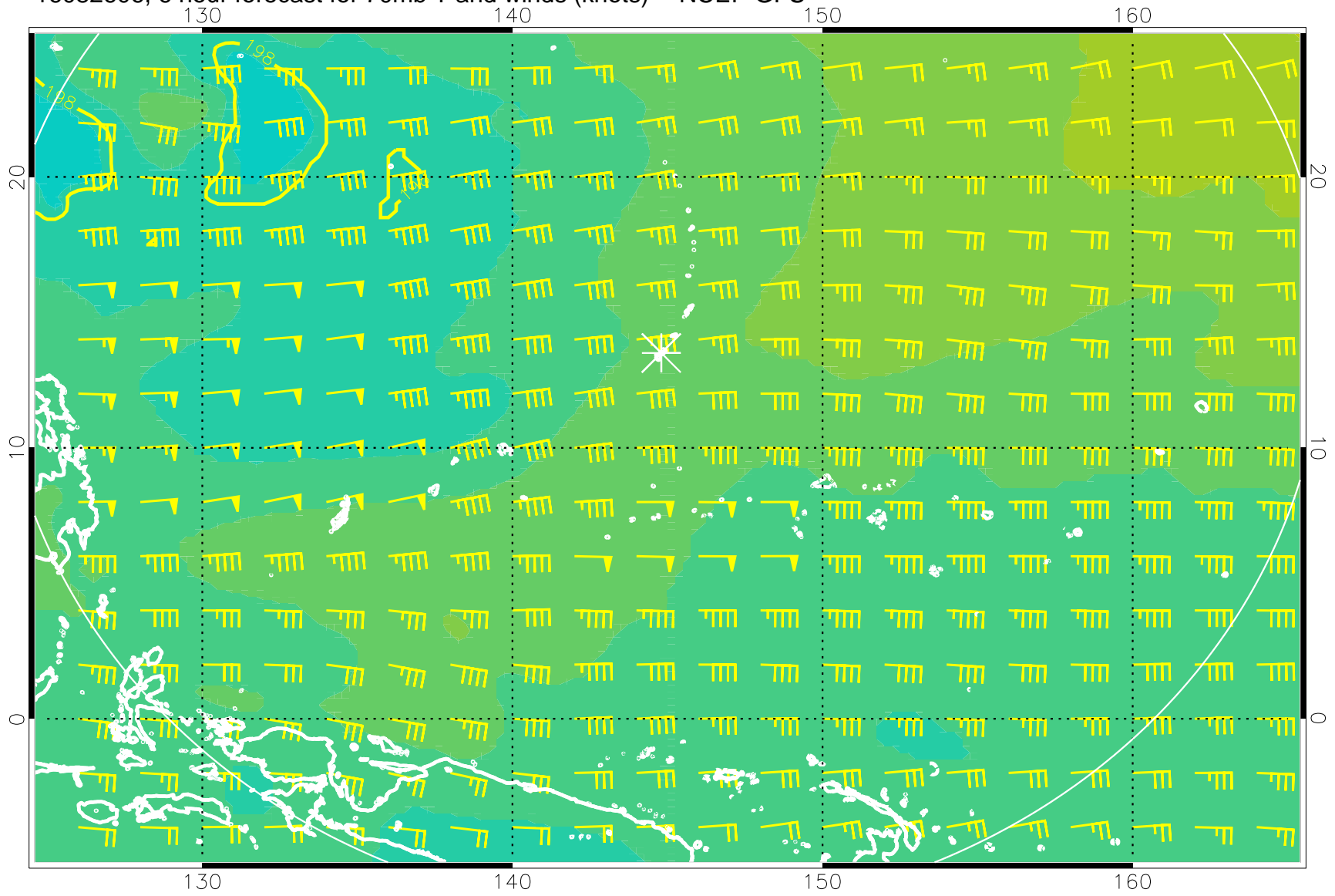
16082606, 6 hour forecast for 70mb T and winds (knots) -- NCEP GFS
