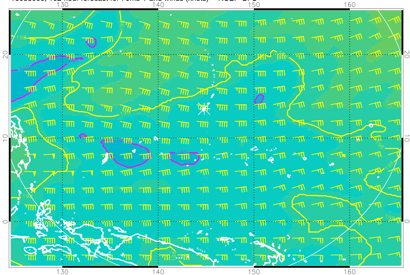
16083006, 102 hour forecast for 70mb T and winds (knots) -- NCEP GFS
