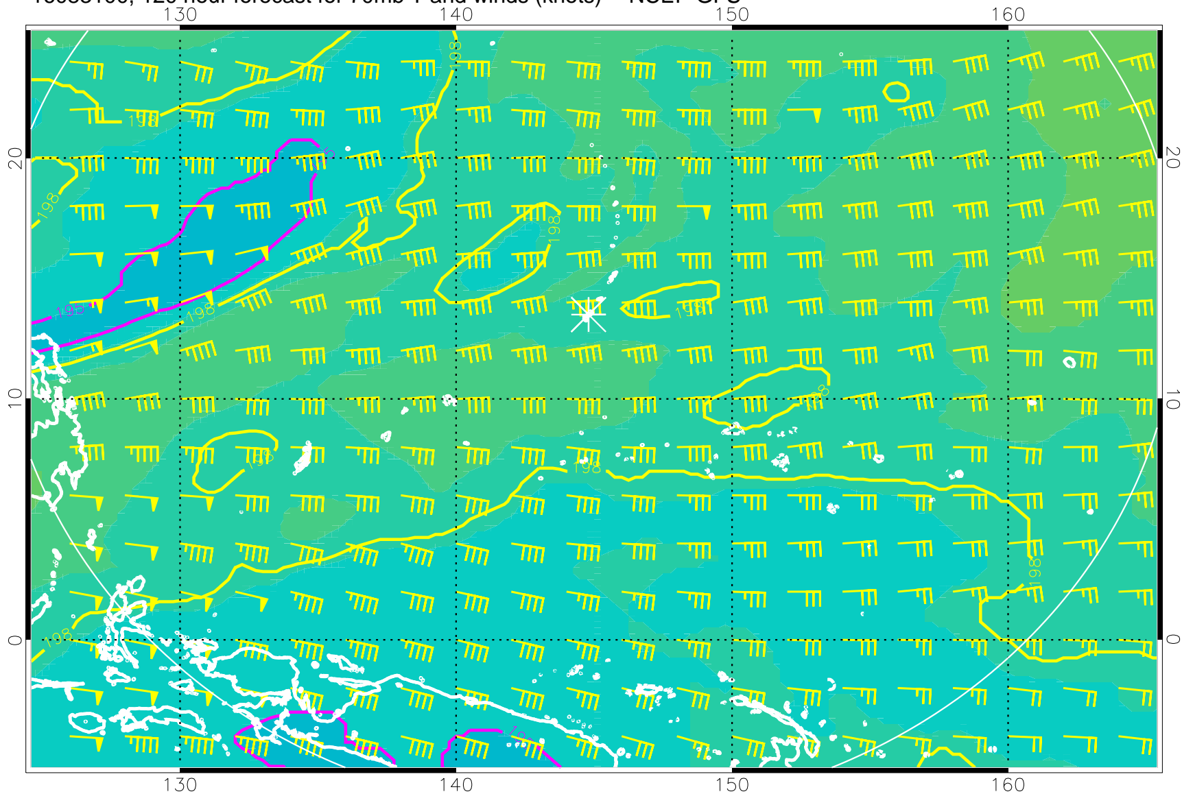
16083100, 120 hour forecast for 70mb T and winds (knots) -- NCEP GFS
