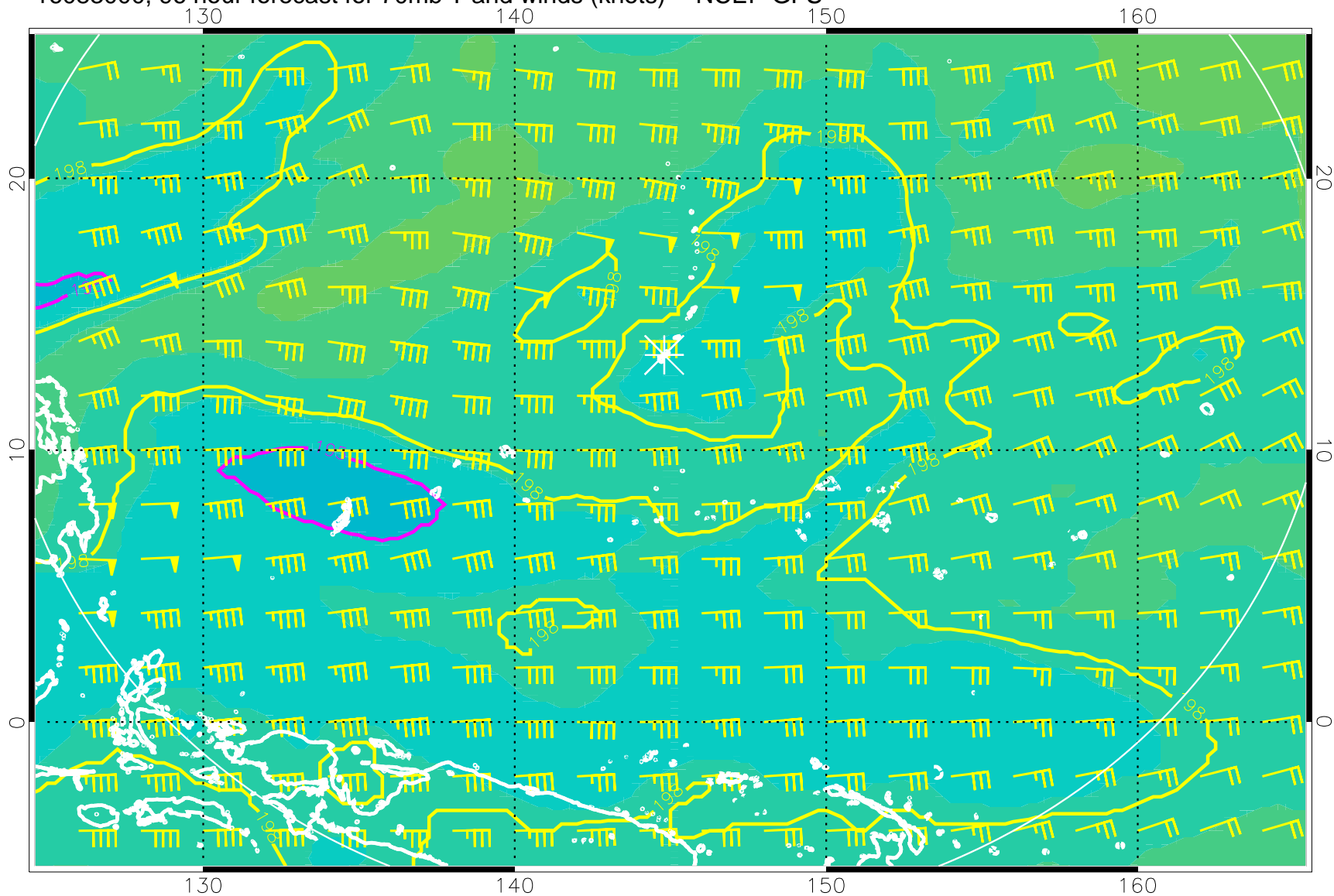
16083000, 96 hour forecast for 70mb T and winds (knots) -- NCEP GFS
