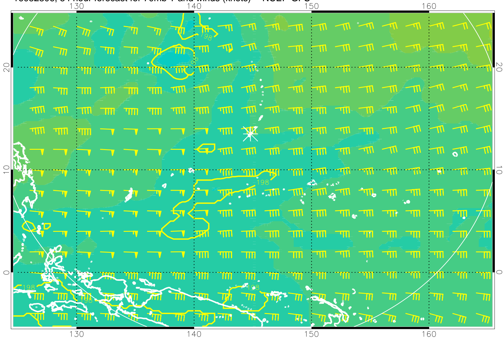
16082806, 54 hour forecast for 70mb T and winds (knots) -- NCEP GFS
