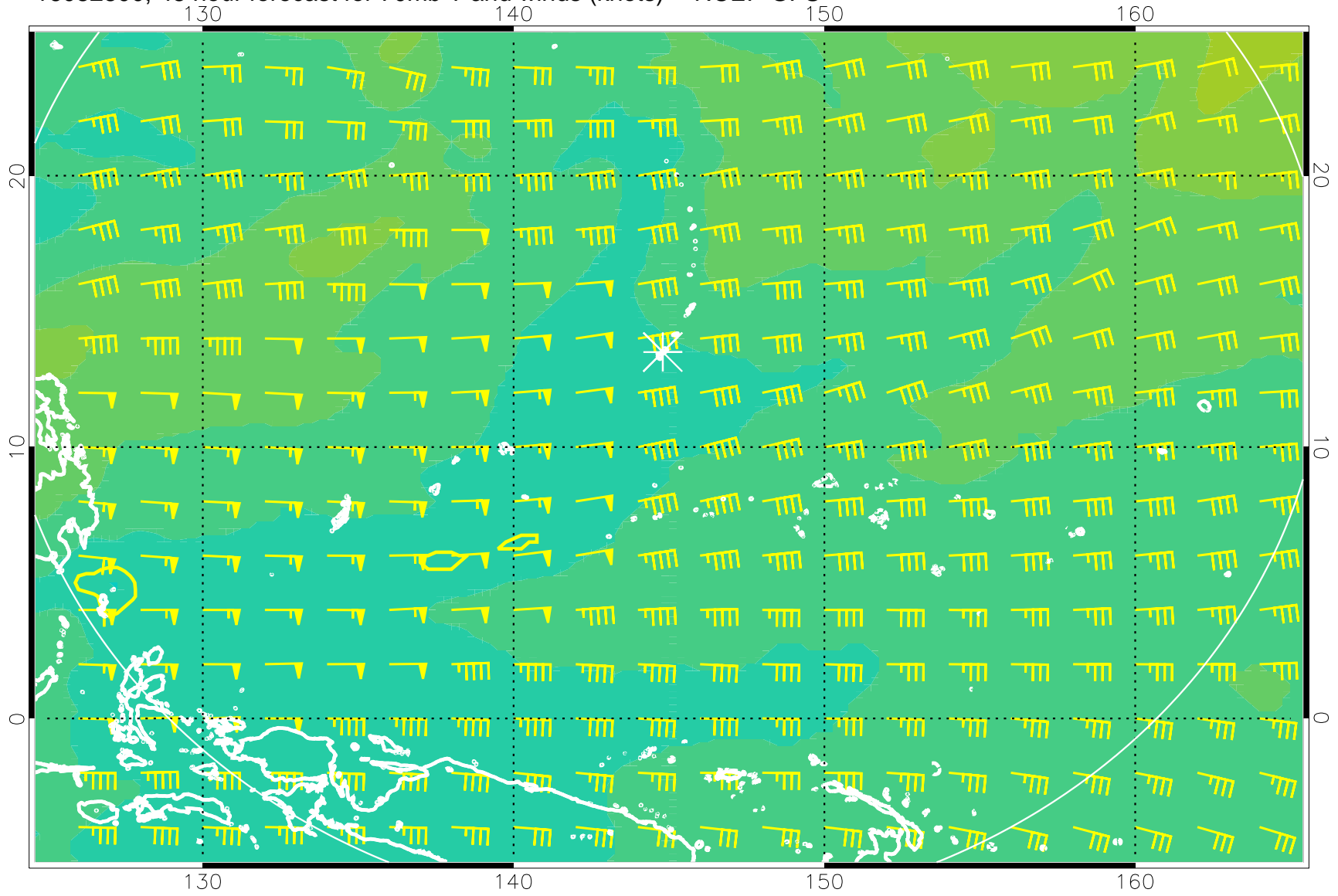
16082800, 48 hour forecast for 70mb T and winds (knots) -- NCEP GFS
