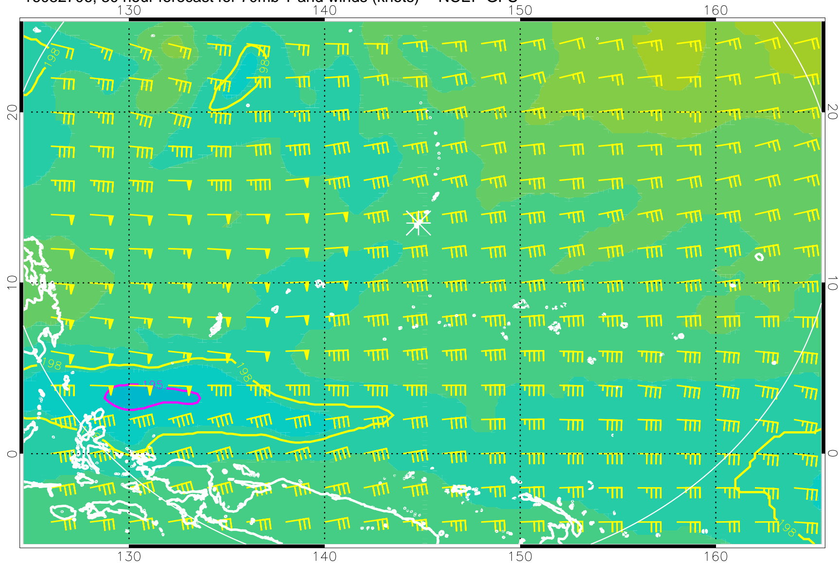
16082706, 30 hour forecast for 70mb T and winds (knots) -- NCEP GFS
