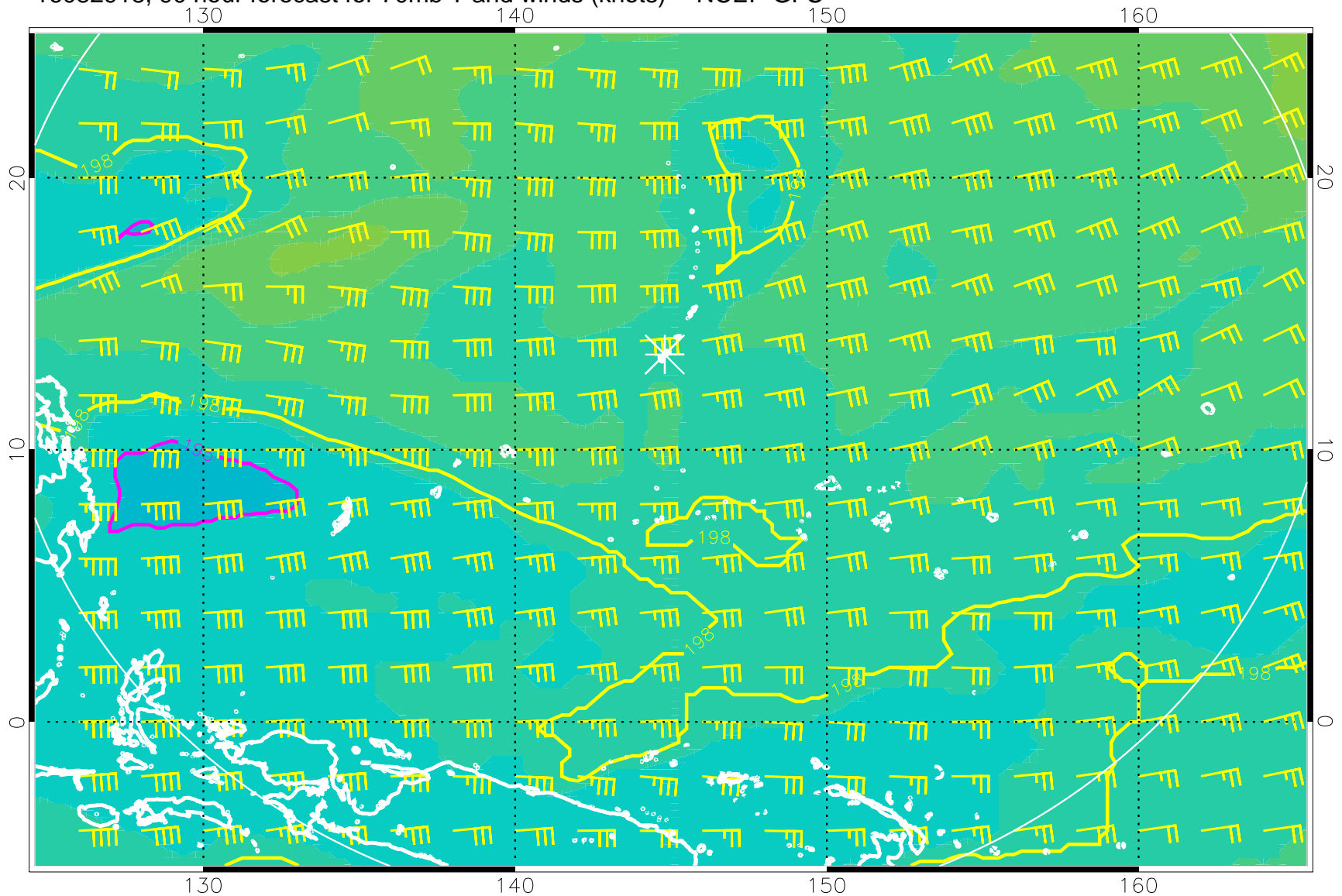
16082918, 90 hour forecast for 70mb T and winds (knots) -- NCEP GFS
