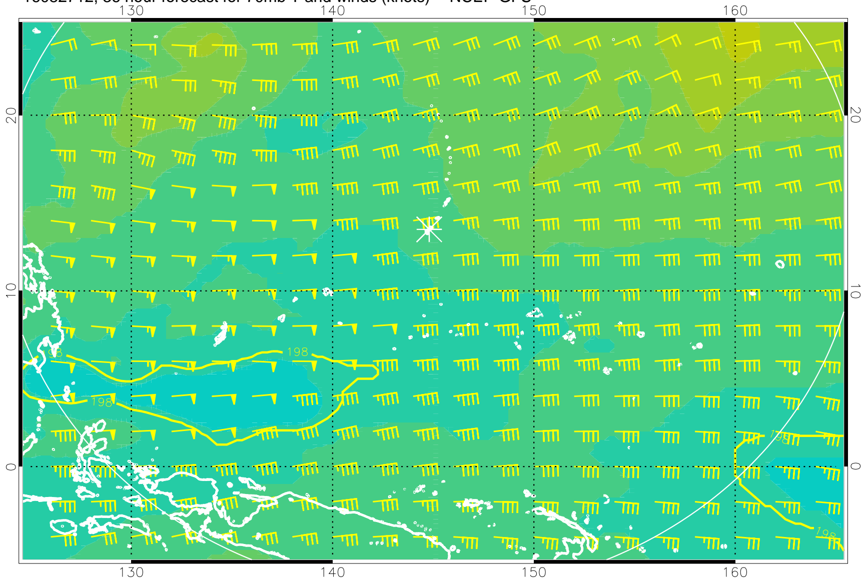
16082712, 36 hour forecast for 70mb T and winds (knots) -- NCEP GFS
