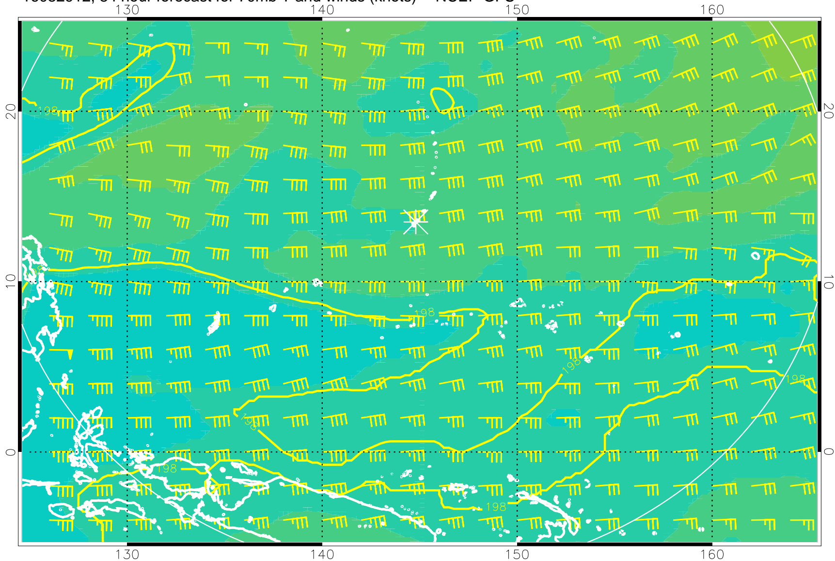
16082912, 84 hour forecast for 70mb T and winds (knots) -- NCEP GFS
