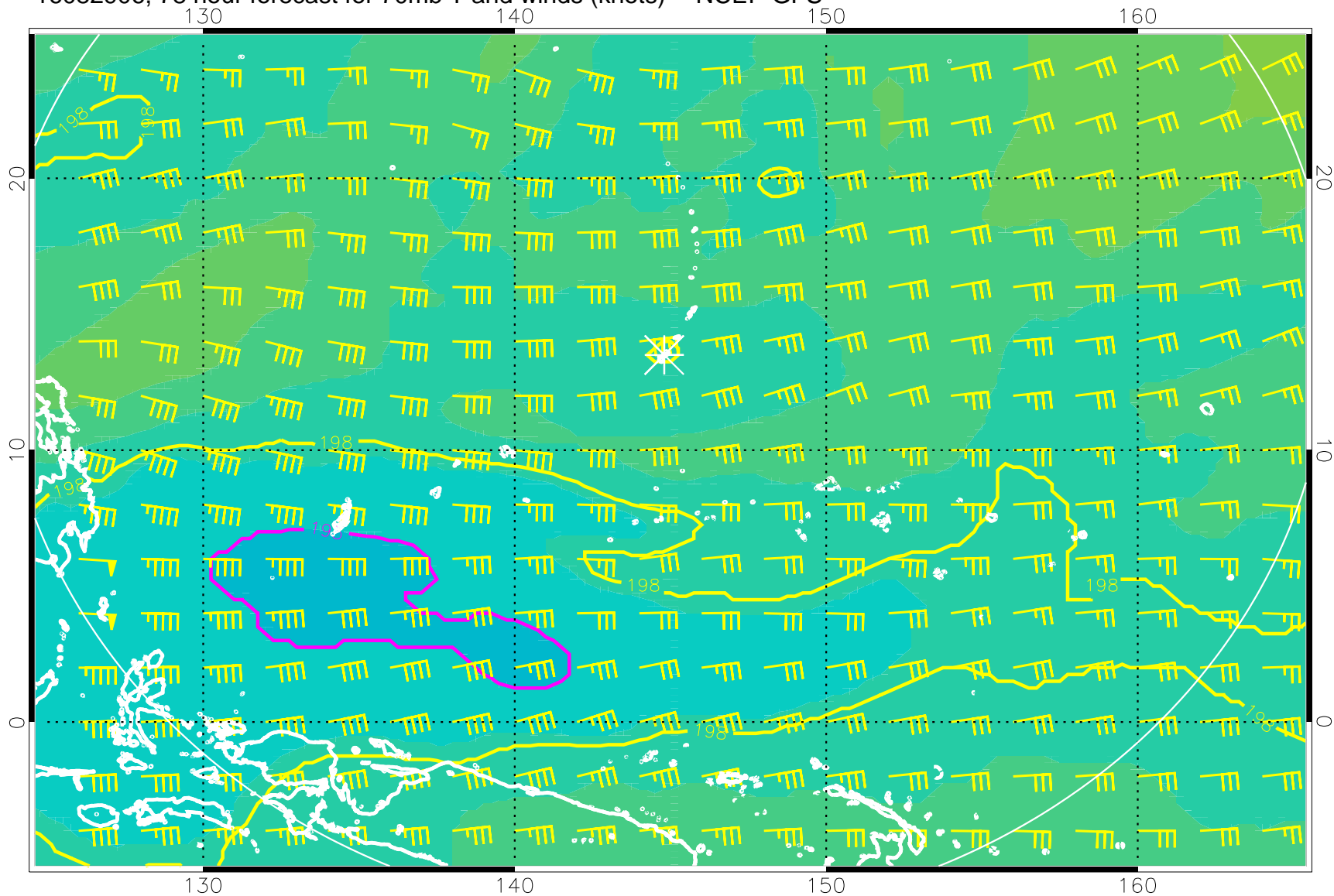
16082906, 78 hour forecast for 70mb T and winds (knots) -- NCEP GFS
