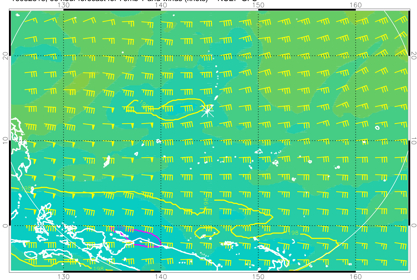
16082818, 66 hour forecast for 70mb T and winds (knots) -- NCEP GFS
