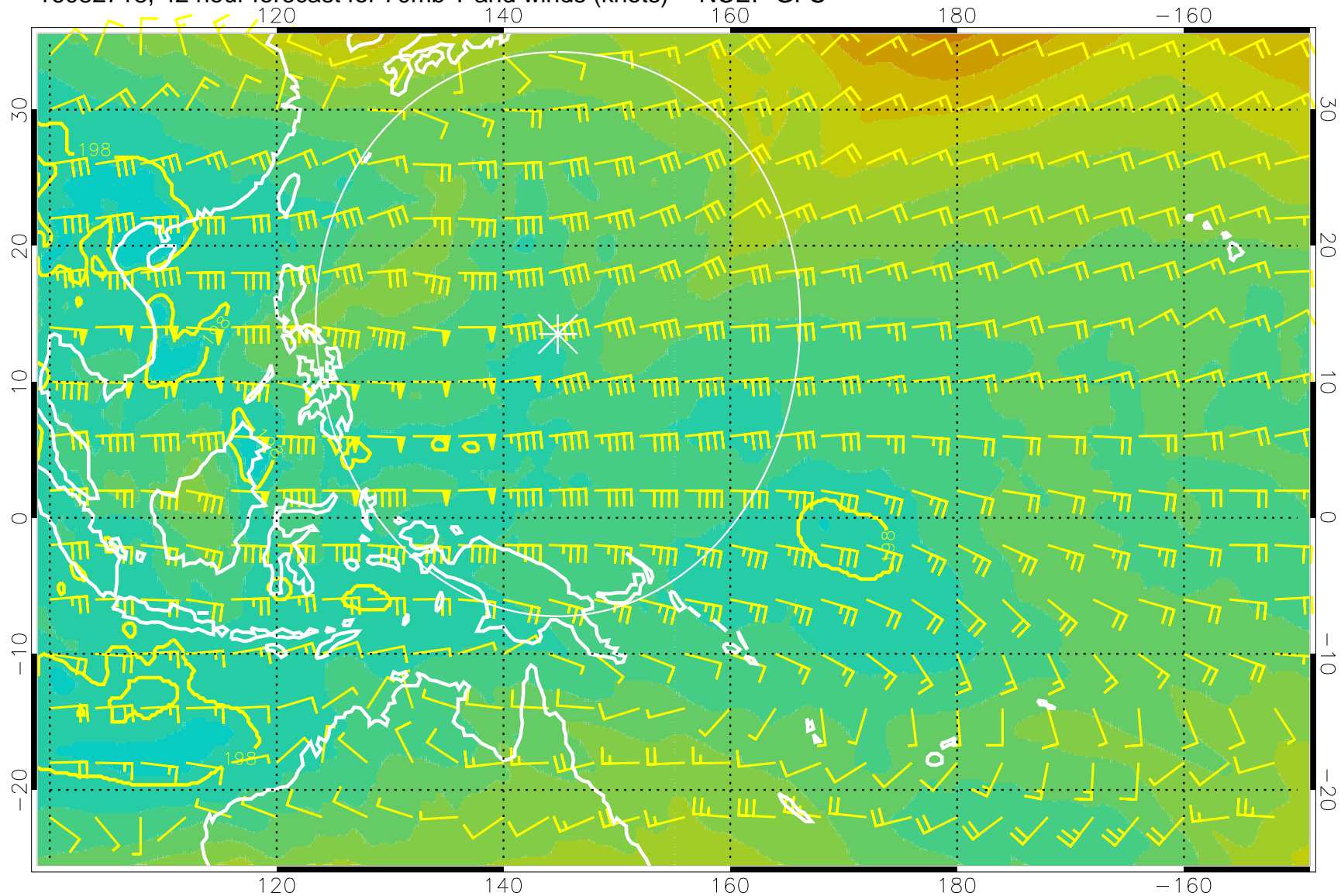
16082718, 42 hour forecast for 70mb T and winds (knots) -- NCEP GFS
