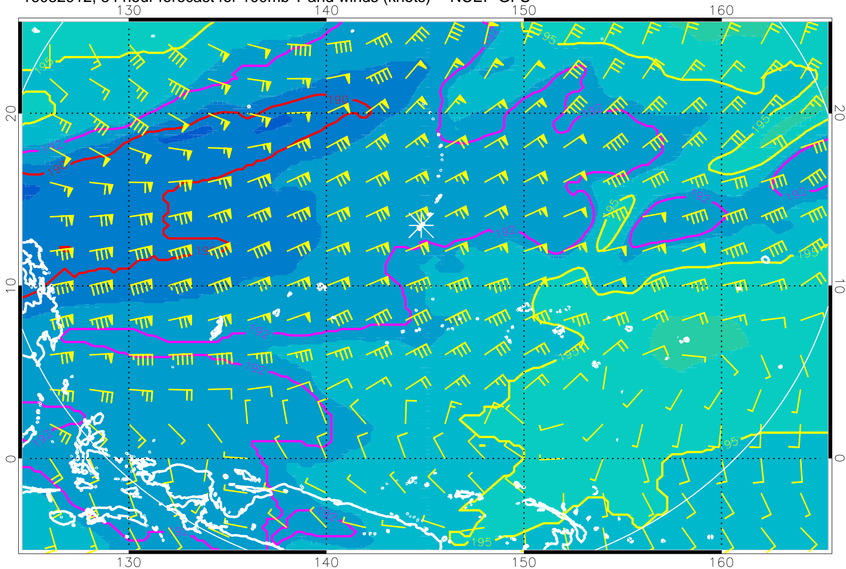
16082912, 84 hour forecast for 100mb T and winds (knots) -- NCEP GFS
