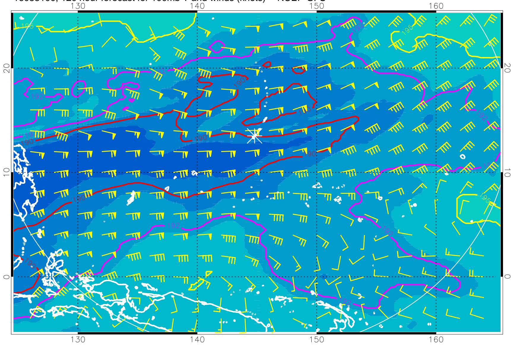
16083100, 120 hour forecast for 100mb T and winds (knots) -- NCEP GFS
