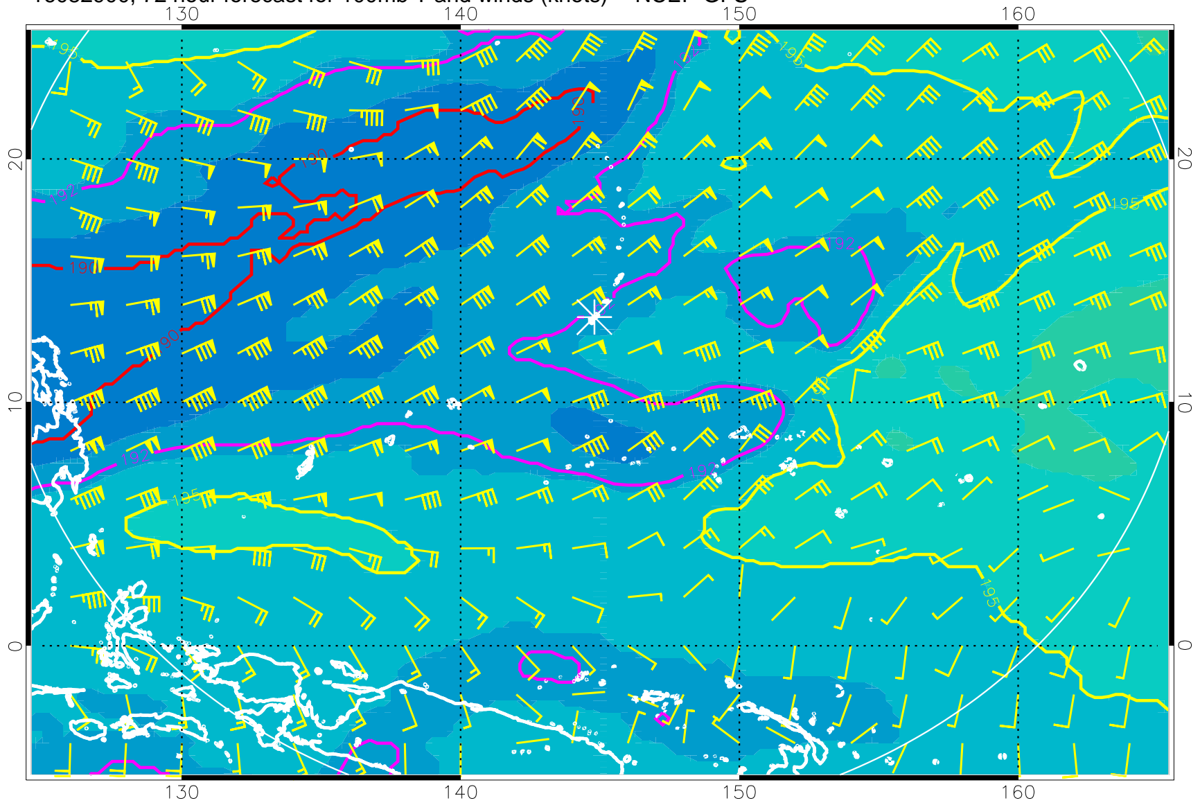
16082900, 72 hour forecast for 100mb T and winds (knots) -- NCEP GFS
