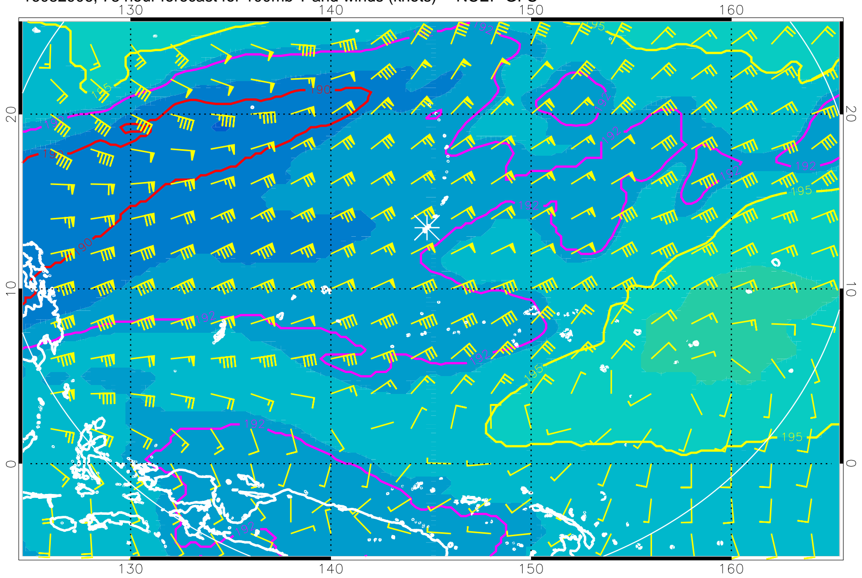
16082906, 78 hour forecast for 100mb T and winds (knots) -- NCEP GFS
