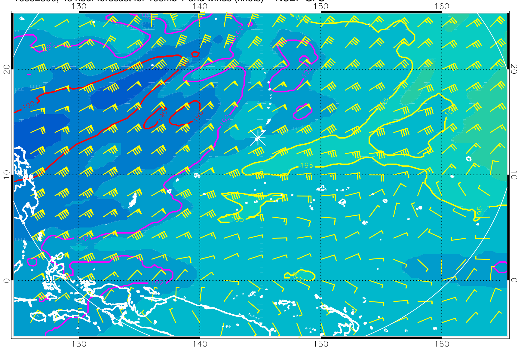
16082800, 48 hour forecast for 100mb T and winds (knots) -- NCEP GFS
