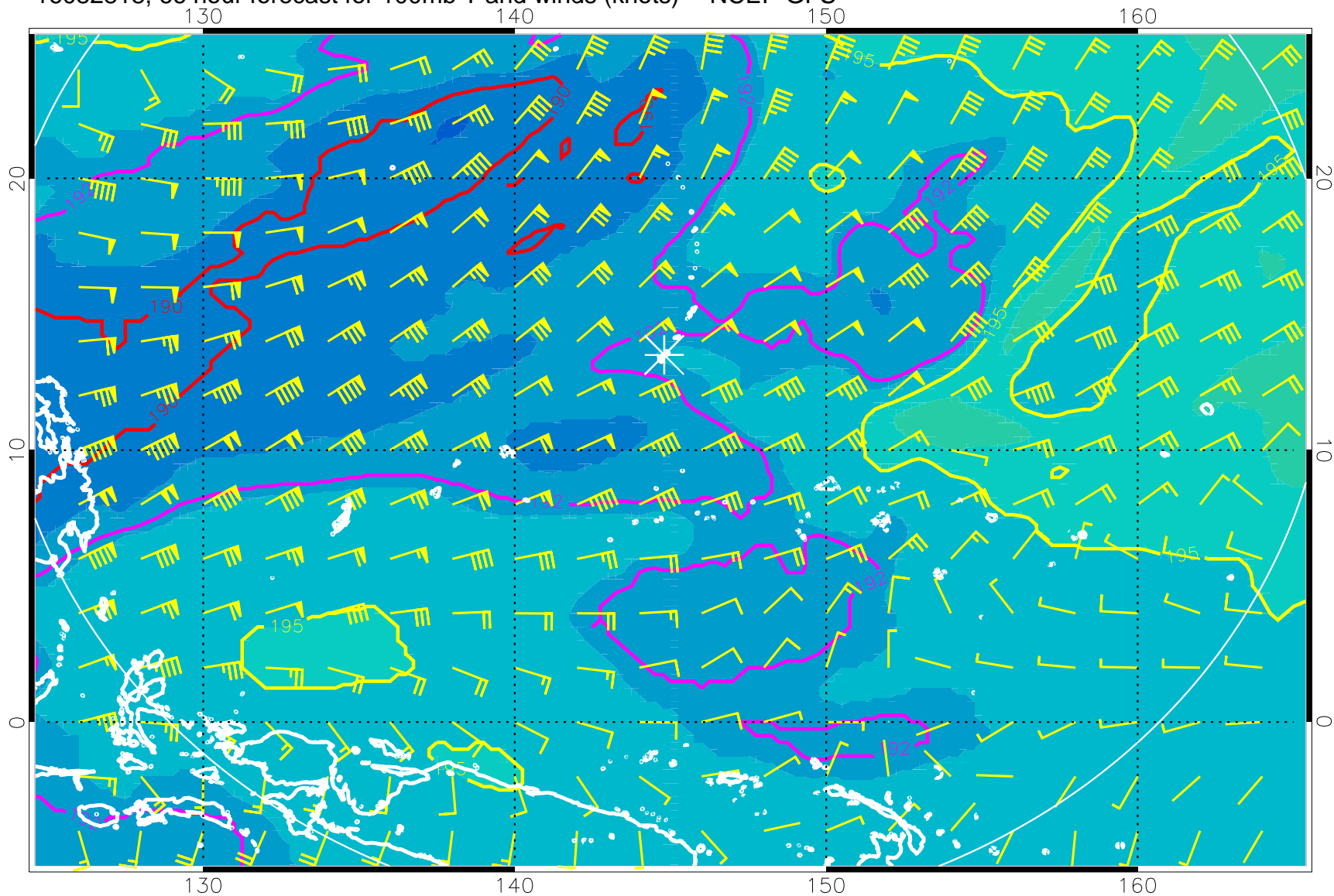
16082818, 66 hour forecast for 100mb T and winds (knots) -- NCEP GFS
