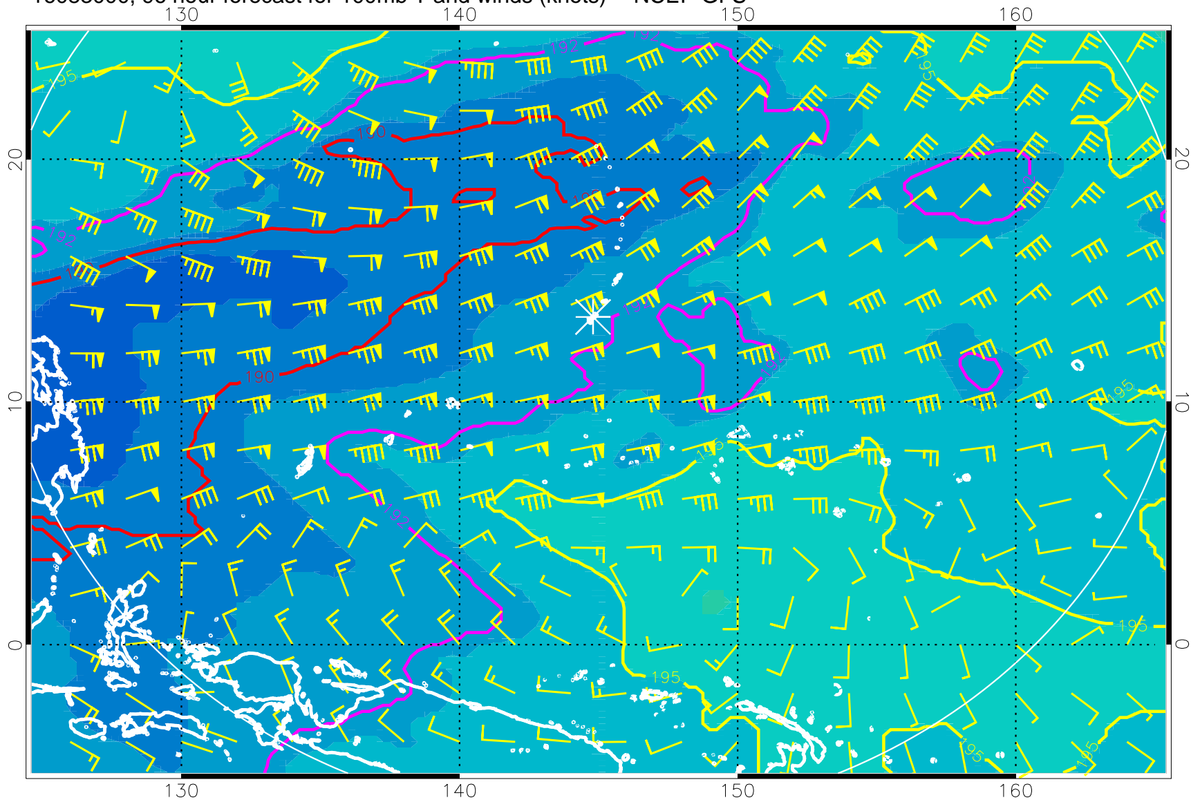
16083000, 96 hour forecast for 100mb T and winds (knots) -- NCEP GFS
