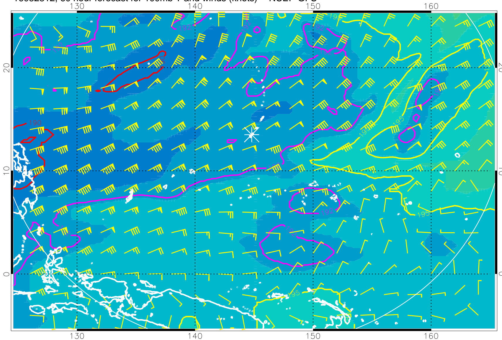
16082812, 60 hour forecast for 100mb T and winds (knots) -- NCEP GFS
