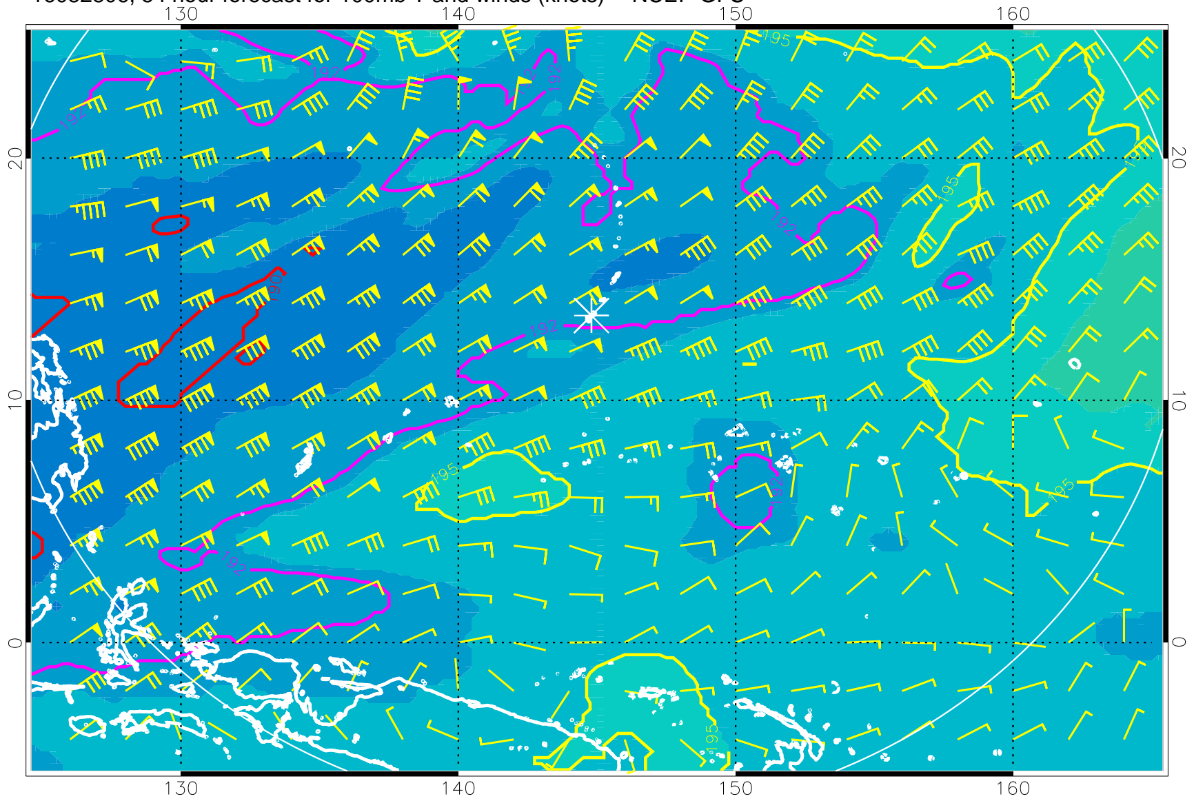
16082806, 54 hour forecast for 100mb T and winds (knots) -- NCEP GFS
