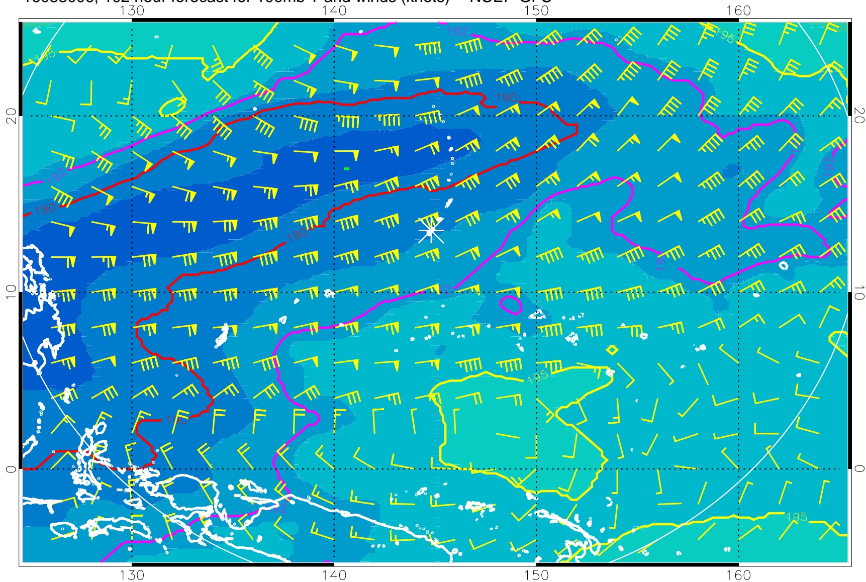
16083006, 102 hour forecast for 100mb T and winds (knots) -- NCEP GFS
