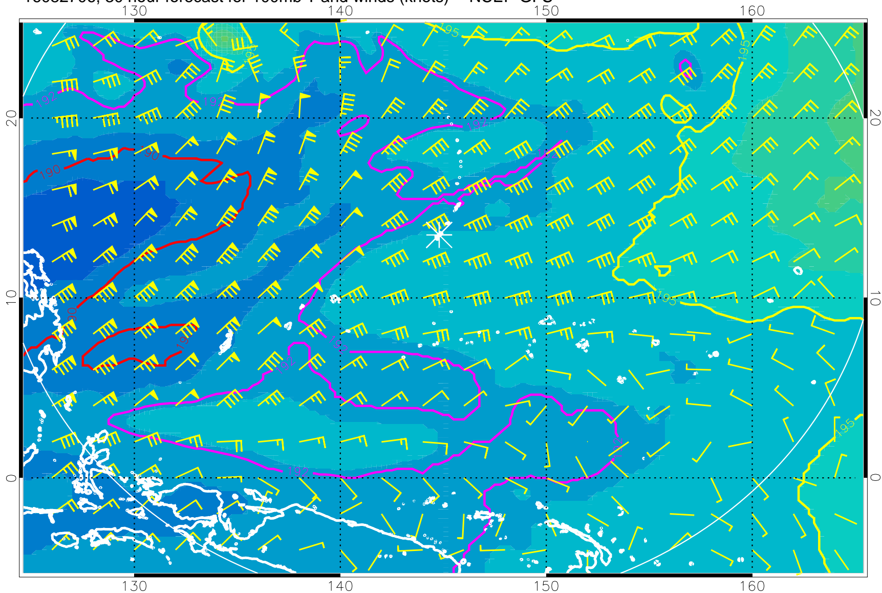
16082706, 30 hour forecast for 100mb T and winds (knots) -- NCEP GFS
