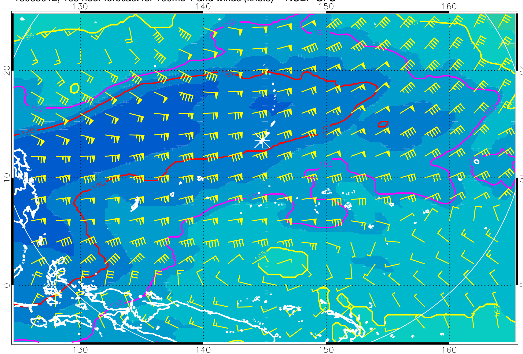
16083012, 108 hour forecast for 100mb T and winds (knots) -- NCEP GFS
