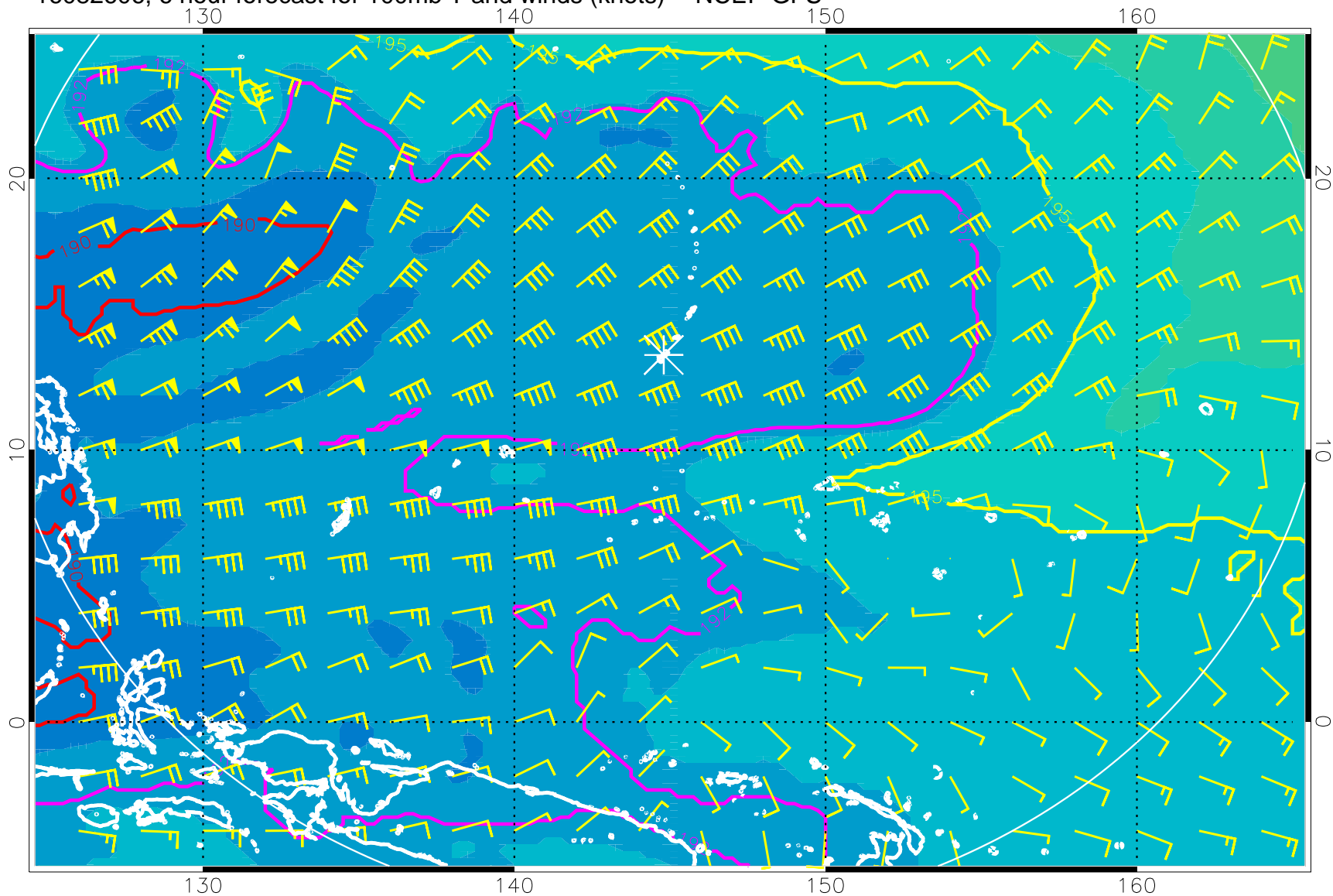
16082606, 6 hour forecast for 100mb T and winds (knots) -- NCEP GFS
