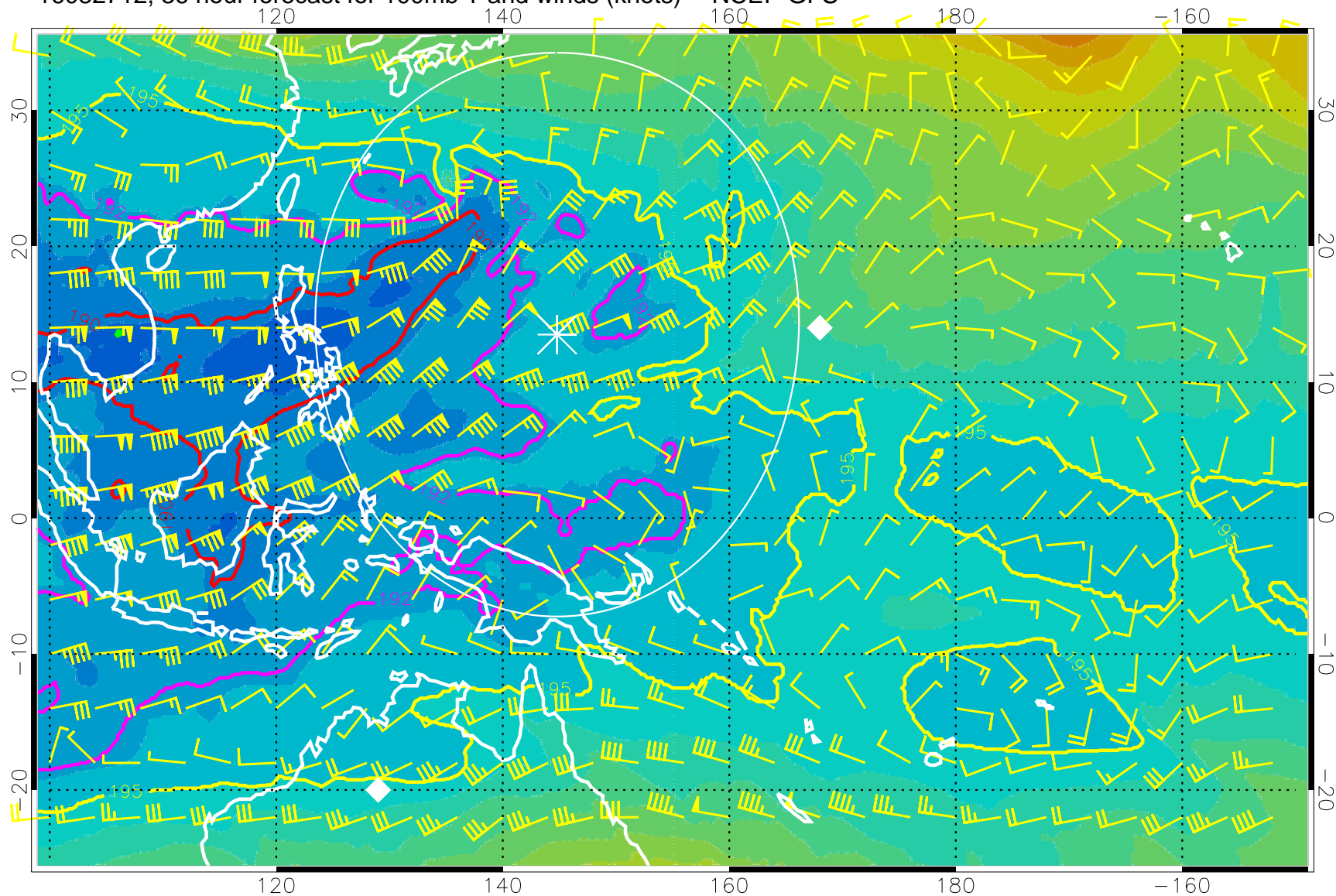
16082712, 36 hour forecast for 100mb T and winds (knots) -- NCEP GFS
