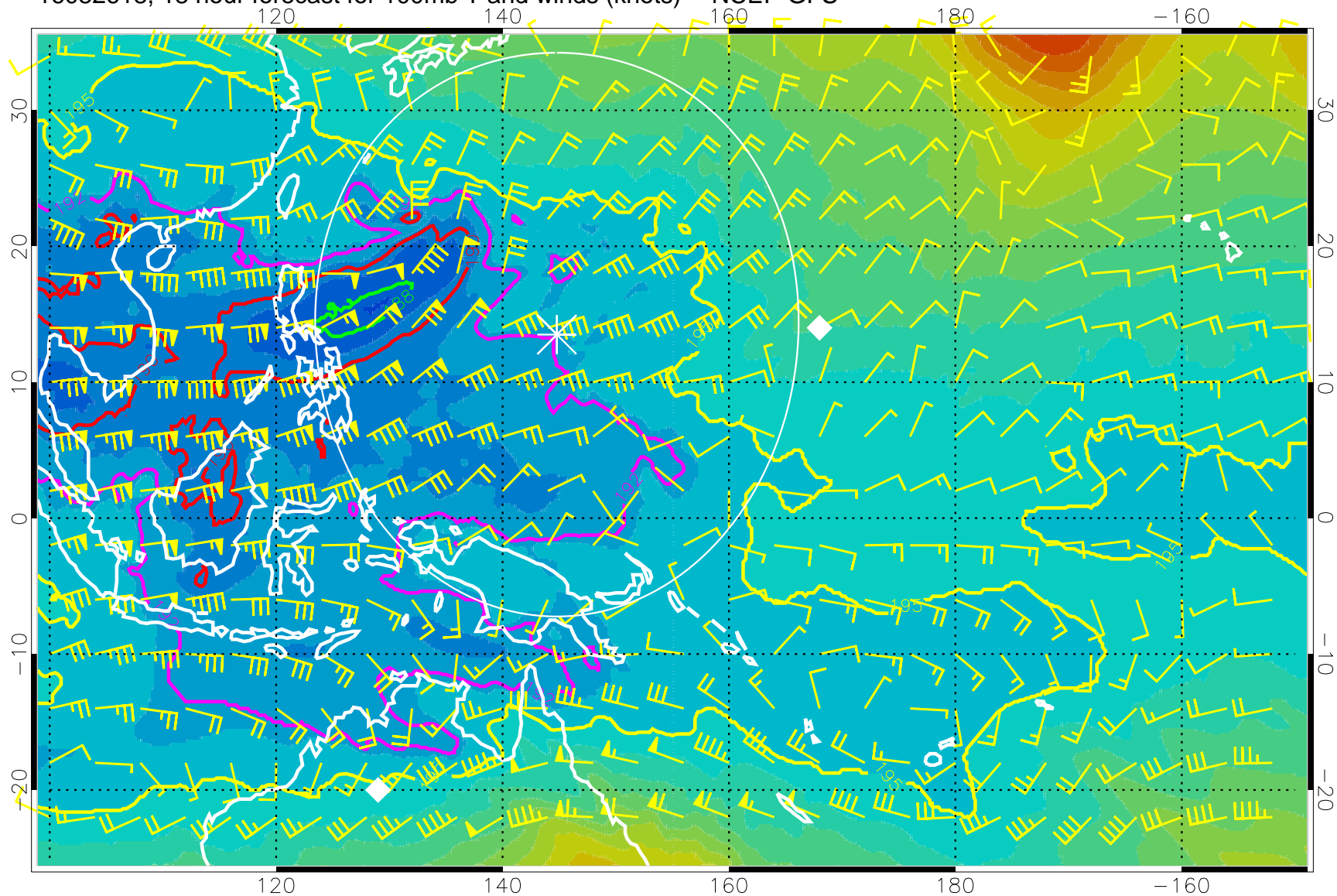
16082618, 18 hour forecast for 100mb T and winds (knots) -- NCEP GFS
