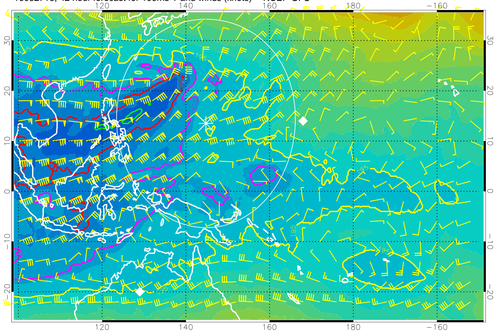
16082718, 42 hour forecast for 100mb T and winds (knots) -- NCEP GFS
