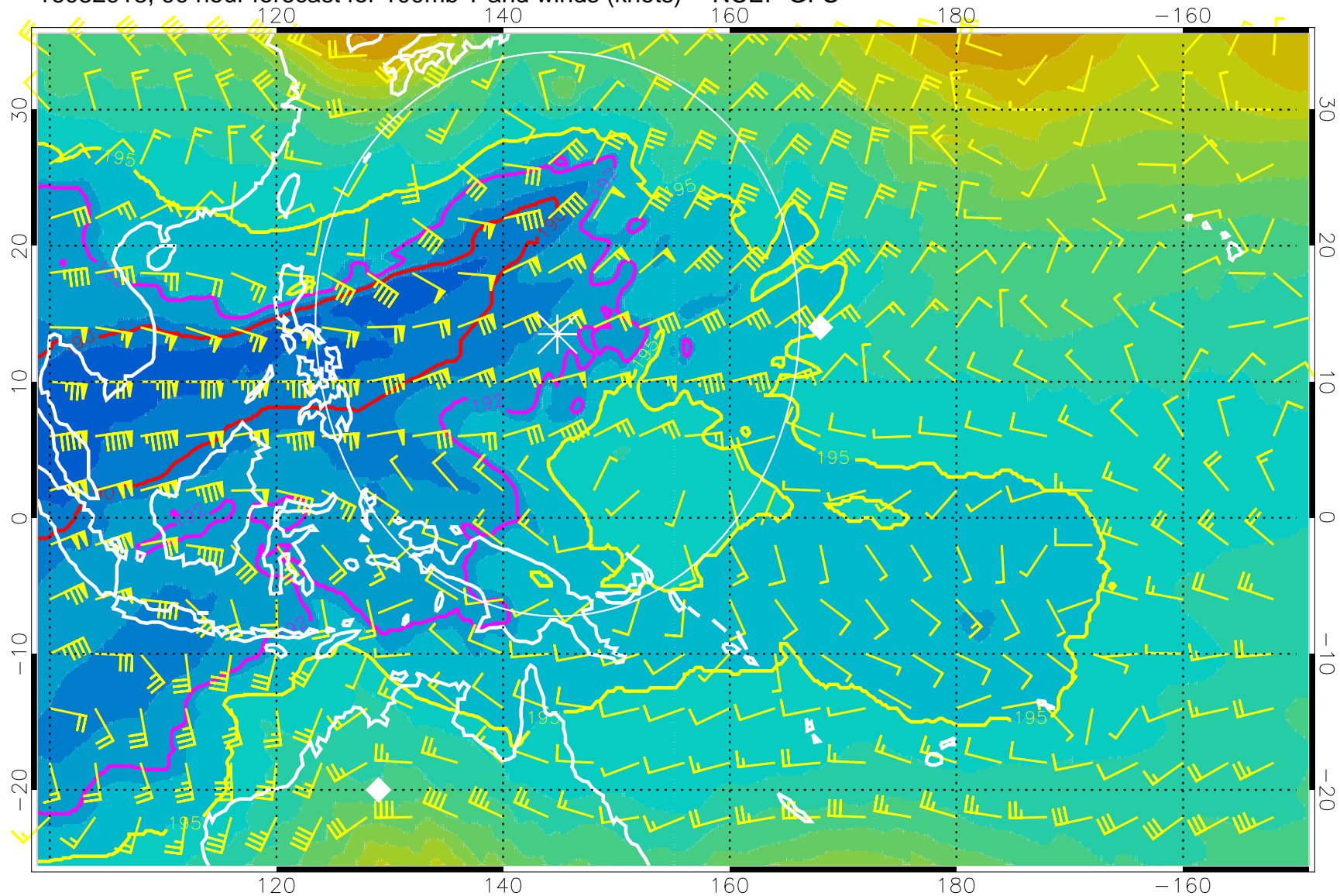
16082918, 90 hour forecast for 100mb T and winds (knots) -- NCEP GFS
