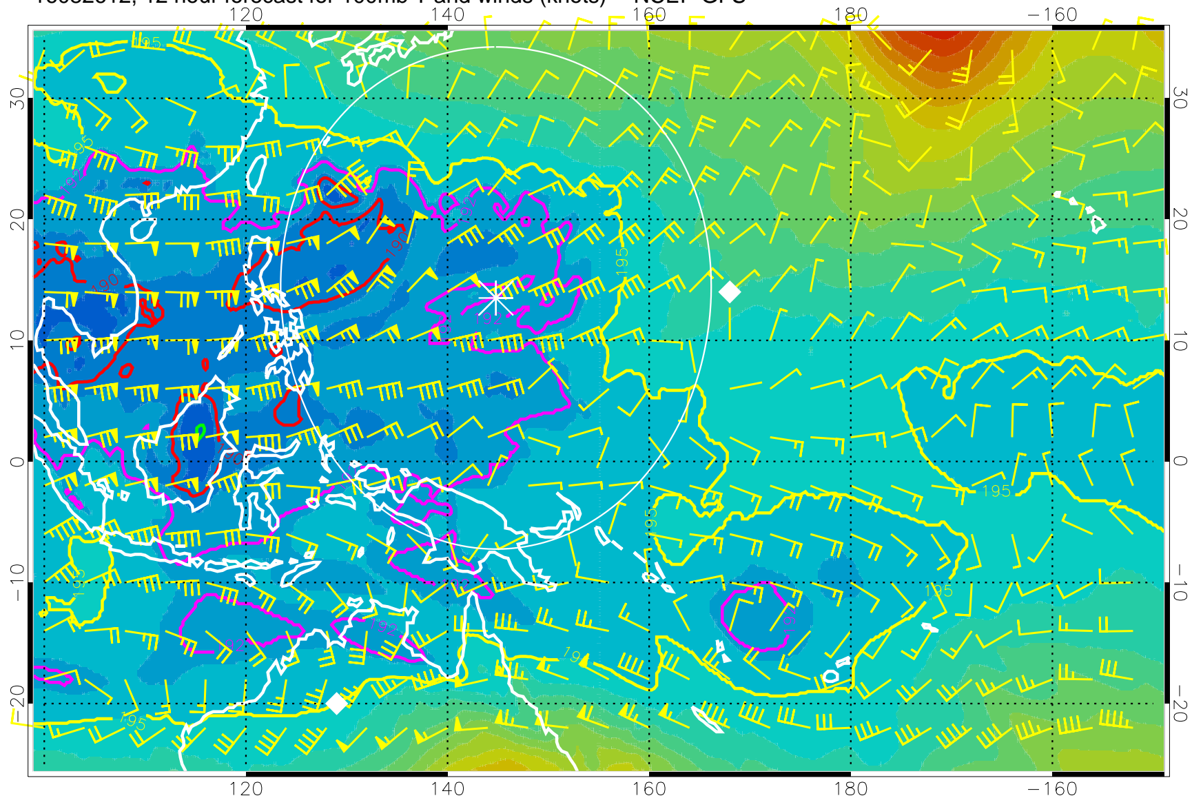
16082612, 12 hour forecast for 100mb T and winds (knots) -- NCEP GFS
