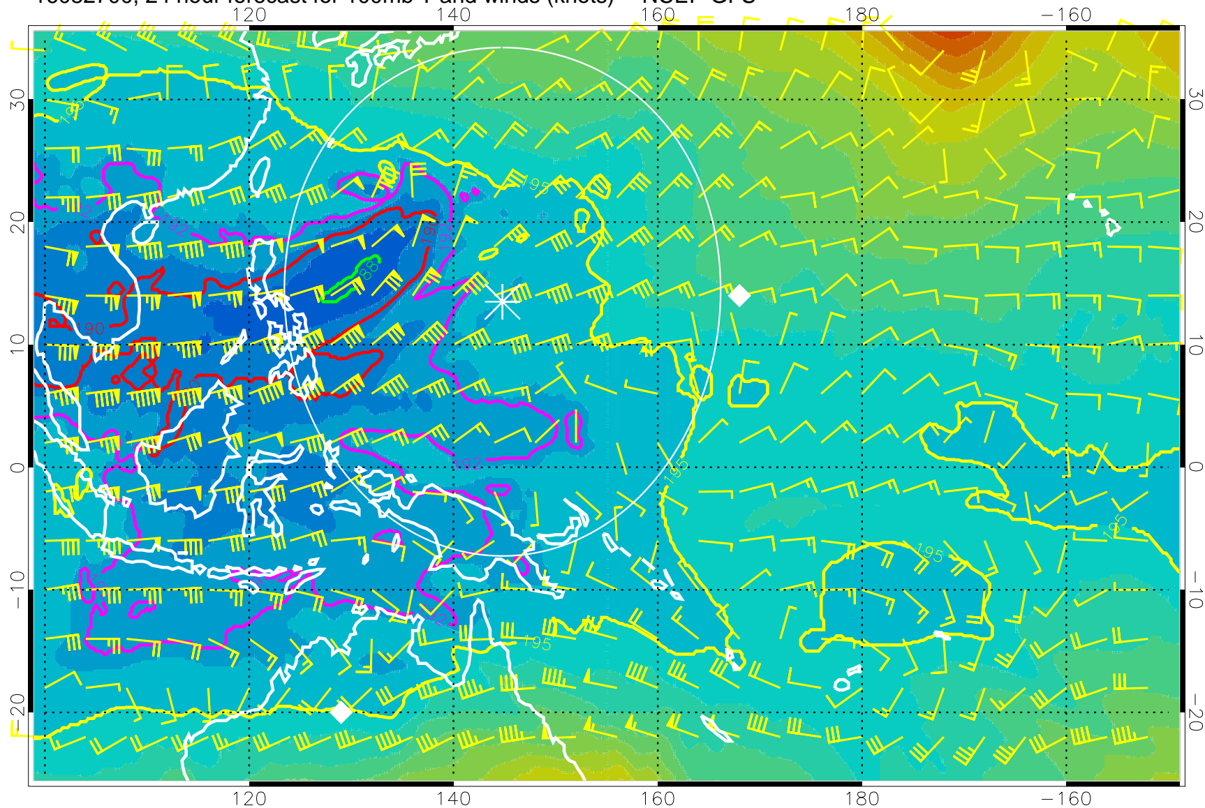
16082700, 24 hour forecast for 100mb T and winds (knots) -- NCEP GFS
