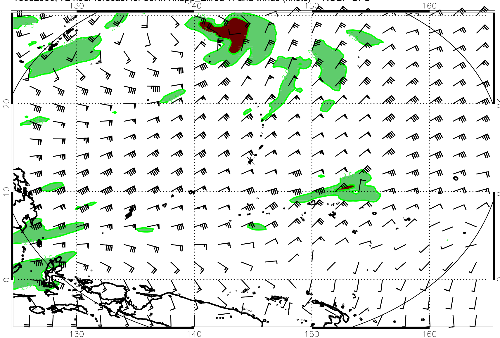
16082900, 72 hour forecast for 53Kft Knapp_Ellrod TI and winds (knots) -- NCEP GFS
