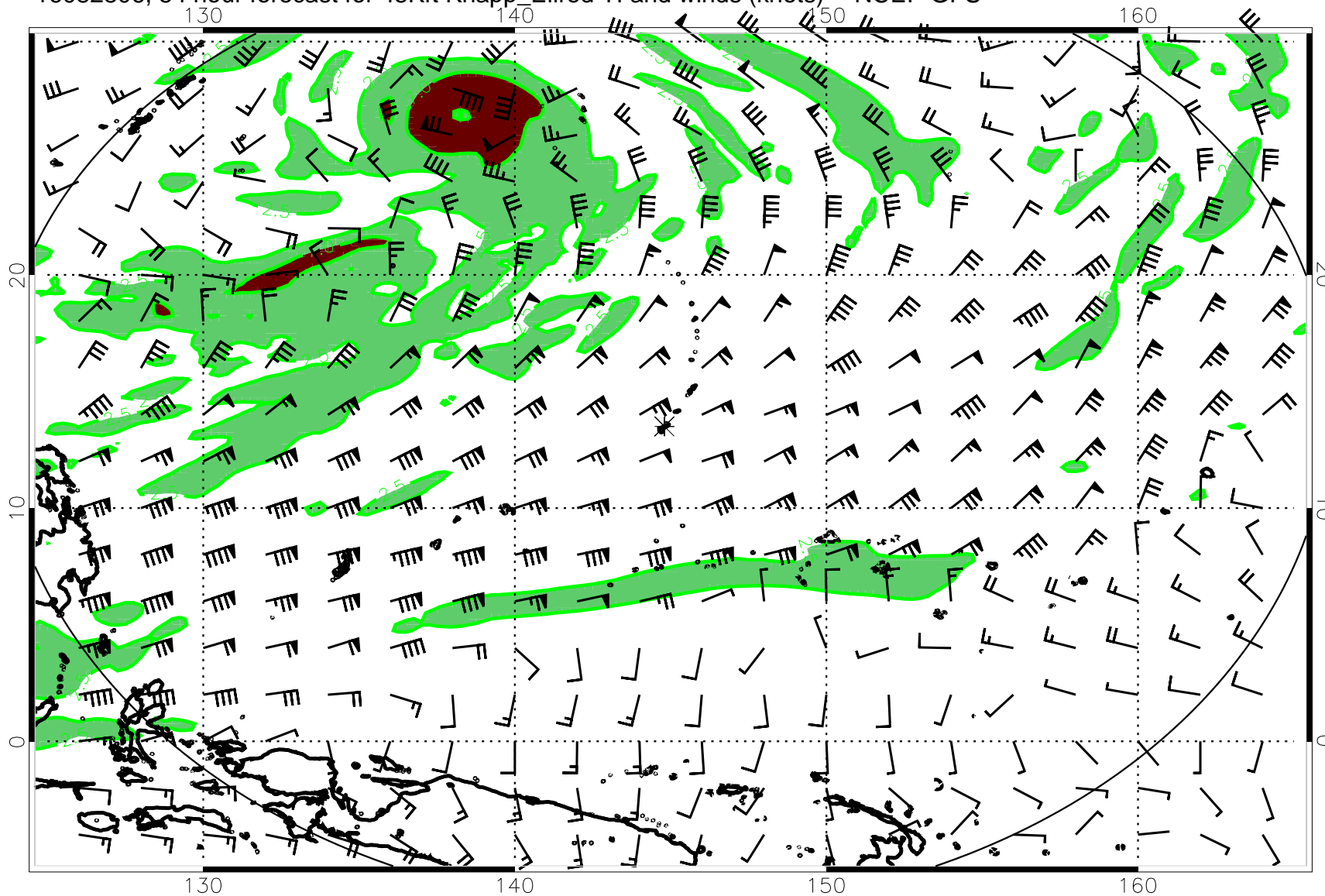
16082806, 54 hour forecast for 45Kft Knapp_Ellrod TI and winds (knots) -- NCEP GFS
