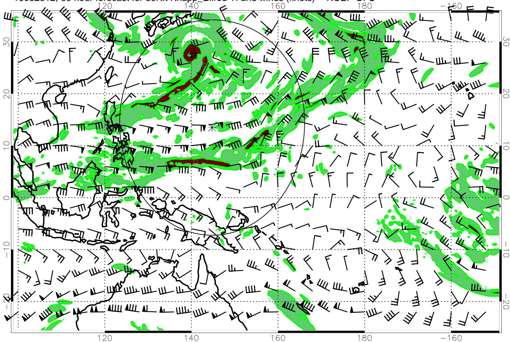
16082812, 60 hour forecast for 39Kft Knapp_Ellrod TI and winds (knots) -- NCEP GFS
