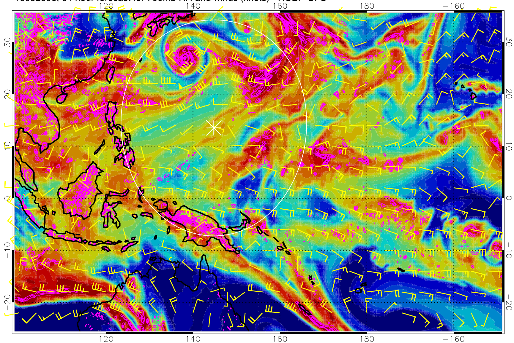
16082806, 54 hour forecast for 700mb RH and winds (knots) - NCEP GFS
