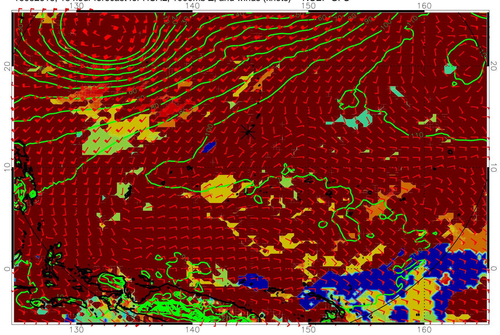
16082618, 18 hour forecast for HCAL, 1000mb Z, and winds (knots) -- NCEP GFS
