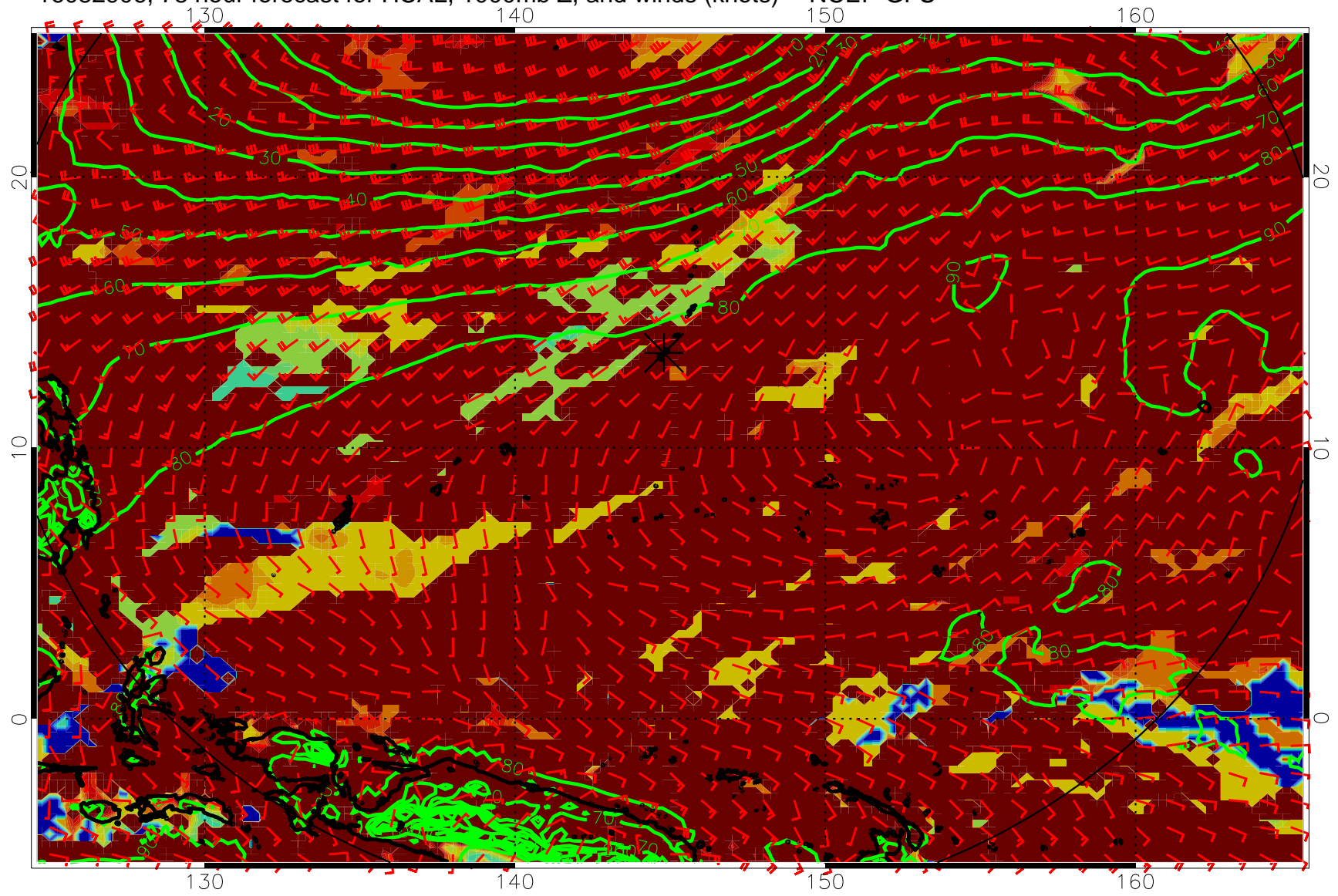
16082906, 78 hour forecast for HCAL, 1000mb Z, and winds (knots) -- NCEP GFS
