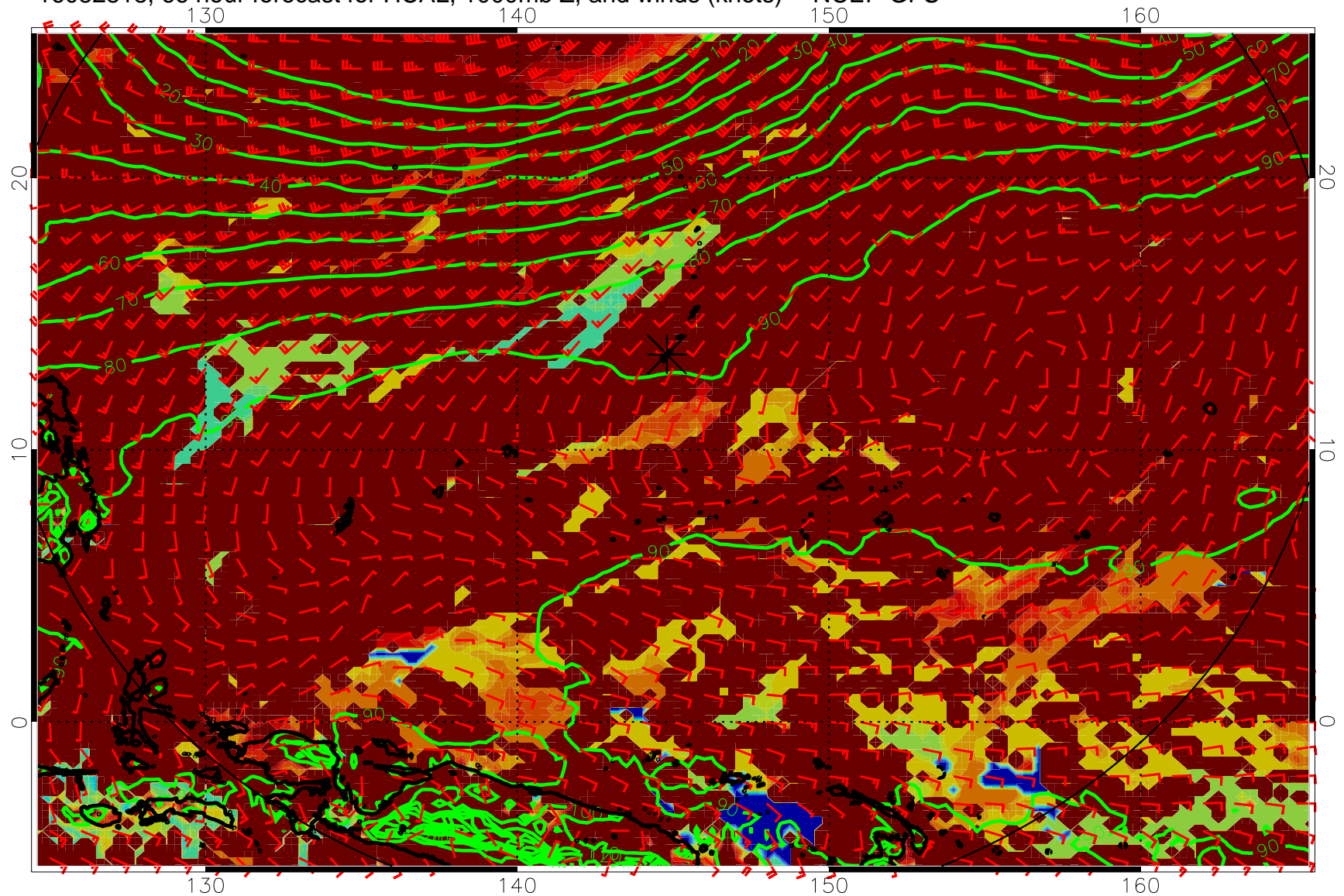
16082818, 66 hour forecast for HCAL, 1000mb Z, and winds (knots) -- NCEP GFS
