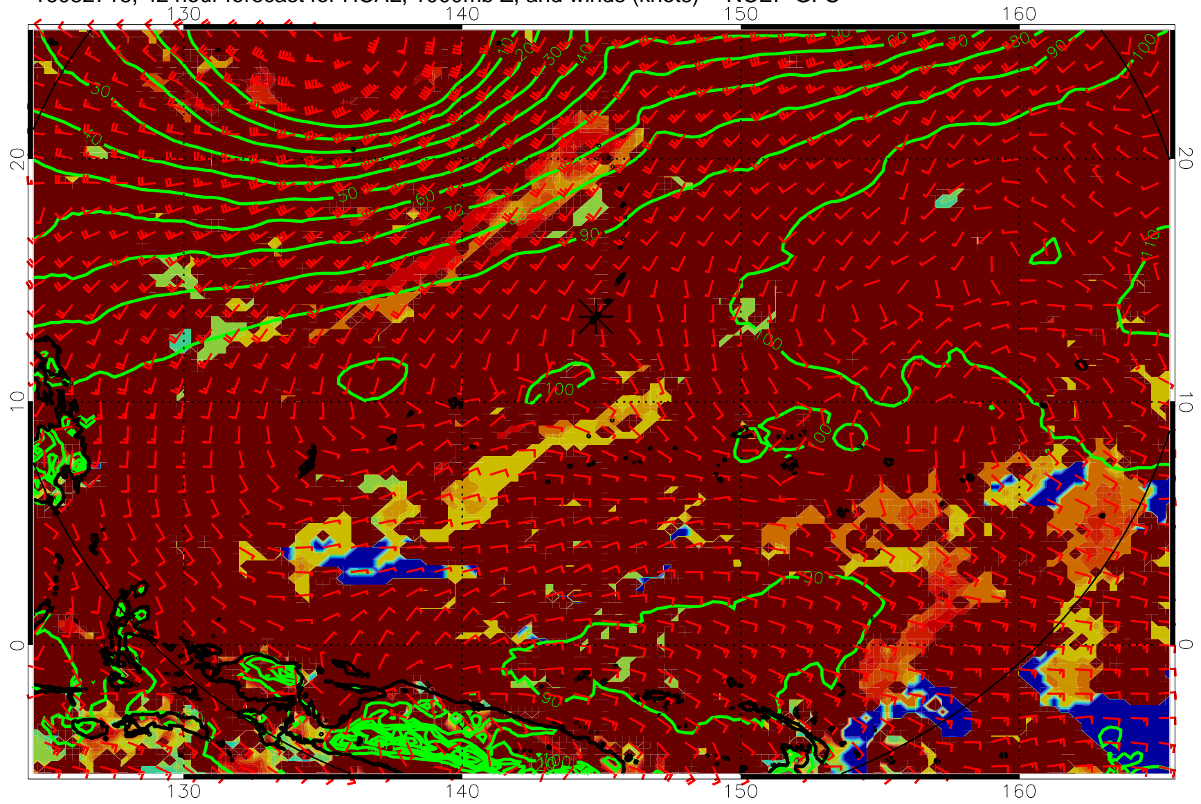
16082718, 42 hour forecast for HCAL, 1000mb Z, and winds (knots) -- NCEP GFS
