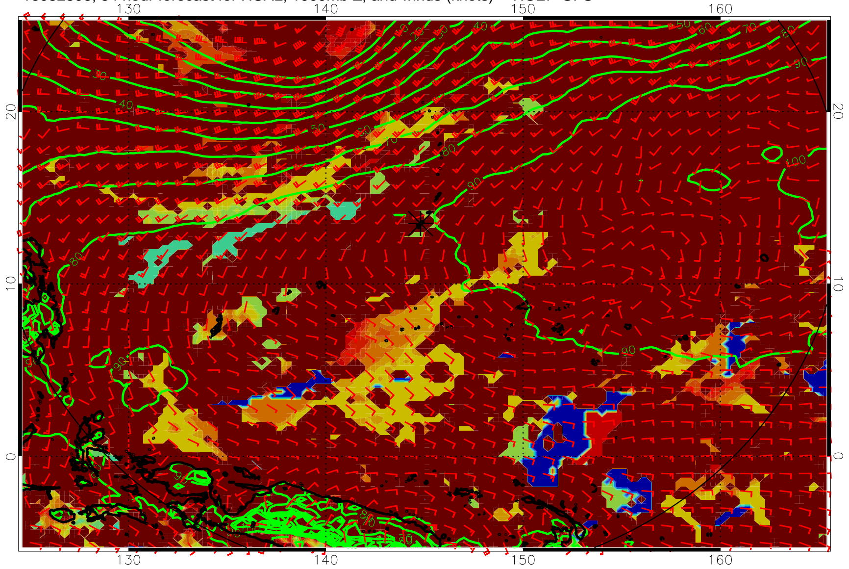
16082806, 54 hour forecast for HCAL, 1000mb Z, and winds (knots) -- NCEP GFS
