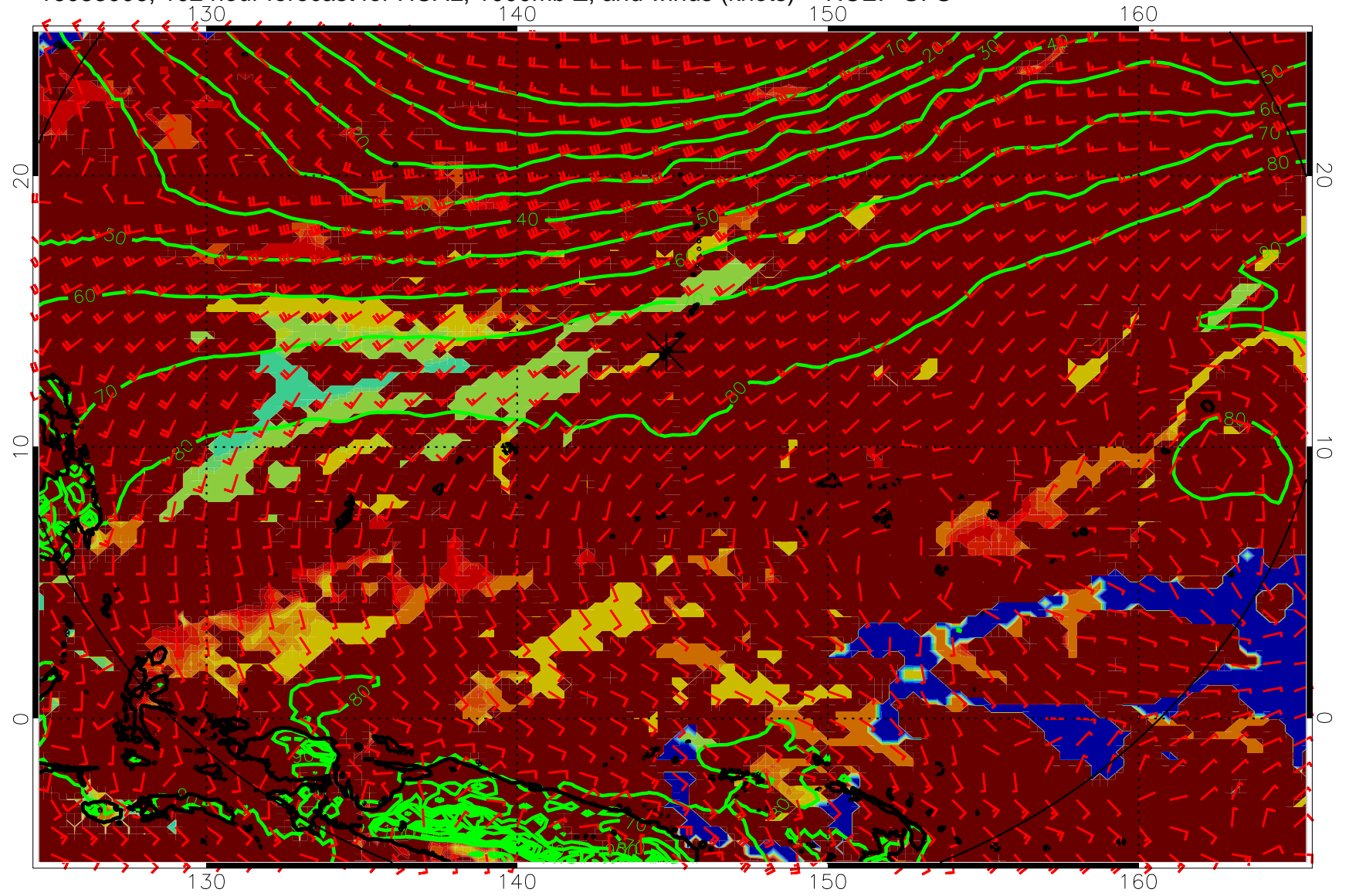
16083006, 102 hour forecast for HCAL, 1000mb Z, and winds (knots) -- NCEP GFS
