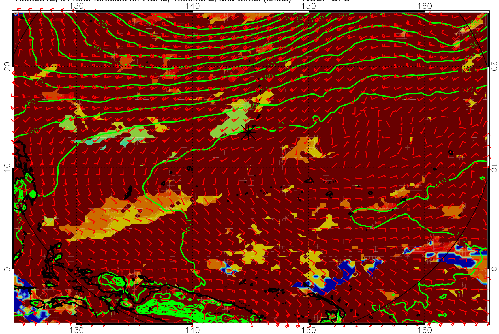
16082912, 84 hour forecast for HCAL, 1000mb Z, and winds (knots) -- NCEP GFS
