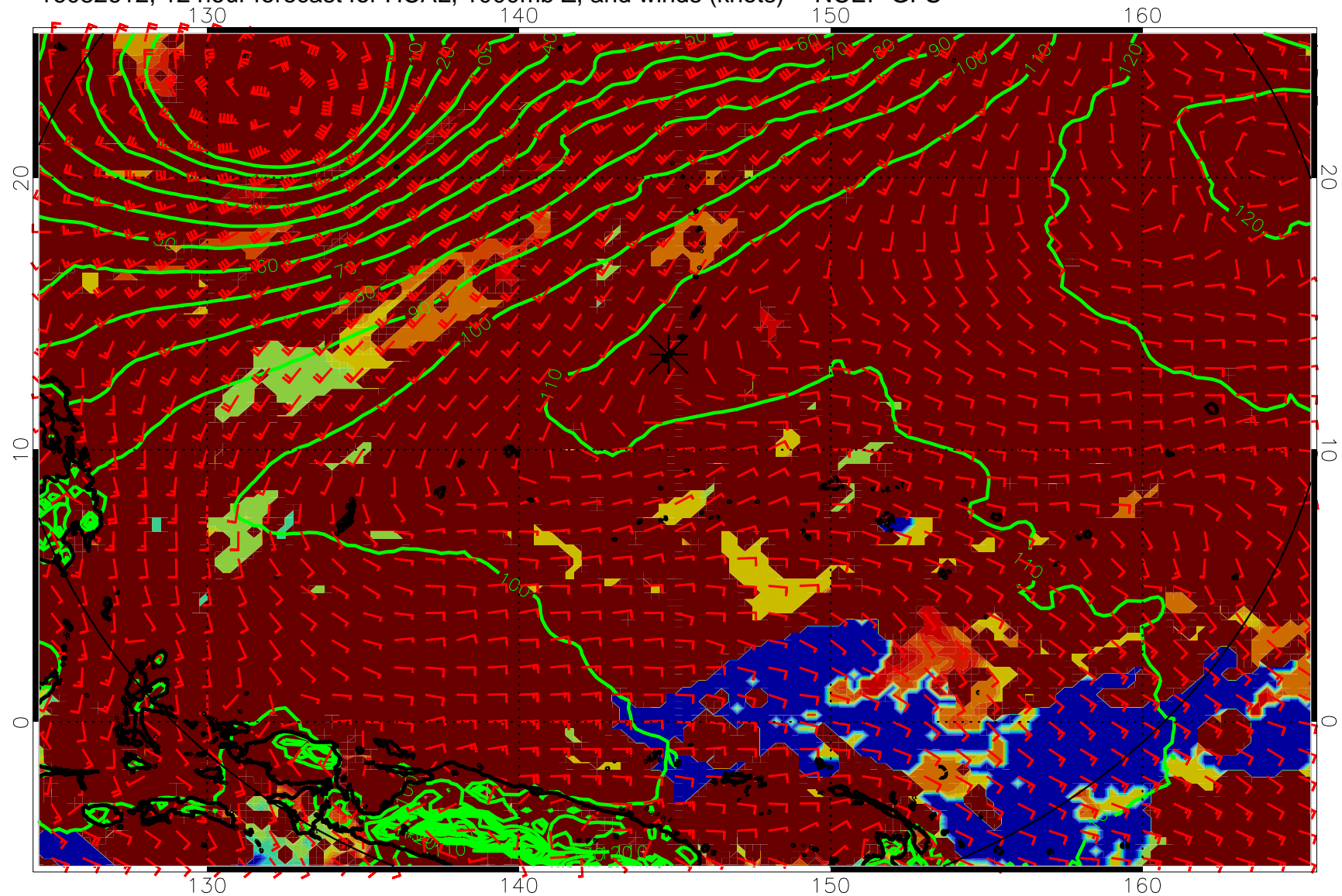
16082612, 12 hour forecast for HCAL, 1000mb Z, and winds (knots) -- NCEP GFS
