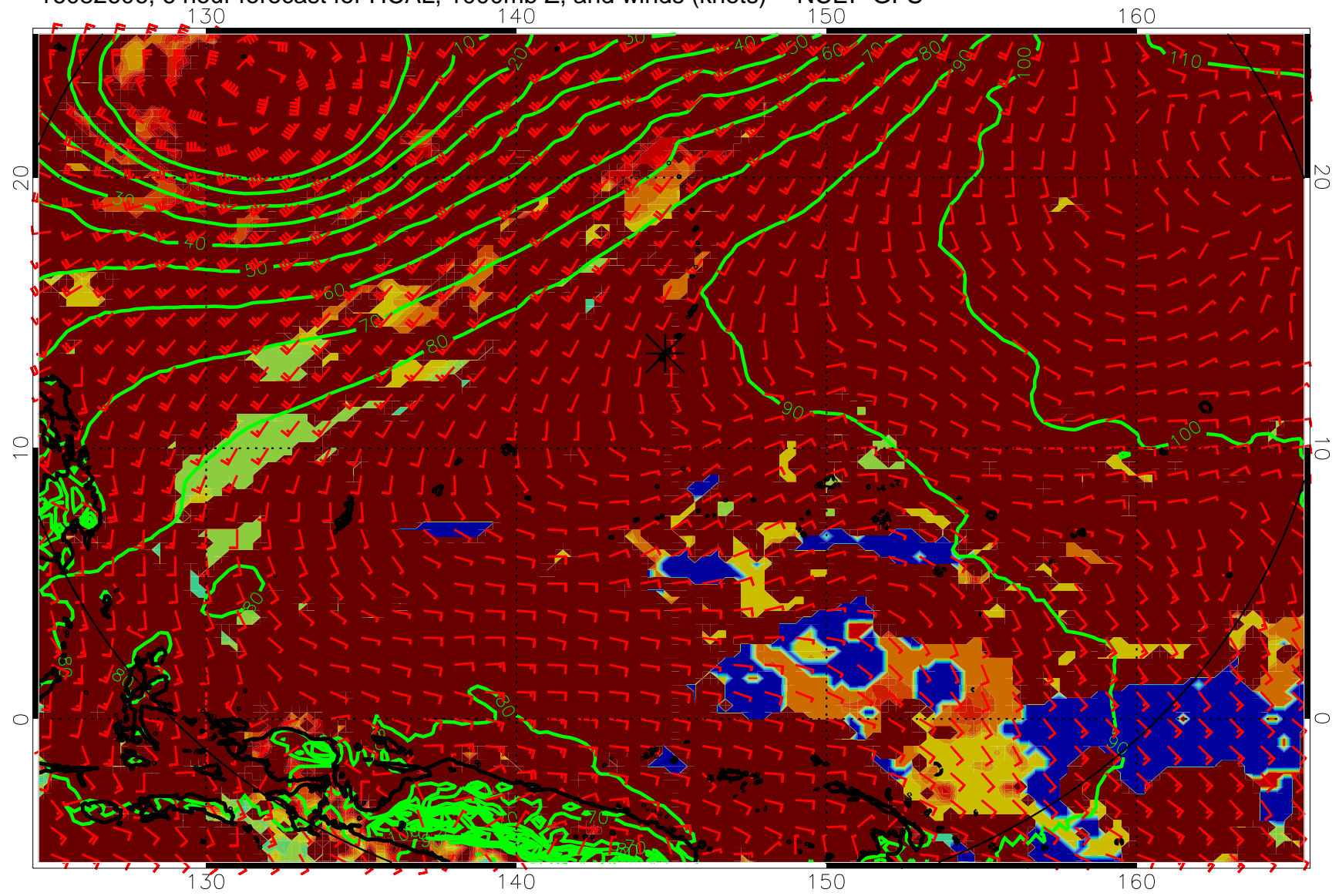
16082606, 6 hour forecast for HCAL, 1000mb Z, and winds (knots) -- NCEP GFS
