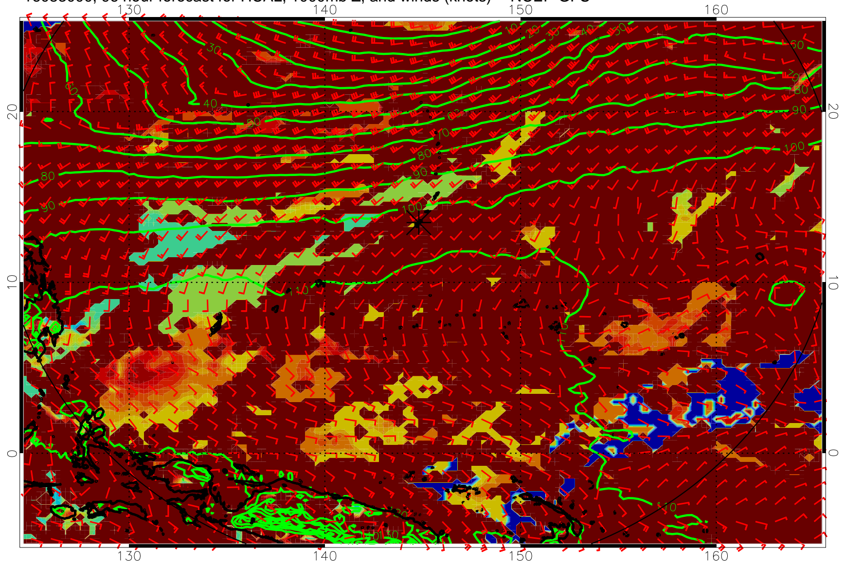
16083000, 96 hour forecast for HCAL, 1000mb Z, and winds (knots) -- NCEP GFS
