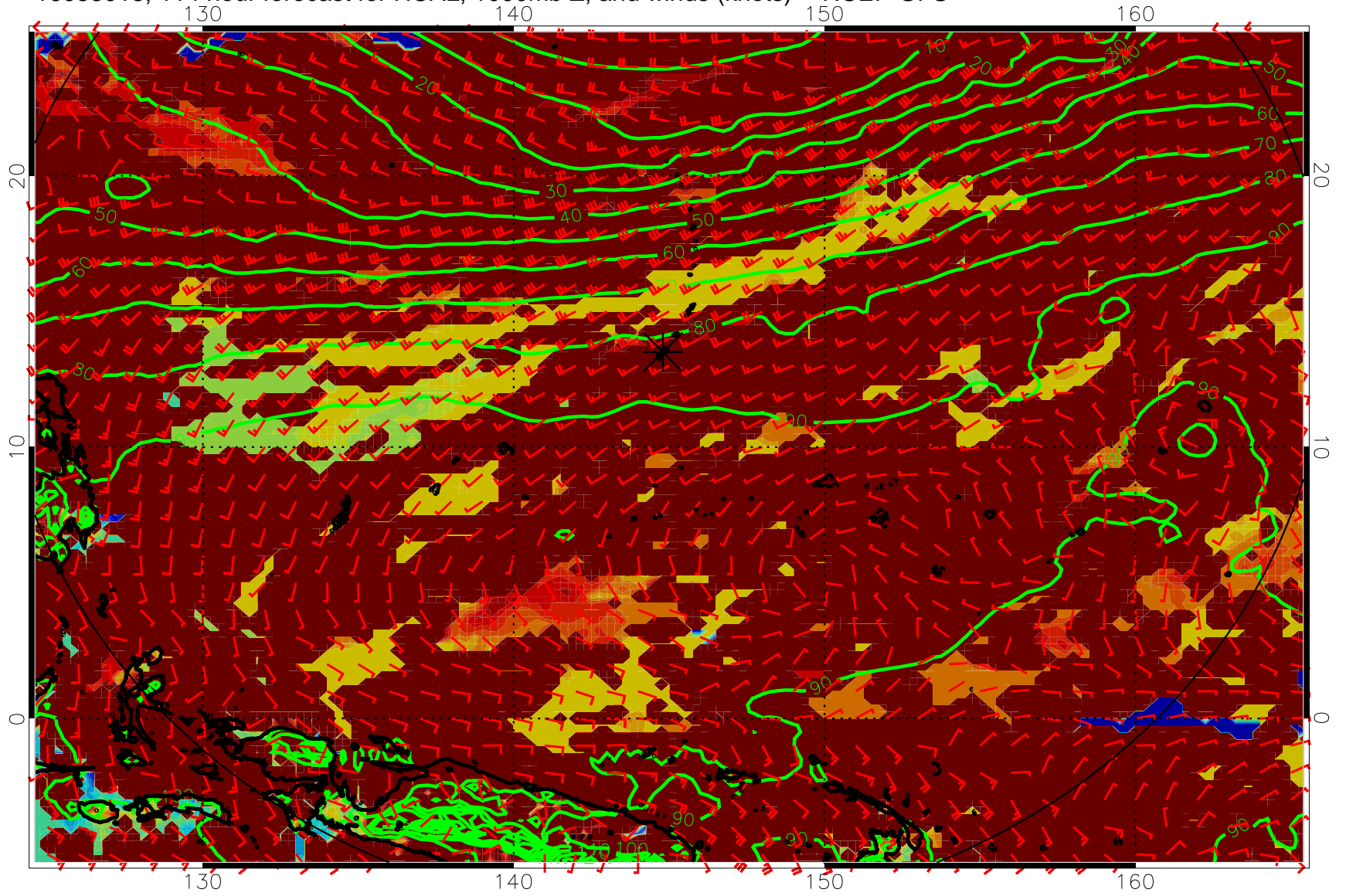
16083018, 114 hour forecast for HCAL, 1000mb Z, and winds (knots) -- NCEP GFS
