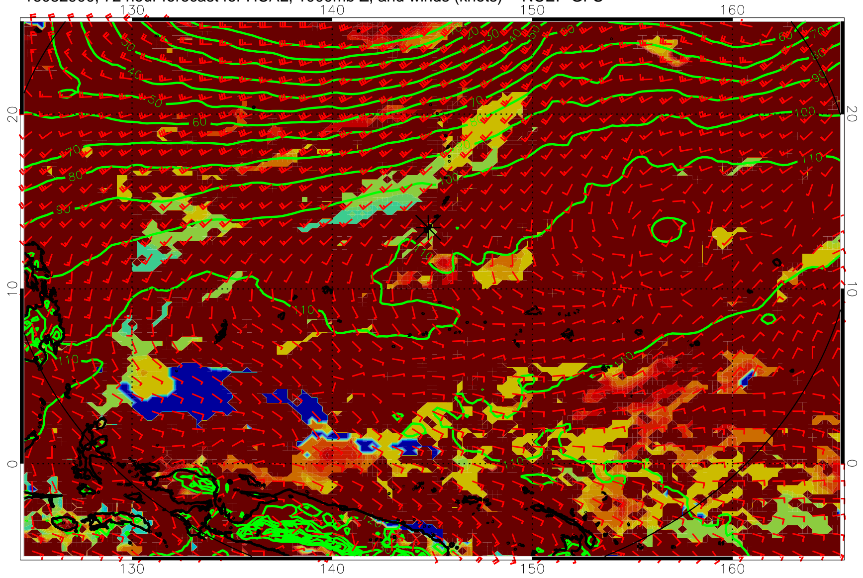
16082900, 72 hour forecast for HCAL, 1000mb Z, and winds (knots) -- NCEP GFS
