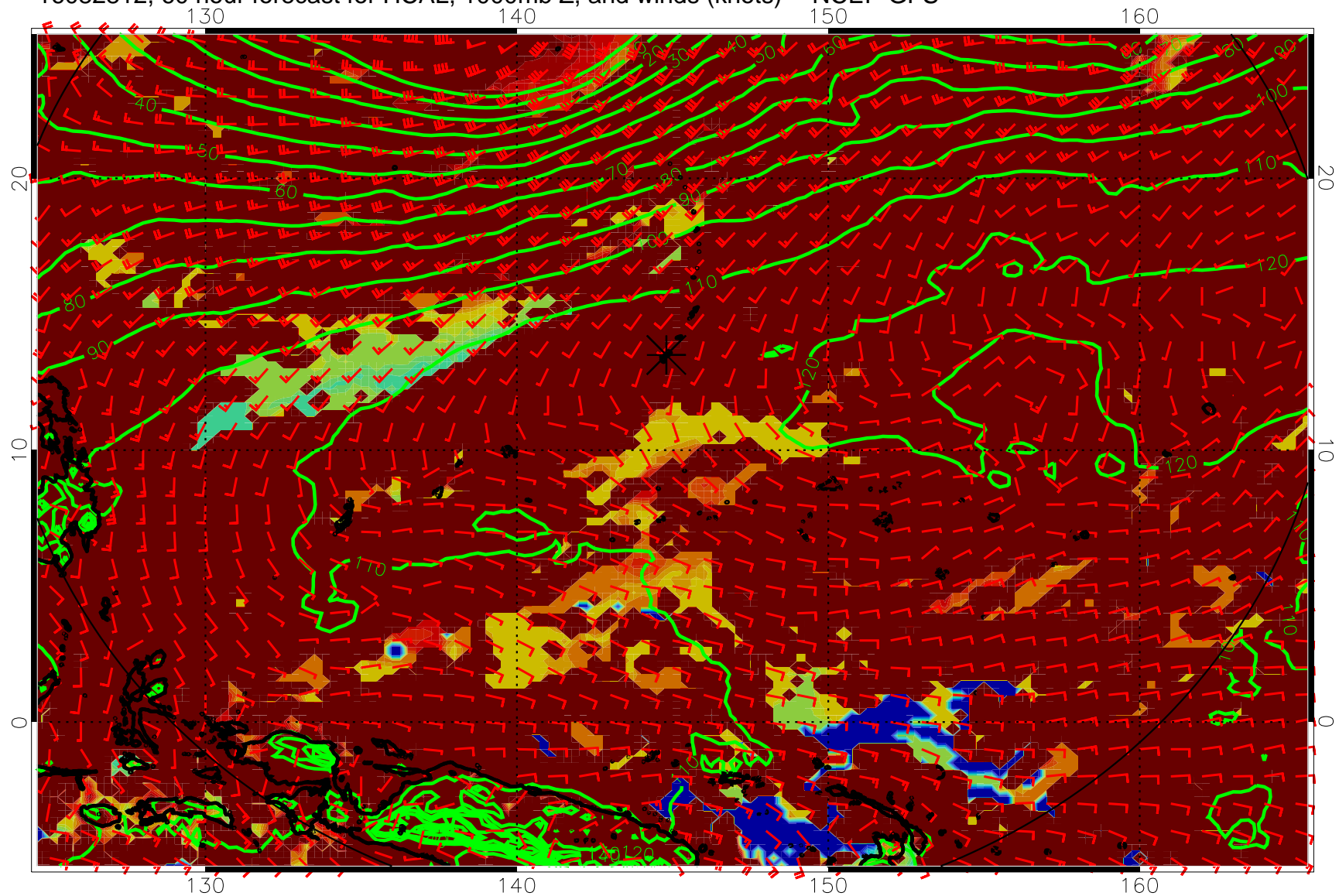
16082812, 60 hour forecast for HCAL, 1000mb Z, and winds (knots) -- NCEP GFS
