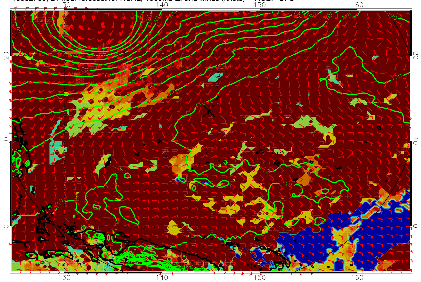
16082700, 24 hour forecast for HCAL, 1000mb Z, and winds (knots) -- NCEP GFS
