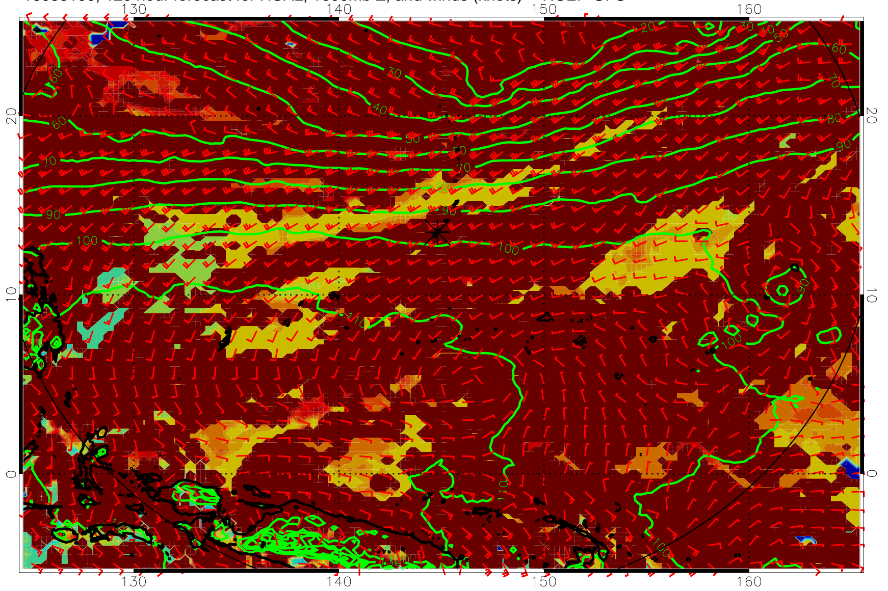
16083100, 120 hour forecast for HCAL, 1000mb Z, and winds (knots) -- NCEP GFS
