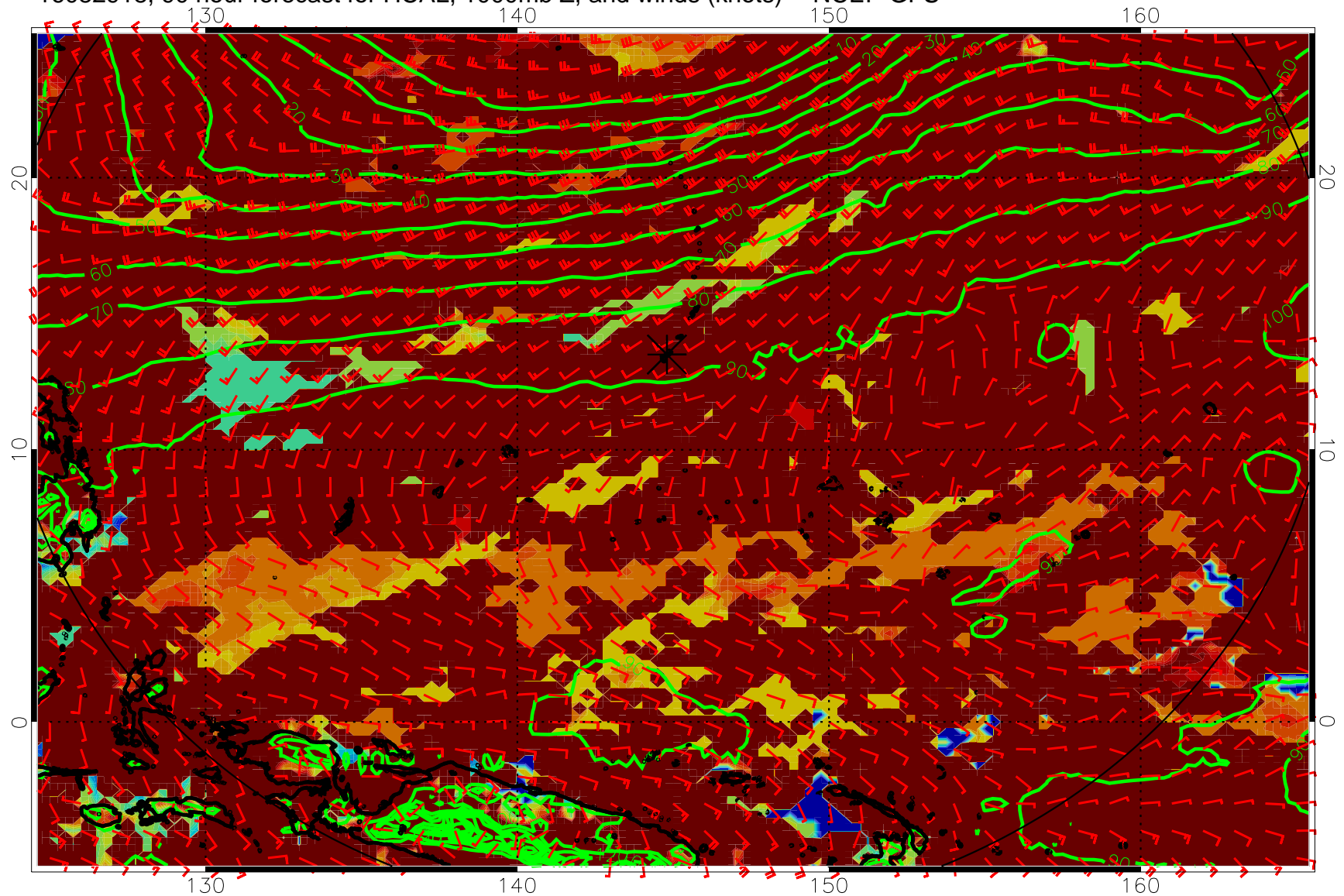
16082918, 90 hour forecast for HCAL, 1000mb Z, and winds (knots) -- NCEP GFS
