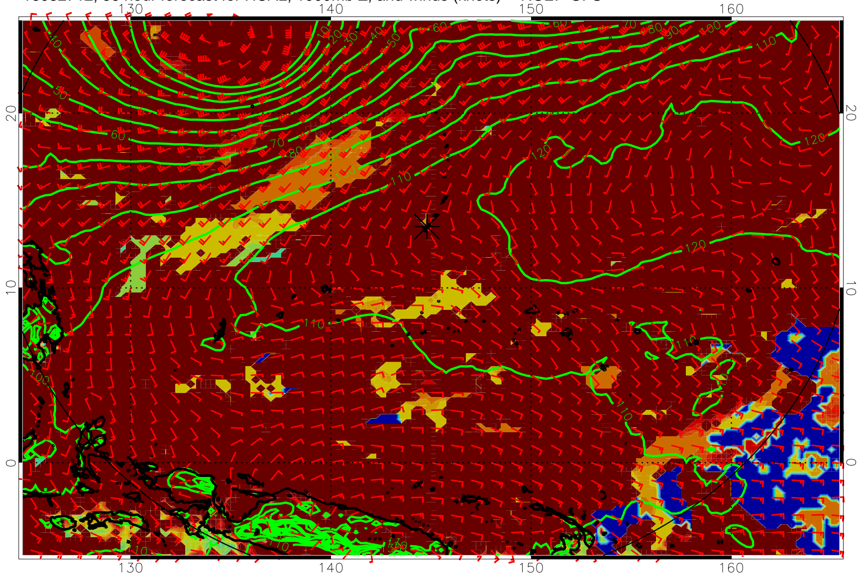
16082712, 36 hour forecast for HCAL, 1000mb Z, and winds (knots) -- NCEP GFS
