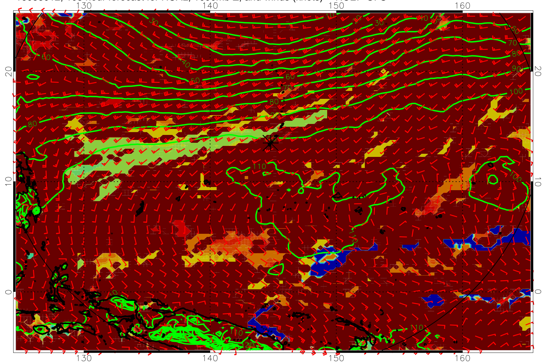
16083012, 108 hour forecast for HCAL, 1000mb Z, and winds (knots) -- NCEP GFS
