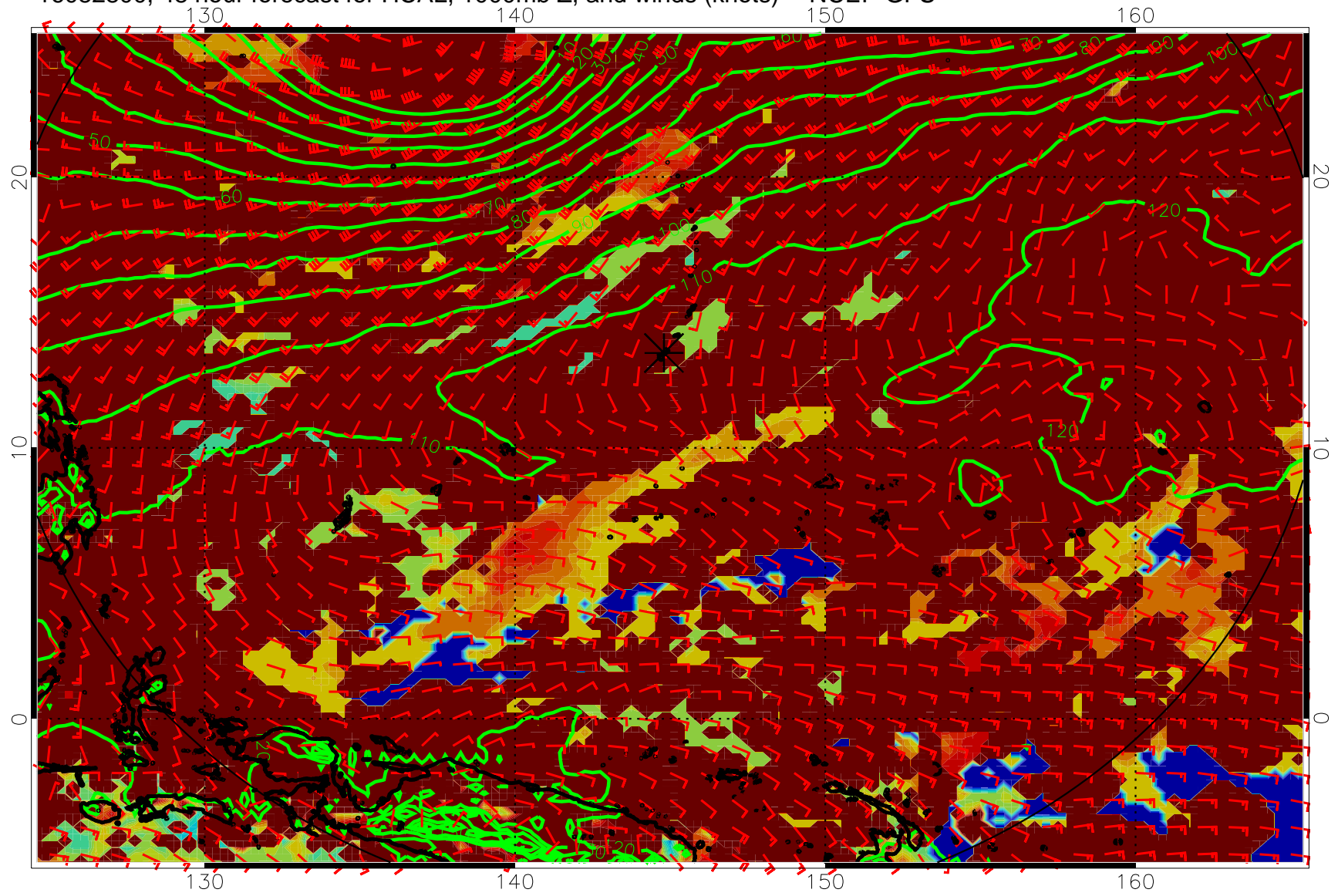
16082800, 48 hour forecast for HCAL, 1000mb Z, and winds (knots) -- NCEP GFS
