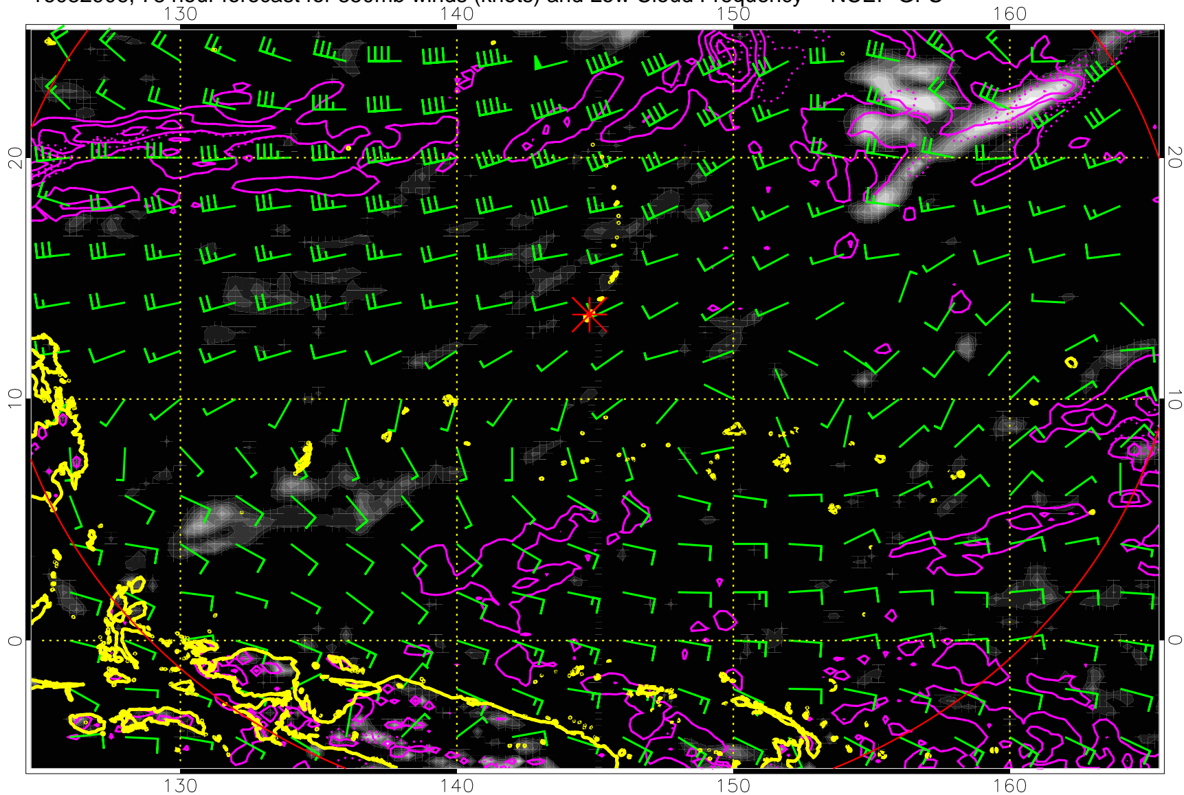
16082906, 78 hour forecast for 850mb winds (knots) and Low Cloud Frequency -- NCEP GFS
