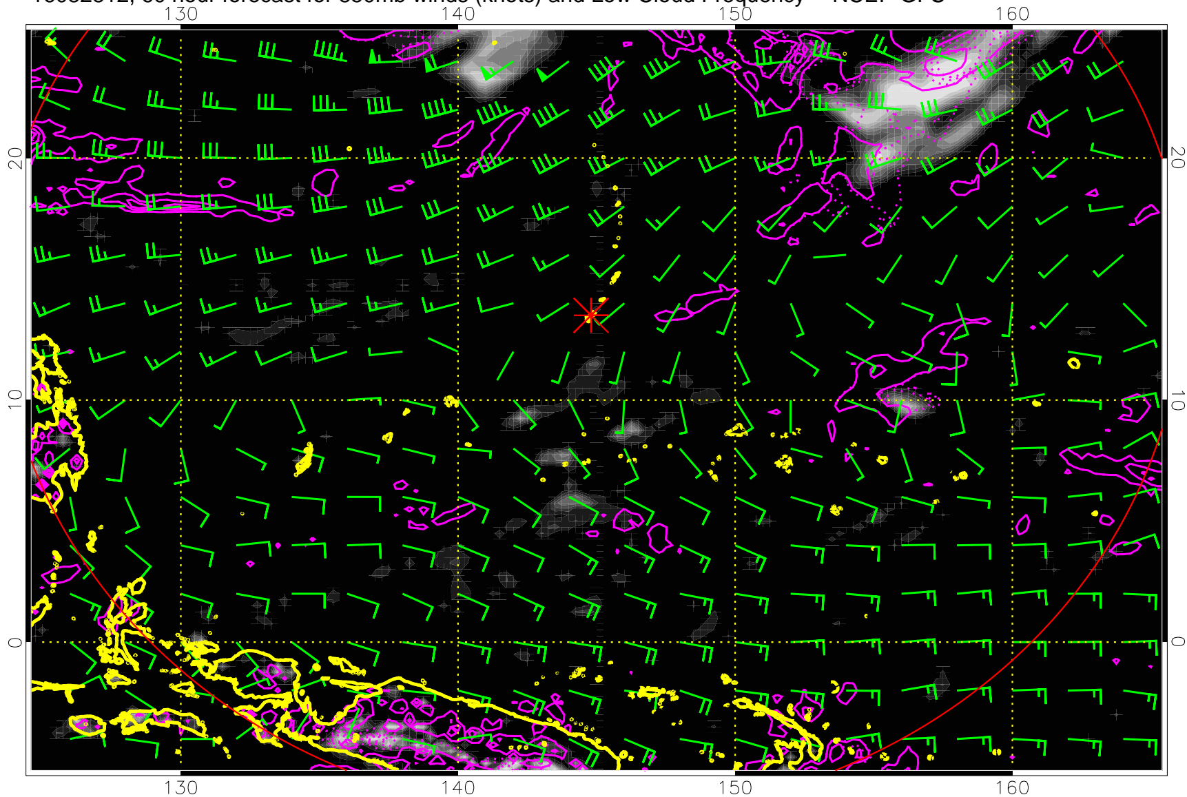
16082812, 60 hour forecast for 850mb winds (knots) and Low Cloud Frequency -- NCEP GFS
