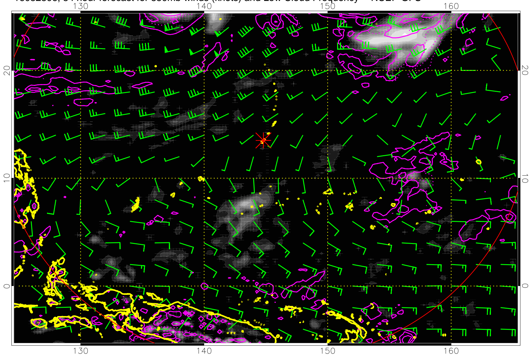
16082806, 54 hour forecast for 850mb winds (knots) and Low Cloud Frequency -- NCEP GFS
