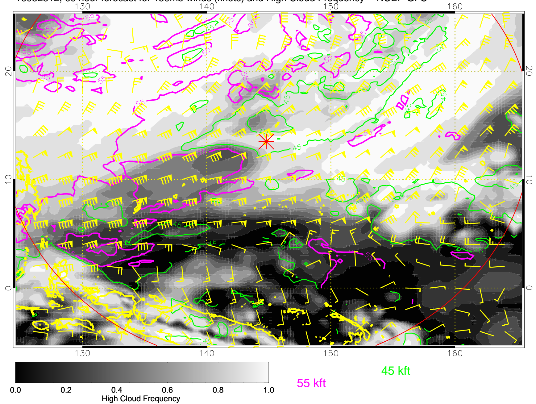
16082812, 60 hour forecast for 150mb winds (knots) and High Cloud Frequency -- NCEP GFS
