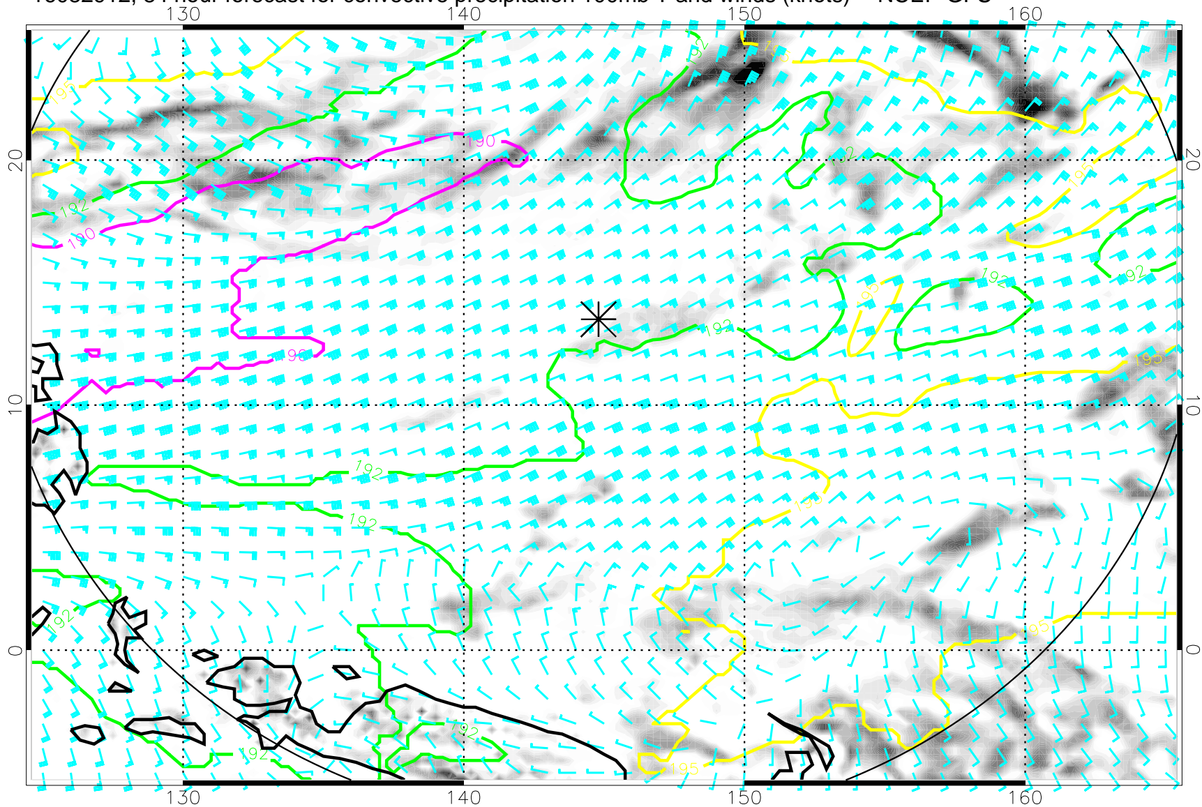
16082912, 84 hour forecast for convective precipitation 100mb T and winds (knots) -- NCEP GFS
