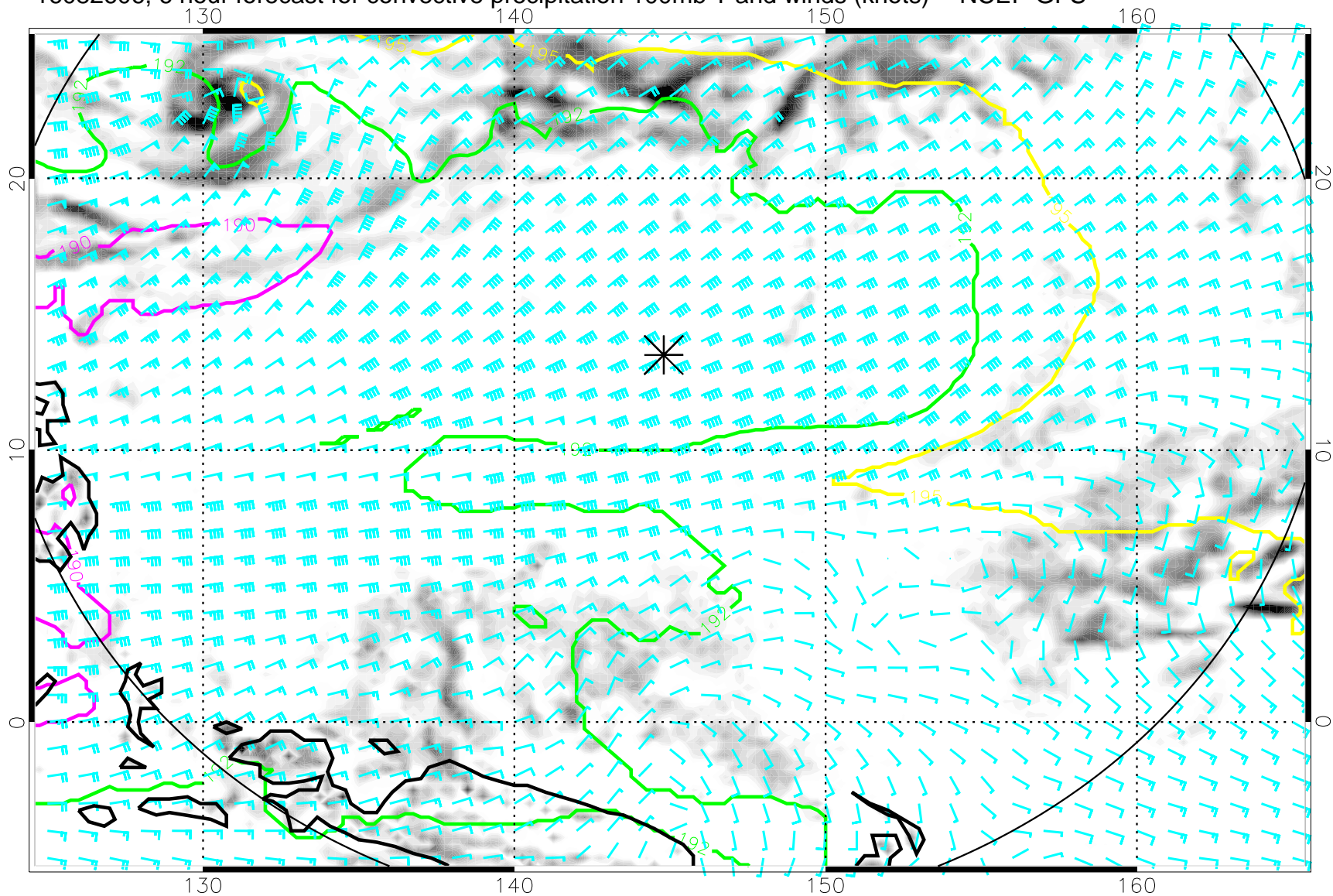
16082606, 6 hour forecast for convective precipitation 100mb T and winds (knots) -- NCEP GFS
