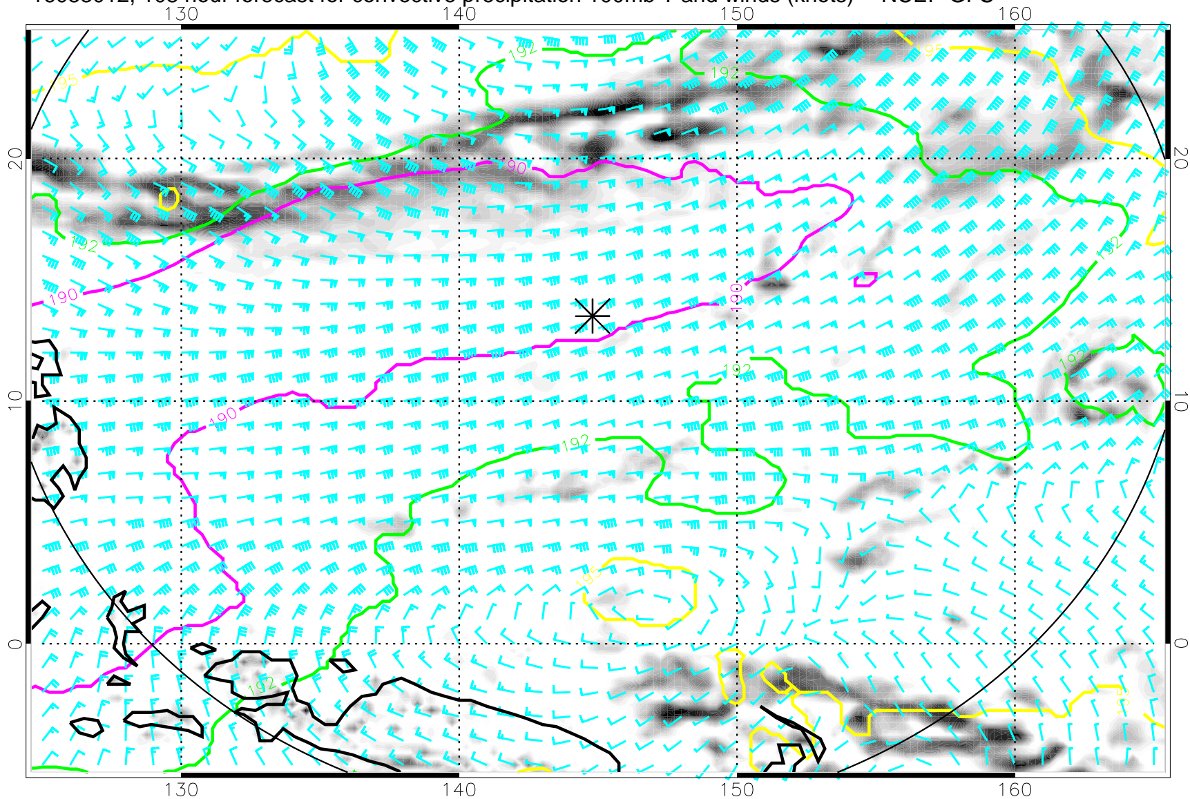
16083012, 108 hour forecast for convective precipitation 100mb T and winds (knots) -- NCEP GFS
