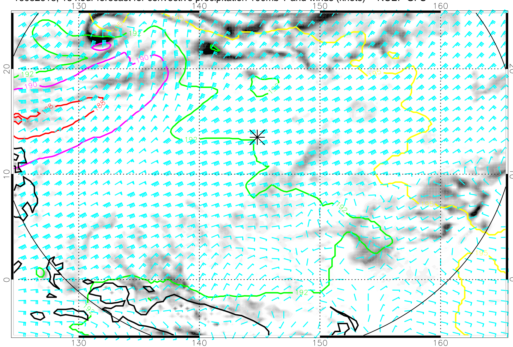
16082618, 18 hour forecast for convective precipitation 100mb T and winds (knots) -- NCEP GFS
