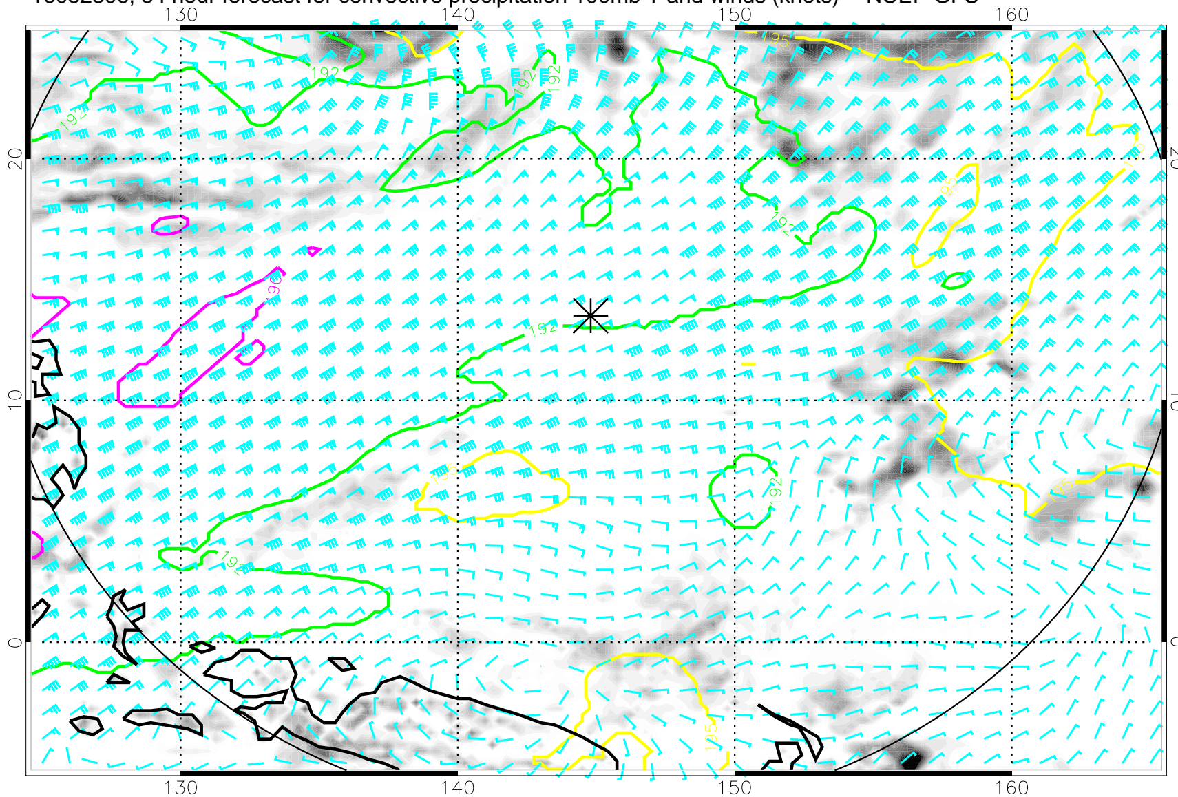
16082806, 54 hour forecast for convective precipitation 100mb T and winds (knots) -- NCEP GFS
