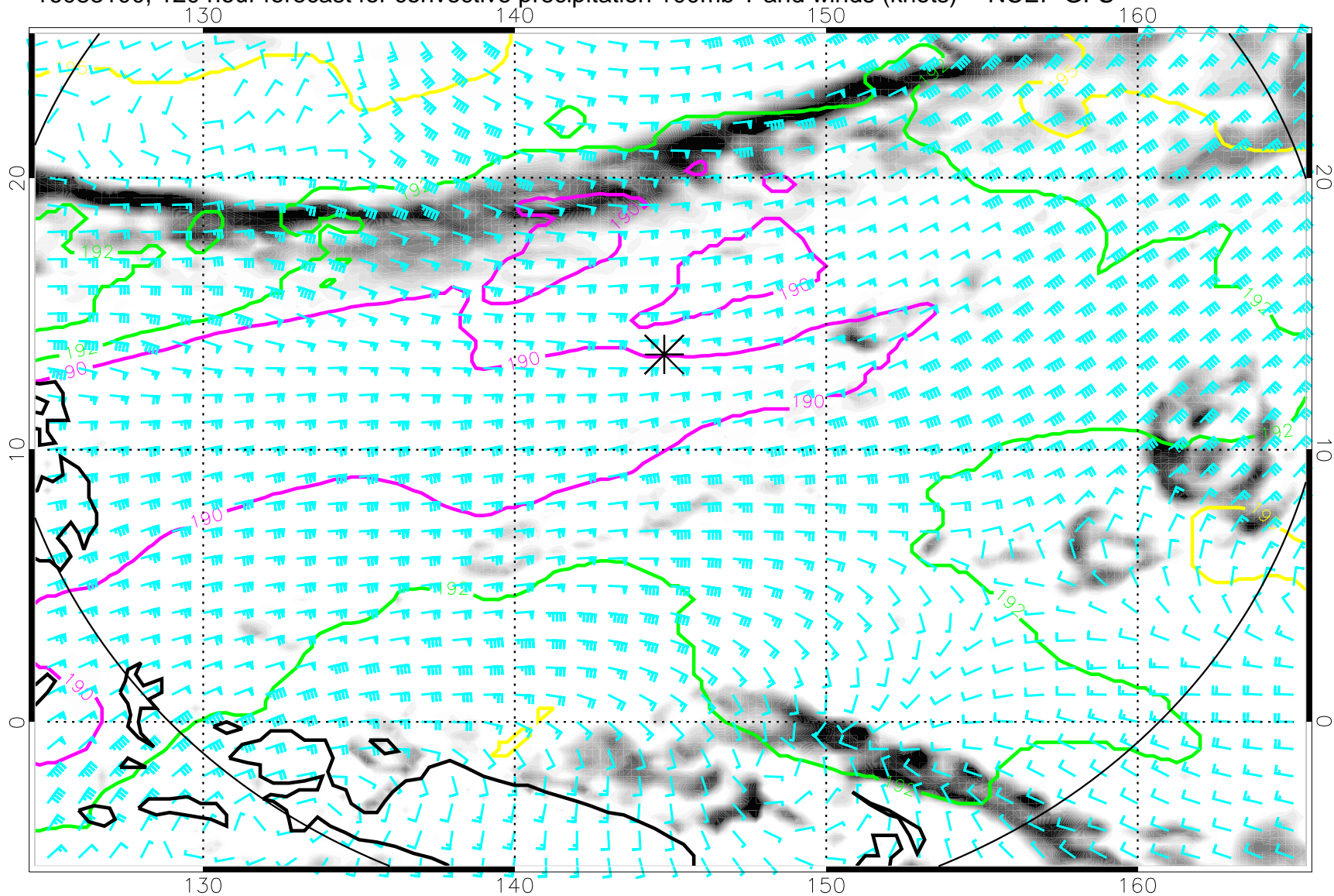
16083100, 120 hour forecast for convective precipitation 100mb T and winds (knots) -- NCEP GFS
