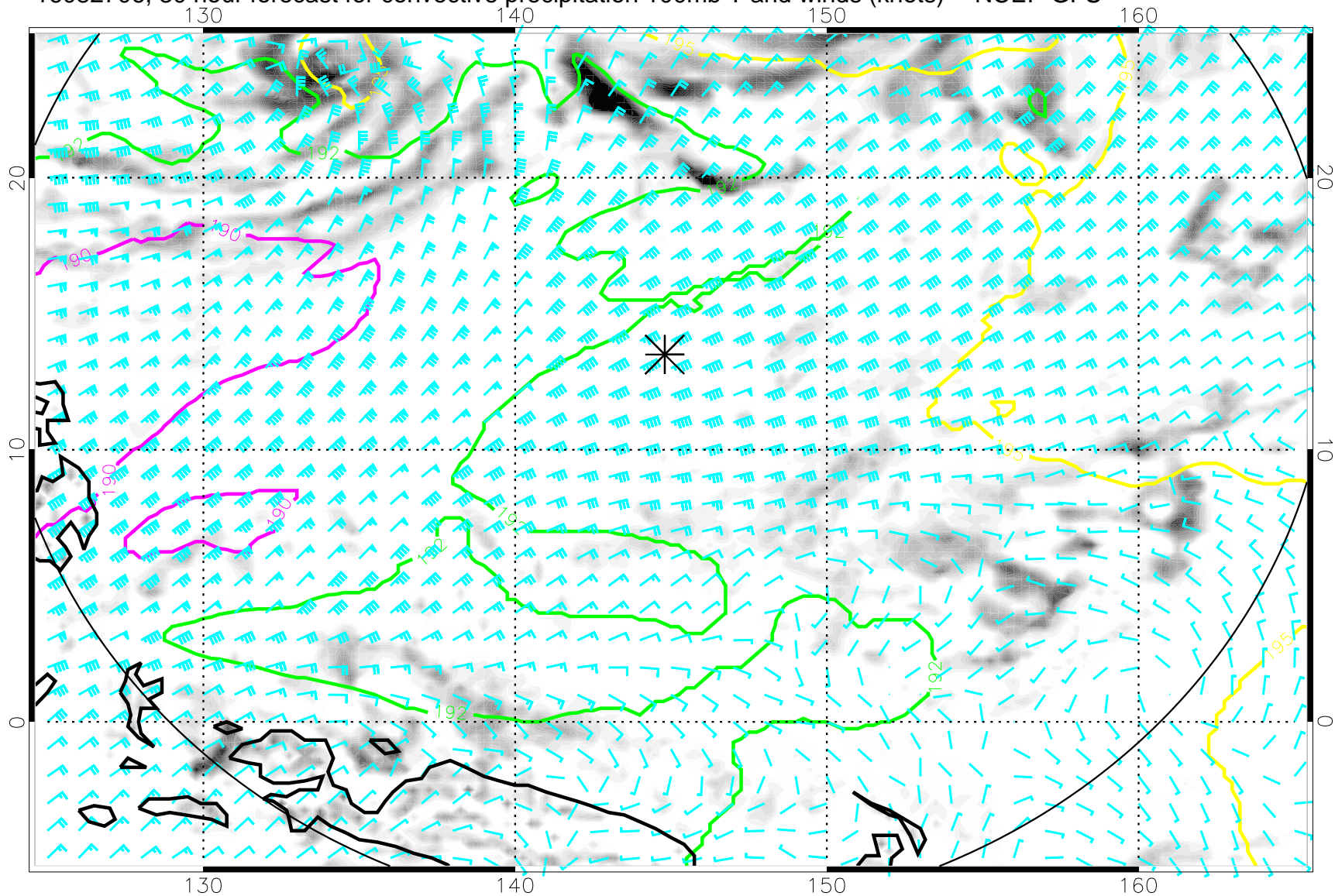
16082706, 30 hour forecast for convective precipitation 100mb T and winds (knots) -- NCEP GFS
