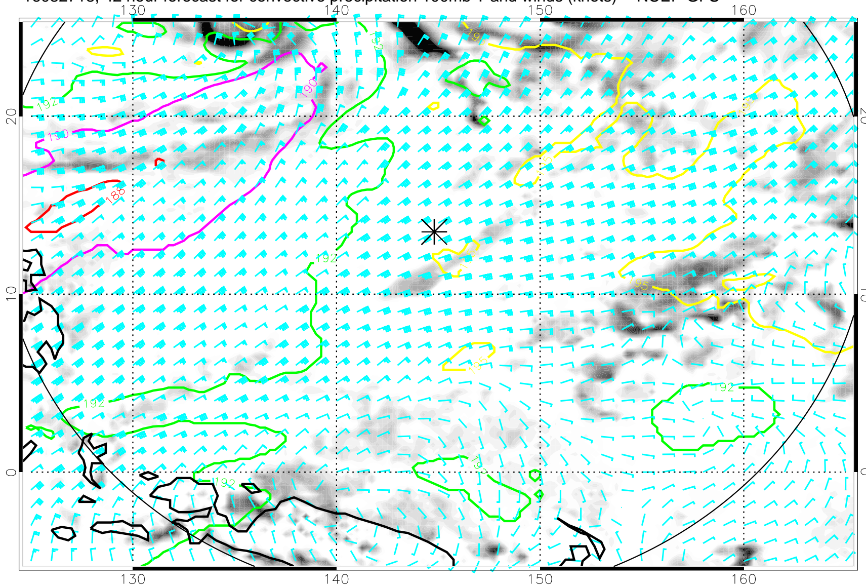
16082718, 42 hour forecast for convective precipitation 100mb T and winds (knots) -- NCEP GFS
