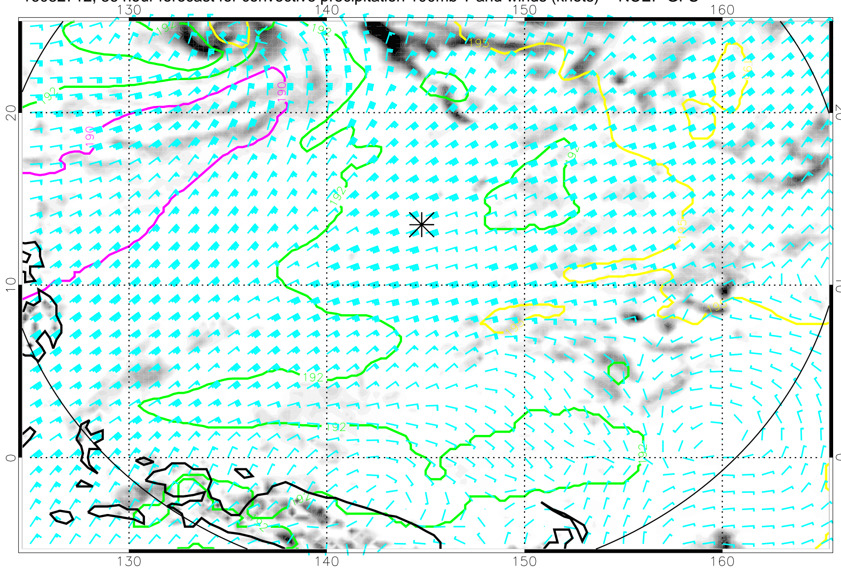
16082712, 36 hour forecast for convective precipitation 100mb T and winds (knots) -- NCEP GFS
