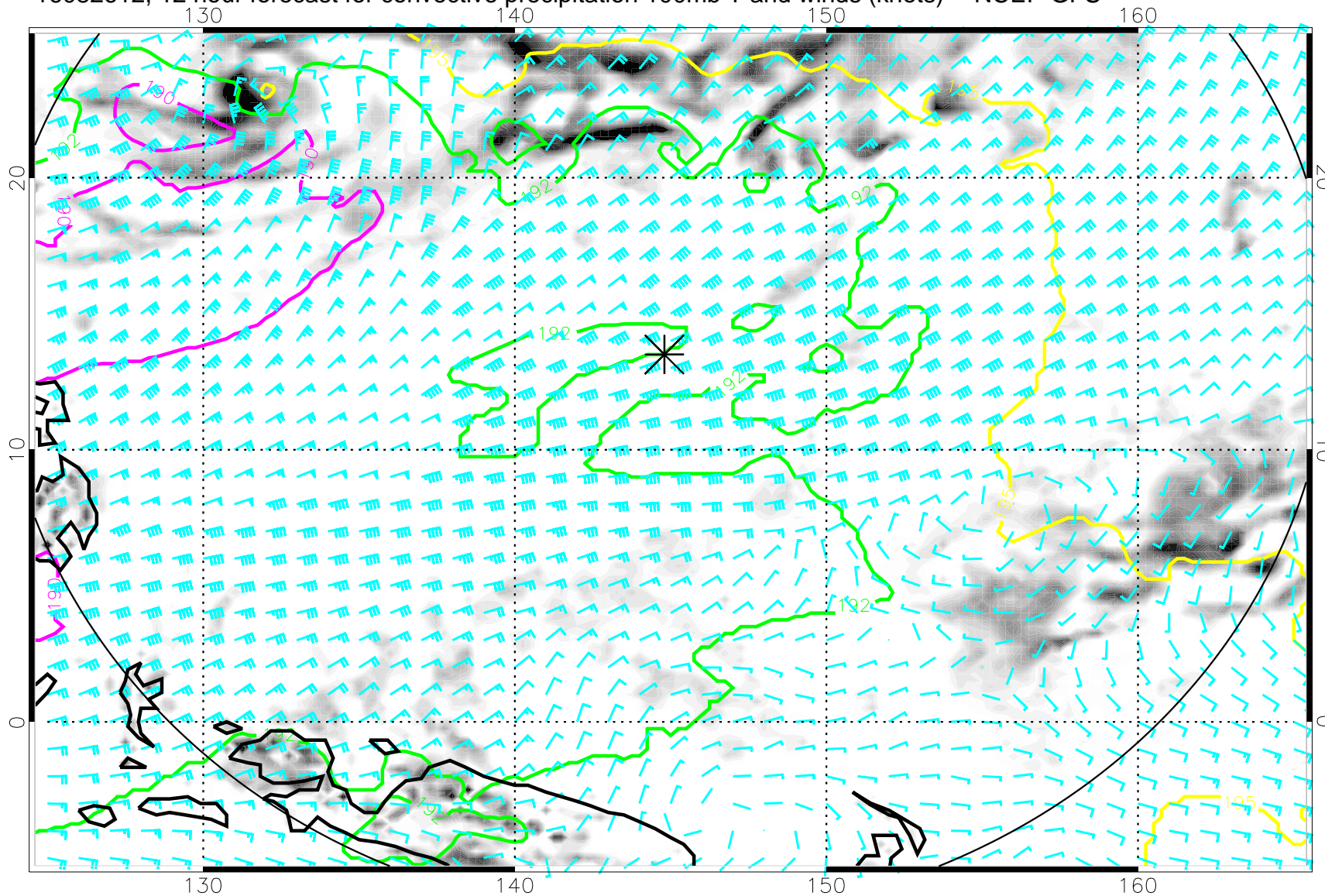
16082612, 12 hour forecast for convective precipitation 100mb T and winds (knots) -- NCEP GFS
