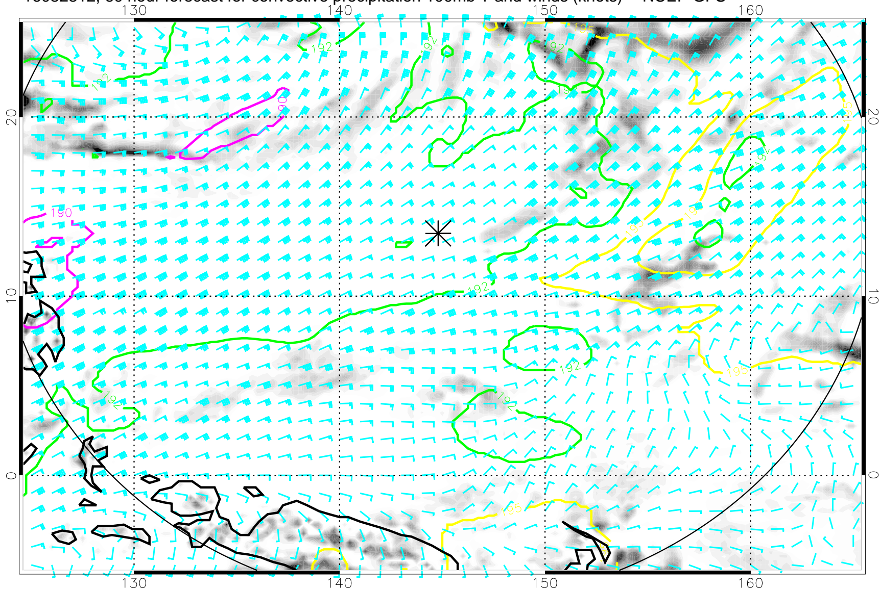
16082812, 60 hour forecast for convective precipitation 100mb T and winds (knots) -- NCEP GFS
