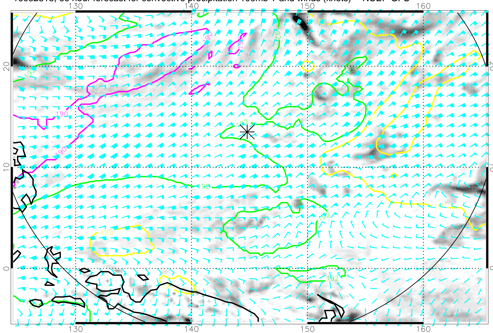
16082818, 66 hour forecast for convective precipitation 100mb T and winds (knots) -- NCEP GFS
