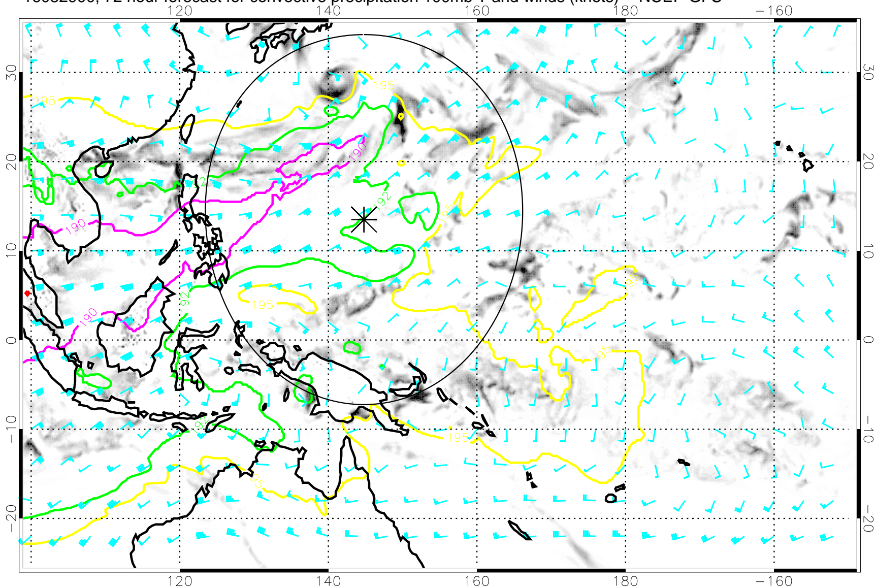
16082900, 72 hour forecast for convective precipitation 100mb T and winds (knots) -- NCEP GFS
