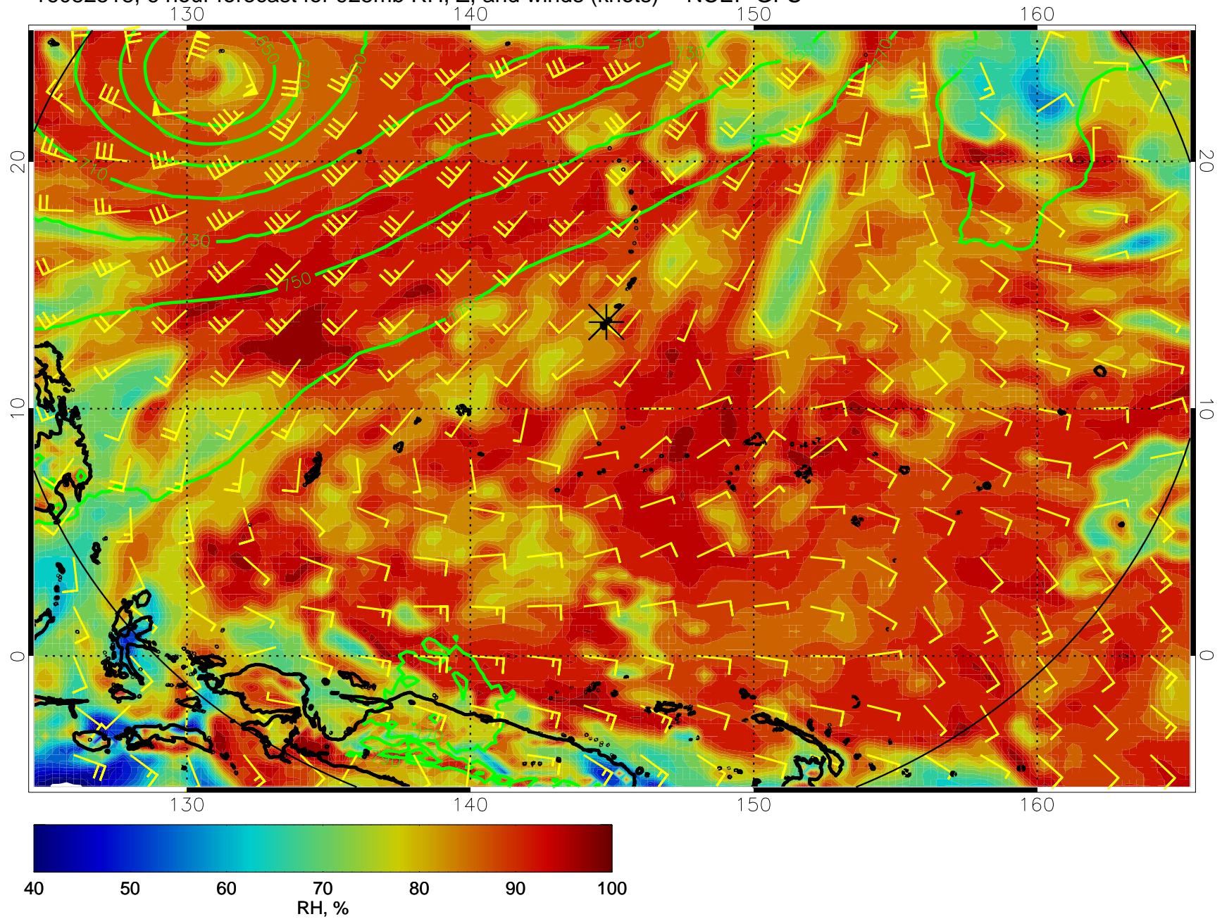
16082518, 6 hour forecast for 925mb RH, Z, and winds (knots) -- NCEP GFS
