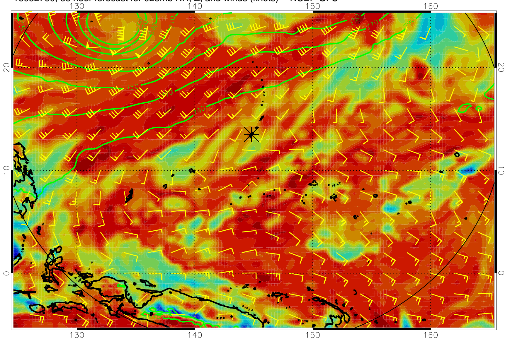
16082700, 36 hour forecast for 925mb RH, Z, and winds (knots) -- NCEP GFS
