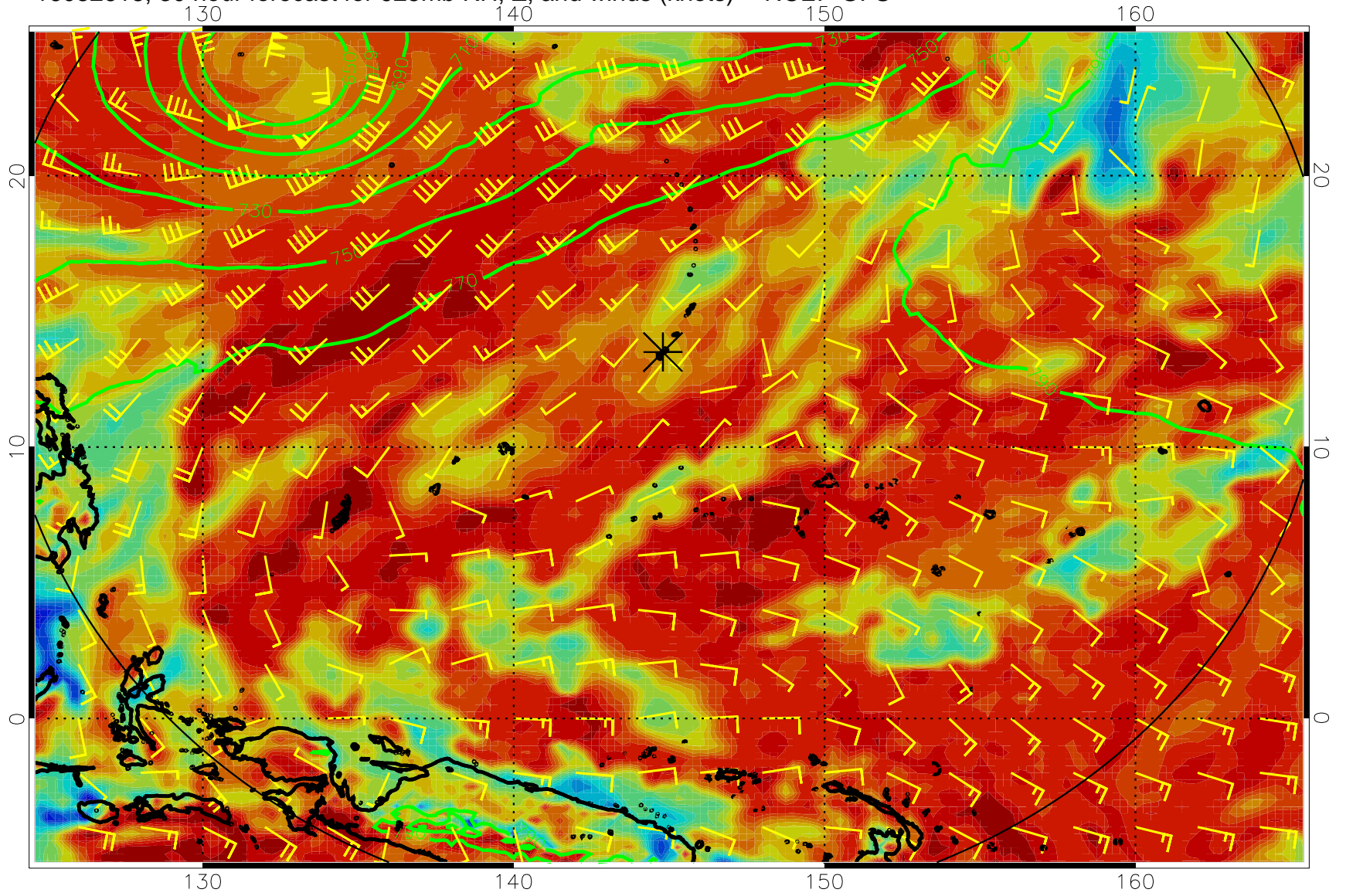
16082618, 30 hour forecast for 925mb RH, Z, and winds (knots) -- NCEP GFS
