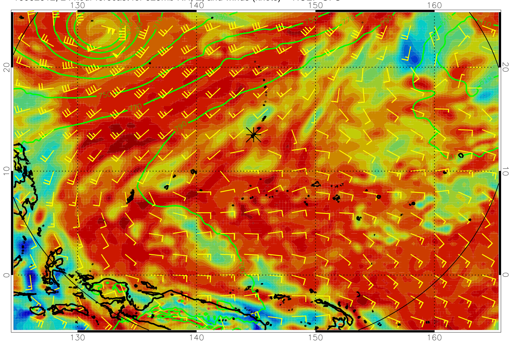
16082612, 24 hour forecast for 925mb RH, Z, and winds (knots) -- NCEP GFS
