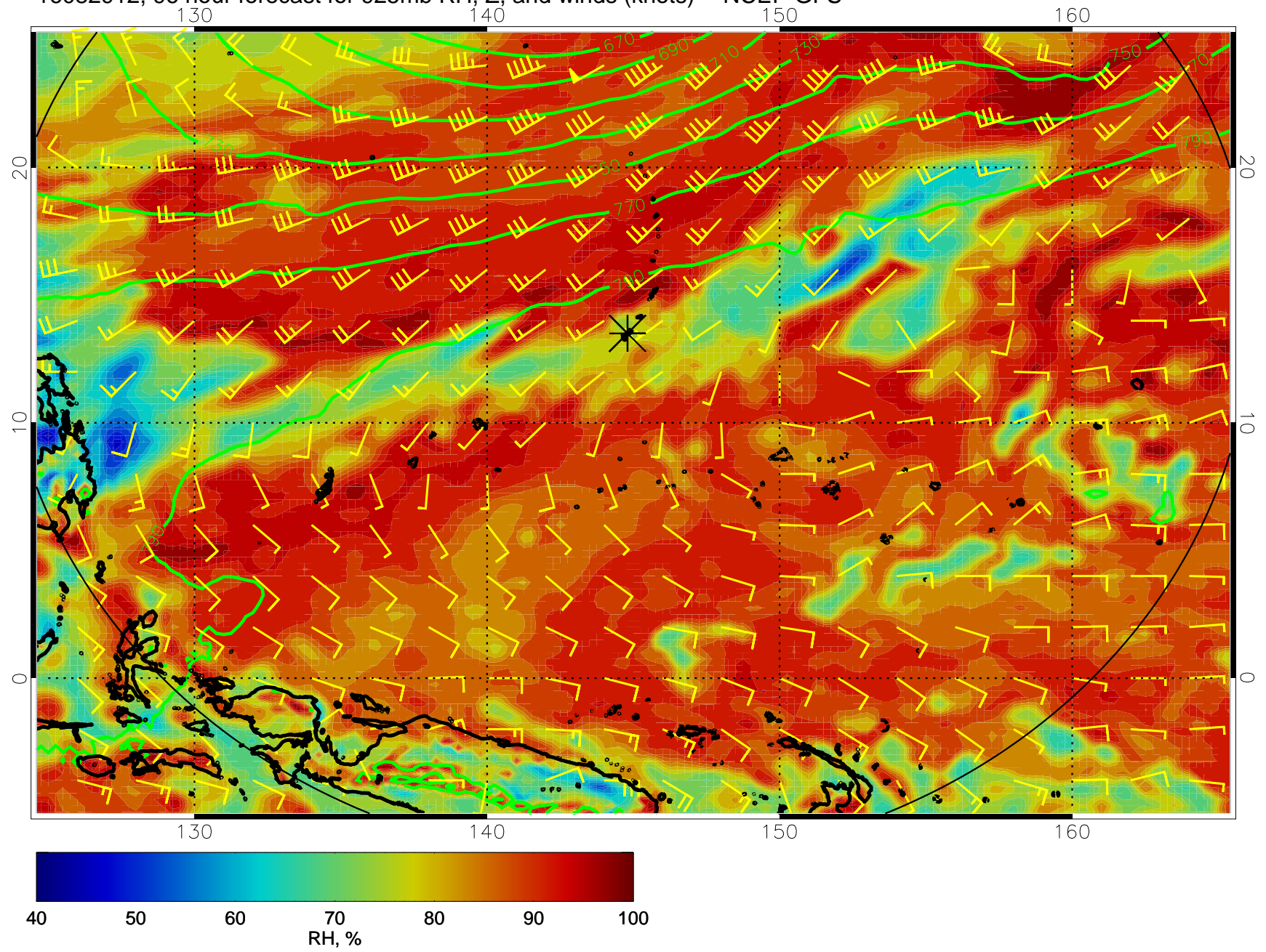
16082912, 96 hour forecast for 925mb RH, Z, and winds (knots) -- NCEP GFS
