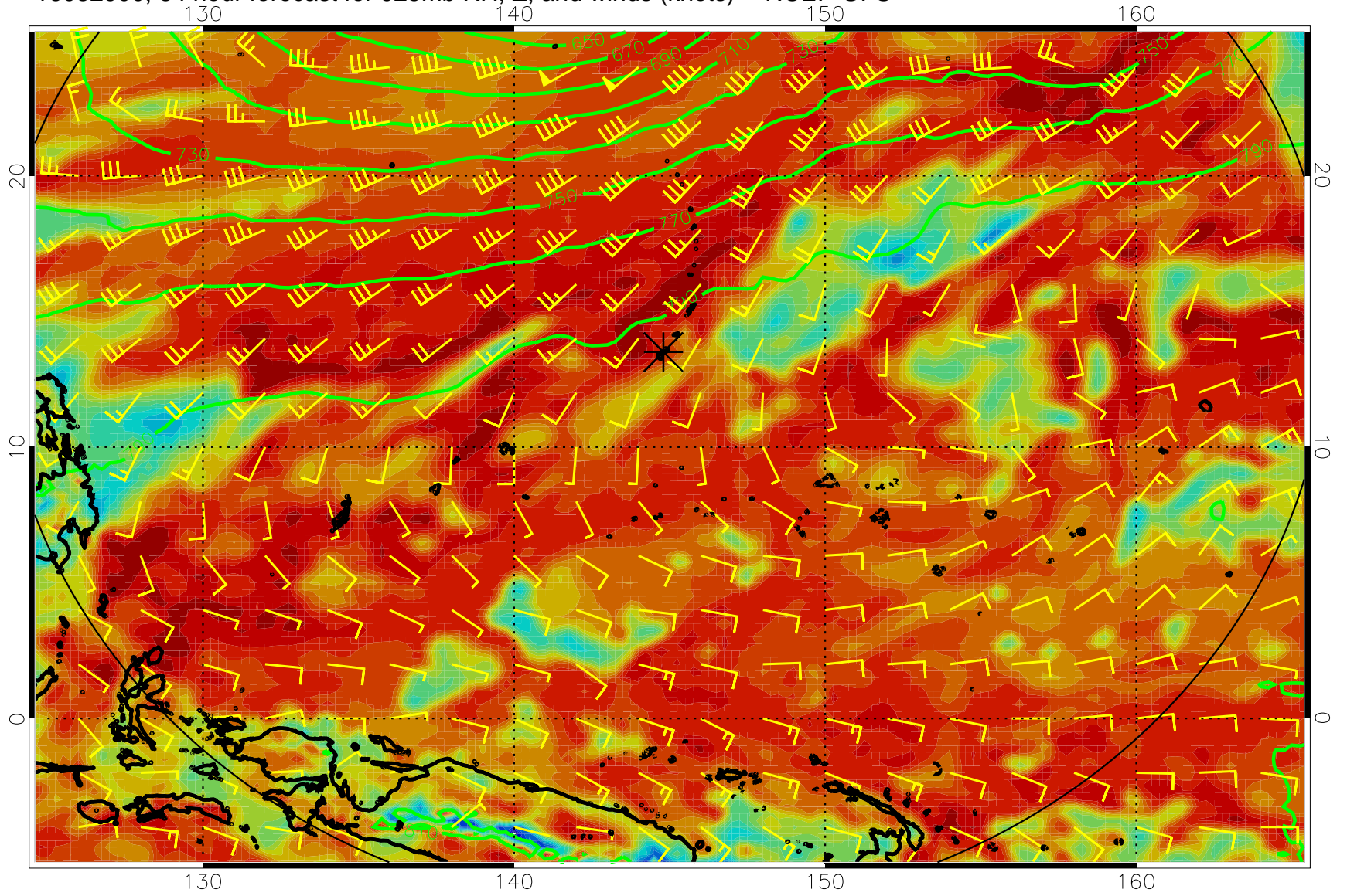
16082900, 84 hour forecast for 925mb RH, Z, and winds (knots) -- NCEP GFS
