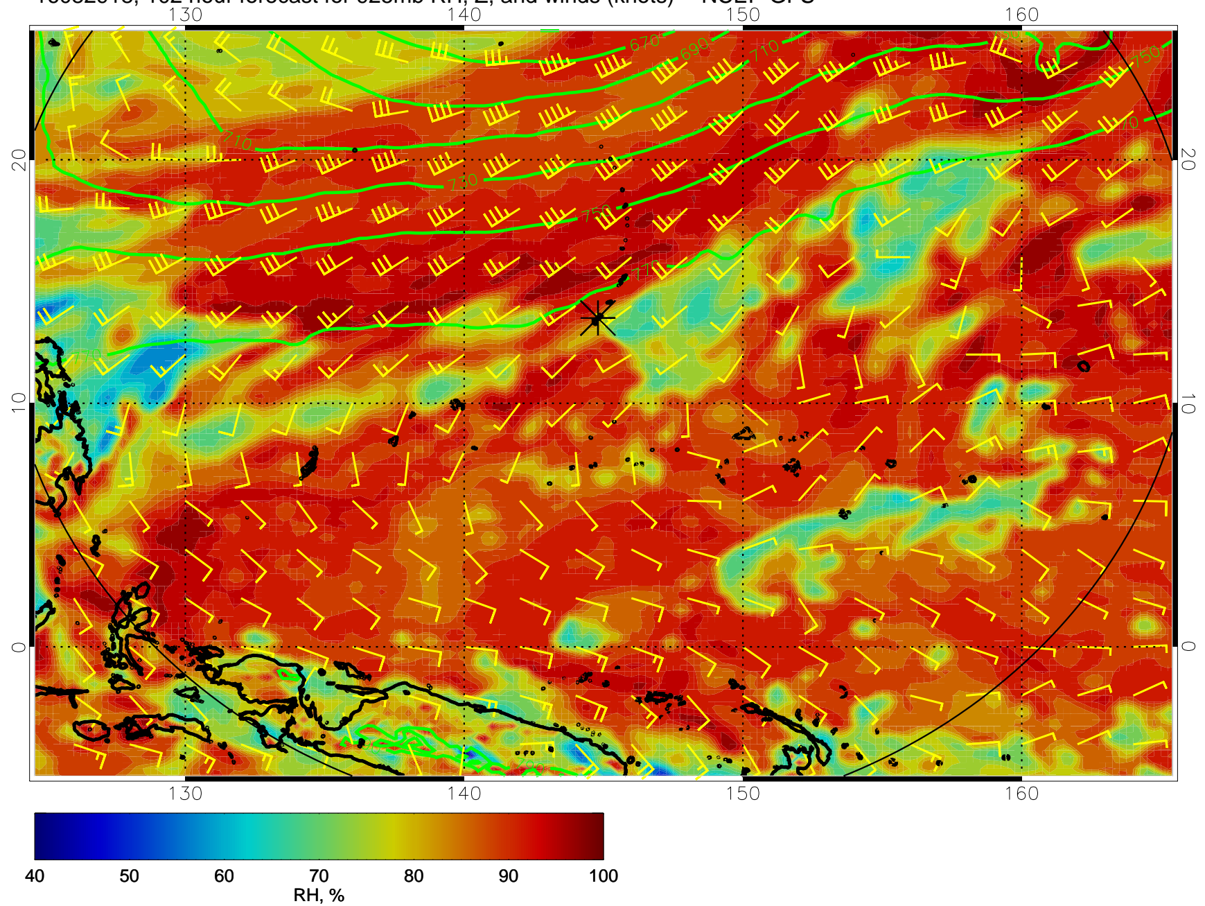
16082918, 102 hour forecast for 925mb RH, Z, and winds (knots) -- NCEP GFS
