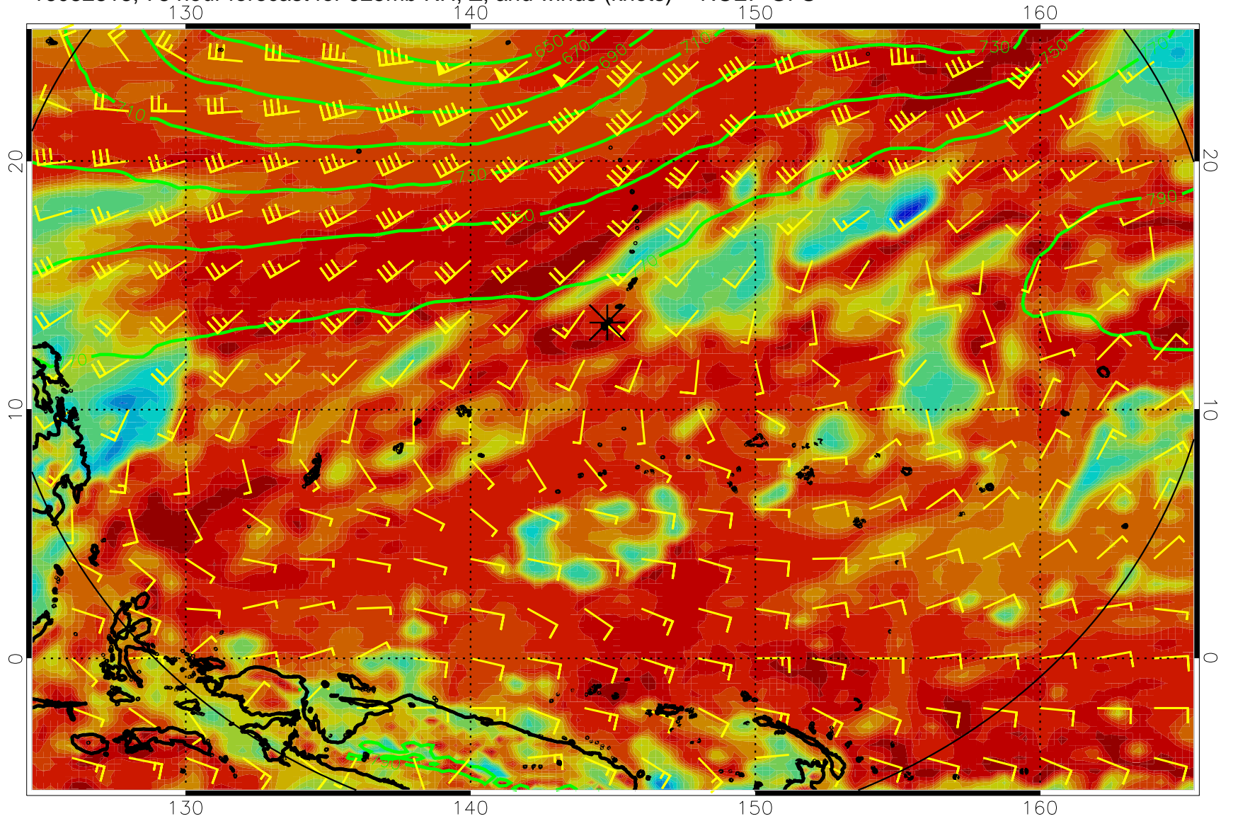
16082818, 78 hour forecast for 925mb RH, Z, and winds (knots) -- NCEP GFS
