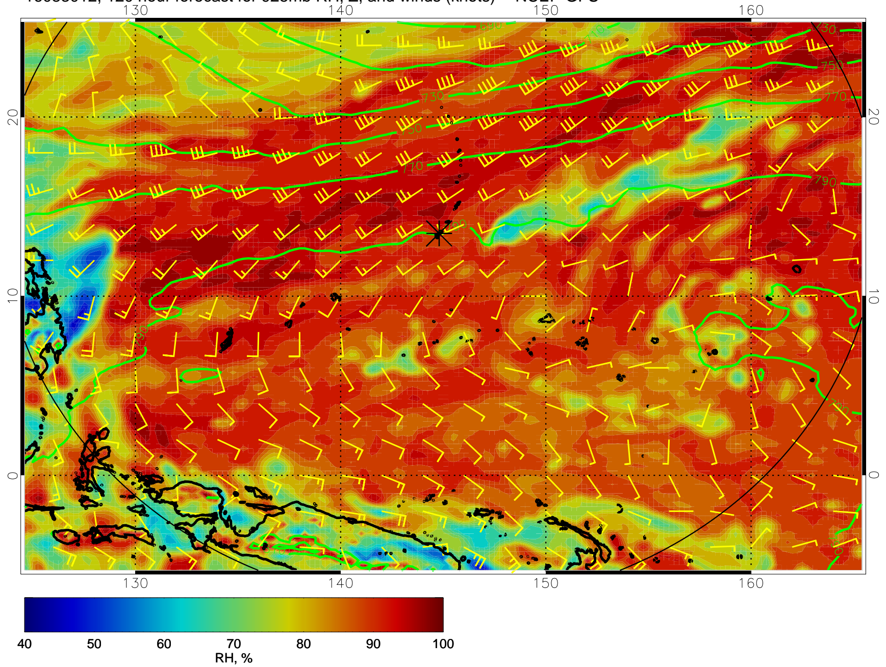
16083012, 120 hour forecast for 925mb RH, Z, and winds (knots) -- NCEP GFS
