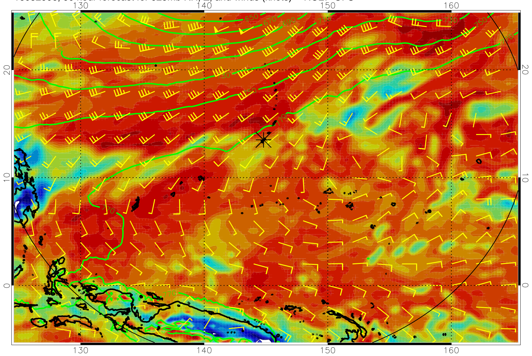
16082906, 90 hour forecast for 925mb RH, Z, and winds (knots) -- NCEP GFS
