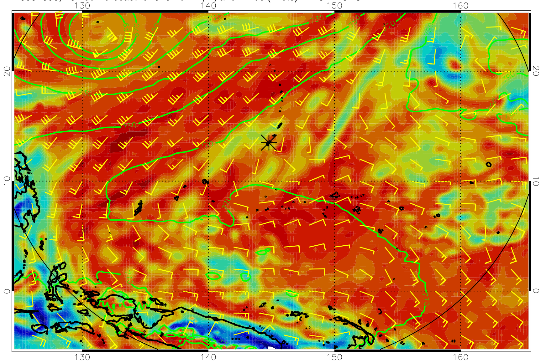
16082606, 18 hour forecast for 925mb RH, Z, and winds (knots) -- NCEP GFS
