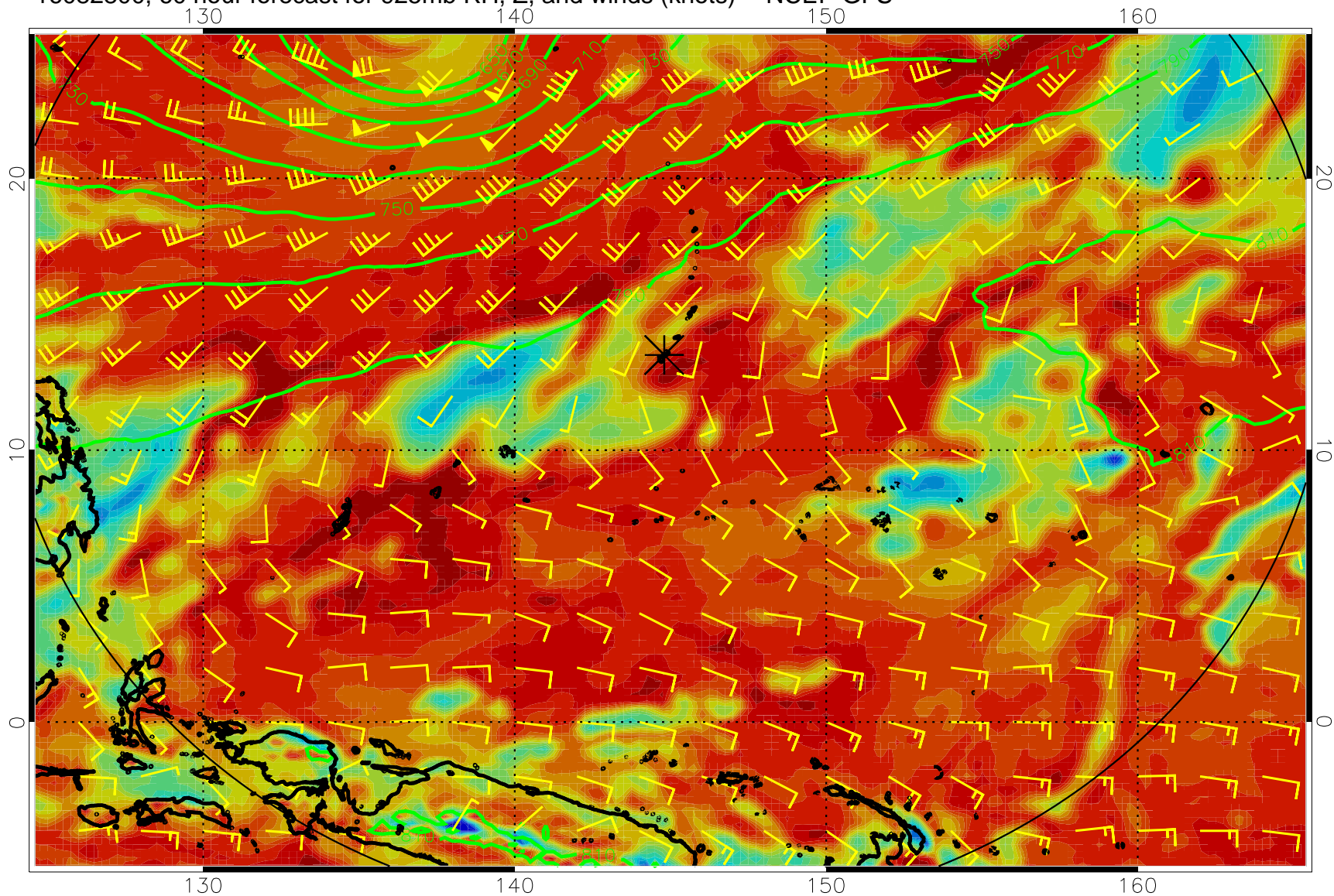
16082800, 60 hour forecast for 925mb RH, Z, and winds (knots) -- NCEP GFS
