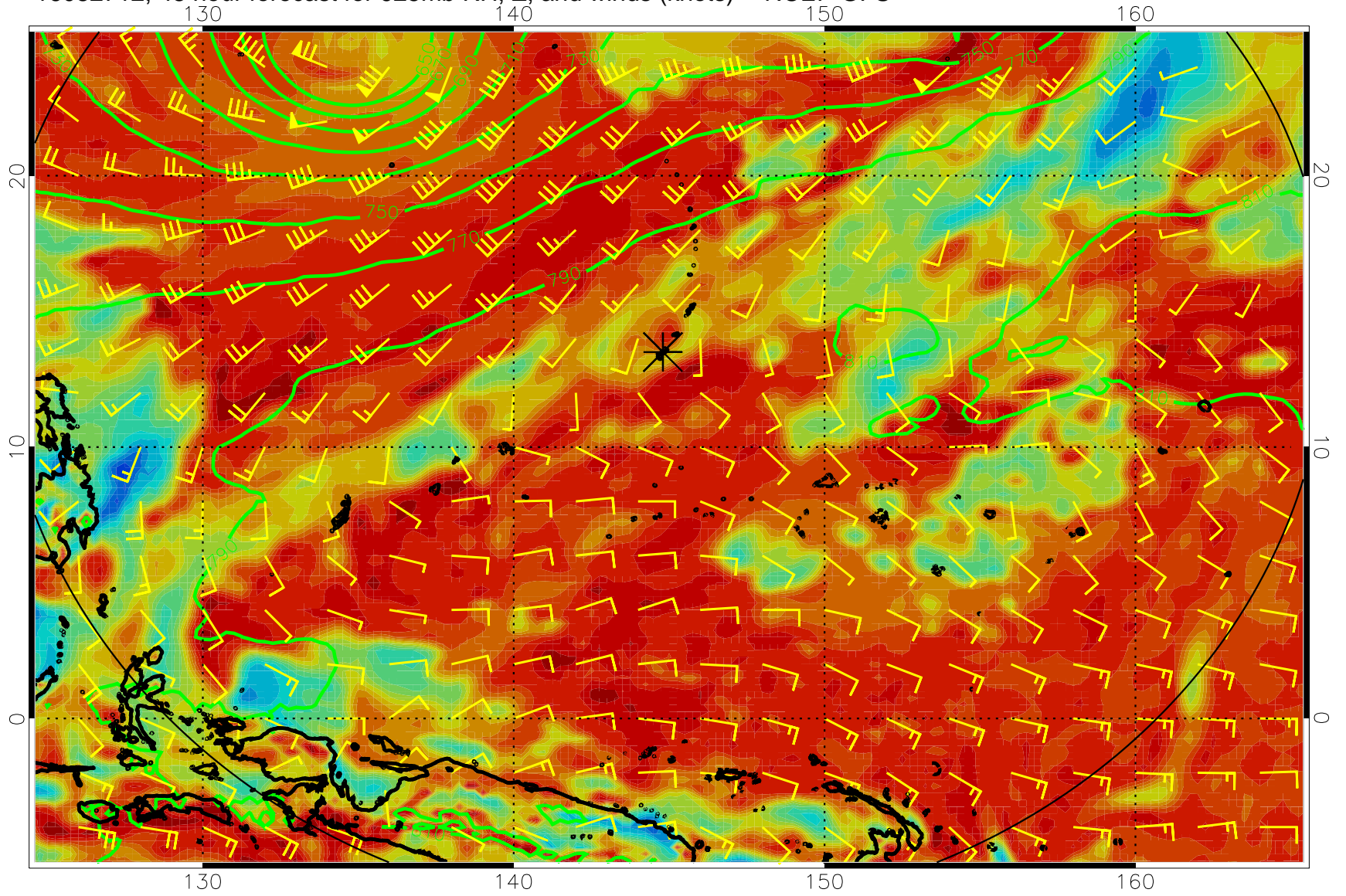
16082712, 48 hour forecast for 925mb RH, Z, and winds (knots) -- NCEP GFS
