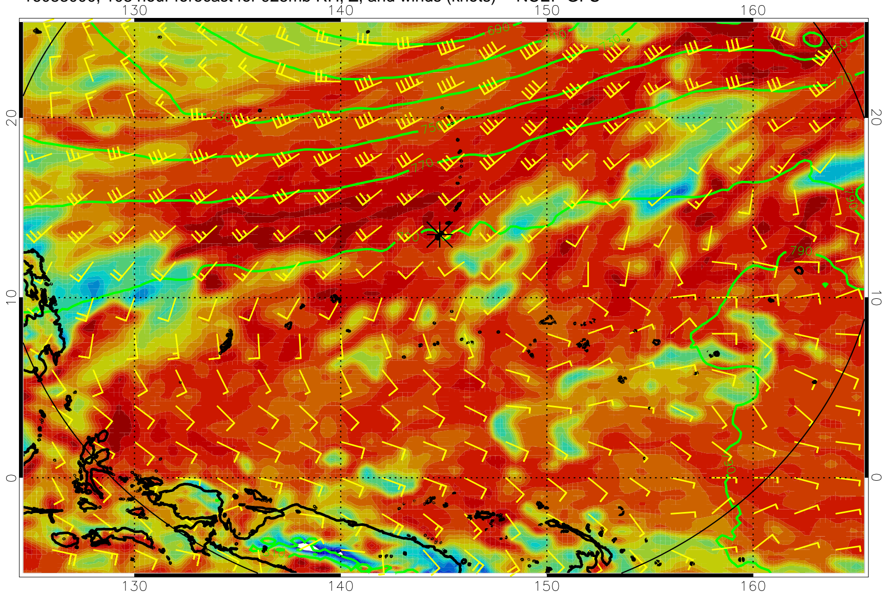
16083000, 108 hour forecast for 925mb RH, Z, and winds (knots) -- NCEP GFS
