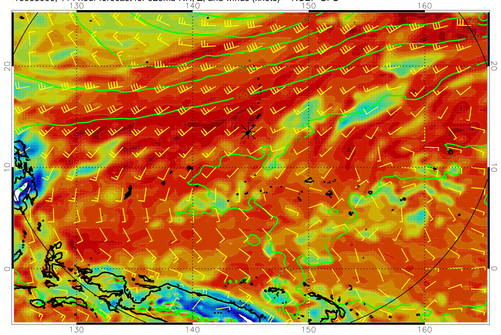
16083006, 114 hour forecast for 925mb RH, Z, and winds (knots) -- NCEP GFS
