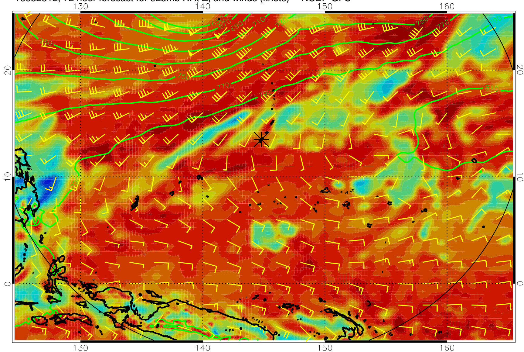
16082812, 72 hour forecast for 925mb RH, Z, and winds (knots) -- NCEP GFS
