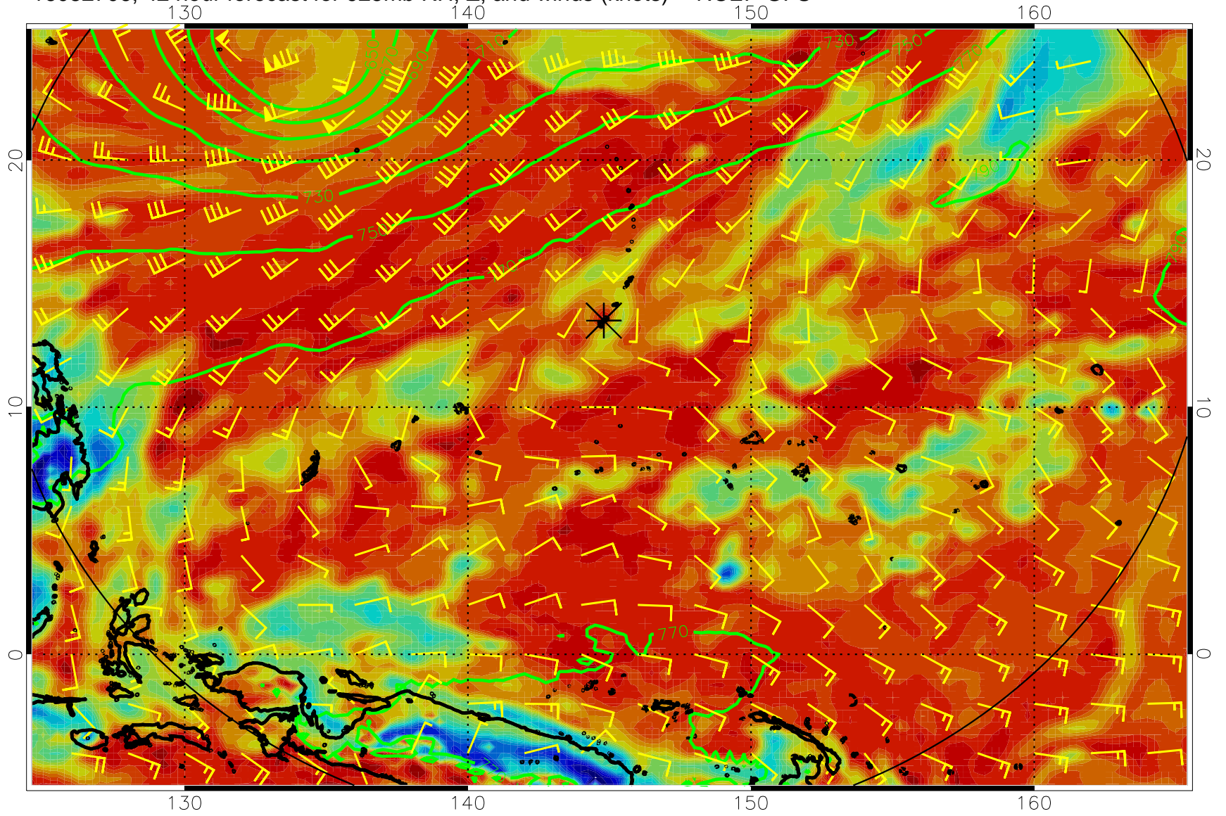
16082706, 42 hour forecast for 925mb RH, Z, and winds (knots) -- NCEP GFS
