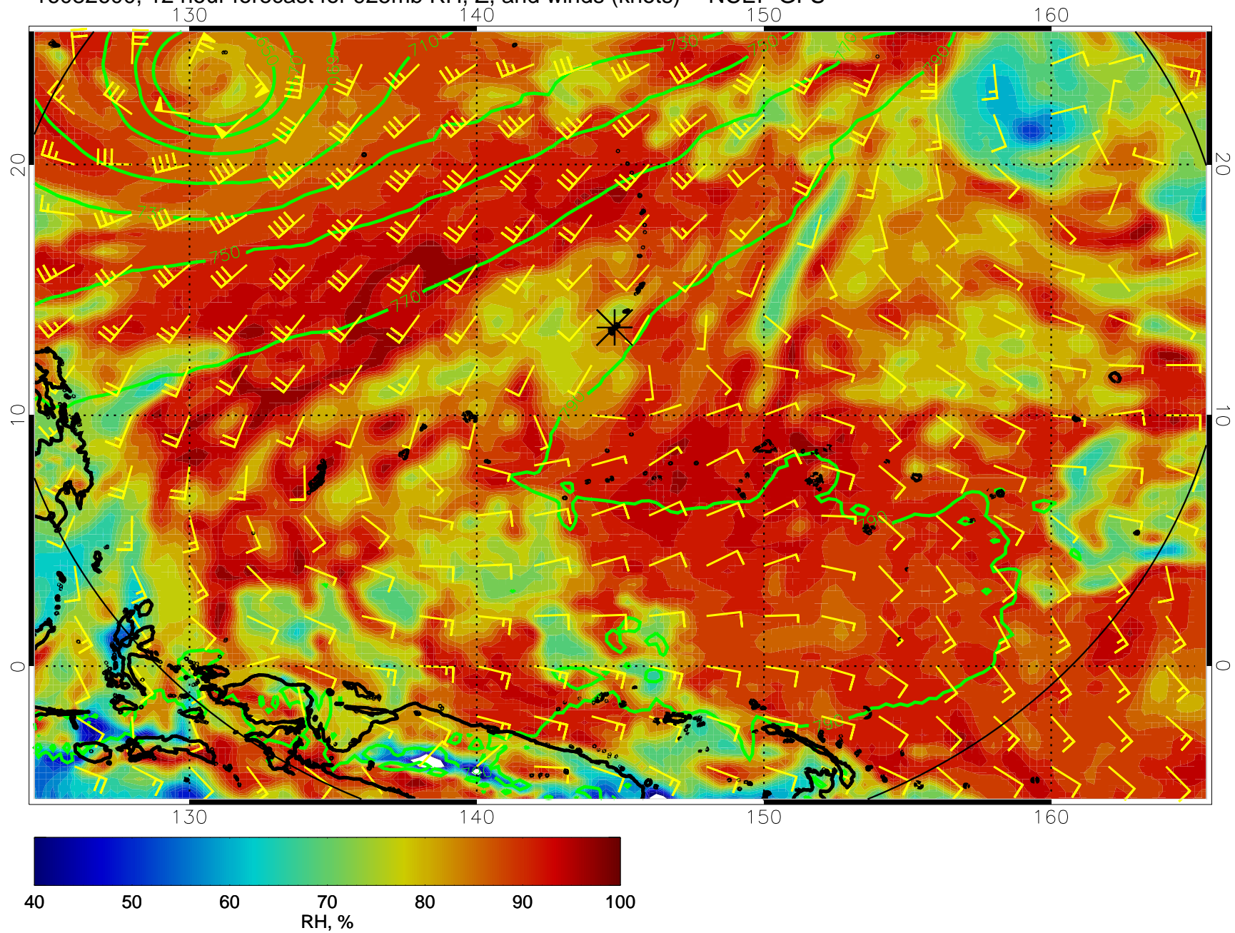
16082600, 12 hour forecast for 925mb RH, Z, and winds (knots) -- NCEP GFS
