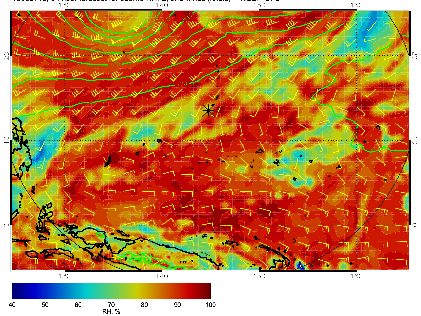
16082718, 54 hour forecast for 925mb RH, Z, and winds (knots) -- NCEP GFS
