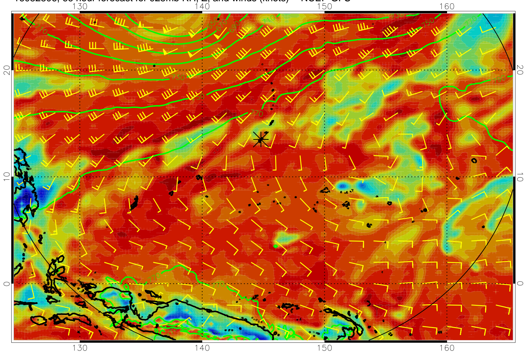
16082806, 66 hour forecast for 925mb RH, Z, and winds (knots) -- NCEP GFS
