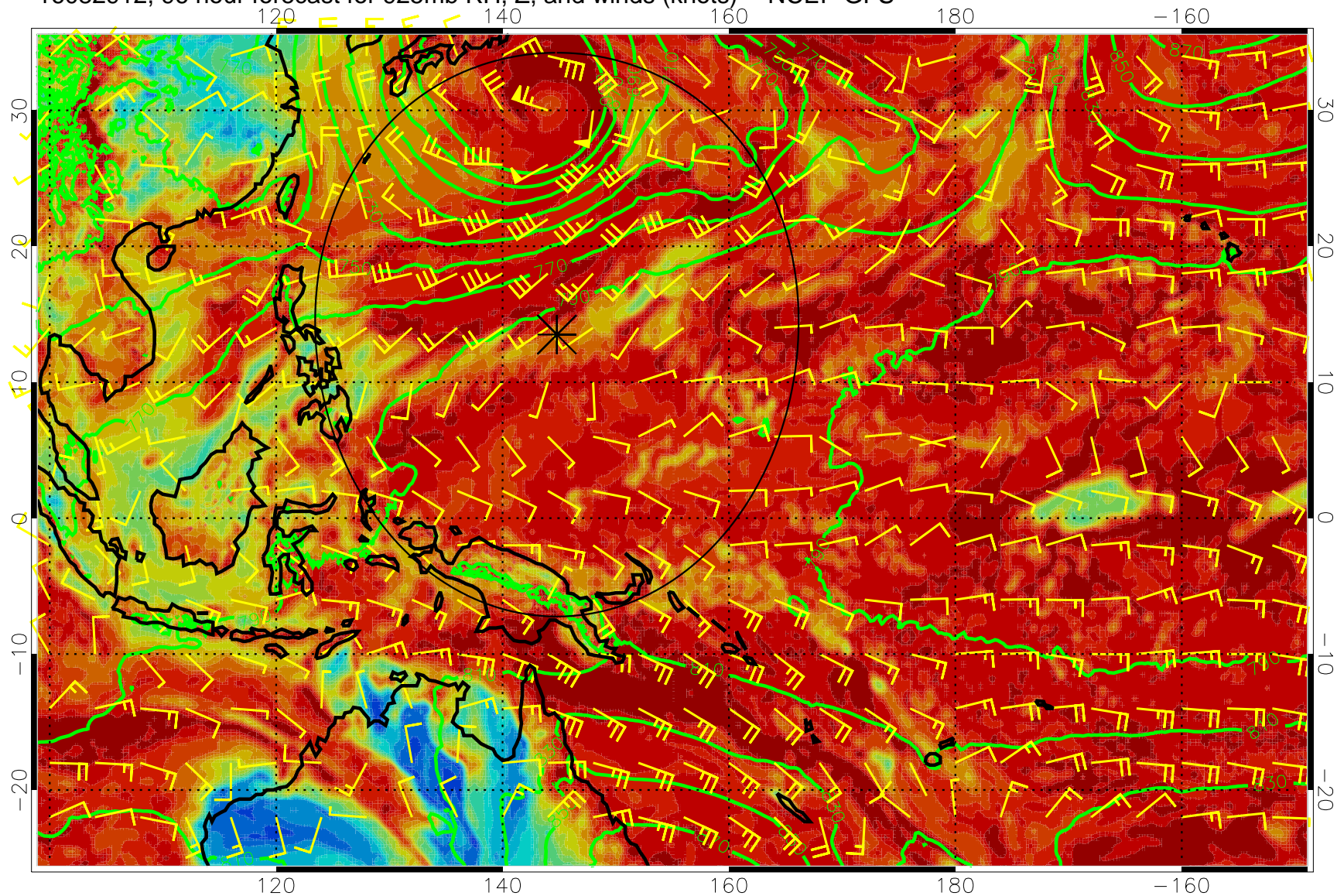
16082912, 96 hour forecast for 925mb RH, Z, and winds (knots) -- NCEP GFS
