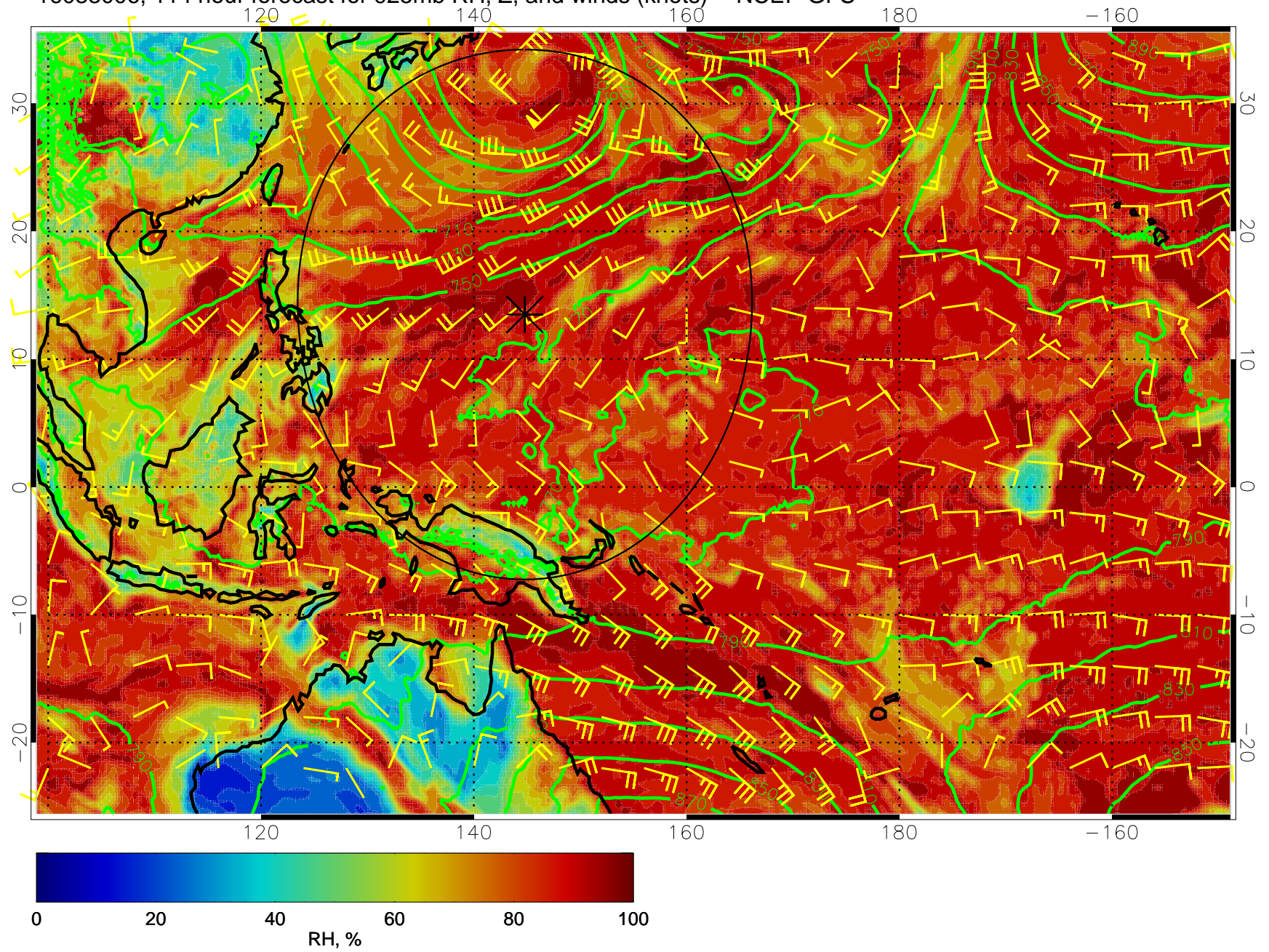
16083006, 114 hour forecast for 925mb RH, Z, and winds (knots) -- NCEP GFS
