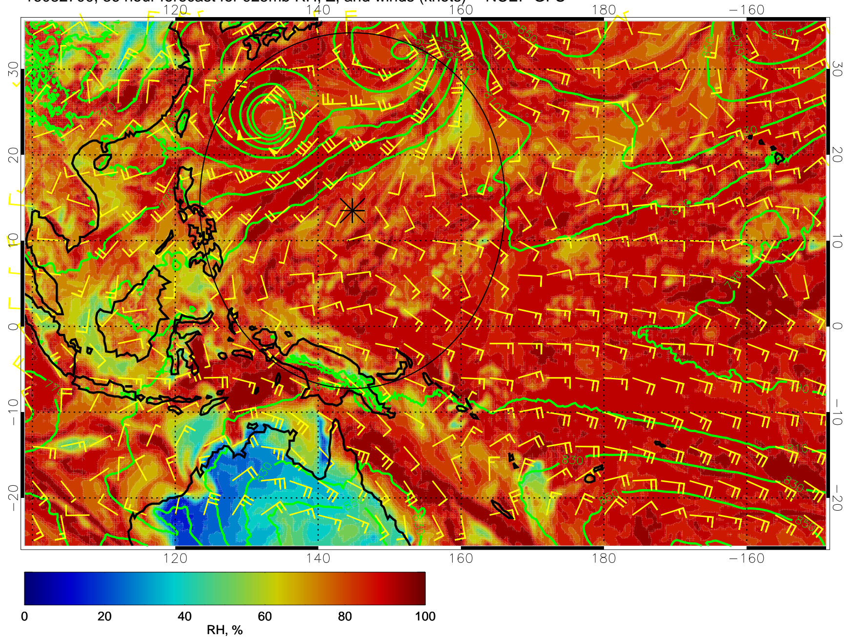
16082700, 36 hour forecast for 925mb RH, Z, and winds (knots) -- NCEP GFS
