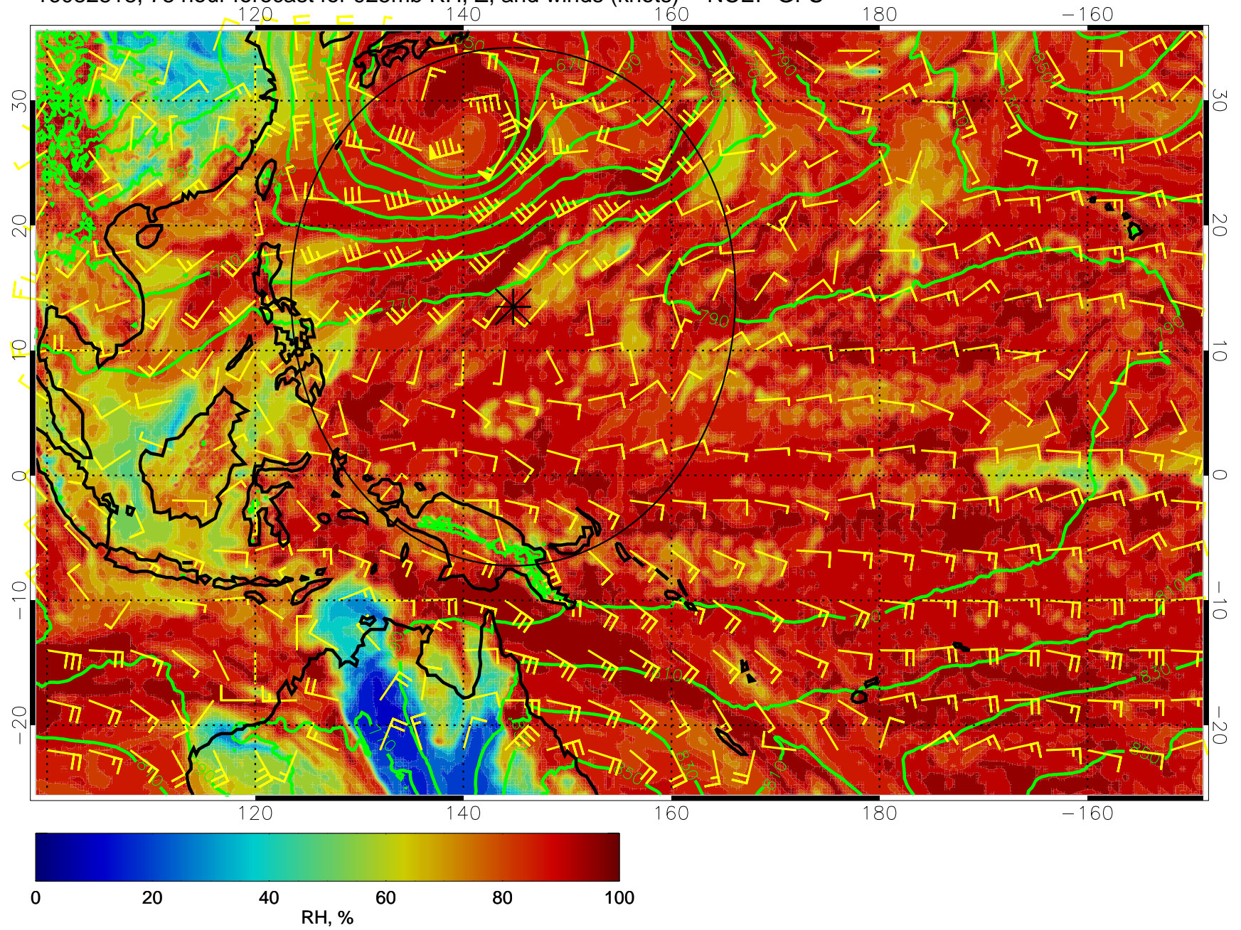
16082818, 78 hour forecast for 925mb RH, Z, and winds (knots) -- NCEP GFS
