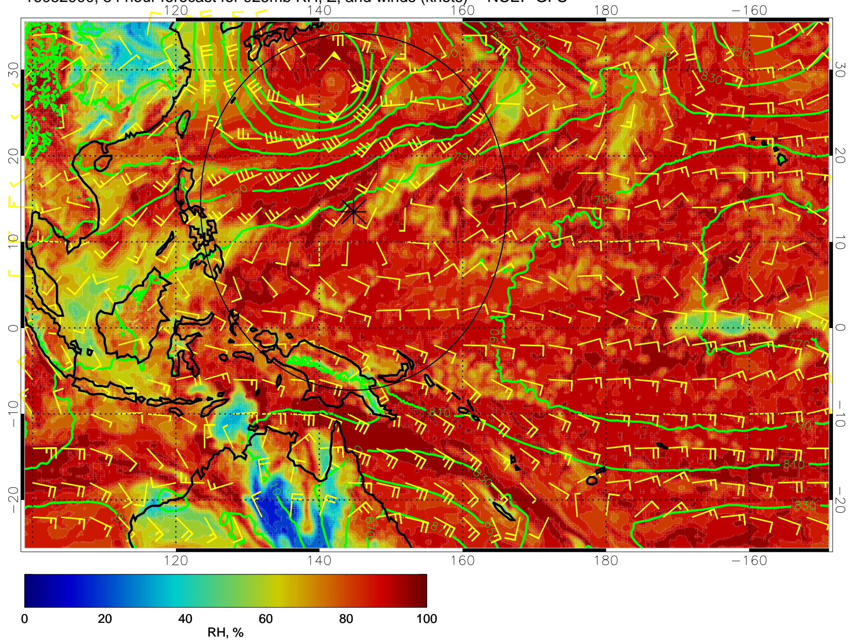
16082900, 84 hour forecast for 925mb RH, Z, and winds (knots) -- NCEP GFS
