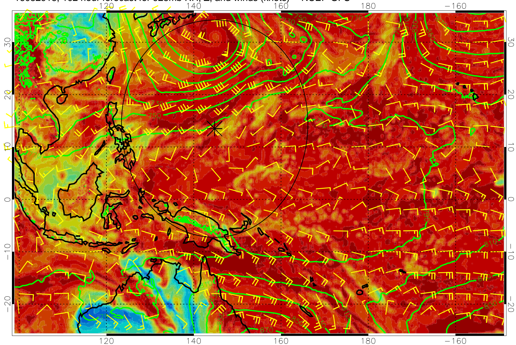
16082918, 102 hour forecast for 925mb RH, Z, and winds (knots) -- NCEP GFS
