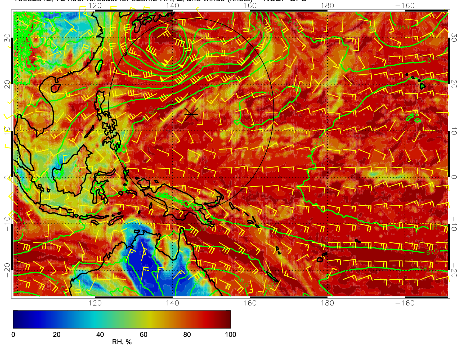
16082812, 72 hour forecast for 925mb RH, Z, and winds (knots) -- NCEP GFS
