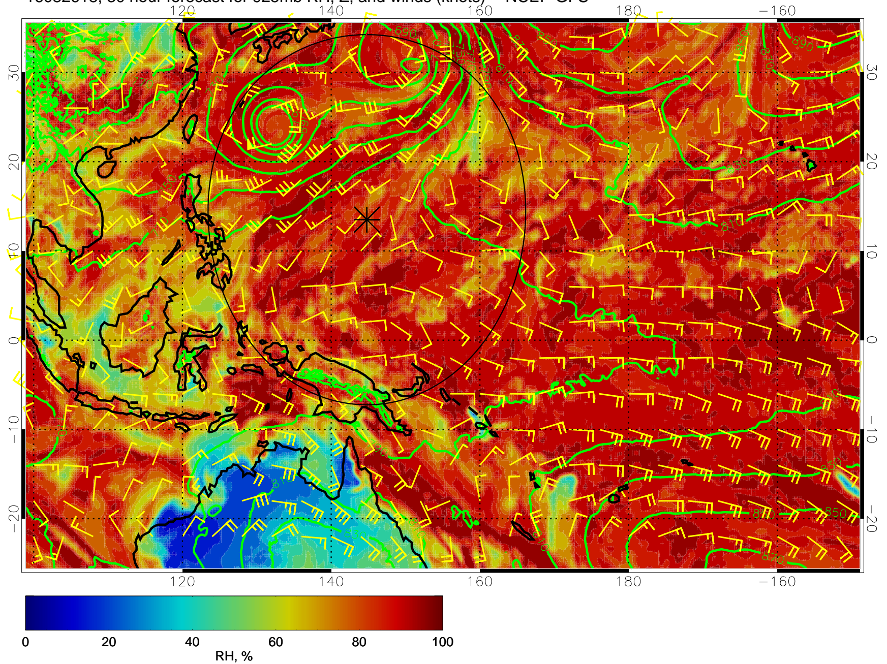
16082618, 30 hour forecast for 925mb RH, Z, and winds (knots) -- NCEP GFS
