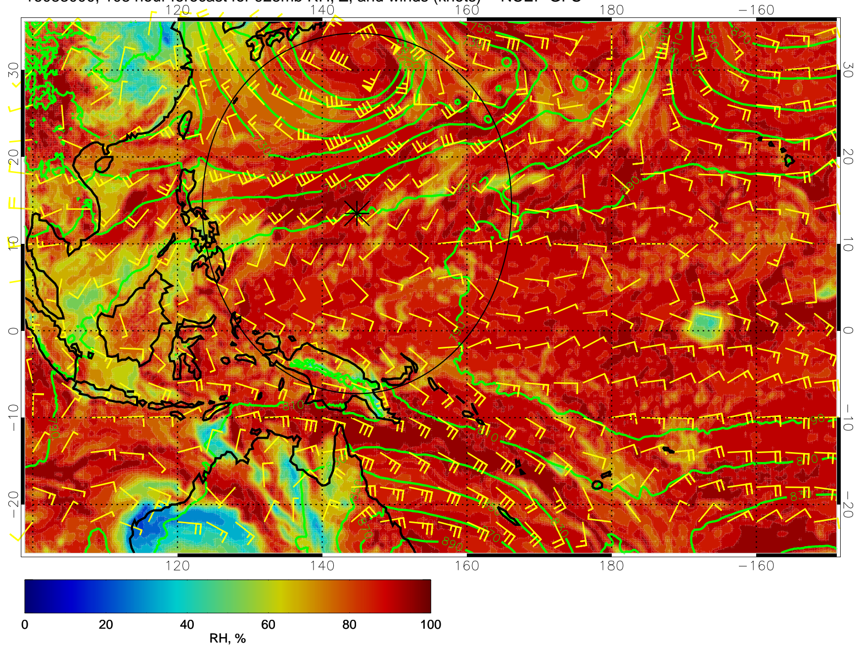
16083000, 108 hour forecast for 925mb RH, Z, and winds (knots) -- NCEP GFS
