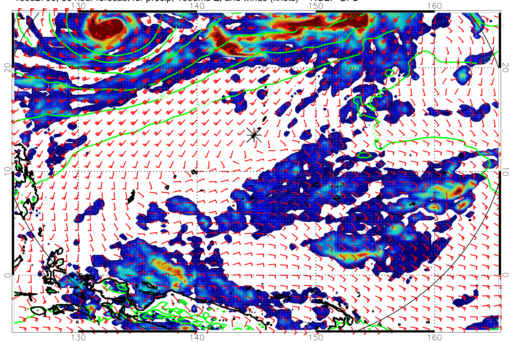
16082700, 36 hour forecast for precip, 1000mb Z, and winds (knots) -- NCEP GFS
