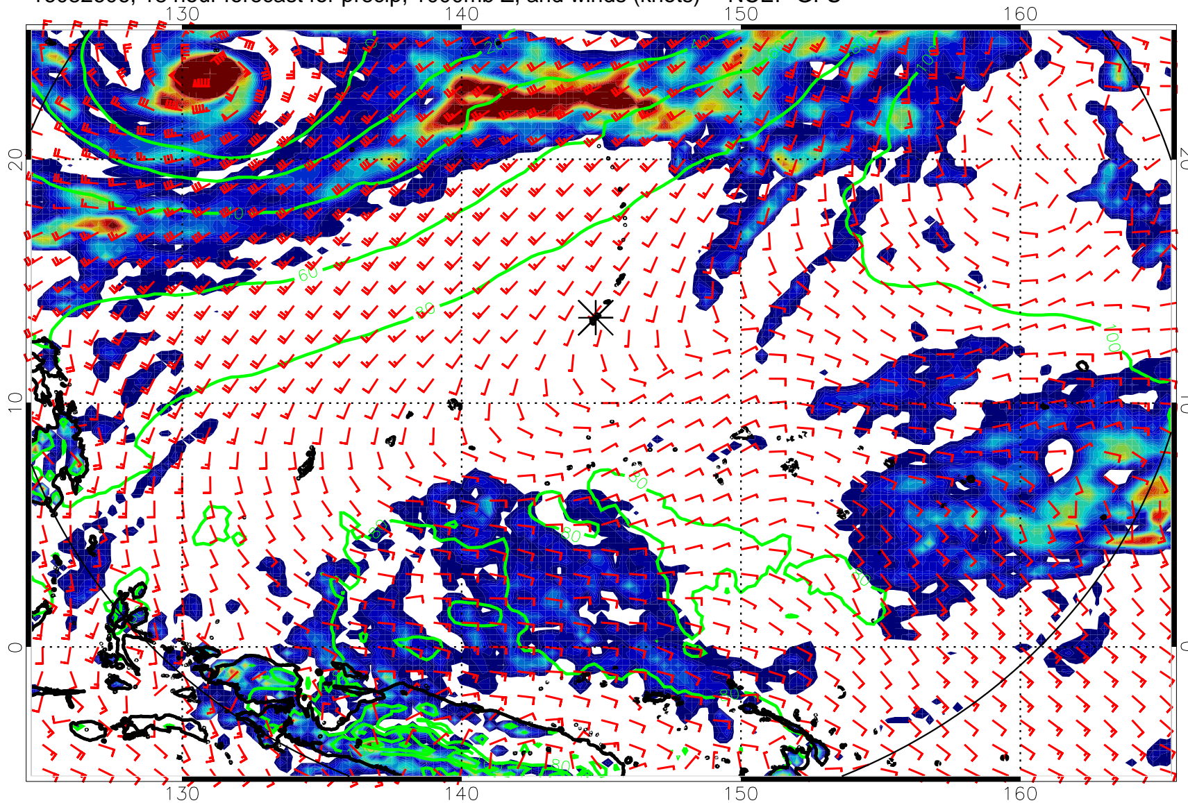
16082606, 18 hour forecast for precip, 1000mb Z, and winds (knots) -- NCEP GFS
