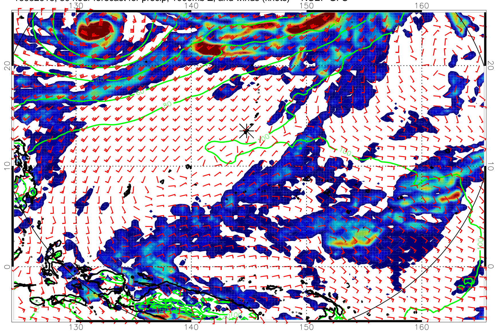
16082618, 30 hour forecast for precip, 1000mb Z, and winds (knots) -- NCEP GFS
