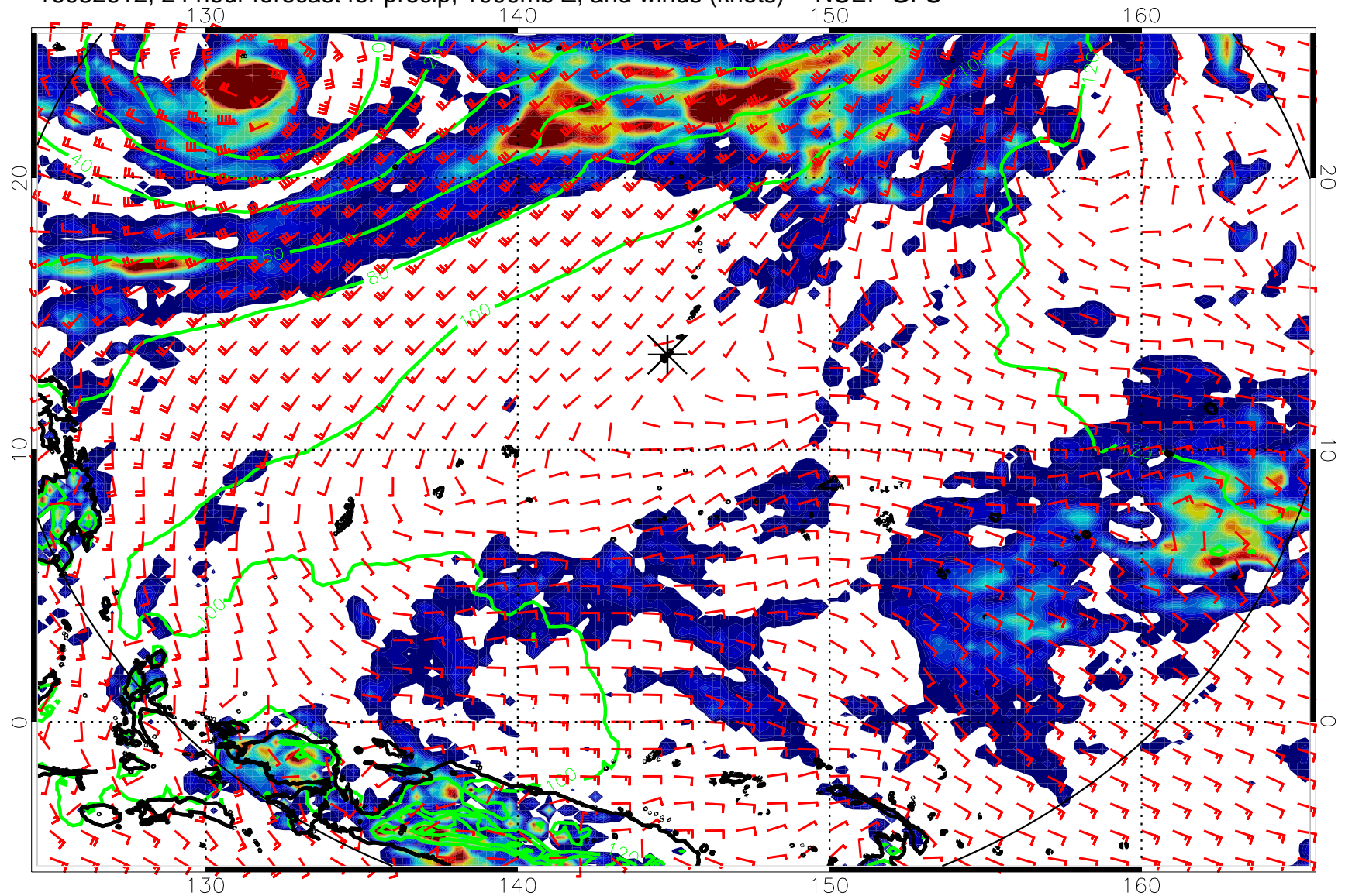
16082612, 24 hour forecast for precip, 1000mb Z, and winds (knots) -- NCEP GFS
