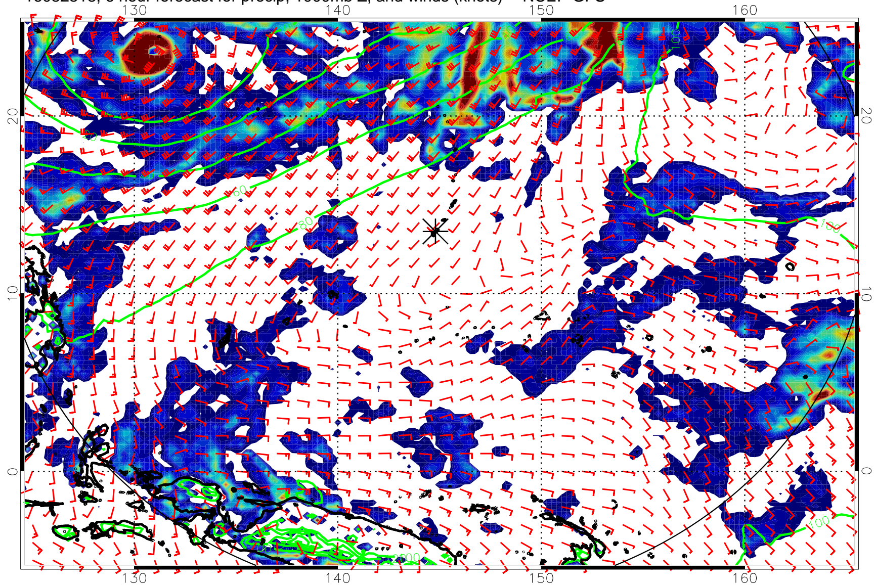
16082518, 6 hour forecast for precip, 1000mb Z, and winds (knots) -- NCEP GFS
