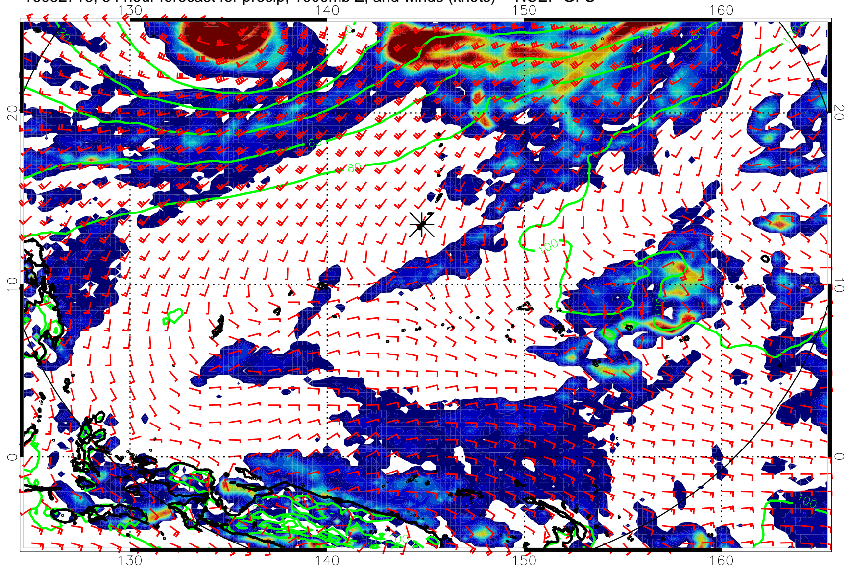
16082718, 54 hour forecast for precip, 1000mb Z, and winds (knots) -- NCEP GFS
