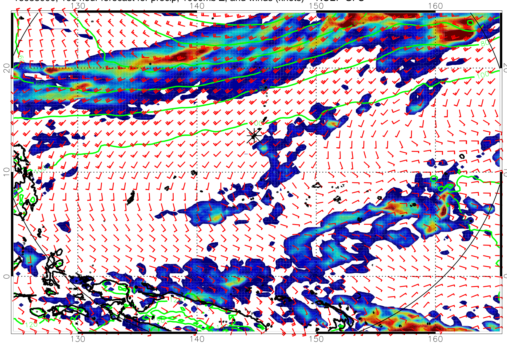
16083000, 108 hour forecast for precip, 1000mb Z, and winds (knots) -- NCEP GFS
