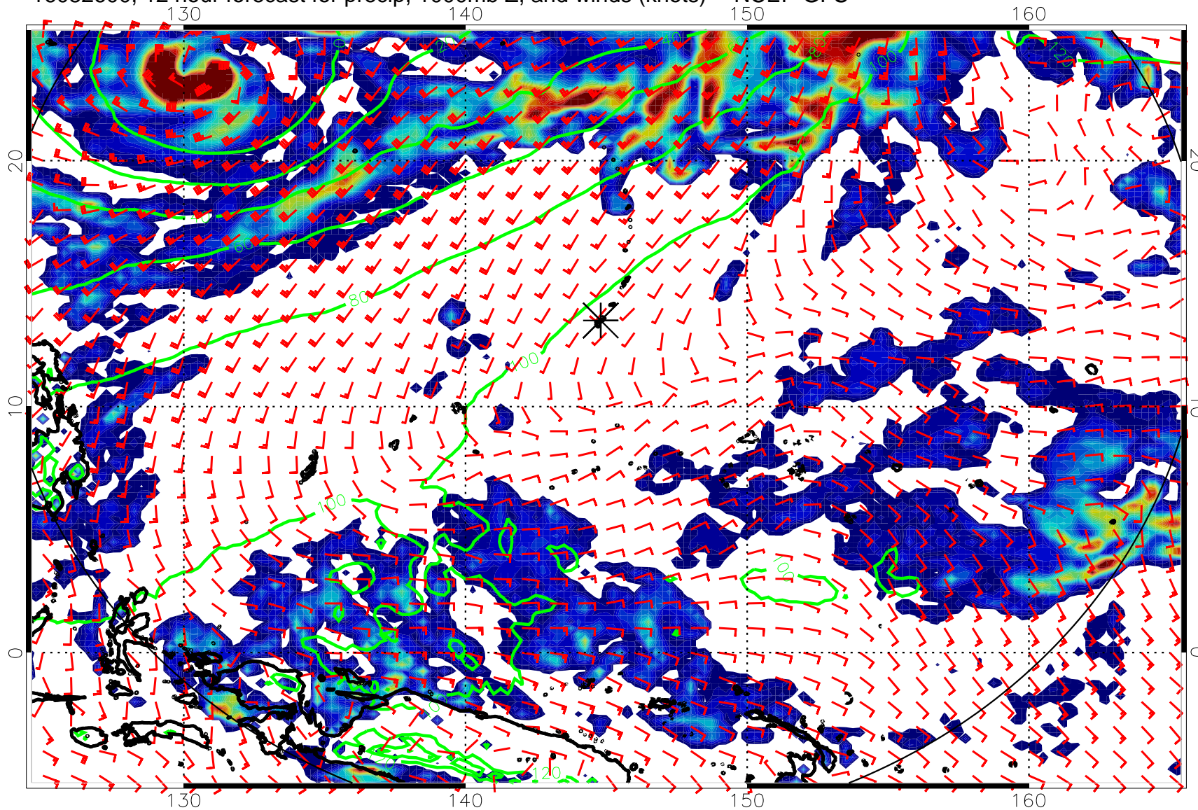
16082600, 12 hour forecast for precip, 1000mb Z, and winds (knots) -- NCEP GFS
