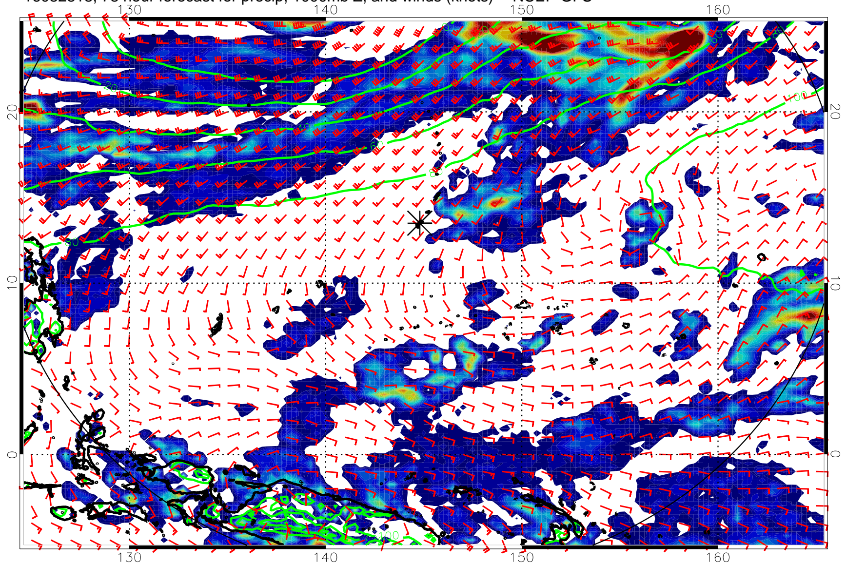
16082818, 78 hour forecast for precip, 1000mb Z, and winds (knots) -- NCEP GFS
