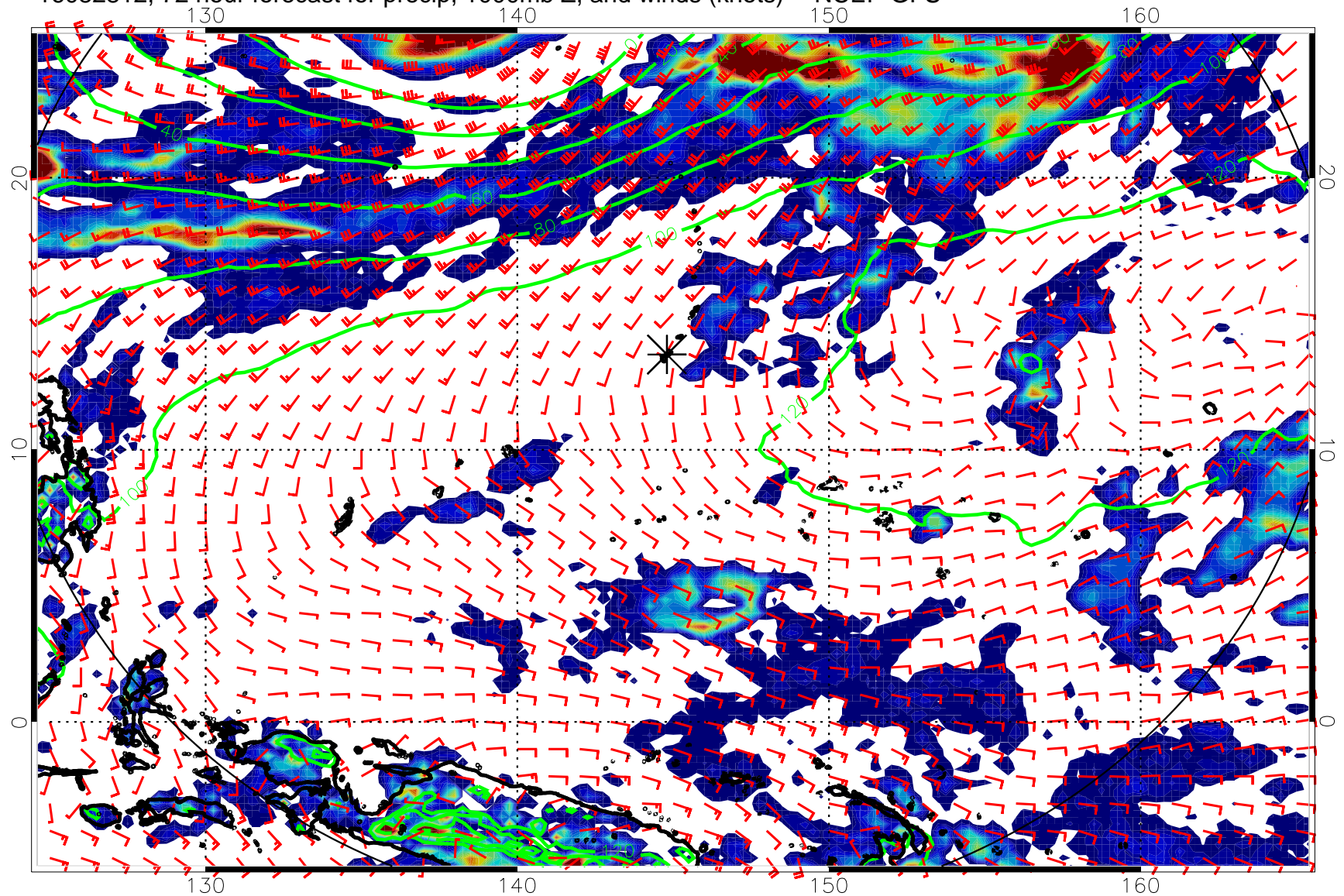
16082812, 72 hour forecast for precip, 1000mb Z, and winds (knots) -- NCEP GFS
