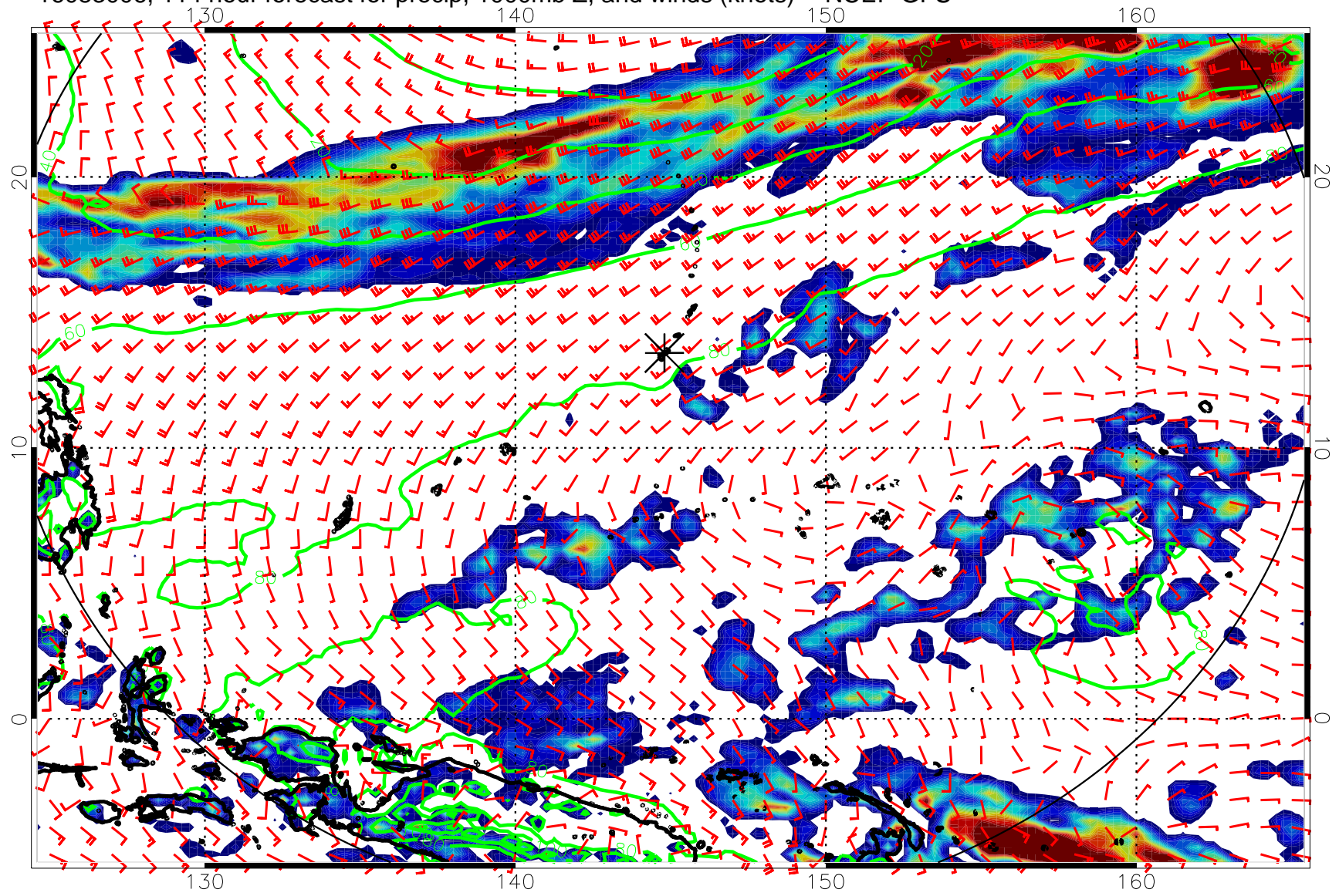
16083006, 114 hour forecast for precip, 1000mb Z, and winds (knots) -- NCEP GFS
