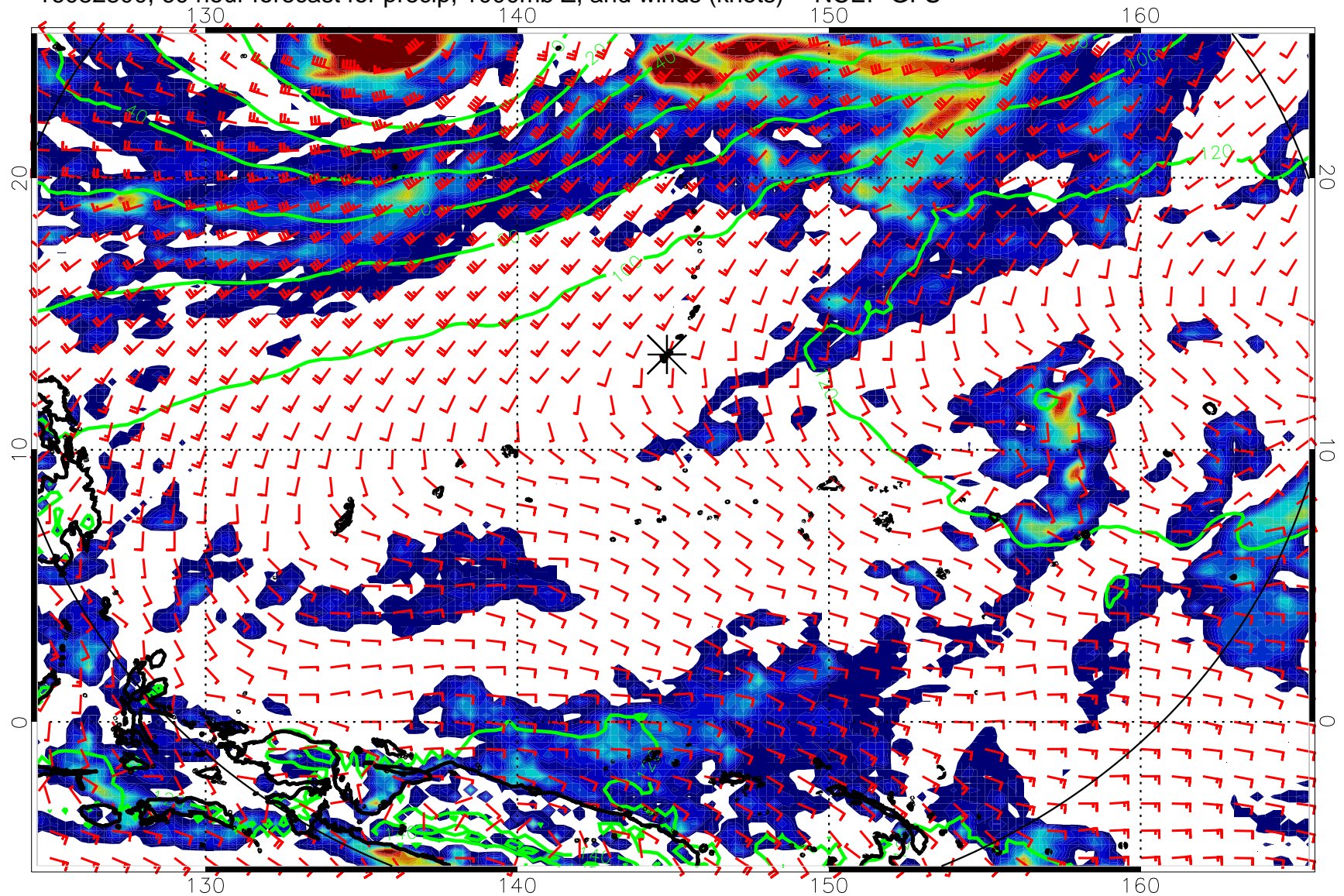
16082800, 60 hour forecast for precip, 1000mb Z, and winds (knots) -- NCEP GFS
