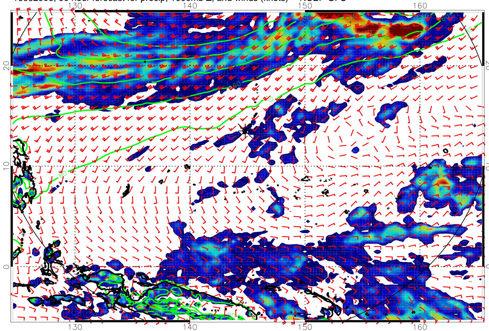
16082906, 90 hour forecast for precip, 1000mb Z, and winds (knots) -- NCEP GFS
