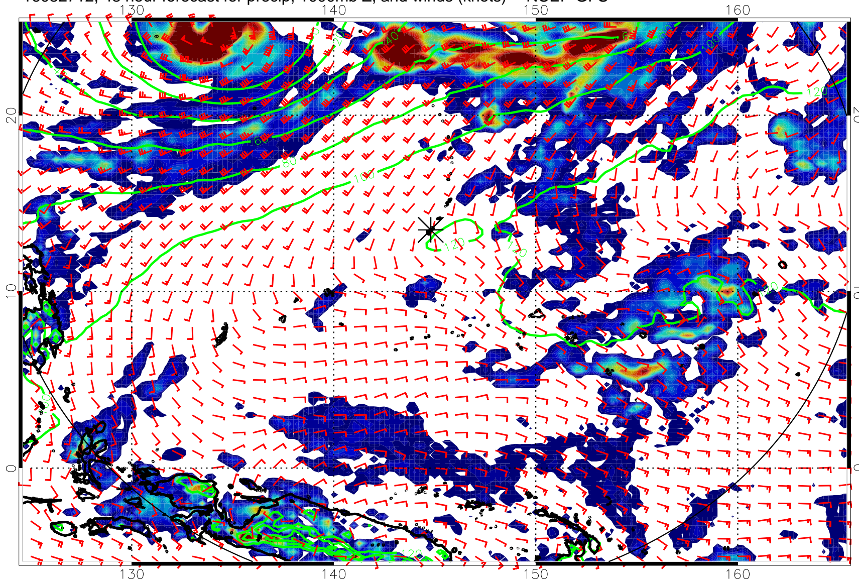
16082712, 48 hour forecast for precip, 1000mb Z, and winds (knots) -- NCEP GFS
