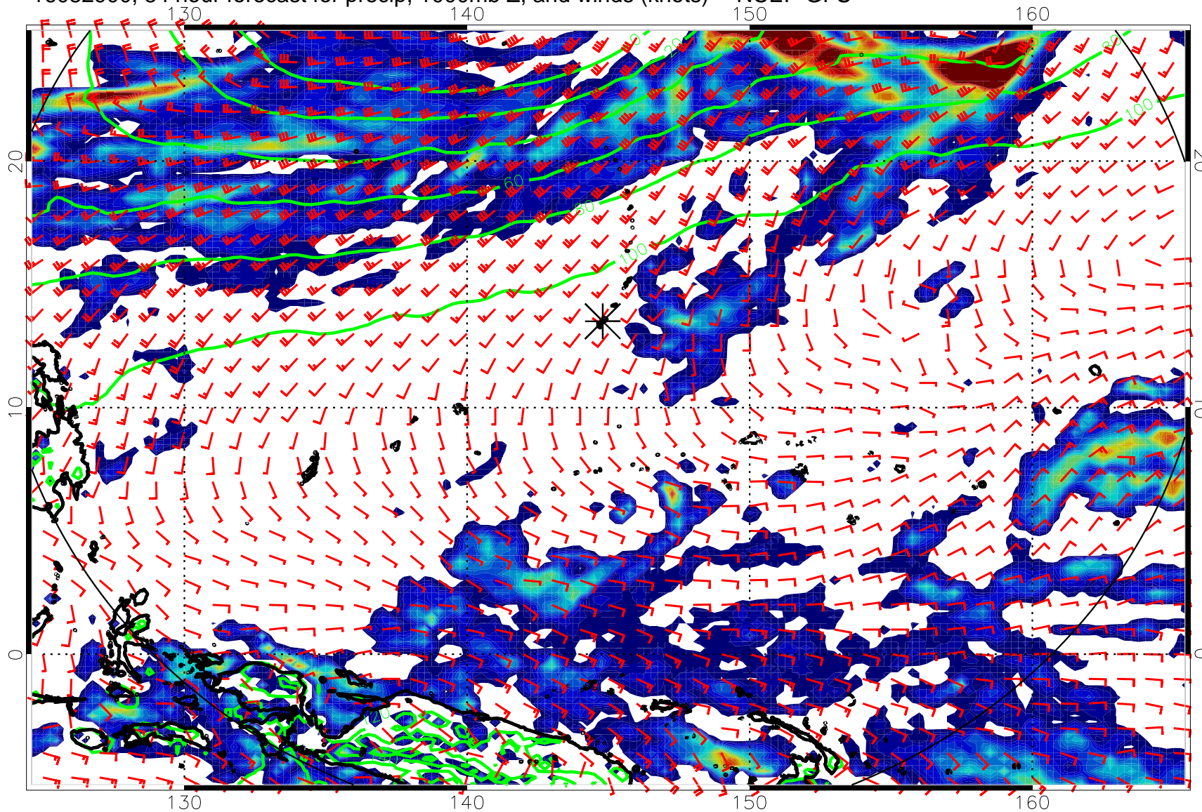
16082900, 84 hour forecast for precip, 1000mb Z, and winds (knots) -- NCEP GFS
