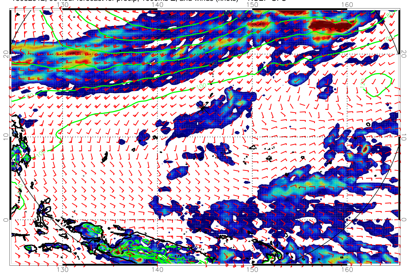
16082912, 96 hour forecast for precip, 1000mb Z, and winds (knots) -- NCEP GFS
