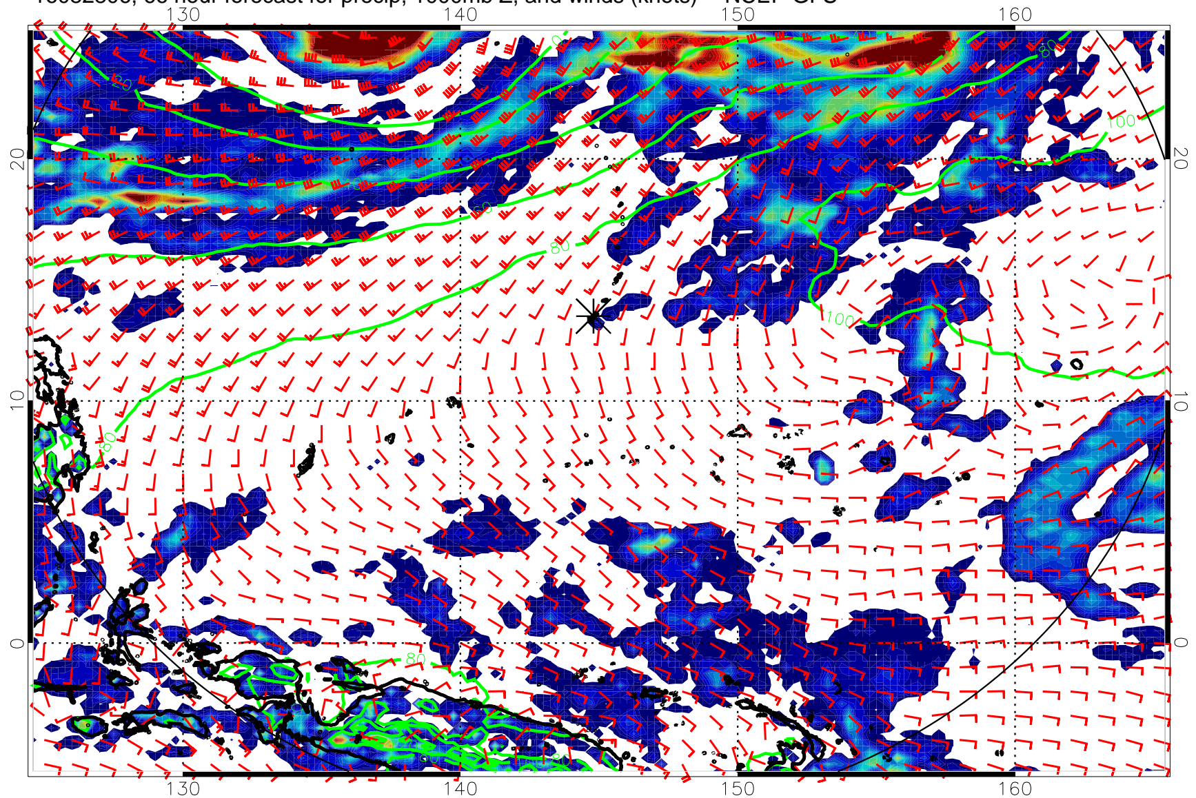
16082806, 66 hour forecast for precip, 1000mb Z, and winds (knots) -- NCEP GFS
