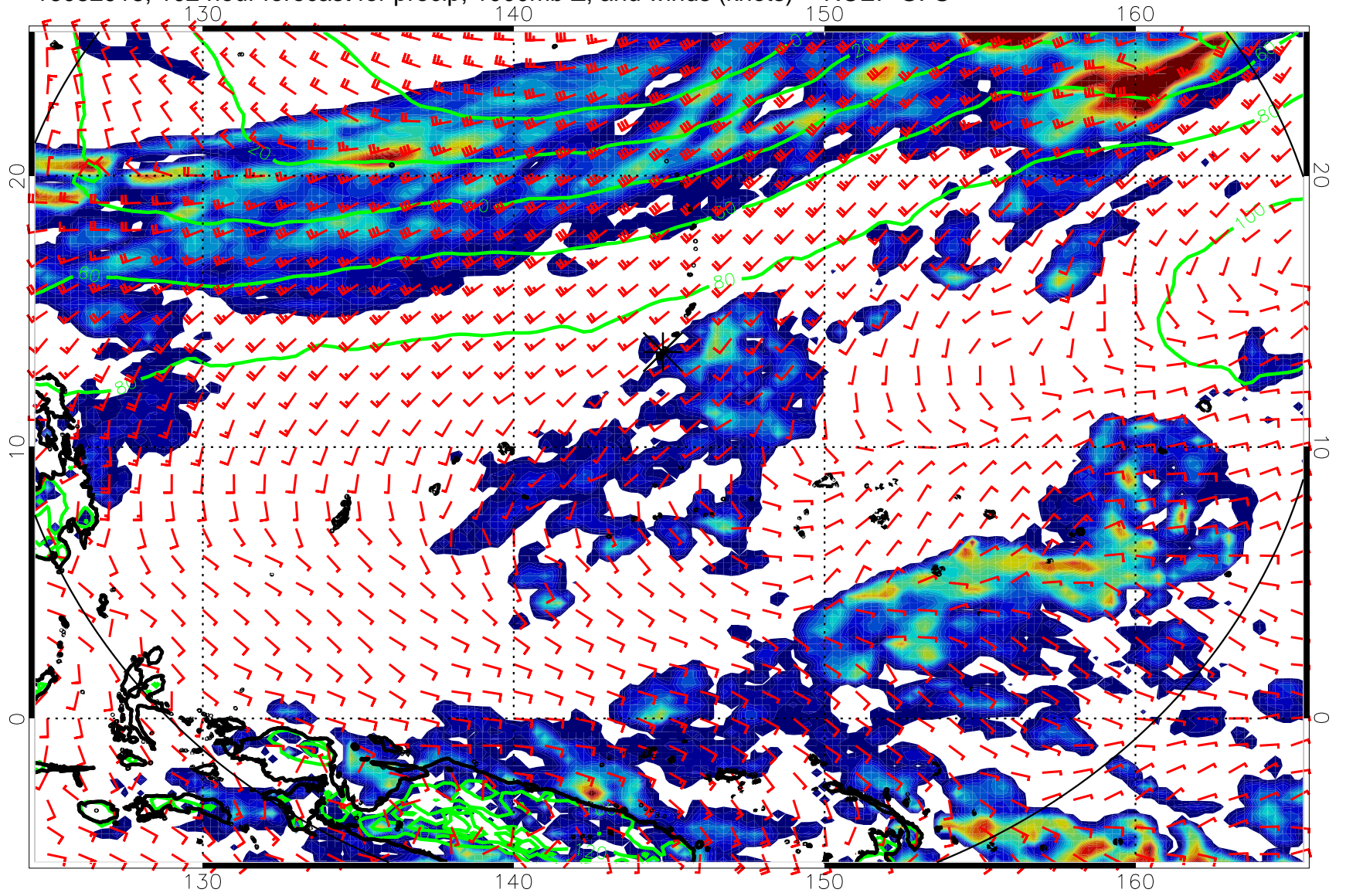
16082918, 102 hour forecast for precip, 1000mb Z, and winds (knots) -- NCEP GFS
