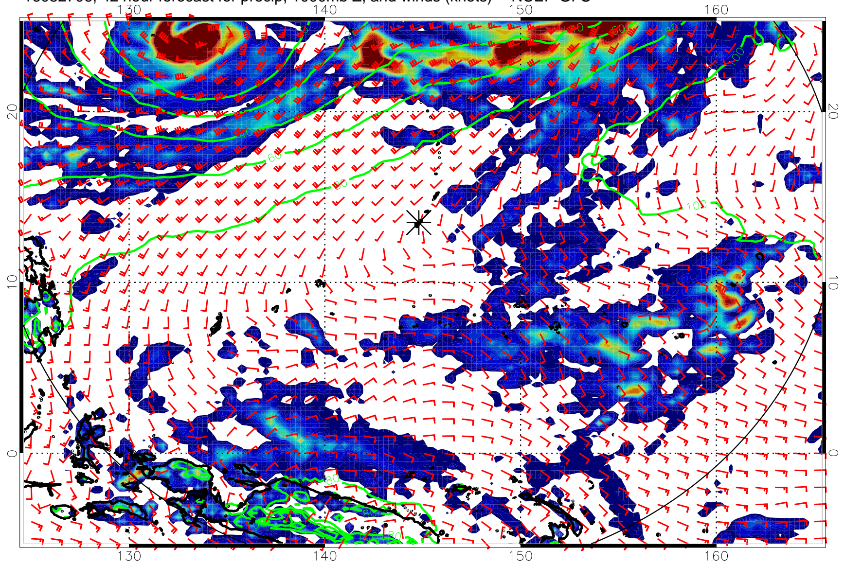
16082706, 42 hour forecast for precip, 1000mb Z, and winds (knots) -- NCEP GFS
