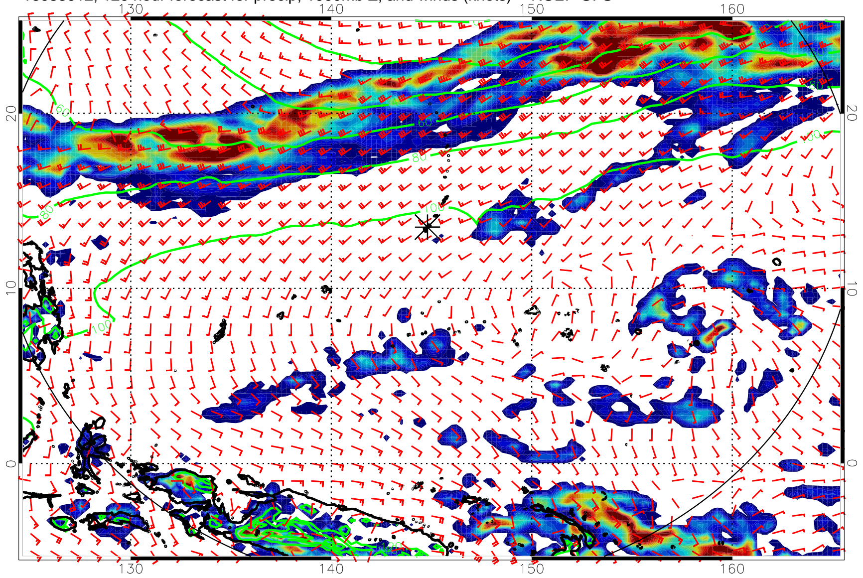
16083012, 120 hour forecast for precip, 1000mb Z, and winds (knots) -- NCEP GFS
