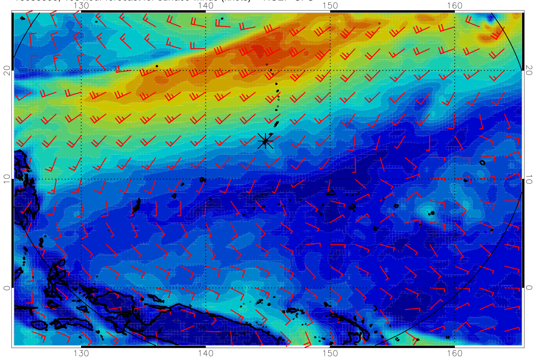
16083000, 108 hour forecast for surface winds (knots) -- NCEP GFS
