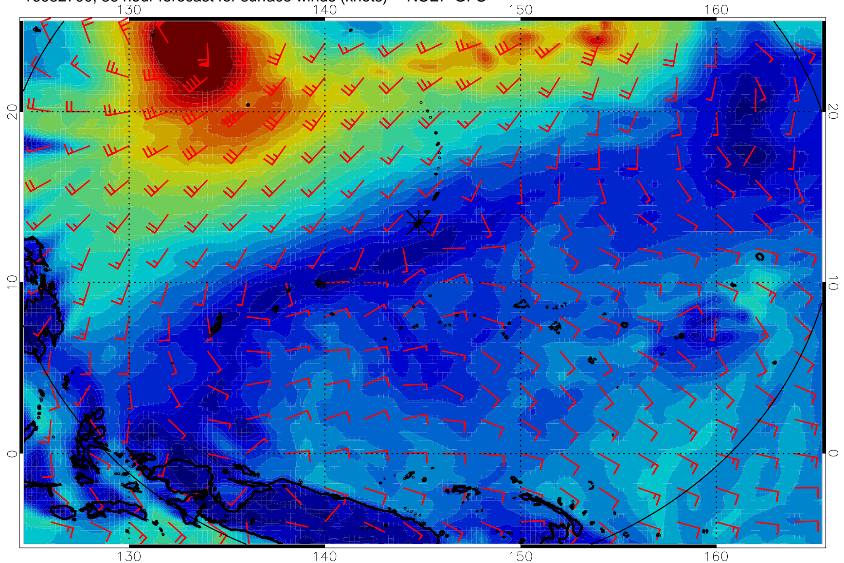
16082700, 36 hour forecast for surface winds (knots) -- NCEP GFS
