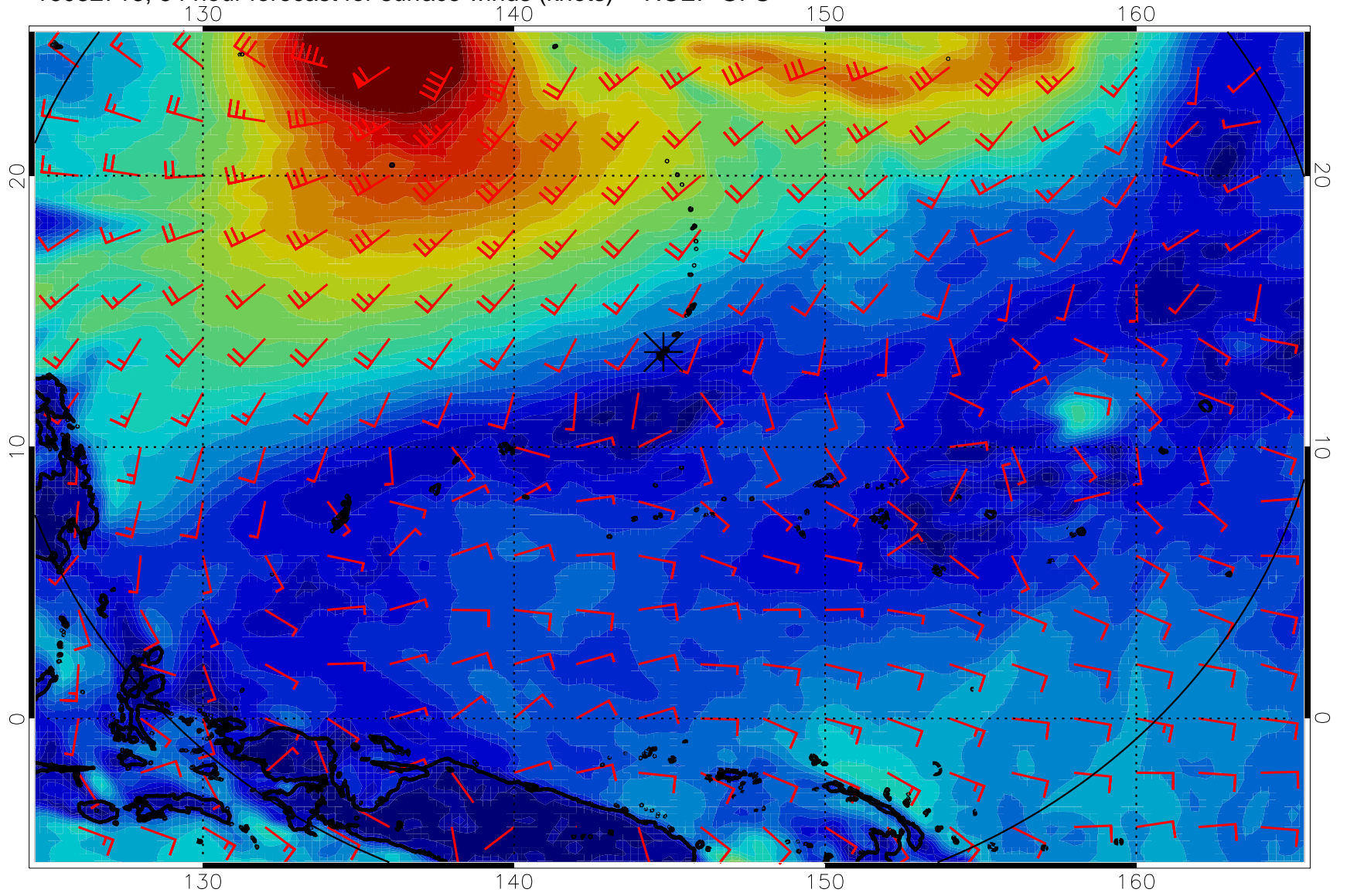
16082718, 54 hour forecast for surface winds (knots) -- NCEP GFS
