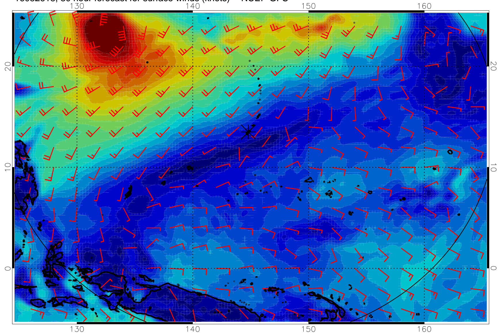
16082618, 30 hour forecast for surface winds (knots) -- NCEP GFS
