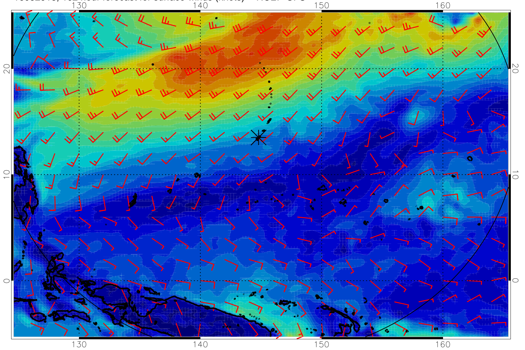
16082918, 102 hour forecast for surface winds (knots) -- NCEP GFS
