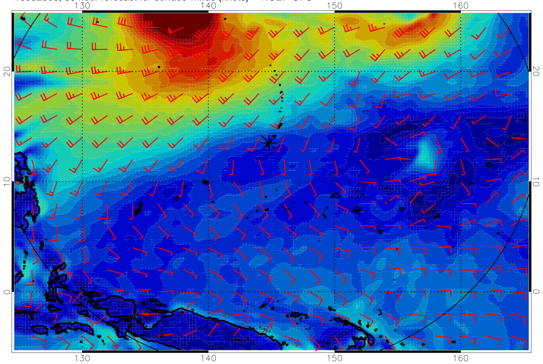
16082806, 66 hour forecast for surface winds (knots) -- NCEP GFS
