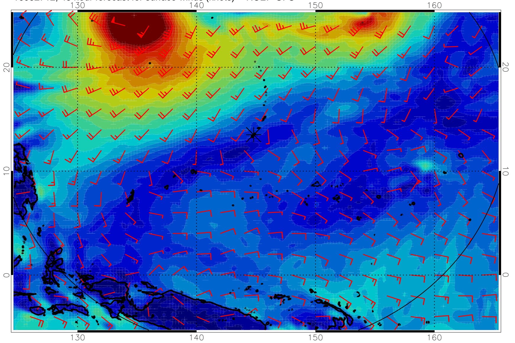
16082712, 48 hour forecast for surface winds (knots) -- NCEP GFS
