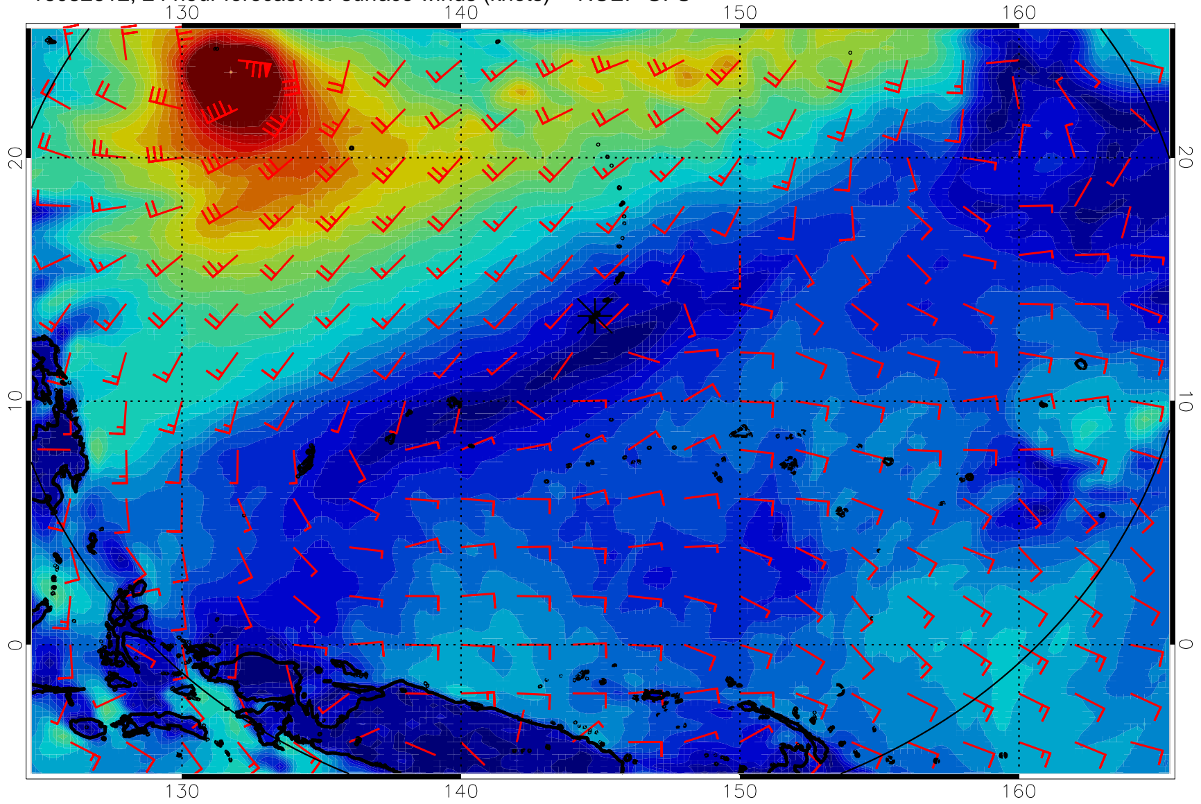
16082612, 24 hour forecast for surface winds (knots) -- NCEP GFS
