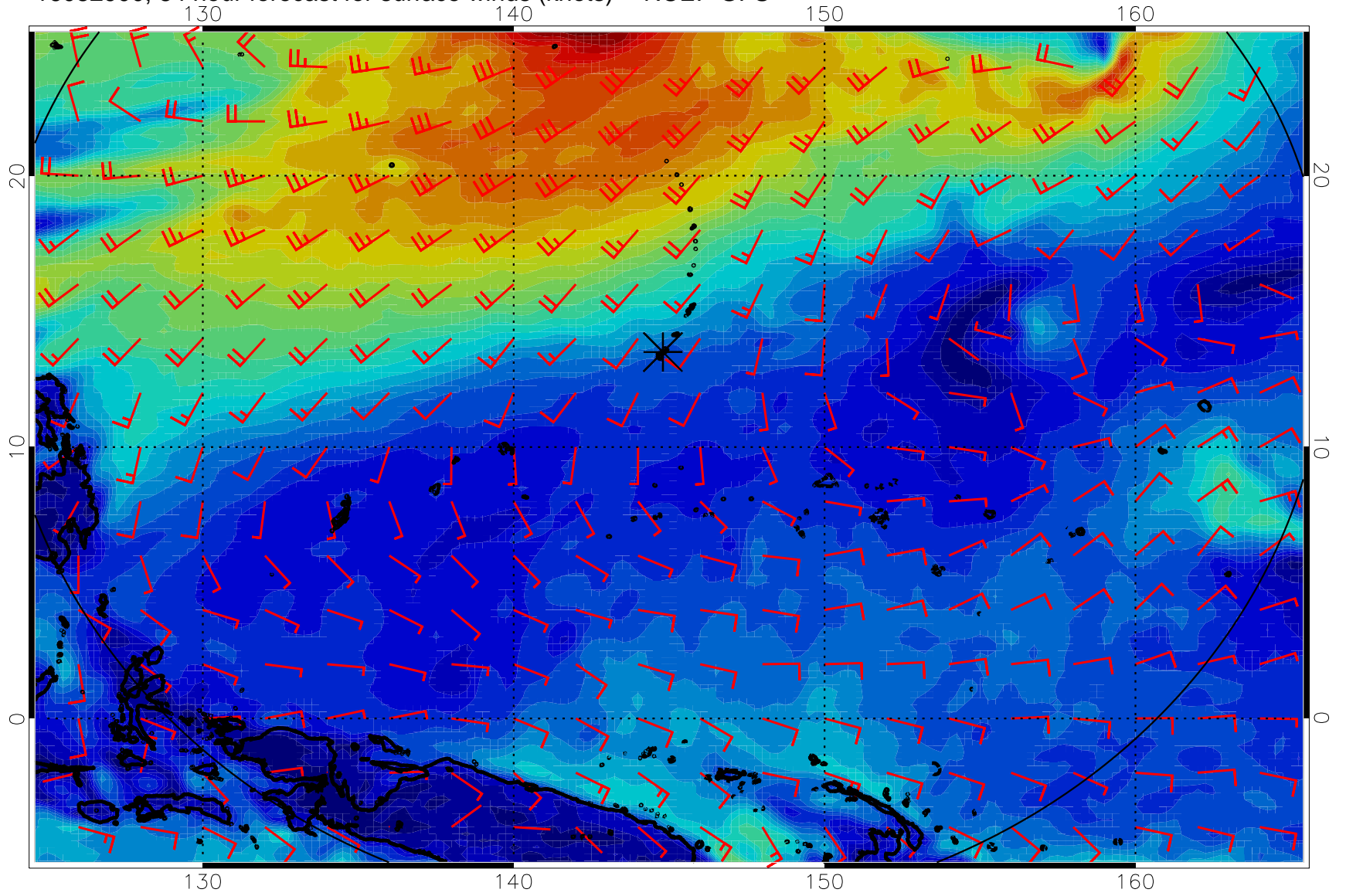
16082900, 84 hour forecast for surface winds (knots) -- NCEP GFS
