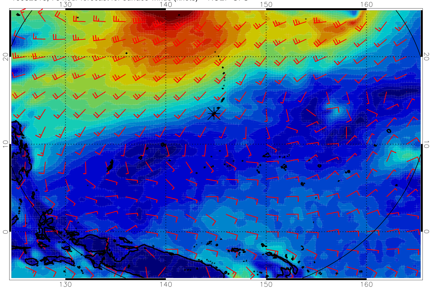
16082818, 78 hour forecast for surface winds (knots) -- NCEP GFS
