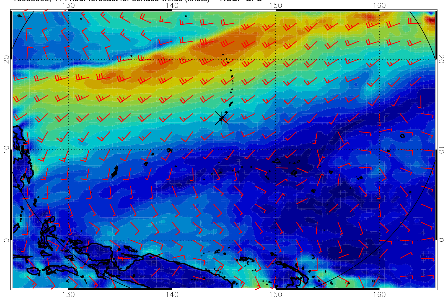
16083006, 114 hour forecast for surface winds (knots) -- NCEP GFS
