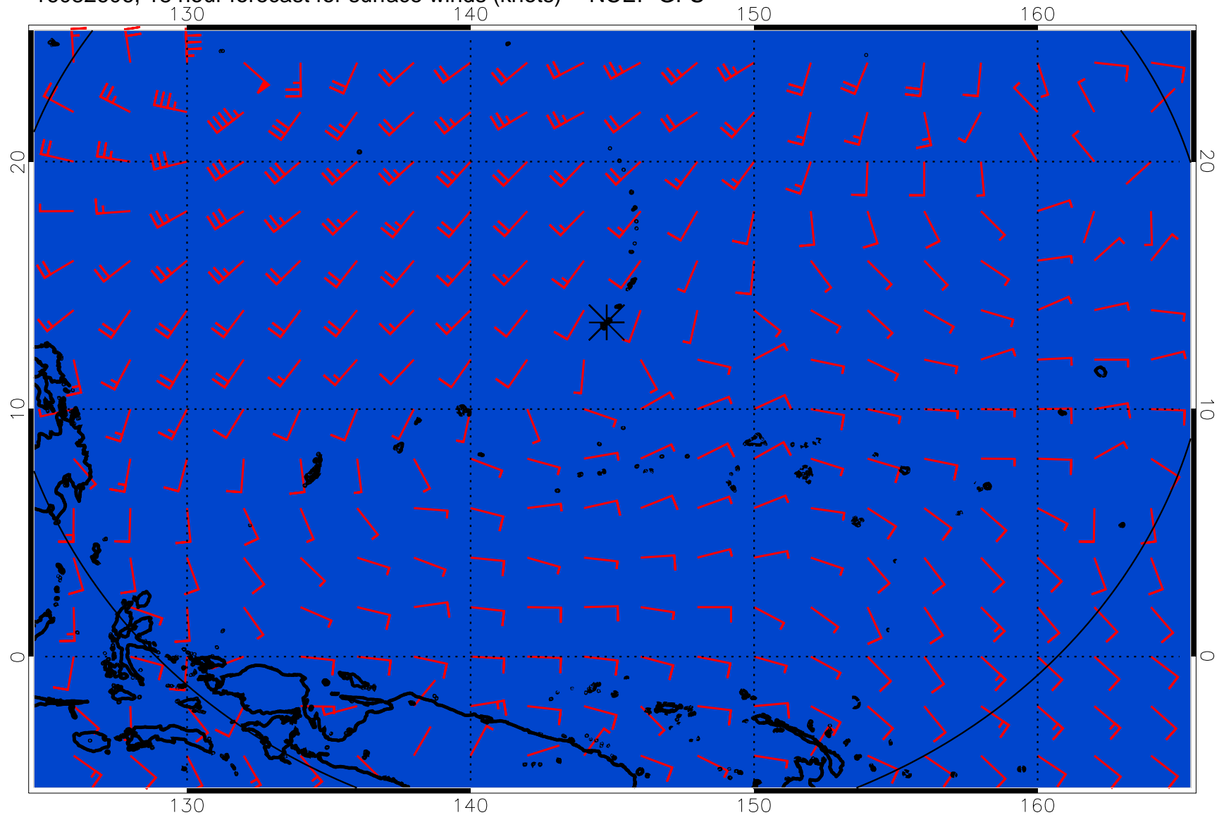
16082606, 18 hour forecast for surface winds (knots) -- NCEP GFS
