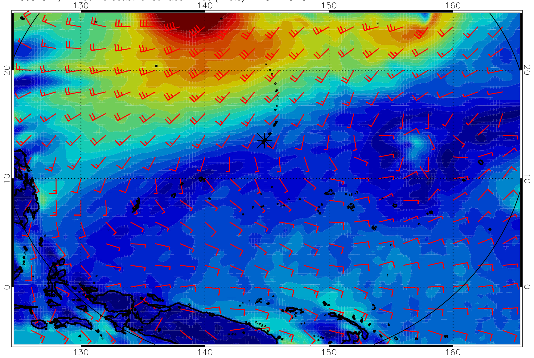
16082812, 72 hour forecast for surface winds (knots) -- NCEP GFS
