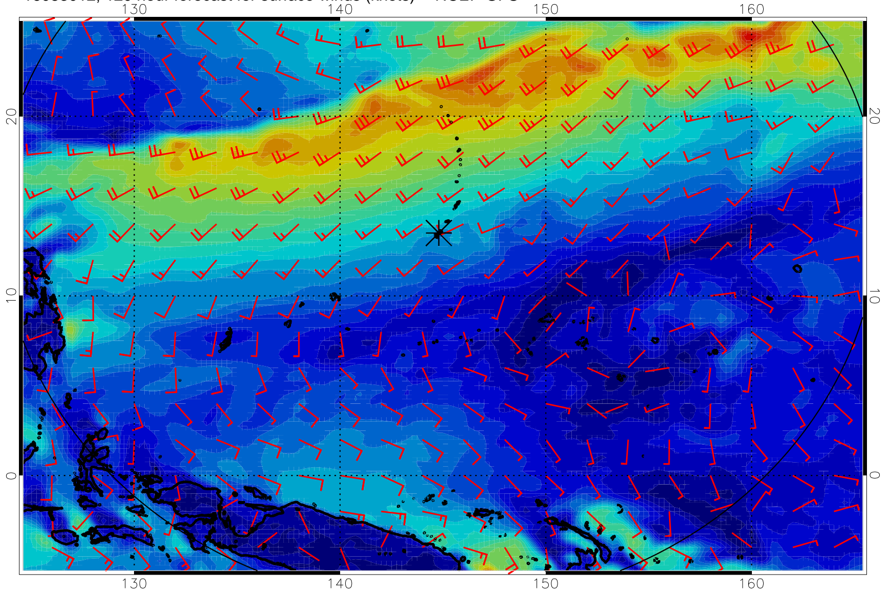
16083012, 120 hour forecast for surface winds (knots) -- NCEP GFS
