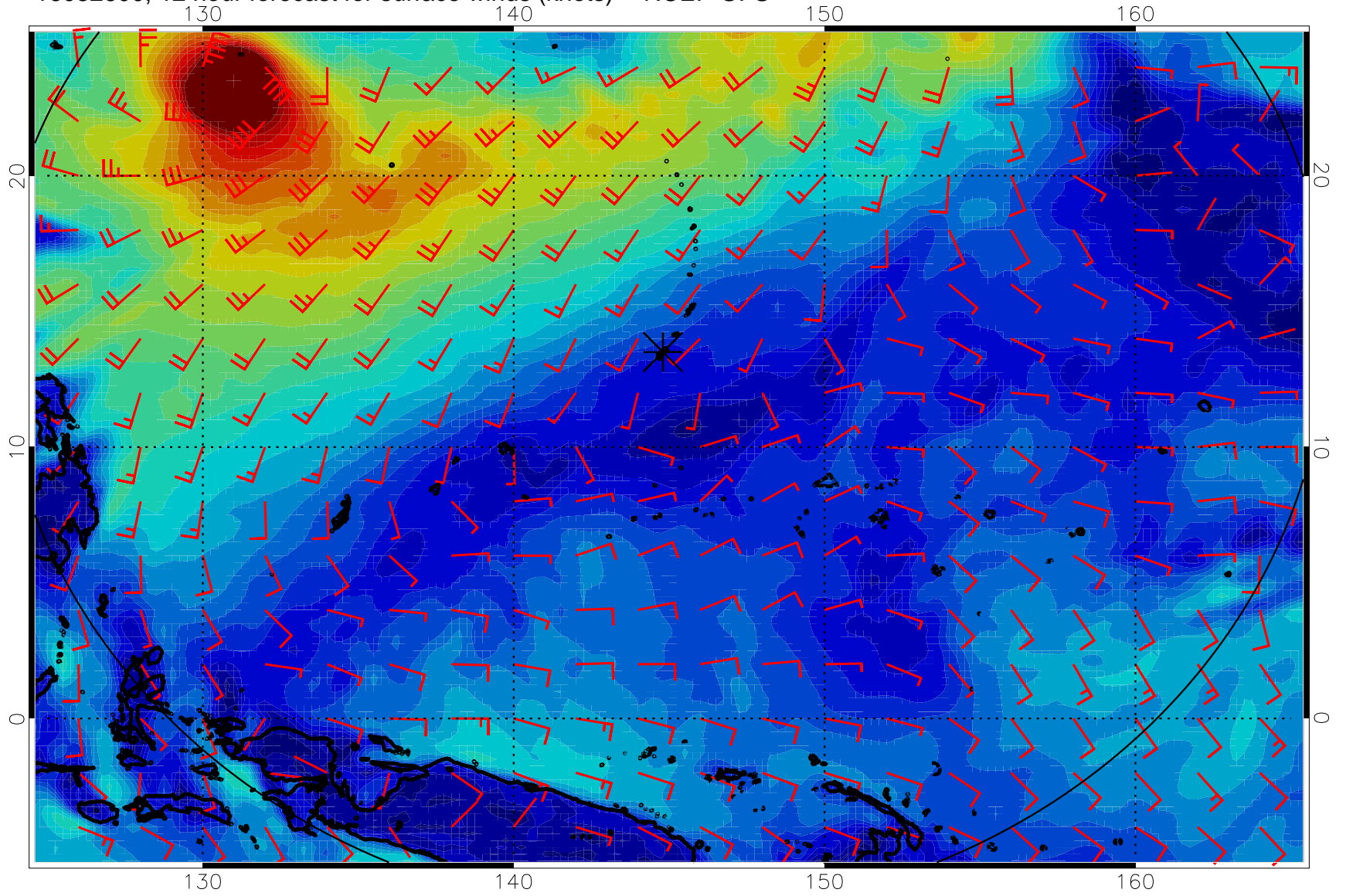
16082600, 12 hour forecast for surface winds (knots) -- NCEP GFS
