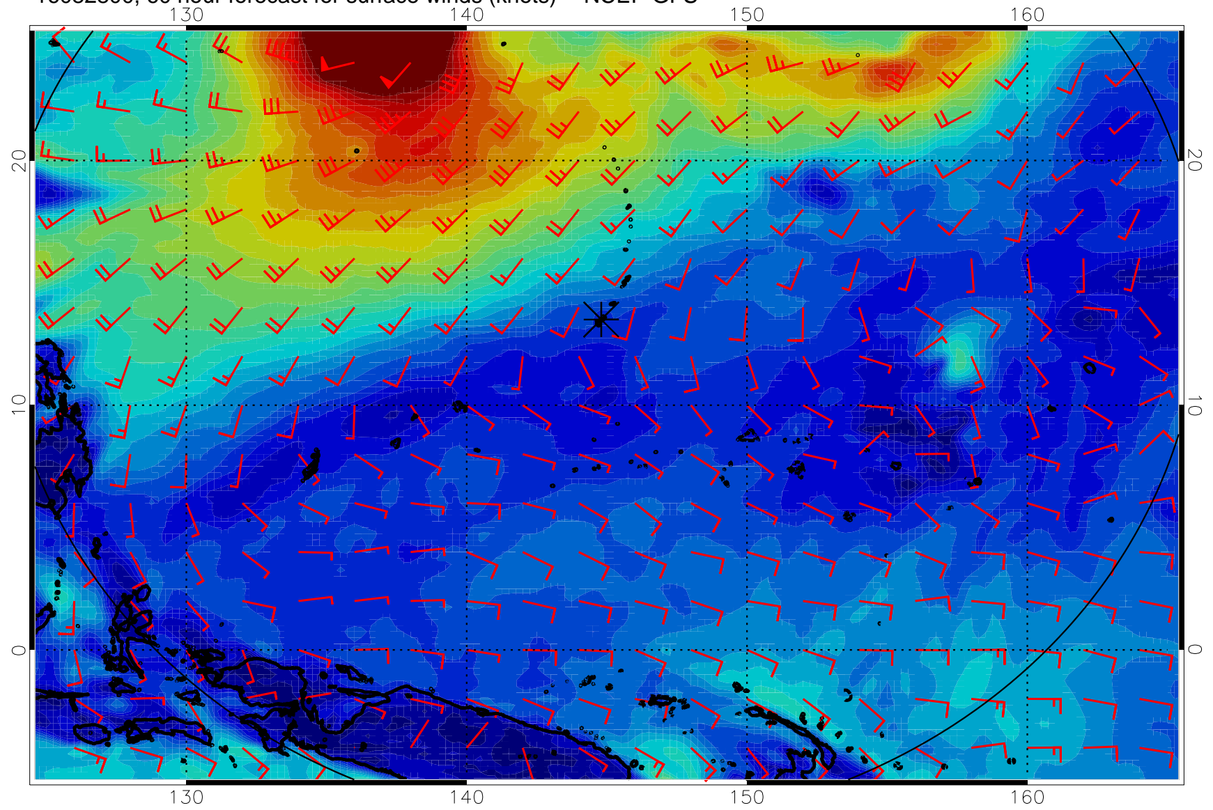
16082800, 60 hour forecast for surface winds (knots) -- NCEP GFS
