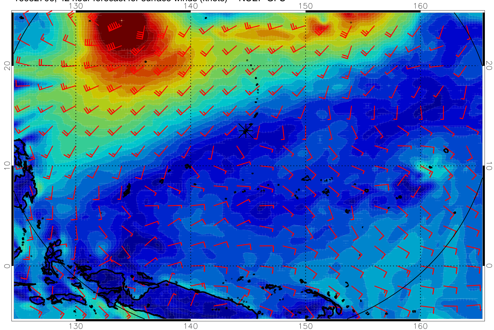
16082706, 42 hour forecast for surface winds (knots) -- NCEP GFS
