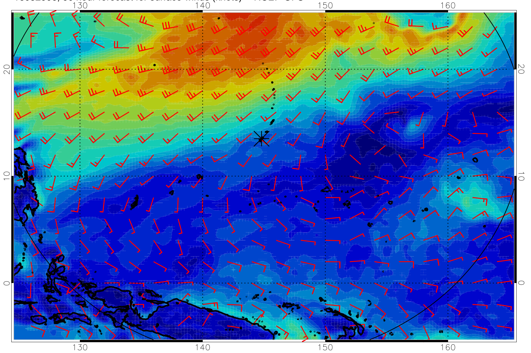
16082906, 90 hour forecast for surface winds (knots) -- NCEP GFS
