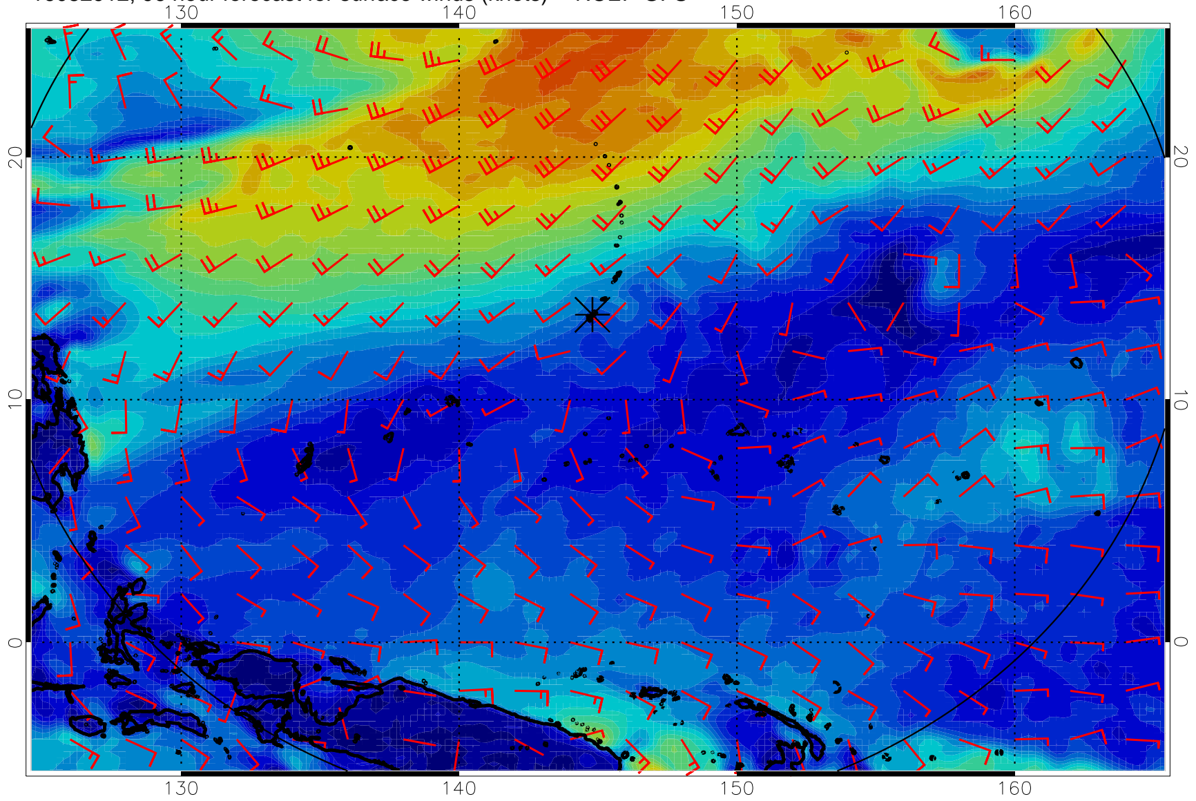
16082912, 96 hour forecast for surface winds (knots) -- NCEP GFS
