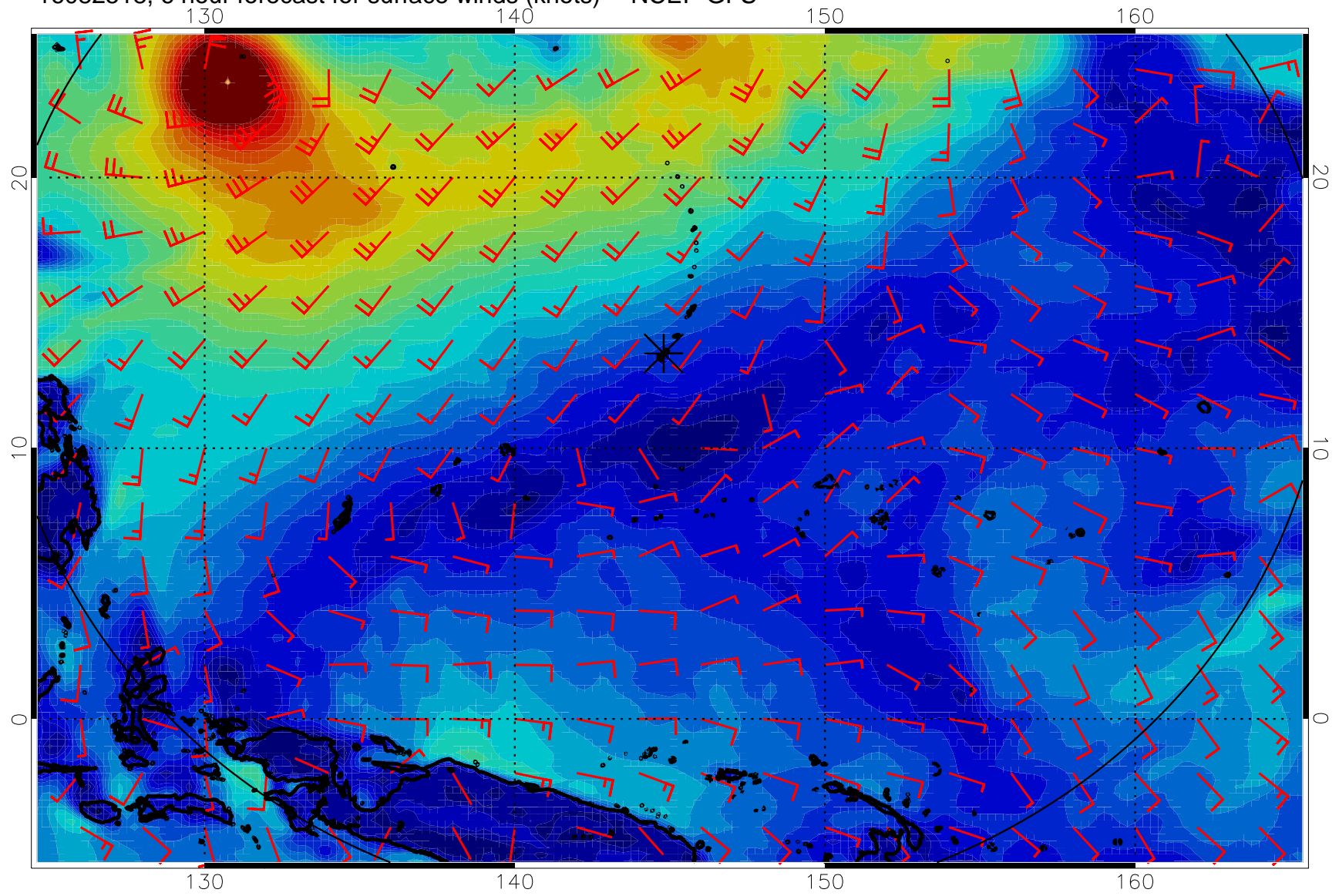
16082518, 6 hour forecast for surface winds (knots) -- NCEP GFS
