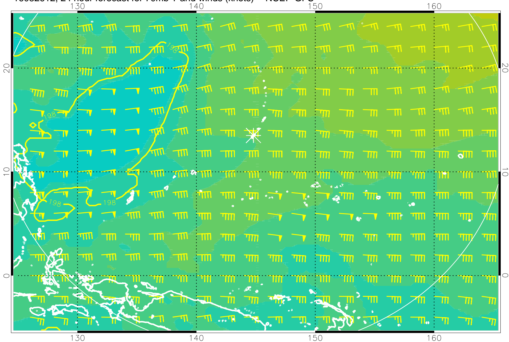
16082612, 24 hour forecast for 70mb T and winds (knots) -- NCEP GFS
