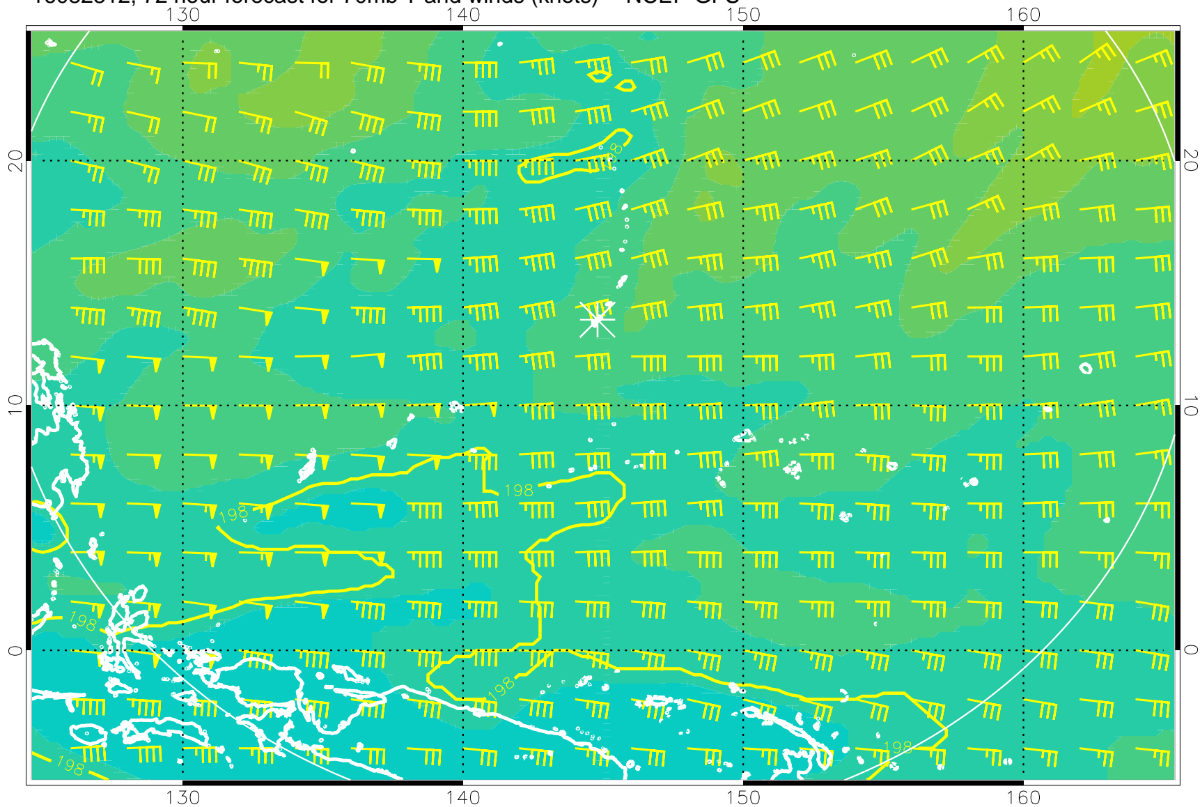
16082812, 72 hour forecast for 70mb T and winds (knots) -- NCEP GFS
