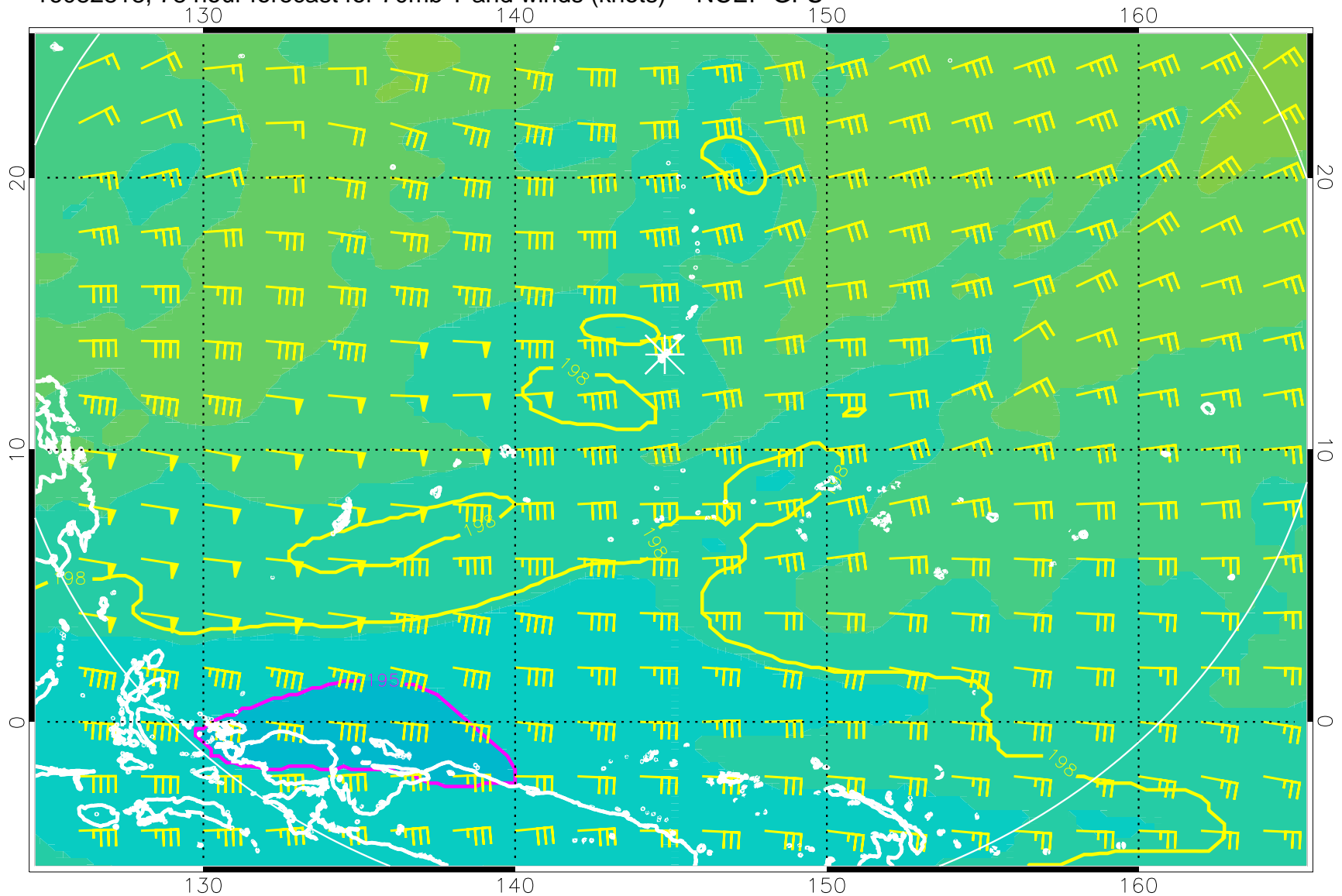
16082818, 78 hour forecast for 70mb T and winds (knots) -- NCEP GFS
