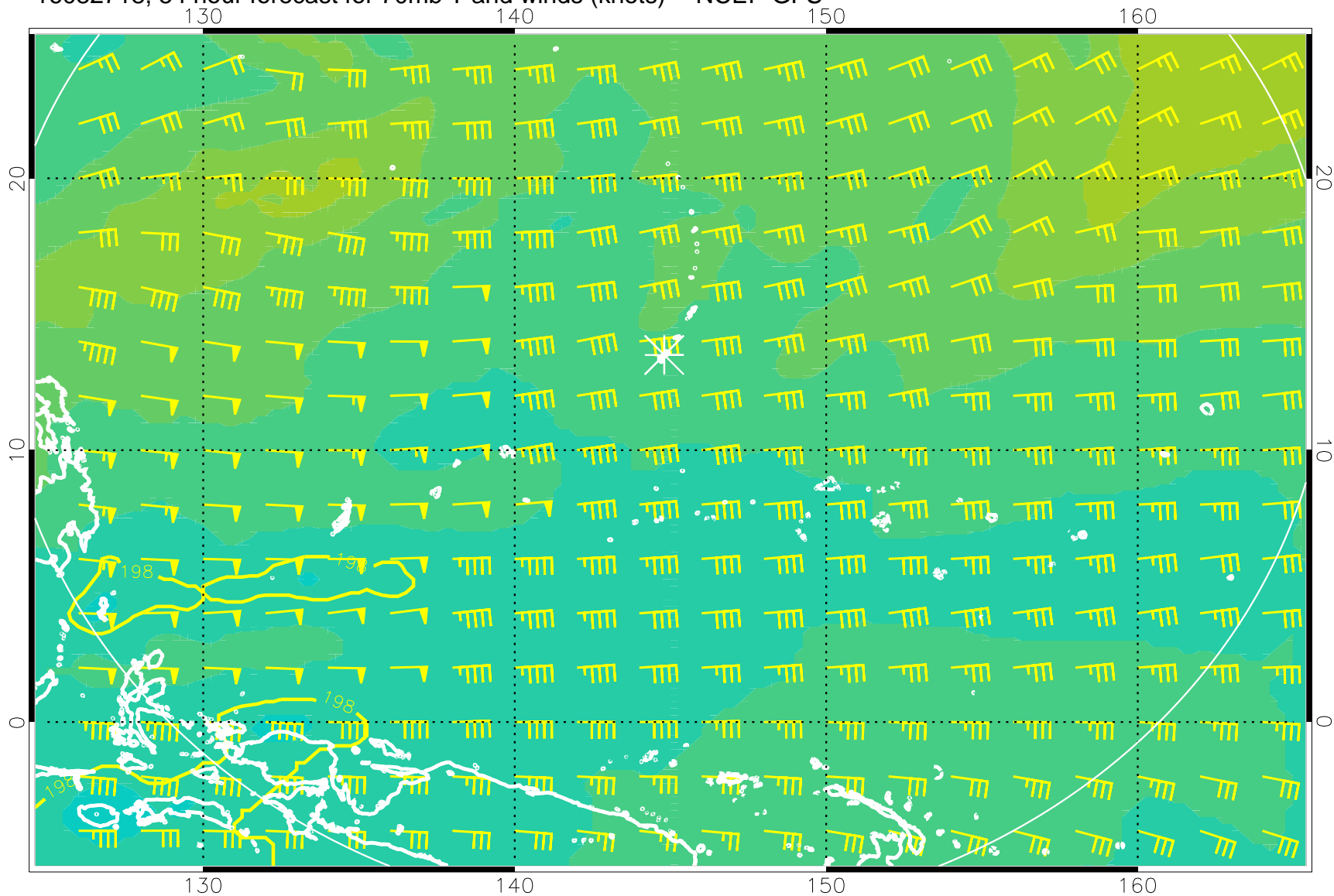
16082718, 54 hour forecast for 70mb T and winds (knots) -- NCEP GFS
