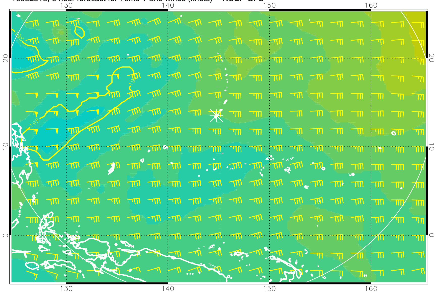
16082518, 6 hour forecast for 70mb T and winds (knots) -- NCEP GFS
