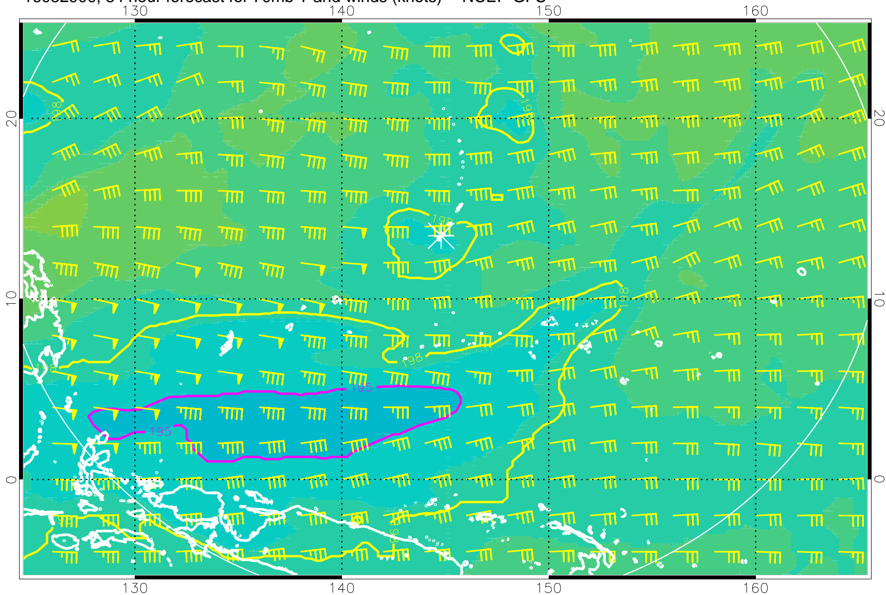
16082900, 84 hour forecast for 70mb T and winds (knots) -- NCEP GFS
