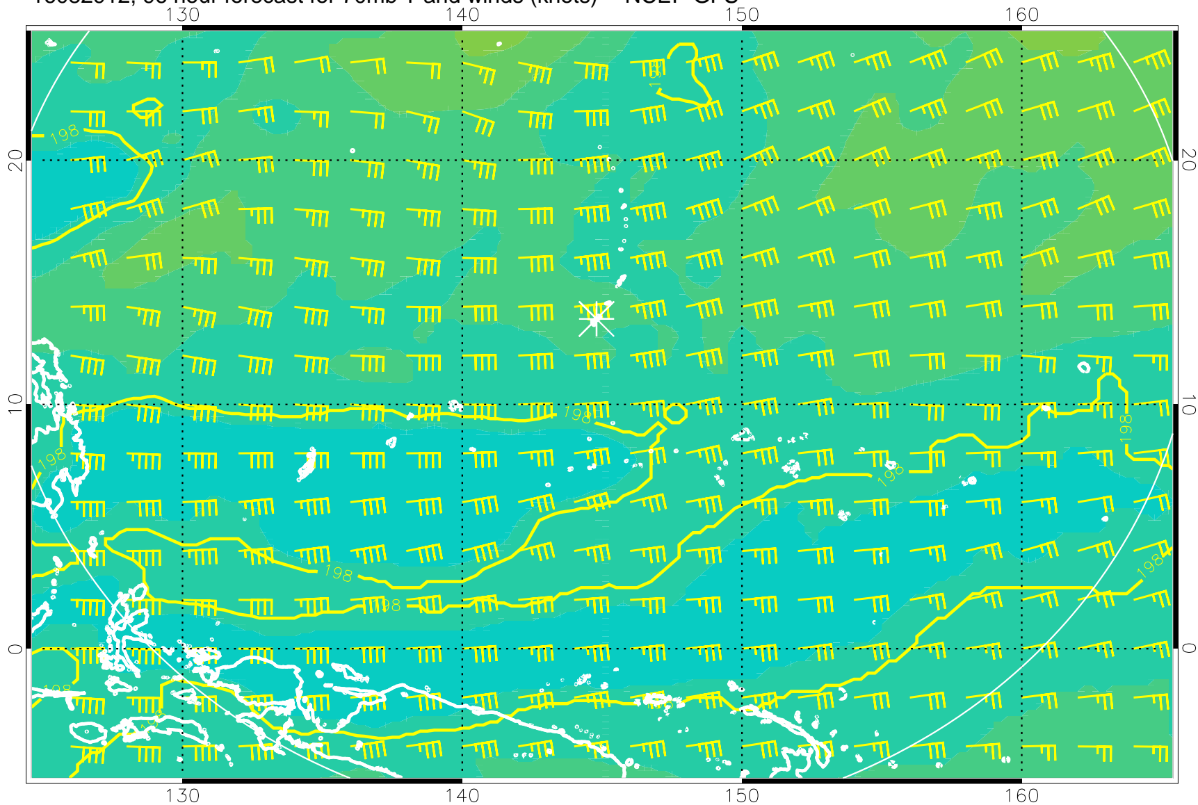
16082912, 96 hour forecast for 70mb T and winds (knots) -- NCEP GFS
