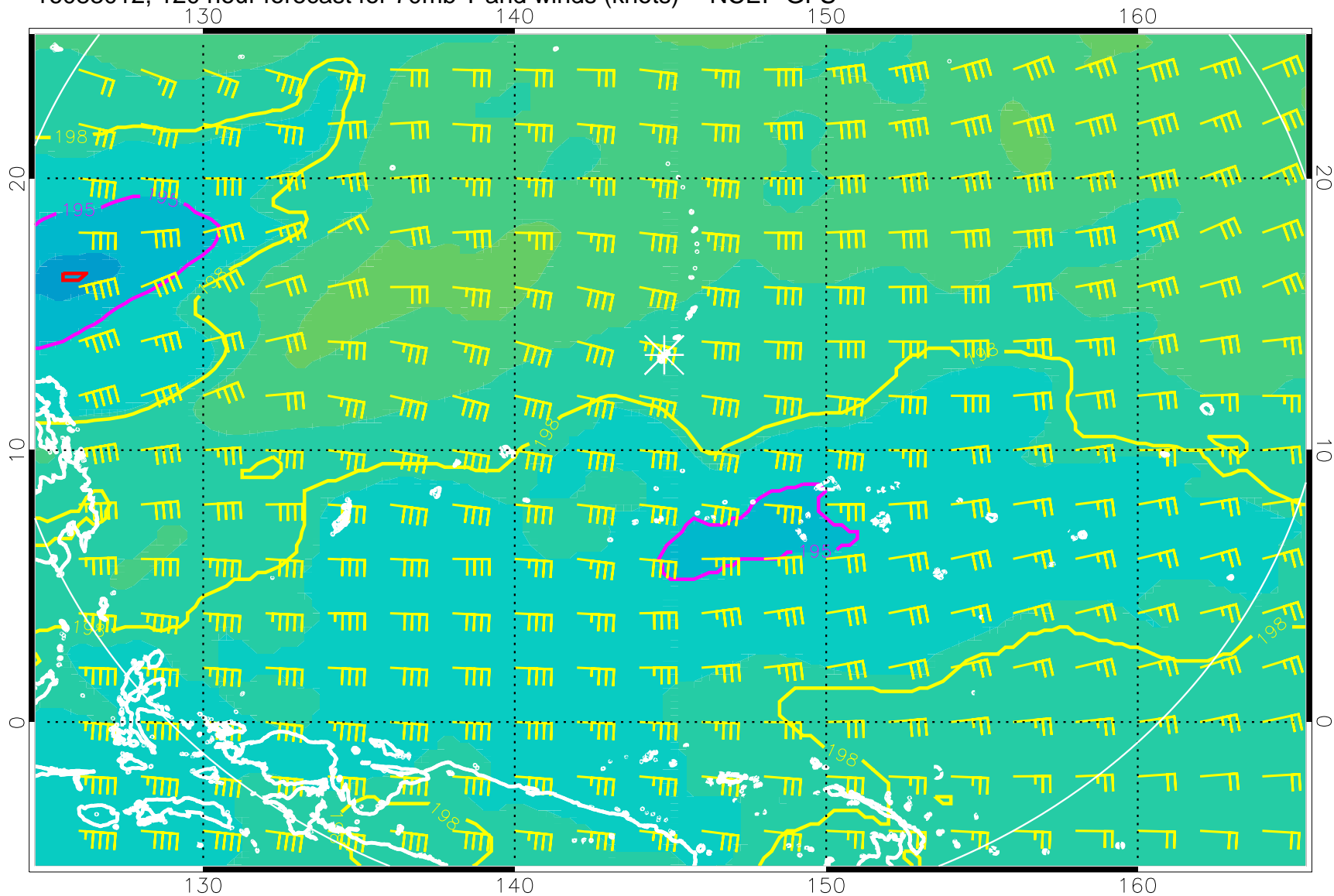
16083012, 120 hour forecast for 70mb T and winds (knots) -- NCEP GFS
