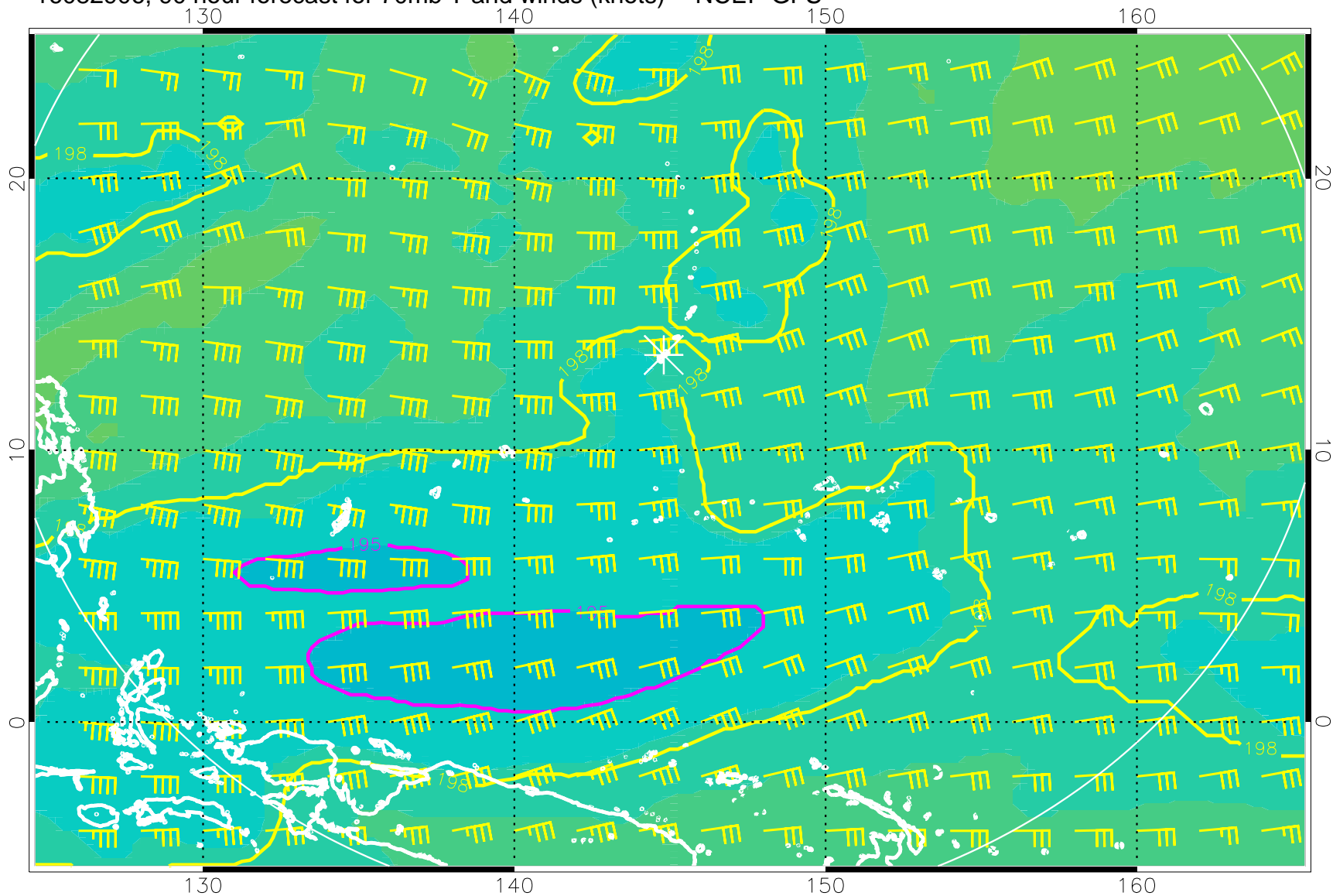
16082906, 90 hour forecast for 70mb T and winds (knots) -- NCEP GFS
