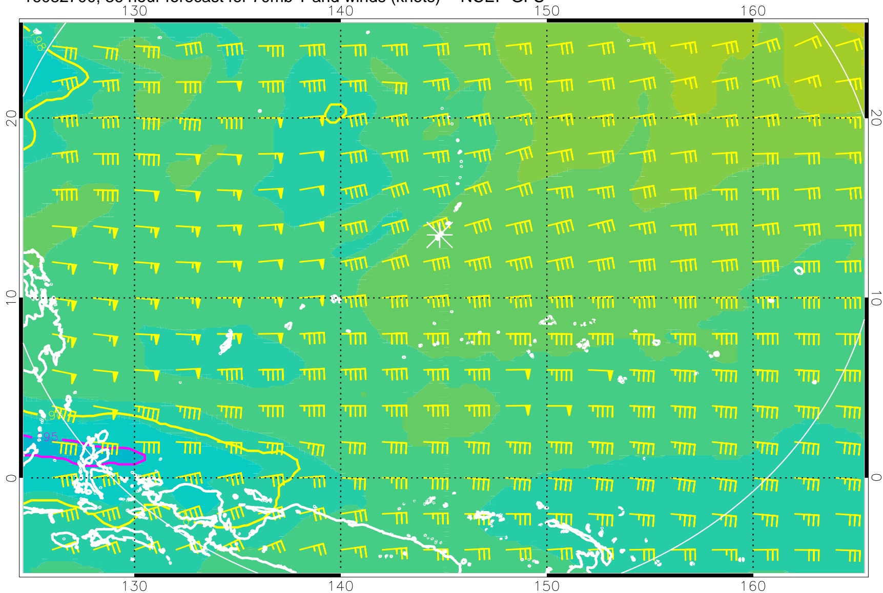
16082700, 36 hour forecast for 70mb T and winds (knots) -- NCEP GFS
