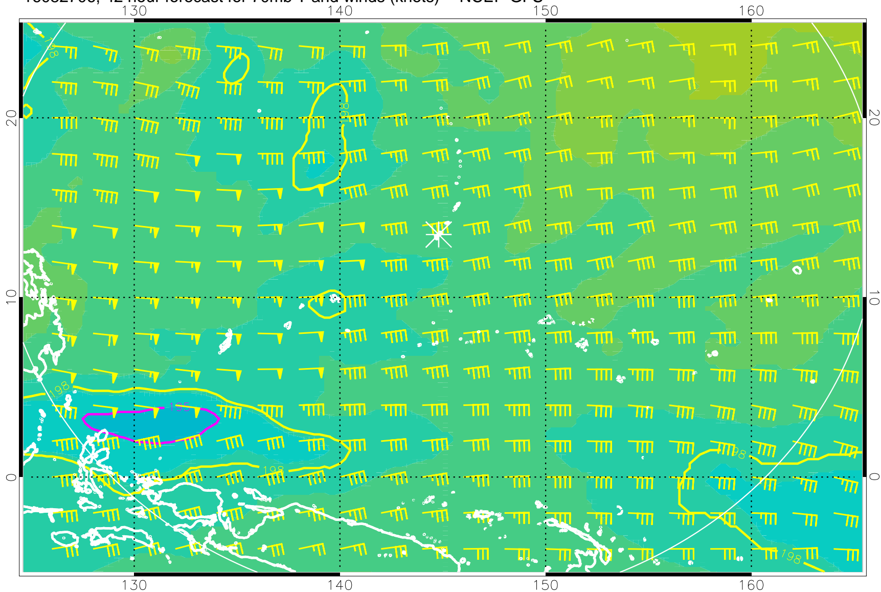
16082706, 42 hour forecast for 70mb T and winds (knots) -- NCEP GFS
