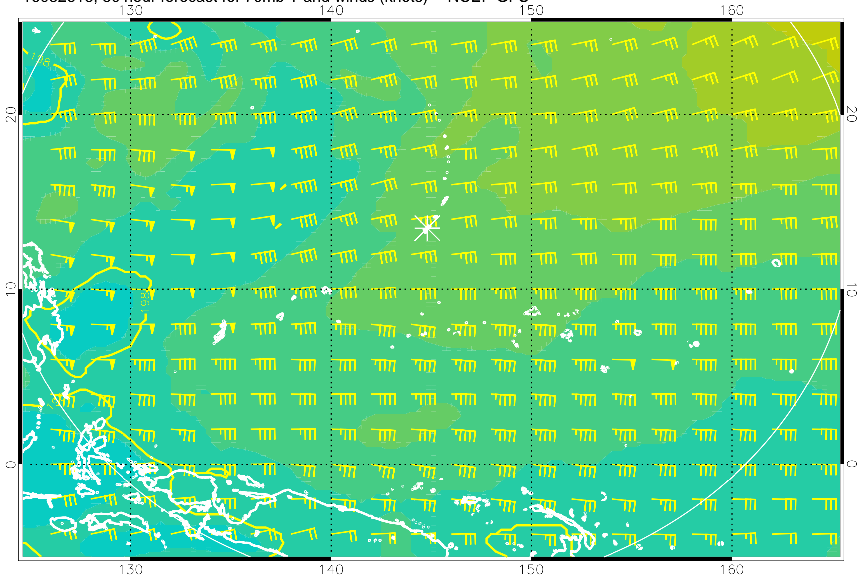
16082618, 30 hour forecast for 70mb T and winds (knots) -- NCEP GFS
