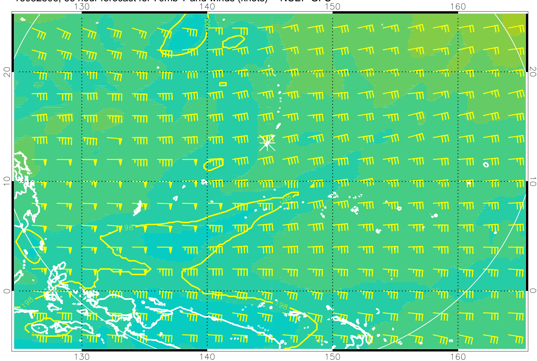
16082806, 66 hour forecast for 70mb T and winds (knots) -- NCEP GFS
