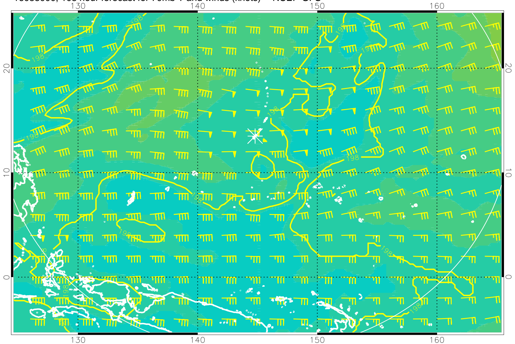
16083000, 108 hour forecast for 70mb T and winds (knots) -- NCEP GFS
