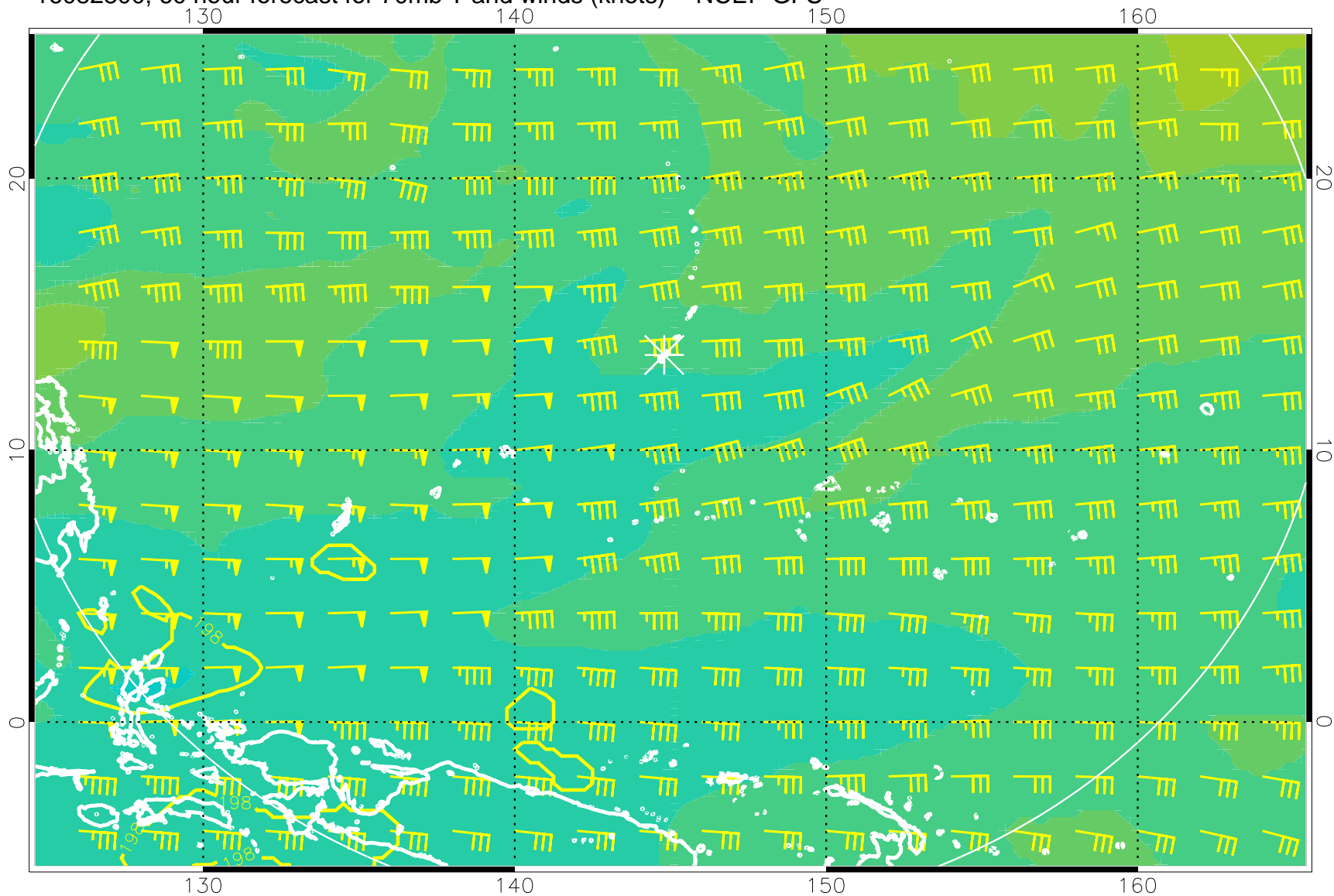
16082800, 60 hour forecast for 70mb T and winds (knots) -- NCEP GFS
