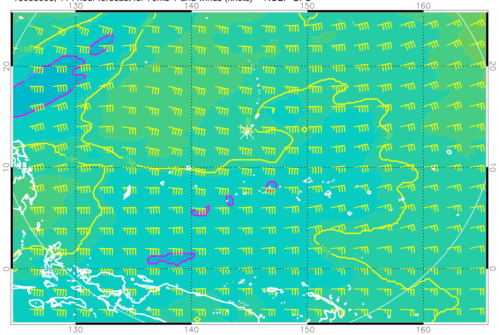
16083006, 114 hour forecast for 70mb T and winds (knots) -- NCEP GFS
