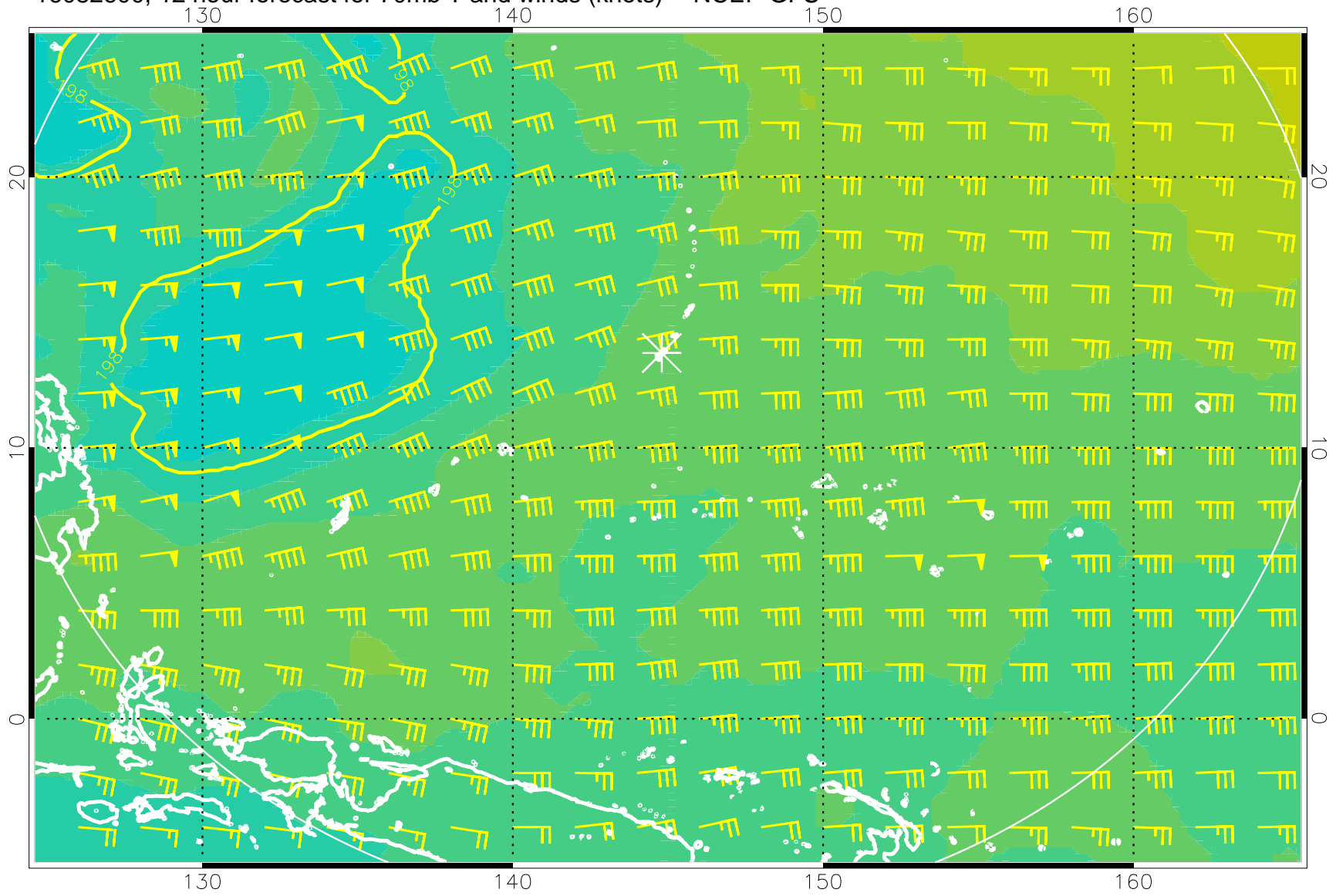
16082600, 12 hour forecast for 70mb T and winds (knots) -- NCEP GFS
