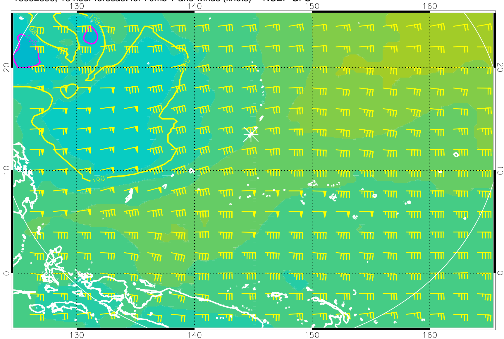
16082606, 18 hour forecast for 70mb T and winds (knots) -- NCEP GFS
