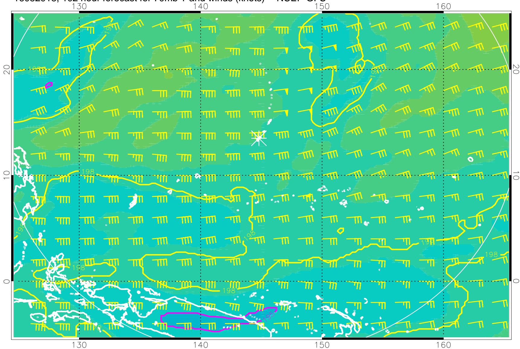
16082918, 102 hour forecast for 70mb T and winds (knots) -- NCEP GFS
