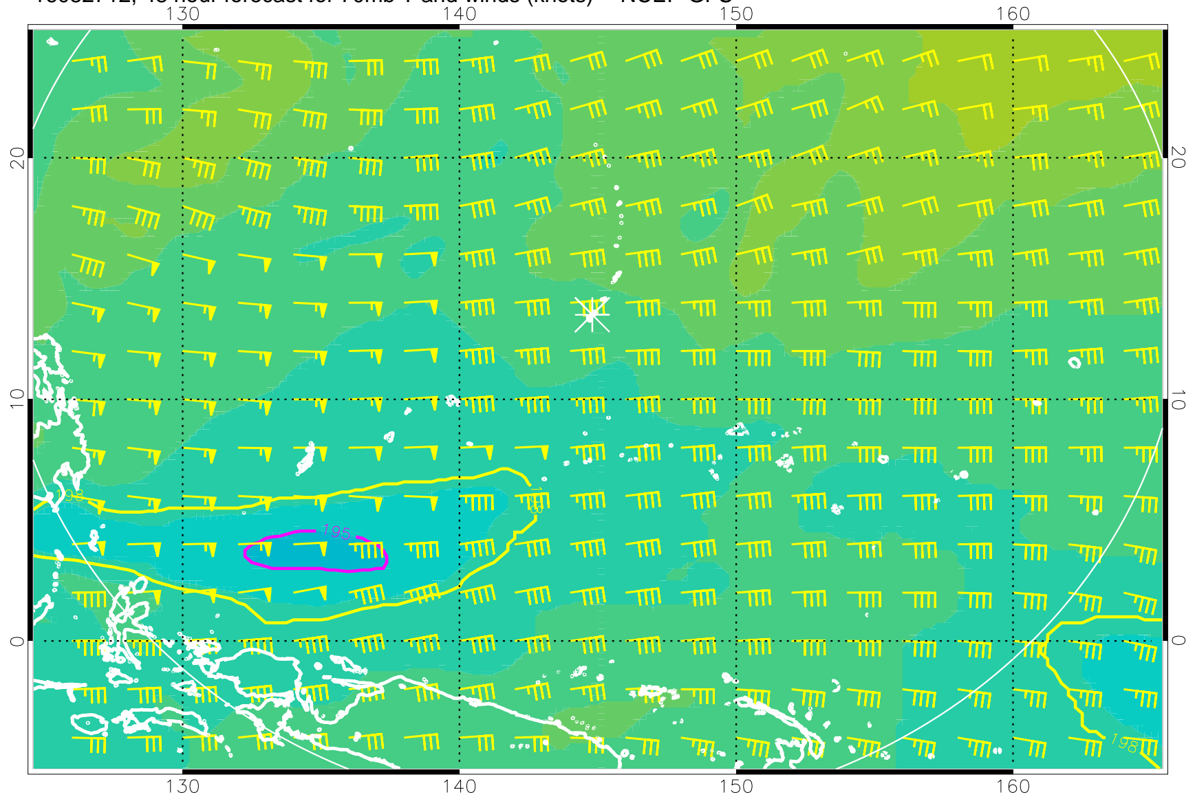
16082712, 48 hour forecast for 70mb T and winds (knots) -- NCEP GFS
