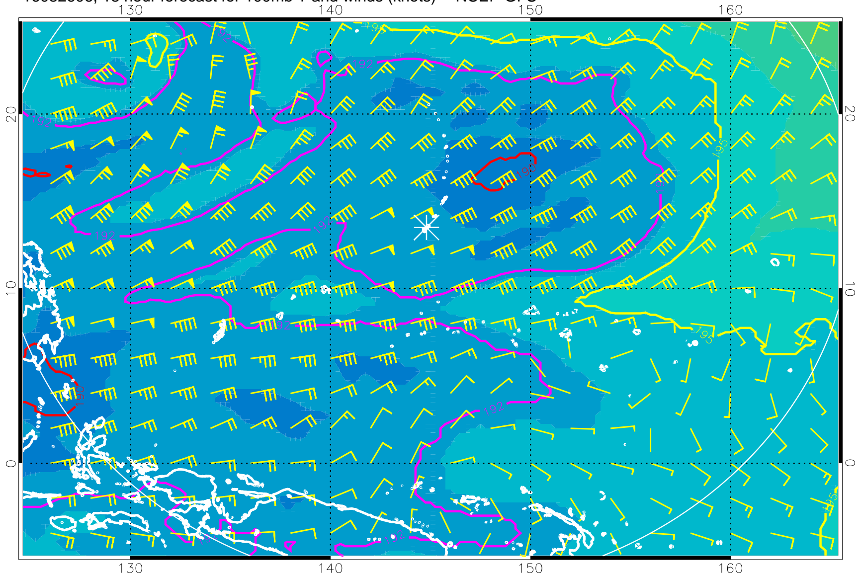
16082606, 18 hour forecast for 100mb T and winds (knots) -- NCEP GFS
