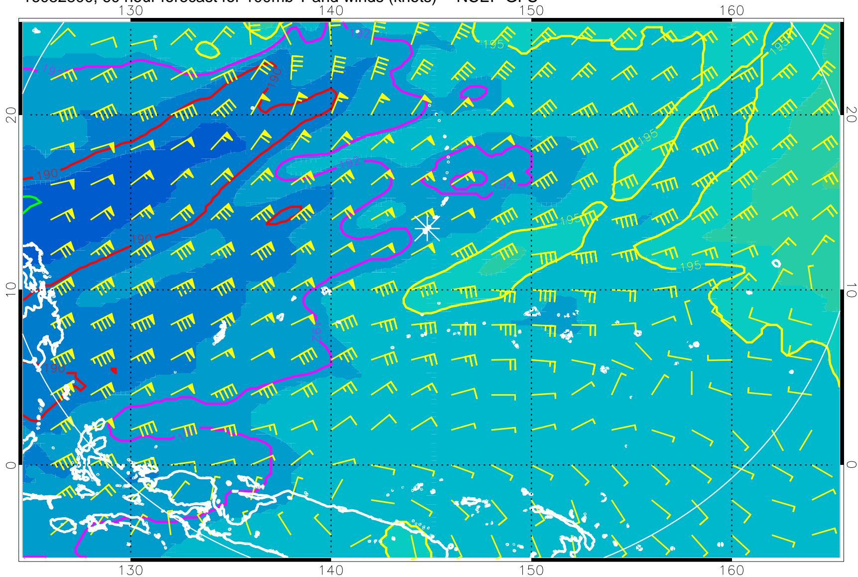
16082800, 60 hour forecast for 100mb T and winds (knots) -- NCEP GFS
