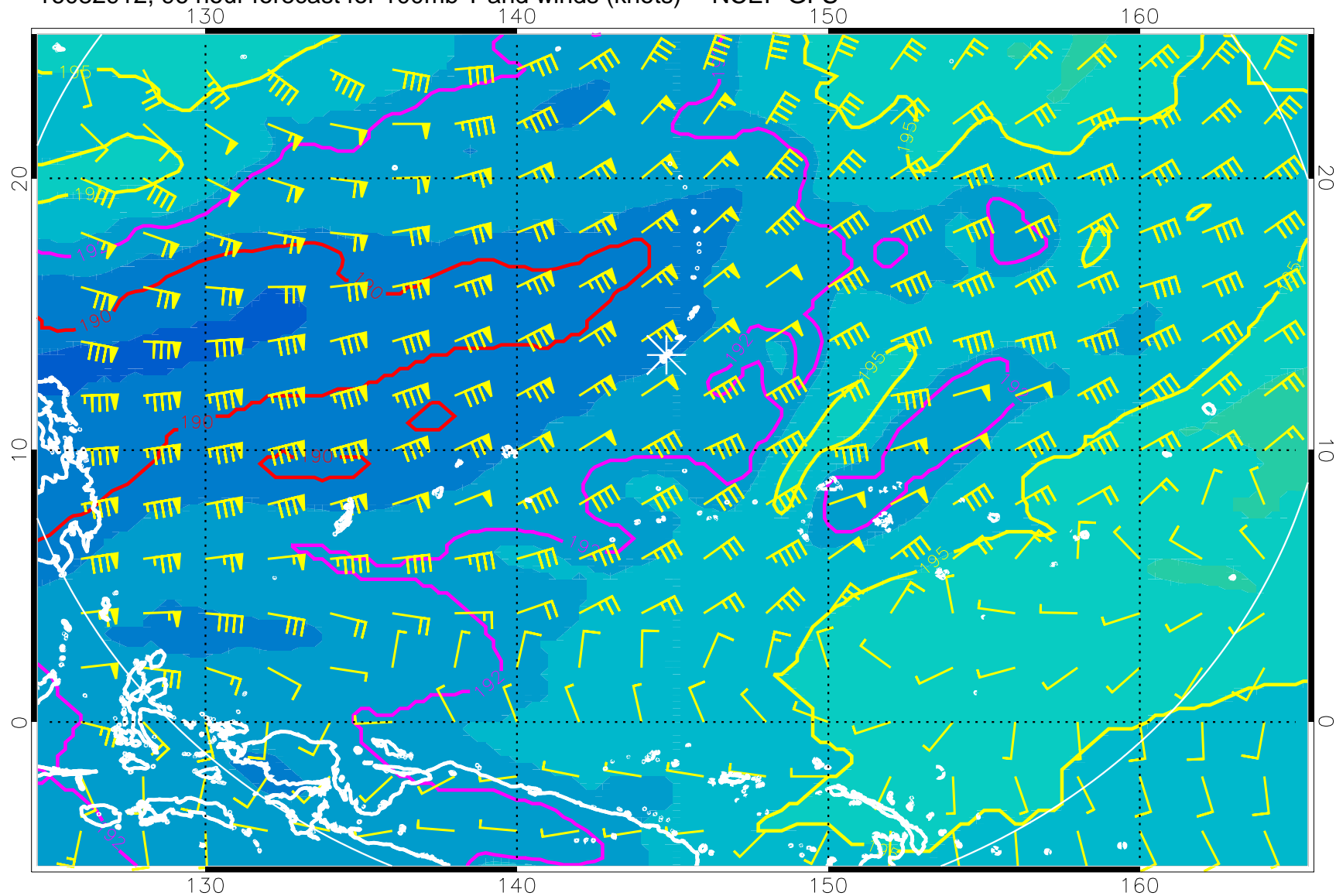
16082912, 96 hour forecast for 100mb T and winds (knots) -- NCEP GFS
