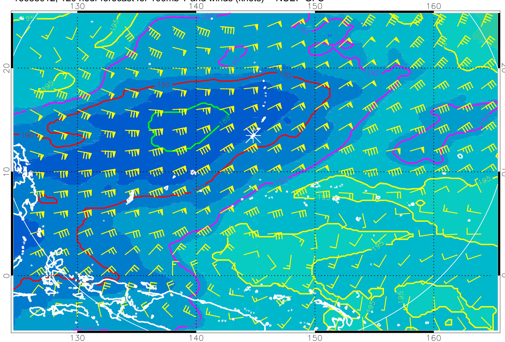
16083012, 120 hour forecast for 100mb T and winds (knots) -- NCEP GFS
