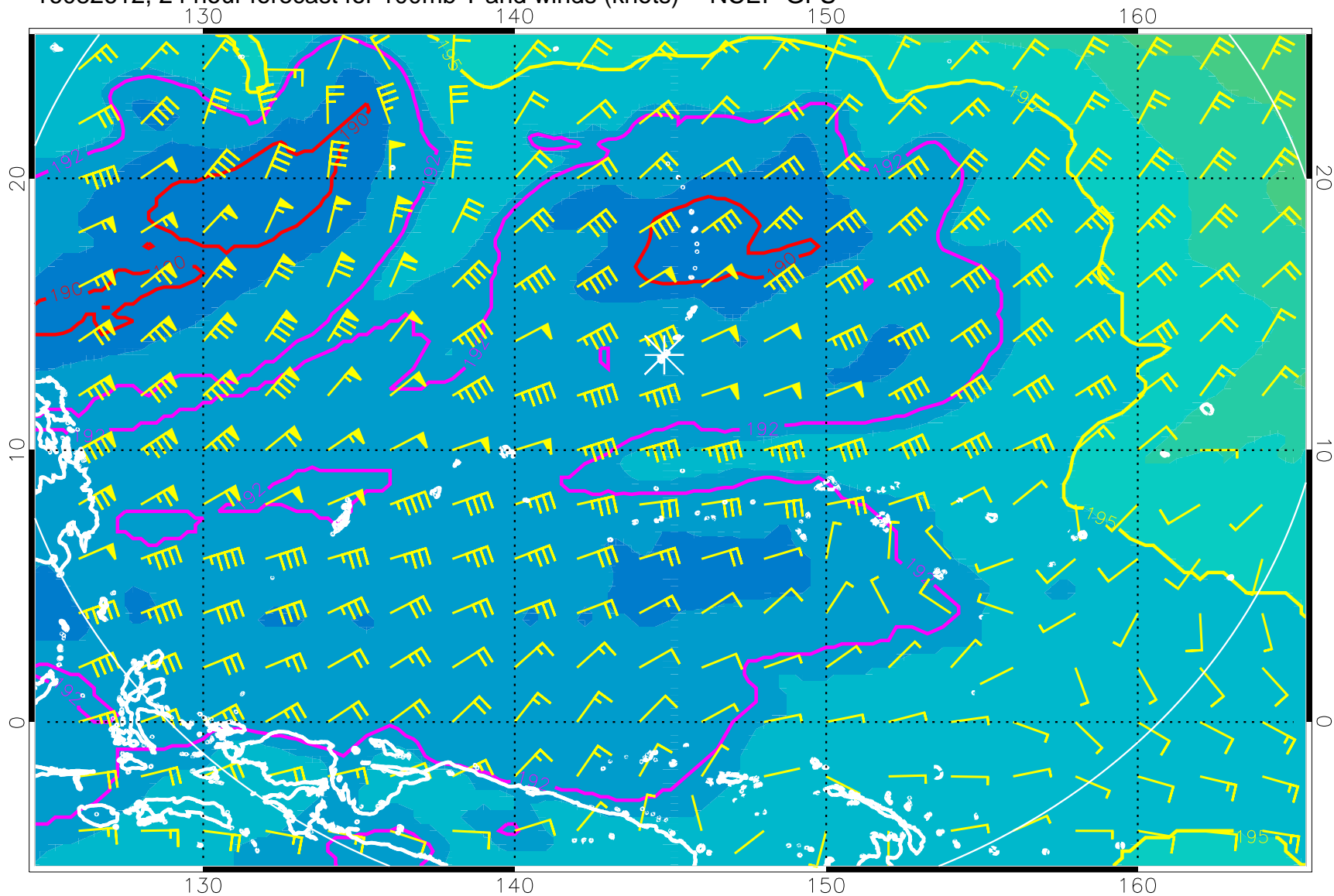
16082612, 24 hour forecast for 100mb T and winds (knots) -- NCEP GFS
