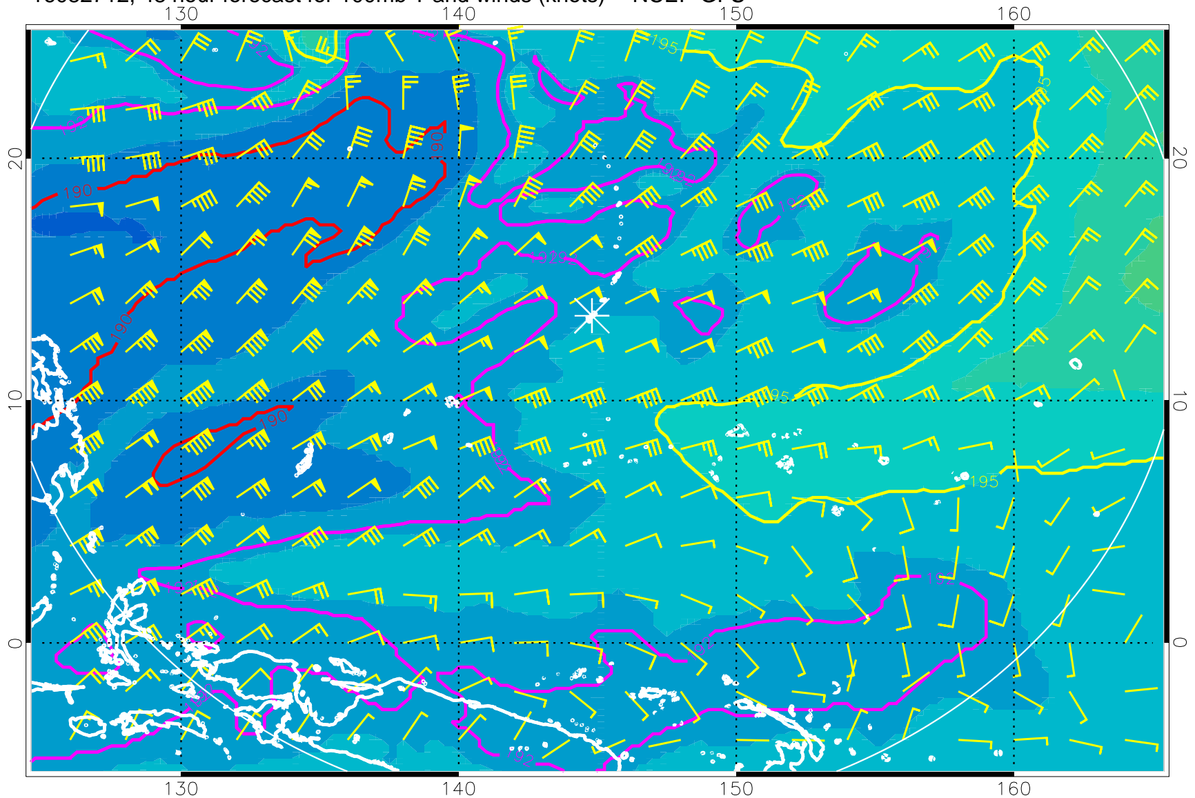
16082712, 48 hour forecast for 100mb T and winds (knots) -- NCEP GFS
