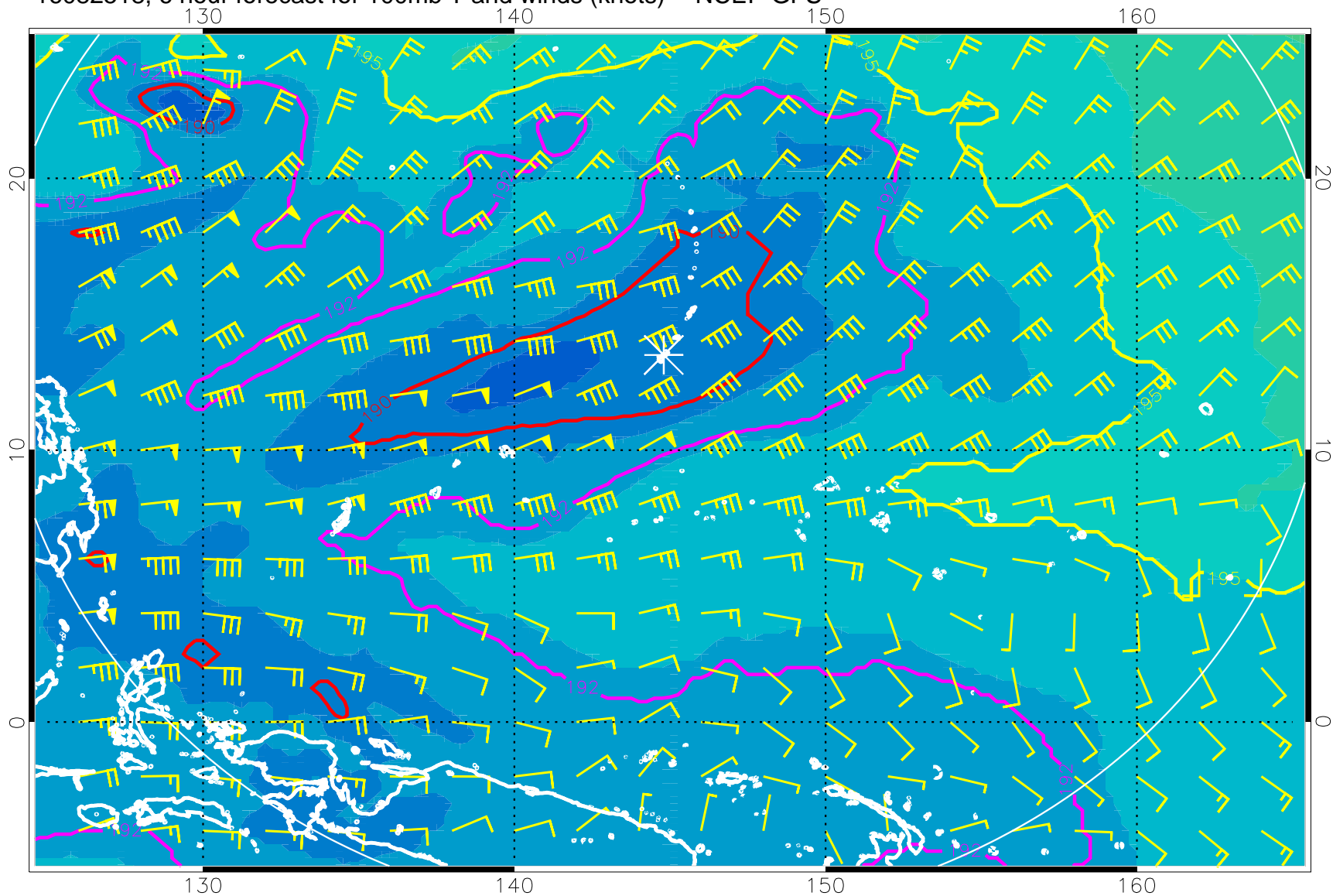
16082518, 6 hour forecast for 100mb T and winds (knots) -- NCEP GFS
