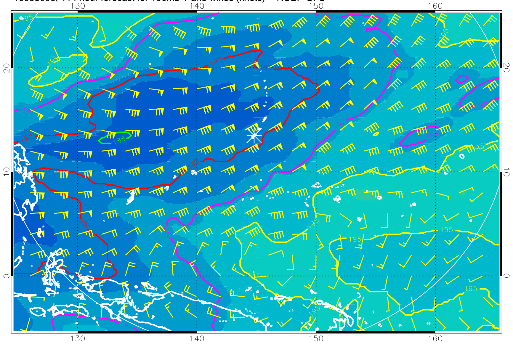
16083006, 114 hour forecast for 100mb T and winds (knots) -- NCEP GFS
