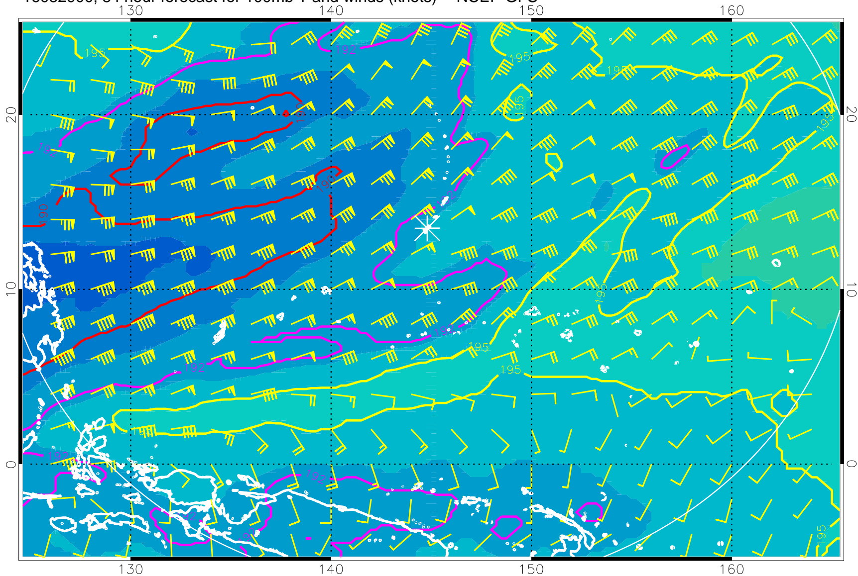
16082900, 84 hour forecast for 100mb T and winds (knots) -- NCEP GFS
