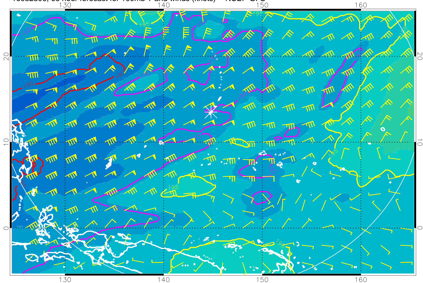
16082806, 66 hour forecast for 100mb T and winds (knots) -- NCEP GFS
