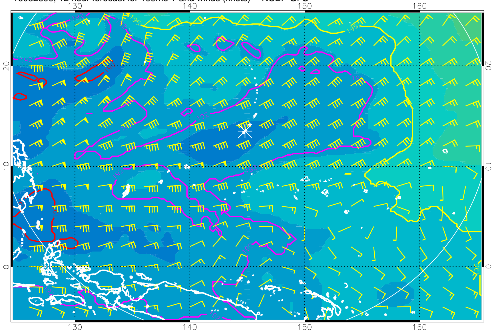
16082600, 12 hour forecast for 100mb T and winds (knots) -- NCEP GFS
