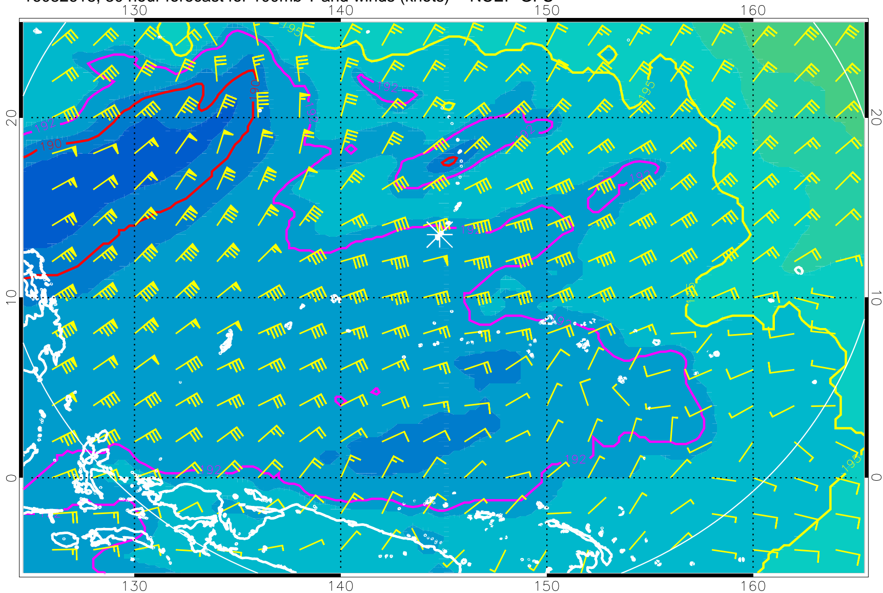
16082618, 30 hour forecast for 100mb T and winds (knots) -- NCEP GFS
