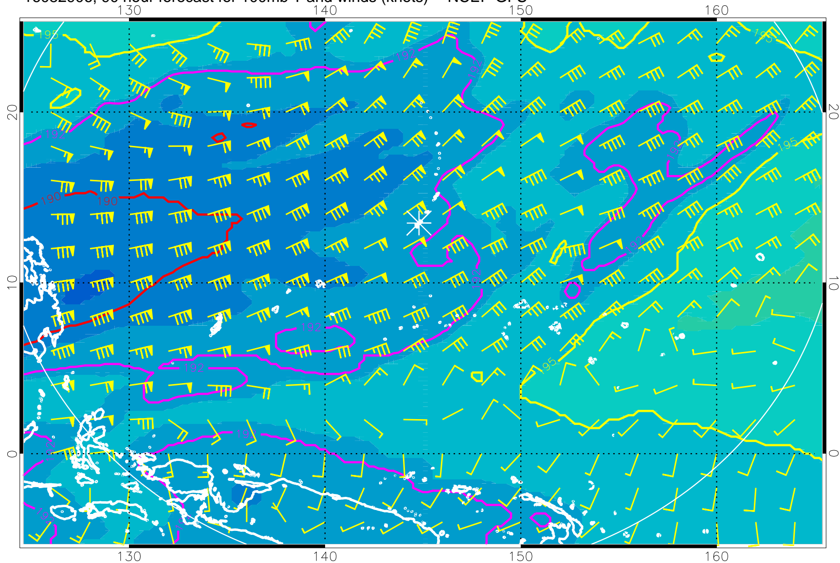
16082906, 90 hour forecast for 100mb T and winds (knots) -- NCEP GFS
