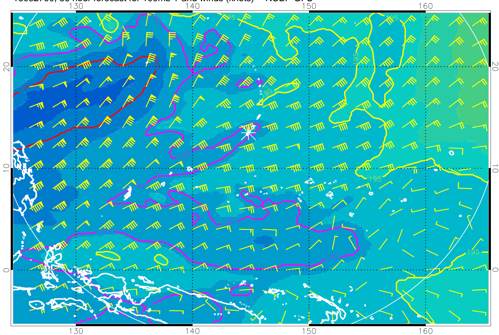
16082700, 36 hour forecast for 100mb T and winds (knots) -- NCEP GFS
