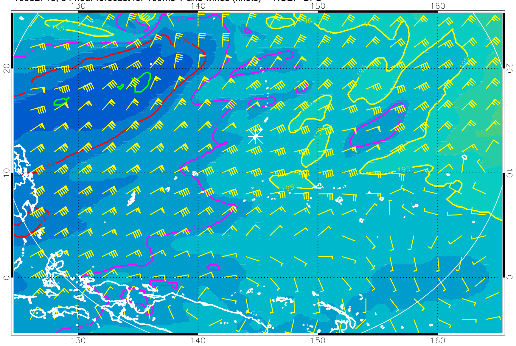
16082718, 54 hour forecast for 100mb T and winds (knots) -- NCEP GFS
