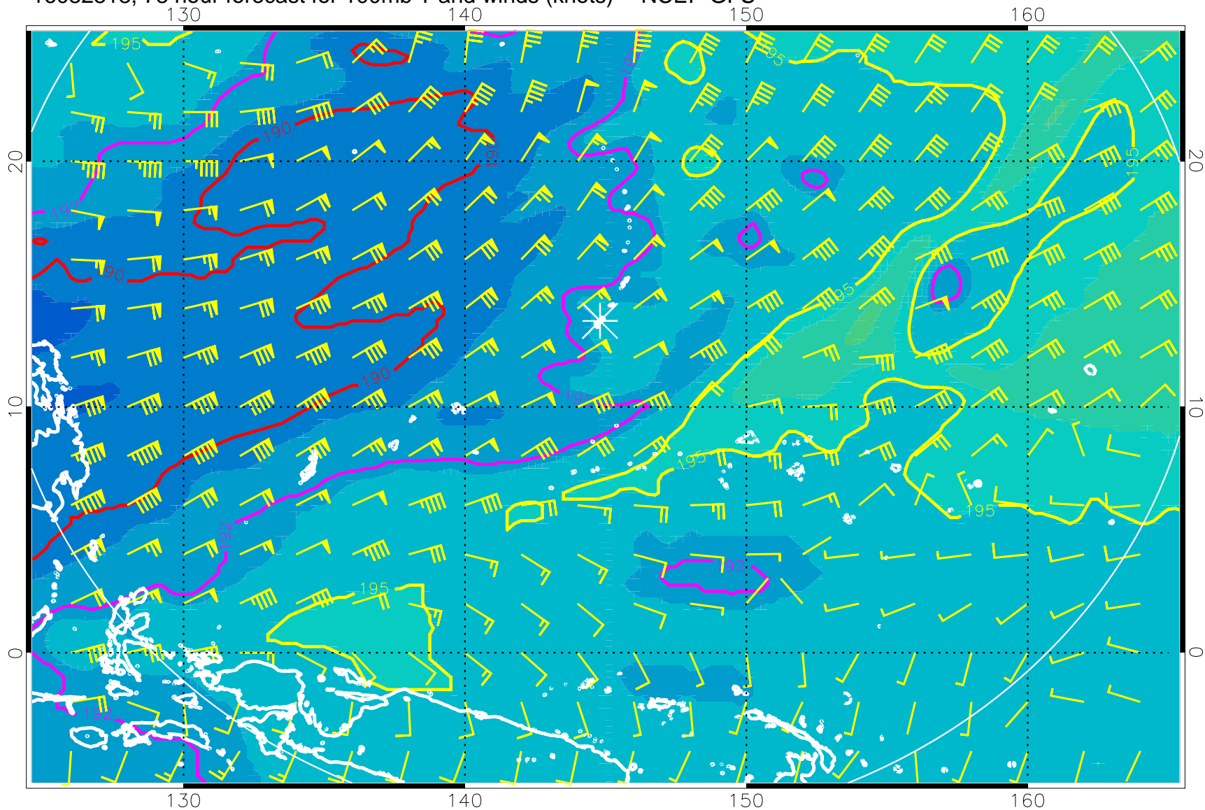
16082818, 78 hour forecast for 100mb T and winds (knots) -- NCEP GFS
