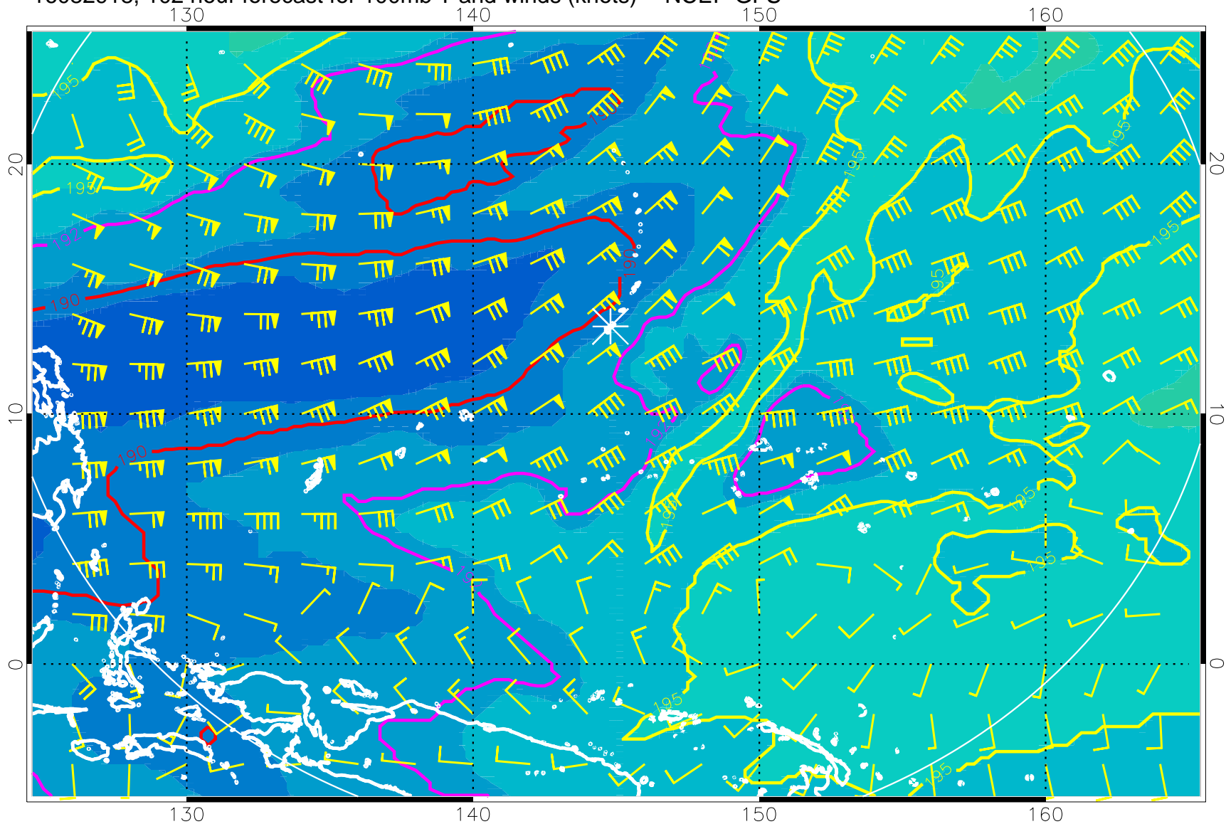
16082918, 102 hour forecast for 100mb T and winds (knots) -- NCEP GFS
