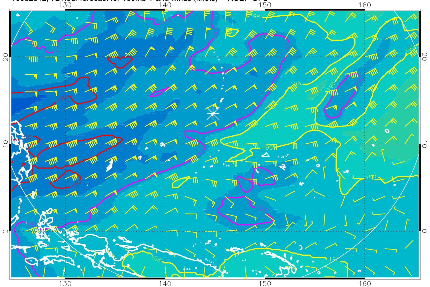
16082812, 72 hour forecast for 100mb T and winds (knots) -- NCEP GFS
