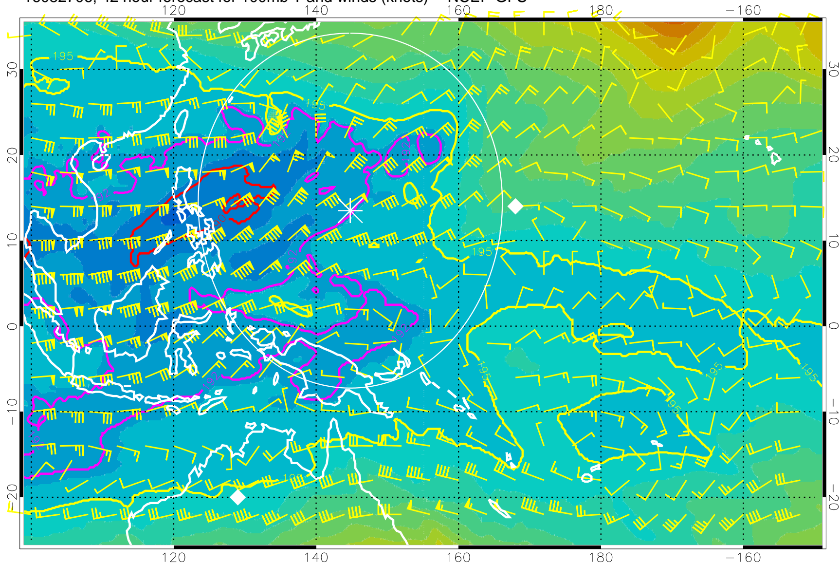
16082706, 42 hour forecast for 100mb T and winds (knots) -- NCEP GFS
