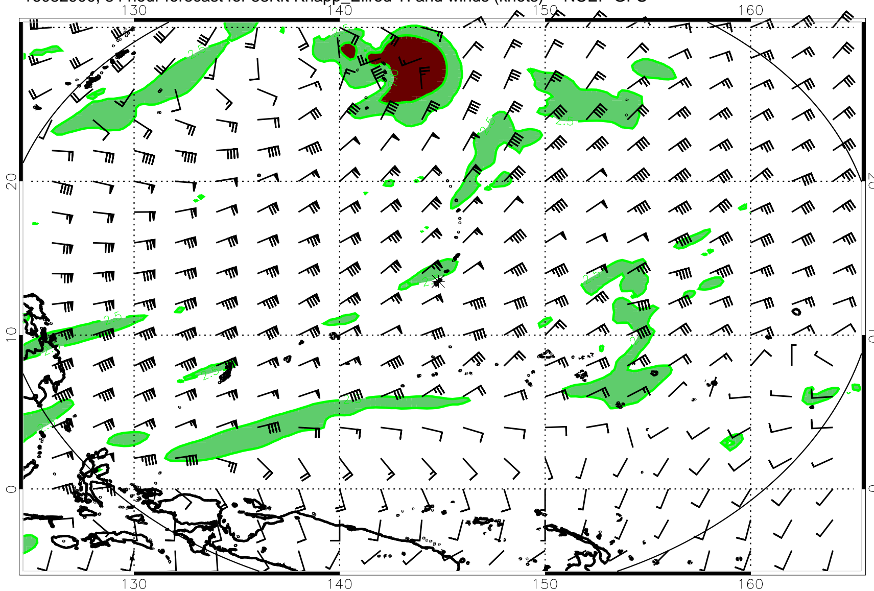
16082900, 84 hour forecast for 53Kft Knapp_Ellrod TI and winds (knots) -- NCEP GFS
