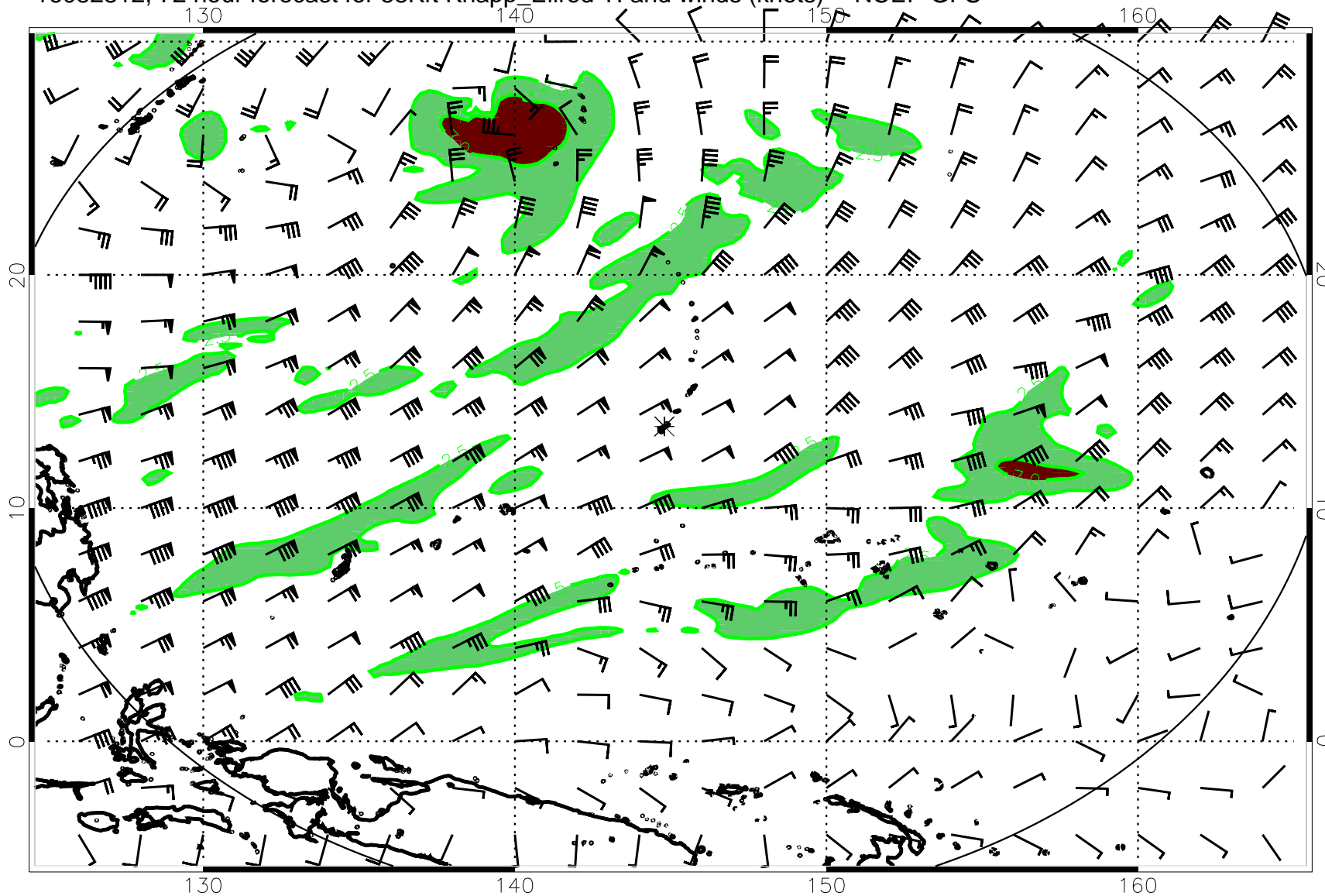
16082812, 72 hour forecast for 53Kft Knapp_Ellrod TI and winds (knots) -- NCEP GFS
