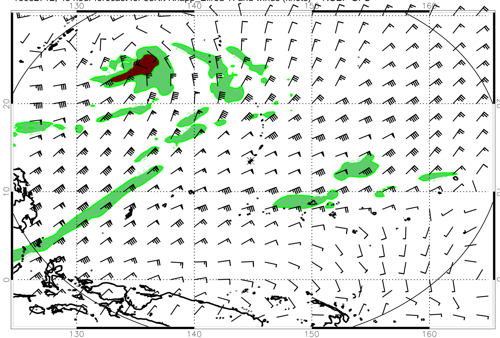
16082712, 48 hour forecast for 53Kft Knapp_Ellrod TI and winds (knots) -- NCEP GFS
