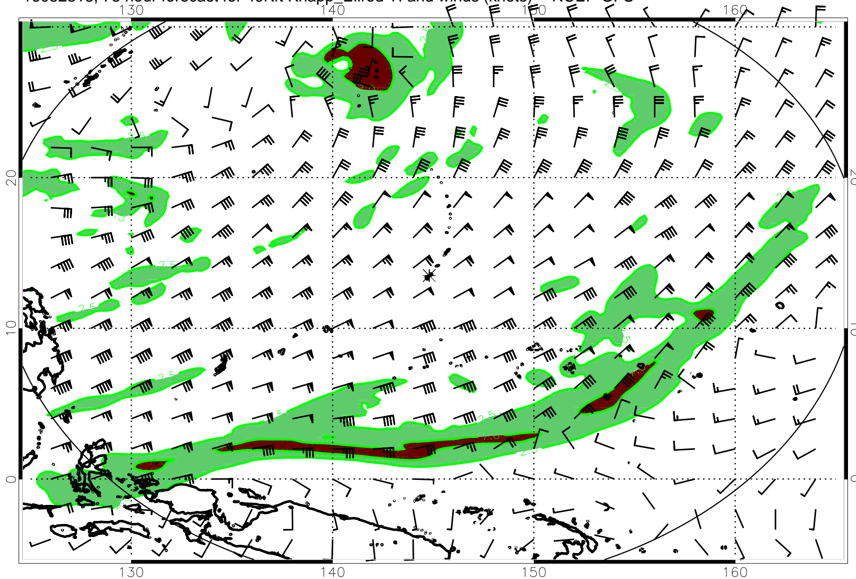
16082818, 78 hour forecast for 49Kft Knapp_Ellrod TI and winds (knots) -- NCEP GFS
