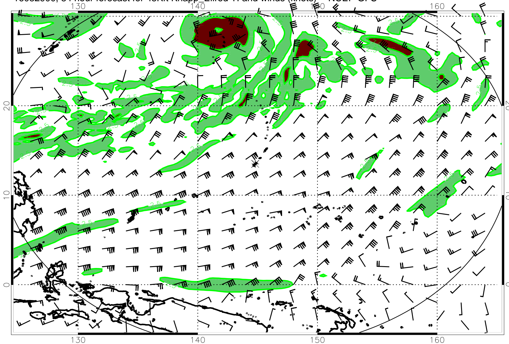
16082900, 84 hour forecast for 45Kft Knapp_Ellrod TI and winds (knots) -- NCEP GFS
