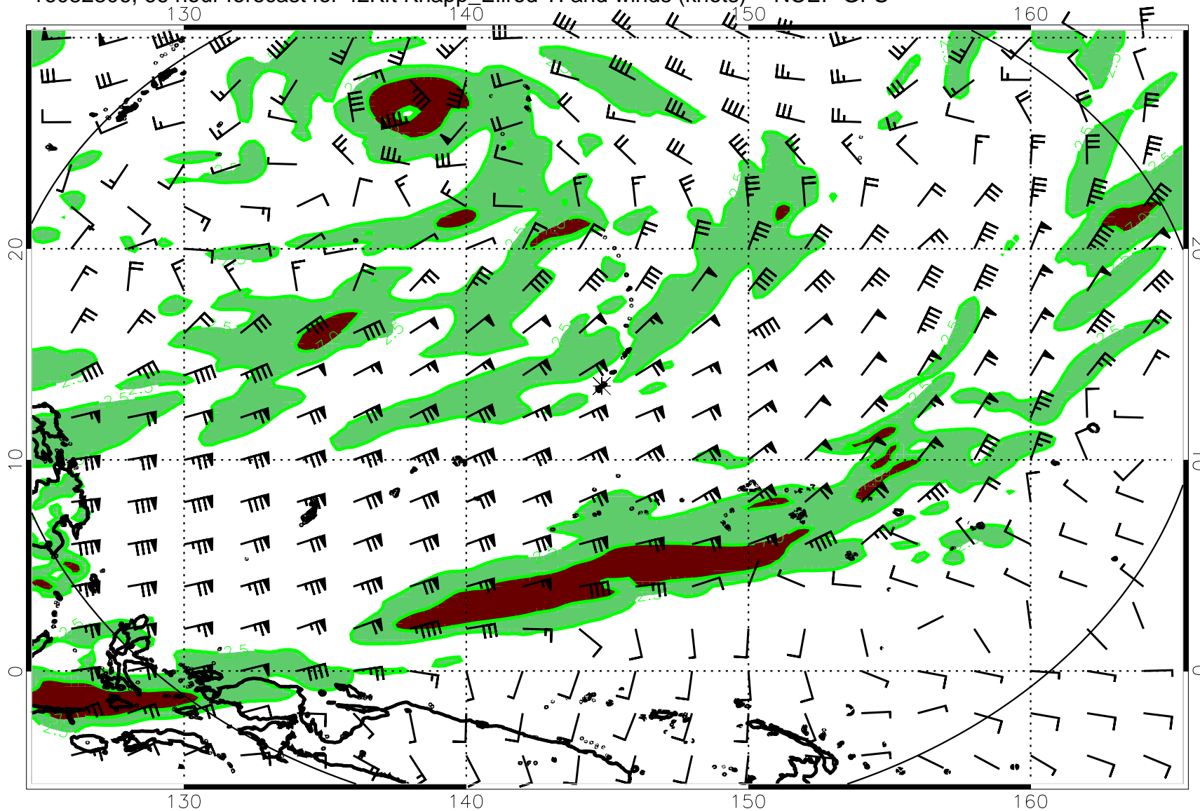
16082806, 66 hour forecast for 42Kft Knapp_Ellrod TI and winds (knots) -- NCEP GFS
