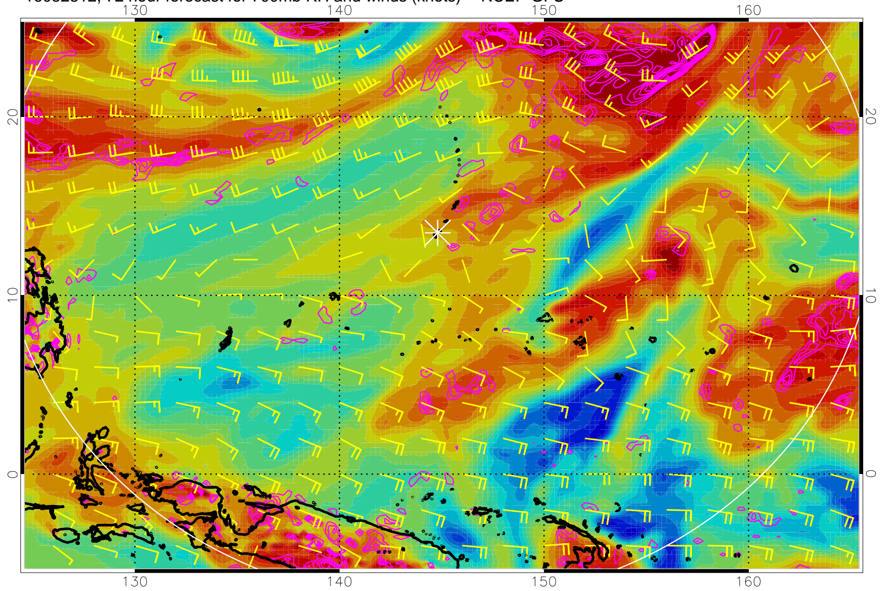
16082812, 72 hour forecast for 700mb RH and winds (knots) -- NCEP GFS
