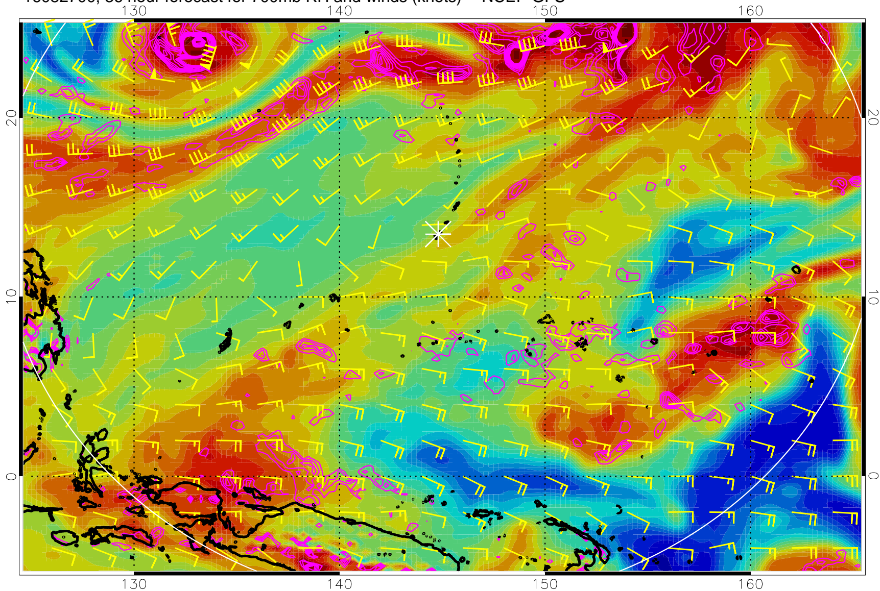
16082700, 36 hour forecast for 700mb RH and winds (knots) -- NCEP GFS
