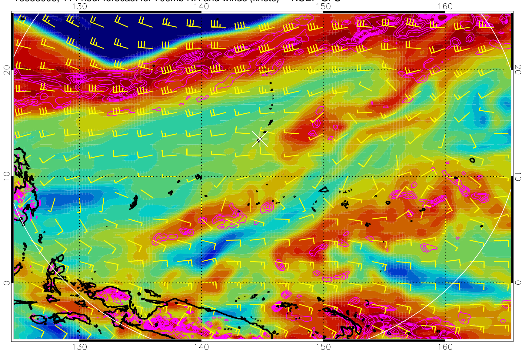
16083006, 114 hour forecast for 700mb RH and winds (knots) -- NCEP GFS
