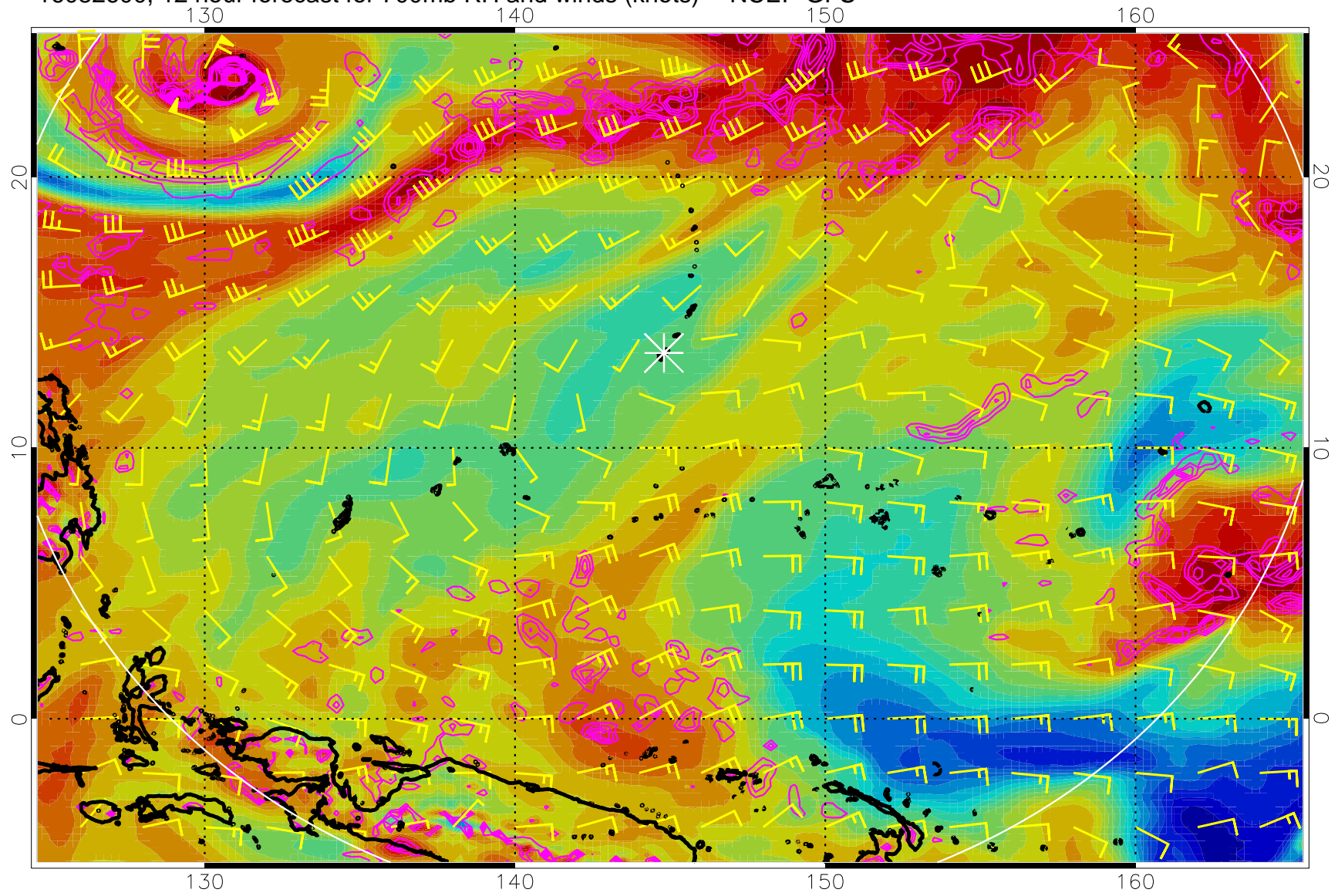
16082600, 12 hour forecast for 700mb RH and winds (knots) -- NCEP GFS
