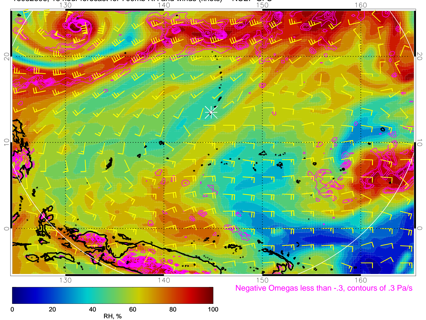
16082606, 18 hour forecast for 700mb RH and winds (knots) -- NCEP GFS
