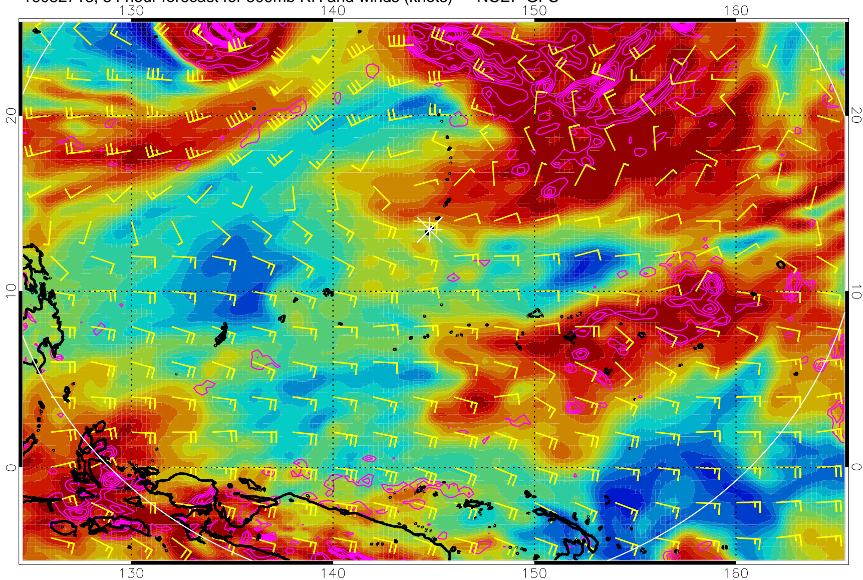
16082718, 54 hour forecast for 500mb RH and winds (knots) -- NCEP GFS
