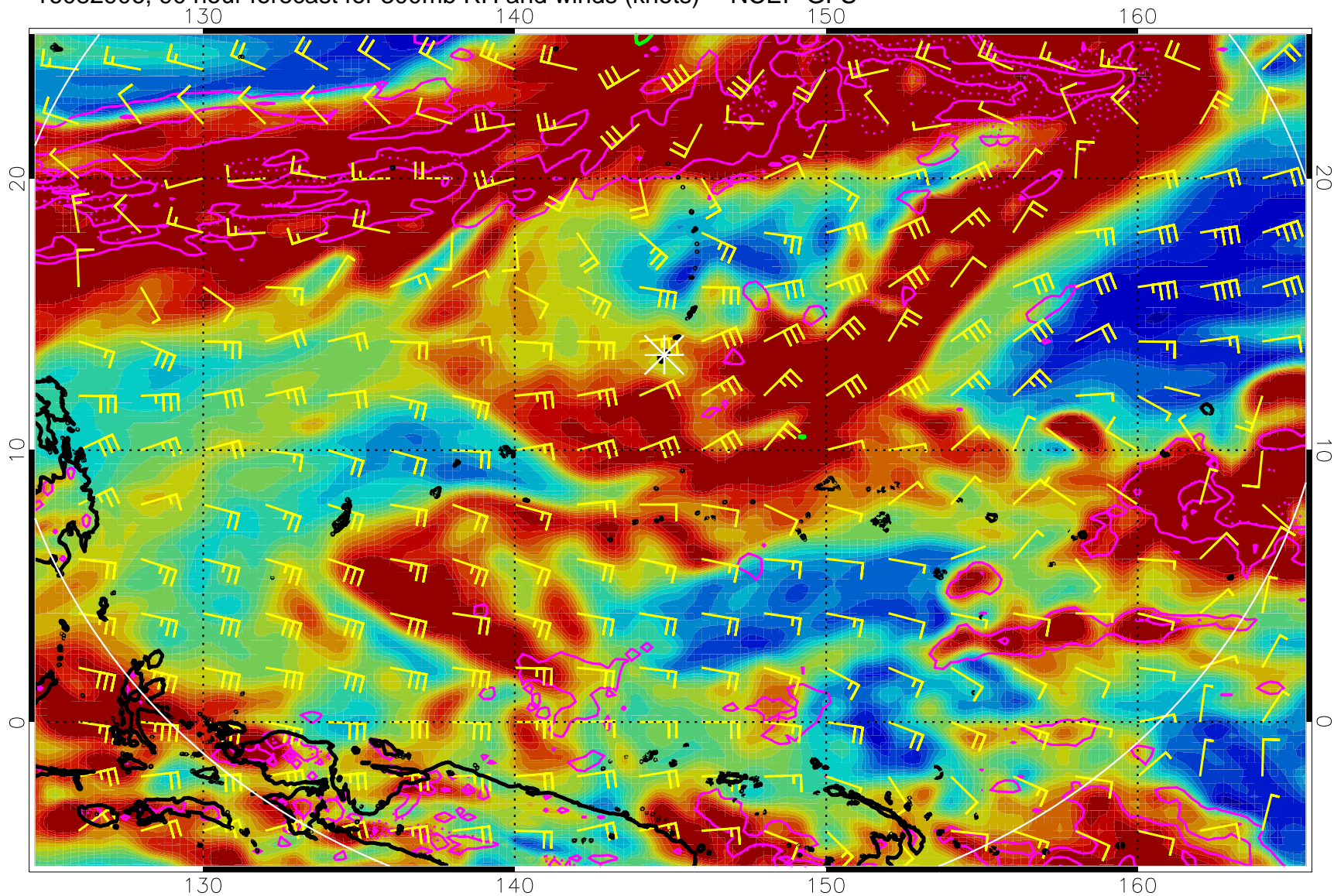
16082906, 90 hour forecast for 300mb RH and winds (knots) -- NCEP GFS
