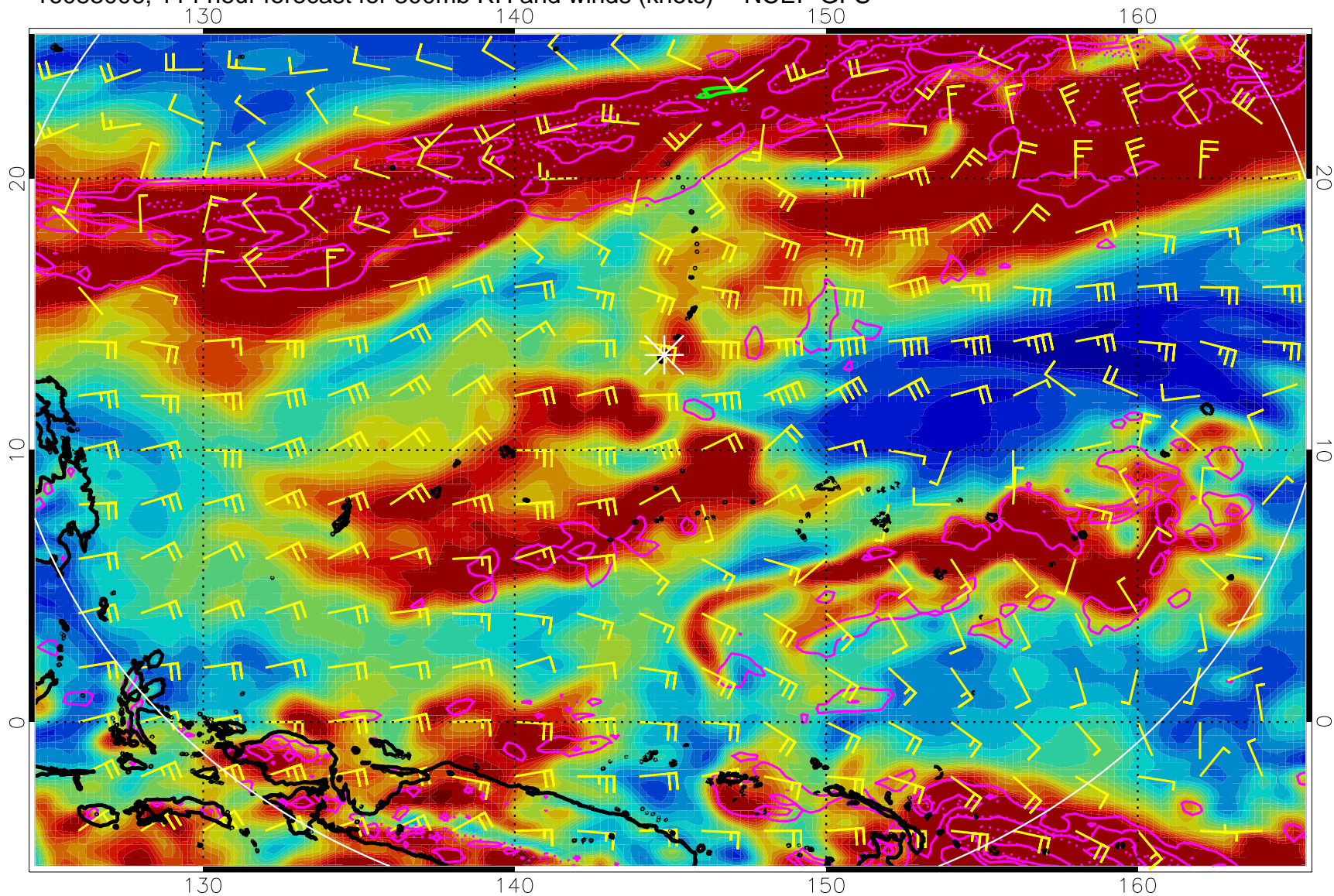
16083006, 114 hour forecast for 300mb RH and winds (knots) -- NCEP GFS
