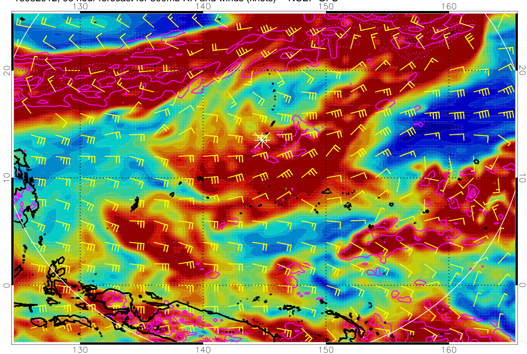
16082912, 96 hour forecast for 300mb RH and winds (knots) -- NCEP GFS
