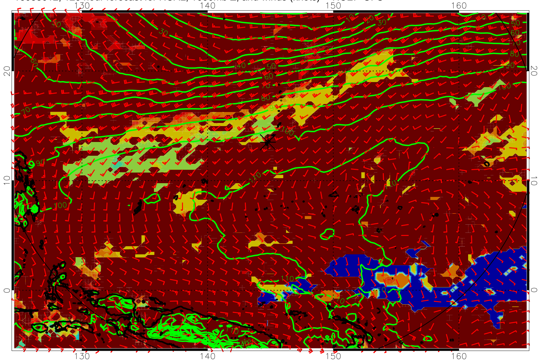
16083012, 120 hour forecast for HCAL, 1000mb Z, and winds (knots) -- NCEP GFS
