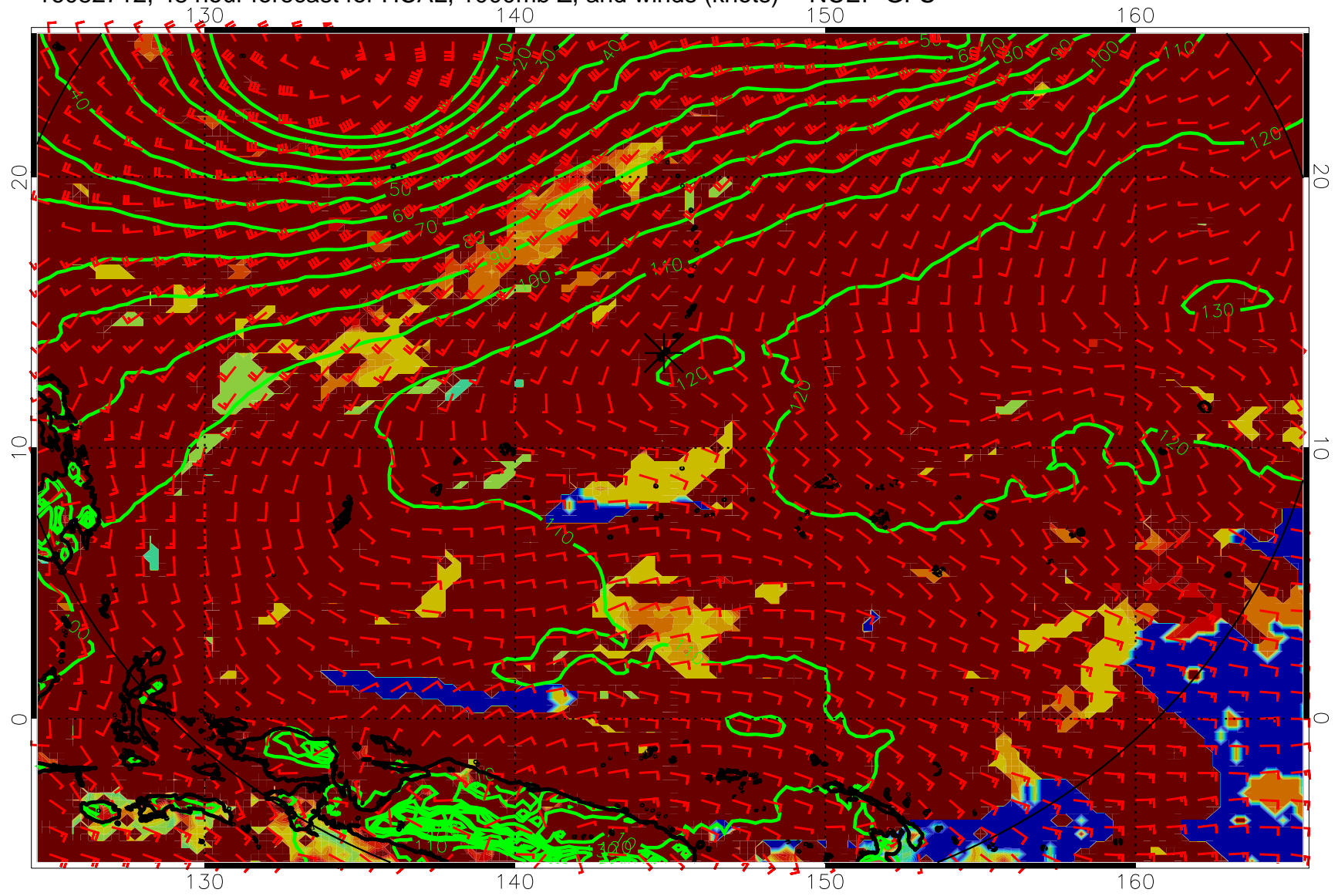
16082712, 48 hour forecast for HCAL, 1000mb Z, and winds (knots) -- NCEP GFS
