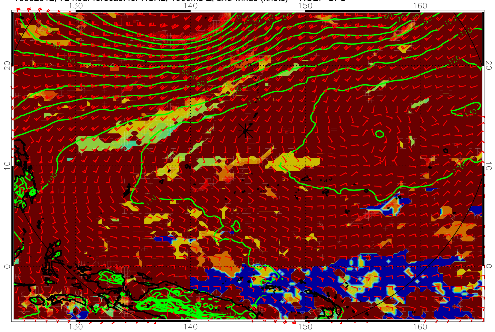
16082812, 72 hour forecast for HCAL, 1000mb Z, and winds (knots) -- NCEP GFS
