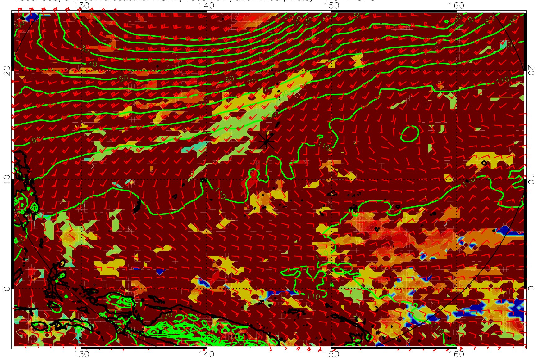
16082900, 84 hour forecast for HCAL, 1000mb Z, and winds (knots) -- NCEP GFS
