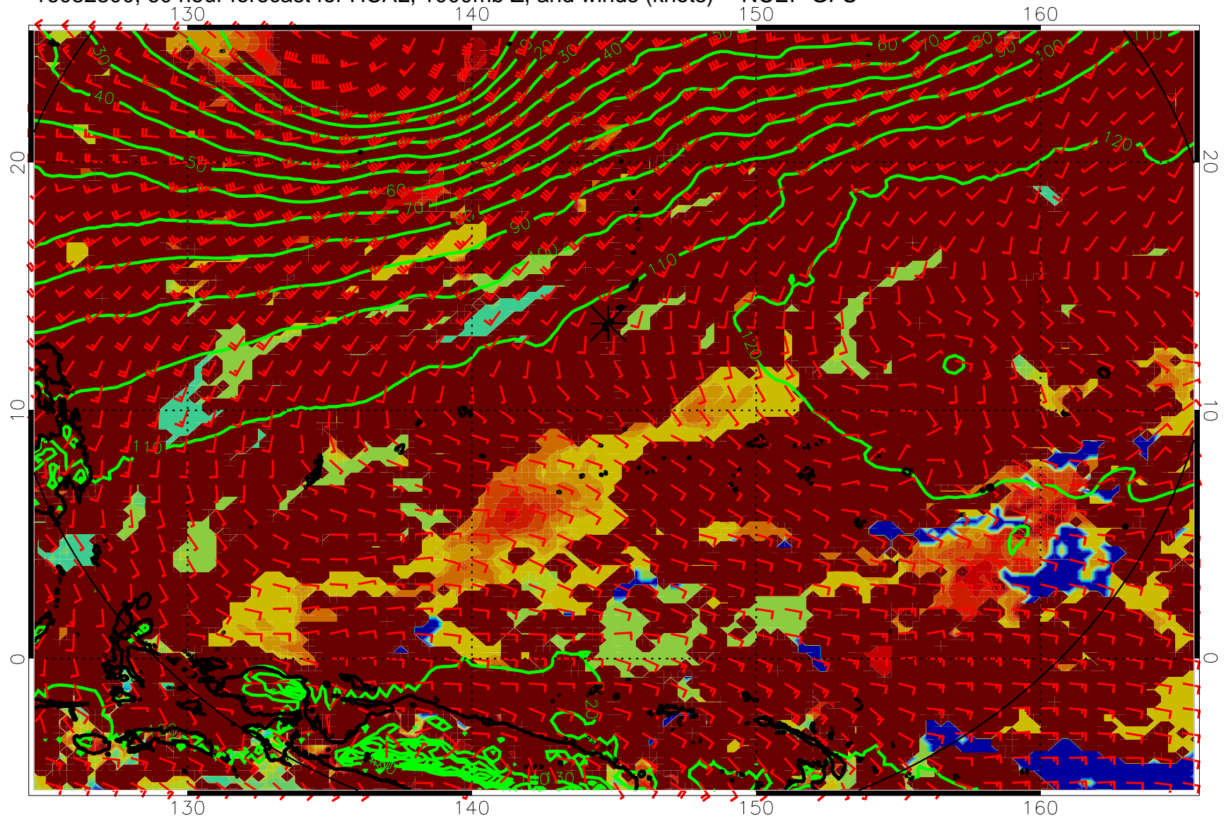
16082800, 60 hour forecast for HCAL, 1000mb Z, and winds (knots) -- NCEP GFS
