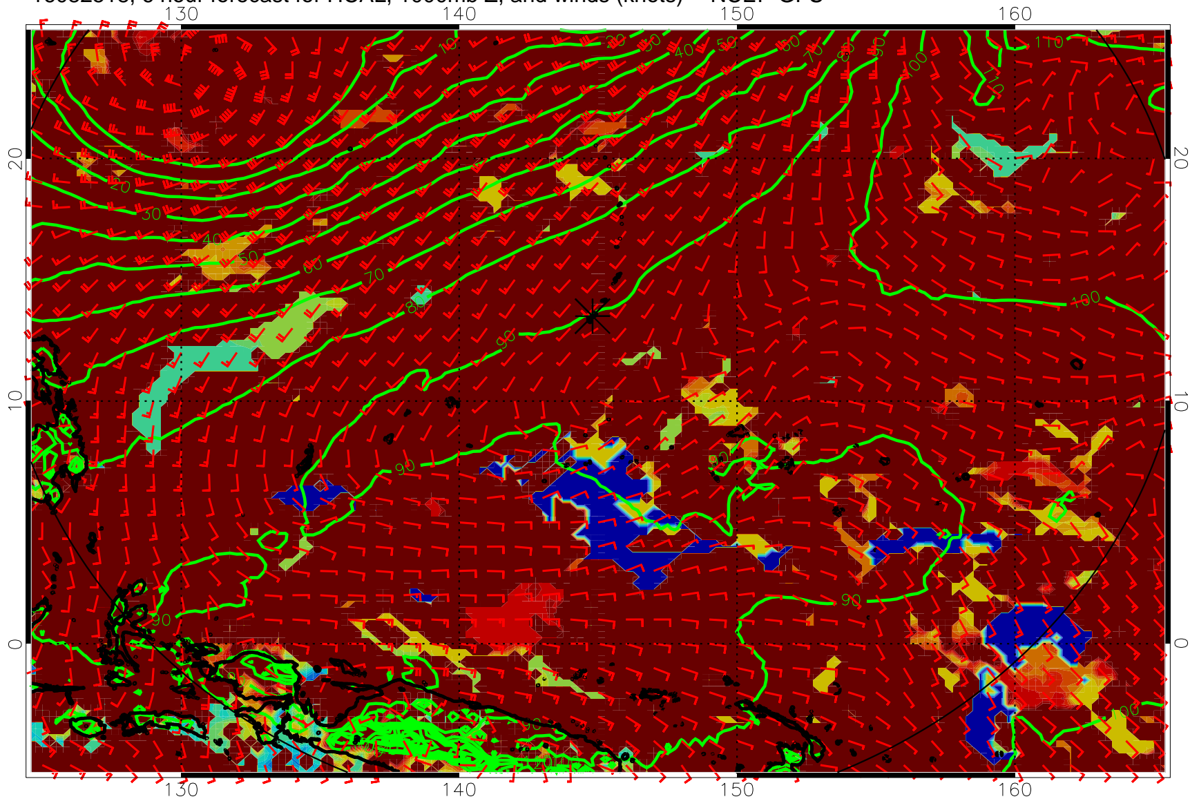
16082518, 6 hour forecast for HCAL, 1000mb Z, and winds (knots) -- NCEP GFS
