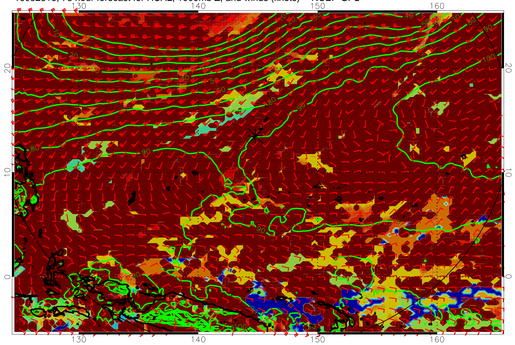
16082818, 78 hour forecast for HCAL, 1000mb Z, and winds (knots) -- NCEP GFS
