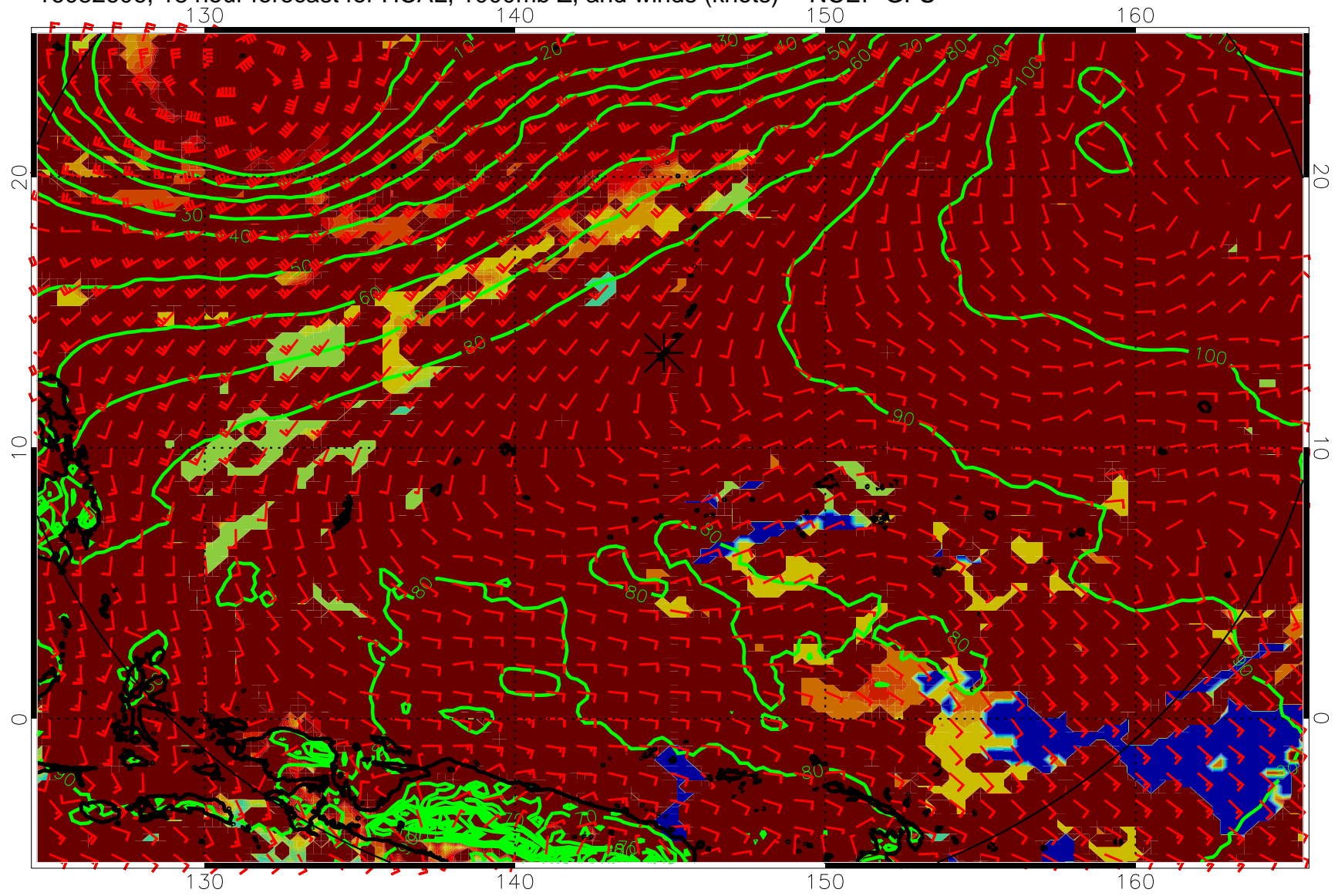
16082606, 18 hour forecast for HCAL, 1000mb Z, and winds (knots) -- NCEP GFS
