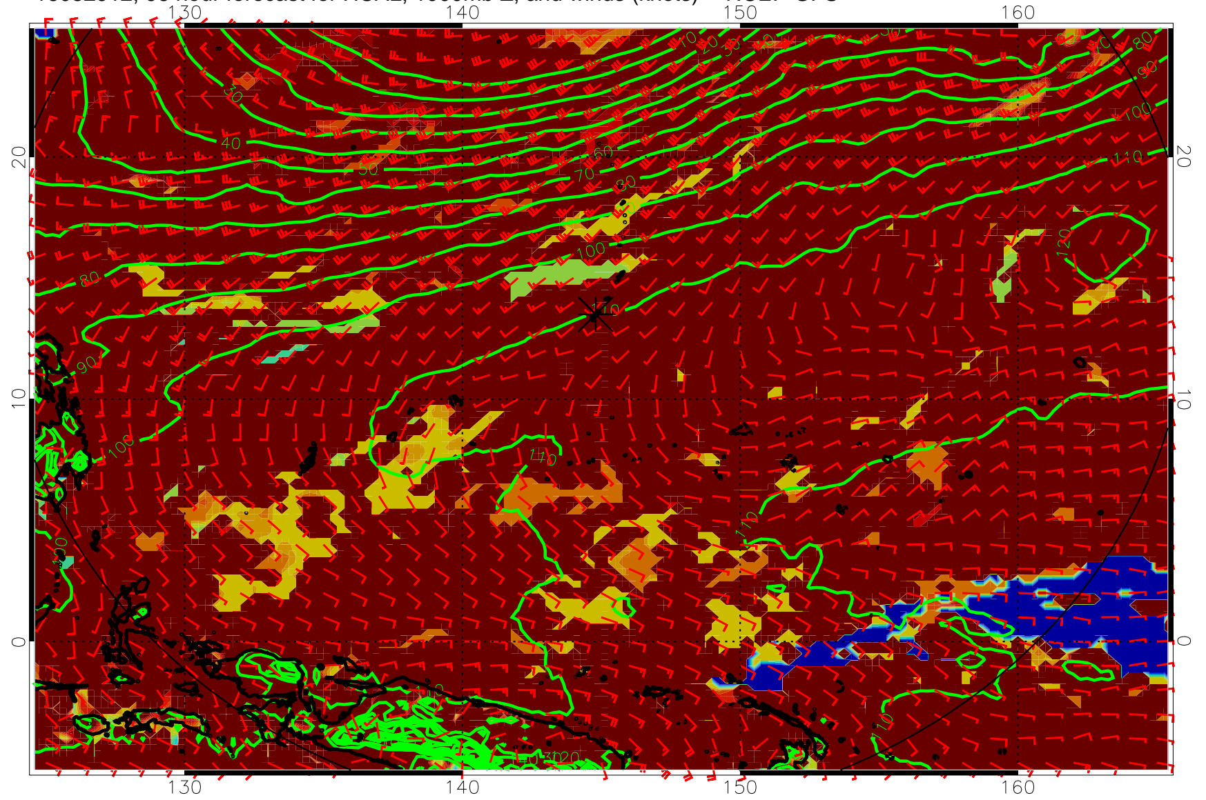
16082912, 96 hour forecast for HCAL, 1000mb Z, and winds (knots) -- NCEP GFS
