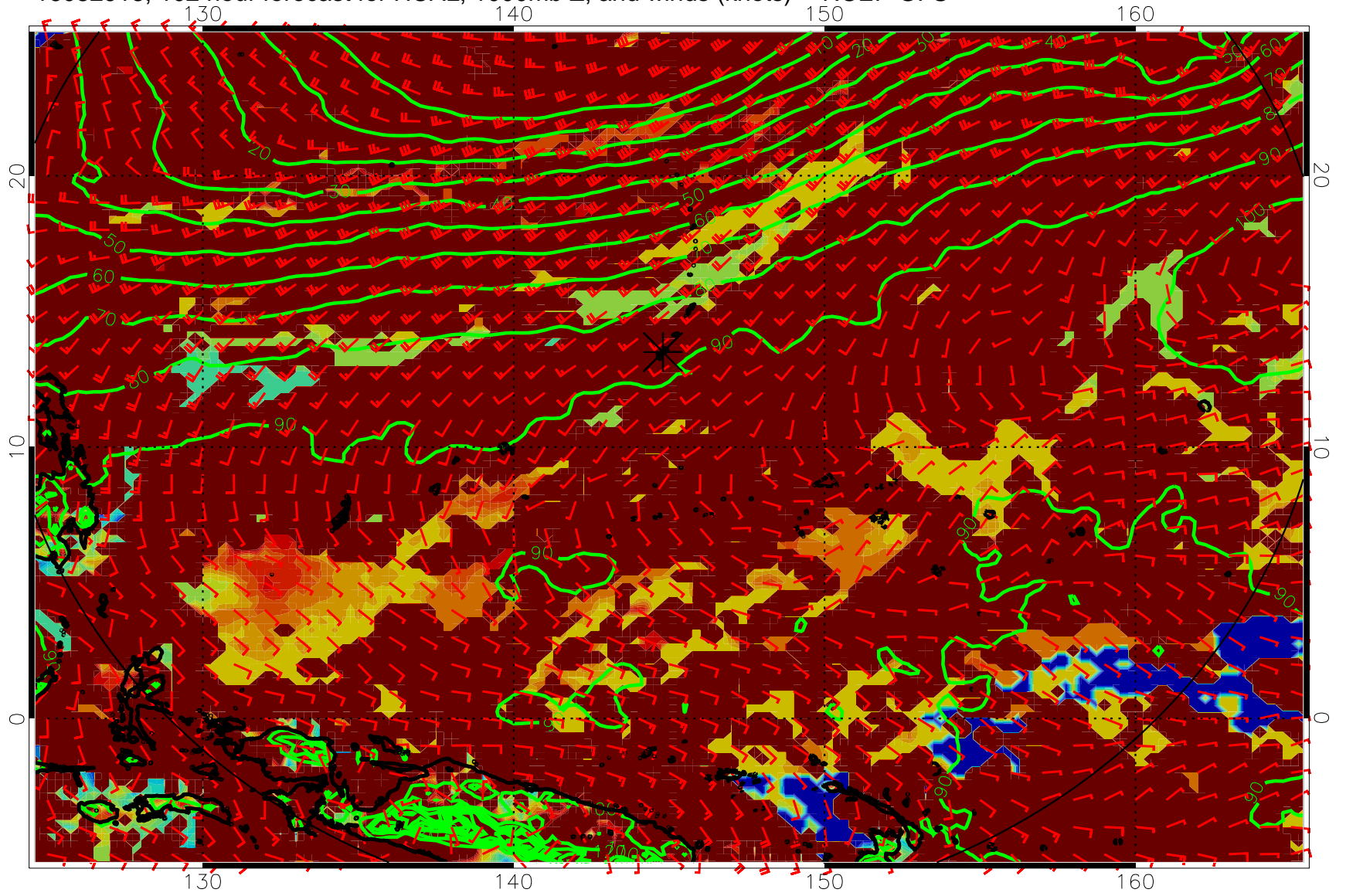
16082918, 102 hour forecast for HCAL, 1000mb Z, and winds (knots) -- NCEP GFS
