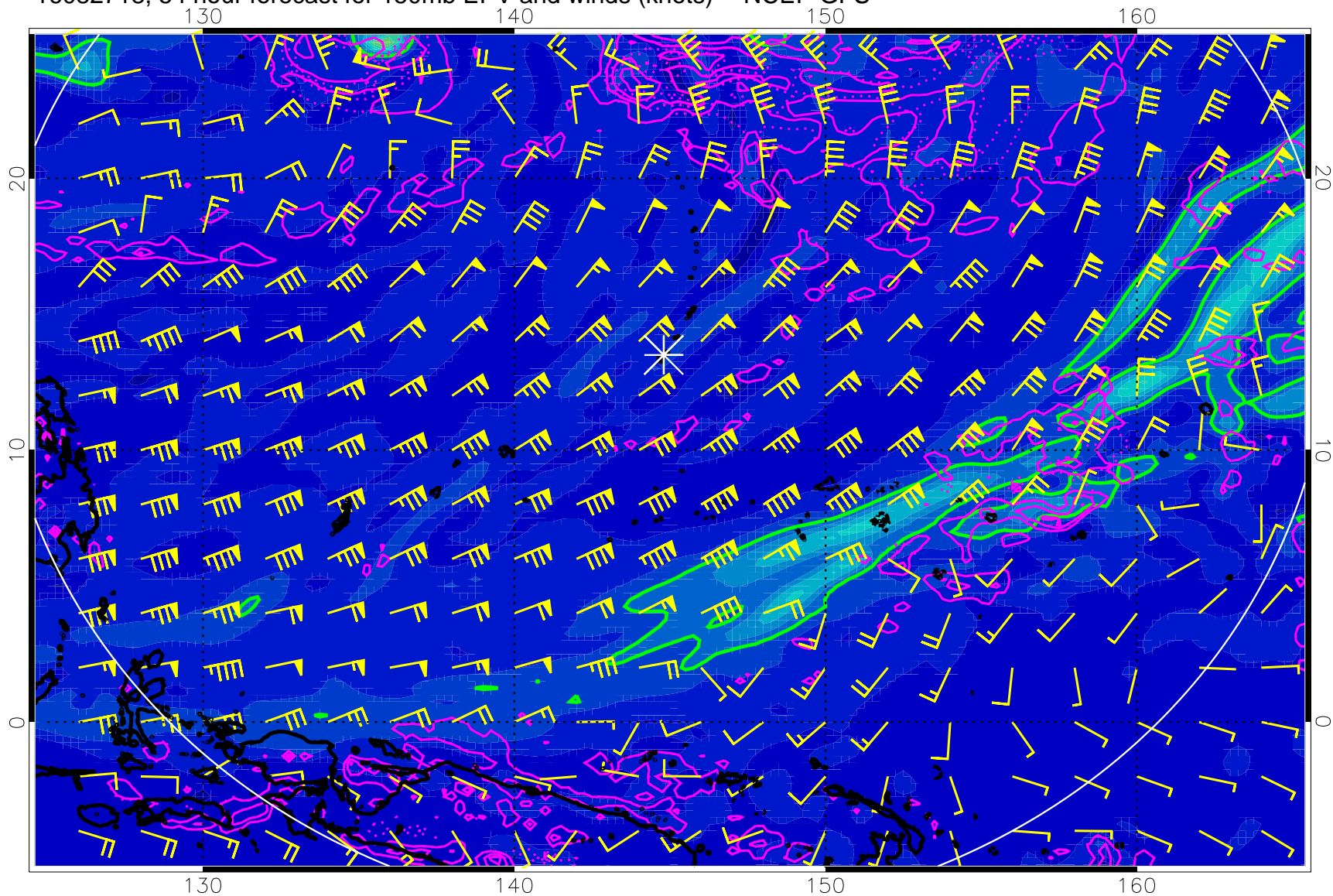
16082718, 54 hour forecast for 150mb EPV and winds (knots) -- NCEP GFS
