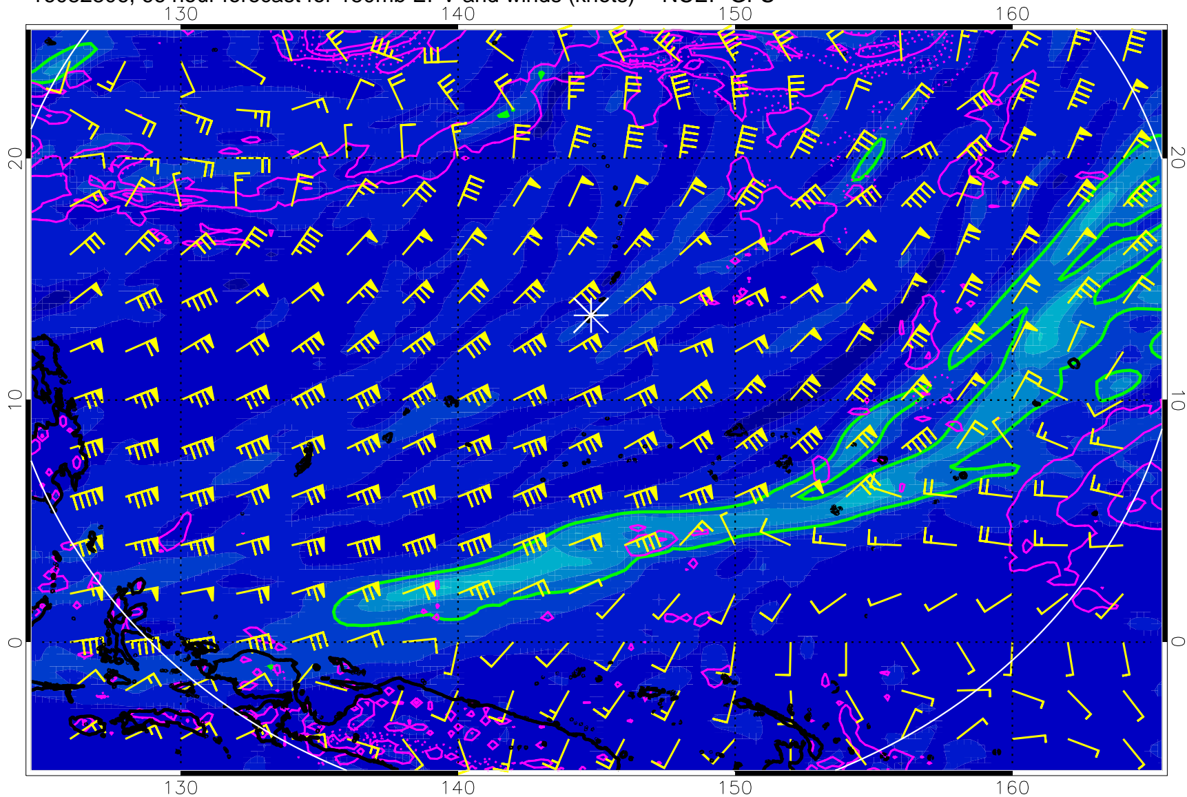
16082806, 66 hour forecast for 150mb EPV and winds (knots) -- NCEP GFS
