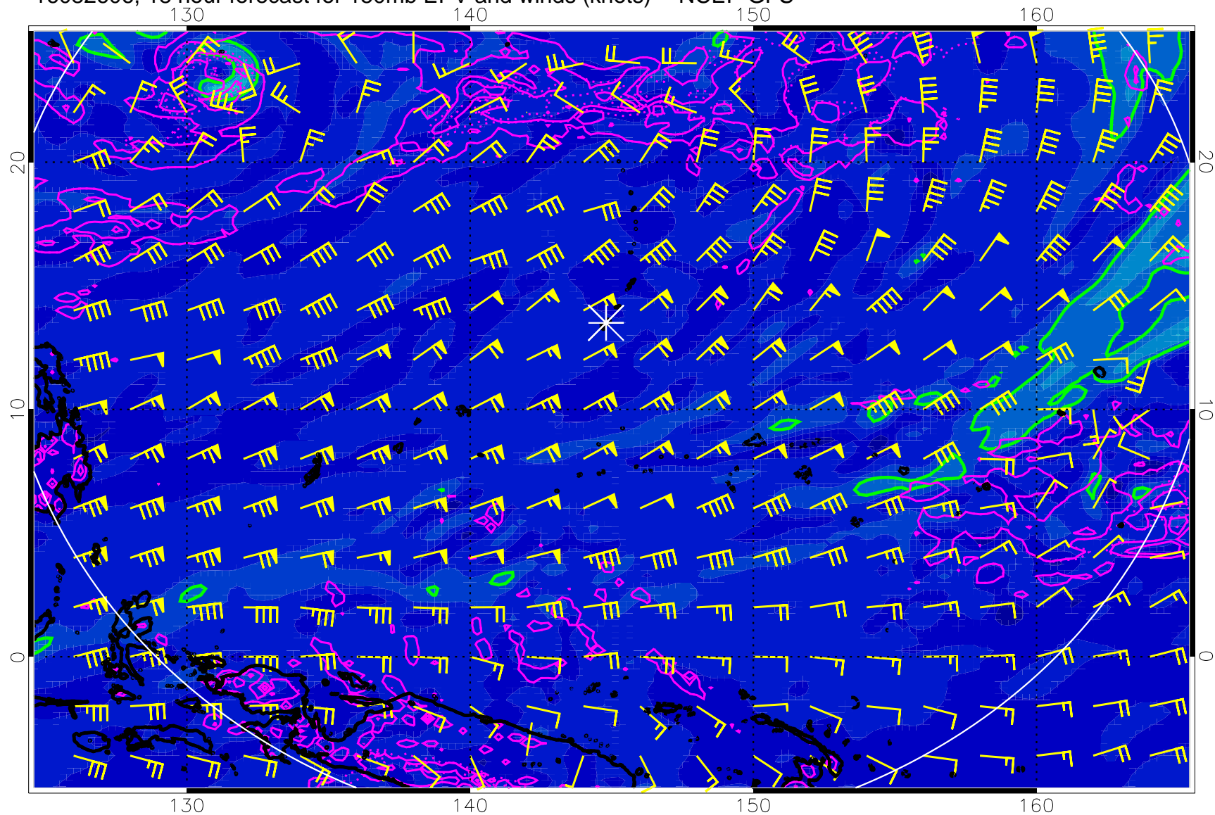
16082606, 18 hour forecast for 150mb EPV and winds (knots) -- NCEP GFS
