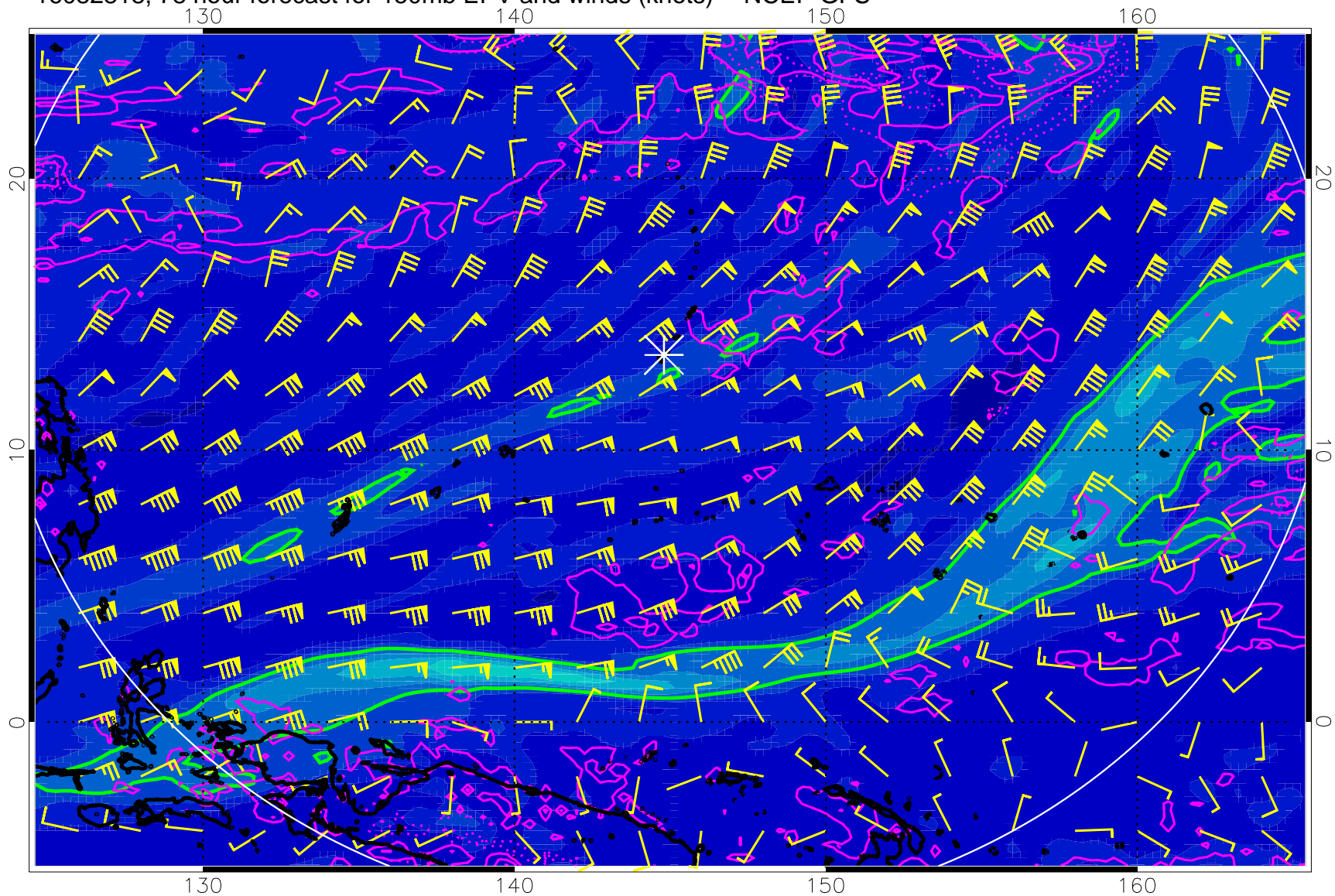
16082818, 78 hour forecast for 150mb EPV and winds (knots) -- NCEP GFS
