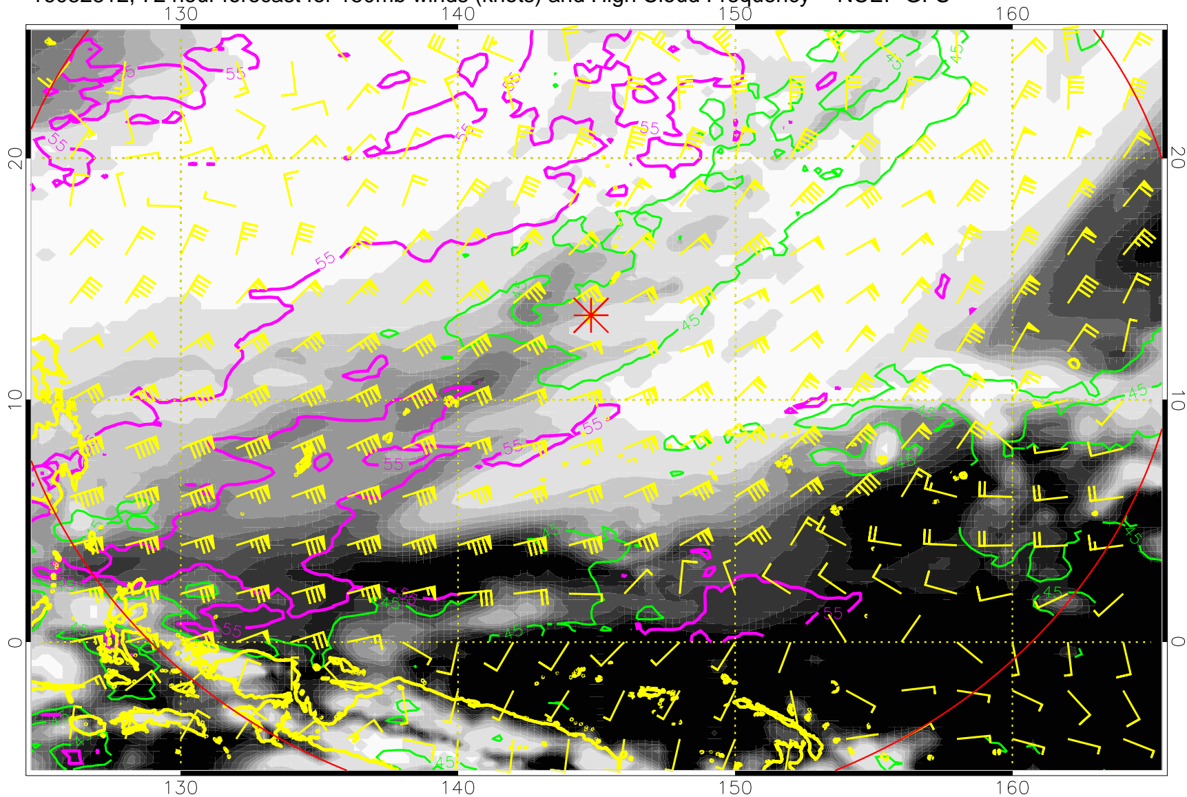
16082812, 72 hour forecast for 150mb winds (knots) and High Cloud Frequency -- NCEP GFS
