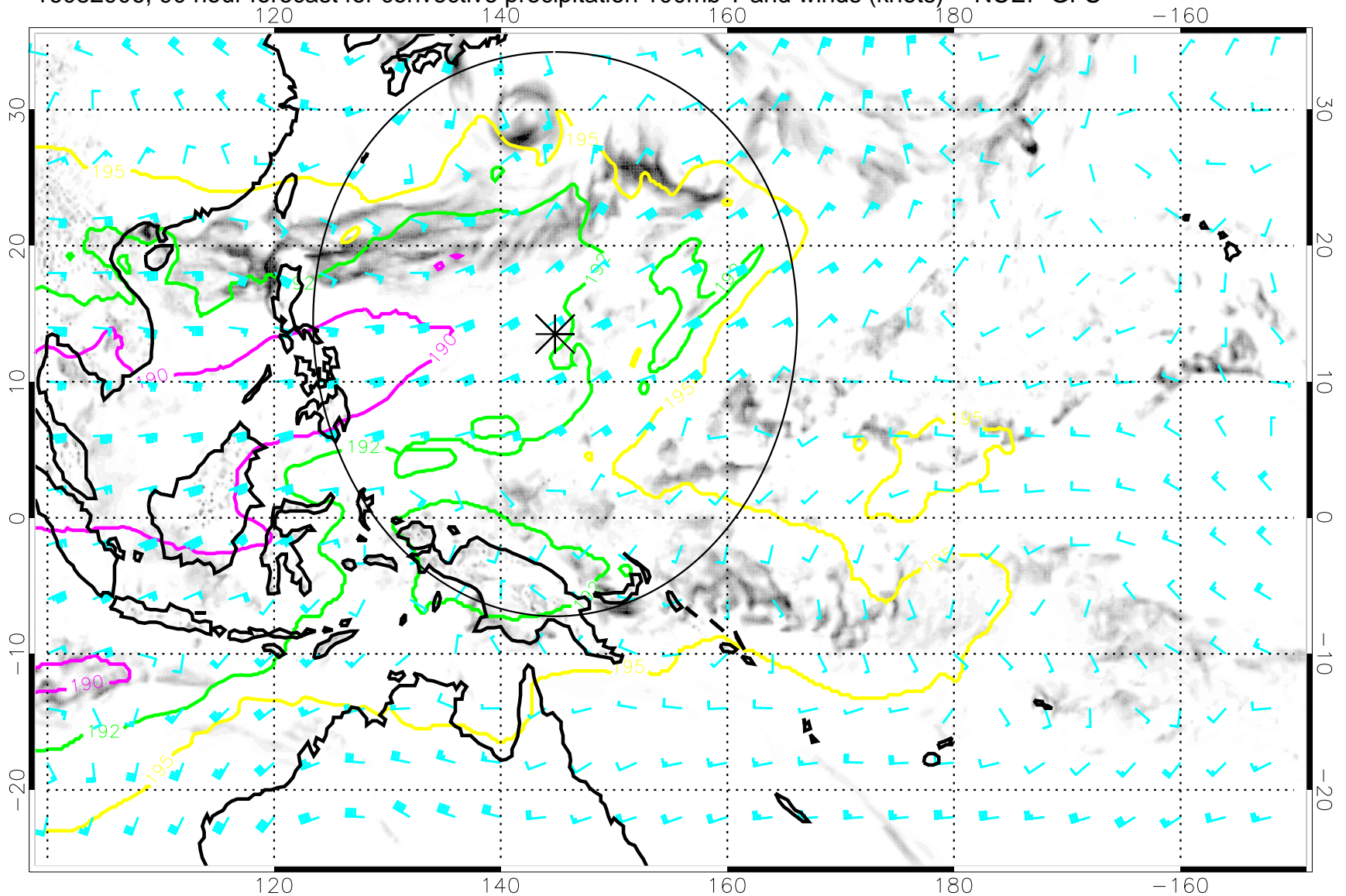
16082906, 90 hour forecast for convective precipitation 100mb T and winds (knots) -- NCEP GFS
