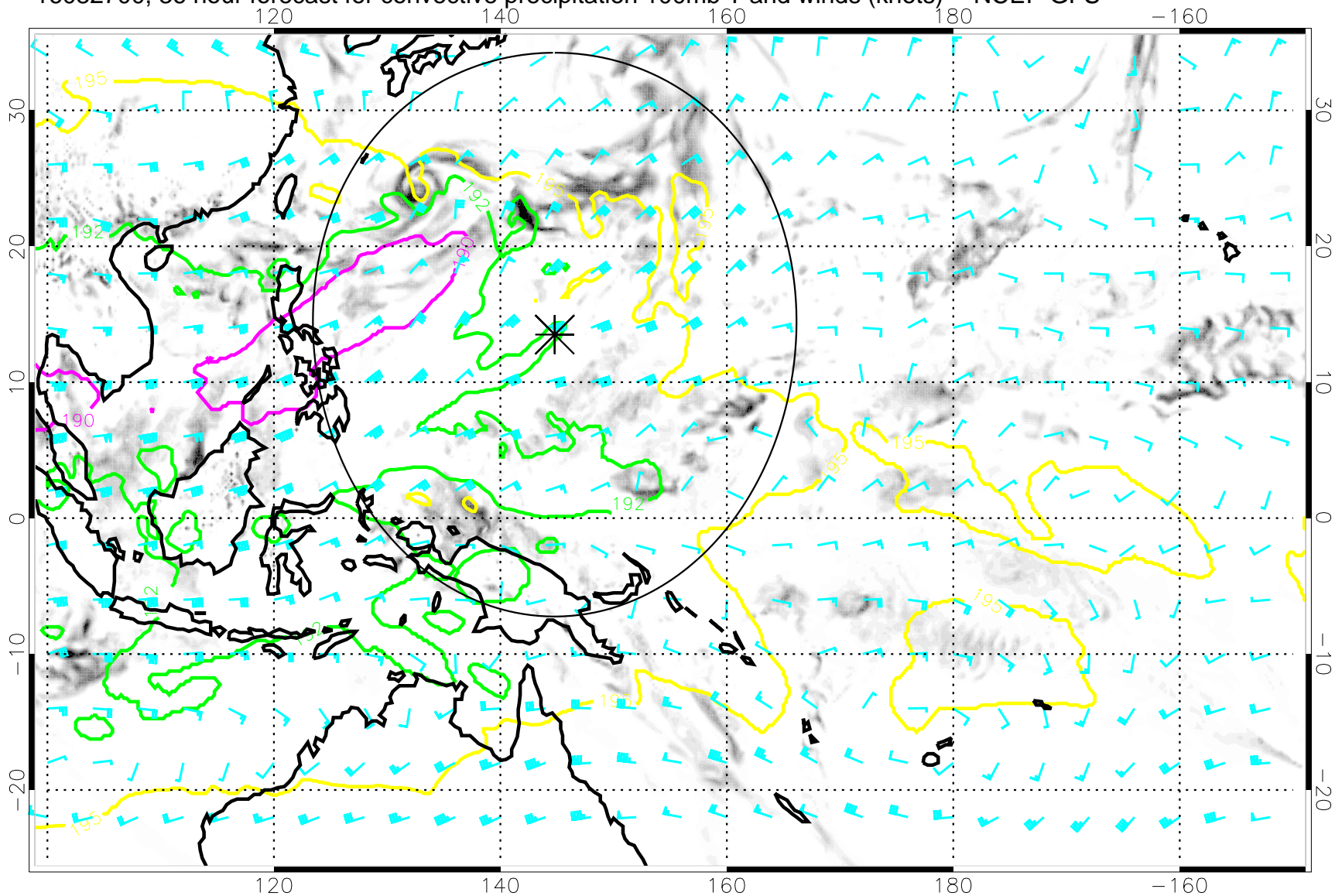
16082700, 36 hour forecast for convective precipitation 100mb T and winds (knots) -- NCEP GFS
