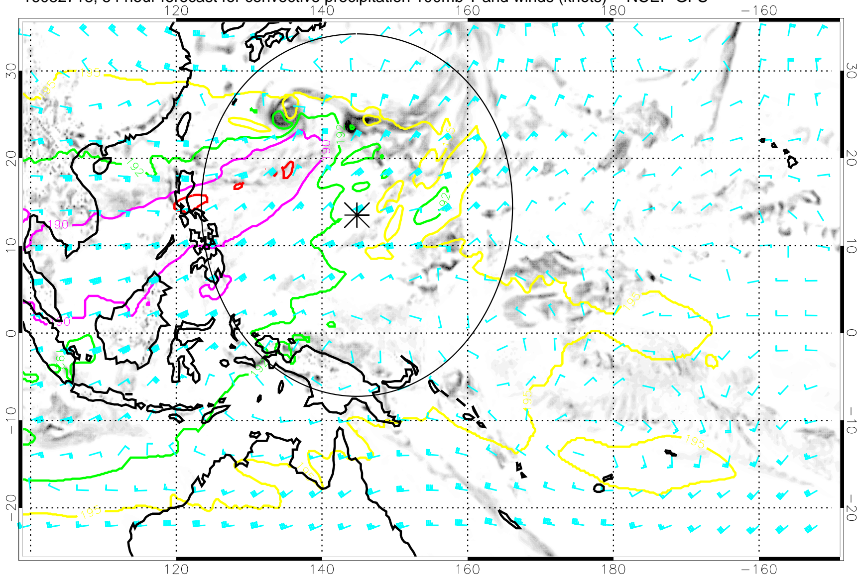
16082718, 54 hour forecast for convective precipitation 100mb T and winds (knots) -- NCEP GFS
